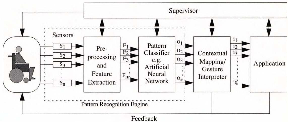
Figure 2.4 Example architecture for gesture recognition system
