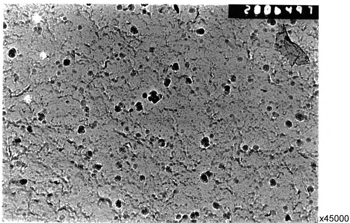
Figure 6.32 Transmission electron micrograph (replica), showing copper precipitation in the normalised and fully-aged (NT550) 1.26% Cu-steel.
