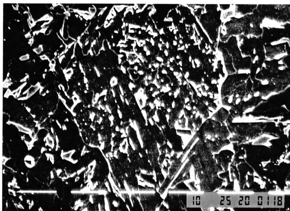
Figure 6.26 Scanning electron micrograph of the as-quenched (Q) 1.26% Cu-steel, showing the arrangement of ferrite laths and (MA) particles.
