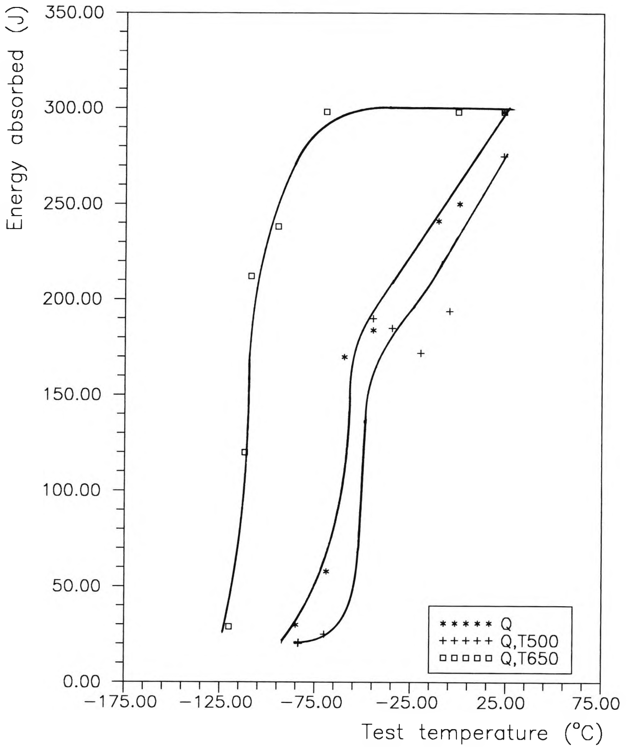
Figure 6.3 Impact transition temperature curves for quenched and aged 1P140M steel.
