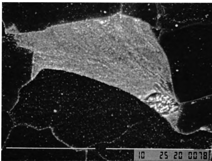
Figure 6.16 Scanning electron micrograph of the as-normalised 1.26% steel, showing a coarse martensite colony.
