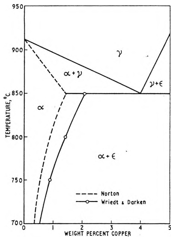
Figure 2.17 Fe-rich side of the Fe-Cu diagram (based on data from ref.[82]).
