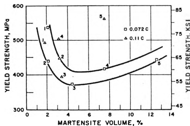
Figure 2.12 Variation in yield strength with increasing martensite volume fraction [41].
