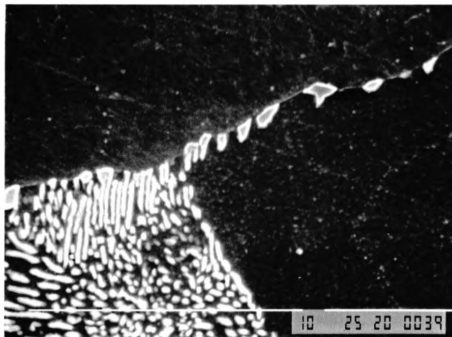
Figure 5.10 (b) Scanning electron micrograph of NT650, copper-free steel, showing spheroidised pearlite and carbides.
