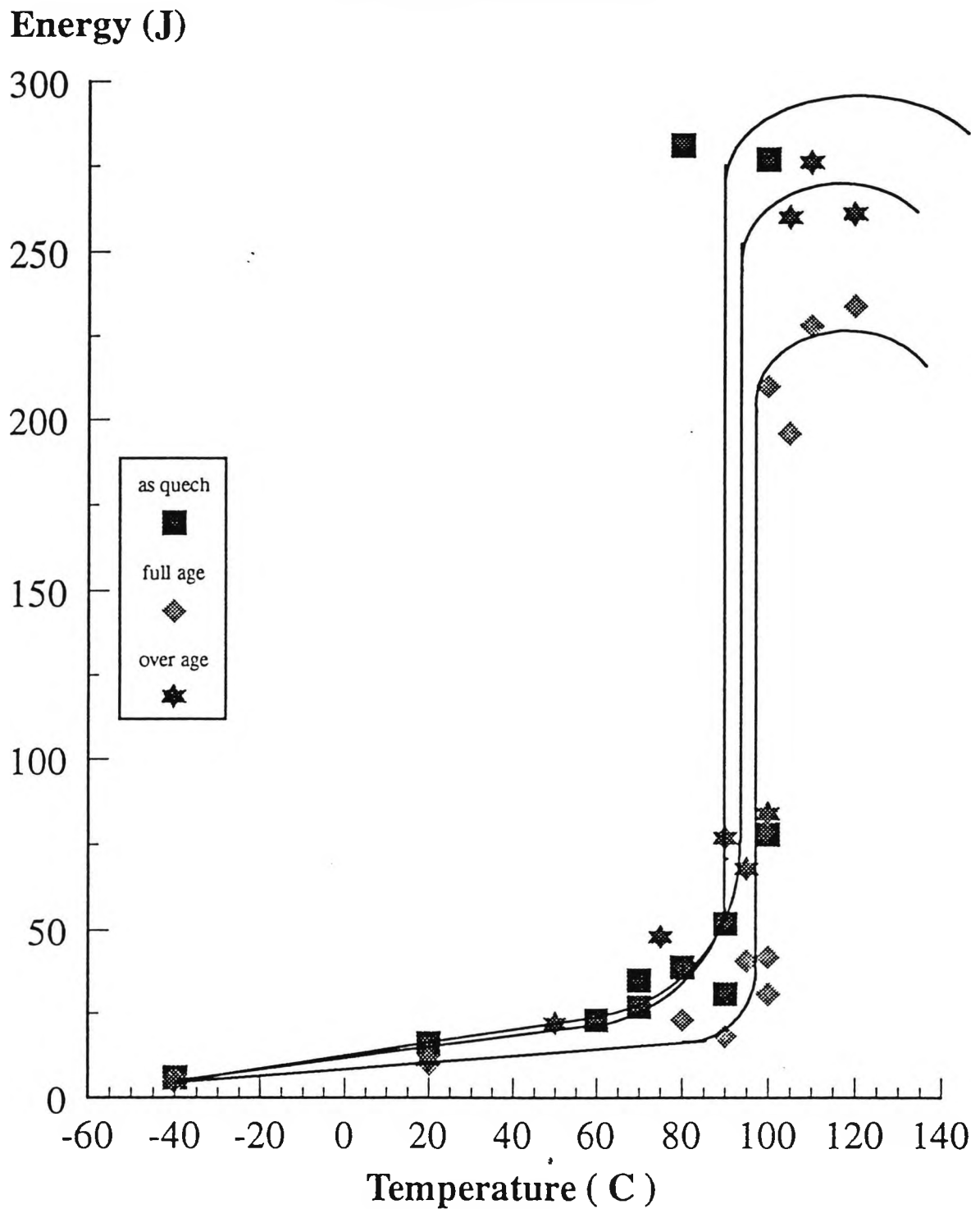
Figure 4.12 Impact transition temperature curves, for quenched and aged, steel 4P28H (the tests have been carried out at British Steel [96]).
