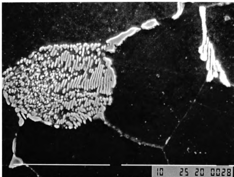
Figure 5.10 (a) Scanning electron micrograph of NT650, copper-free steel, showing spheroidised pearlite and carbides.
