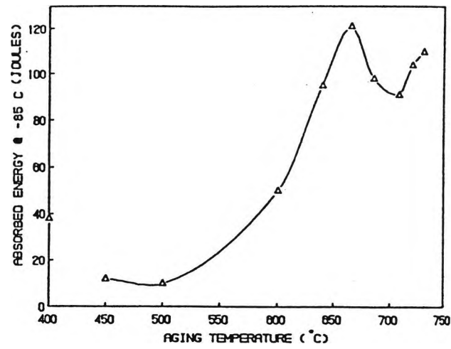
Figure 2.30 The effect of tempering (1 h) of (a) the yield strength and (b) -84^{\circ}\text{C} impact strength, of a water-quenched (1 h at 900^{\circ}\text{C} ) HSLA-100 steel plate (19 mm in thickness) [39].
