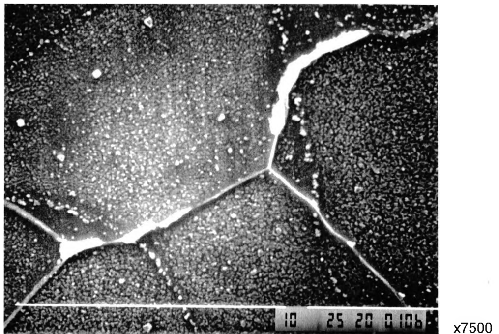
Figure 5.14 Scanning electron micrograph, showing grain boundary carbides of as "normalised", 1.22% Cu steel.
