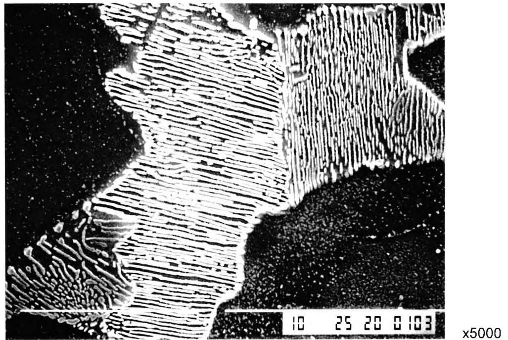
Figure 5.15 Scanning electron micrograph, showing pearlite colonies of the as “normalised”, 1.22% Cu steel.
