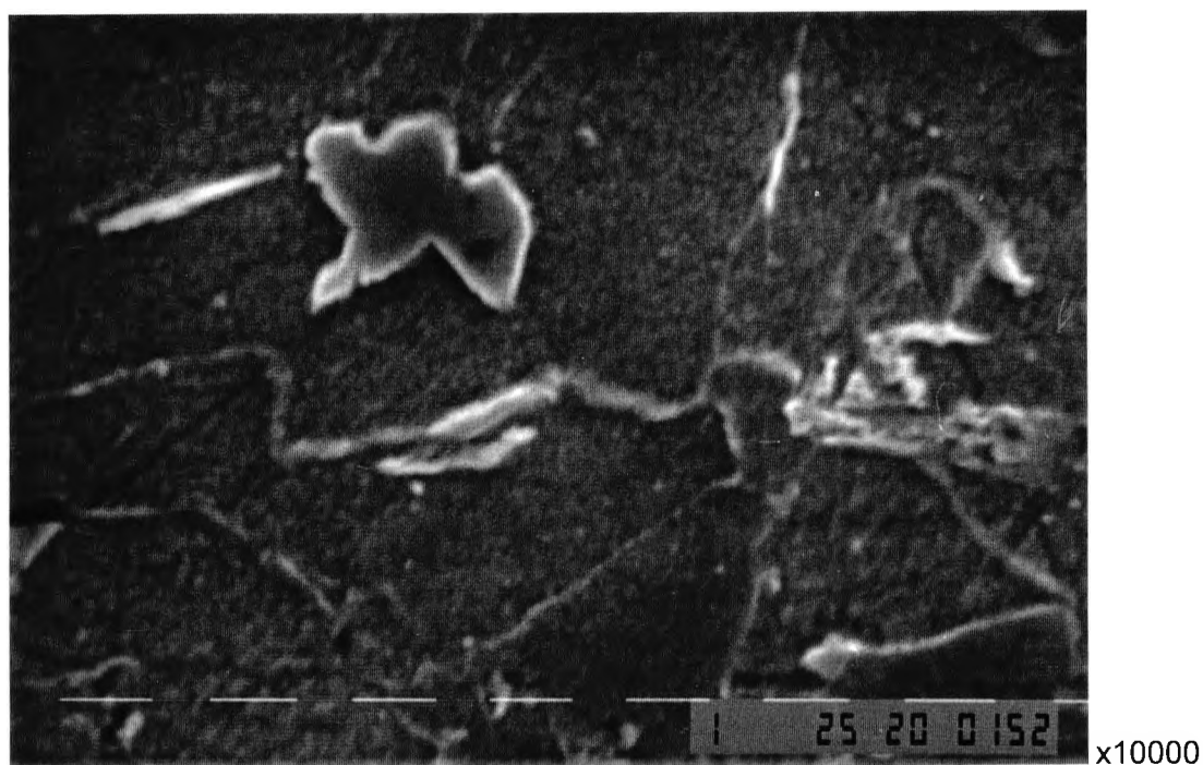
Figure 6.29 Scanning electron micrograph of the (QT500) condition, 1.26% Cu-steel, showing a martensitic particle unaffected by tempering.
