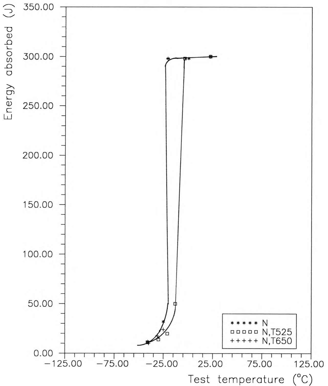
Fig.5.2 Impact transition temperature curves for "normalised" and aged 2P148H steel
