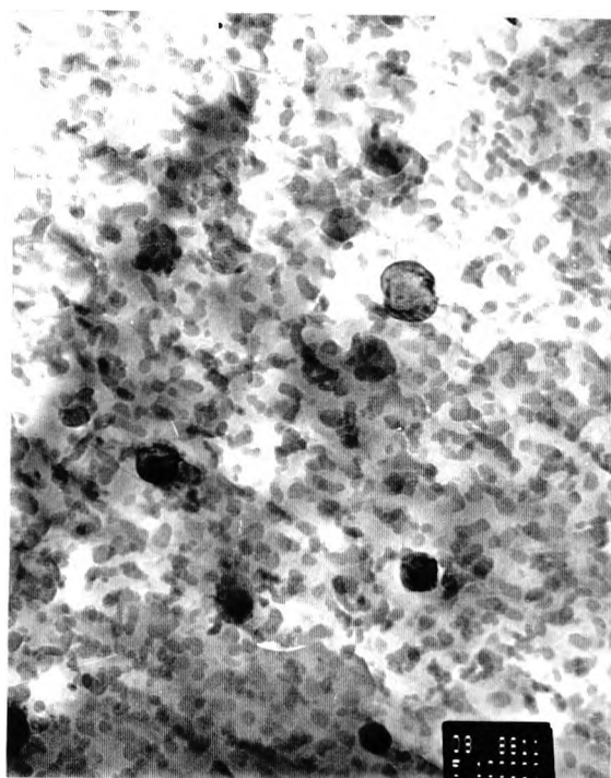
Figure 5.25 TEM of thin foil, showing copper precipitation, in the as "normalised" 1.22% Cu steel.
