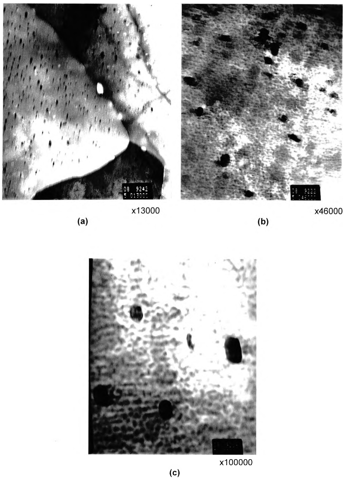
Figure 5.31 TEM of vermiculite-cooled and tempered, NT700, 2.02% Cu steel, showing (a) the intensity of precipitation (thin foil) (b), (c) the morphology of copper precipitates.
