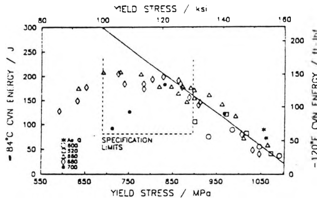
Figure 2.29 The relationship between the -84°C impact strength and the yield strength of a water-quenched and tempered HSLA-100 steel plate [73].
