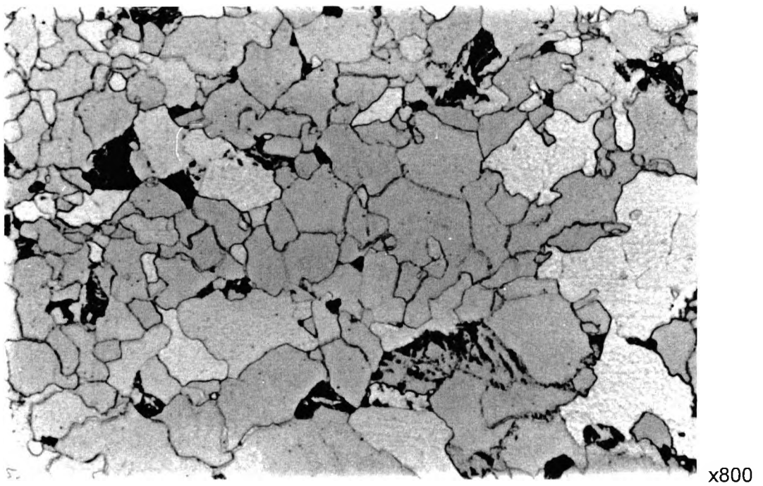
Figure 6.10 Optical micrograph of the normalised and over-aged 1.26%-Cu steel plate, (NT650).
