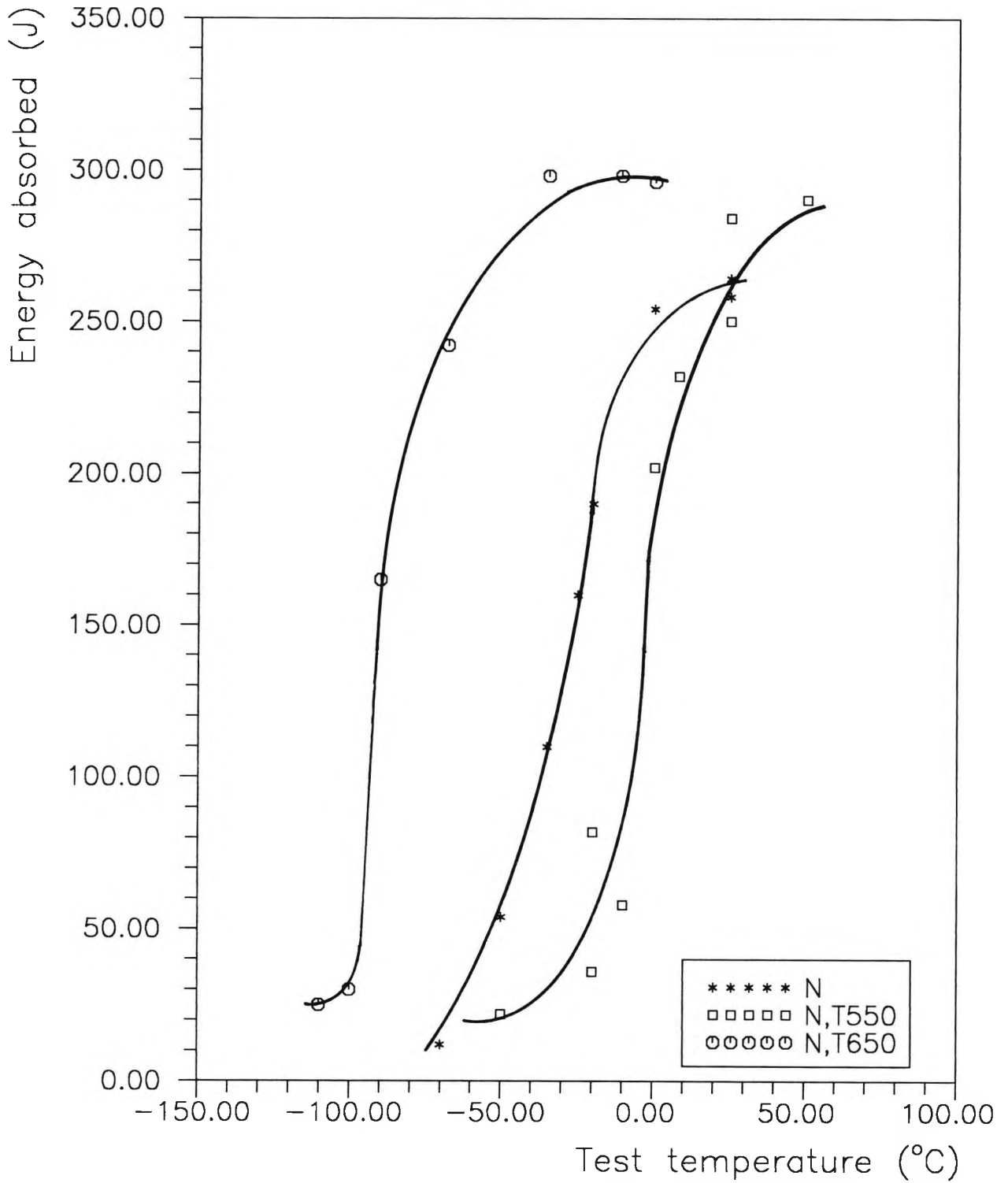
Figure 6.2 Impact transition temperature curves for normalised and aged 1P140M steel.
