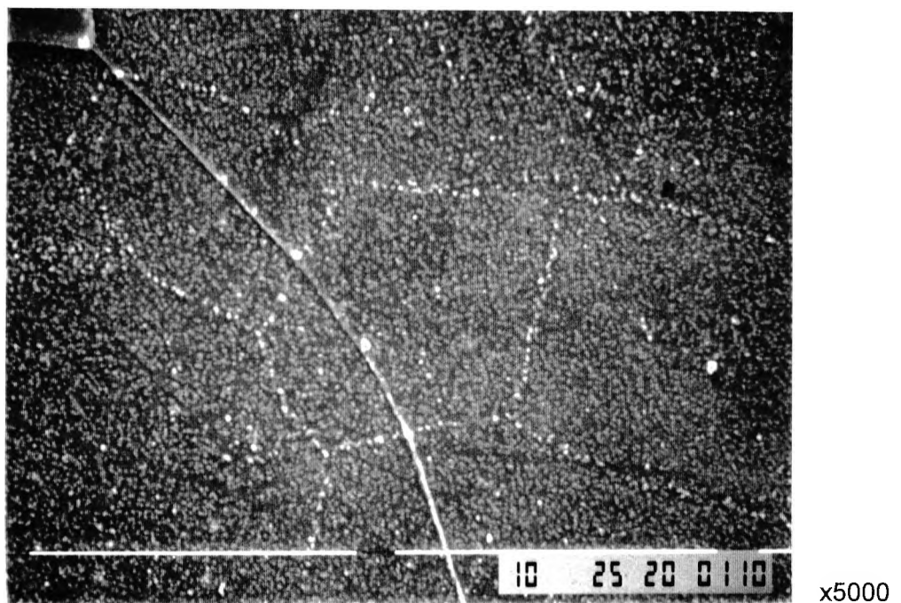
Figure 5.16 (a) Scanning electron micrograph, showing ghost boundaries formed by fine particles, on the ferrite matrix of as “normalised”, 1.22% Cu steel.
