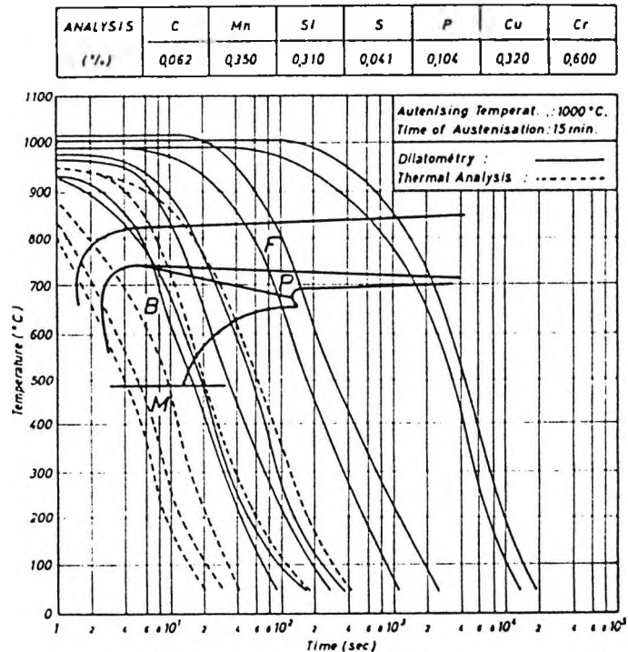
Figure 2.20 CCT diagram of COR-TEN steel [7].
