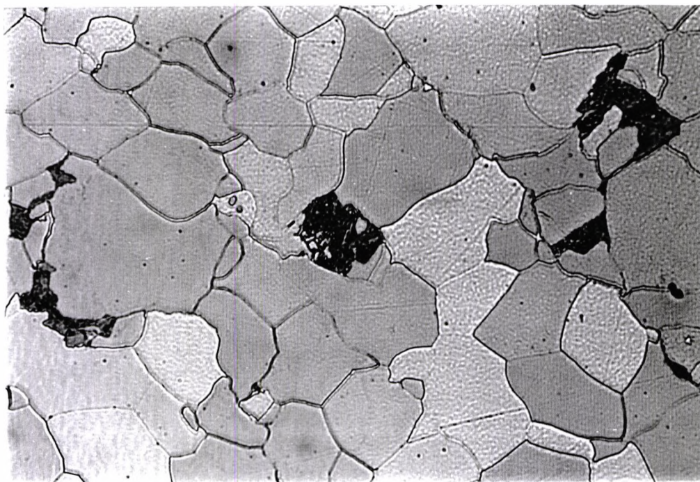
Figure 5.6 (a) Optical micrograph of the NT525 1.22% Cu steel.
