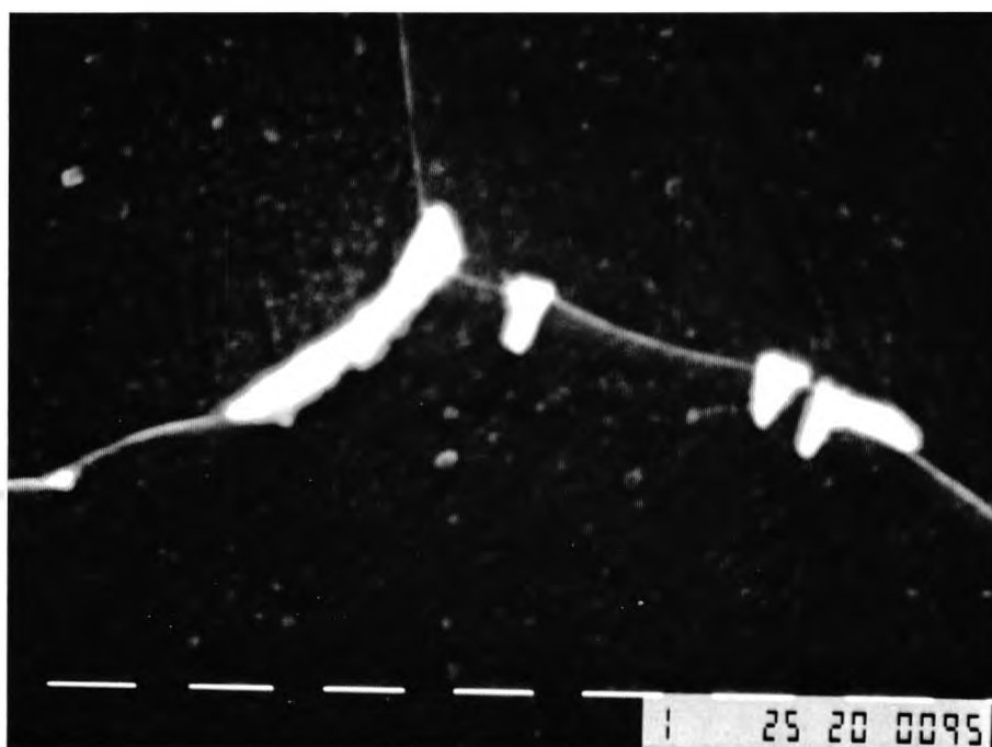
Figure 5.11 Scanning electron micrograph, showing carbides at the grain boundaries of the as "normalised", (N), copper-free steel.
