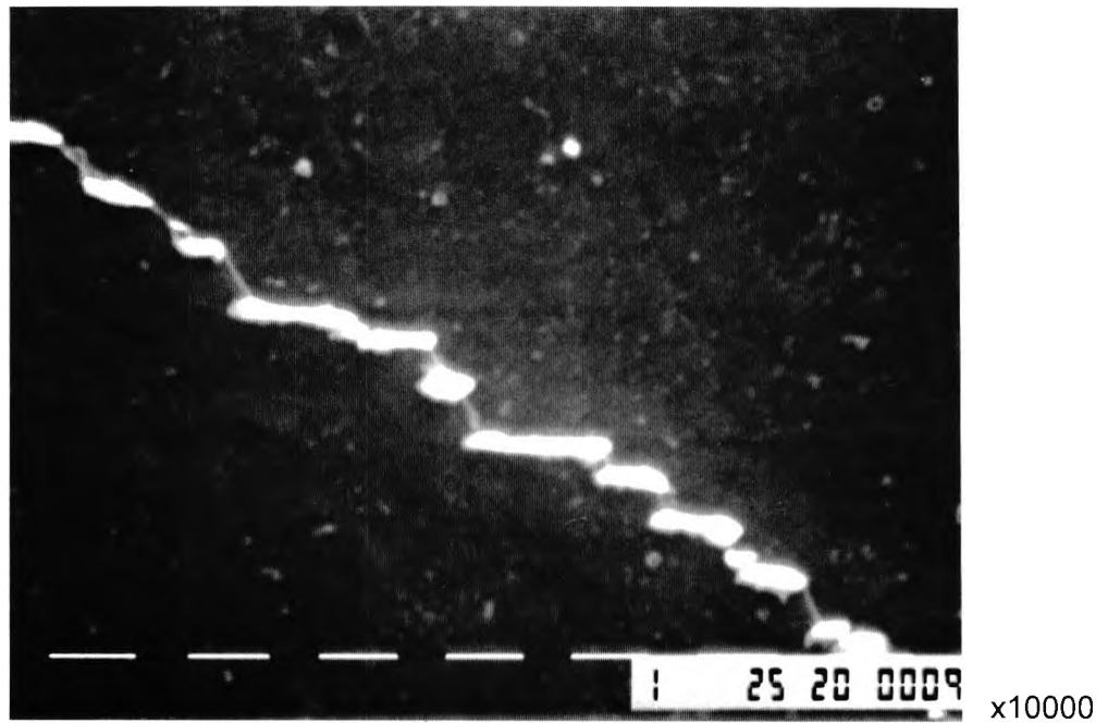
Figure 5.13 Scanning electron micrograph of NT525, copper-free steel; showing fine grain boundary carbides.
