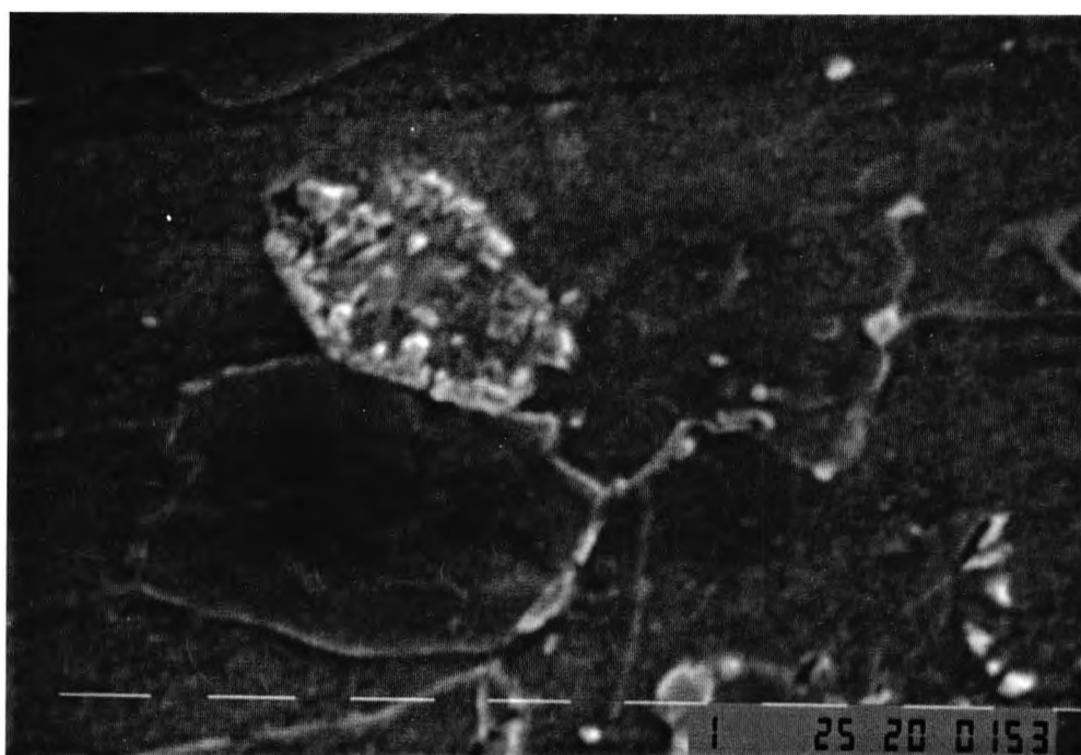
Figure 6.27 Scanning electron micrograph of the quenched and fully-aged (tempered at 500°C for 1 h) 1.26% Cu-steel, showing carbide precipitation from a martensitic particle..
