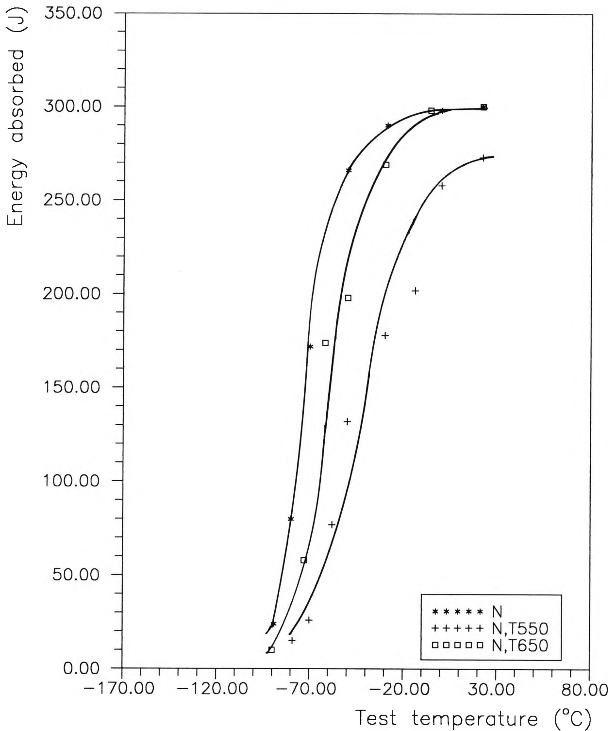
Fig.5.4 Impact transition temperature curves for "normalised" and aged 2P150H steel
