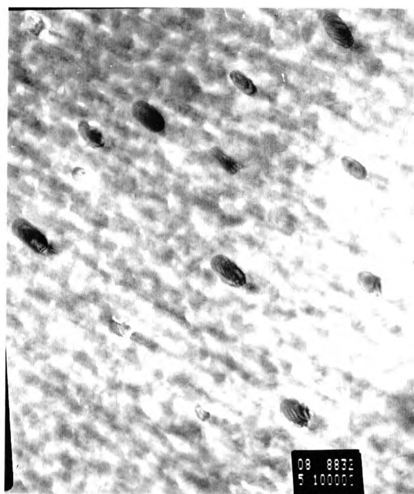
Figure 5.27 Transmission electron micrographs, showing copper precipitation in the as "normalised" 2.02% Cu steel (thin foils).
