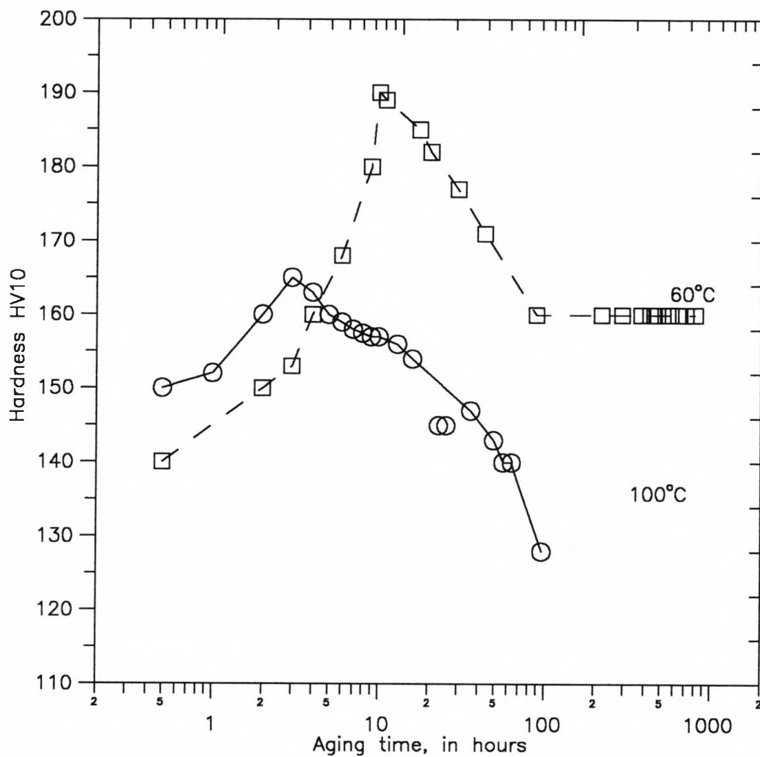
Figure 4.2 Age-hardening behaviour of steel 4P28H, quenched from 720°C and then aged at 60 and at 100 °C for various periods of time.
