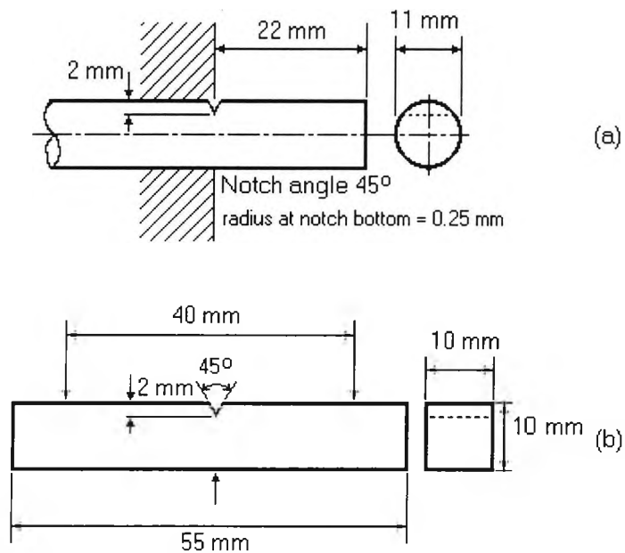
Figure 3.2 V-notch impact test specimens: (a) Izod (round) and (b) Charpy (as used in the present exercise).
