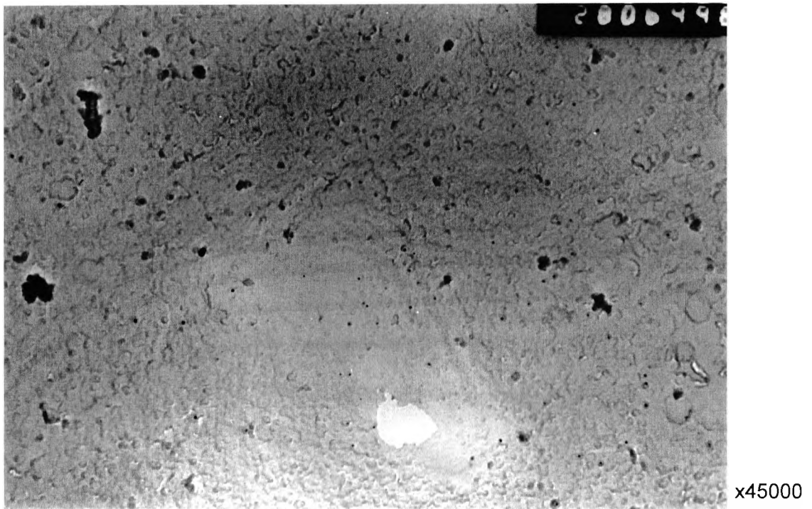
Figure 6.35 Transmission electron micrograph (replica), showing coarse Cu and fine Nb(CN) precipitates in the quenched and fully-aged condition, (QT500), of 1.26% Cu-steel plate.
