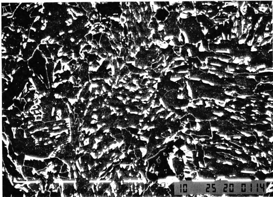
Figure 6.24 Scanning electron micrograph, of the as-quenched (Q), 1.26% Cu-steel.
