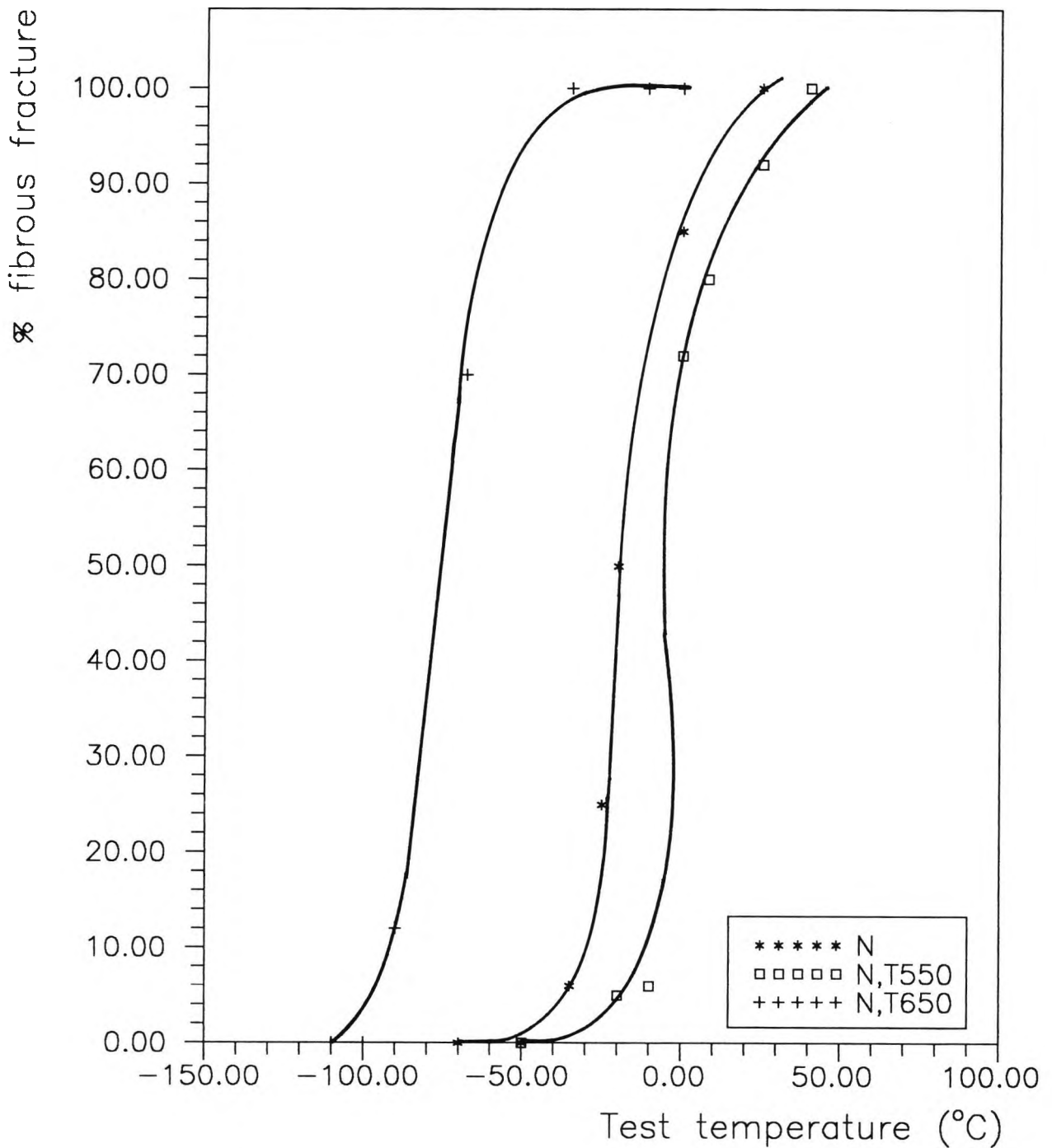
Figure 6.4 50% Fibrous appearance transition temperature curves for normalised and aged 1P140M steel
