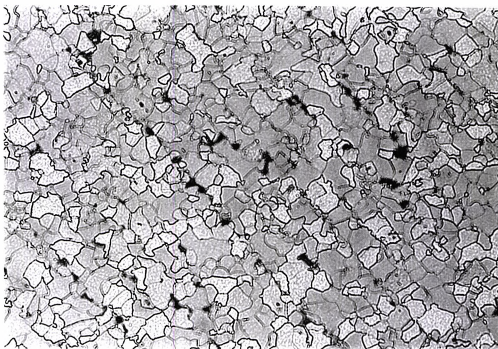
Figure 5.6 (b) Optical micrograph of the NT525, 1.22% Cu steel.
