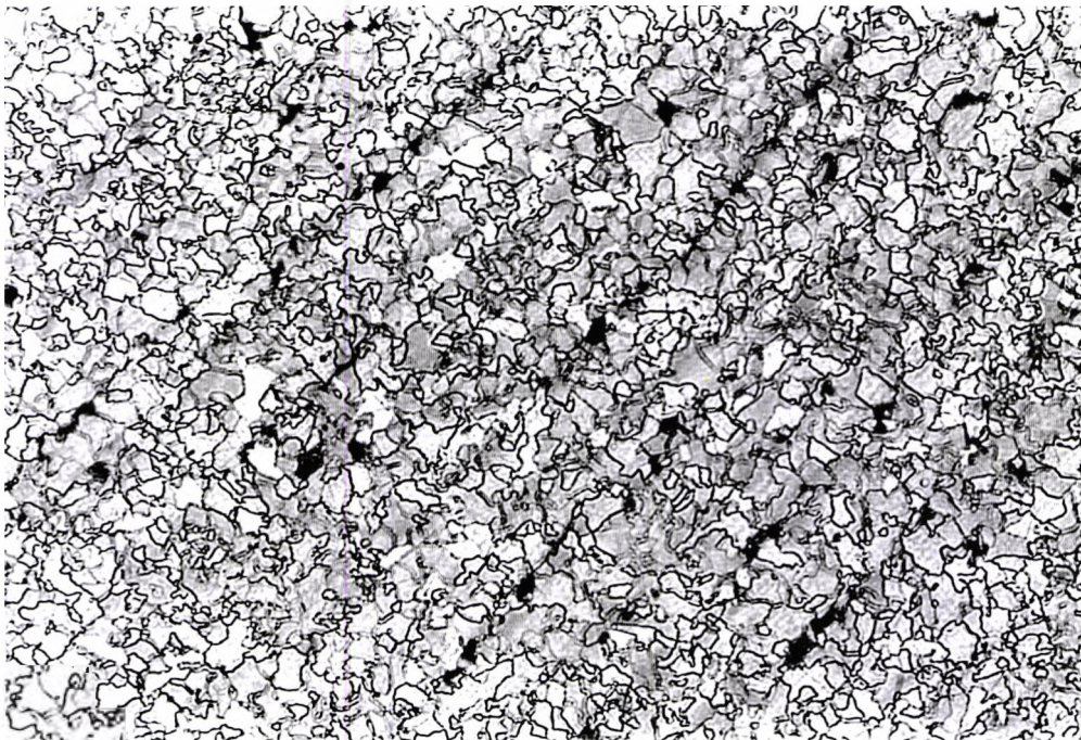
Figure 5.7 (b) Optical micrograph of the NT650, 2.02% Cu steel, showing the banding effect and the variation in ferrite shade.
