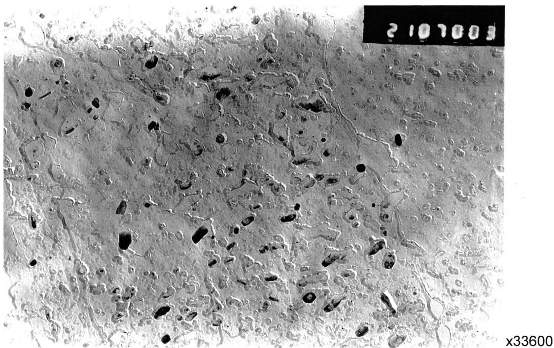
Figure 6.33 (a) Cu and Nb(CN) precipitation in the normalised and over-aged (NT650) 1.26% Cu-steel, (TEM replica).
