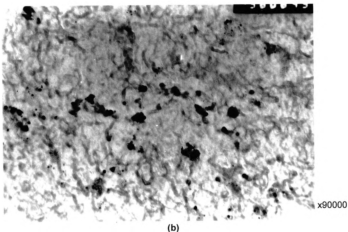
Figure 6.36 Transmission electron micrographs (replica) of the quenched and overaged (QT650) 1.26% Cu-steel plate showing Cu and Nb(CN) precipitation.
