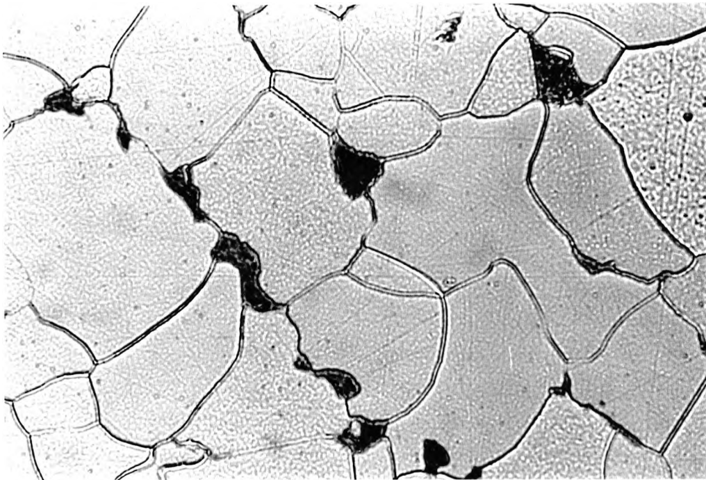
Figure 5.5 (a) Optical micrograph of as "normalised" copper-free steel.
