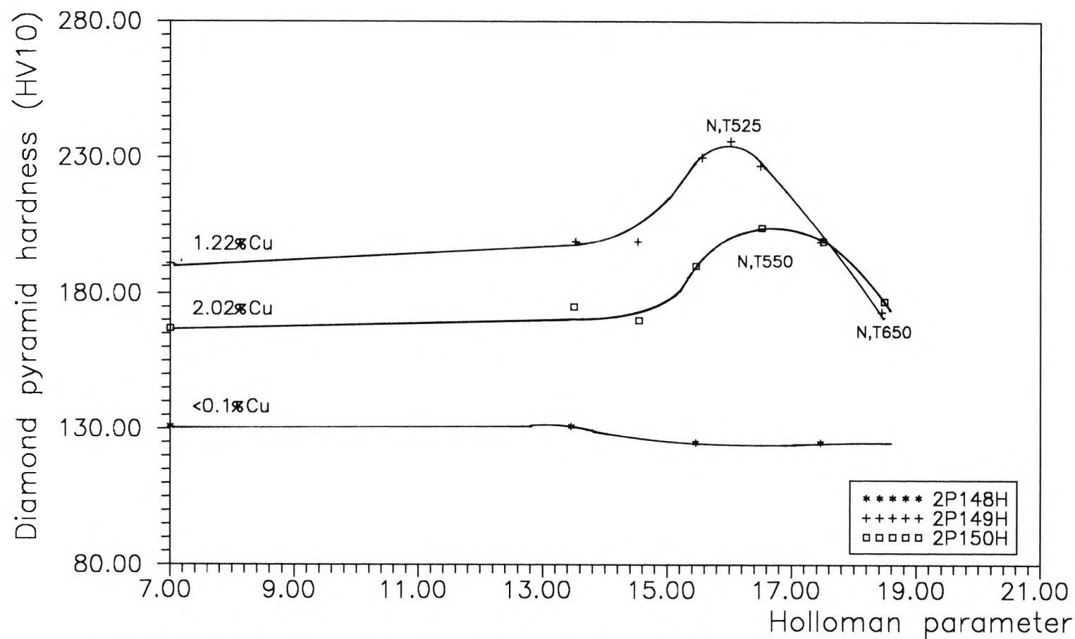
Figure 5.1 Age-hardening effect of tempering, on "normalised" 2P148H, 2P149H and 2P150H steels
