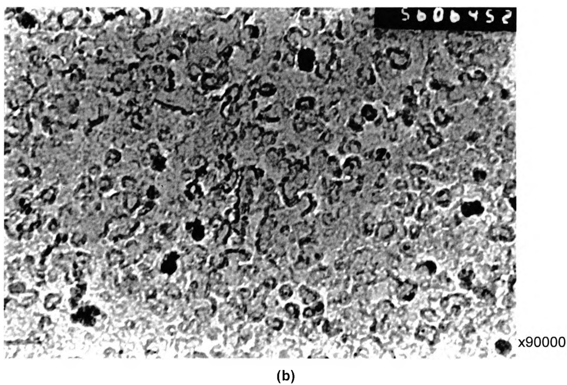
Figure 6.31 Transmission electron micrographs (replica) of the as-normalised 1.26% Cu-steel. The coarse precipitates are Cu, the fine are Nb(CN).
