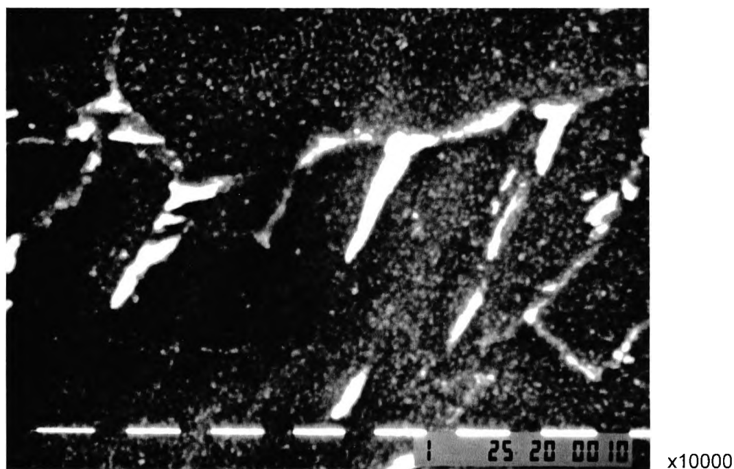
Figure 6.28 Scanning electron micrograph of the quenched and fully-aged 1.26% Cu-steel (QT500), showing evidence of copper precipitation.
