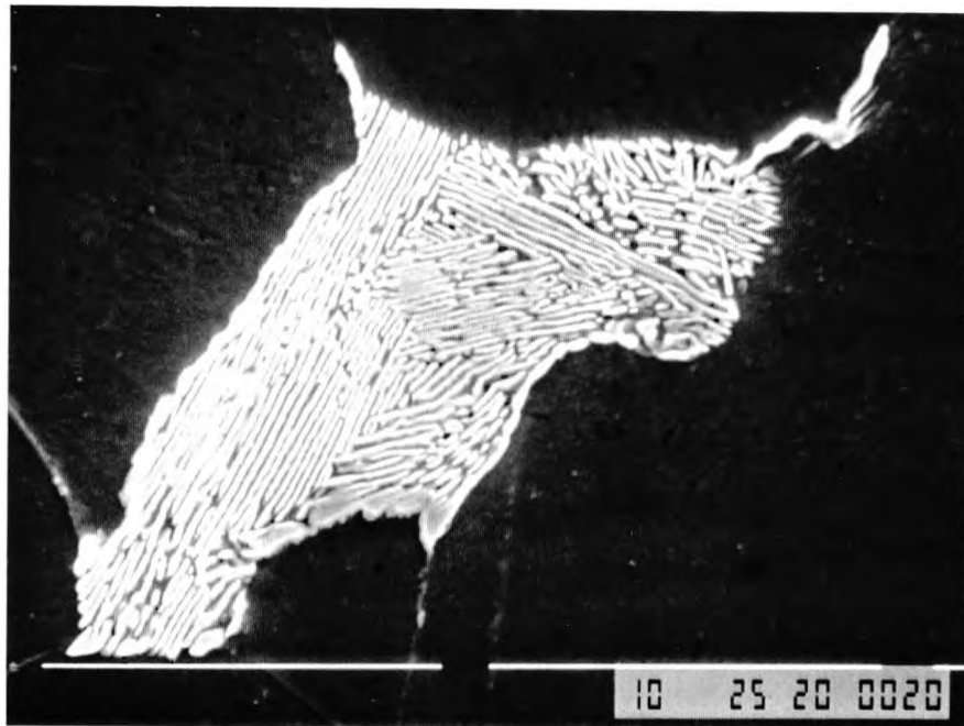
Figure 5.9 Scanning electron micrograph of the NT525, copper-free steel showing a pearlite colony.
