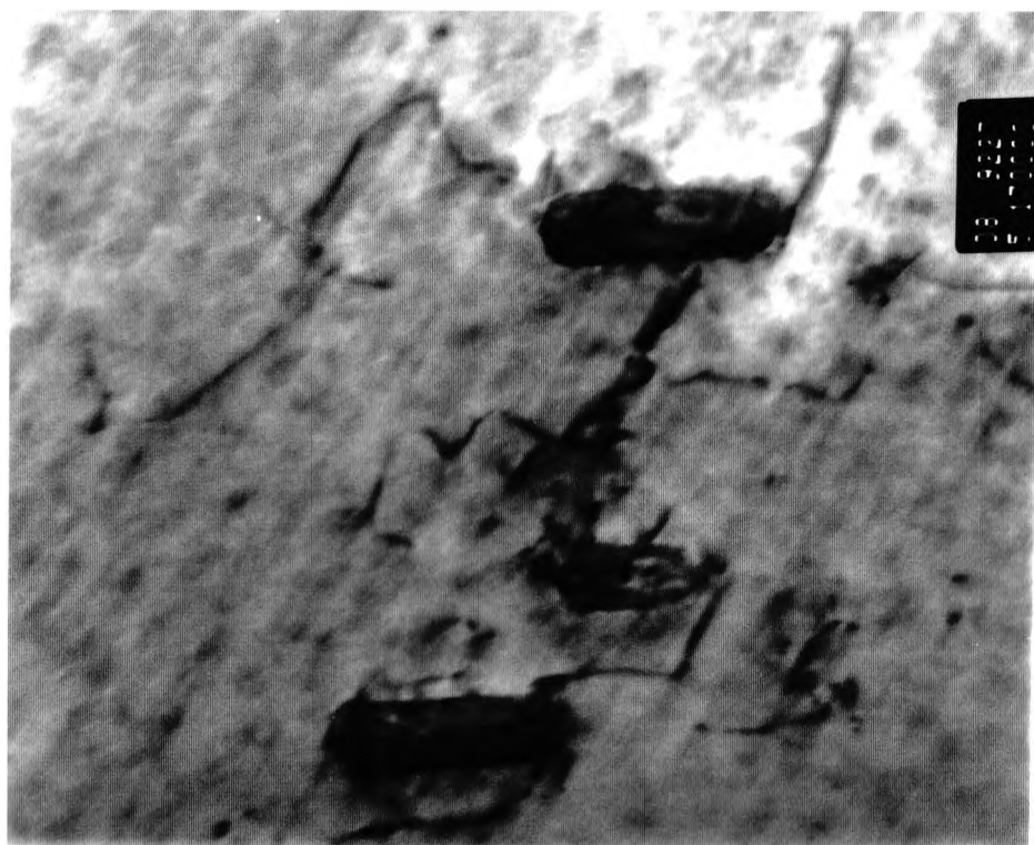
Figure 5.32 TEM of NT700, 2.02% Cu steel, that has been strained by 15%, showing precipitates surrounded by dislocations (thin foil).
