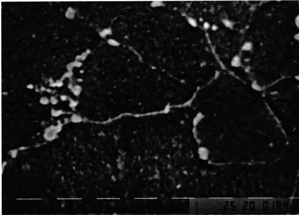
Figure 6.23 Scanning electron micrograph of sample (NT650), 1.26% Cu-steel, showing the increased number of grain boundary carbides.
