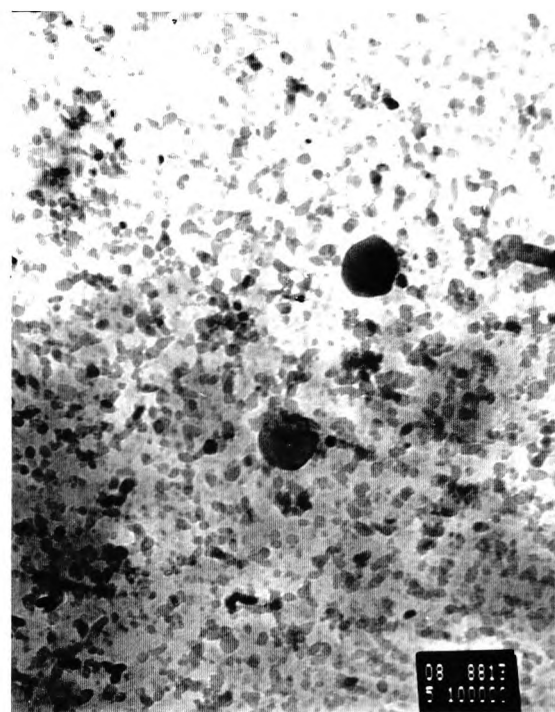
Figure 5.26 TEM of thin foil, showing copper precipitation, in the fully-aged 1.22% Cu steel.
