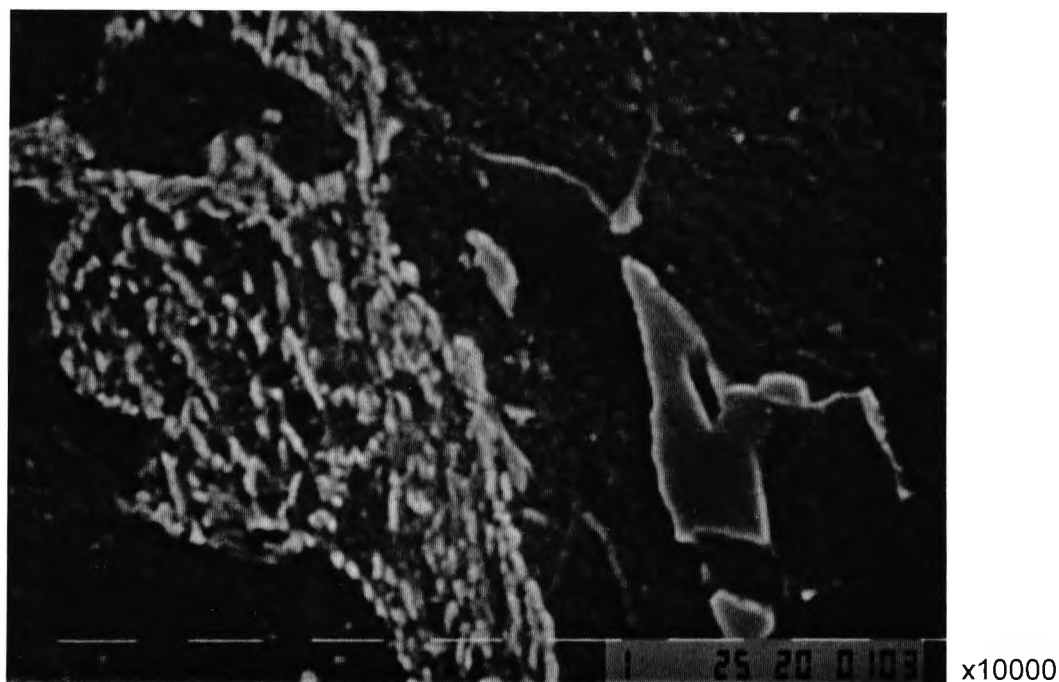
Figure 6.20 Scanning electron micrograph of the (NT550) 1.26% Cu-steel, showing two (MA) particles, one showing carbide precipitation, the other being unaffected by tempering.
