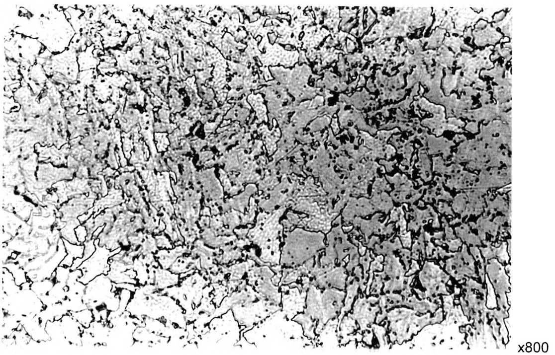
Figure 6.12 Quenched and fully-aged (QT500) microstructure of 1.26% Cu-steel.
