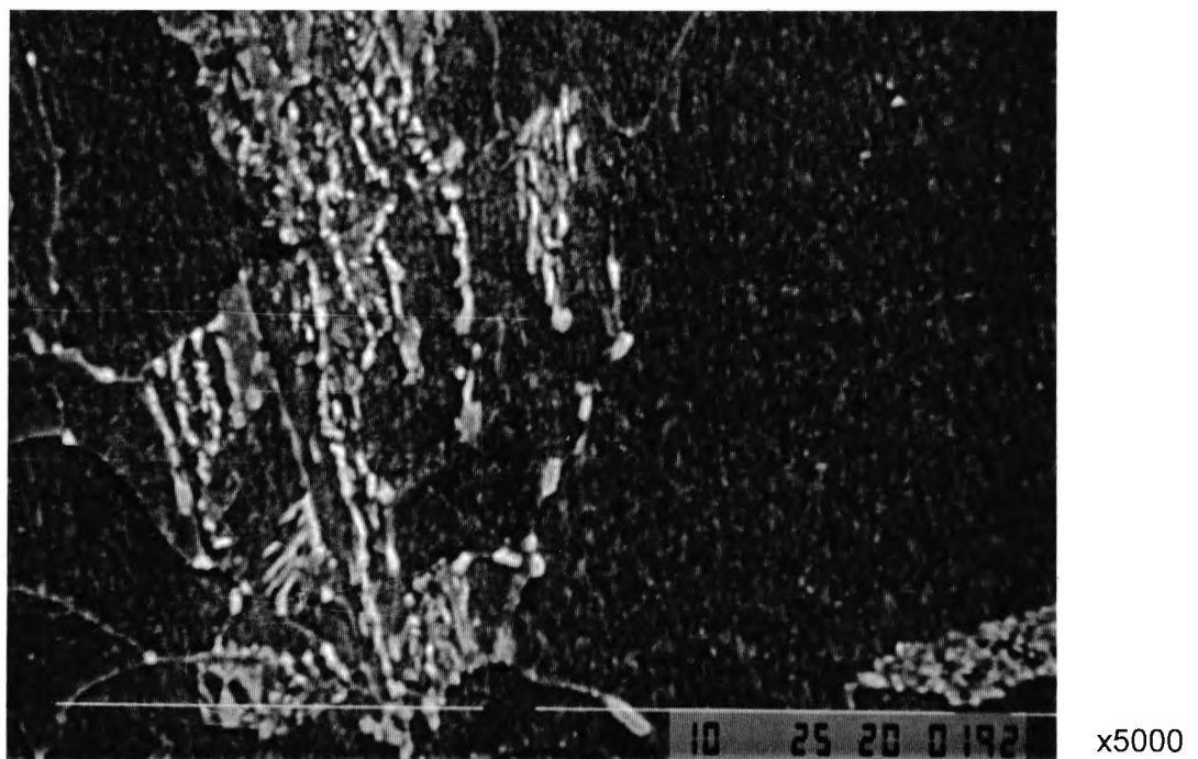
Figure 6.22 Scanning electron micrograph of 1.26% Cu-steel, in the normalised and over-aged condition (NT650).
