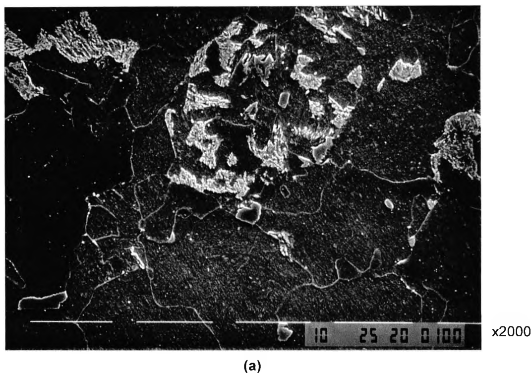
Figure 6.19 Scanning electron micrographs of (NT550) 1.26% Cu-steel, showing groups of (MA) islands: (a) fully tempered (b) unaffected by the tempering treatment.
