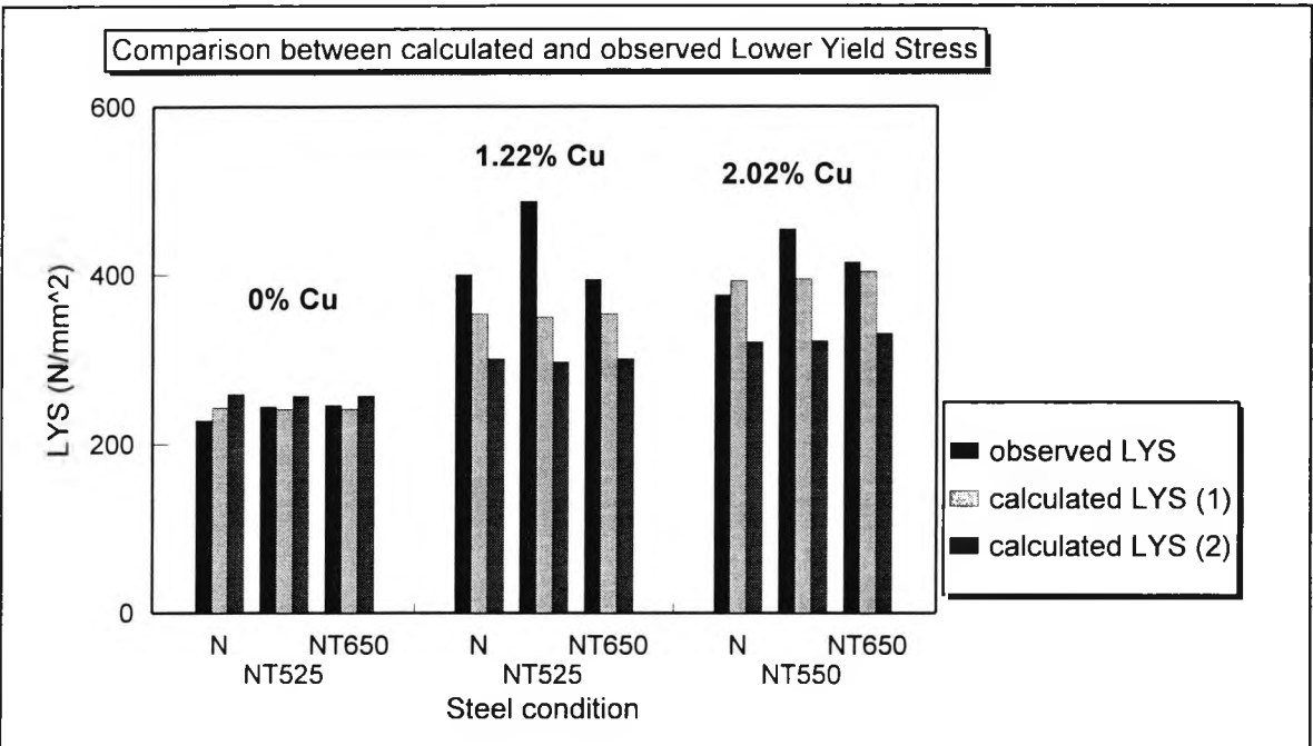
Figure 5.37 Comparison between calculated and observed LYS.
