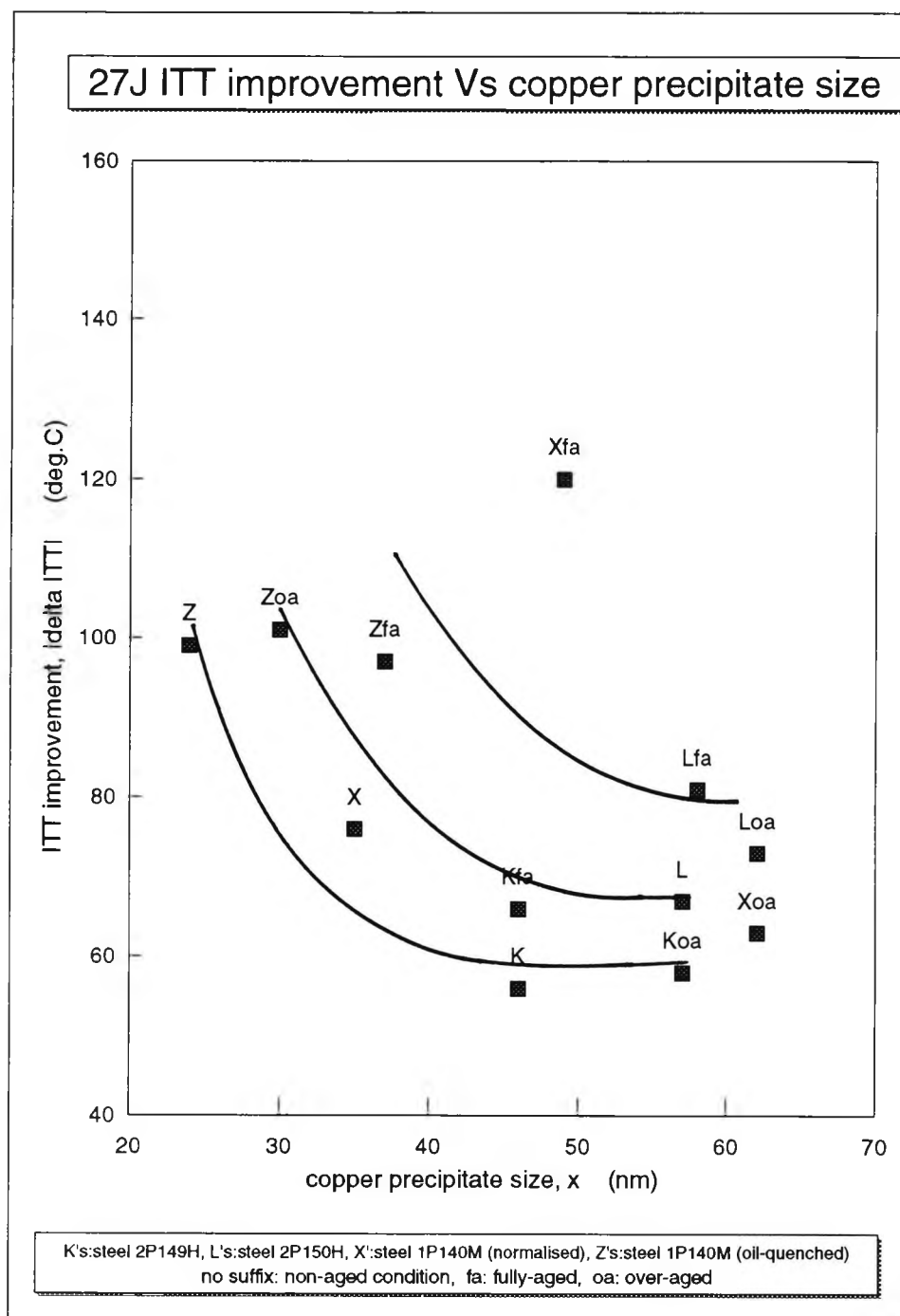
Figure 6.38 The relationship between impact transition temperature improvement and copper precipitate size (a) 54J ITT criterion (b) 27J ITT criterion.
