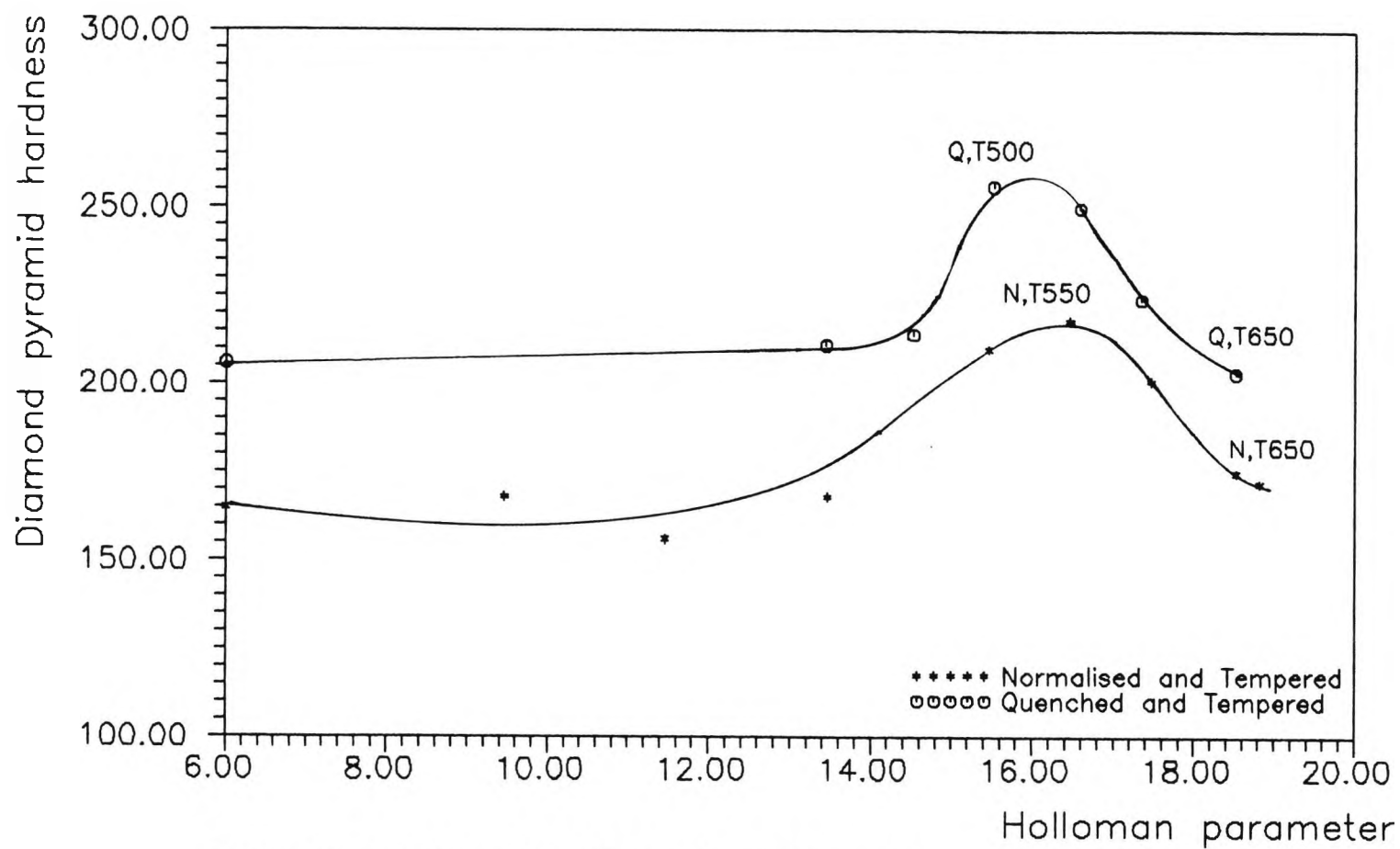
Figure 6.1 Age-hardening effect of tempering on normalised and oil-quenched 1P140M steel plate.
