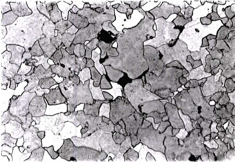
Figure 5.7 (a) Optical micrograph of the NT650, 2.02% Cu steel.
