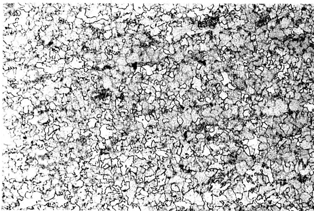
Figure 6.6 Optical micrograph of the as-normalised 1.26% Cu-steel.
