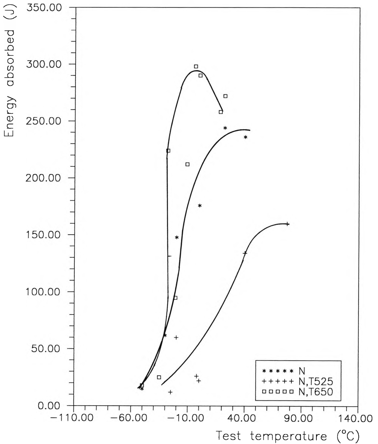
Fig.5.3 Impact transition temperature curves for "normalised" and aged 2P149H steel
