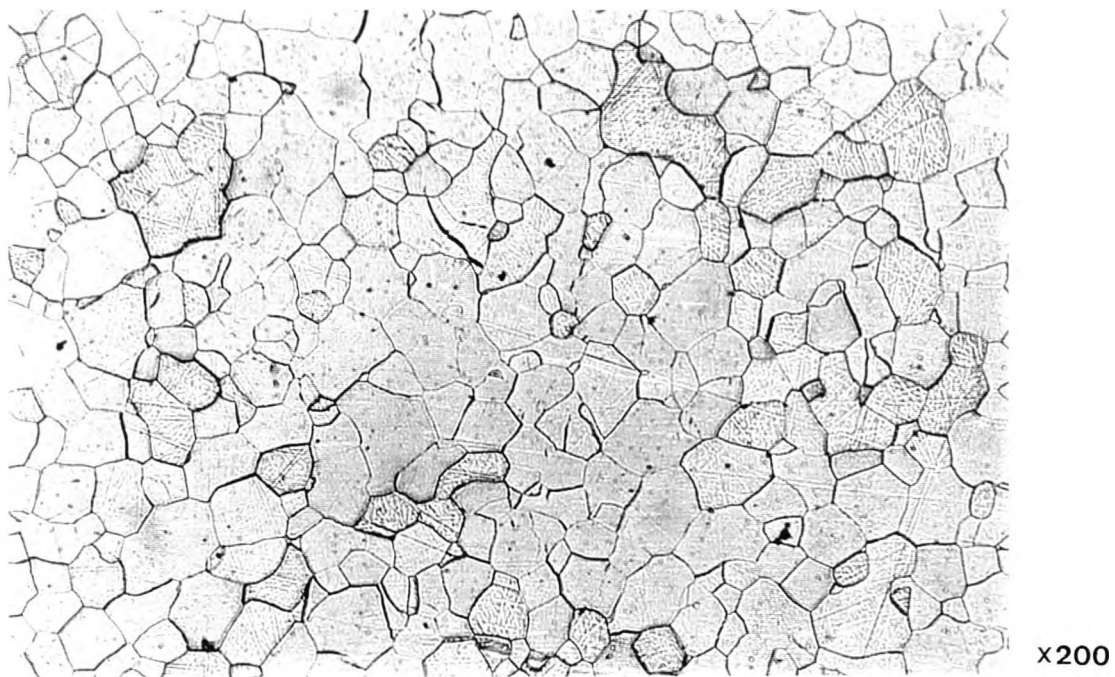
Figure 4.4 Optical micrograph of steel No1, solution treated at 700°C for 1 h and ice-quenched and then aged at 60°C for 16 h.
