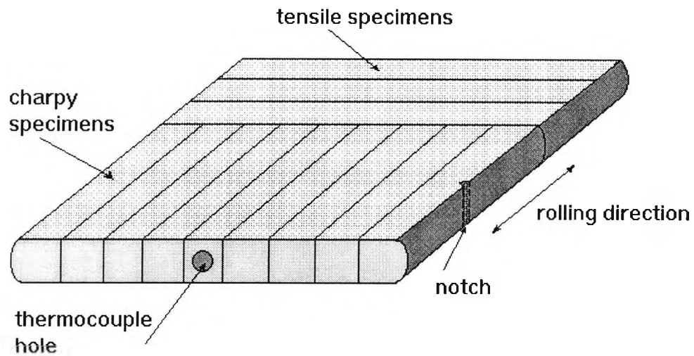
Figure 3.1 Standard outlook of steel-plates used for heat treatments.
