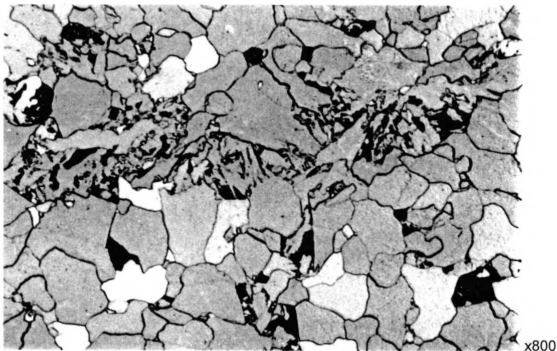
Figure 6.8 The darkening of the second phase after tempering the normalised 1.26% Cu-steel at 550°C for 1h. (Optical micrograph)
