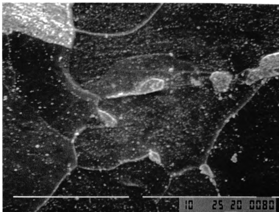
Figure 6.17 Scanning electron micrograph, showing coarse grain boundary particles, in the as-normalised 1.26% Cu-steel.
