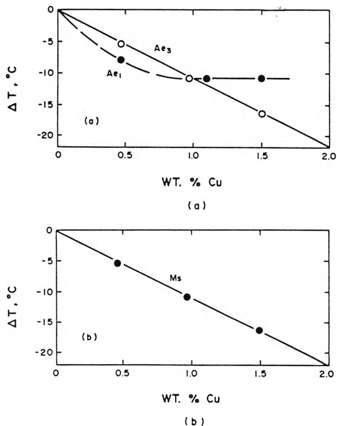
Figure 2.18 The effect of copper on (a) equilibrium transformation temperatures and (b) M_s temperature [7].
