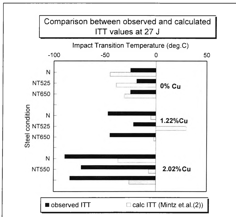
Figure 5.40 Comparison between observed and calculated 27J ITT values.
