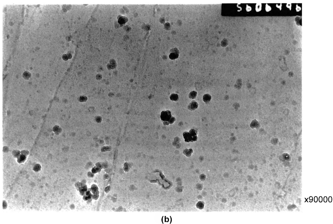
Figure 6.34 Transmission electron micrographs (replica) showing copper precipitation in the as-quenched (Q) condition of 1.26% Cu-steel.
