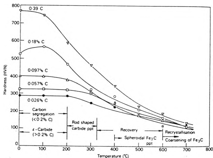
Figure 2.9 Hardness of iron-carbon martensites tempered for 1 h at 100-700°C [91].
