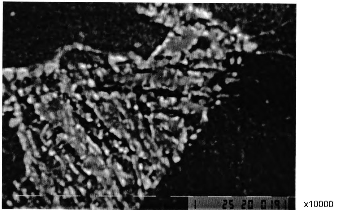
Figure 6.21 Scanning electron micrograph of normalised and over-aged 1.26% Cu-steel (NT650), showing carbide precipitation from a tempered martensitic particle.
