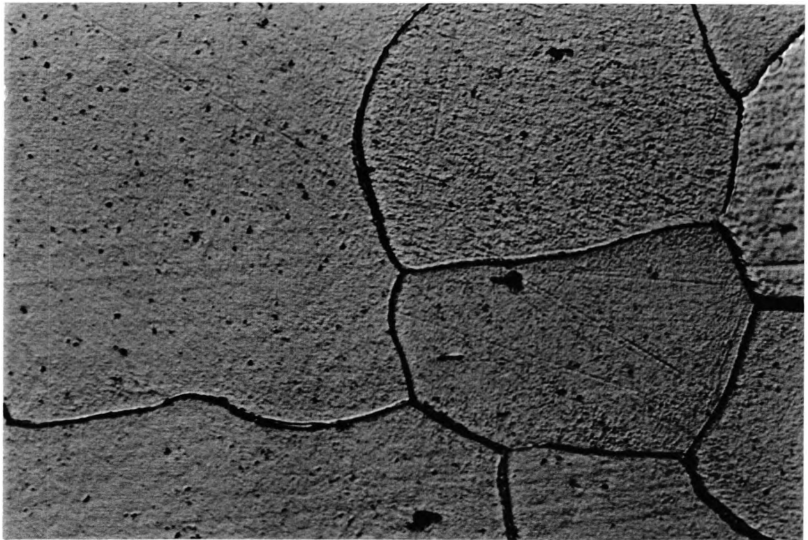
Figure 4.5 (b) Optical micrograph of steel 4P28H, as-quenched from 720°C, showing carbide precipitation in ferrite.
