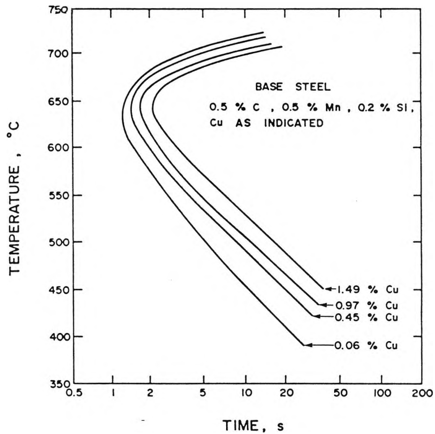
Figure 2.19 The effect of copper on the time for 50% isothermal transformation in a medium carbon steel [83].
