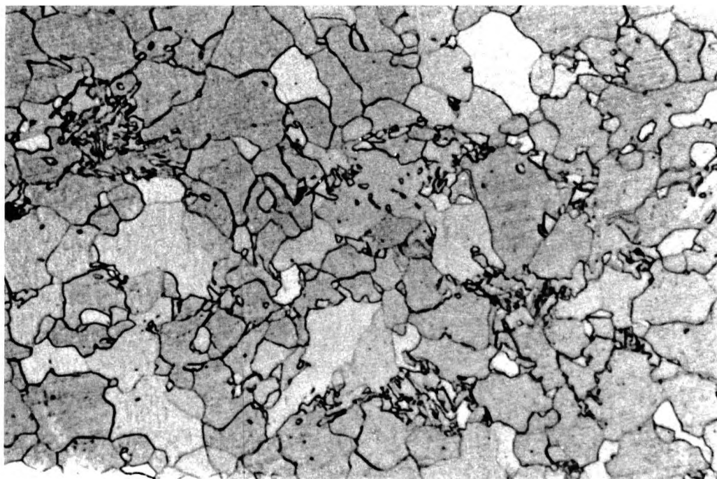
Figure 6.5 Optical micrograph of the as-normalised 1.26% Cu-steel.
