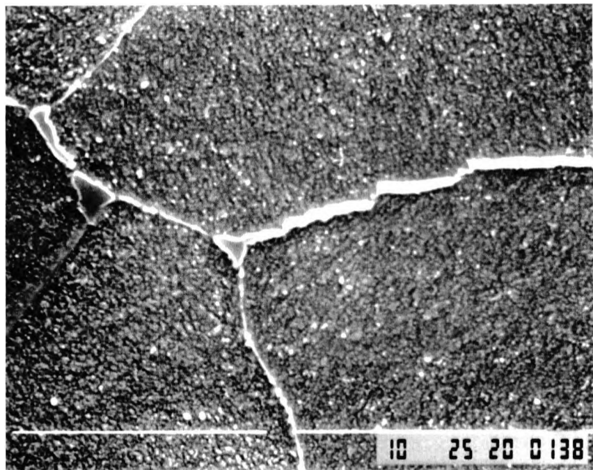
Figure 5.19 Scanning electron micrograph, showing grain boundary carbides of the 1.22% Cu steel, in the over-aged condition (NT650).
