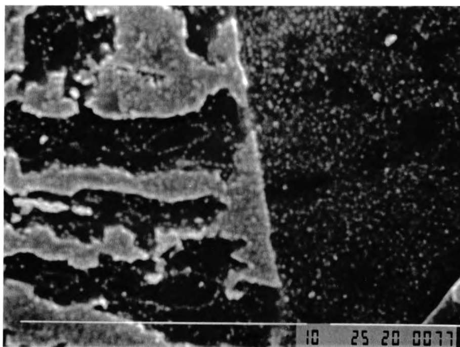
Figure 6.15 Scanning electron micrograph of the as-normalised, (N), 1.26% Cu steel, showing: (a) a group of martensite-austenite islands (b) coarse precipitation -possibly copper- in the ferrite matrix and in the (MA) constituent.
