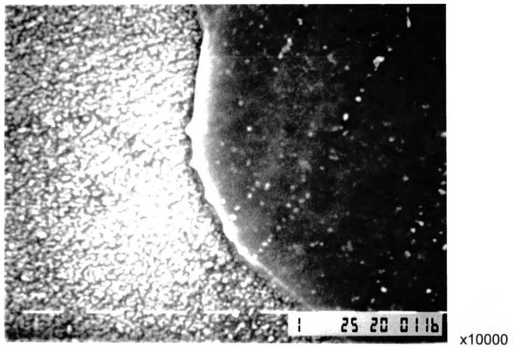
Figure 5.17 Scanning electron micrograph, showing the shade difference between adjacent ferrite grains, of "normalised" and fully-aged (NT525) 1.22% Cu steel.
