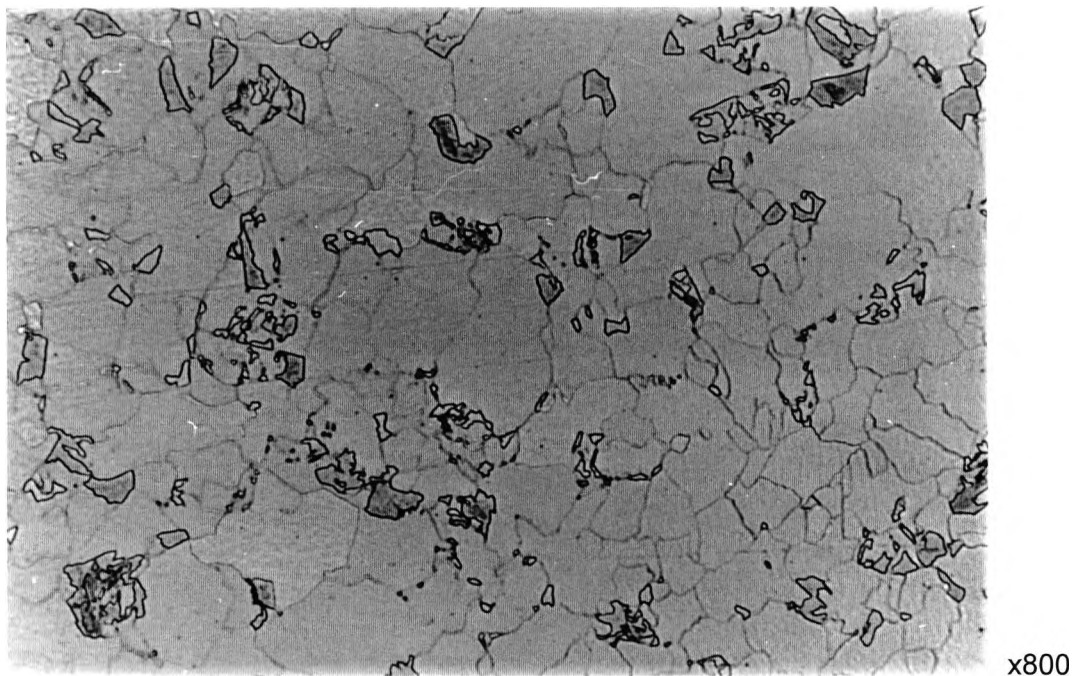
Figure 6.7 The distinction between the ferrite and the second phase in the normalised and aged (200°C for 1h) 1.26% Cu steel (light etching, optical micrograph).
