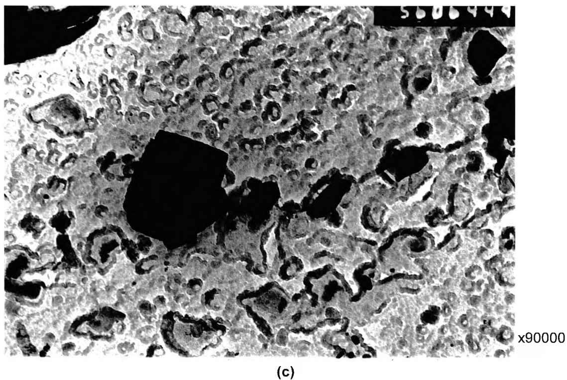
Figure 6.33 Transmission electron micrographs (replica) of the normalised and over-aged (NT650) 1.26% Cu-steel, showing : (b) Cu and Nb(CN) precipitation and grain boundary carbides, (c) grain boundary particles and Nb(CN) precipitates.
