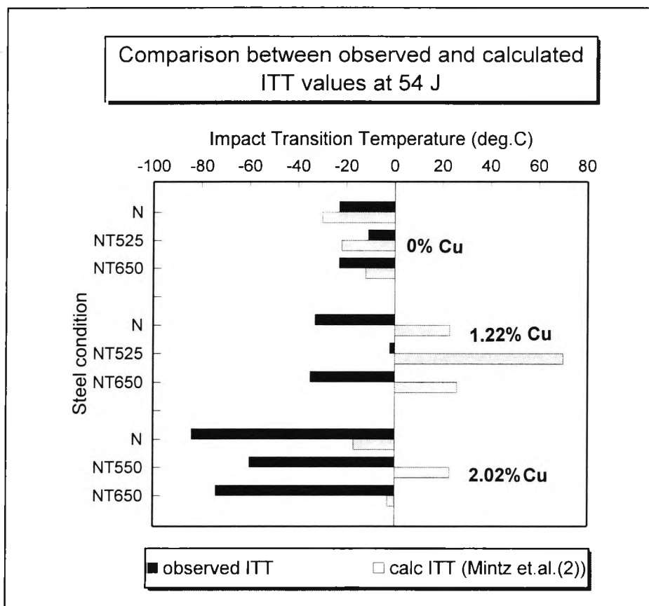
Figure 5.39 Comparison between observed and calculated 54J ITT values.
