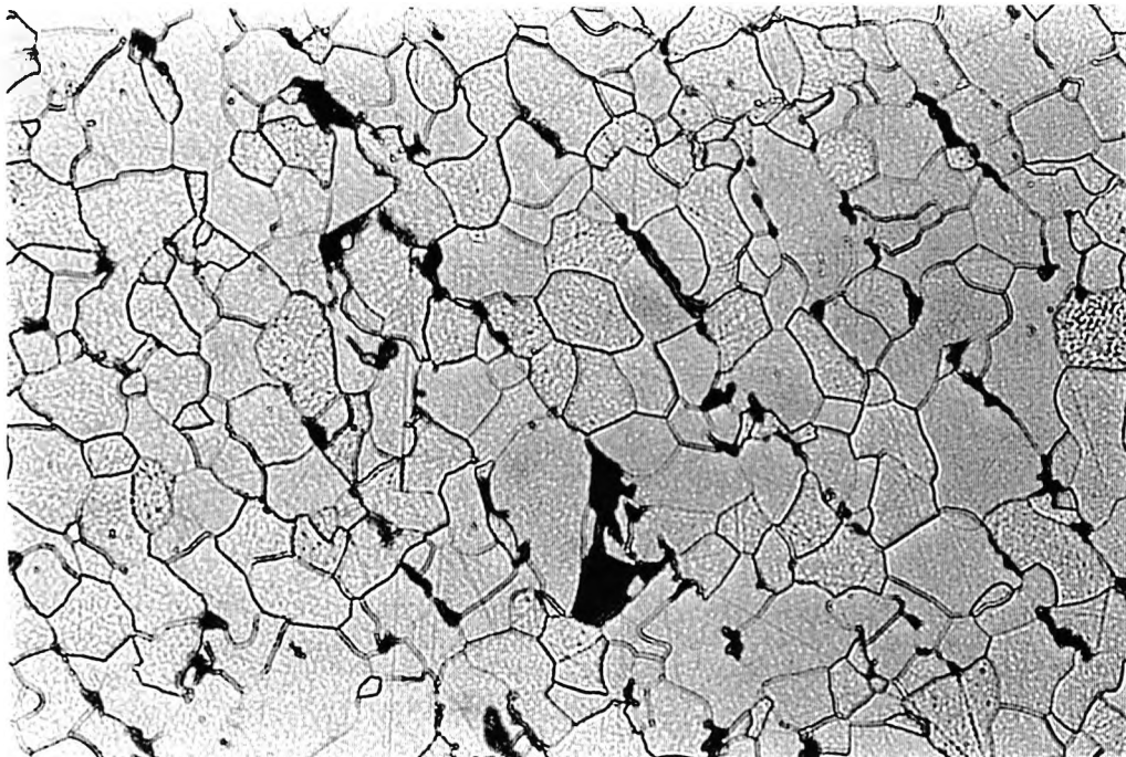
Figure 5.5 (b) Optical micrograph of the NT525 copper-free steel, showing banding.
