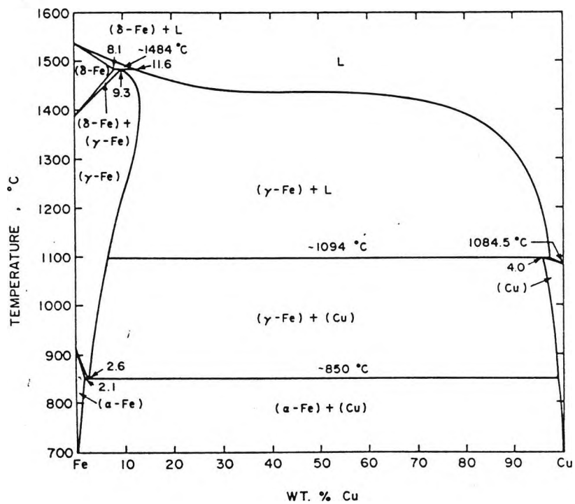
Figure 2.16 The Fe-Cu diagram (based on data from ref.[12].)
