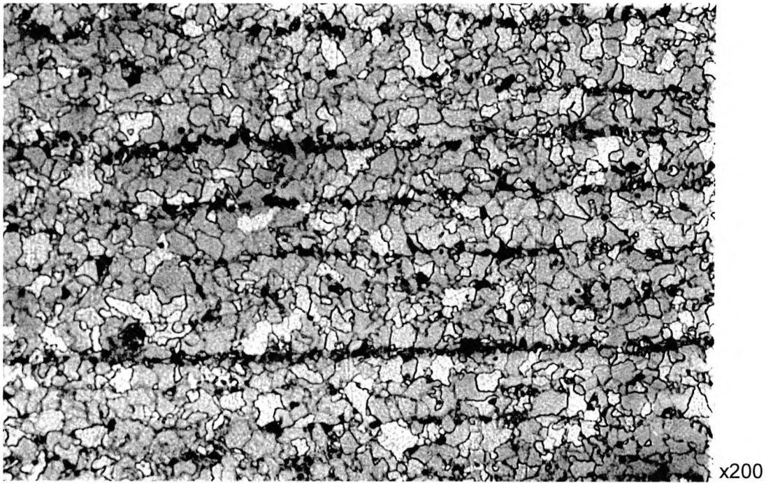
Figure 6.9 Optical micrograph of sample (NT550), 1.26% Cu-steel.
