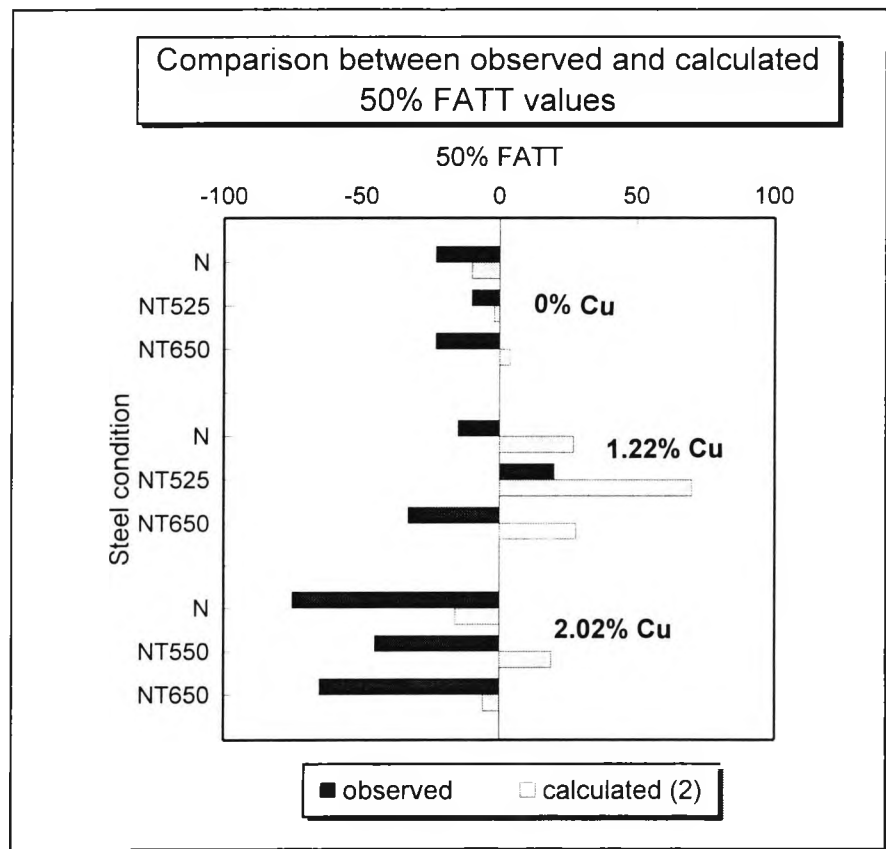
Figure 5.38 Comparison between observed and calculated 50% FATT values.
