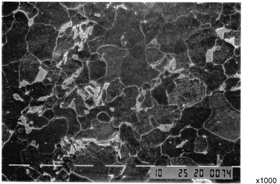
Figure 6.14 Scanning electron micrograph showing the microstructure of the as-normalised 1.26% Cu-steel.
