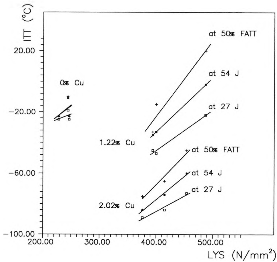
Figure 5.41 The variation of the observed impact transition temperatures as a function of the observed lower yield strength, of steels 2P148H, 2P149H and 2P150H.
