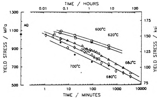
Figure 2.28 The effect of tempering on the 0.2% offset yield strength of a water-quenched (1 h at 950°C) HSLA-100 steel plate (19 mm in thickness) [73].
