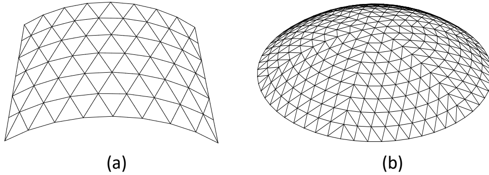
Figure 3: Single-layer reticulated shells: (a) Cylindrical shell (b) Dome. The probability of various instabilities leading to progressive collapse is greater in these single-layer spatial structures than in multi-layer spatial structures.
