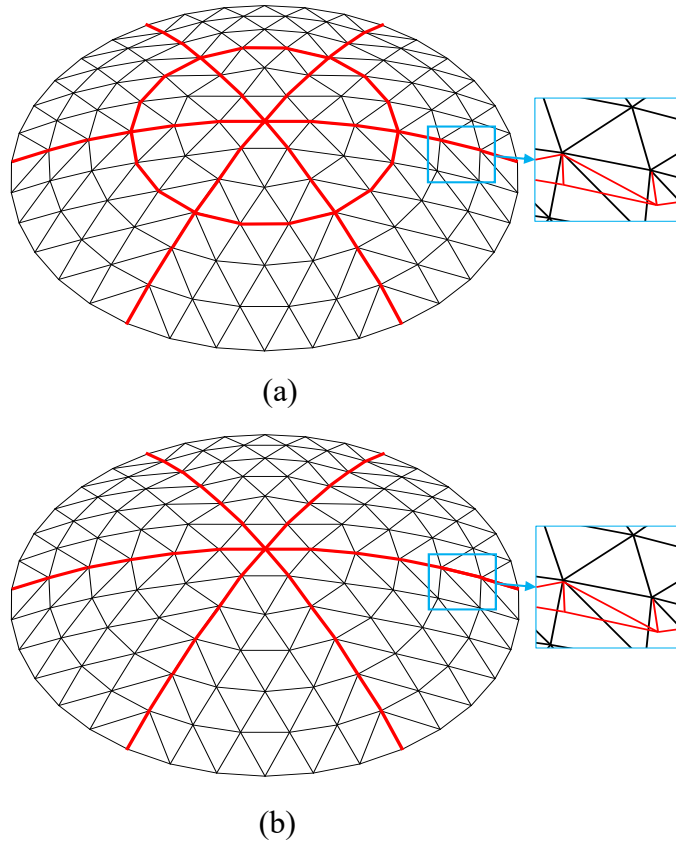
Figure 26: A partial double-layer arrangement was adopted to enhance the resistance to the progressive collapse of Kiewitt-6 dome: (a) double-layer member arrangement is provided along radial members and latitudinal members in the middle region [113], and (b) double-layer member arrangement is provided along radial members [97]. The double-layer member arrangement is highlighted using red colour to indicate its location in the figure.
