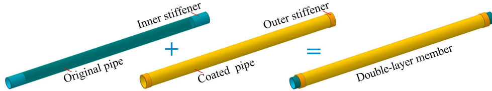
Figure 24: Double-layer member arrangement for increasing the stability [114]. The image reproduced with permission.
