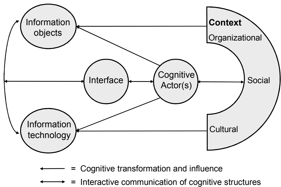
Figure 4. Model of interactive information seeking, retrieval and behavioural processes (Ingwersen and Järvelin, 2005, p. 261, Figure 6.1) Reproduced with kind permission from Springer Science+Business Media B.V.
