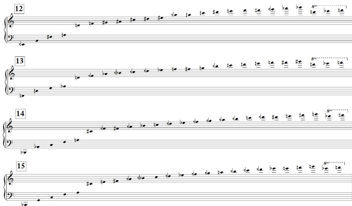
Fig. 33 Sonic spectra transcribed from a sample of howling wind and arranged in a chord progression. The spectra are numbered in progression order, so spectrum 1 begins the progression and 15 ends it.
