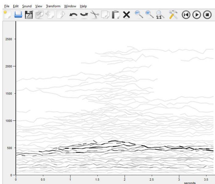
Fig. 32 SPEAR analysis of howling wind
