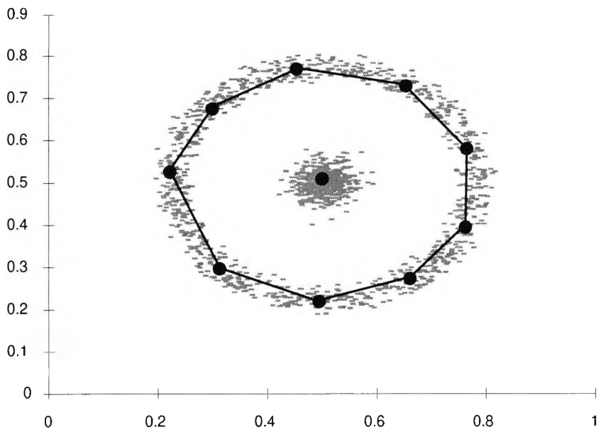
Figure 4.1: The APC solution to a two cluster problem. The heavy dots represent the initial cluster centroids found via k-means while the lines indicate agglomerations. The circular shape is represented via a piecewise linear approximation using the linked line segments.
