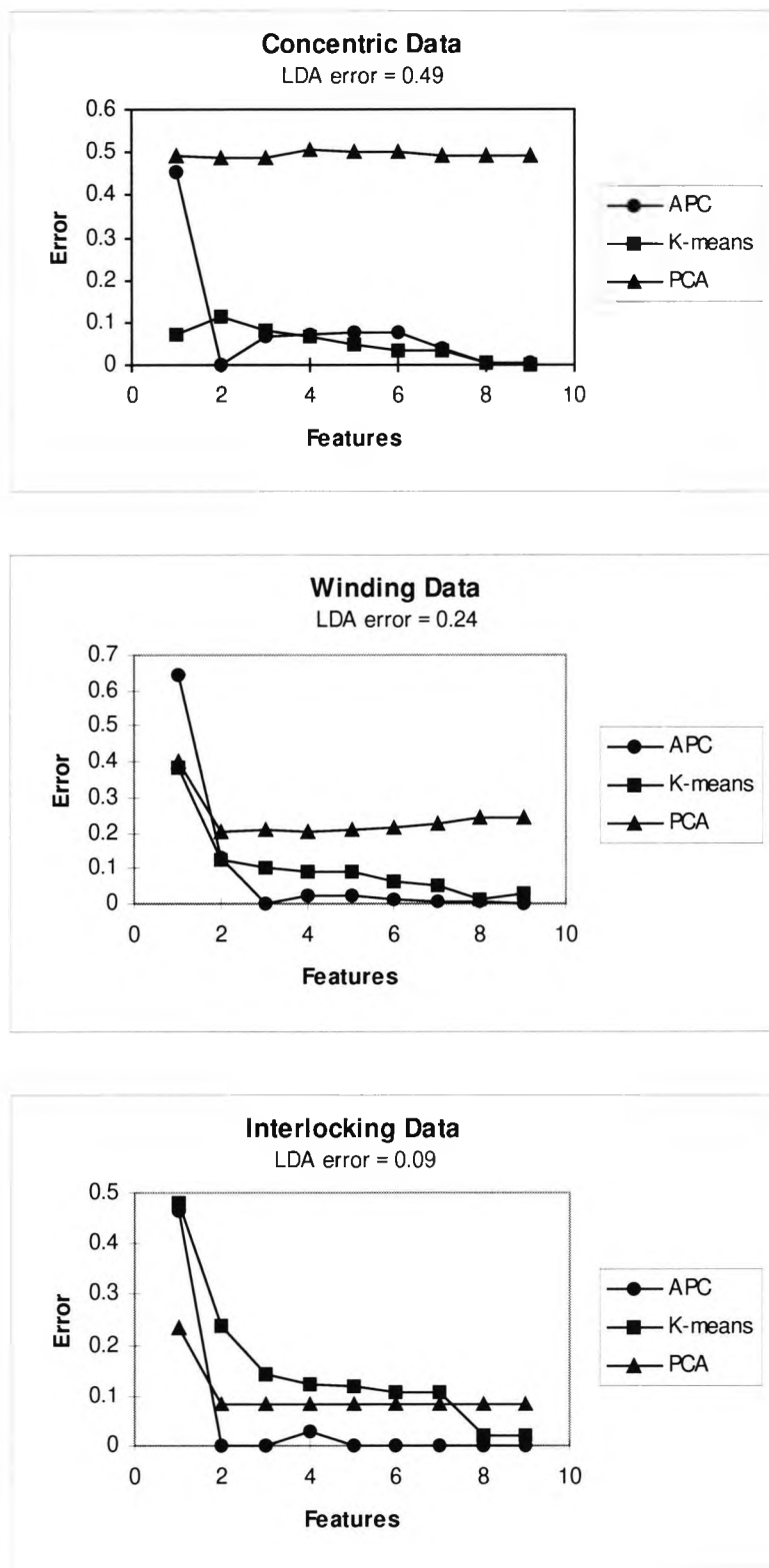
Figure 8.4 The relative performances of the three feature extraction methods on simulated data. The performance of LDA on the 10 original variables is given below the chart titles.
