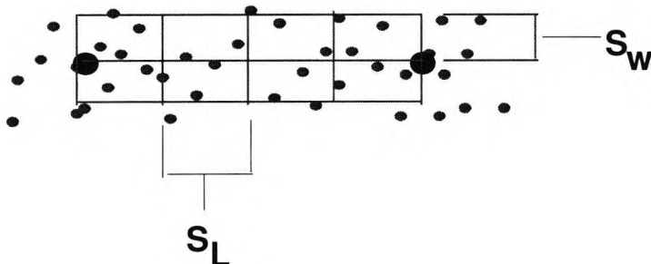
Figure 4.4: Intercluster density is estimated via a series blocks of s_W \times s_L regions of the intercluster area. The heavy dots are the k-means derived centroids
