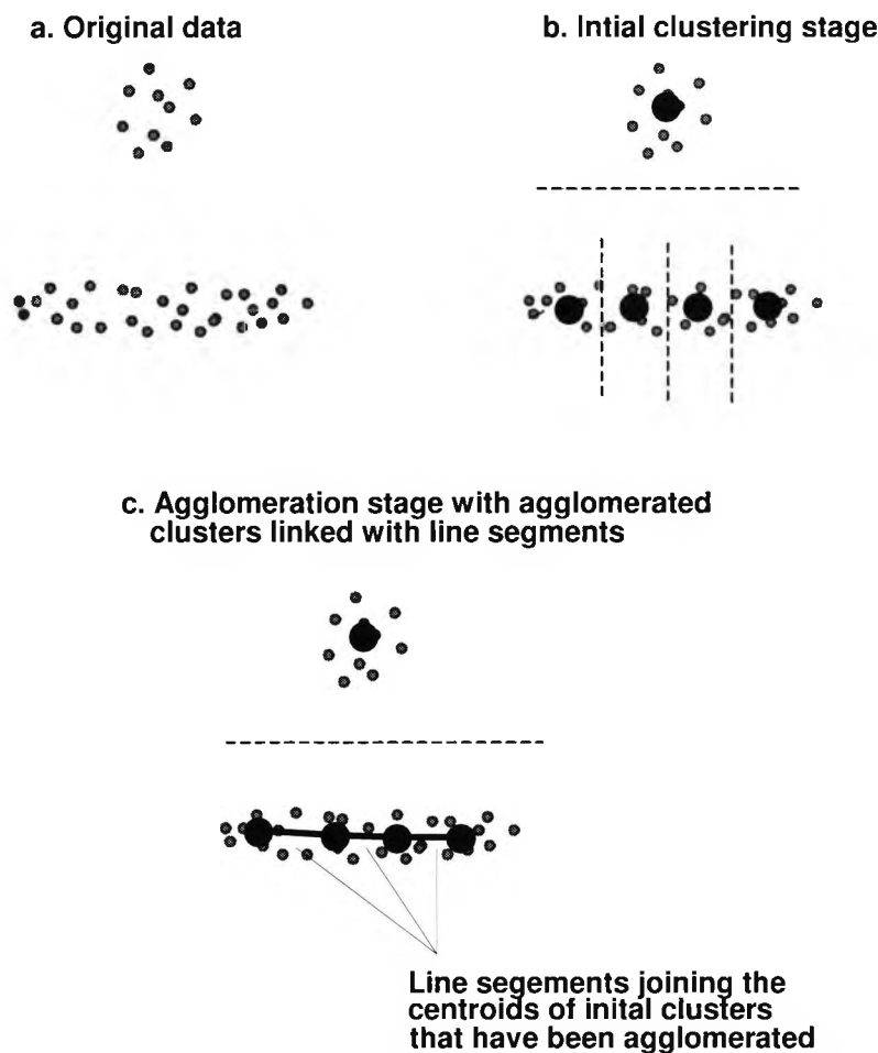
Figure 1.1: APC begins with an initial clustering of the data (a) using any standard pattern partitioning algorithm (b). The centroids of the resulting clusters (separated by dashed lines) are then presented to the agglomeration stage. The agglomeration stage (c) seeks to agglomerate initial clusters that are found in contiguous regions of high density as in the case of the elongated cluster at the bottom. Once agglomerated, the structure of the agglomerated clusters is represented by joining together with line segments the centroids of the initial clusters that are agglomerated into the new cluster.
