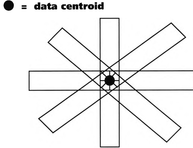
Figure 3.4: Type-I splitting involves searching strips of the pattern space for areas of low density. 4 strips are constructed corresponding the 2^d - 1 + d directions from the cluster centroid to be searched.
