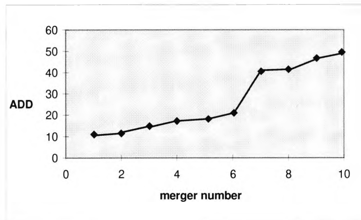
Figure 4.13: Plot of the ADD value at which clusters are agglomerated. The "elbow" at the 7th merger may be taken as a candidate point for stopping the agglomeration process and partitioning the data.
