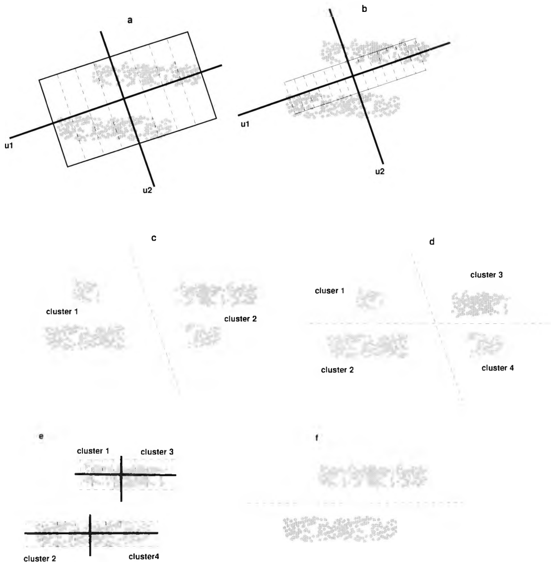
Figure 3.3: The Liu and Tsai (1989) approach begins with searching subregions along the axis determined by the largest eigenvector, u_1 (a). If no sparsely populated subregion is found, the size of the subregions is reduced which increases the likelihood of finding sparse areas. This is shown in (b) where reducing the size of the subregions has led to three sparsely populated subregions near the intersection of u_1 and u_2 . The data is then partitioned along the line the bisects the subregions orthogonal to u_1 . This process is repeated on the two resulting partitions which generates the four clusters shown in (d). As no further division of these clusters is possible, each pair of clusters is tested for merging. This leads to clusters 1 and 3 and clusters 2 and 4 being merged as when these clusters are tested using the same process used in stage 1 no partition is found to exist (e). The final result is the data partitioned into the two original hyperellipsoidal clusters (f).
