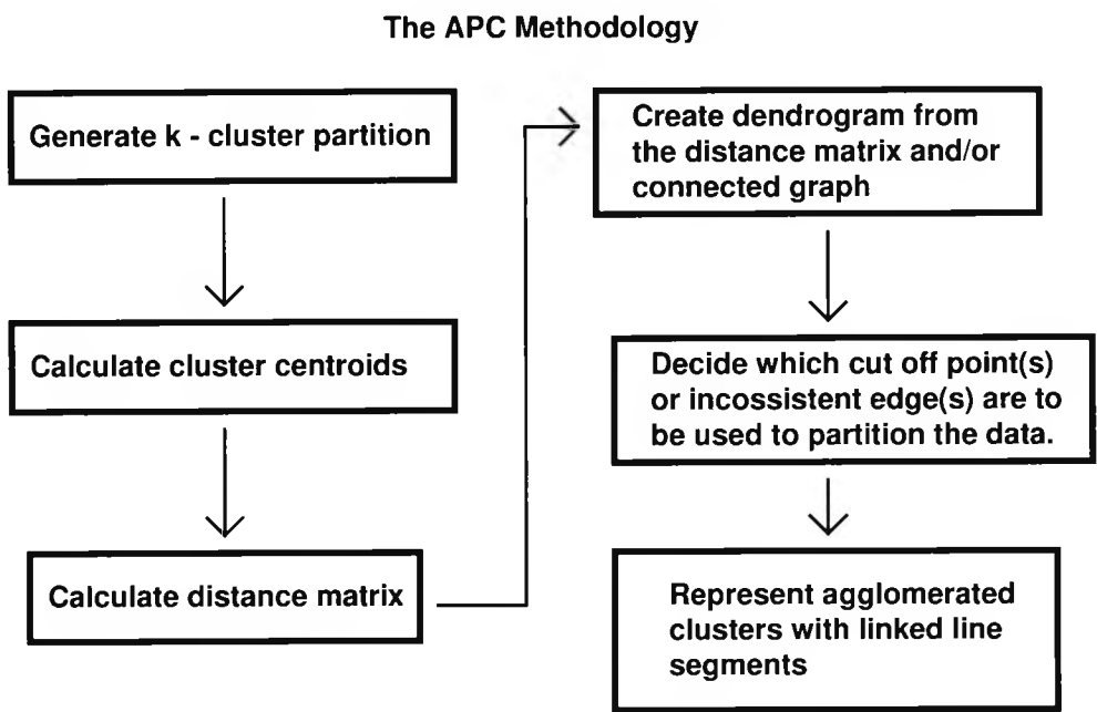
Figure 4.14: Flow chart of the APC methodology.
