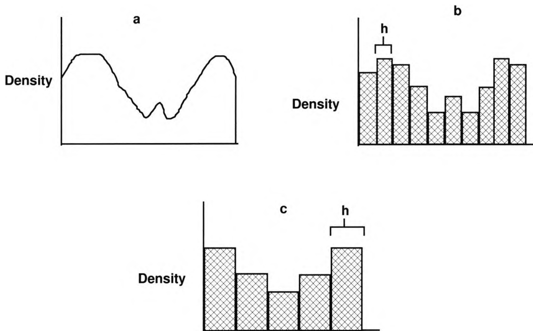
Figure 4.6: Increasing the bin size smooths the density estimate.
