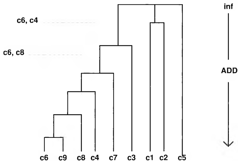
Figure 4.12: Dendrogram generated for Figure 4.11 by ADD. Note the dashed lines indicating agglomerations between initial cluster centroid that have already been agglomerated into the same cluster.
