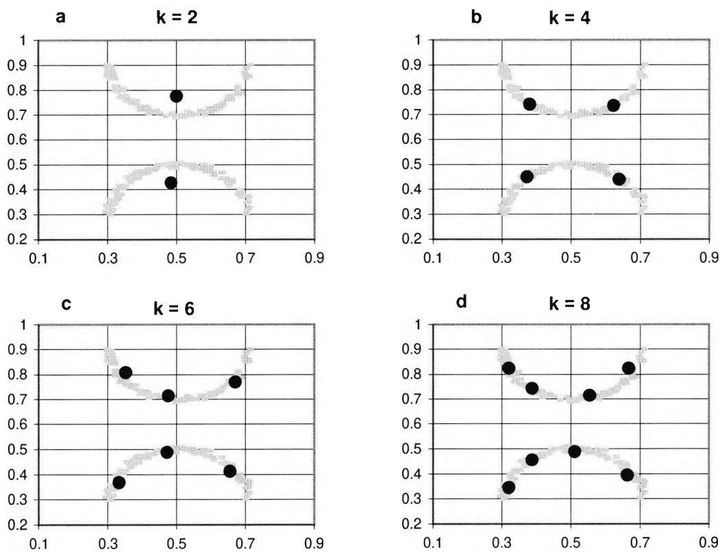
Figure 4.2: Increasing k increases the likelihood of correctly spanning the cluster shape.
