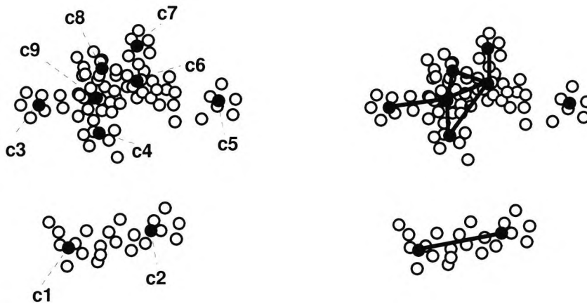
Figure 4.11: A three cluster problem and the APC representation of cluster structure. The heavy dots are the centroids of the initial clusters found in the pattern partitioning stage and the heavy lines indicate agglomerations between initial clusters. Note that the agglomeration between clusters can occur at any time between any two clusters that have not already been agglomerated together even if the two particular initial clusters have already been agglomerated into the same cluster but not with each other.
