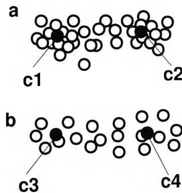
Figure 4.3: ADD and UDD will agglomerate the clusters in this figure in different orders as they measure intercluster density differently.
