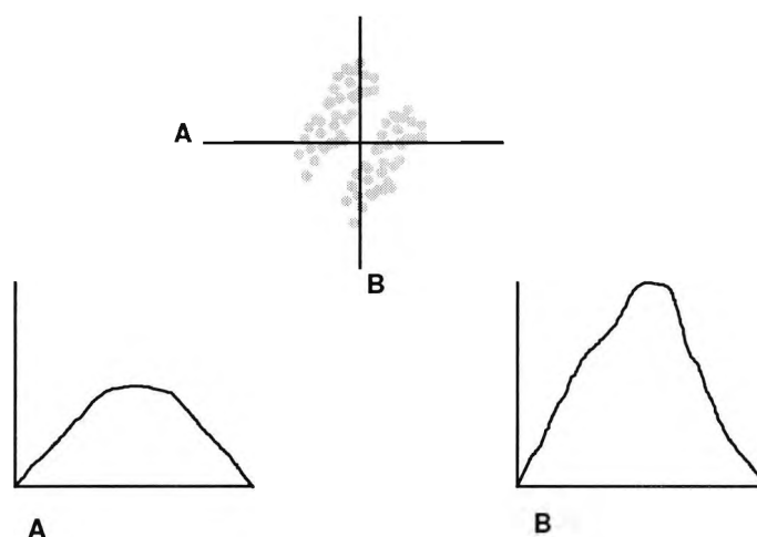
Figure 3.2: Potential problem with moment preserving clustering.
