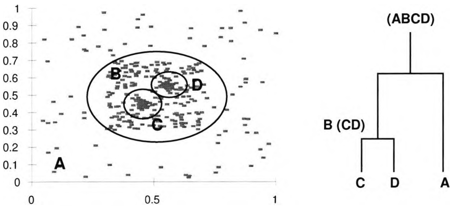
Figure 2.3: A density contour tree created from this data set. With f_t = 0 , all of the clusters are treated as a single cluster. As f_t increases, the different clusters begin to separate. Initially, cluster A (the surrounding low density area) is separated from cluster B, the high density square. Increasing f_t further, causes clusters C and D to be separated from cluster B. The density based relationships between clusters can be represented with the hierarchical tree (dendrogram - see Chapter 3) on the right.
