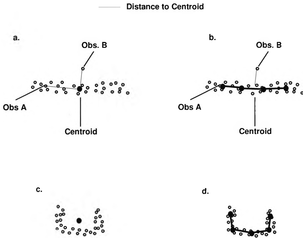
Figure 1.2: The use of the linked line segment representation ( b and d ) allows for more accurate measurements of how individual patterns reside within a cluster compared to using the centroid of the cluster ( a and c ).
