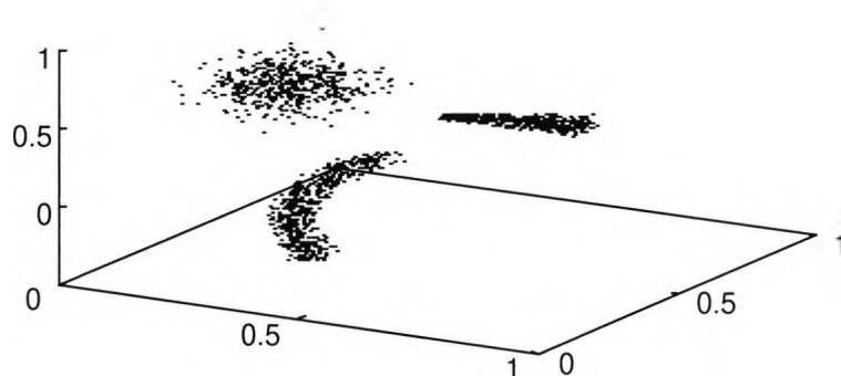
Figure 6.1: Cluster shapes: hyperellipsoid, arc and cone used in this evaluation.
