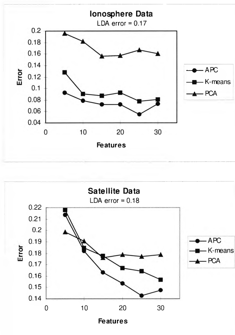
Figure 8.5 The relative performances of the three feature extraction methods on the ionosphere and satellite data.
