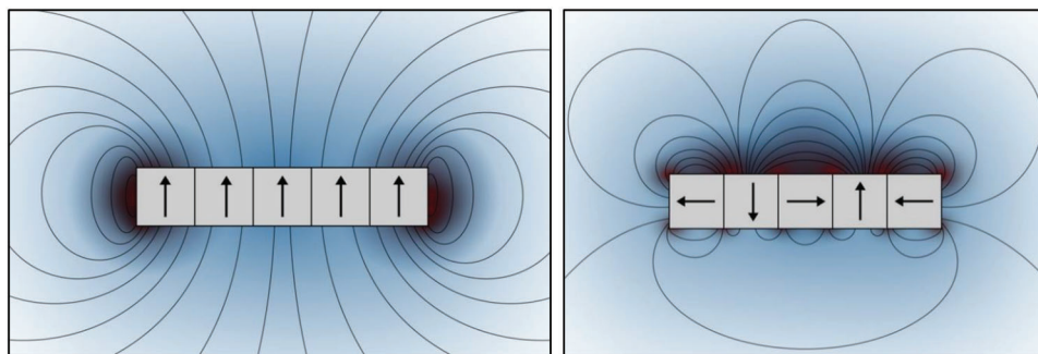
Figure 1. Single row magnet on the left and Halbach array on the right.
