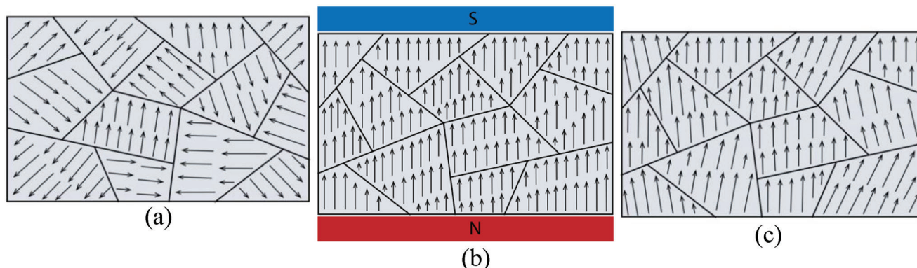
Figure 2. a) Domains in the iron section before the magnetic field was applied. b) Domains in the iron section while the magnetic field is applied and c) domains in the iron section after the magnetic field was removed.
