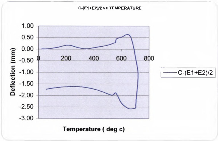
Figure 7.5.2 Centre less average end deflection vs. Average concrete temperature Beam (N/0.5/C1/HM)
