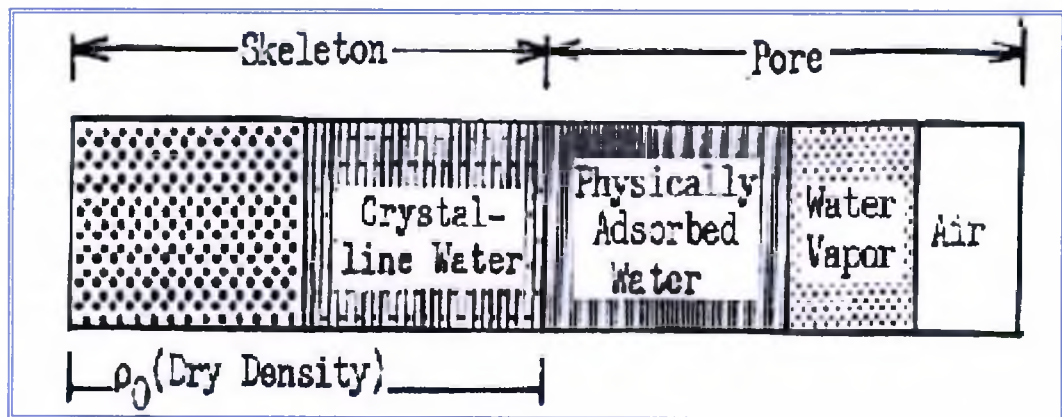
Figure 4.3 Model of concrete for Harada's program.
