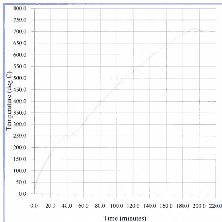
Figure 6.4 Time - Temperature Curve for Low Rate of Heating
