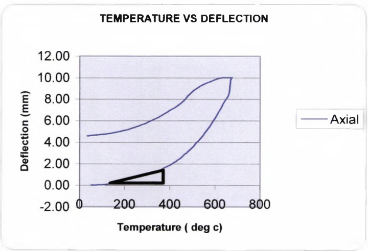
Figure 7.4.2 Relationship between axial expansions vs. Average concrete temperature Beam (M/0.25/HM/F2)
