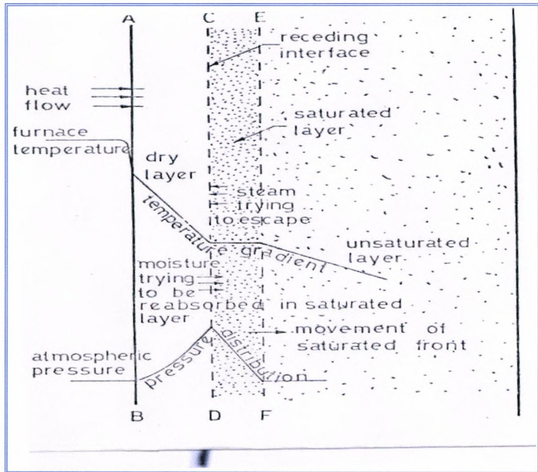
Figure 4.1 Formation of moisture clog when heated from one side (Ref.4.14)
