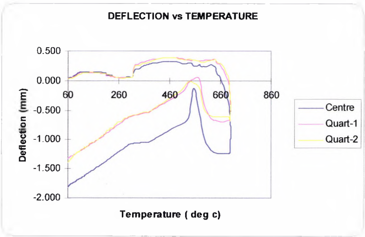
Figure 7.3.2 Centre and quarter point deflections vs. Average concrete temperature Beam (L0.35/00/HM/F3)
