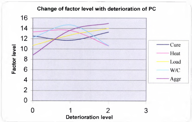
Figure 8.2a Change of factor level with deterioration of P.C
