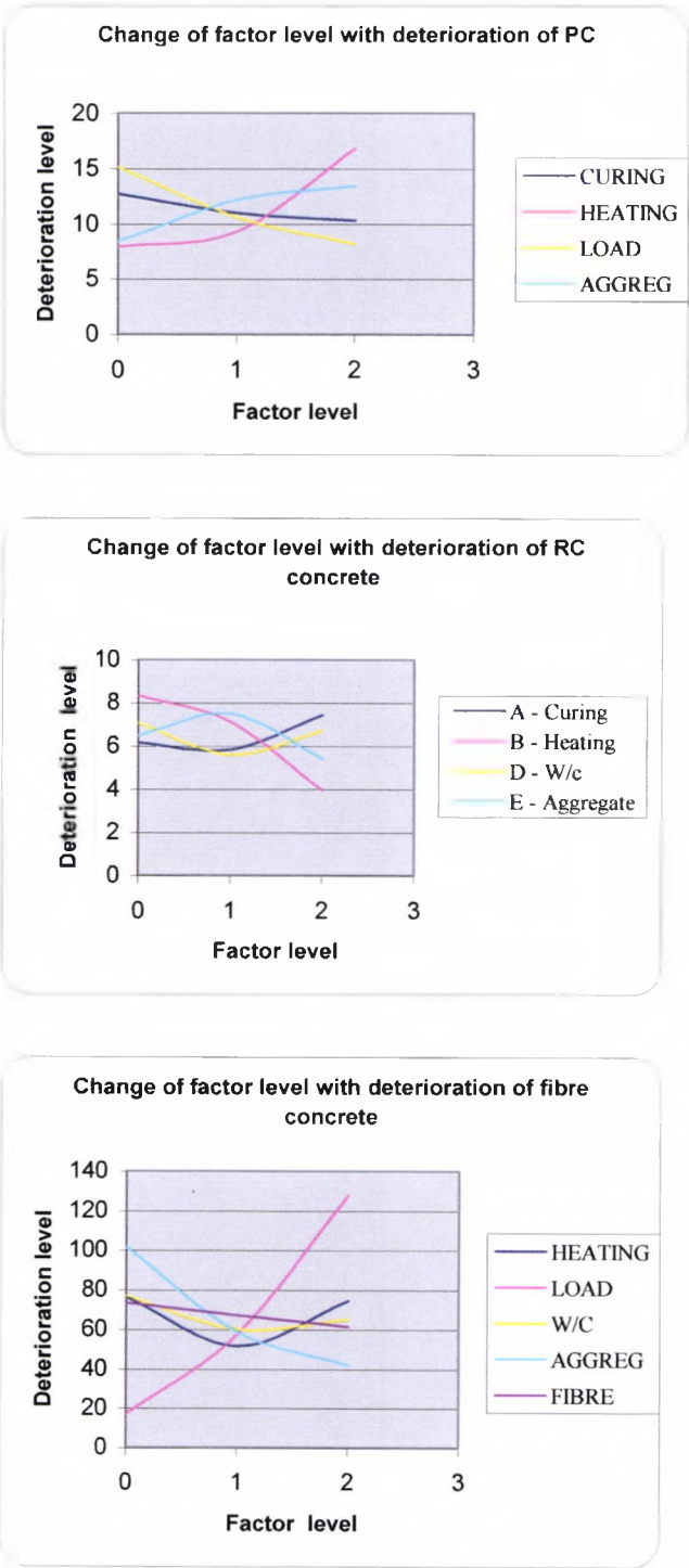
Figure 8.2 Change of factor level with deterioration of PC, RC, and FC
