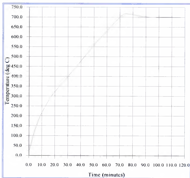
Figure 6.3 Time - Temperature Curve for Medium Rate of Heating
