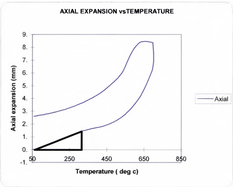
Figure 7.3.1 Relationship between axial expansions vs. Average concrete temperature Beam (L0.35/00/HM/F3)
