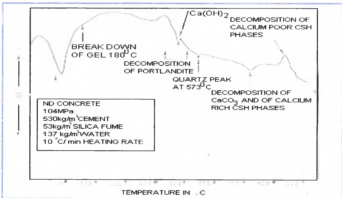
Figure 1.1. Sketch of a thermograph of ND concrete with compressive cylinder strength of 104Mpa
