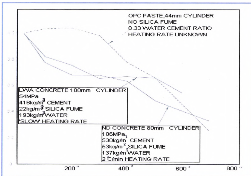
Figure 1.2. Response of high strength lightweight and high strength normal weight concrete to fire
