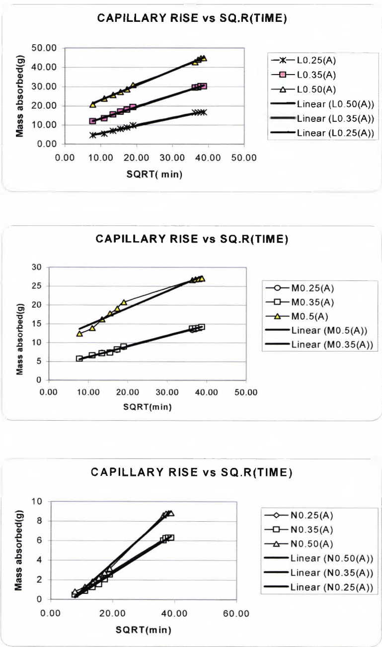
Figure 7.1 Capillary rise of limestone (N), modified normal (M) and LWA (L) concrete.
