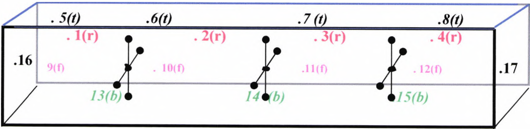
Figure 6.5 Sketch of thermocouple positioning within beam (15) and on beam (17)
