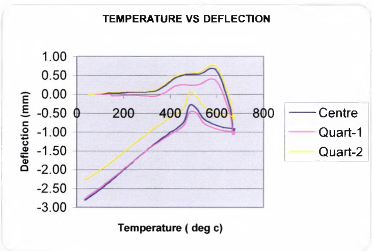
Figure 7.4.1 Center and quarters vs. Average concrete temperature Beam (M/0.25/HM/F2)
