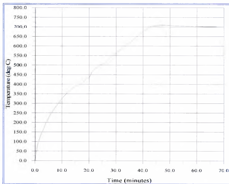
Figure 6.2 Time - Temperature Curve for High Rate of Heating
