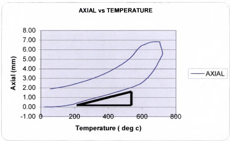
Figure 7.5.1 Relationship between axial expansions vs. average concrete temperature Beam (N/0.5/C1/HM)
