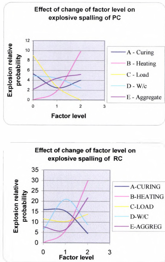
Figure 8.1 Effect of factor level on explosive spalling of PC and RC
