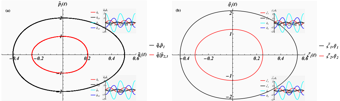
Figure 11: Affine G_2 -Toda lattice \tilde{H} and \tilde{Q}_6 phase spaces for the variables (\tilde{q}_i, \tilde{p}_i) , i = 1, 2, 3 and (\tilde{\zeta}_i, \tilde{\eta}_i) , i = 1, 2 as functions of t panel (a) and panel (b), respectively. The initial conditions are taken in both cases as \tilde{q}_1(0) = \tilde{q}_2(0) = \tilde{q}_3(0) = 0 , \tilde{p}_1(0) = 2 , \tilde{p}_2(0) = \tilde{p}_3(0) = -1 and \tilde{\zeta}_1(0) = \tilde{\zeta}_2(0) = 0 , \tilde{\eta}_1(0) = 3/\sqrt{2} and \tilde{\eta}_2(0) = -\sqrt{3}/\sqrt{2} .
