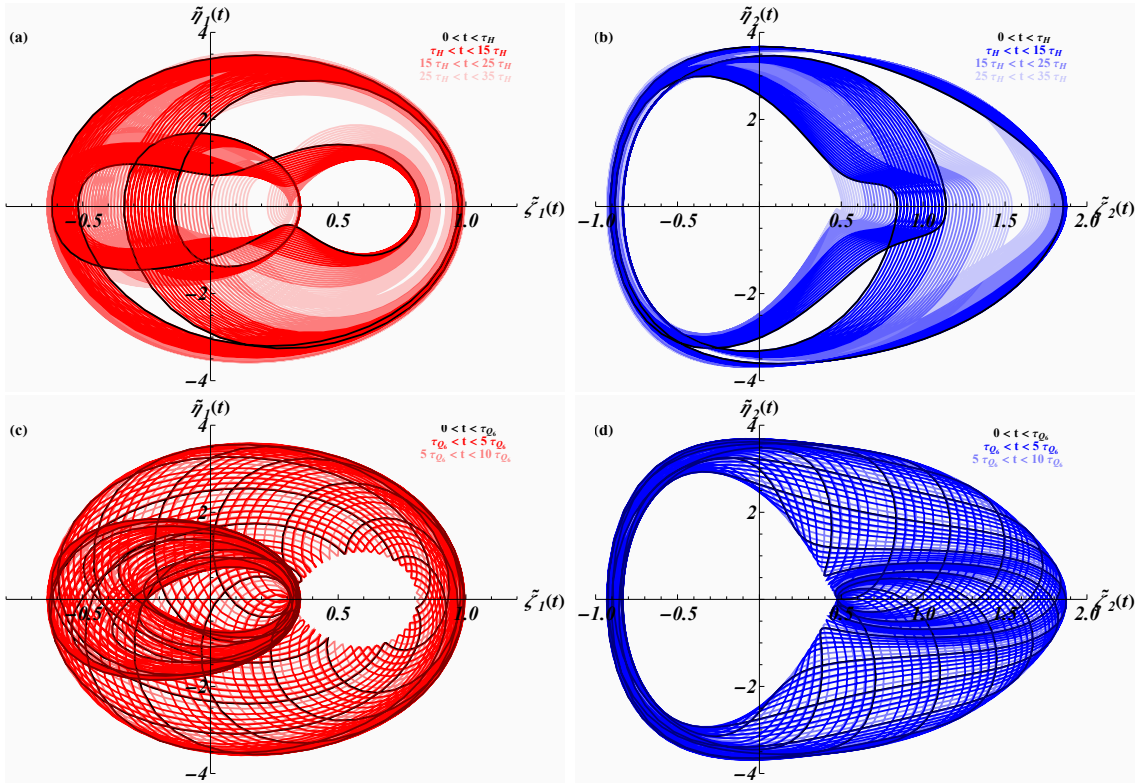
Figure 10: Affine G_2 -Toda lattice \tilde{H} and \tilde{Q}_6 phase spaces for the variables (\tilde{\zeta}_i, \tilde{\eta}_i) , i = 1, 2 as functions of t panels (a), (b) and panels (c), (d), respectively. The initial condition are taken in both cases as \tilde{\zeta}_1(0) = \tilde{\zeta}_2(0) = 0 , \tilde{\eta}_1(0) = 3/2\sqrt{2} and \tilde{\eta}_2(0) = -\sqrt{3}/2\sqrt{2} .
