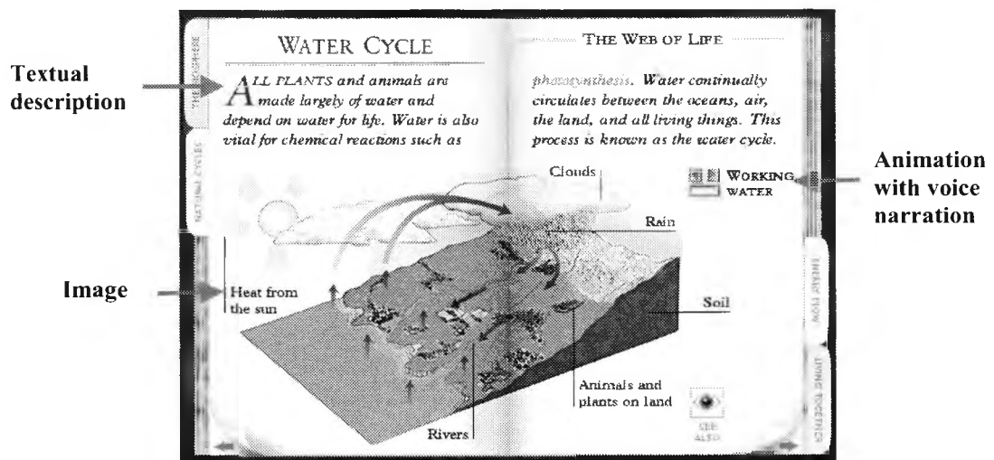
Figure 1: Water Cycle (from DK© Encyclopaedia of Nature)
