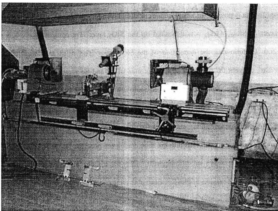
Figure 5.1 Photos of MCVD apparatus for fibre preform fabrication (a) MCVD Chamber (b) MCVD lathe
