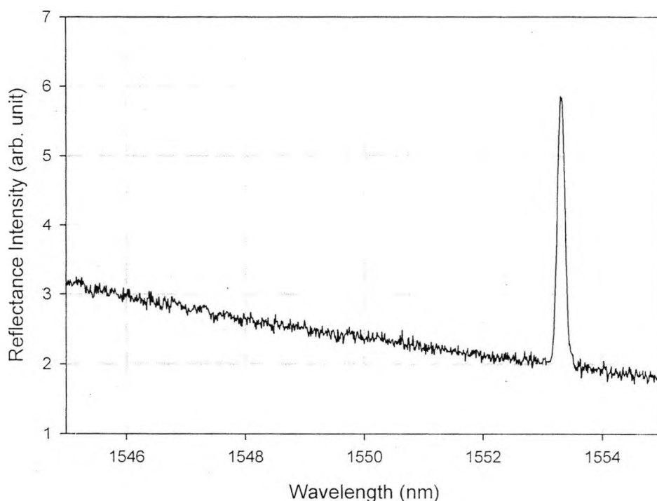
Figure 5.5 The reflectance spectra of an FBG written into the Sb/Er/Ge fibre at 900^{\circ}\text{C} , after long term annealing from room temperature to 850^{\circ}\text{C} . The time period of the annealing is 24 hours at each hundred degree Celsius point below 850^{\circ}\text{C} .
