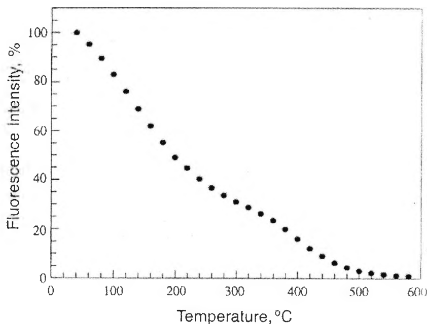
Figure 2.17 The ruby fluorescence intensity recorded in the experiment (after Ref.30)
