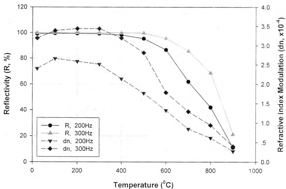
Figure 6.4 Annealing results for two FBGs (with laser parameters of 200 mJ/cm 2 per pulse and repetition rates of 200 Hz and 300 Hz respectively) written into In-Ge fibre, with temperature, from room temperature to 900 °C, showing the change in reflectivity (R) and the refractive index modulation (dn) with temperature. For each data in each curve, the annealing period is 24 hours.
