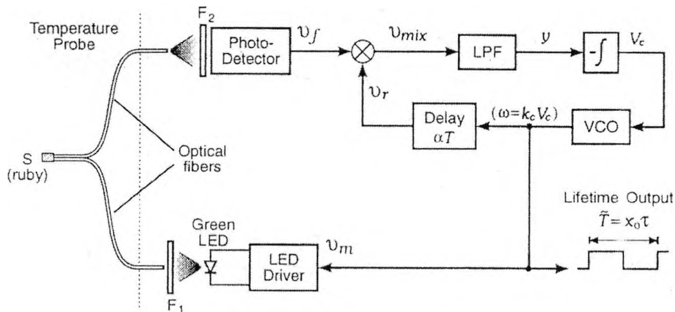
Figure 2.15 The ruby fluorescence lifetime based fibre optic thermometer system.
