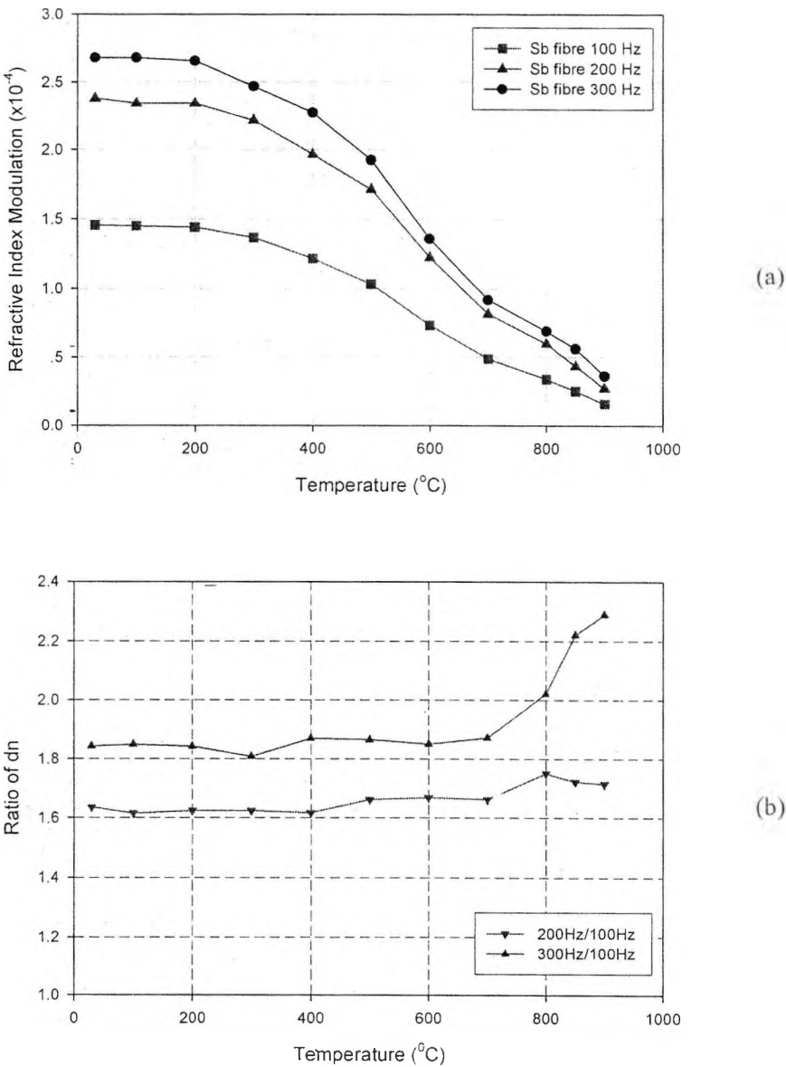
Figure 6.7 (a). Decay of the refractive index modulation ( dn ) of FBGs written into the Sb/Gc fibre after annealing at different temperatures. The annealing time was 24 hours at each temperature. (b) Ratio of dn after annealing. The ratio was obtained for dn in the FBGs written at 300 Hz and 200 Hz when divided by dn for the FBGs written at 100 Hz
