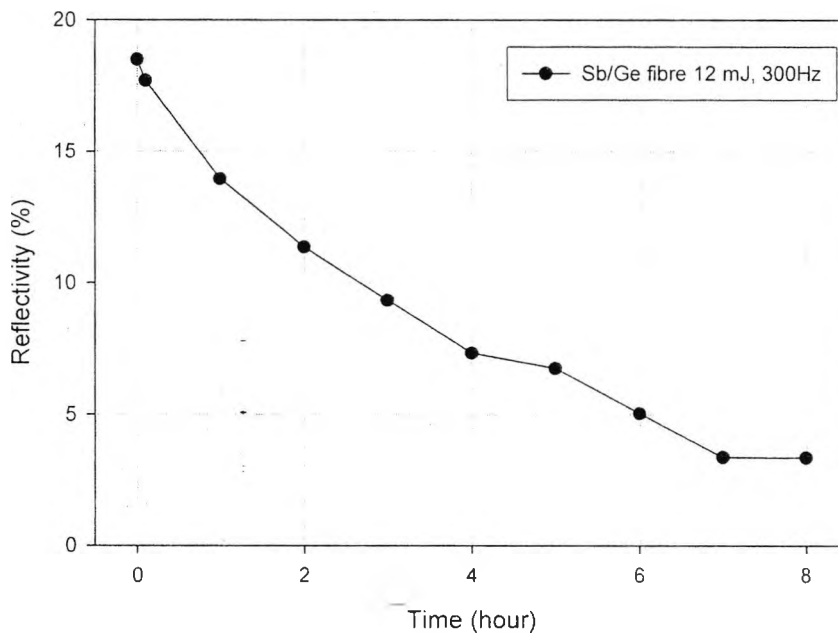
Figure 5.13 Reflectivity decay of an FBG written into the Sb/Ge fibre with time, in an oven operating at 950^{\circ}\text{C} , where the data were recorded continually for 8 hours until the reflectivity decreased to a value of 3.4%.
