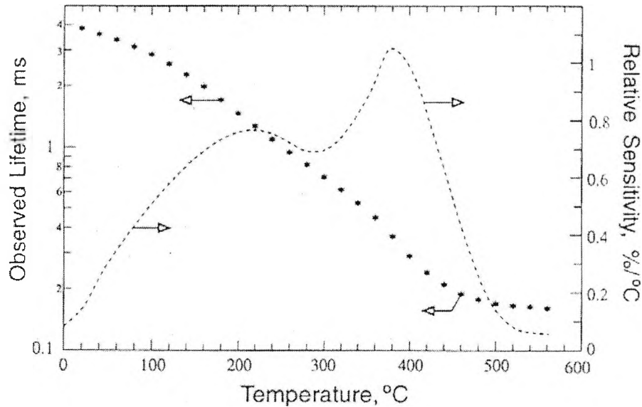
Figure 2.16 Characteristic calibration curve for the ruby fluorescence based thermometer in the region from room temperature to \sim 550 ^{\circ}\text{C} (after Ref.28)
