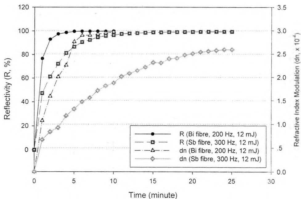
Figure 6.2 Reflectivity (R) and refractive index modulation (dn) increase for FBGs written into Bi-Ge fibre and Sb-Ge fibre when using a UV excimer laser with parameters of 200 mJ/cm 2 per pulse, and repetition rates of 200 Hz and 300 Hz respectively
