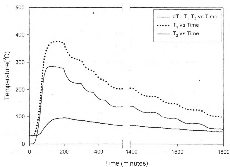
Figure 7.9 Temperature changes of the probes with time when silica powder was used as the medium, (a) with the fluorescence lifetime based fibre thermometer, System A and (b) with the FBG-based fibre-optic sensor, System B
