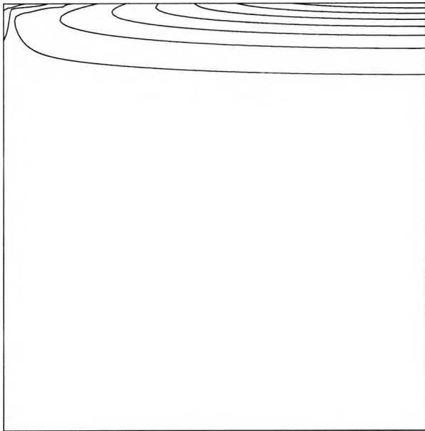
Figure 3.14: Isotherms from the numerical calculation for R = 5000 and L = 1
