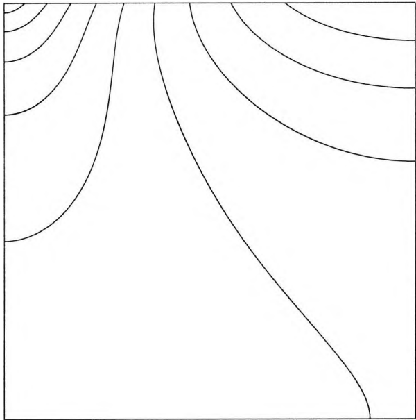
Figure 3.6: Isotherms from the numerical calculation for R = 30 and L = 1
