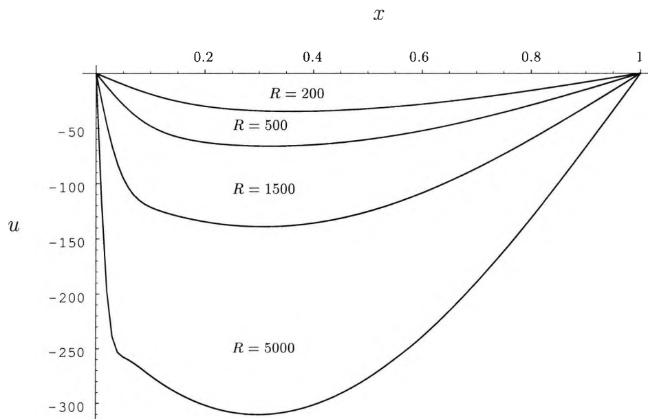
Figure 2.26: Slip velocity u for L = 1 and different values of R at the upper boundary z = 1 from the numerical calculation
