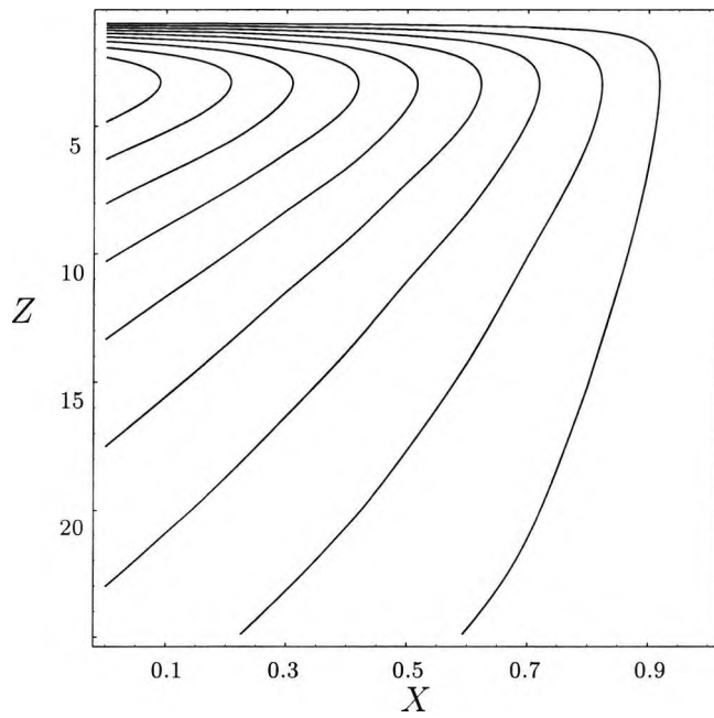
Figure 6.20: Streamlines from the numerical solution of the horizontal boundary layer equations
