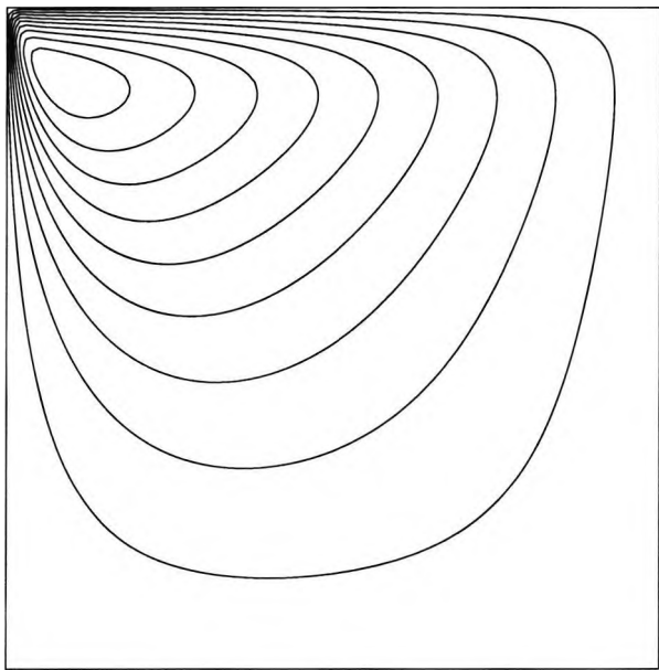
Figure 6.11: Streamlines from the numerical calculation for R = 5000 and L = 1
