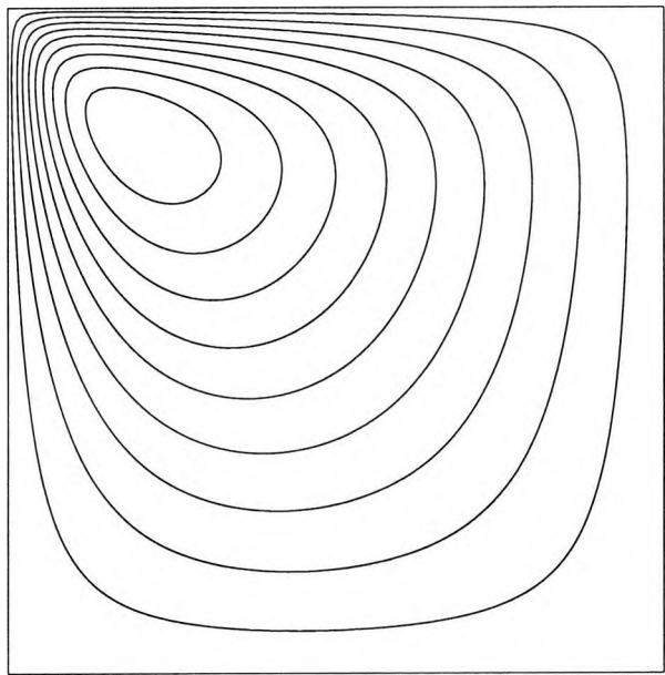
Figure 3.11: Streamlines from the numerical calculation for R = 500 and L = 1
