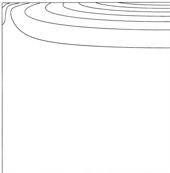
Figure 3.12: Isotherms from the numerical calculation for R = 1500 and L = 1
