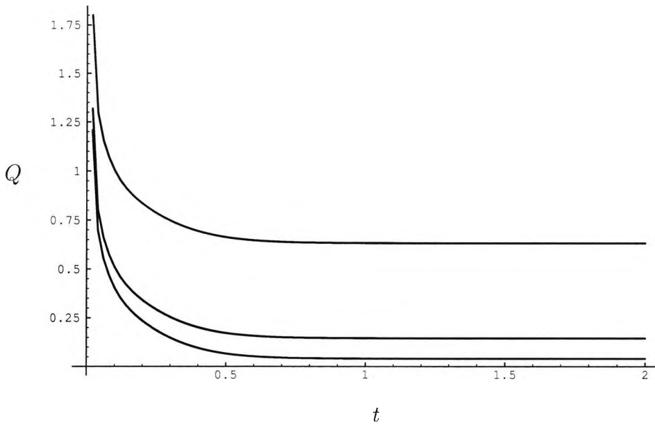
Figure 2.9: Total heat flux Q across the upper boundary for L = 1 and R=500 versus t for different grid sizes where the upper curve is for h = 0.05, k = 0.05 , the middle curve for h = 0.02, k = 0.02 and the lower curve for h = 0.01, k = 0.01 .
