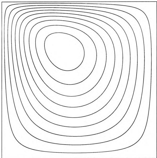
Figure 3.7: Streamlines from the numerical calculation for R = 30 and L = 1
