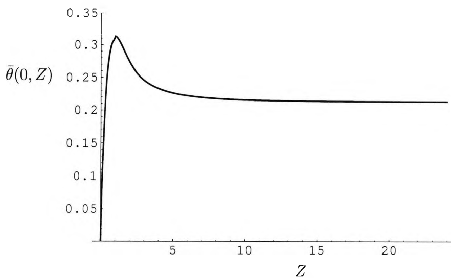
Figure 6.17: Temperature at X = 0 from the numerical solution of the horizontal boundary layer equations
