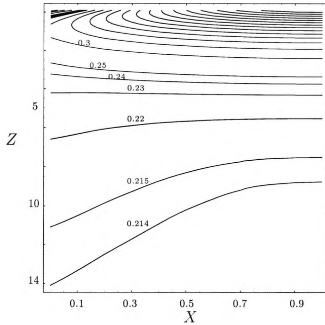
Figure 6.19: Isotherms from the numerical solution of the horizontal boundary layer equations. The upper contours are at intervals of 0.05 in \bar{\theta}
