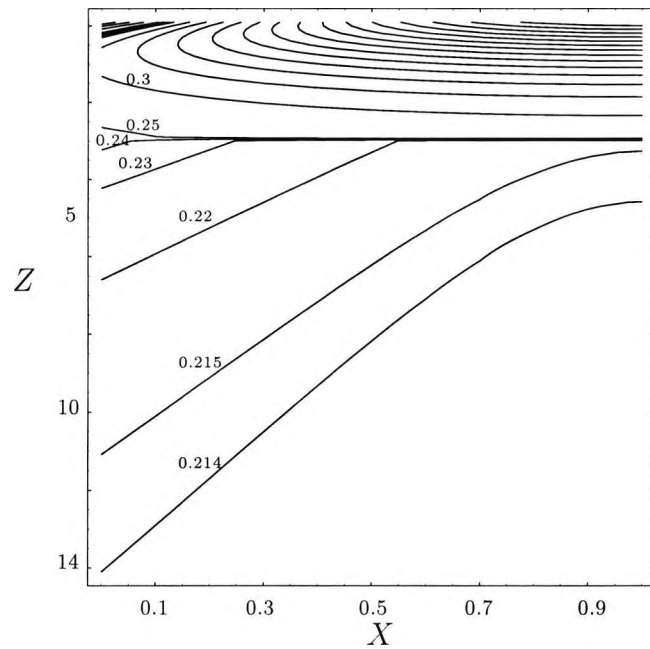
Figure 6.15: Isotherms in the horizontal boundary layer. The upper contours are at intervals of 0.05 in \bar{\theta} .
