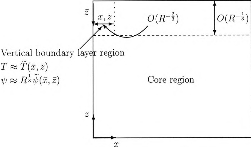
Figure 5.1: Vertical boundary layer region
