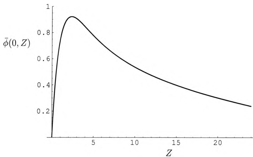
Figure 6.18: Stream function at X = 0 from the numerical solution of the horizontal boundary layer equations
