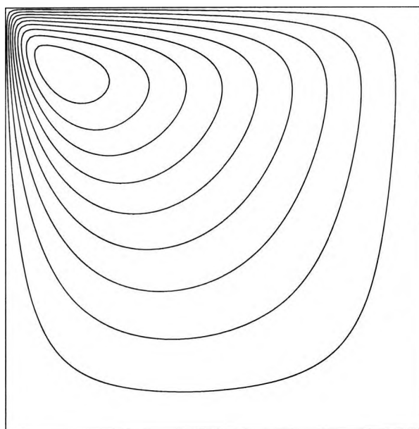
Figure 3.13: Streamlines from the numerical calculation for R = 1500 and L = 1
