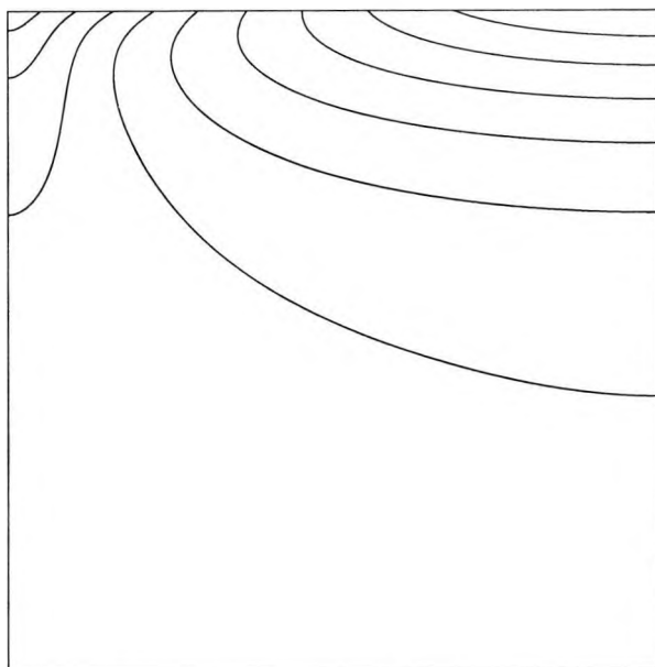
Figure 3.8: Isotherms from the numerical calculation for R = 200 and L = 1
