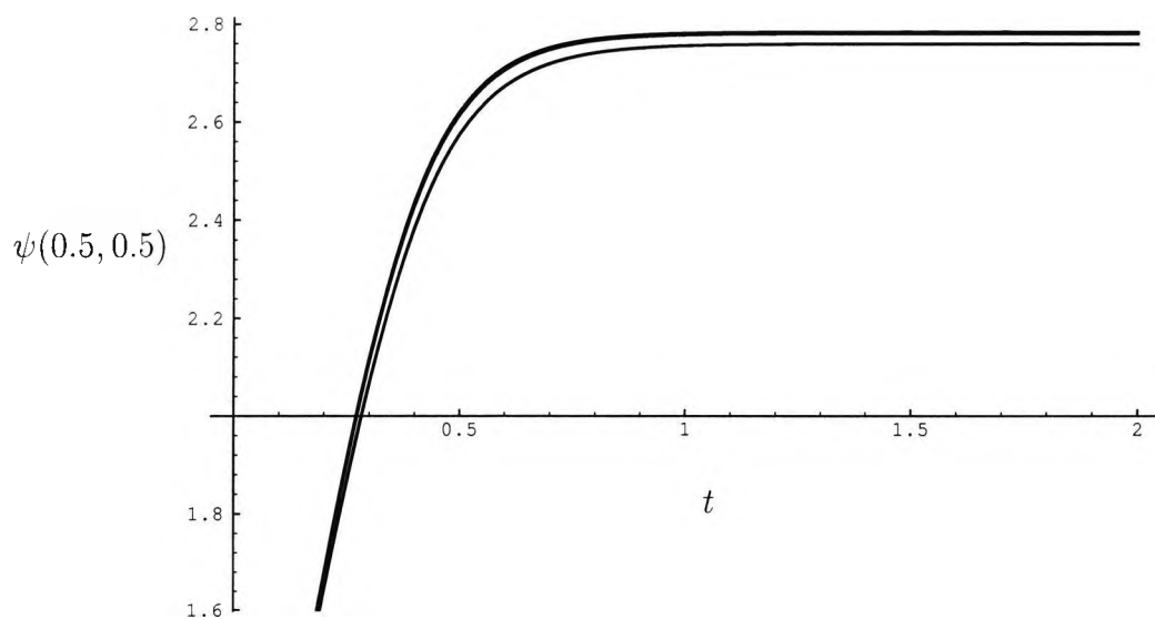
Figure 2.12: Value of the stream function at the centre of the cavity for L = 1 and R = 20 versus t for different grid sizes, where the upper curves are for h = 0.01, k = 0.01 and h = 0.02, k = 0.02 , and the lower curve for h = 0.05, k = 0.05 .
