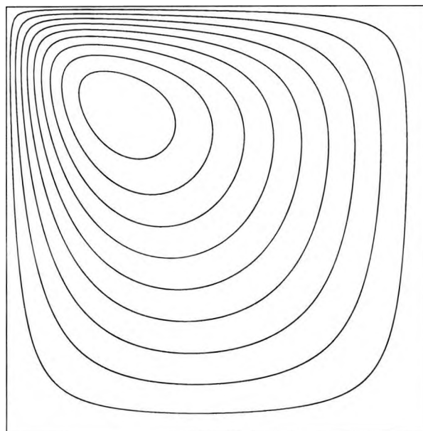
Figure 3.9: Streamlines from the numerical calculation for R = 200 and L = 1
