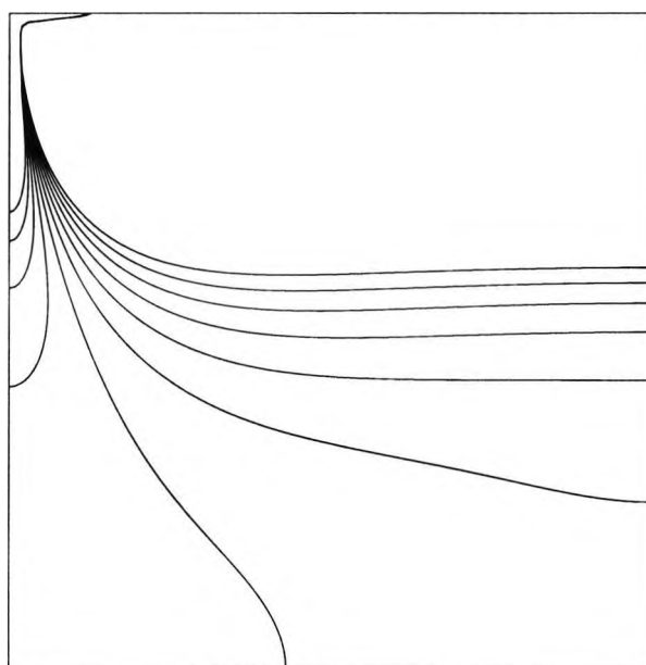
Figure 3.16: Isotherms between 0.23 and 0.24 from the numerical calculation for R = 5000 and L = 1
