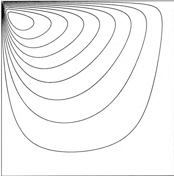
Figure 3.15: Streamlines from the numerical calculation for R = 5000 and L = 1
