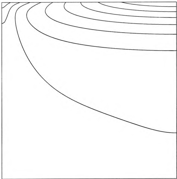
Figure 3.10: Isotherms from the numerical calculation for R = 500 and L = 1
