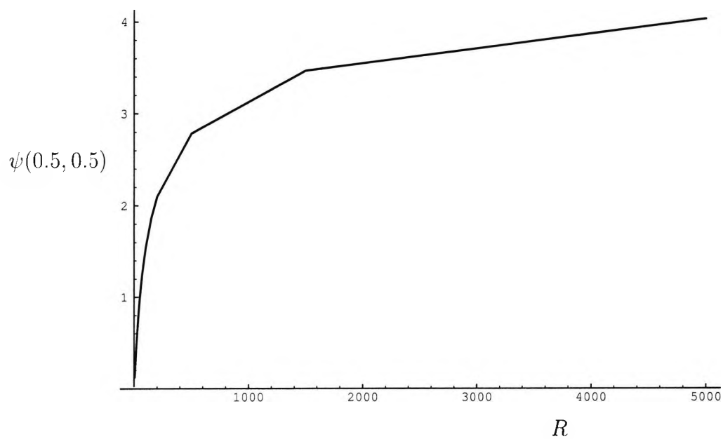
Figure 2.33: Temperature at the centre of the cavity versus R from the numerical calculation for L = 1
