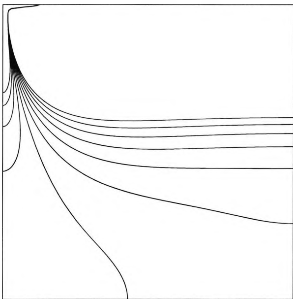
Figure 6.10: Isotherms between 0.23 and 0.24 from the numerical calculation for R = 5000 and L = 1
