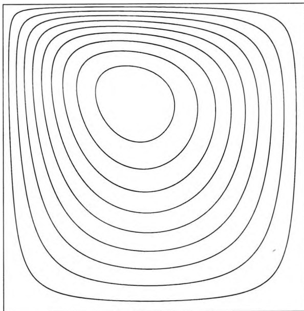
Figure 3.5: Streamlines from the numerical calculation for R = 5 and L = 1
