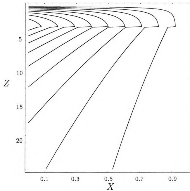
Figure 6.16: Streamlines in the horizontal boundary layer
