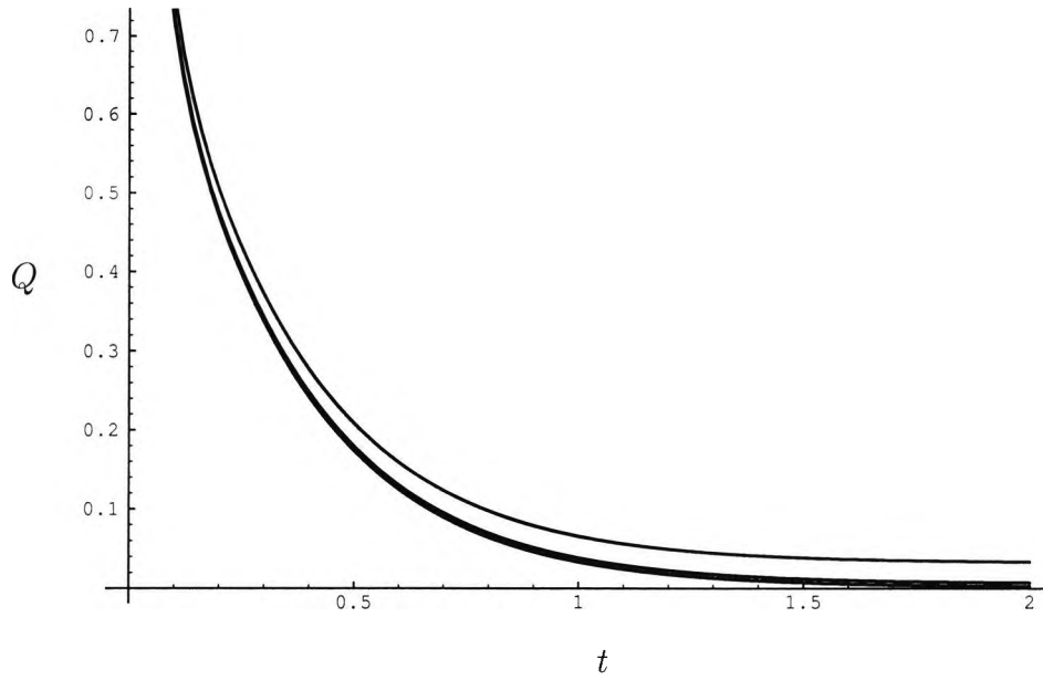
Figure 2.8: Total heat flux Q across the upper boundary for L = 1 and R=20 versus t for different grid sizes where the upper curve is for h = 0.05, k = 0.05 , the middle curve for h = 0.02, k = 0.02 and the lower curve for h = 0.01, k = 0.01 .
