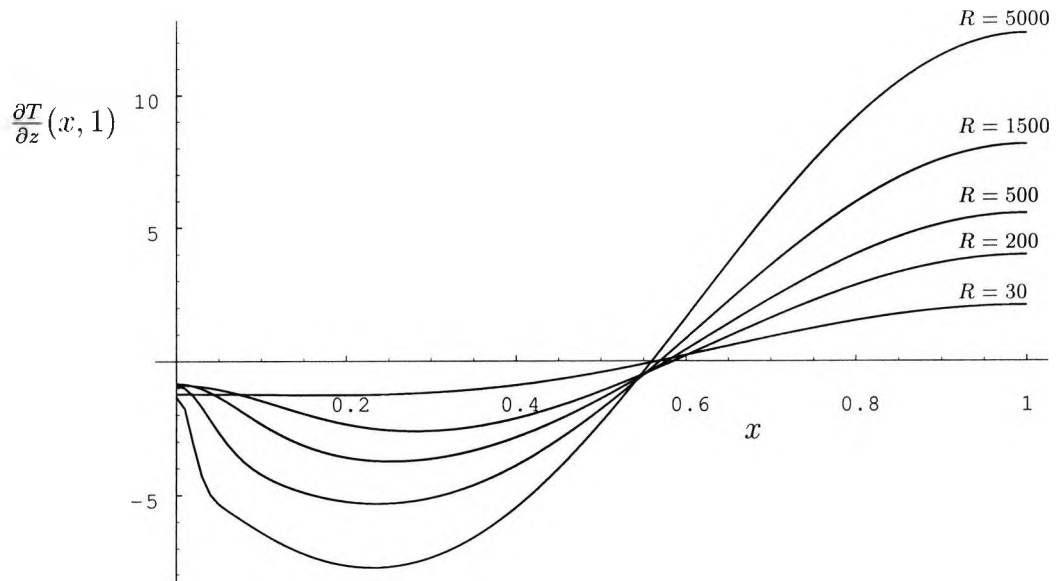
Figure 2.28: Local heat flux at the upper boundary z = 1 from the numerical calculation for L = 1 and different values of R .
