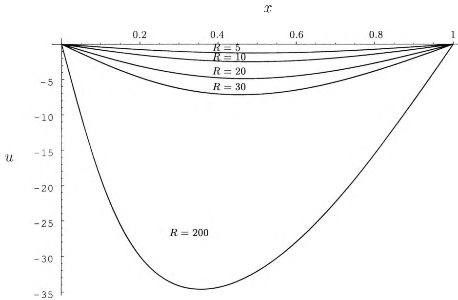
Figure 2.25: Slip velocity u for L = 1 and different values of R at the upper boundary z = 1 from the numerical calculation
