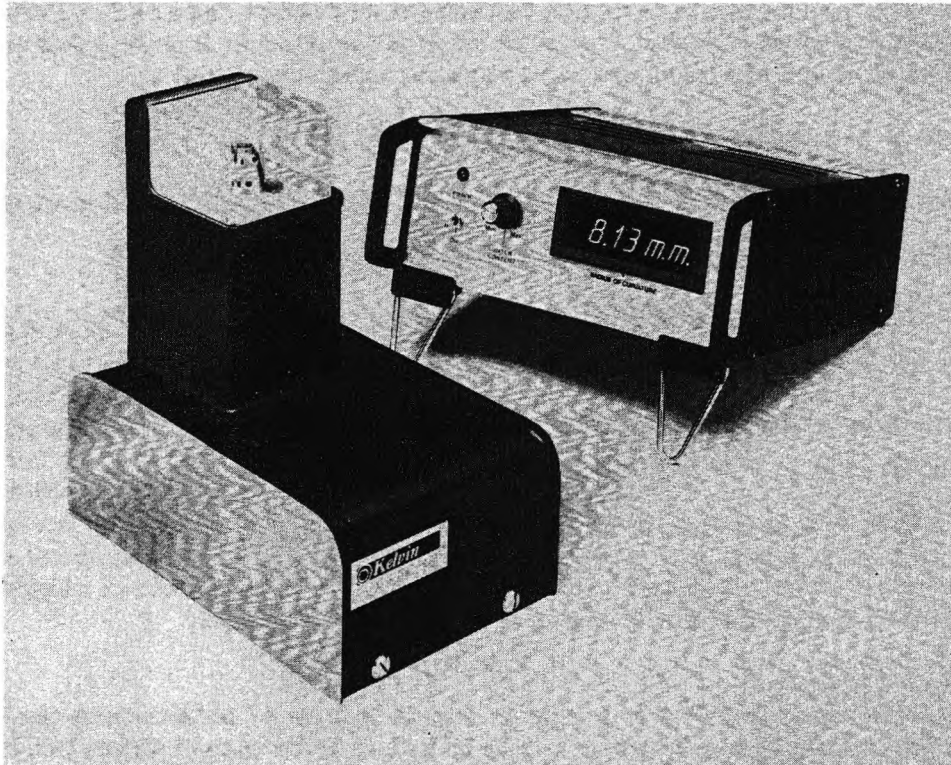
Fig. 2. The two main units of the Kelvin measurement system. On the left is the wet cell together with the motorized probe mechanism and on the right the unit housing the control system and digital read-out.
