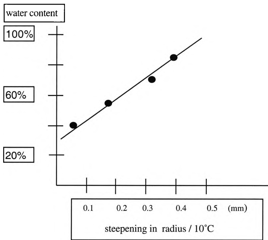
Figure 5.1 The steepening effect of temperature on hydrogel materials of different water content
