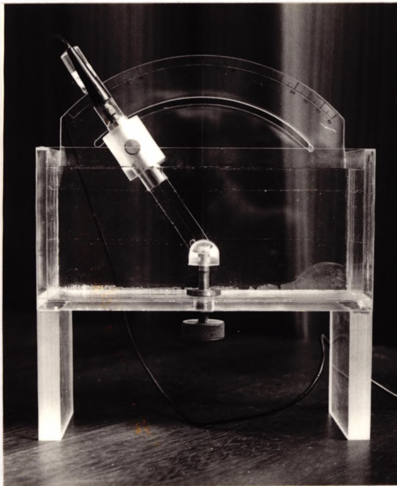
Figure 5.5.1 Front elevation of apparatus used to investigate the topography of lens surfaces. The PMMA hemisphere is shown in position and this is adjusted vertically by the brass knurled knob underneath.
