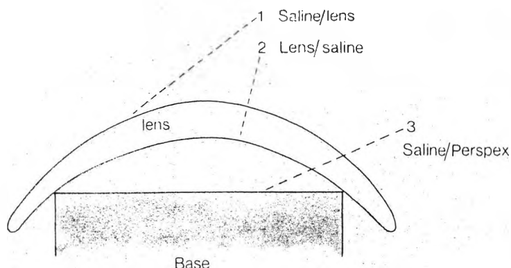
Fig 5: Interfaces 'detected' by ultrasonic beam
