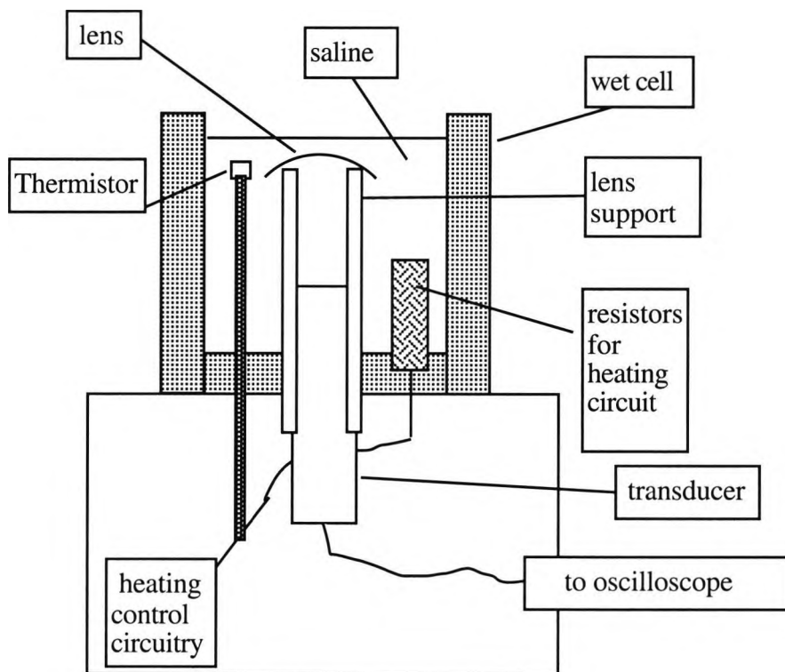
Figure 4.5 Diagrammatic version of the final design to measure the BOZR of soft lenses.
