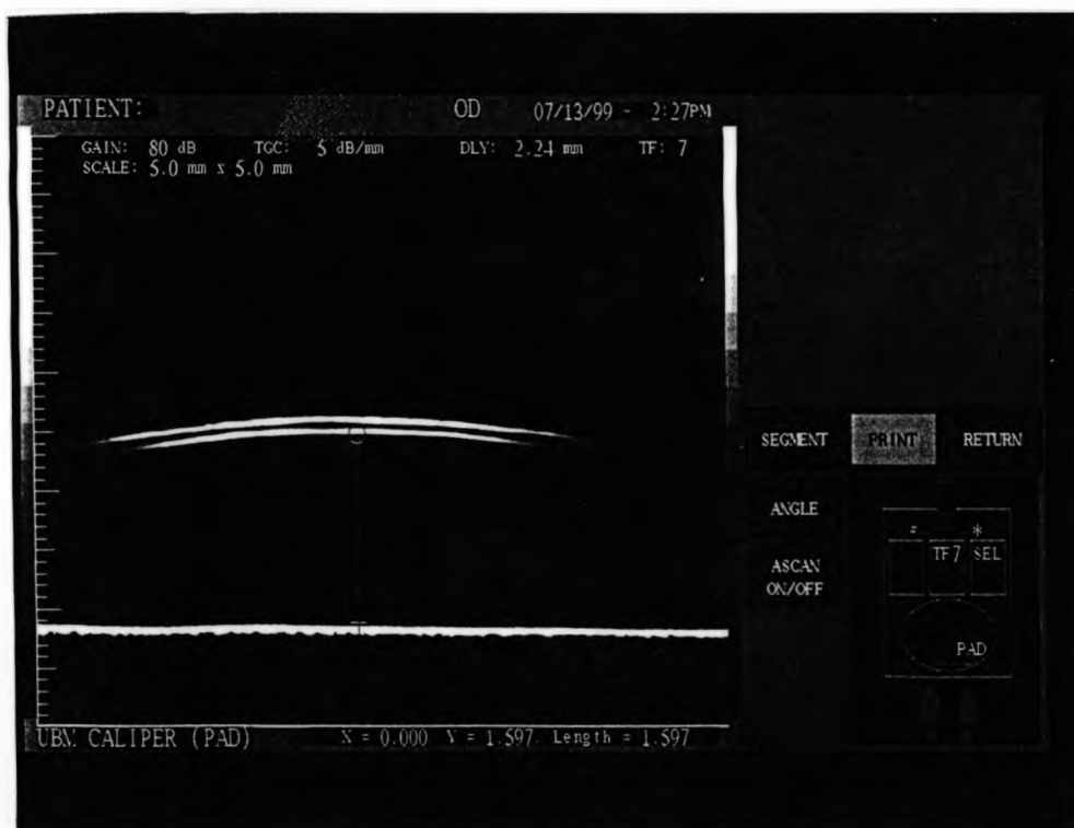
Figure 5.3.2 A USM image used to assess the sagitta of a contact lens back (concave) surface. The cursor used to obtain the raw sag data is shown. The sag value (mm) would be 1.597 multiplied by the conversion factor 1.387 for the example shown in this figure.
