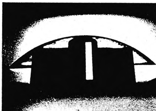
Figure 10.7 The back optic zone radius of a soft lens being measured on an Optimec device. The soft lens is resting on the 10 mm cylinder and the central probe can be seen near the back vertex of the lens. It is also possible to assess the edge profile of the lens.
