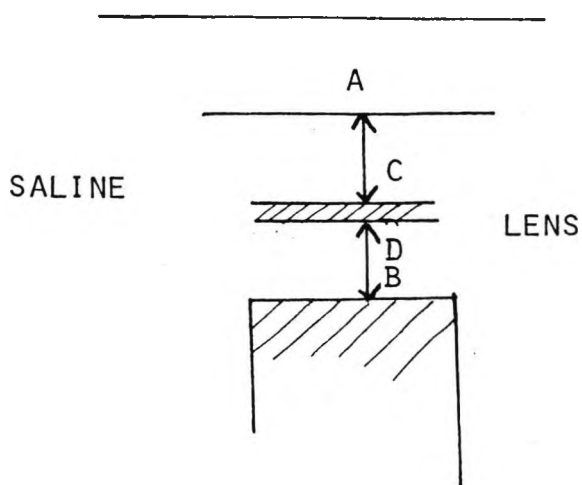
Figure 10. CD = AB - (AC + BD) . AB = RTT_1 \times V/2 . AC = RTT_2 \times V/2 . BD = RTT_3 \times V/2 . CD (lens thickness) = V/2 \cdot [RTT_1 - (RTT_2 + RTT_3)] . V = velocity of sound in saline at known temperature. A and B are reference surfaces or points. C and D are the contact lens surfaces.
