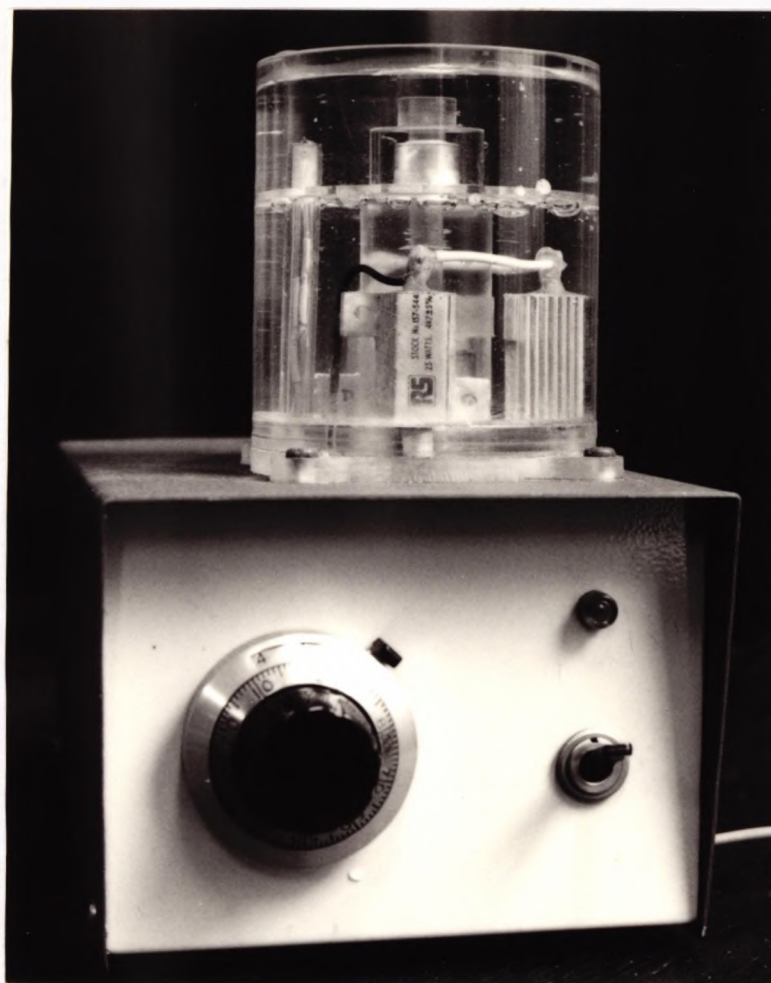
Figure 4.7 Front view of the final apparatus showing the saline filled wet cell on the top of a metal box which housed the saline heating circuitry. The temperature control is shown on the left side of the front panel.
