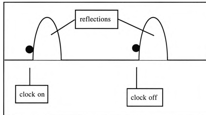
Fig. 2.3.2 The use of an interval counter to measure the RTT between two reflections visualised on the oscilloscope. The trigger points can be on any selected corresponding parts of the reflection envelopes
