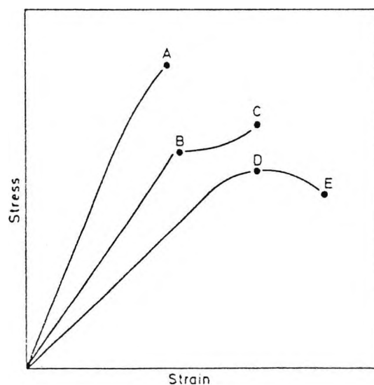
Figure 1.2 Stress-strain curves for three materials: (A) tensile strength and elongation at break; (B) tensile stress and elongation at yield; (C) tensile strength and elongation at break; (D) tensile strength and elongation at yield; (E) tensile stress and elongation at break. From Bier and Lowther, 1977.
