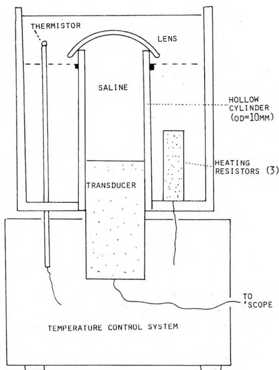
Figure 6. Latest design of measurement cell and temperature control system.
