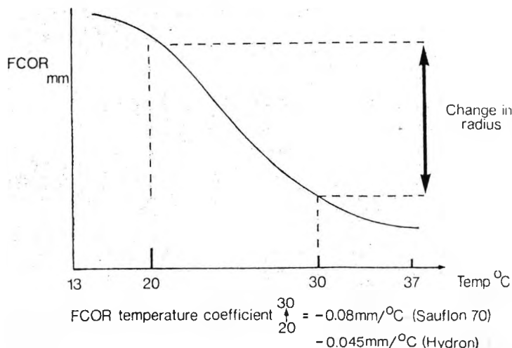
Fig 8: Effect of temperature on the FCOR
