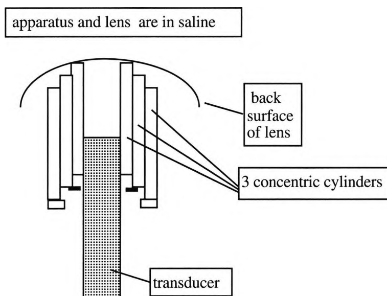
Figure 6.1 A design using ultrasound to measure three sagitta values on the back surface of a soft lens. From these three values a best fit equation could indicate the asphericity of the surface.
