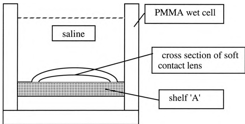
Figure 5.5.6b Alternate side elevation of the wet cell used to photograph a cross section of a soft lens. This is the view see from the camera viewfinder.
