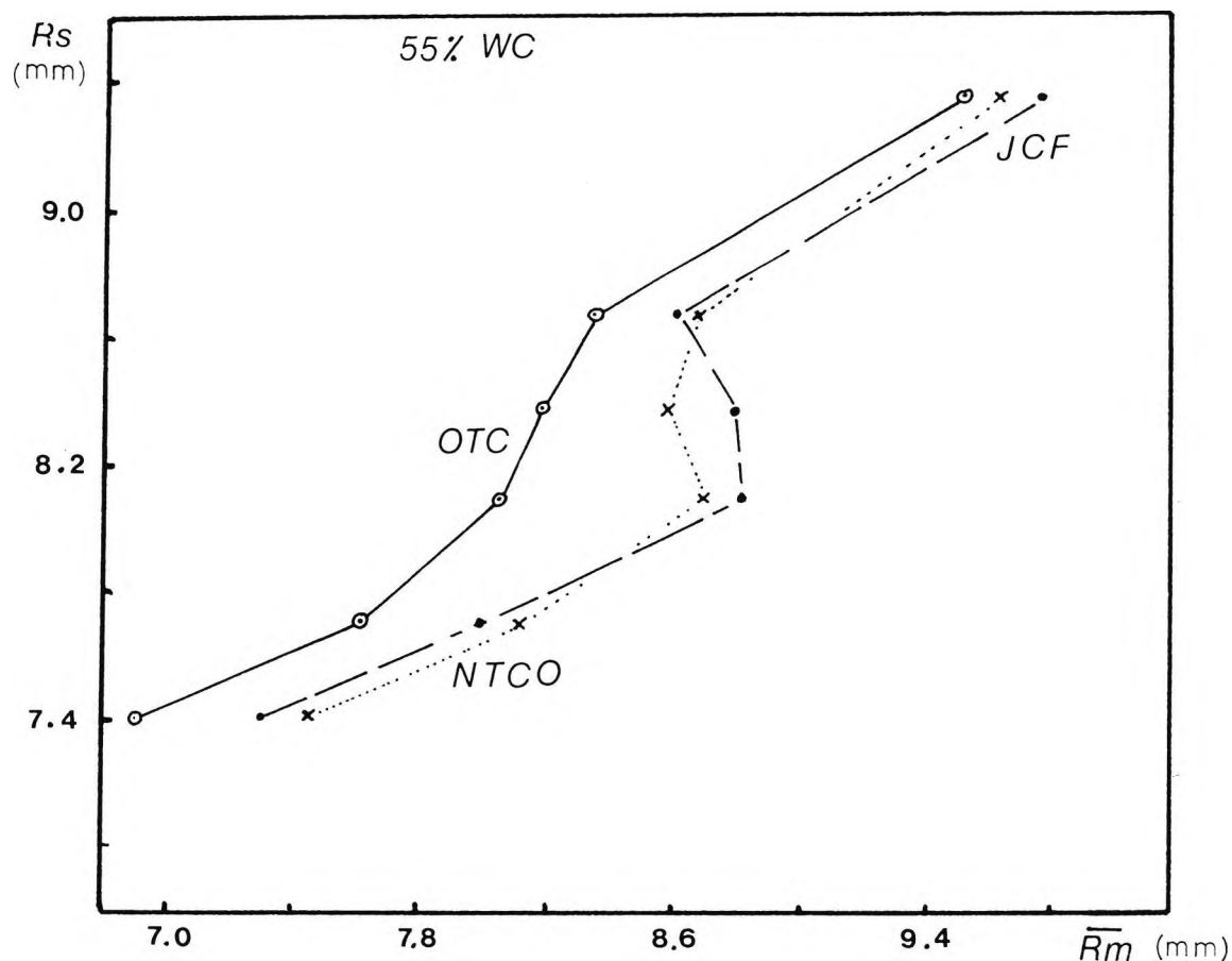
Fig. 3. The 55% water content group. The specified lens radii ( R_s ) are plotted against the experimental mean radius values ( R_m ). NTCO values and JCF values were obtained using the same pH saline.
