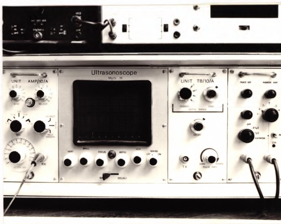
Figure 3.1 The Ultrasonoscope. Supplementary controls are on the far right panel. The screen and raster are on the larger panel.
