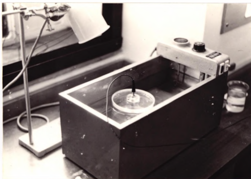
Figure 4.2 The Mk II apparatus (Port, 1975). Concentric construction allowed the transducer axis to be aligned with the support cylinder's axis. The apparatus could be placed in a water bath to control temperature.
