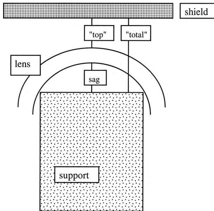
Figure 5.2.6 The three values calculated from the frozen USM image are depicted ie the sag, "top" and "total" values. The thickness of the lens is ( 'total' - sag - 'top' )
