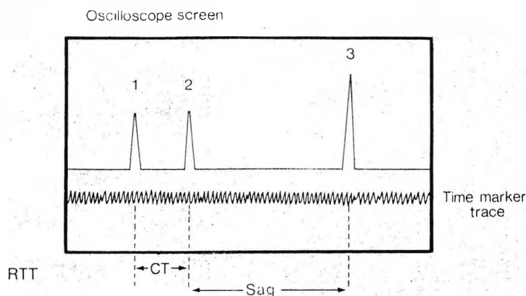
Fig 6: Visual detection of interfaces
