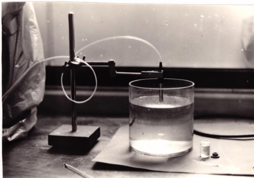
Figure 4.1 The first prototype apparatus (Port, 1975). There was no temperature control system and the transducer axis was not accurately centred on the lens axis
