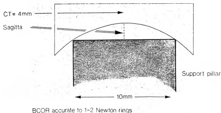
Fig 3: Calibration template, made from Perspex
