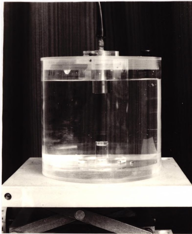
Figure 3.6 An early version of the measurement apparatus showing a contact lens support at the bottom of the saline. For measurement of sound velocity, this support was removed and the device in Fig. 3.5 substituted.
