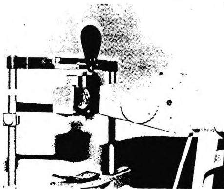
Figure 10.8 A wet cell (filled with saline and holding the soft lens) is clamped to the headrest of a Zeiss Jena ophthalmometer to enable the Back Optic Zone Radius to be measured. The instrument value for the soft lens in saline would not be accurate as the instrument conventionally determines radius values (of the cornea) in air.
