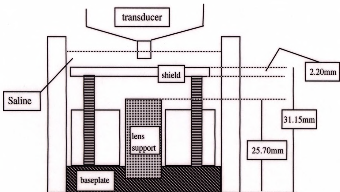
Figure 5.2.5 The measurements taken with the micrometer in order to deduce the distance from the top of the lens support to the lower surface of the shield .
