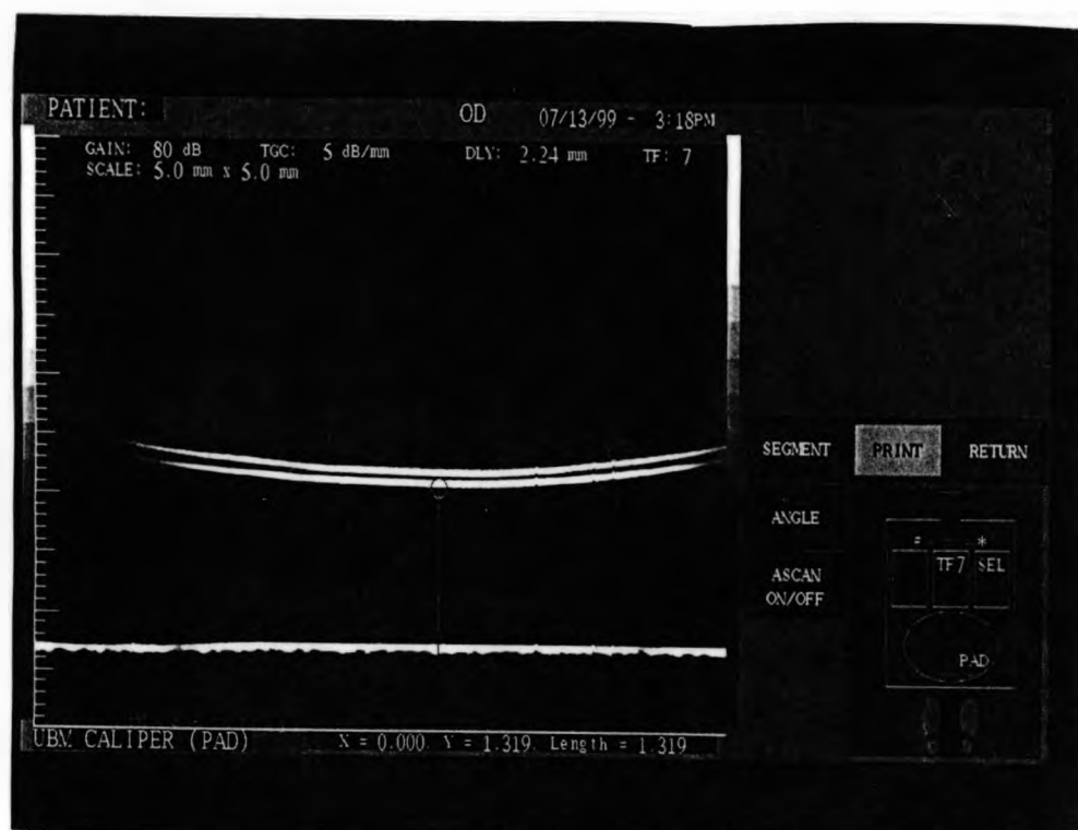
Figure 5.3.3 Assessment of the contact lens front surface. A USM image showing the ultrasound beam incident on the rear surface of a contact lens. The reference surface is below the level of the lens support. The lens support is a hollow cylinder with a moveable core. The top of this core provides the reference surface for the measurement of front surface radii.
