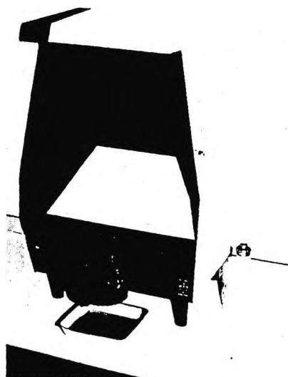
Figure 10.6 A current Optimec soft lens analyser. This model has two wet cells – one to measure the back optic zone radius and centre thickness, the other to measure total diameter and to carry out inspection of the surfaces.
