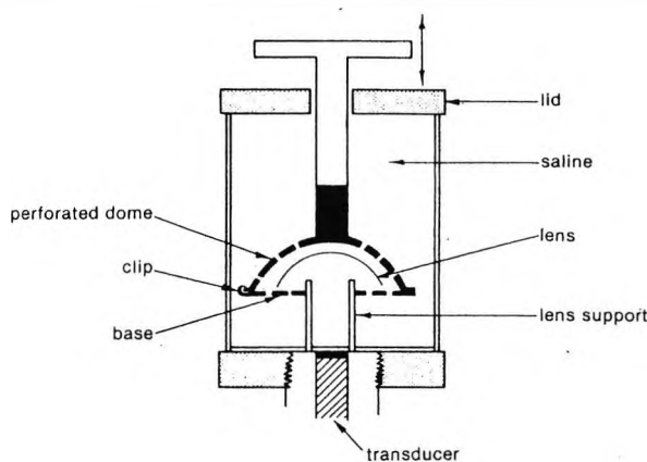
2 The Optison wet cell and centration device for positioning lenses on the stainless steel lens support.
