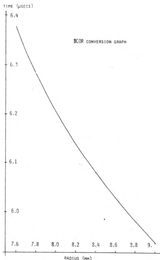
Figure 8. BCOR conversion graph.
