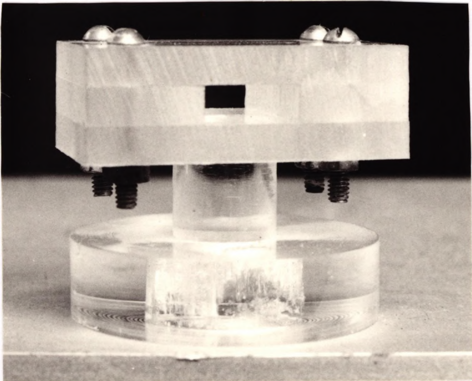
Figure 3.5 The device used to create a known thickness of saline in order to measure the velocity of sound at specified temperatures. The device is positioned in the apparatus in place of a soft lens support. The saline gap (4.47mm) is positioned in the waist of the ultrasound beam.
