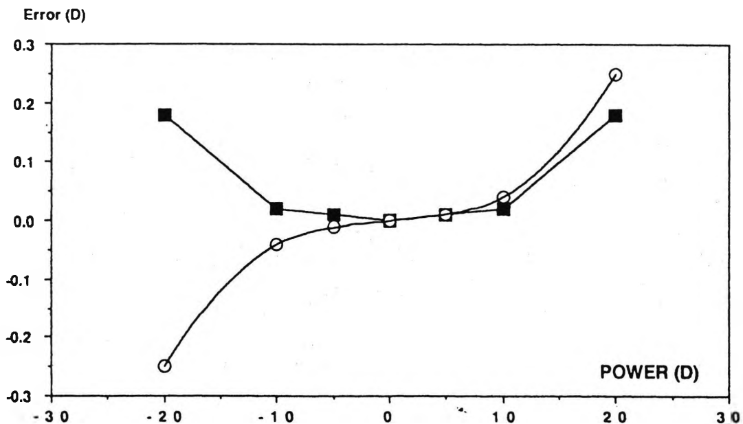
Figure 10.2 Calibration curves for two different focimeters. Both curves are non-linear and the use of linear regression to establish a best fit line is inappropriate. One can either join the points (solid squares) and intrapolate where necessary, or, fit a mathematical curve which has a polynomial equation (open circles).
