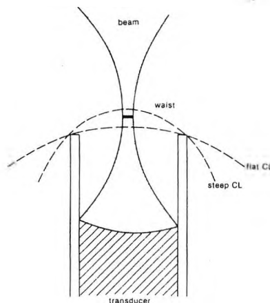
1 The principal part of an ultrasound beam formed by a strongly focusing transducer. Contact lenses of different curvatures are positioned in different parts of the beam.
