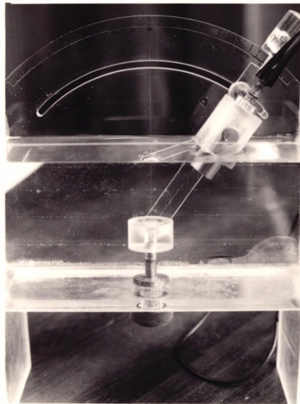
Figure 5.5.3b The protractor scale with the transducer in situ. The face of the transducer is below the saline surface at all times.
