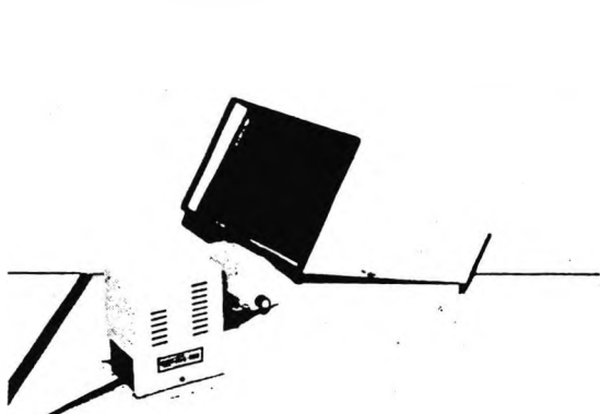
Figure 10.3 The Hydro-Vue™ soft lens analyser. This is an in-saline device where the image of the lens on a spherical dome is projected on to a translucent screen.
