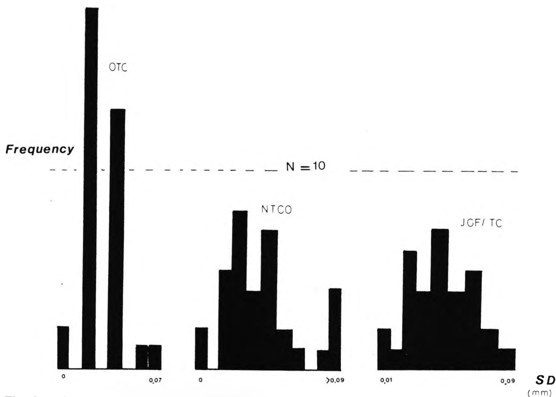
Fig. 2. Histograms of SD values for individual lenses measured on the temperature controlled Optison (OTC), the non-temperature controlled Optison (NTCO) and the Optimec JCF (JCF/TC)
