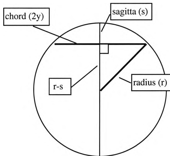
Figure 1.4. The geometrical principles used to determine the radius of curvature of a spherical surface.
