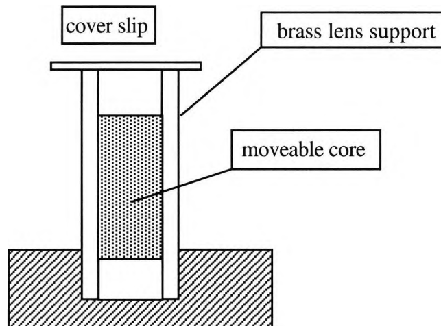
Fig 5.3.1 The brass lens support showing the moveable central core and the cover slip in situ.
