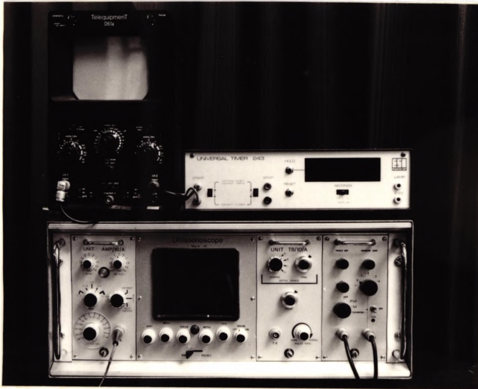
Figure 3.2 The Tektronics oscilloscope and interval timer on top of the Ultrasonoscope
