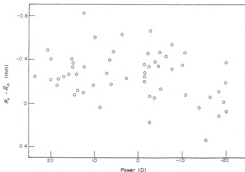
Fig. 6. A scattergram of the difference between the specified radius and the experimental mean radius as a function of the lens power.
