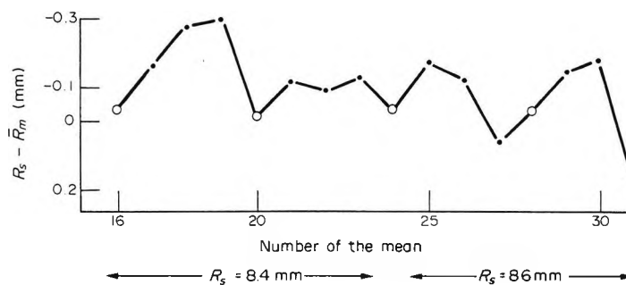
Fig. 4. Results for lenses having different specified radii. The difference between the specified radius and the experimental mean radius is plotted for each lens against the number of the mean. Six lenses have a specified radius of 8.4 mm and six a specified radius of 8.6 mm. \odot denotes results for the control lens which was remeasured with each group of three test lenses.
