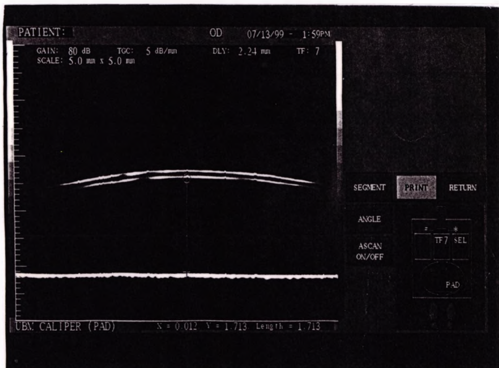
Figure 5.2.8 In this image the lens shield is not in position. Reflections are only shown from the contact lens and the lens support. The cursor is shown measuring the distance equivalent to the lens back surface sag. The value 1.713 shown at the bottom of the screen has to be multiplied by a conversion factor to give the real distance.
