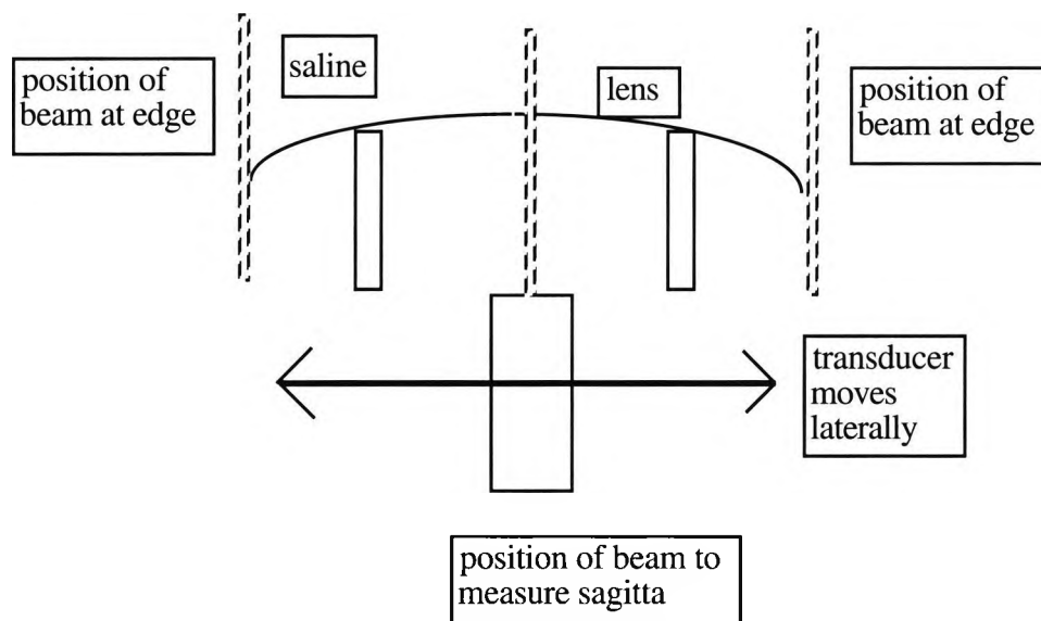
Figure 6.2 An arrangement that could measure both the back surface sagitta above the lens support and also measure the total diameter of the lens by moving the transducer laterally. The width of the beam would have to be taken into account when the transducer travel was recorded. This could be ascertained with rigid test pieces of known diameter.
