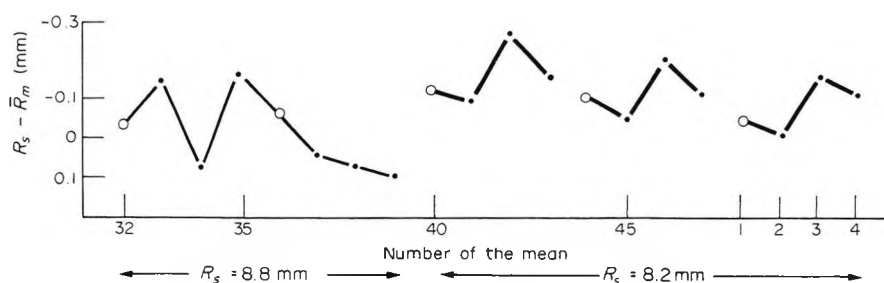
Fig. 5. The difference between the specified radius and the experimental mean radius plotted against the number of the mean. Means 33–35 and 37–39 refer to lenses with a specified radius of 8.8 mm. Means 40–43 show the results obtained in experiment 1 of the repeatability test. Means 44–47 are those obtained in experiment 2 of the repeatability test. Means 1–4 are included for comparison. ○ denotes results for the control lens.
