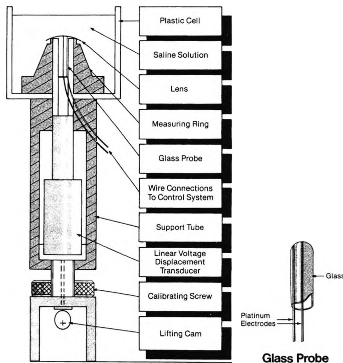
Fig. 1. A cross-section of the Kelvin Soft Lens Measuring Gauge showing the essential components.
