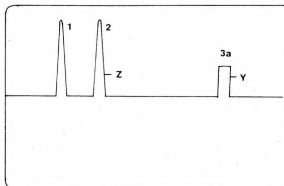
Figure 6. The time locked artificial reflection (3a) is shown. Amplitude Y opens the counter gate. Amplitude Z closes the counter gate. Position of peak 2 varies with BCOR.
