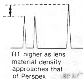
Fig 10: To obtain cross-section of a lens, transducer can be scanned across the lens
