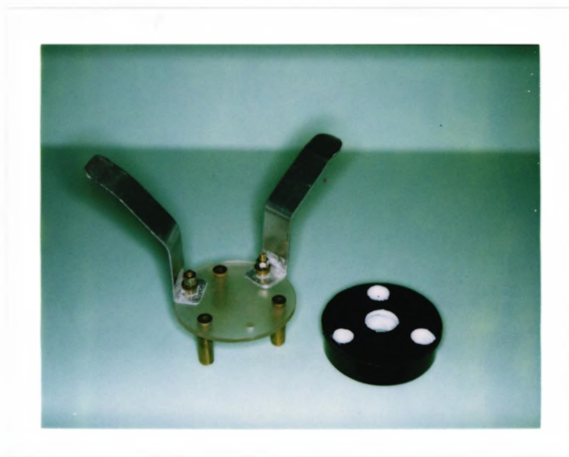
Figure 5.2.3 On the left is the 'shield' which separated the transducer head from the contact lens. The shield could be removed from and replaced in the wet cell by means of the aluminium handles. On the right is the black PMMA disc which was placed over the lens support. There are three holes in this disc which allow the legs attached to the shield to pass through.
