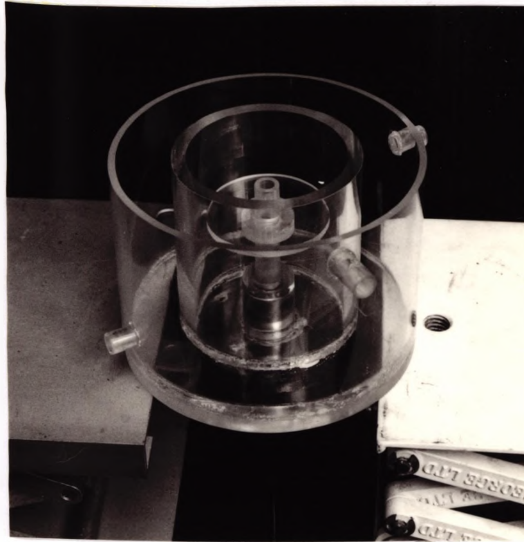
Figure 4.3 The Mk III apparatus shown without saline and without tubes connected to the water jacket.. For measurement purposes a perspex lid covered the water in the external jacket but allowed access to the central measurement cell.
