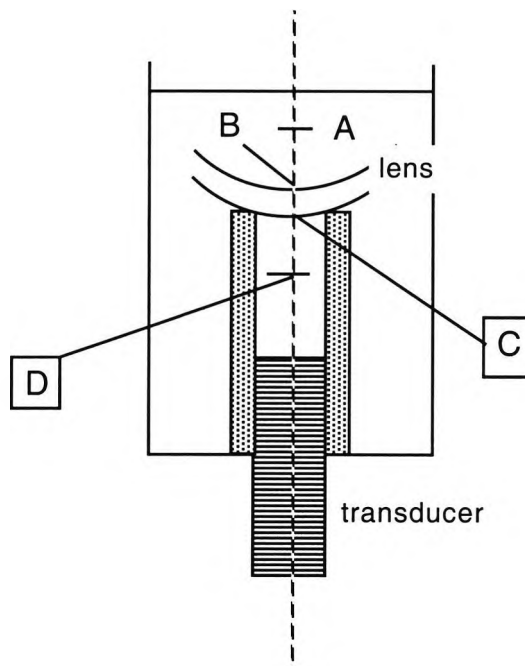
Figure 5.2.1 A method for determining the lens thickness in saline without knowing the velocity of sound through the lens material itself.
