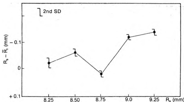
4 The difference between the specified BCOR and the measured mean using a radiuscope compared to the specified radius.
