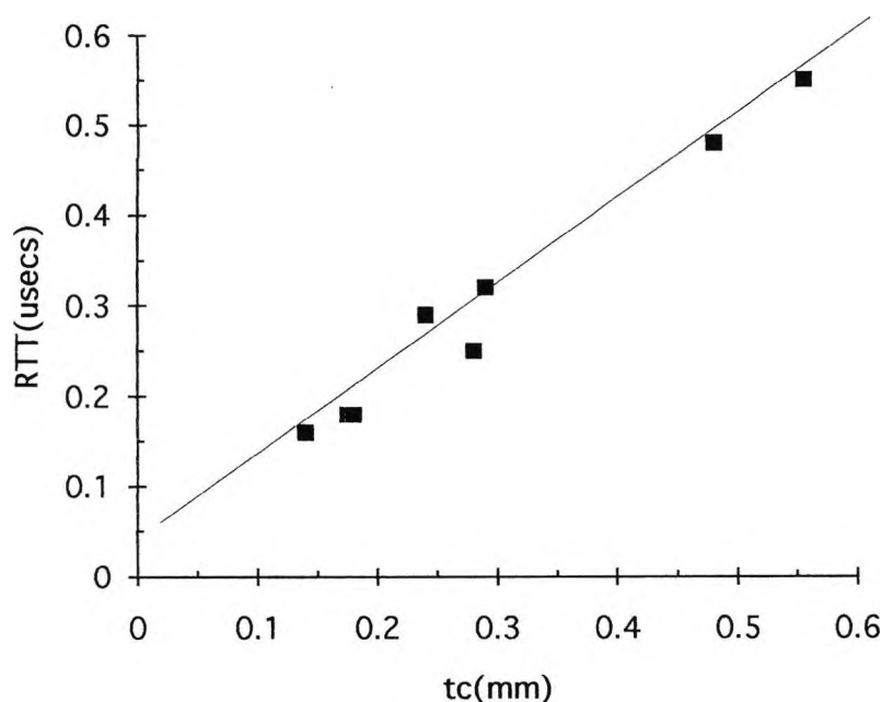
Figure 5.2.0 The relationship for S85 material when the centre thickness measured with a radiuscope (as a travelling microscope) was compared to the RTT values obtained using ultrasound.
