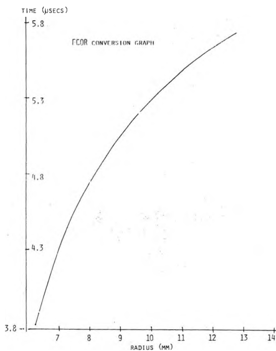
Figure 9. FCOR conversion graph.
