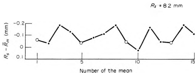
Fig. 3. Results for 12 lenses, one of which was the control lens, all having a nominal specified radius, R_s , of 8.2 mm. The difference between the R_s and the mean experimental radius, \bar{R}_m , is plotted against the number of the mean. \odot denotes the results for the control lens, which was remeasured with each group of three lenses.
