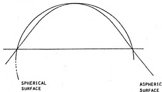
Figure 2. Sagitta measurements are the same for both curves but there are different central curvatures.
