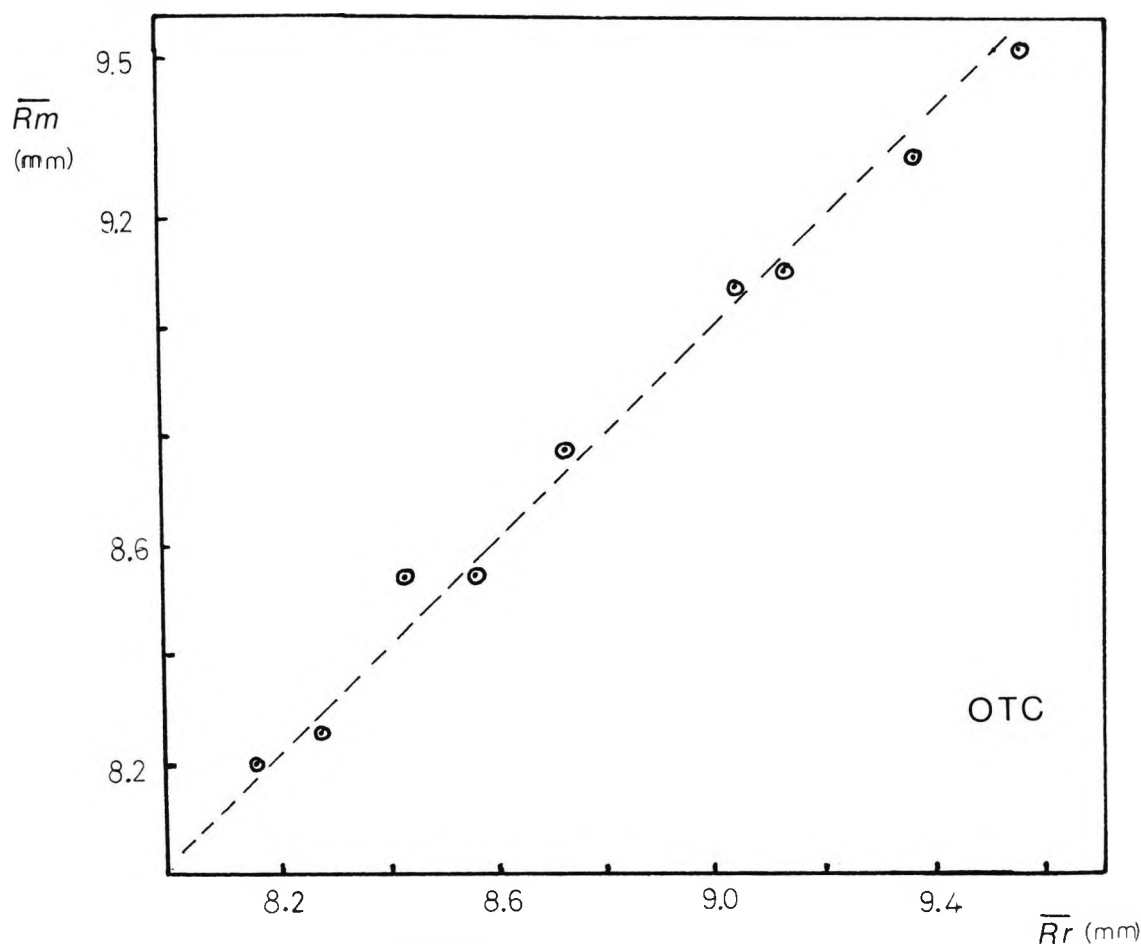
Fig. 1. PMMA 'FLOM' lenses. The mean radius values ( \bar{R}_m ) obtained from the Optison TC plotted against the mean vertex radii ( \bar{R}_r ) obtained from an American Optical radiuscope.
