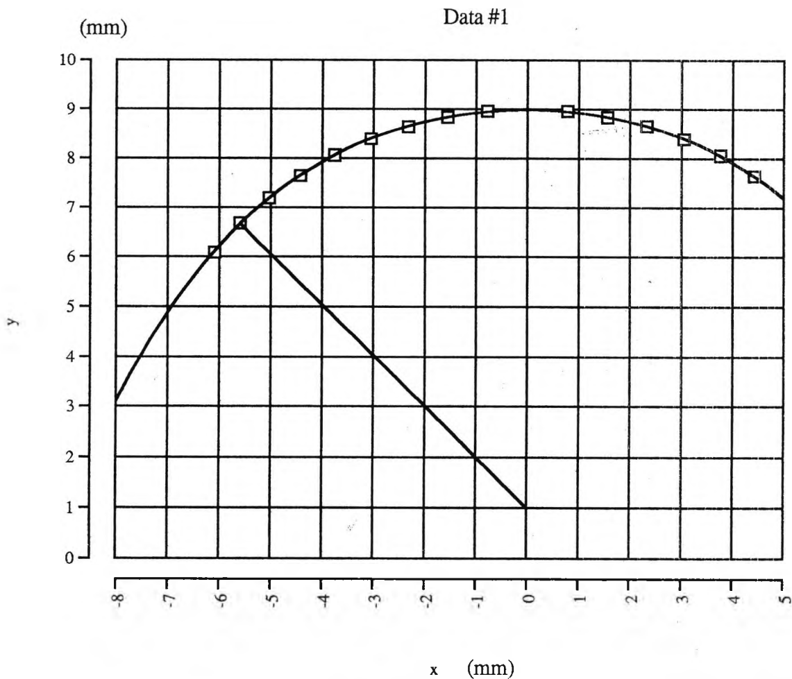
Figure 5.5.5 A plot of the x and y coordinates for the steel ball. Note that less values are plotted on one side of the vertical as the transducer values were unreliable at the larger angles.
