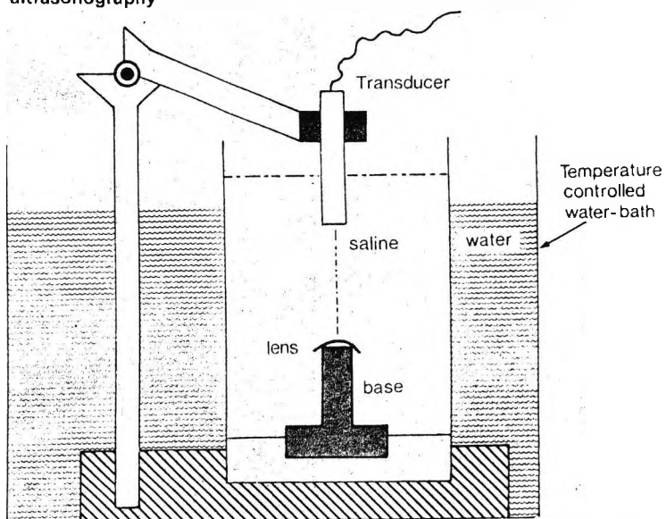
Figs 1 & 2: Apparatus for measuring anterior chamber in ocular ultrasonography
