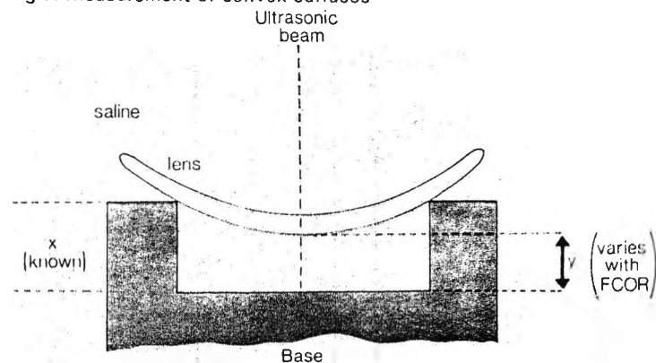
Fig 7: Measurement of convex surfaces
