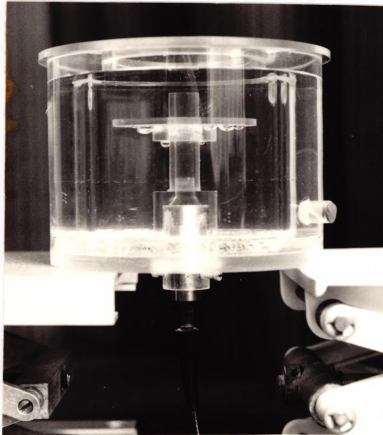
Figure 4.4 Elevation view of the Mk III apparatus. The transducer can be seen at the bottom of the measurement cell. The contact lens is supported on the hollow cylinder above the transducer. The circular shelf both enabled test lenses to be kept in saline at the correct temperature and prevented lenses from falling to the bottom of the measurement cell.
