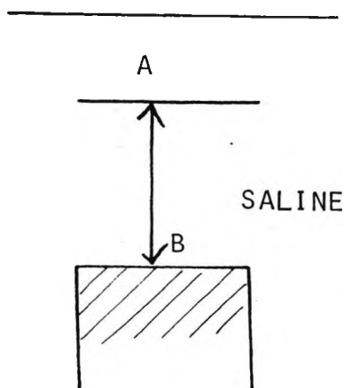
Figure 10. CD = AB - (AC + BD) . AB = RTT_1 \times V/2 . AC = RTT_2 \times V/2 . BD = RTT_3 \times V/2 . CD (lens thickness) = V/2 \cdot [RTT_1 - (RTT_2 + RTT_3)] . V = velocity of sound in saline at known temperature. A and B are reference surfaces or points. C and D are the contact lens surfaces.
