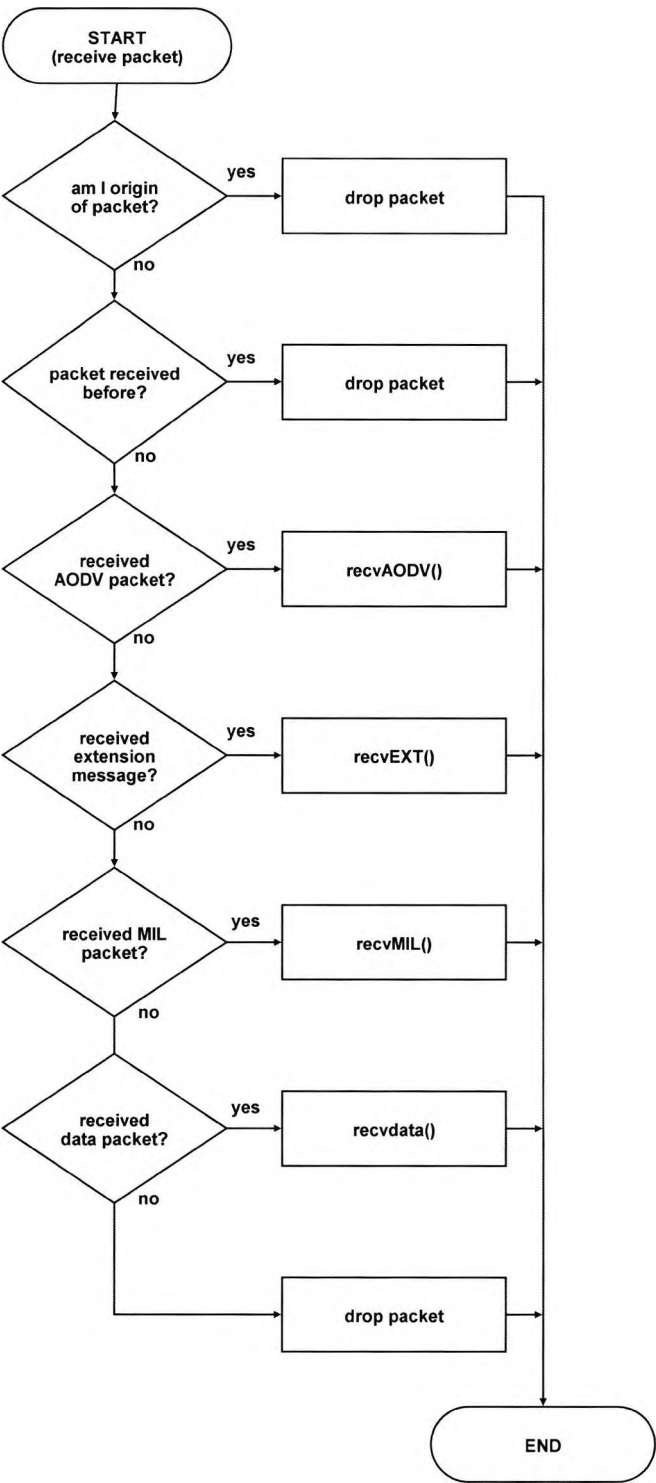
Figure 6.3: Receiving packets (1)
