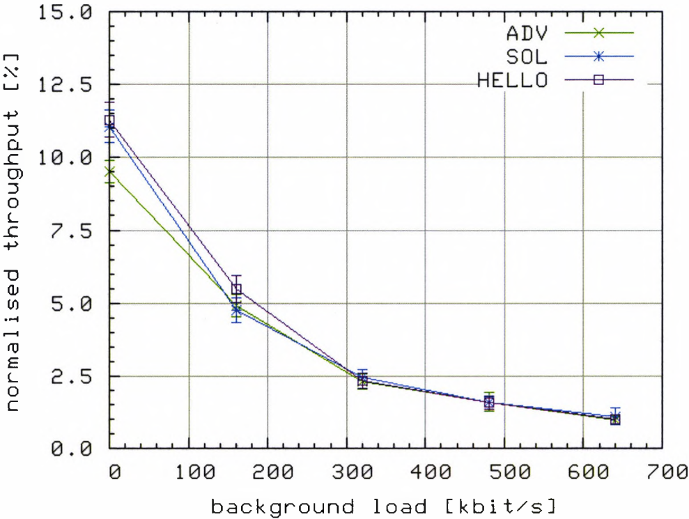
(b) Throughput
