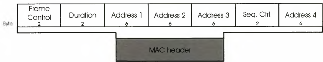
Figure 2.7: W-LAN MAC header
