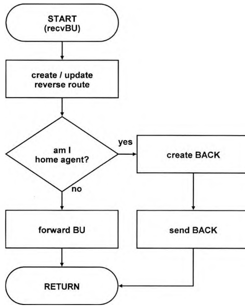
Figure 6.15: Receiving a binding update message (BU)
