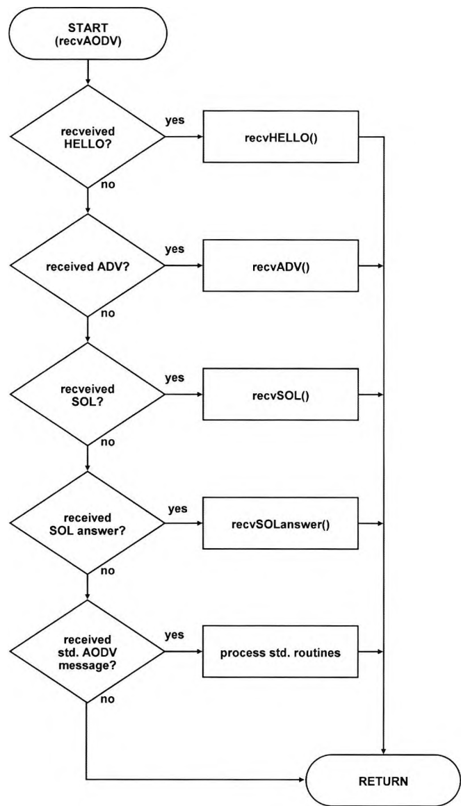
Figure 6.4: Receiving packets (2)
