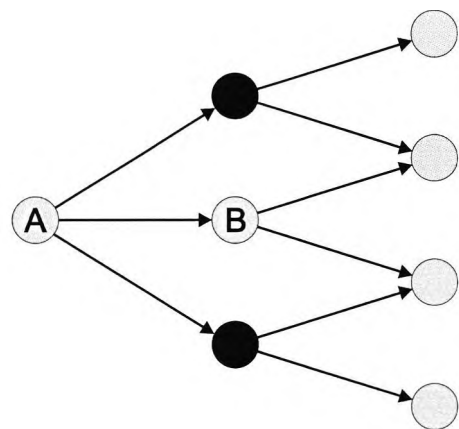
Figure 2.13: MPR selection in OLSR
