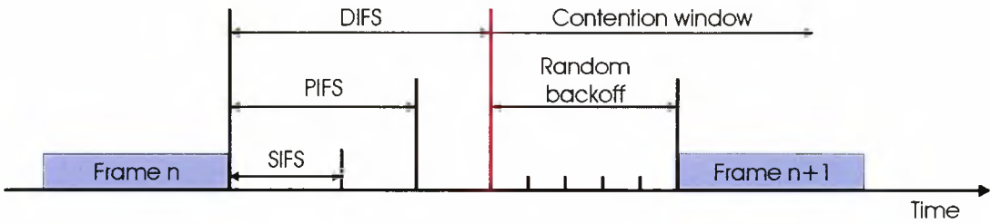
Figure 2.8: Medium access
