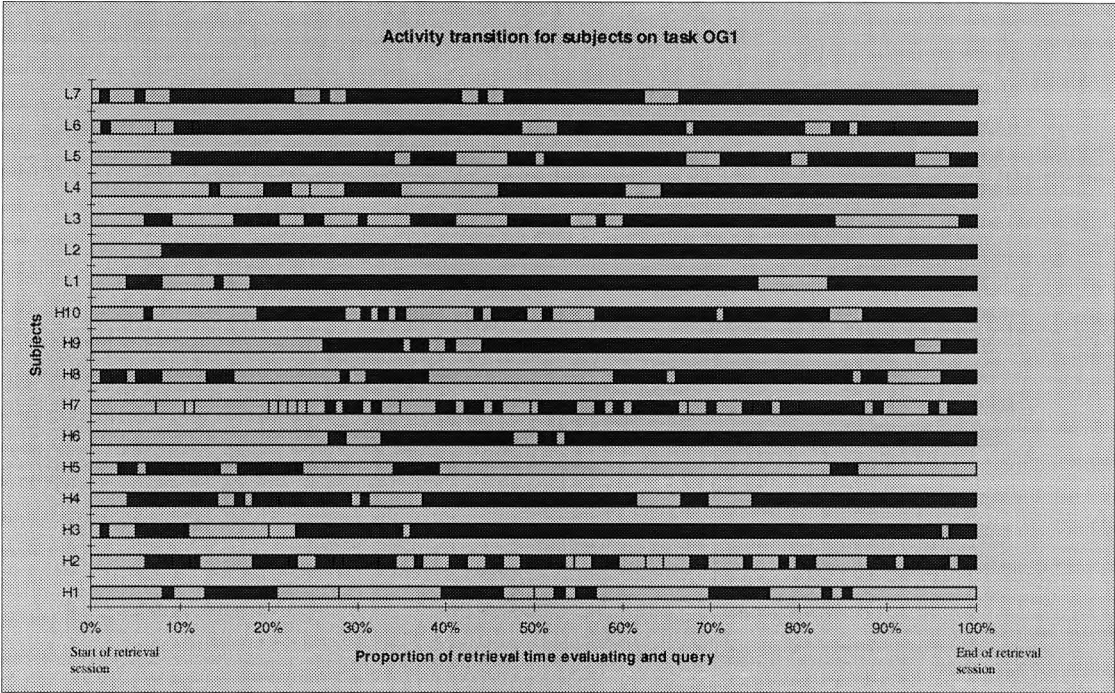
Activity transitions for searchers on task OG1
