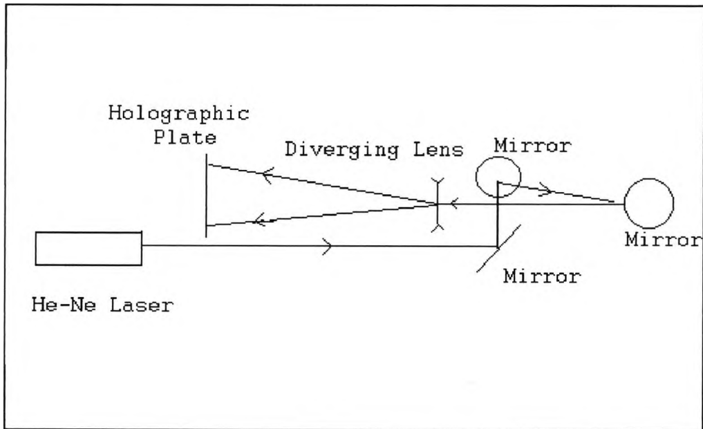
Figure A3. Hologram Reconstruction Optics
