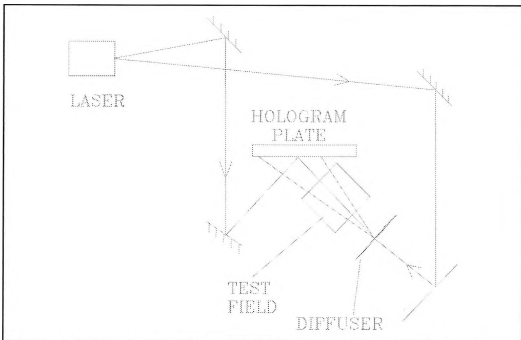
Figure 90 The revised optical path with diffuser
