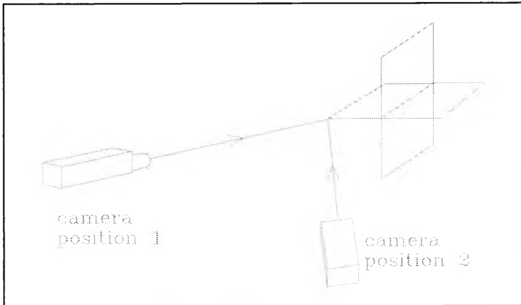
Figure 88 The photogrammetric layout
