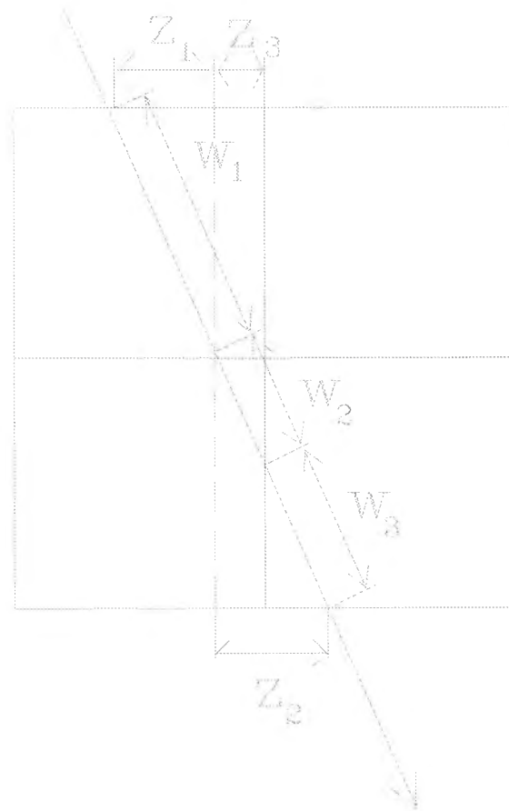
Figure 15 A plan view of a ray passing through three voxels
