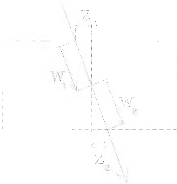
Figure 13 The plan view of a ray that passes through two voxels
