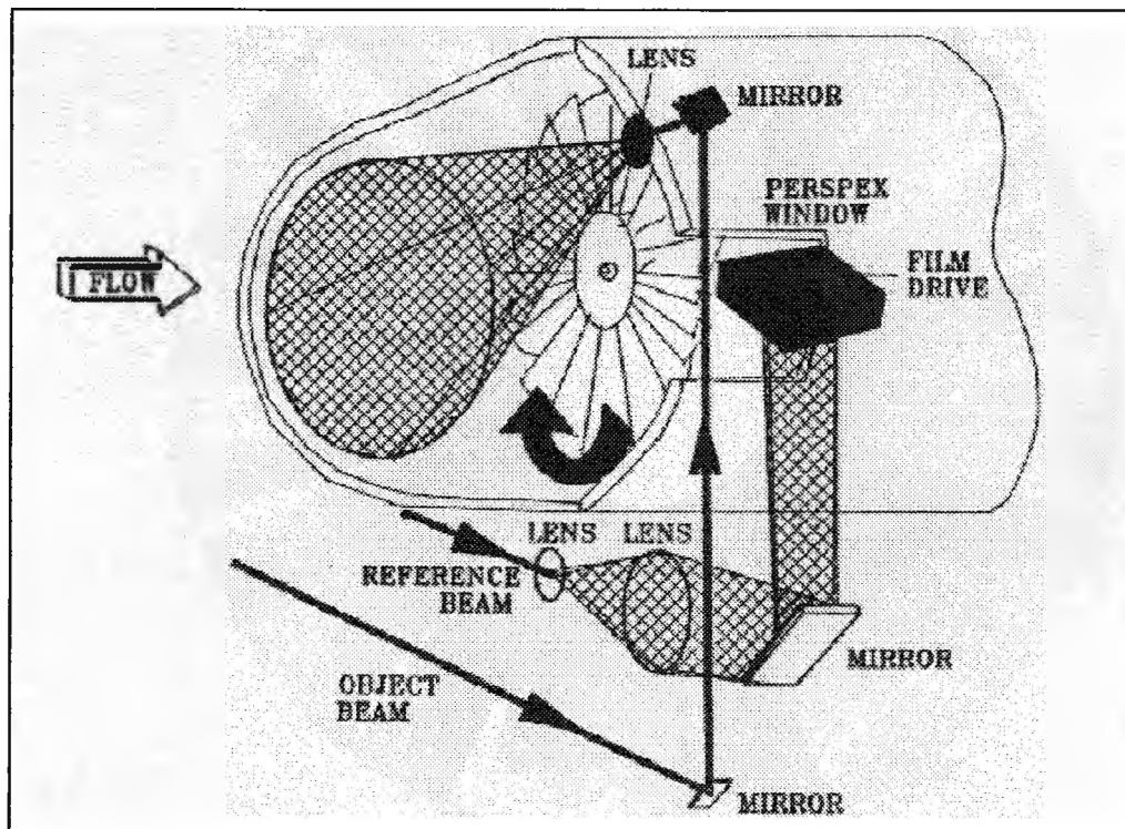
Figure 7 The Rolls Royce optical configuration
