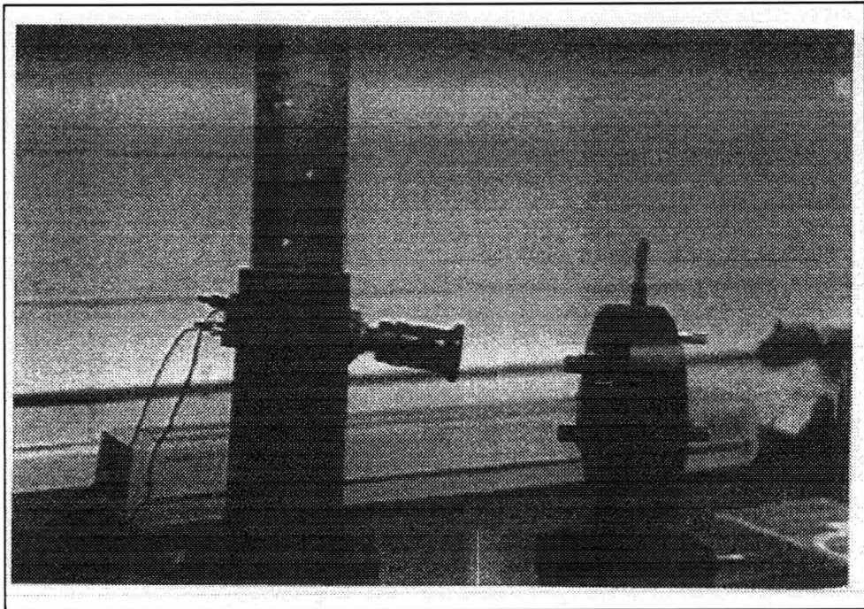
Figure 81 The image capture apparatus
