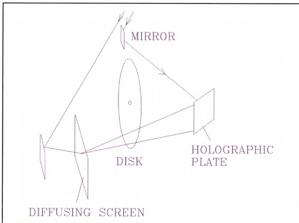
Figure 92 The rotating disk object and optical path.
