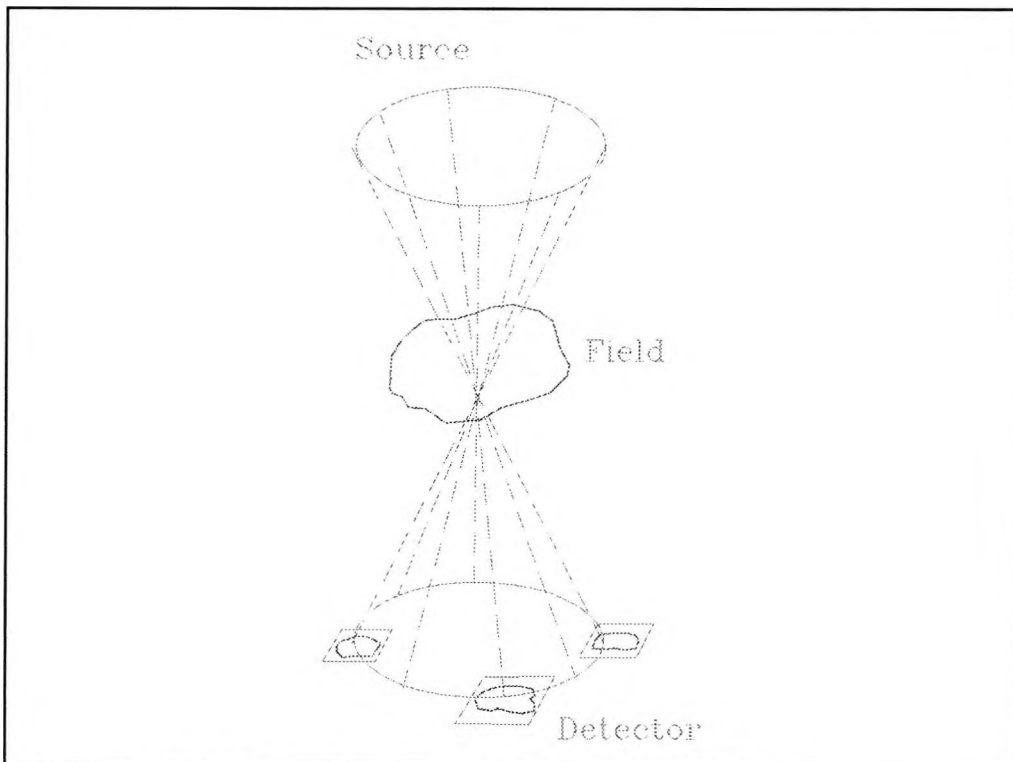
Figure 6 Colsher Conical Projection Scheme.
