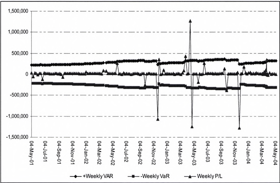
Figure 3.6 Backtesting of AA- sub-portfolio
