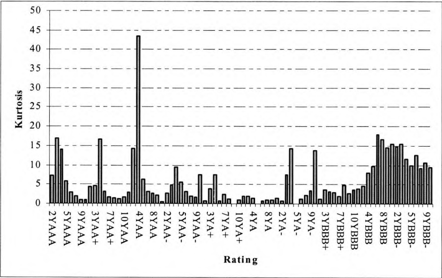
Figure 2.7 Kurtosis vs Rating
