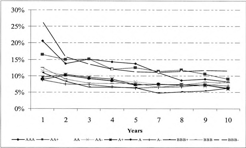
Figure 2.6 Term Structure of Volatilities of Credit Spreads
