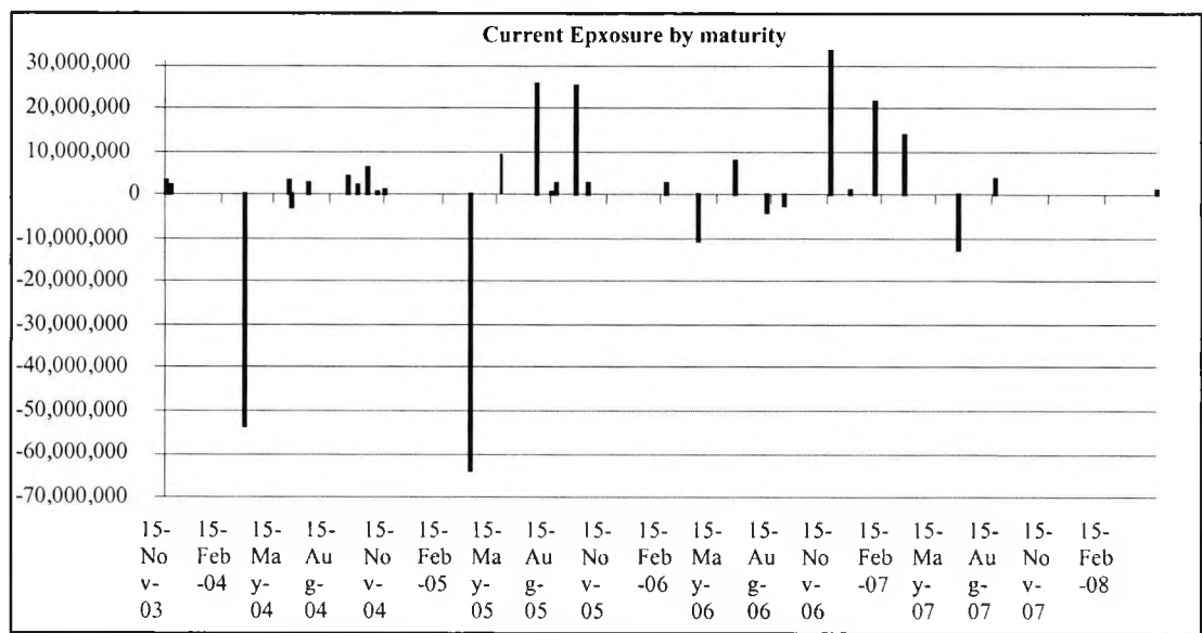
Figure 3.5 Exposure by maturity
