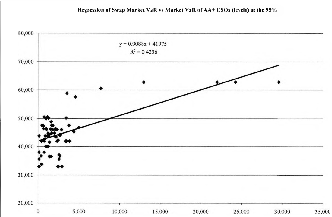
Figure 3.11 Regression between AA+ Swap VaR against the VaR of AA+ CSIO
