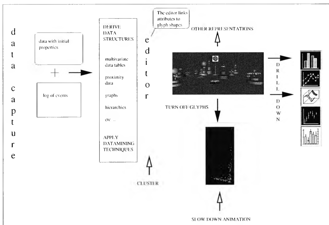
Figure 5.1: Technique combination for viewing complex data based upon an animated glyph world with editor for linking attributes and datamining techniques to derive different data structures.
