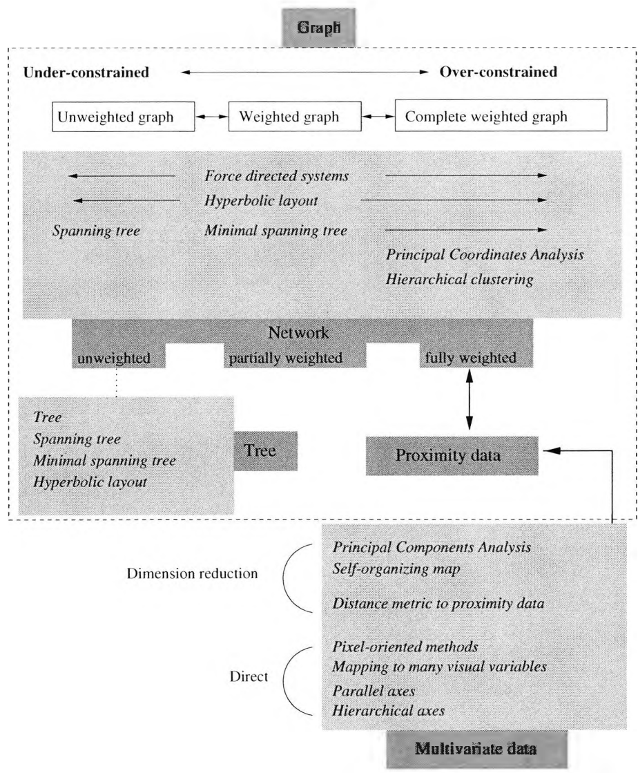
Figure 3.1: Overview of layout methods by data type. The two main boxes show methods for ‘graph’ layout (within the dotted line) and ‘multivariate data’ layout. Multivariate data layout methods divide into those involving dimensions reduction and those directly mapping the variables to the graphic. Graph layout is constrained by the presence or absence of weights for the edges, and by its completeness. This corresponds to layout for networks. Trees lie at the incomplete end of the graph constraints. Proximity data derived from multivariate data correspond to a complete weighted graph.
