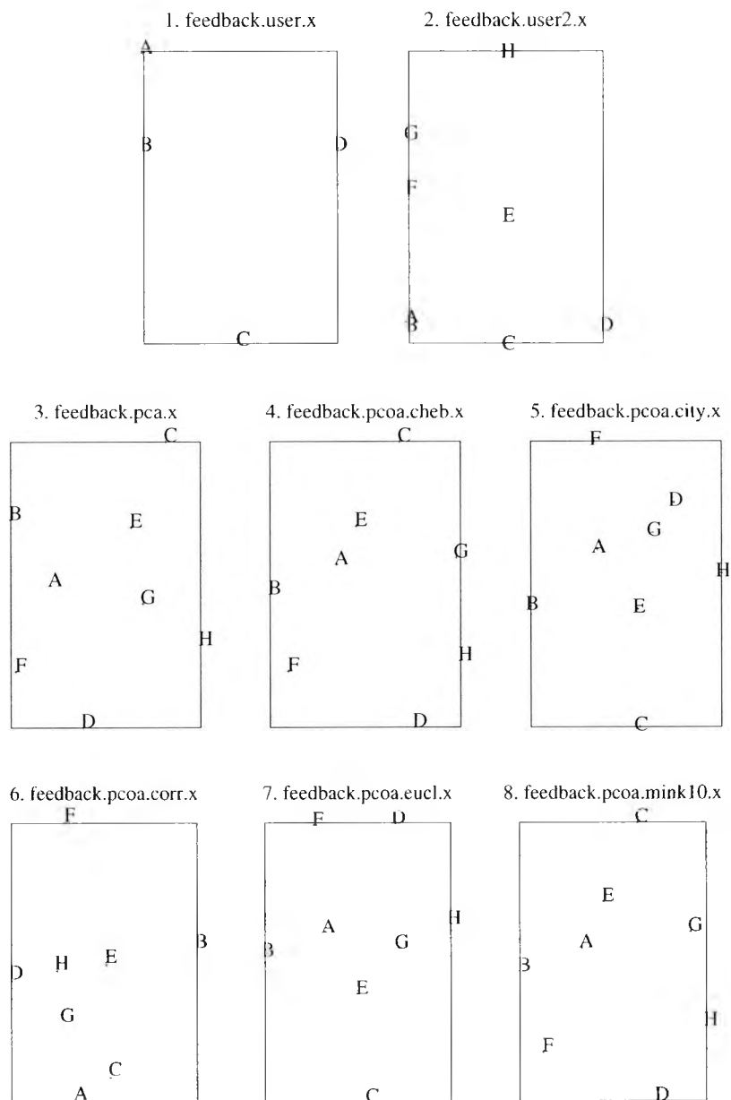
Figure 10.5: 1. Four entities placed by a user. 2. Generalisation of these placements and application to all entities. 3-8. Scatterplot of the eight entities using PCA and PCoA with Chebychev, City or Manhattan (Minkowski with \lambda = 1 ), angular, Euclidean and Minkowski ( \lambda = 10 ) distance. From visual comparison of the layouts, the user's initial placement of ABCD (1) is generalized by essentially separating ABCD and EFGH (2). None of the metrics (3-8) separate these two groups, though City distance (5) and correlation (6) do to some extent, correlation the most. On the other hand, the commonly used mean square distance error gives a lower value for PCA (3) than for correlation, indicating that PCA is closer to the user's layout.
