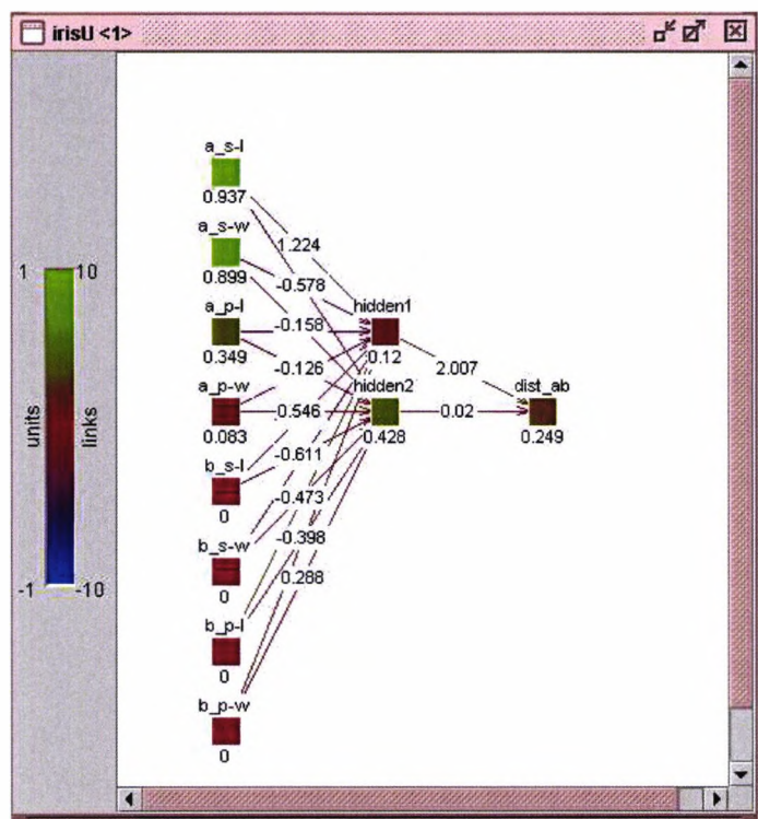
Figure 10.8: The single hidden layer feedforward net used to learn the distances obtained from the user arrangement of 8 iris examples on the screen (shown in Figure 10.6. This is a screenshot of one of the windows in the Java interface for the Stuttgart Neural Network Simulator. The inputs are the four values (s-l: sepal length, s-w: sepal width, p-l: petal length, p-w: petal width) for patterns a and b . For example, a_s-l is the sepal length for a . The output, dist_ab , is the distance between a and b in the user arrangement.
