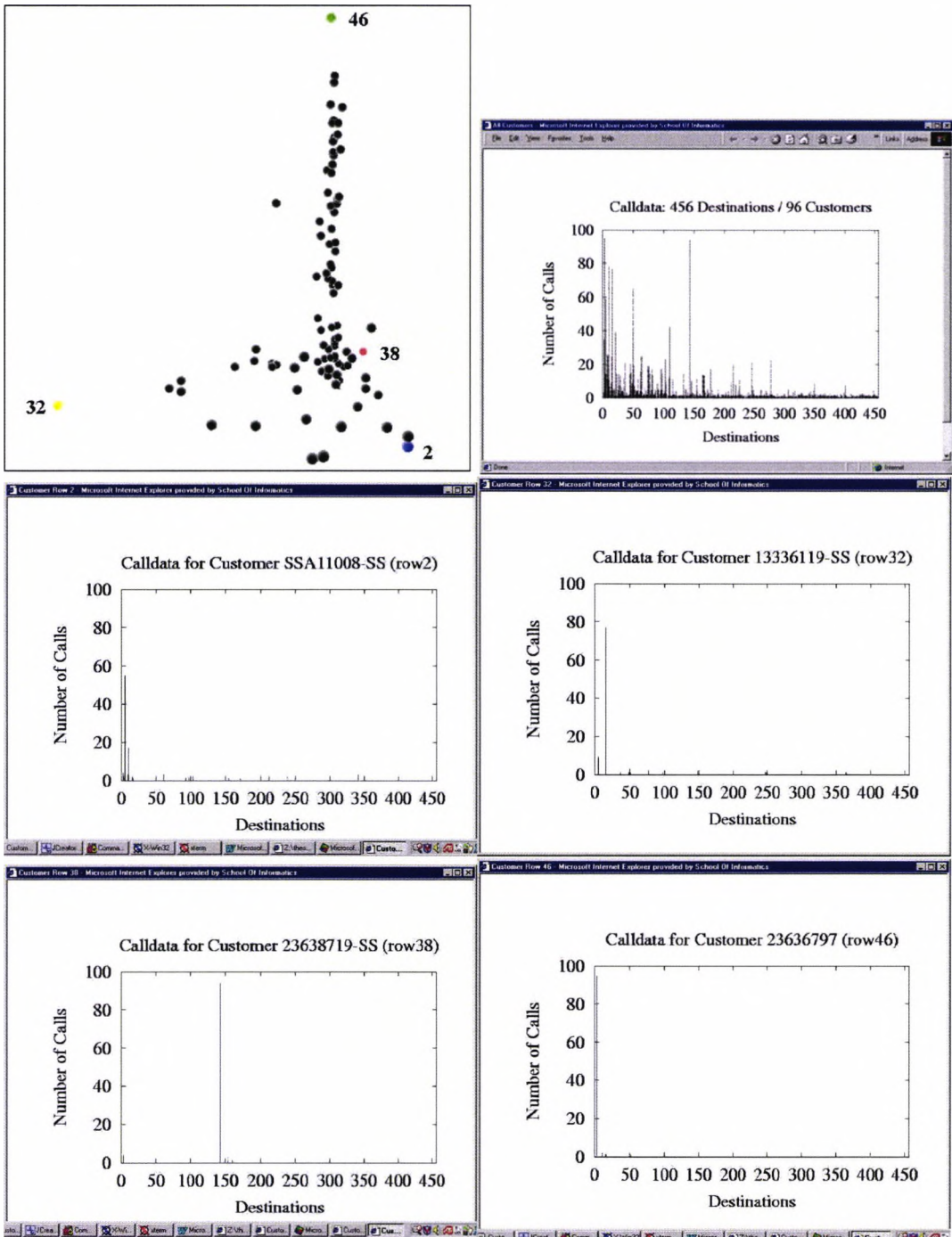
Figure 9.1: Example of direct visual querying of the calldata set - selection of the extremities. First the bar chart showing all customer calls superimposed (top right) is examined. It shows that there are a few peaks of high numbers of calls to a destination, but that the majority of values are low. The scatterplot produced using the Euclidean distance measure followed by PCoA for 3 dimensions (top left) shows the duck’s leg and webbed foot shape. The numbers 2, 32, 38 and 46 correspond to the row in the data table in which the customer appears (row 38 customer is the furthest sphere to the back of the screenshot). Charts of these selected extremities (middle and bottom) show that the highlighted customers correspond to peaks for single destinations.
