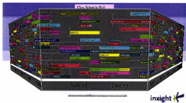
Figure 4.2: A perspective wall using Xerox's Information Visualizer ( http://www.parc.xerox.com/istl/projects/uir/projects/InformationVisualization.html ).
