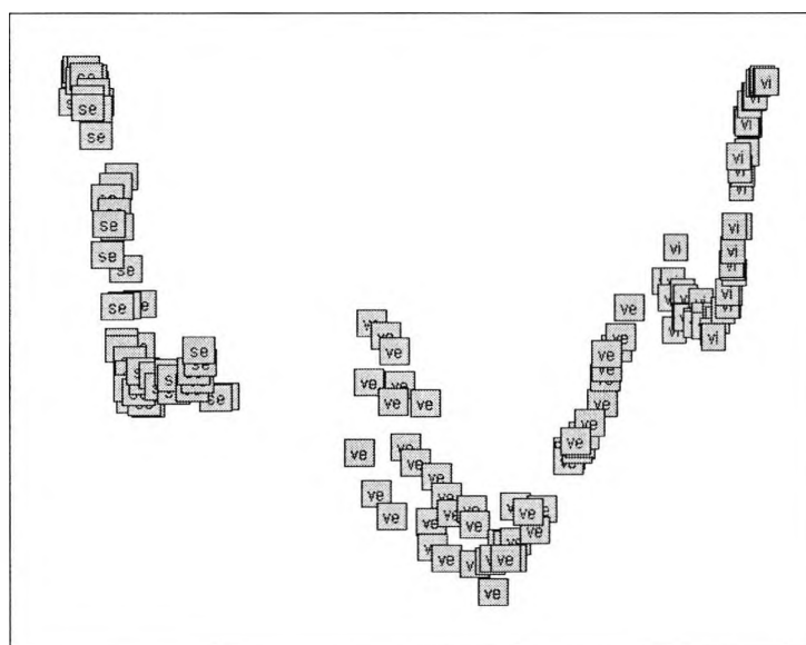
Figure 10.9: The layout of the Iris dataset using a neural network trained on the user distance data for a subset of 8 examples (shown in Figure 10.6). This shows that the species Iris-versicolor (ve) and Iris-virginica (vi) are now in separate clusters. Compare this to the original shown in Figure 10.7 (top), where these two species overlap.
