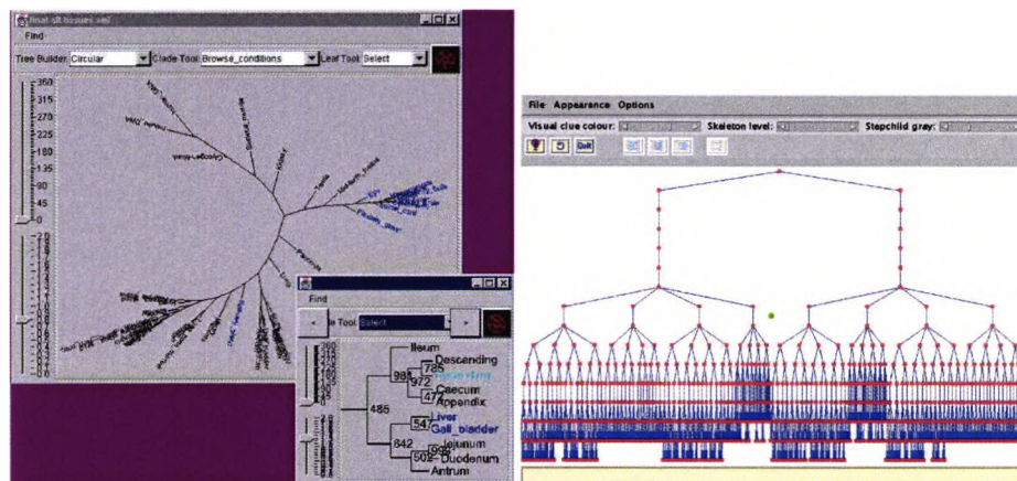
Figure 4.14: Tree layout: An unrooted and rooted dendrogram using the Expression browser ( http://www.sanger.ac.uk/Users/mrp/java/ExpressionBrowser/TheTutorial.html ) (left) and a tree constructed with the Latour tree visualization toolkit ( http://www.cwi.nl/InfoVisu/Past.html ) (right).
