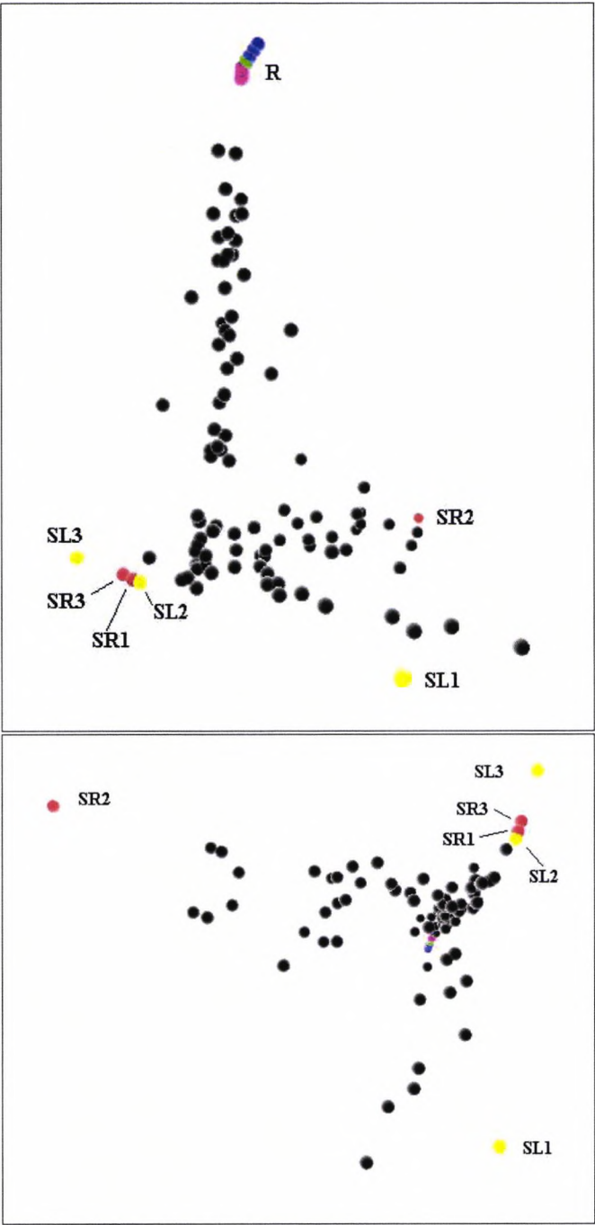
Figure 9.4: Feature fingerprinting with 'shifting' feature - addition of constructed data shifted with respect to a reference entity. Calldata dataset with Euclidean distance followed by PCoA for 3 dimensions and additional customers formed by adding (and subtracting) with respect to reference customer R as shown in the previous figure (9.3). Additional customers are added by shifting R 's values 1, 2 or 3 columns (destinations) to the right or left. These customers are labelled SL1 , SL2 , SL3 and SR1 , SR2 , SR3 . Both pictures are of the 3D representation, from two different angles, the lower one is a shot from underneath with respect to the upper one. From the bottom picture, it can be seen that SL1 and SR2 are far away from the main group - which is not shown very well in the top 3D shot.
