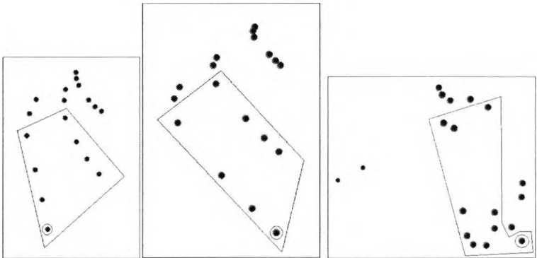
Figure 8.2: A user-specified constructed dataset of agent profiles, displayed with three different distance metrics - (left to right) City, Euclidean and Angular Separation - followed by PCoA layout. The areas indicated contain agents with 3 or more joint interests with intensity of overlap greater than 66% with respect to the circled, reference agent. The linear groupings reflect the way that the data were constructed (see text).
