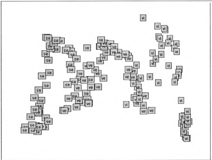
Figure 10.12: The layout of the Iris dataset using weights derived using a genetic algorithm: using polynomial relationship of order 5, including only the order 5 terms. Genetic algorithm run for 500 generations, utility 30.5.
