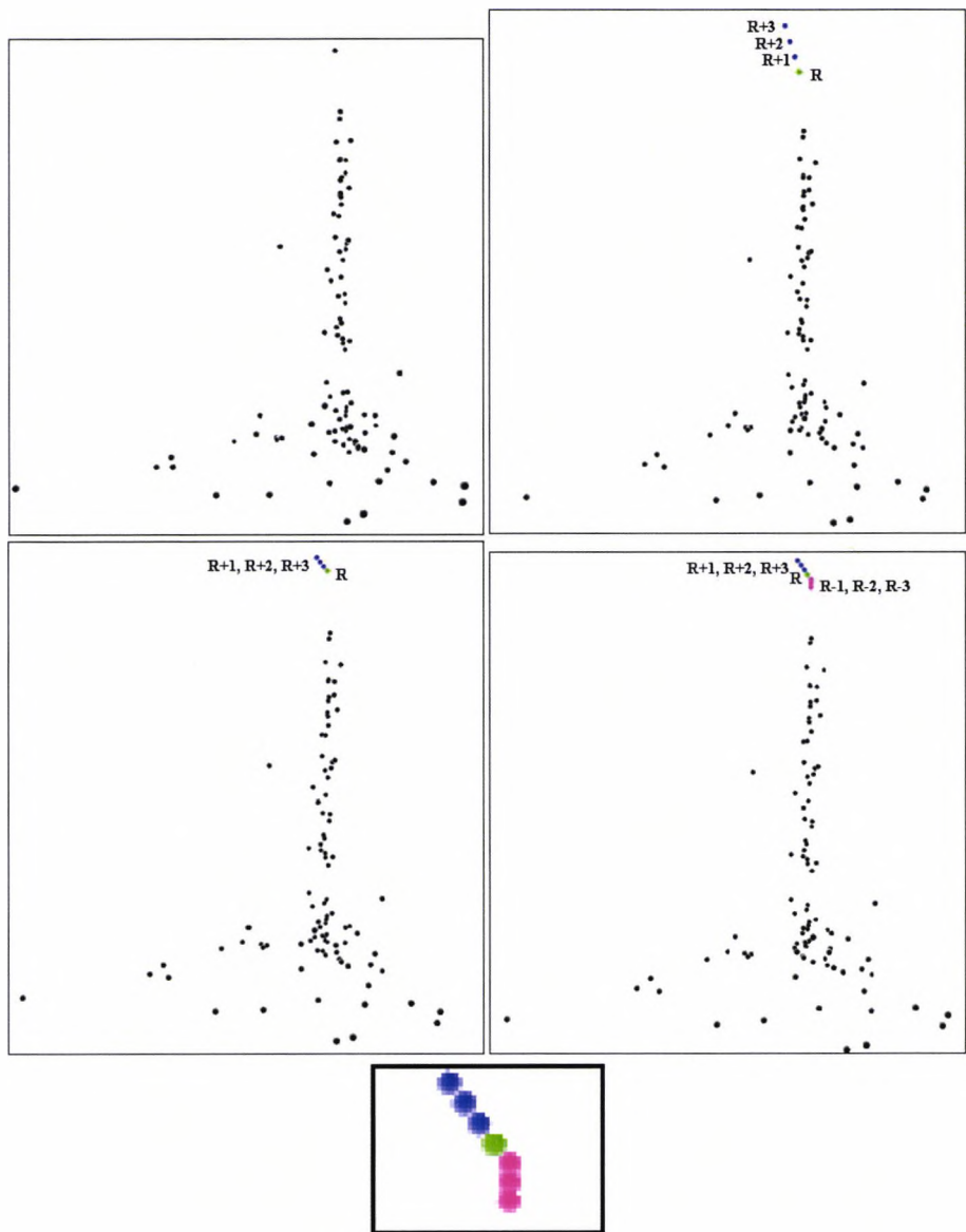
Figure 9.3: Feature fingerprinting with scaling feature - addition of constructed data scaled with respect to a reference entity. Top left: calldata dataset with Euclidean distance followed by PCoA for 3 dimensions. Top right: calldata dataset with a customer selected as a reference entity ( R ) and 3 new customers added to the dataset by increasing R 's values by 1 ( R+1 ), 2 ( R+2 ) and 3 ( R+3 ) respectively. Middle left: as top right, but R 's zero values are not incremented, to maintain the characteristic sparsity of the data. Middle right: as middle left with 3 extra customers whose data is obtained by decreasing R 's values by 1 ( R-1 ), 2 ( R-2 ) and 3 ( R-3 ) respectively. Bottom: enlargement of middle right additions.
