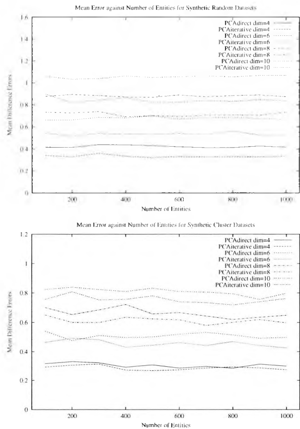
Figure 11.6: Mean Error against Number of Entities for Synthetic Random Datasets (top) and Cluster Datasets (bottom)
