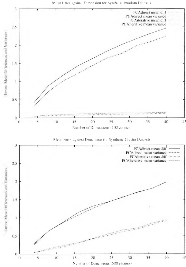
Figure 11.7: Mean Error against Dimension for Synthetic Random Datasets (top) and Cluster Datasets (bottom)
