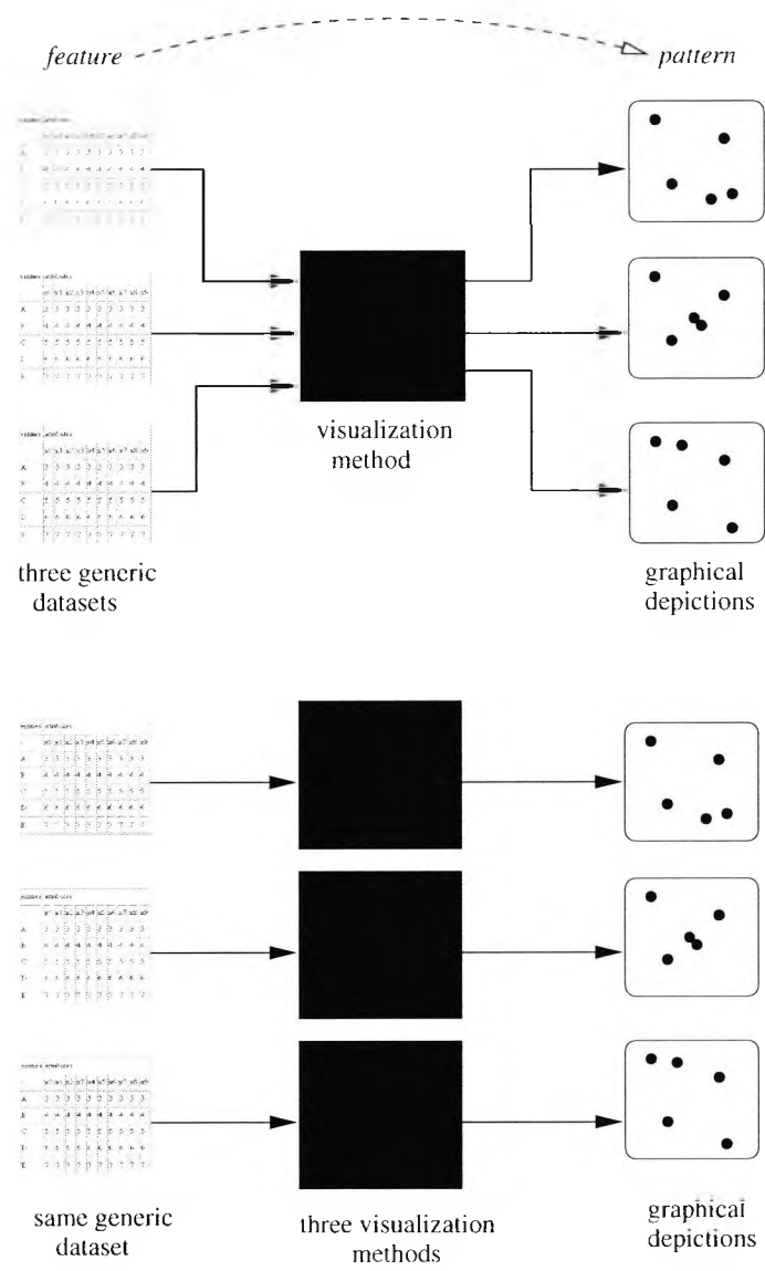
Figure 7.1: Generic dataset provision. Two scenarios: examining a single visualization method using several datasets (top); comparing different visualization methods using the same dataset (bottom). The visualization method is treated as a black box with the aim of seeing how features in the dataset, which can be seen directly in the table form, map to patterns in the graphic. Some other representation for the dataset may be used, depending upon the type of data, for instance, for time series data, line plots may be more appropriate. Line plots are used in addition to tables in the feasibility test in Section 7.3.1.
