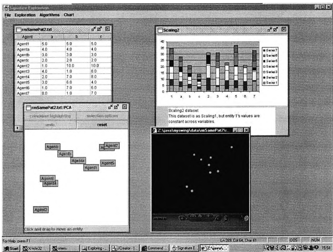
Figure 7.12: Set of windows for the scaling2 generic dataset with PCA applied: spreadsheet, stacked bar chart, 2D and 3D scatterplots.
