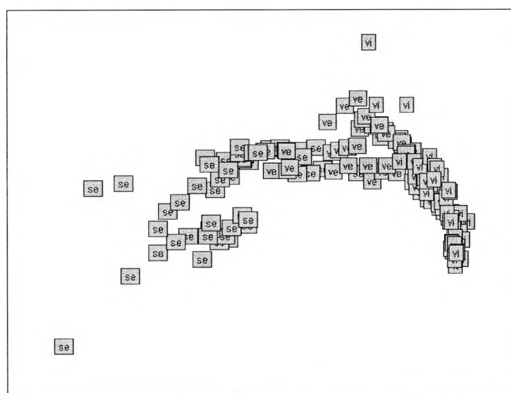
Figure 10.10: The layout of the Iris dataset using weights derived using a genetic algorithm: using polynomial relationship of order 2. Genetic algorithm run for 700 generations, utility 15.
