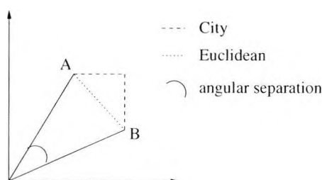
Figure 3.2: Distance measure examples for two-dimensional data. Three ways of measuring the 'difference' between entities A and B: Euclidean distance, City distance and angular separation.
