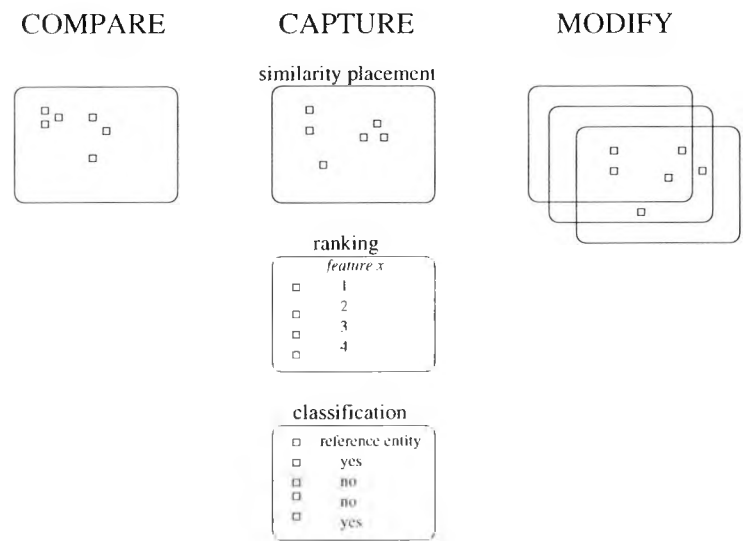
Figure 10.1: The compare, capture, modify process illustrates feedback from system to user and user to system. Left: The user gives known data to the application to see how the system places their data. Middle: The user arranges entities on screen by referring to the actual data or their own intuition. Tacit knowledge can be elicited from the user by ranking or classifying with respect to a reference entity or a feature. Right: The system modifies the algorithm (using for example, least squares multiple regression) and replots or presents different possibilities. New data can then be plotted based upon these results.
