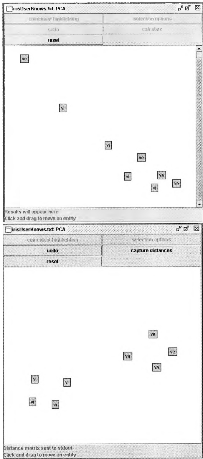
Figure 10.6: Capturing user similarities between entities on screen using a subset of the Iris dataset. Top: before user arrangement. The user can click and drag the entities to wherever they want them to be. When they are satisfied with their arrangement, they click the 'capture distances' button for the distances to be calculated and stored (bottom).
