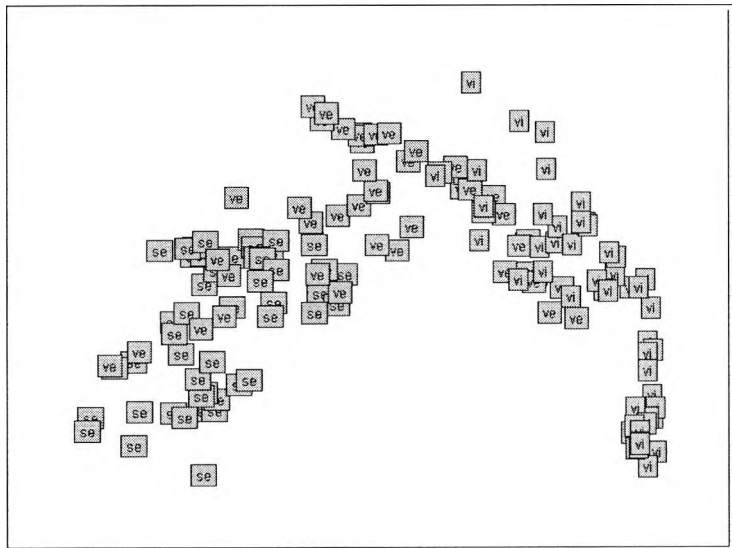
Figure 10.13: The layout of the Iris dataset using weights derived using a genetic algorithm: using polynomial relationship of order 5 (all terms). Genetic algorithm run for 500 generations, utility 22.75.
