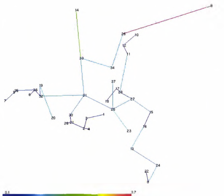
Figure 11.3: Superimposition of coloured minimum spanning tree on a dataset projected from 4 dimensions to 2 using PCA. Coloured scale shows actual Euclidean interdistances calculated in the original space, ranging from 0.1 to 3.7. Large interdistances are represented by red, short ones by a violet-dark blue line.
