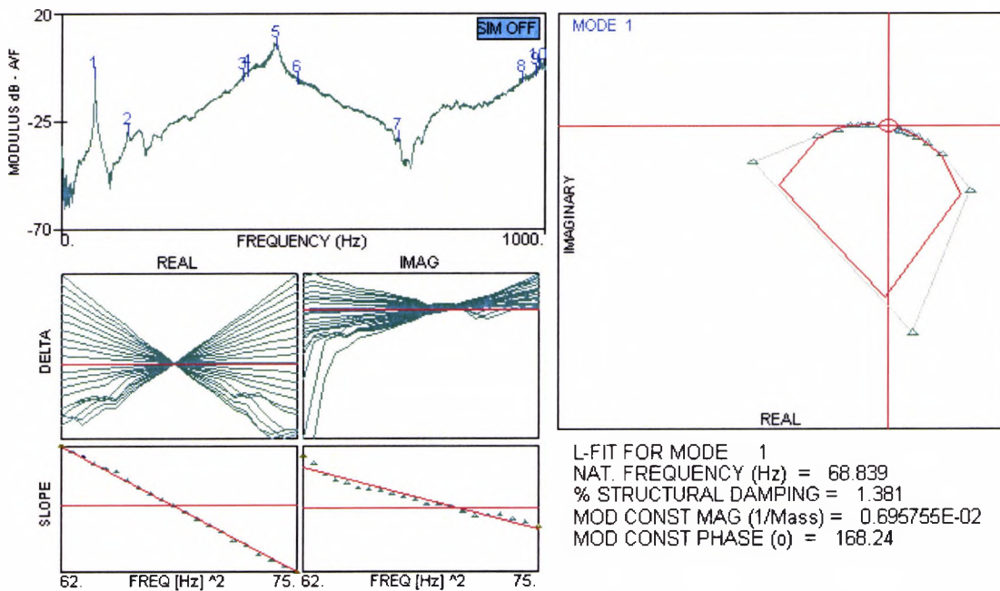
Figure 9.9 Line-fit for first mode for the 0^\circ ply orientation CFRP composite beam
