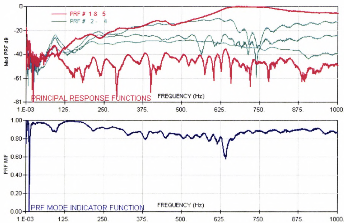
Figure 6.9 Principal response frequencies (PRF) analysis 0-1000 Hz for aluminium-natural rubber-aluminium sandwich composite beam
