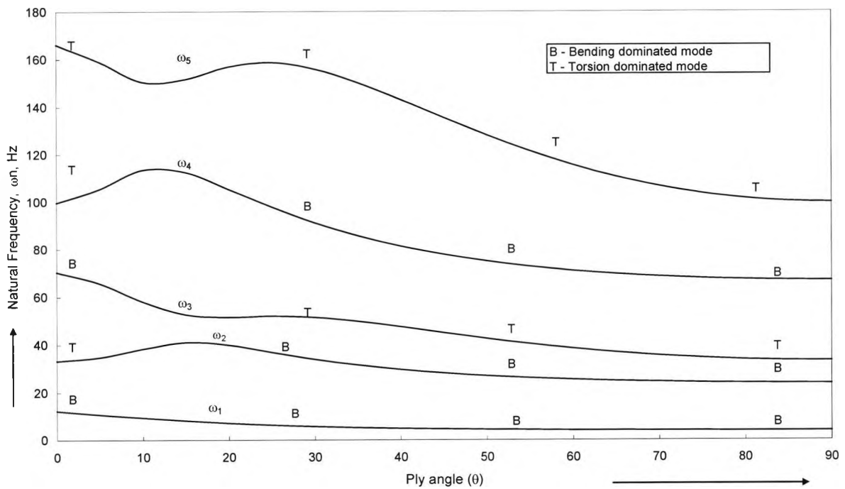
Figure 9.2 Natural frequencies for the MIT beam. \omega_1 - \omega_5 represents the first to the fifth natural frequency while the letters B and T have been used to denote bending or torsion dominated modes.
