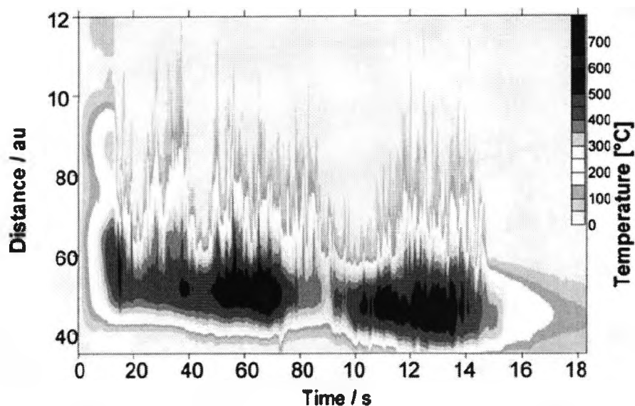
Figure 3.13 Temperature distribution during the burning under ambient conditions.
