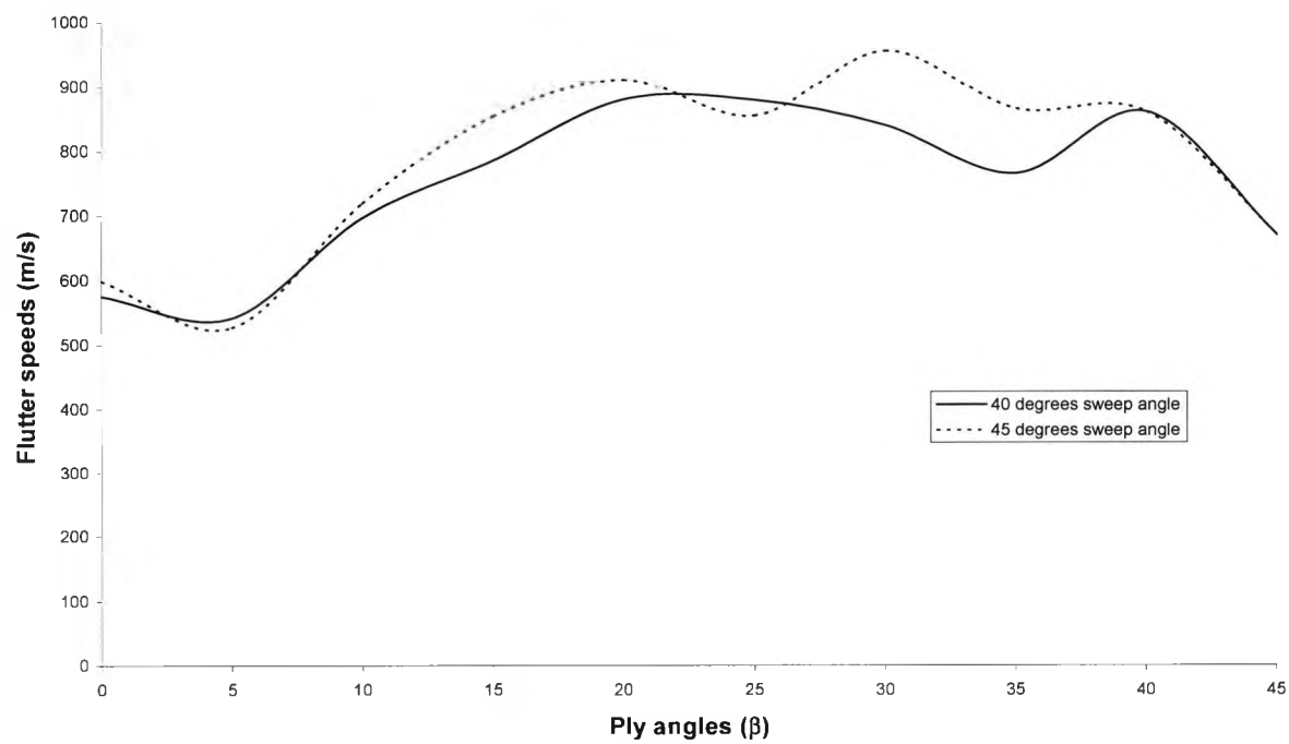
Figure 10.6 The variation of flutter speeds against ply angles at \Lambda = 40^\circ and 45^\circ .
