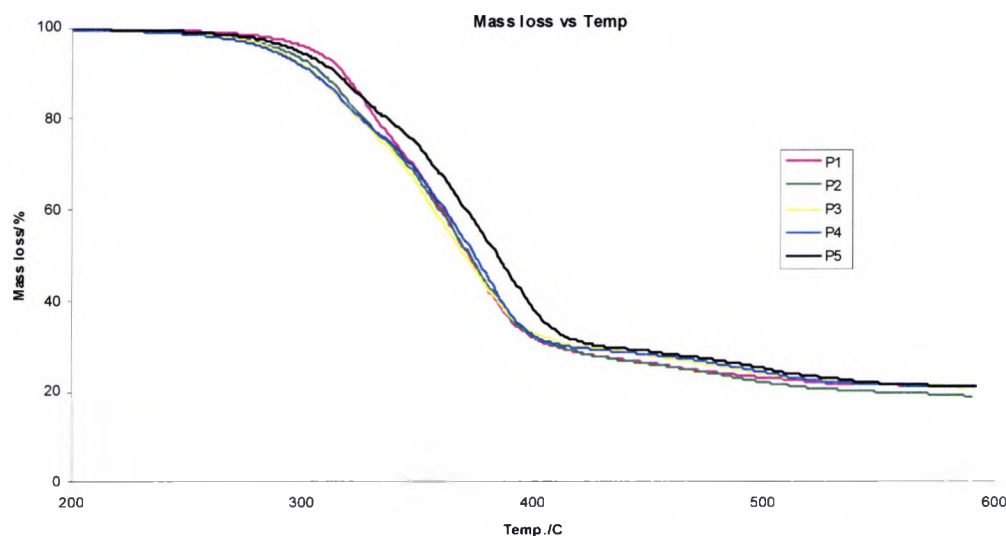
Figure 4.2 The TGA traces under nitrogen conditions of PU and PU/PANI samples displaying the mass loss against temperature
