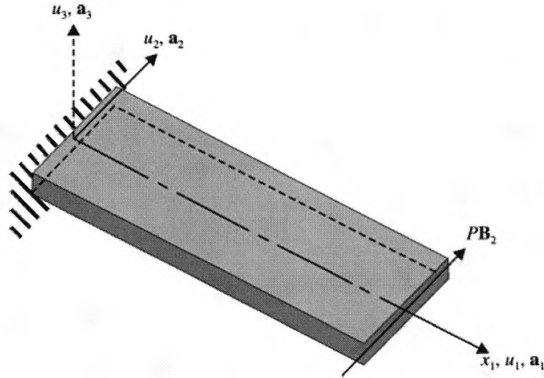
Figure 2.2 Schematic of wing showing co-ordinate systems and follower force [2.128].
