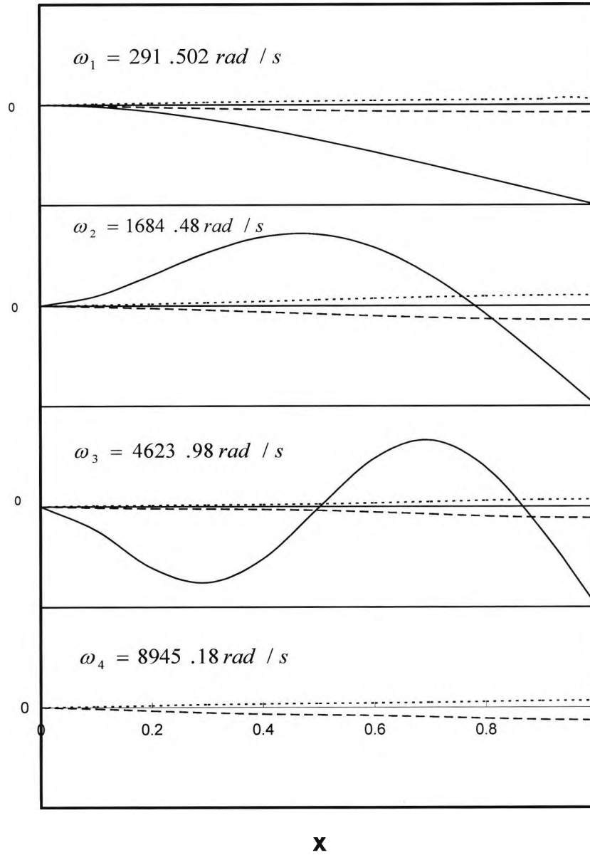
Figure 6.3 Natural frequencies and mode shapes of the three-layered sandwich beam of Example 1 (....) U_1 ; (---) U_3 ; (—) W
