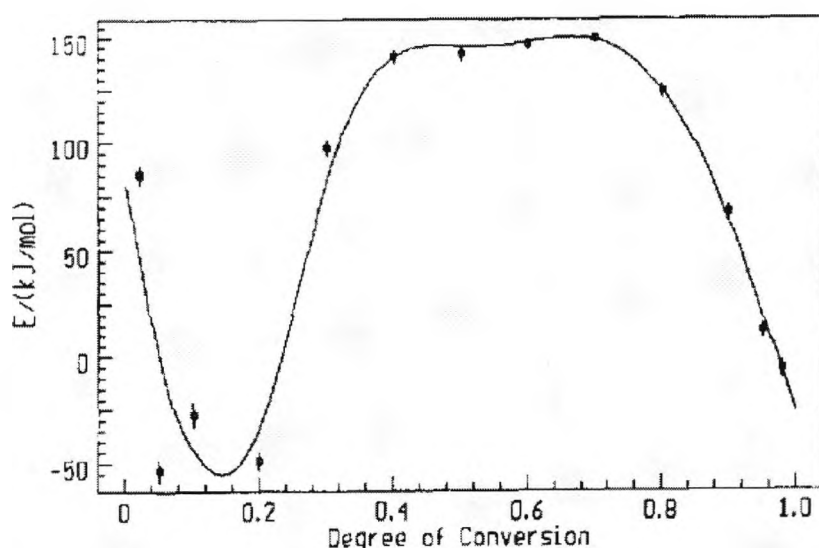
Figure 3.9 Energy of activation ( E ) as a function of the degree of conversion of degradation process of PANI in its emeraldine salt form under air calculated by Ozawa-Flynn-Wall method.
