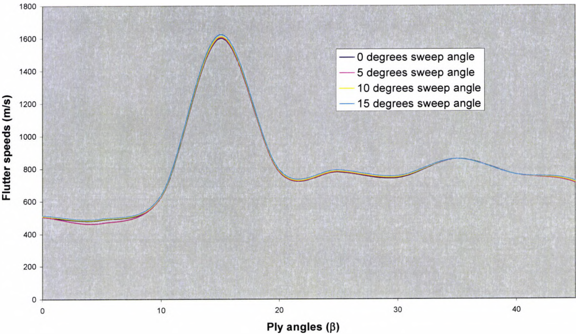
Figure 10.8 The variation of flutter speeds against ply angles at \Lambda = 0^\circ - 15^\circ .
