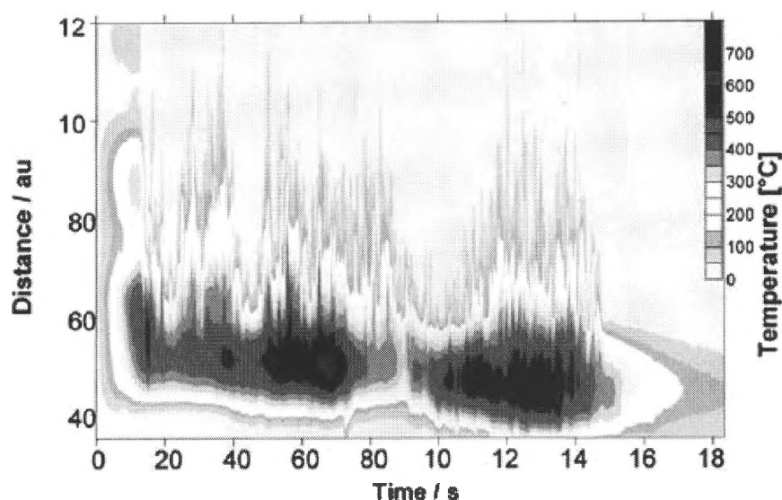
Figure 3.12 Temperature distribution during the burning under LOI conditions.
