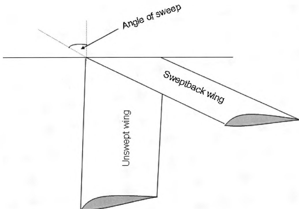
Figure 10.1 An illustration of a conventional unswept and sweptback aircraft wing
