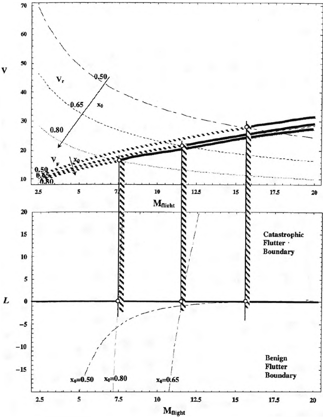
Figure 2.5 Benign and catastrophic portions of the flutter critical boundary as a function of the elastic axis position [2.136].
