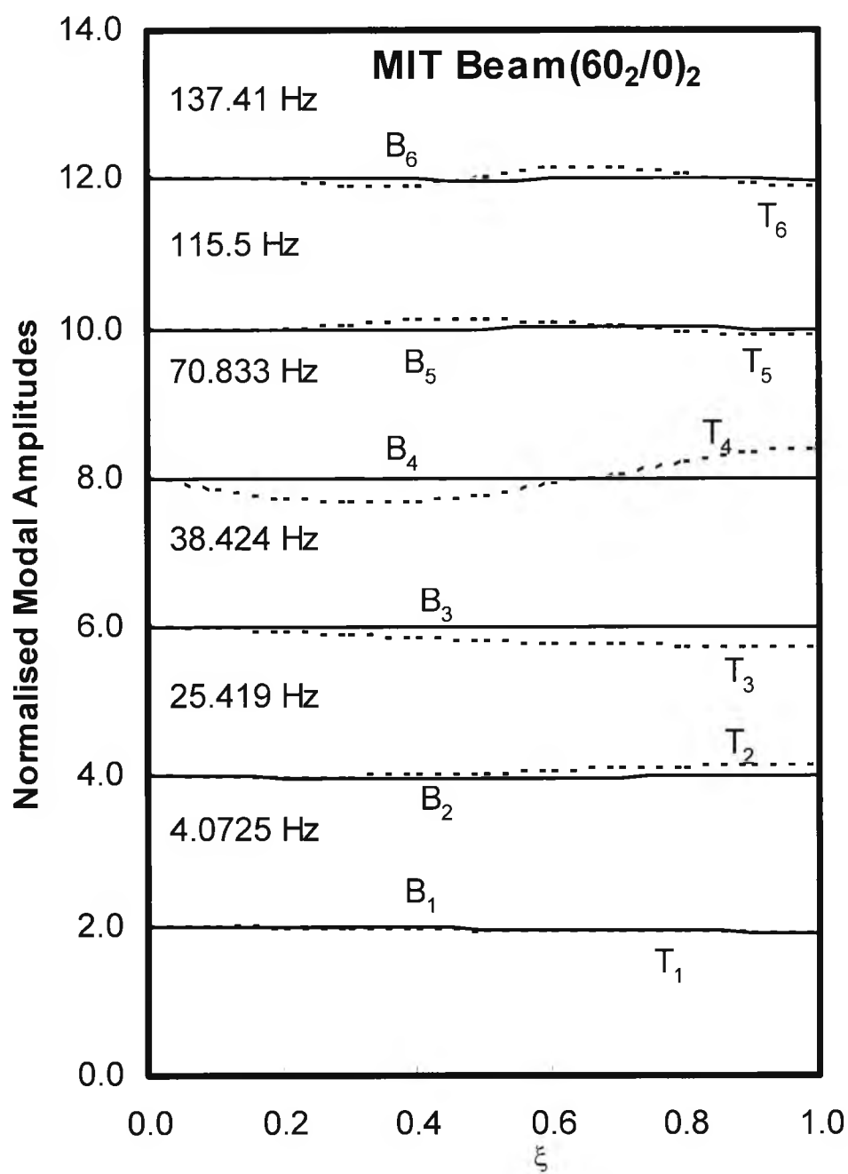
Figure 9.4(c) \theta = 60 . The letters B and T have been used to denote bending or torsion dominated modes and the numbers 1-6 represent mode numbers.
