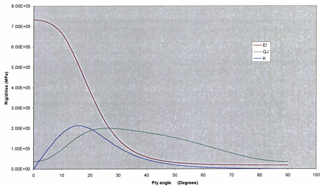
Figure 10.3 The effect of ply orientation on rigidity properties for GIT beam
