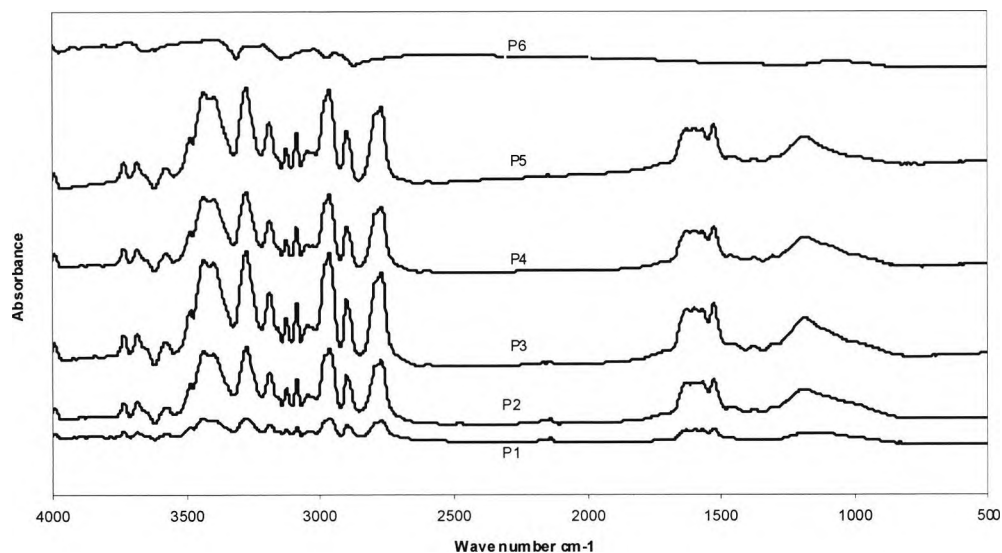
Figure 4.4 FTIR spectra of PU, PU/PANI and PANI samples
