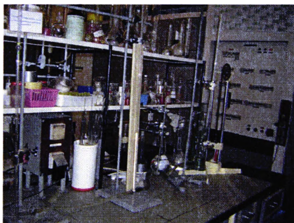
Figure 3.4 Typical experimental set up for the synthesis of PU, PANI, PU/PANI and PU/MMT thermoplastic elastomers (top) and a selection some of the test equipment (below) used in the experiments
