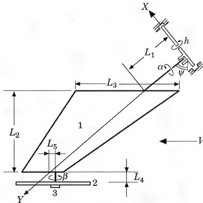
Figure 2.3 Sketch of wing/store model. 1 wing; 2 store; 3 electromagnetic friction damper [2.132].
