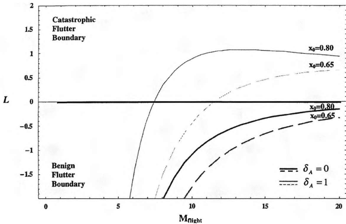
Figure 2.4 Influence of the aerodynamic non-linearities and of the elastic axis position on the first Liapunov quantity, L , in the presence of physical non-linearities [2.136].
