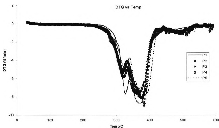
Figure 4.3 The TG results under nitrogen conditions of PU and PU/PANI showing the DTG against temperature
