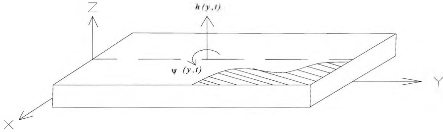
Figure 7.1 Coordinate system and sign convention for positive ply angle of a laminated composite beam
