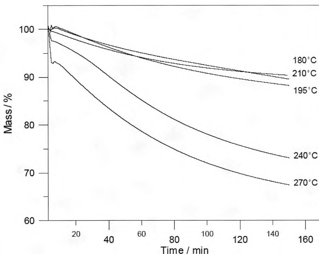
Figure 3.7 Thermogravimetric profiles under isothermal conditions.
