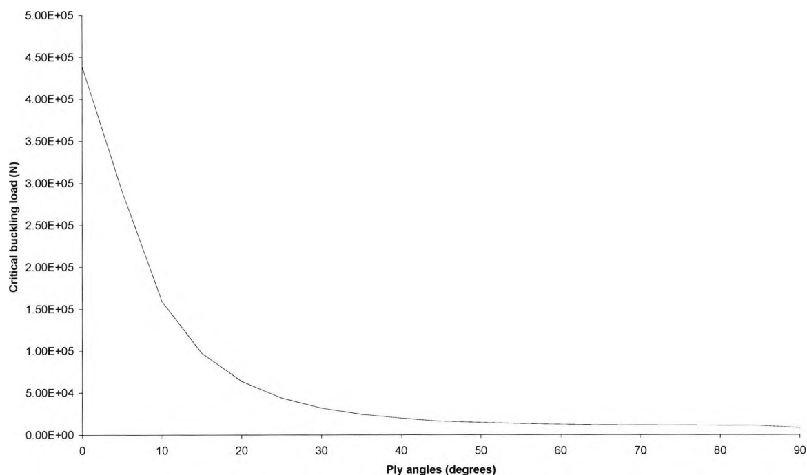
Figure 8.5 The critical buckling load for GIT beam
