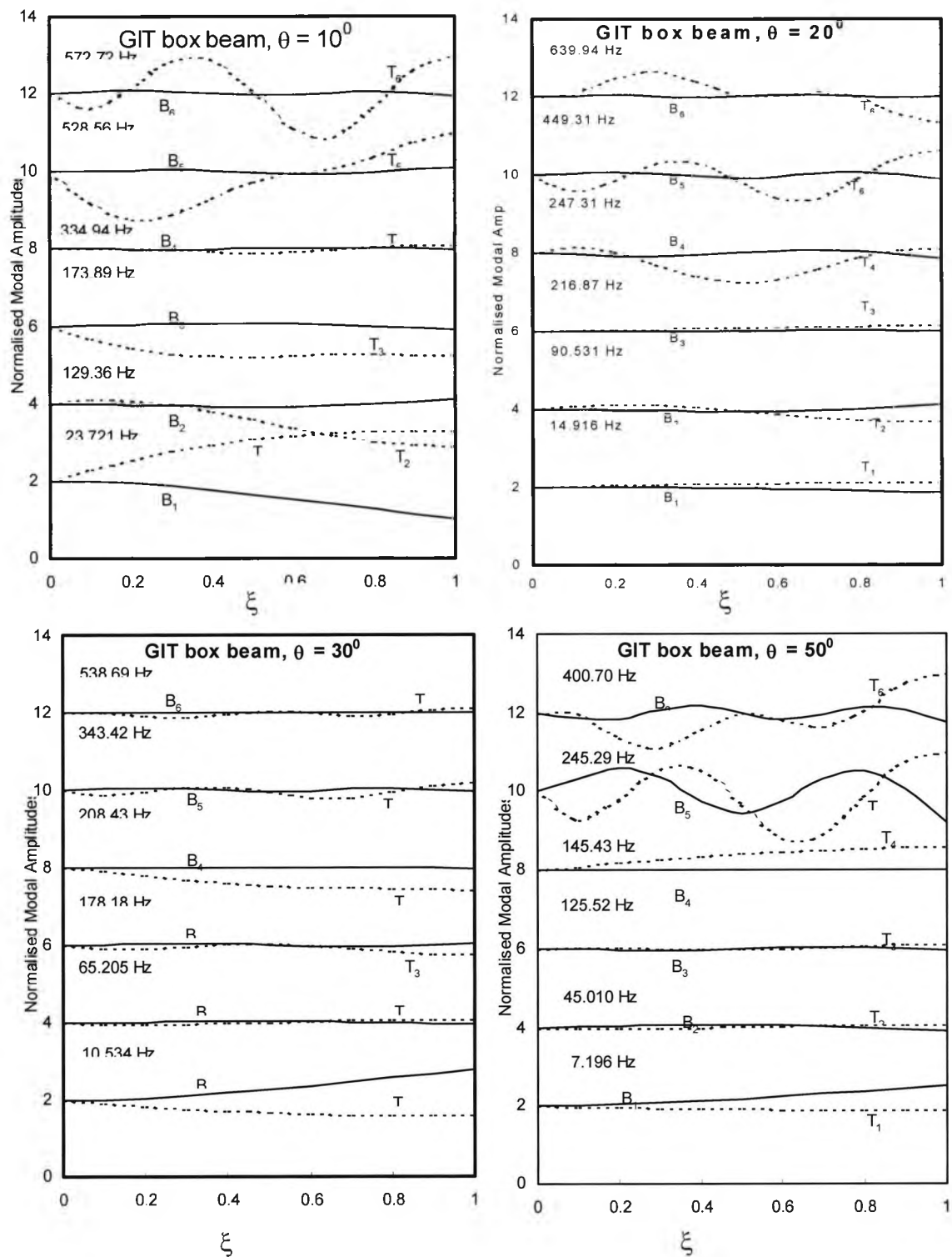
Figure 9.5 The modal amplitudes for the GIT box-beam, with ply angles of (a) \theta = 10^\circ (b) \theta = 20^\circ , (c) \theta = 30^\circ and (d) \theta = 50^\circ . The letters B and T have been used to denote bending or torsion dominated modes and the numbers 1-6 represent mode numbers.
