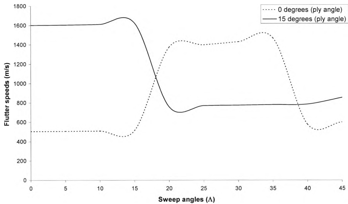
Figure 10.5 Flutter speeds against sweep angles at \beta = 0^\circ and \beta = 15^\circ .
