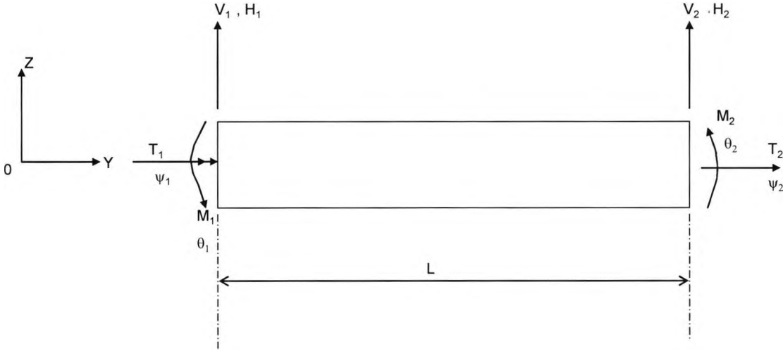
Figure 8.3 End conditions for forces and displacements at the elastic axis
