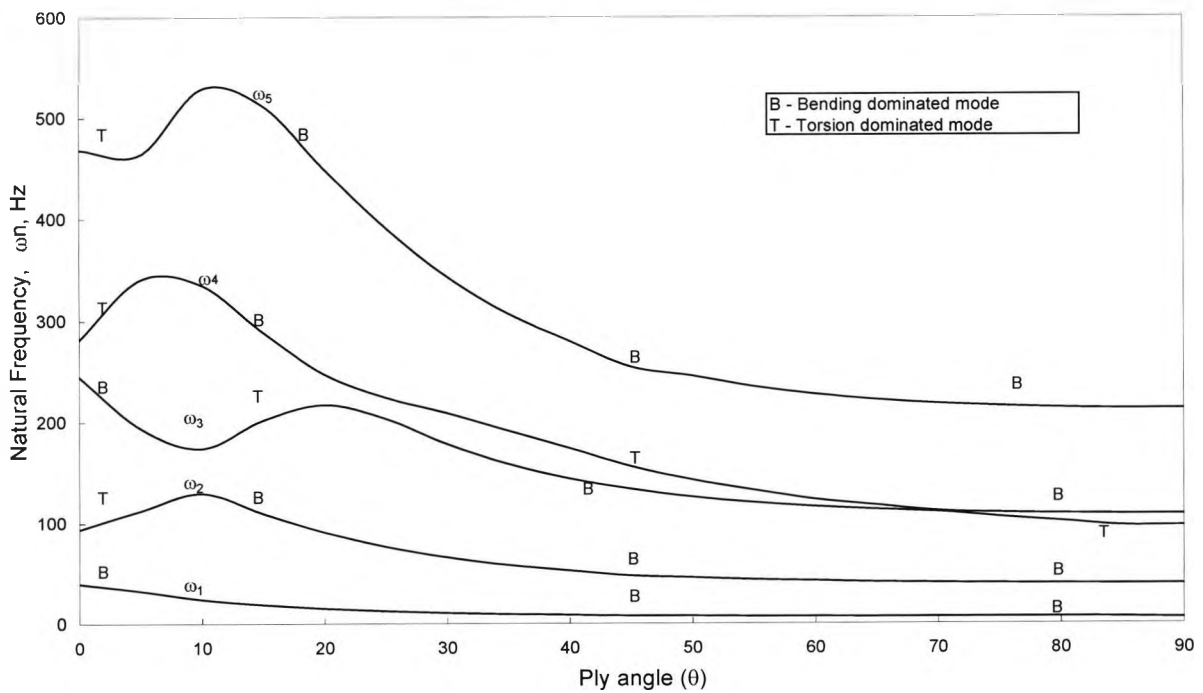
Figure 9.3 Natural frequency for the GIT beam. \omega_1 - \omega_5 represents the first to the fifth natural frequency while the letters B and T have been used to denote bending or torsion dominated modes.
