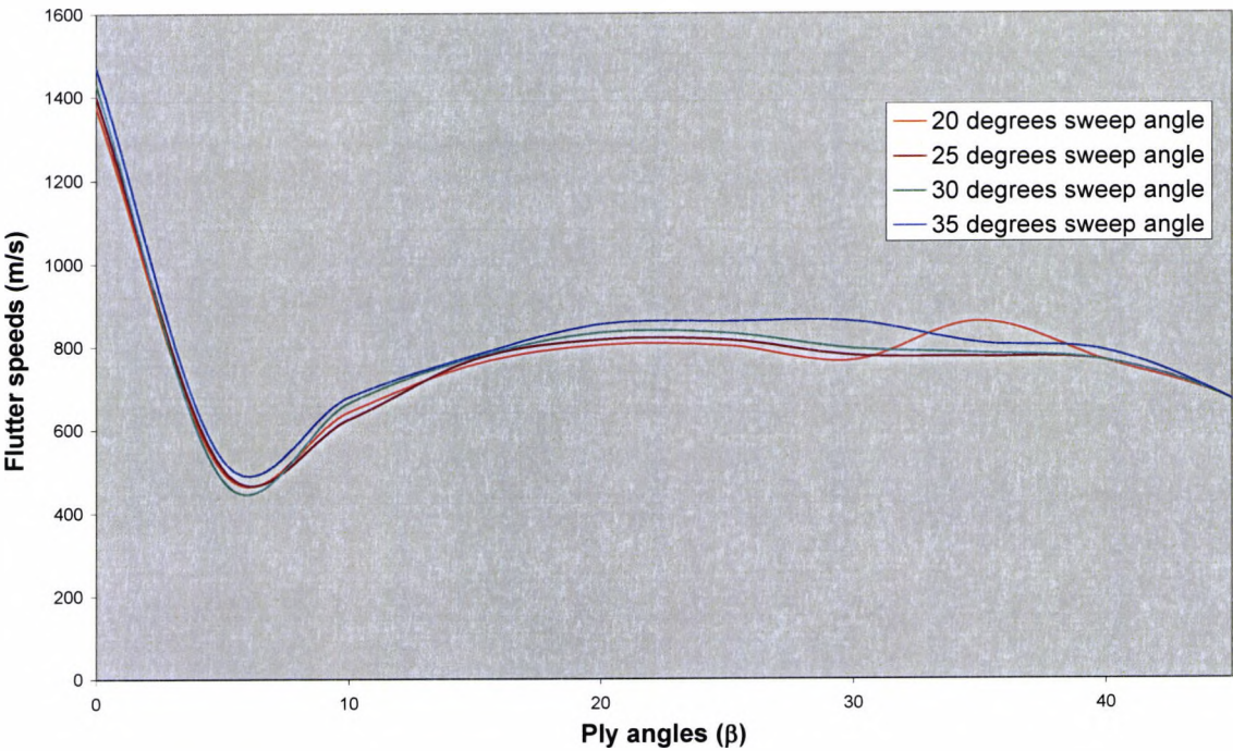
Figure 10.7 The variation of flutter speeds against ply angles at \Lambda = 20^\circ - 35^\circ .
