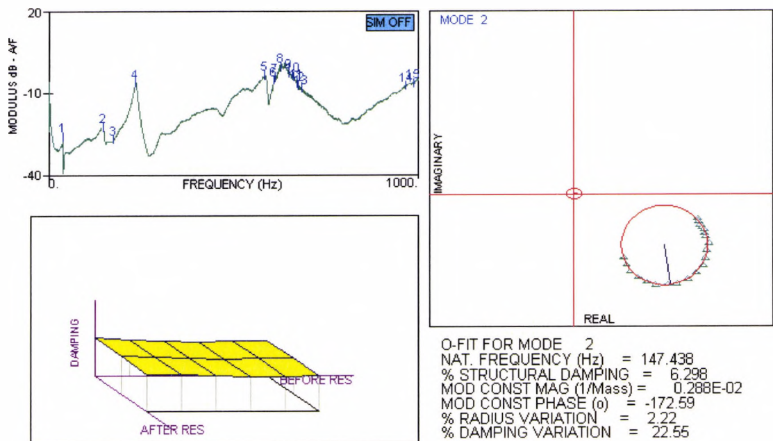
Figure 9.8 Circle-fit for second mode for the 25° ply orientation CFRP composite beam
