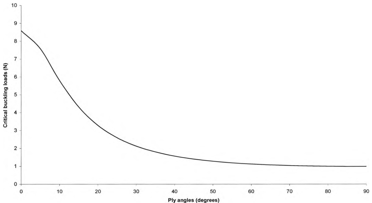
Figure 8.4 The influence of ply angle orientation into critical buckling load for the MIT beam
