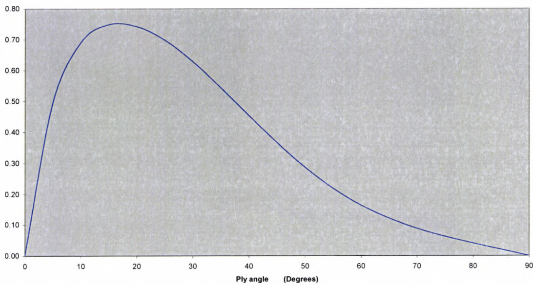
Figure 10.4 The effect of ply orientation on the coupling parameter \psi for GIT beam
