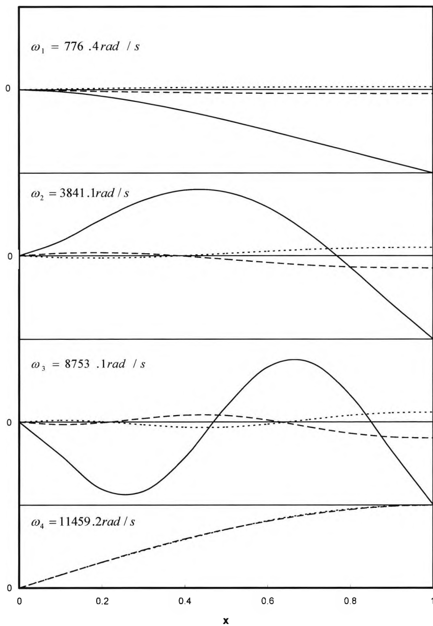
Figure 6.4 Natural frequencies and mode shapes of the three-layered sandwich beam of Example 2 (....) U_1 ; (---) U_3 ; (-) W
