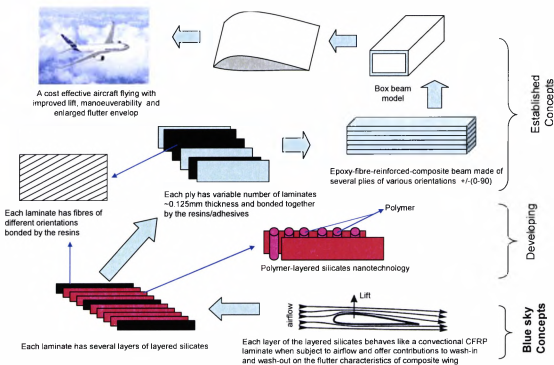
Figure 5.7 Futurist application of polymer nanocomposites incorporated into carbon-fibre reinforced composites
