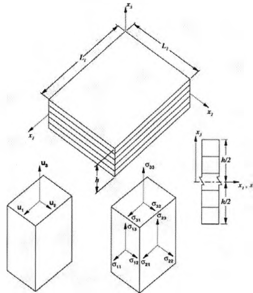
Figure 2.1 Laminated panel: geometry, coordinates axes, and sign convention for displacements and stresses
