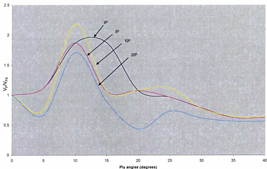
Figure 10.2 The effect of ply orientation on unswept ( 0^\circ ) and swept-back wings ( 5^\circ – 20^\circ )
