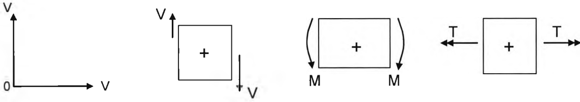
Figure 8.2 Sign conversion for positive shear force (V) bending moment (M) and torque (T) at the elastic axis.
