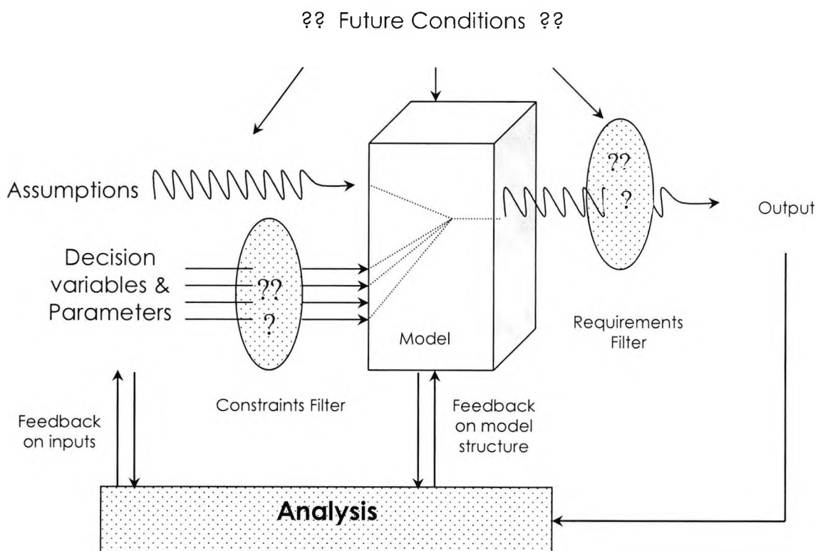
Figure 10.4: Uncertainty Analysis flow chart
