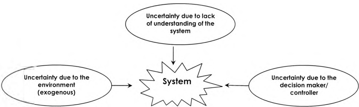
Figure 10.1: The sources of uncertainty in a systemic framework.
