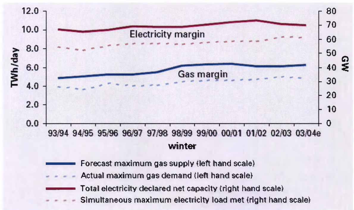
Figure 8.3: Gas and electricity capacity margins – maximum supply and maximum demand 1993/4 to 2003/4 [DTI-SEP]
