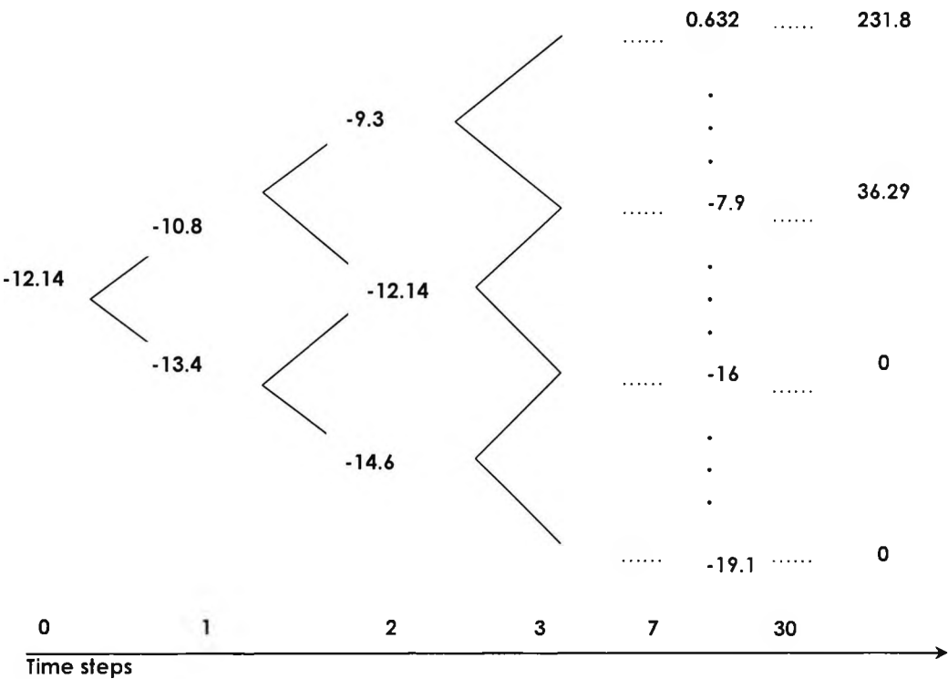
Figure 9.6: The binomial value lattice
