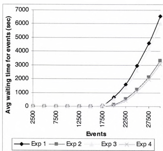
Figure 6.9a: Average waiting time for events due to recorded events and large inter arrival time of events (EL)
