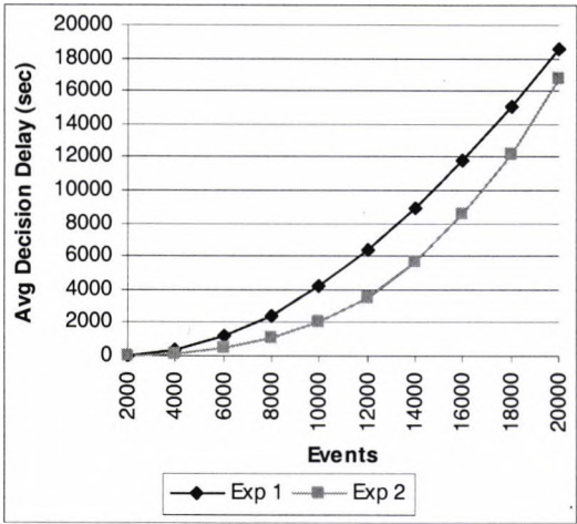
Figure 6.12a: Average d-delay due to small inter arrival time of events
