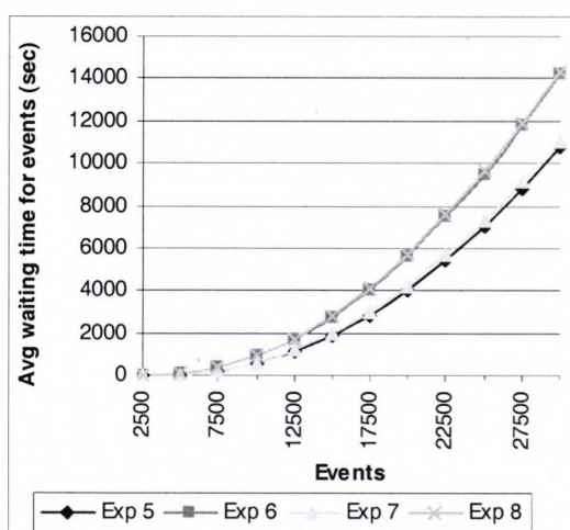
Figure 6.9b: Average waiting time for events due to recorded events and small inter arrival time of events (ES)
