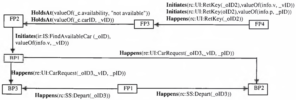
Figure 4.7: Formula interdependency graph
