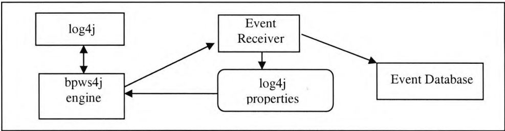
Figure 5.6: Event generation from bpws4j engine
