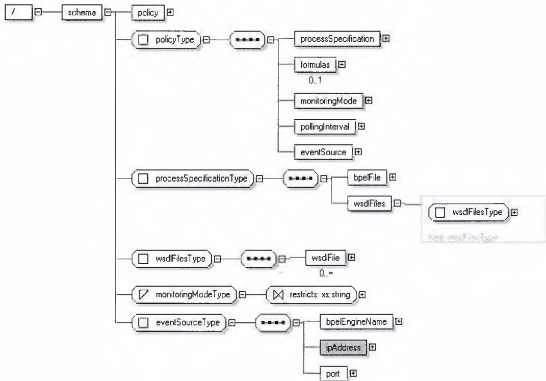
Figure 3.1: Graphical view of the monitoring policy schema
