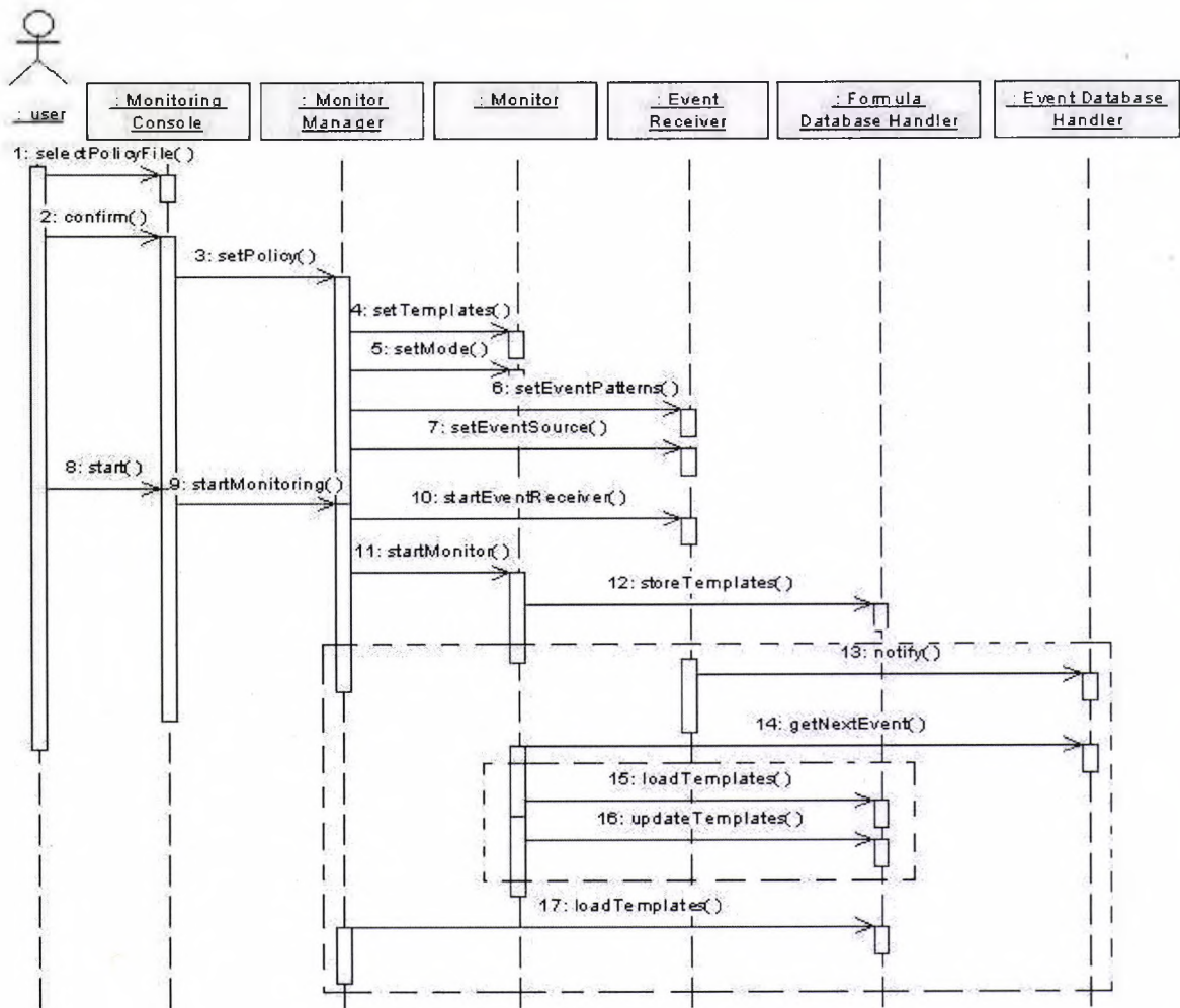
Figure 5.8. A typical user interaction scenario with the monitoring framework
