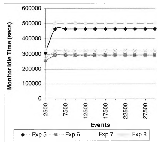
Figure 6.7b: Monitor's idle time due to recorded events and small inter arrival time of events (ES)
