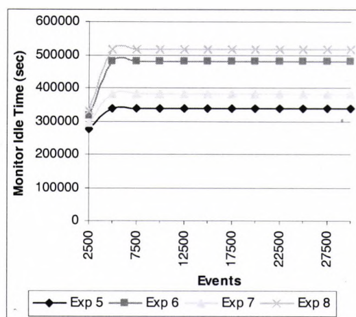
Figure 6.8b: Monitor's idle time due to mixed events and small inter arrival time of events (ES)
