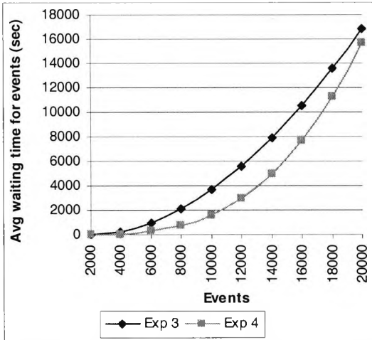
Figure 6.14b: Average waiting time for events due to large inter arrival time of events
