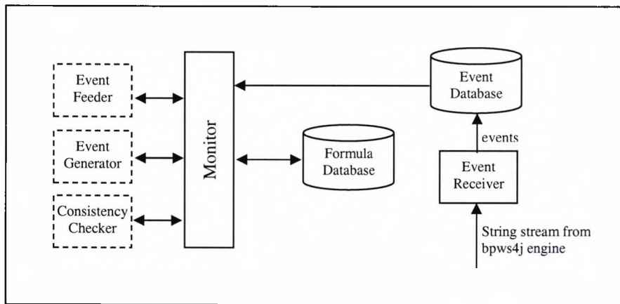
Figure 4.5: Runtime components of the monitoring architecture
