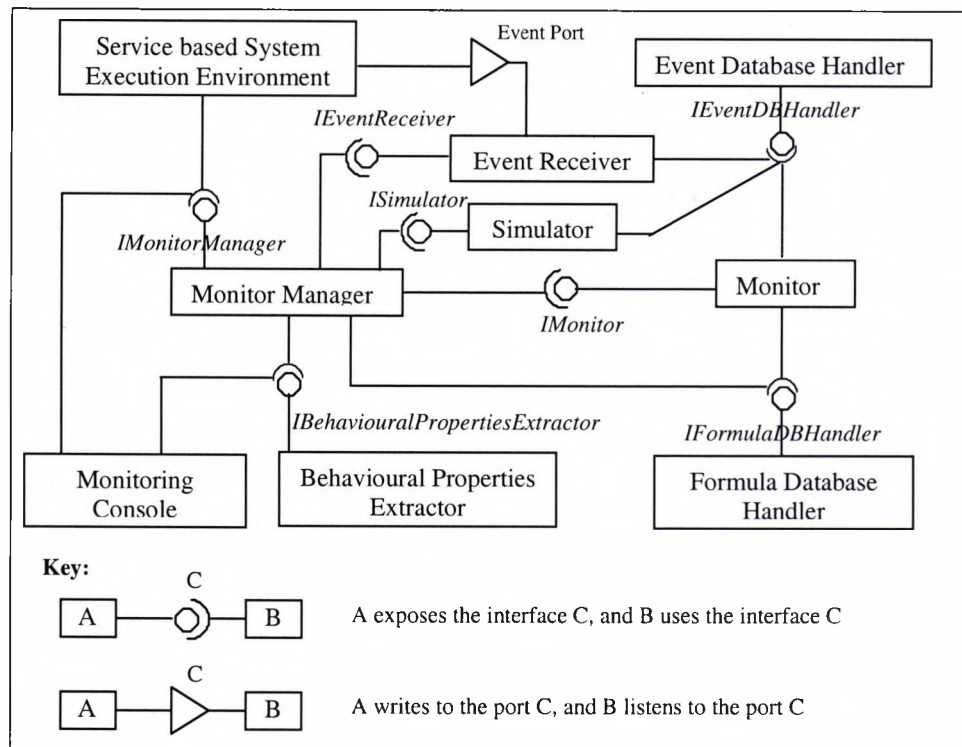
Figure 5.1: Implementation architecture of the monitoring framework
