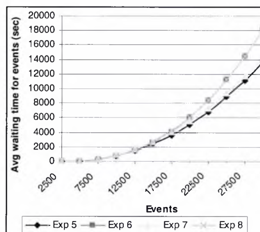
Figure 6.10b: Average waiting time for events due to mixed events and small inter arrival time of events (ES)
