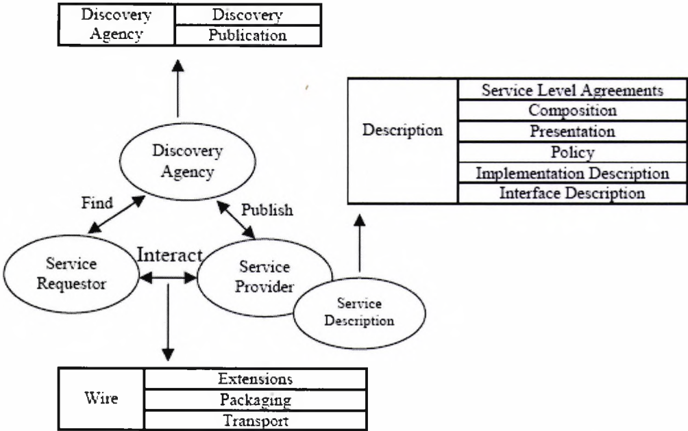
Figure 2.3: Mapping between basic web service architecture and extended web service architecture
