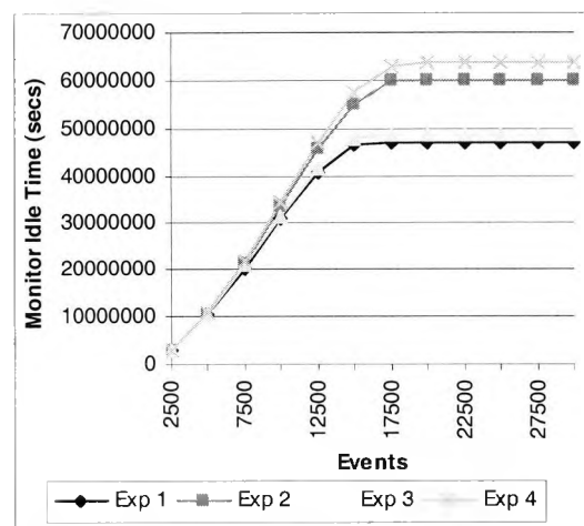
Figure 6.7a: Monitor's idle time due to recorded events and large inter arrival time of events (EL)
