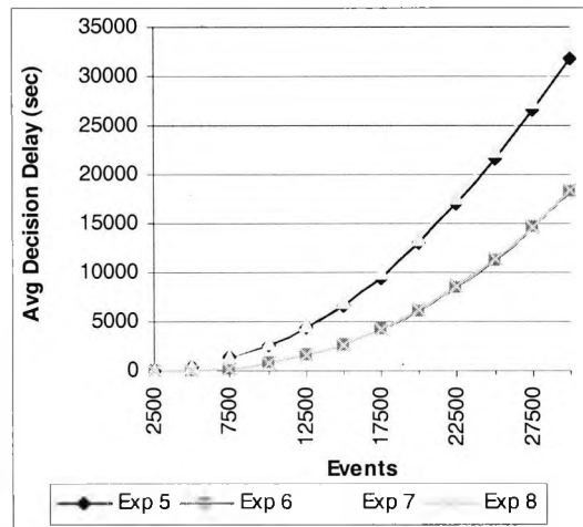
Figure 6.6b: Average d-delay due to mixed events and small inter arrival time of events (ES)
