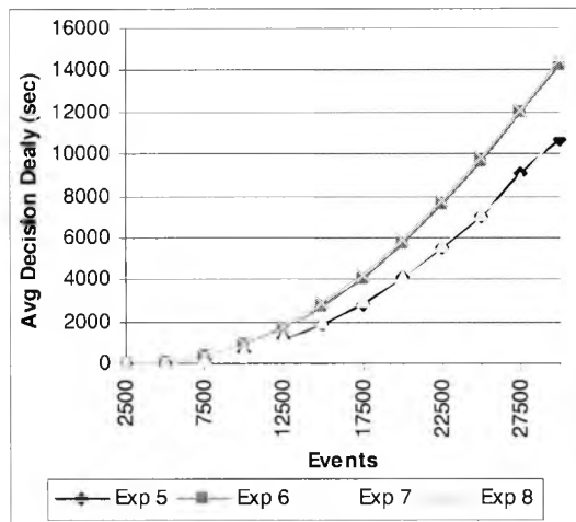
Figure 6.5b: Average d-delay due to recorded events and small inter arrival time of events (ES)
