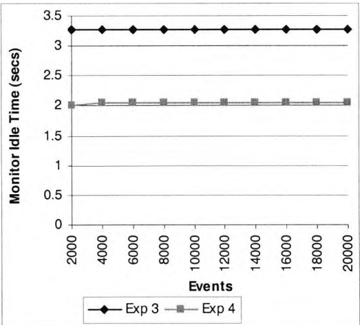
Figure 6.13b: Monitor's idle time due to large inter arrival time of events
