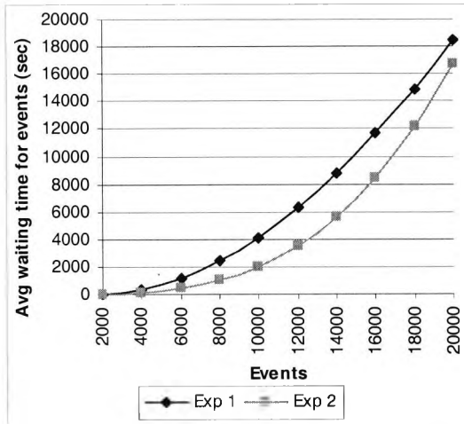
Figure 6.14a: Average waiting time for events due to small inter arrival time of events
