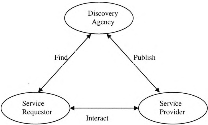
Figure 2.1: Basic web-service architecture
