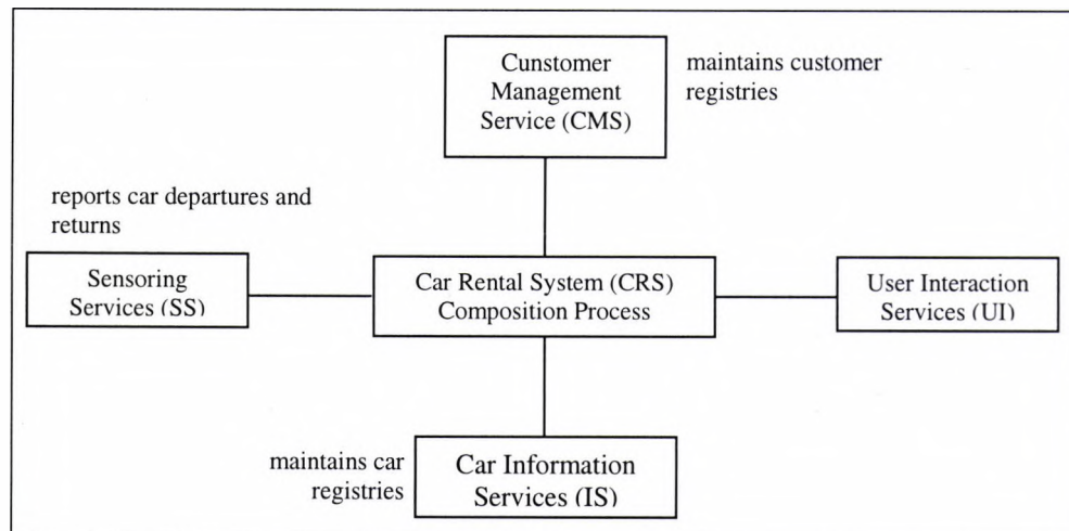
Figure 4.1: Structure of the car rental system (CRS)
