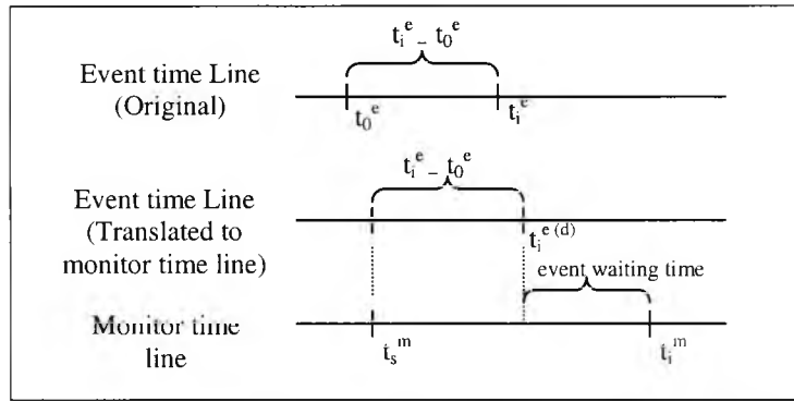
Figure 6.1: Event waiting time
