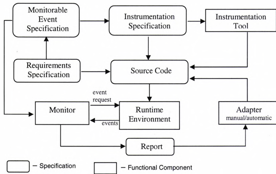
Figure 2.14: A general framework for requirements monitoring
