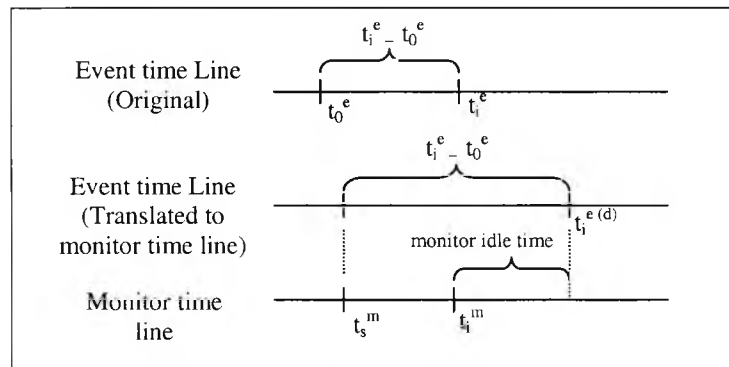
Figure 6.2: Monitor's idle time
