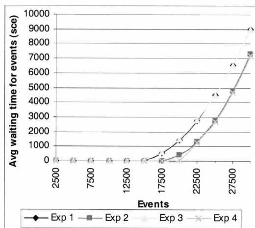
Figure 6.10a: Average waiting time for events due to mixed events and large inter arrival time of events (EL)
