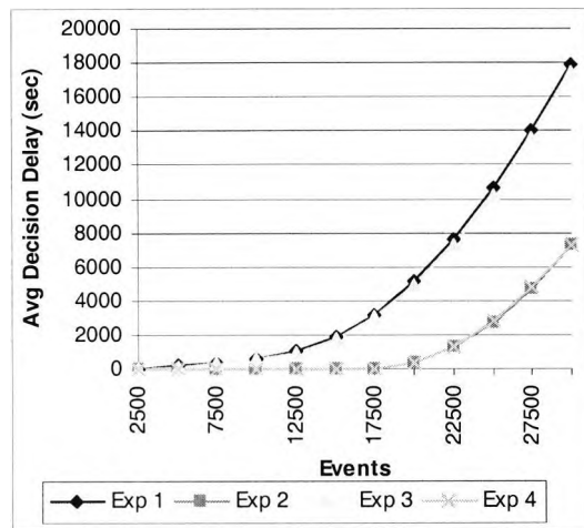
Figure 6.6a: Average d-delay due to mixed events and large inter arrival time of events (EL)
