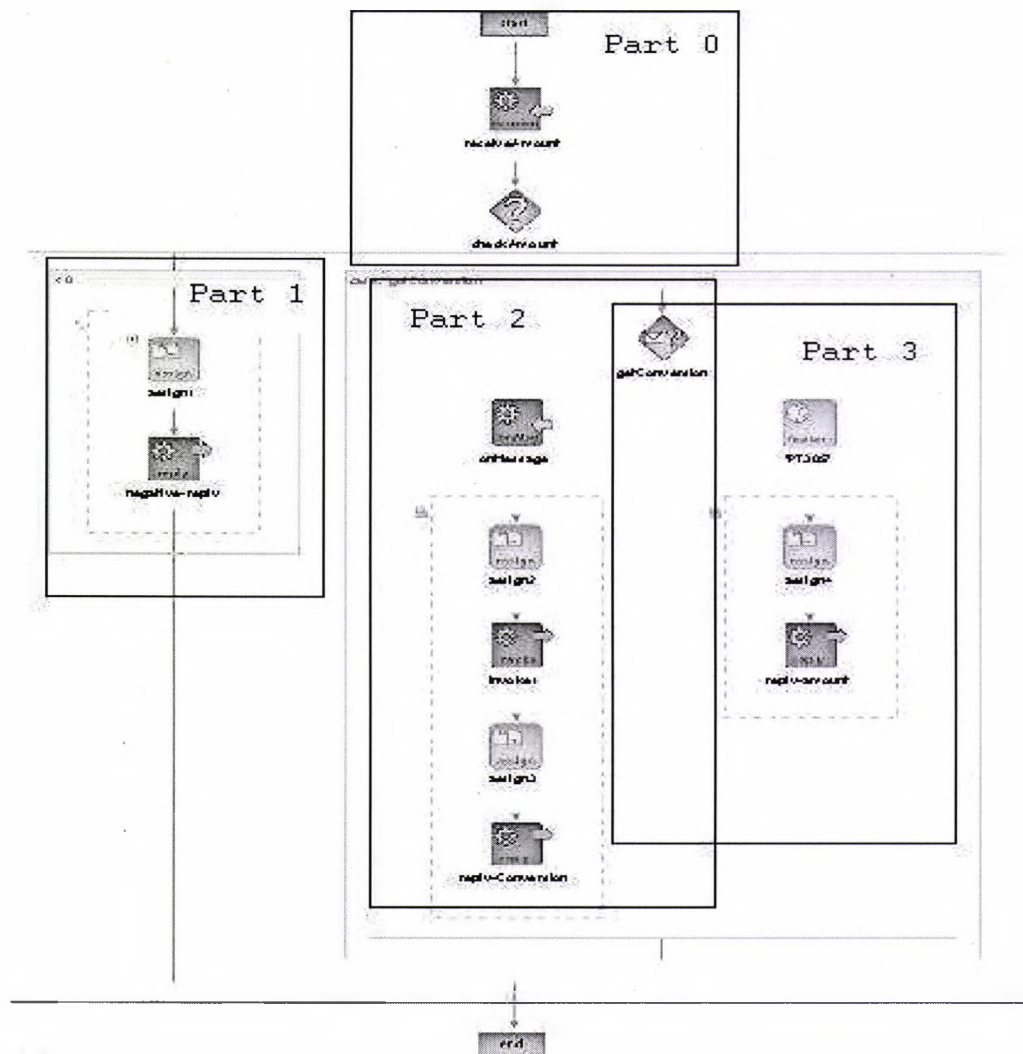
Figure 5.4: Sequences of activities in the Rate Tracker BPEL process
