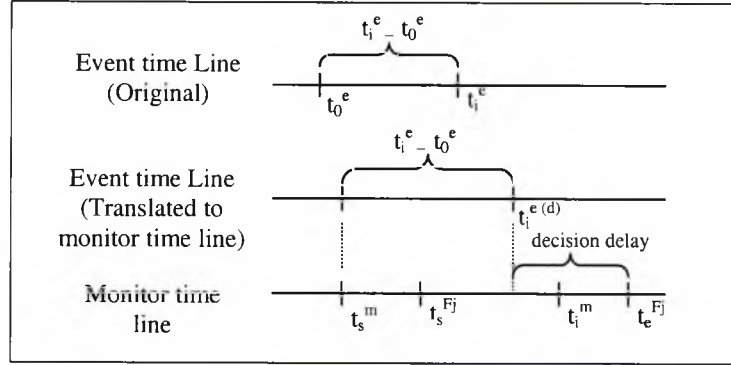
Figure 6.3a: Decision delay
