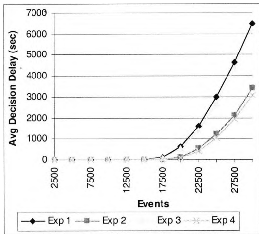
Figure 6.5a: Average d-delay due to recorded events and large inter arrival time of events (EL)
