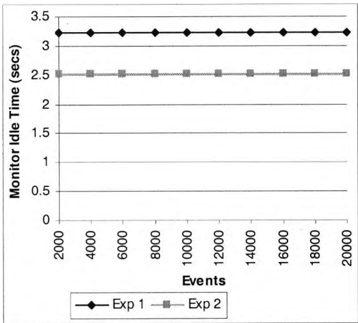
Figure 6.13a: Monitor's idle time due to small inter arrival time of events
