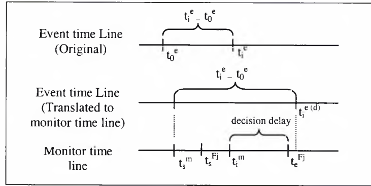
Figure 6.3b: Decision delay
