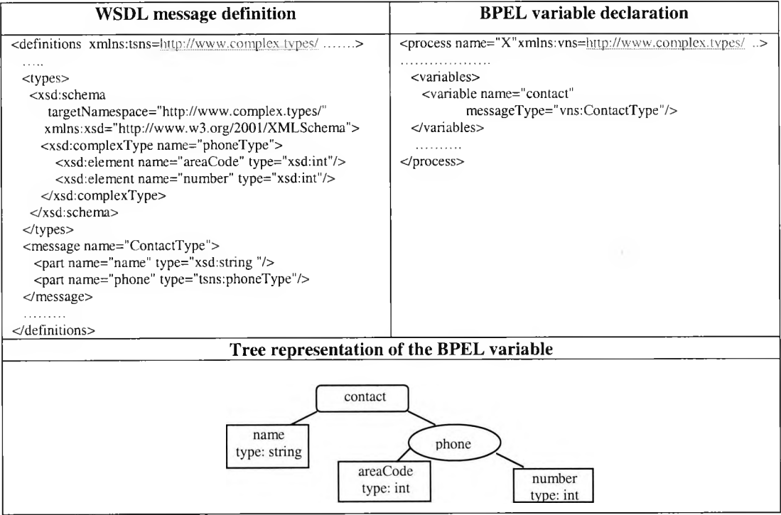
Figure 3.2: Tree representation of BPEL variable
