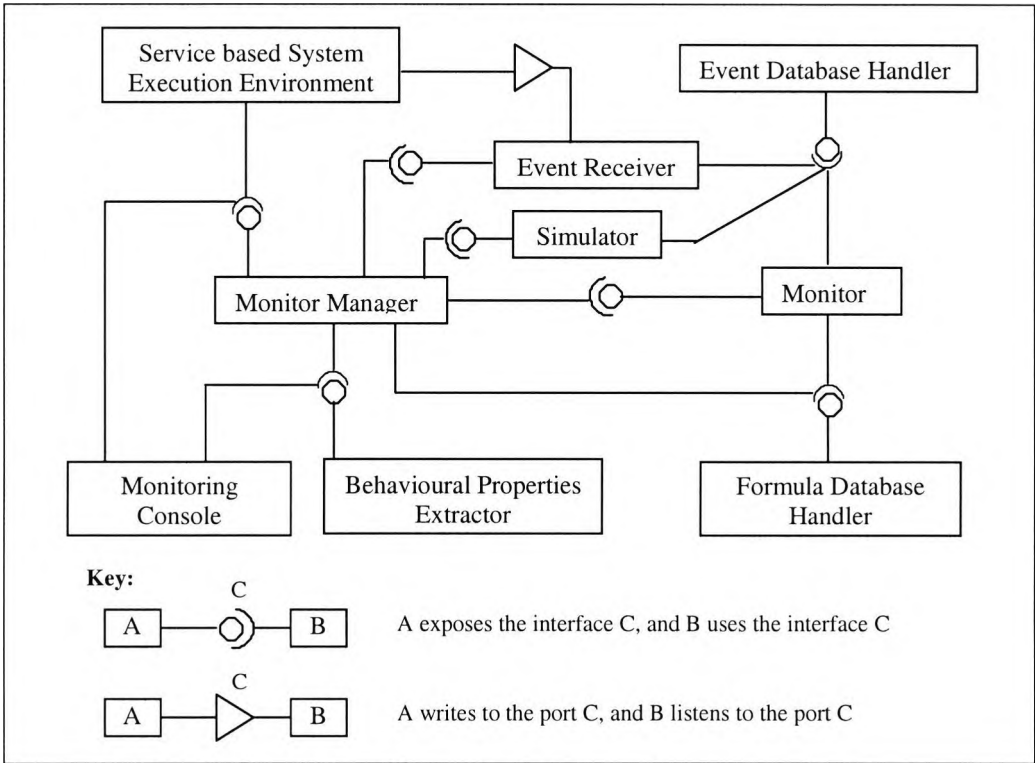
Figure 2.15: Architecture of the monitoring framework
