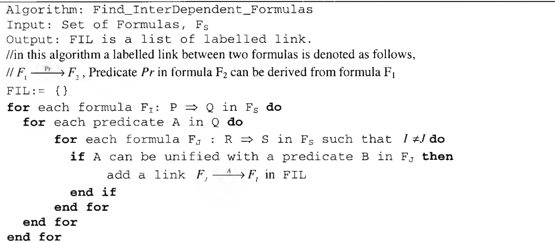
Figure 4.6: Formula interdependency identification algorithm
