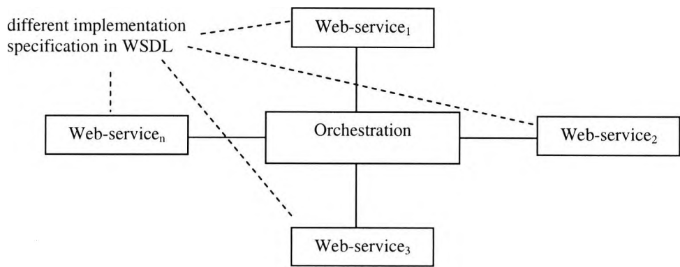
Figure 2.10: Web service orchestration
