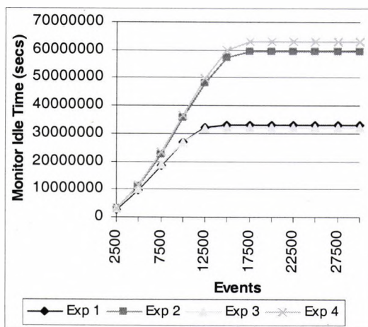
Figure 6.8a: Monitor's idle time due to mixed events and large inter arrival time of events (EL)
