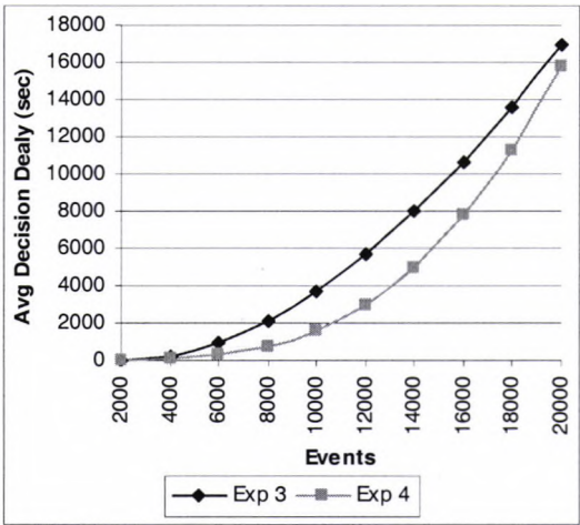
Figure 6.12b: Average d-delay due to large inter arrival time of events
