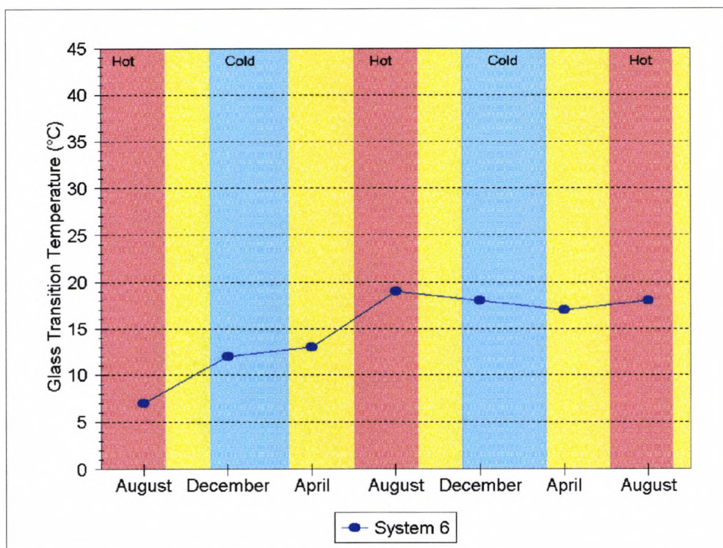
Figure 9.3.3. Variation of T_g of an alkyd-acrylic hybrid with month of measurement.
