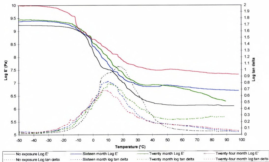
Figure 9.3.1.3.b. The effect of up to twenty-four months natural weathering on System 2
