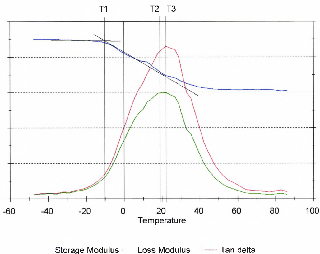
Figure 8.3.3. DMTA plot of an unexposed, unpigmented alkyd (System 1).
