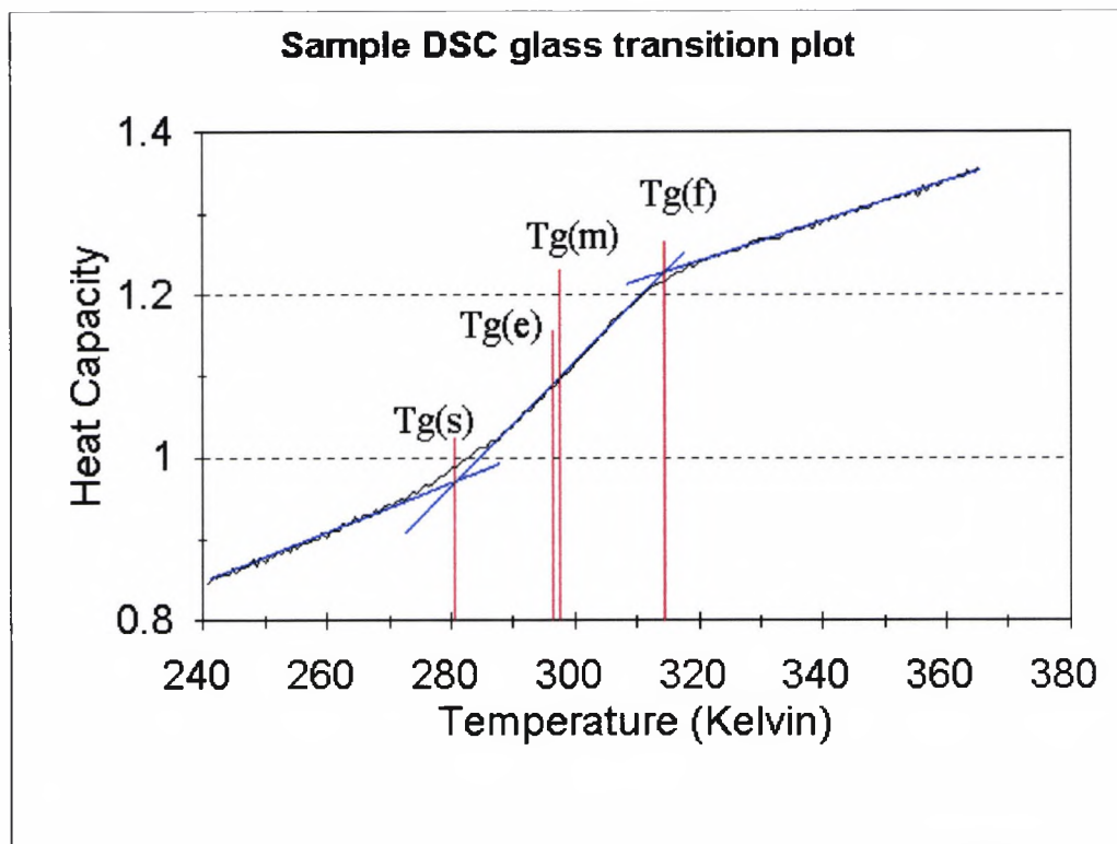
Figure 8.2. Glass transition plot of an unexposed traditional pigmented alkyd. The black trace is from the original data, blue lines are the intersection lines, and the red lines show the T_g s.
