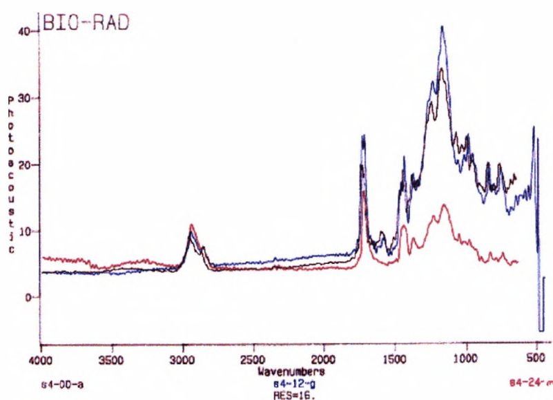
Figure 9.4.3.1. The effect of natural exposure on the infra-red spectra of System 4. The black, blue and red spectra are of the coating unexposed, and after 12, and 24 months respectively.
