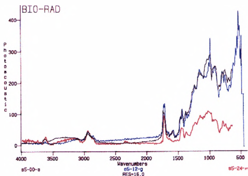
Figure 2.4.3.2. The effect of natural exposure on the infra-red spectra of System 5. The black, blue and red spectra are of the coating unexposed, and after 12, and 24 months respectively.
