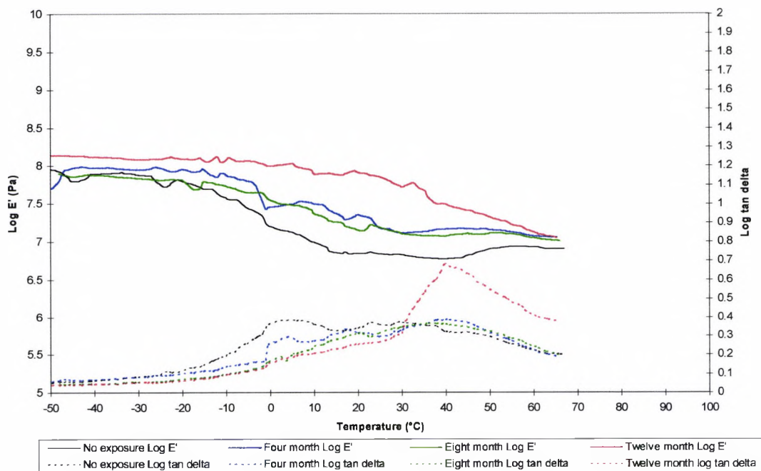
Figure 9.3.3.a. The effect of up to twelve months natural weathering on System 6
