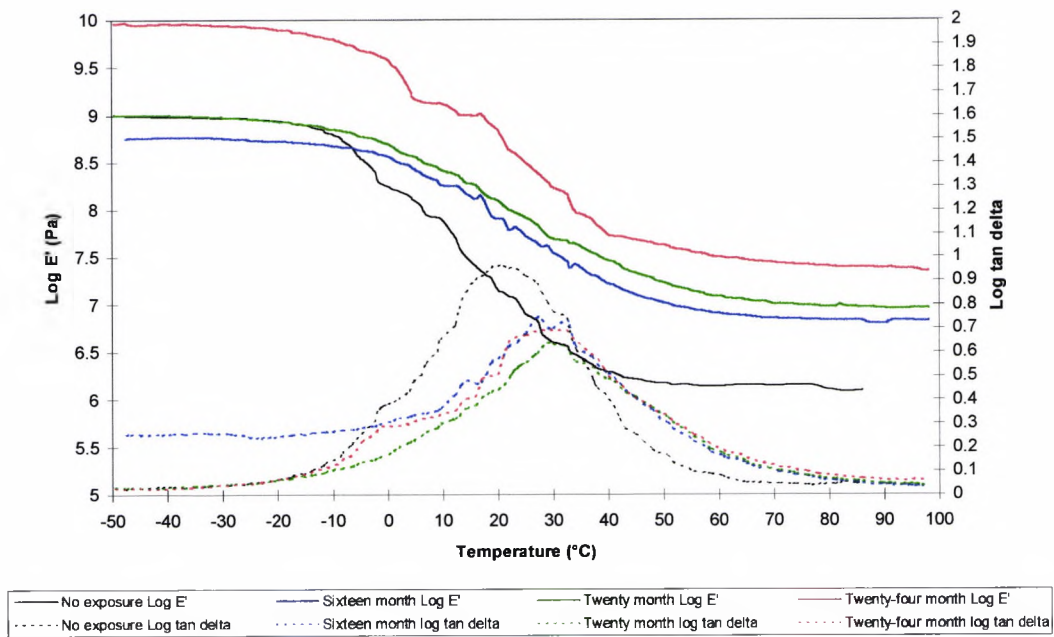
Figure 9.3.1.2.b. The effect of up to twenty-four months natural weathering on System 1
