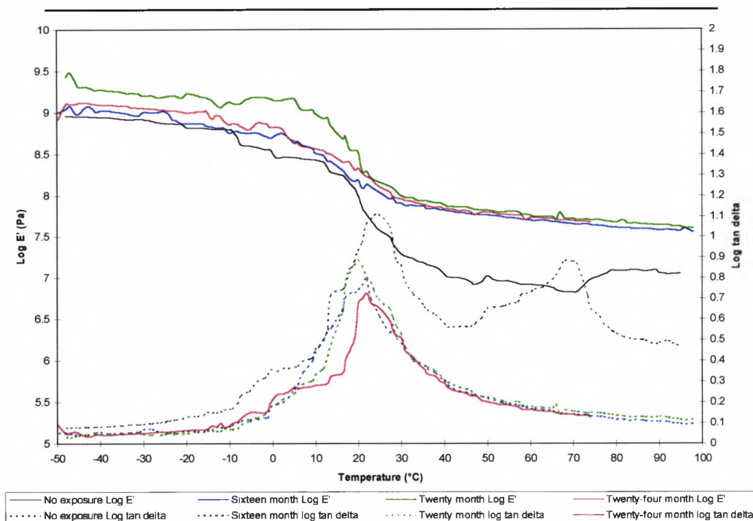
Figure 9.3.2.3.b. The effect of up to twenty-four months natural weathering on System 5
