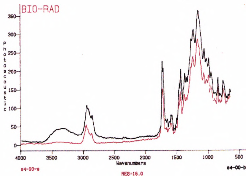
Figure 9.4.1.2. Unexposed System 4. The two spectra are taken from different samples, within a few minutes of each other.
