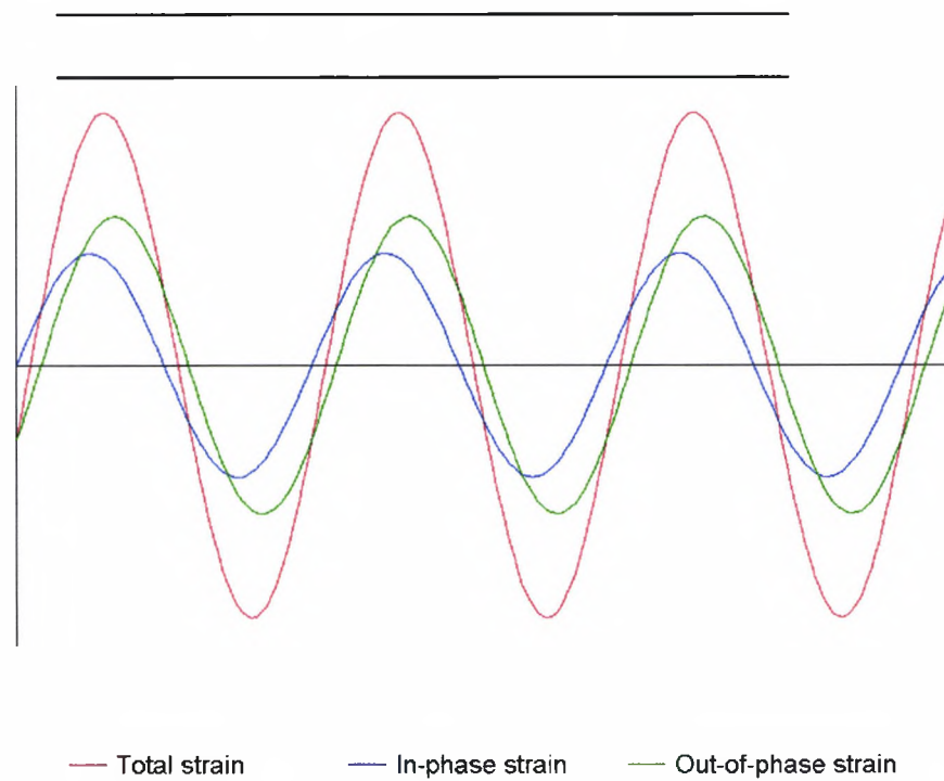
Figure 8.3.1. An applied sinusoidal stress results in a corresponding strain.
