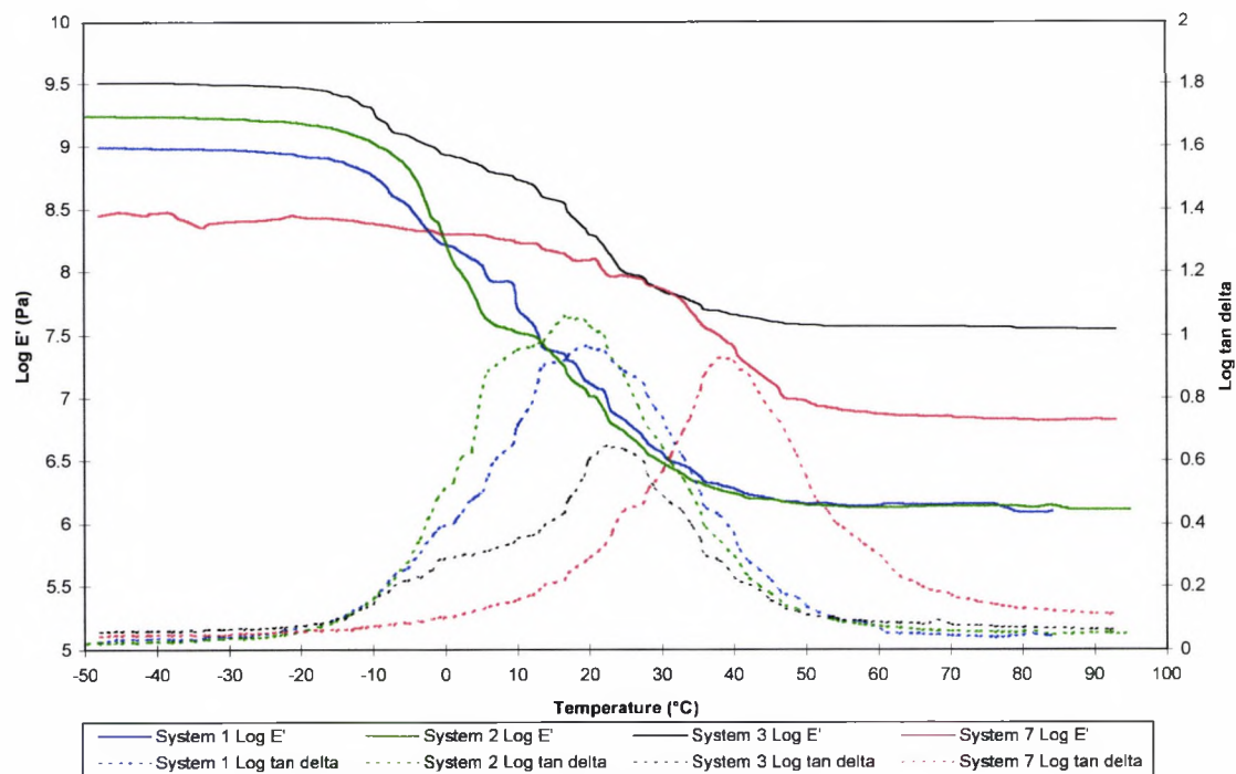
Figure 9.2.1. DMTA plots of the unexposed coatings based on alkyd resins.
