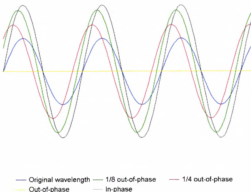
Figure 8.4.1.3. Effect of position of the moving mirror on one wavelength.
