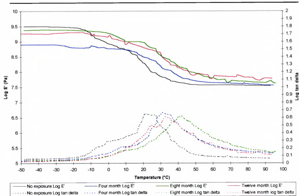
Figure 9.3.1.4.a. The effect of up to twelve months natural weathering on System 3
