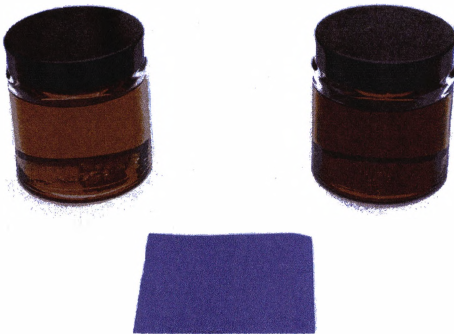
Figure 4.1. A long oil alkyd without driers on the left, and with 0.05% w/w cobalt on the right. Even a small deepening in colour can have a significant effect, especially for white and pale coloured paints. The purple square is the colour of a piece of white paper moistened with cobalt drier solution, and allowed to dry. It was placed on identical paper, which forms the background to the photograph.
