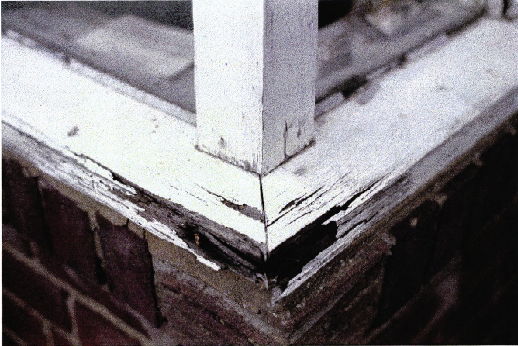
Figure 3.4.2.1. By poor design and by poor maintenance, water has entered the wood through the transverse face exposed by the butt joint, and has been retained by the coating, causing rot to set in.
