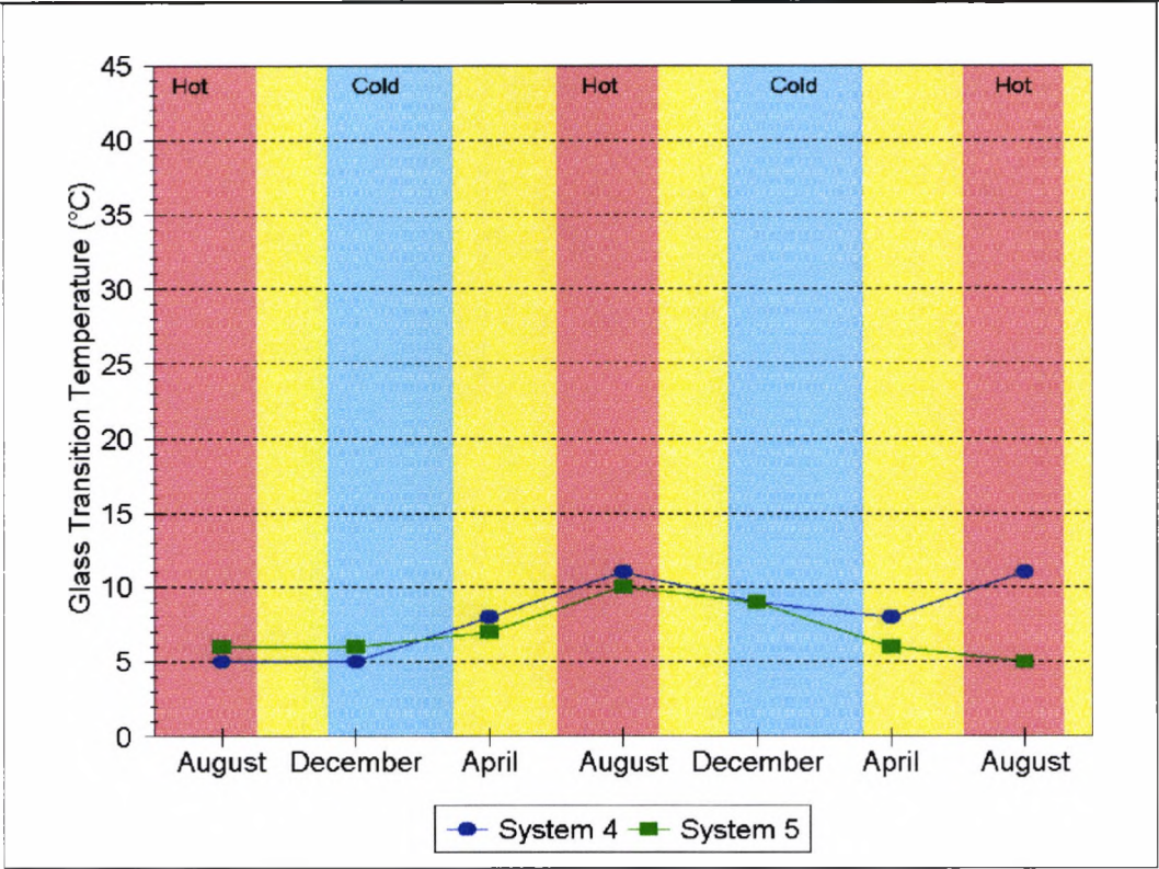
Figure 9.3.2.1. Variation of T_g of acrylics with month of measurement.
