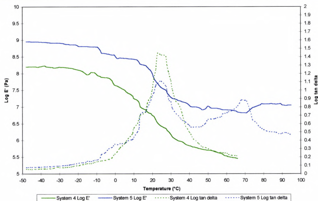
Figure 9.2.2.1. DMTA plots of the unexposed coatings based on acrylic resins.
