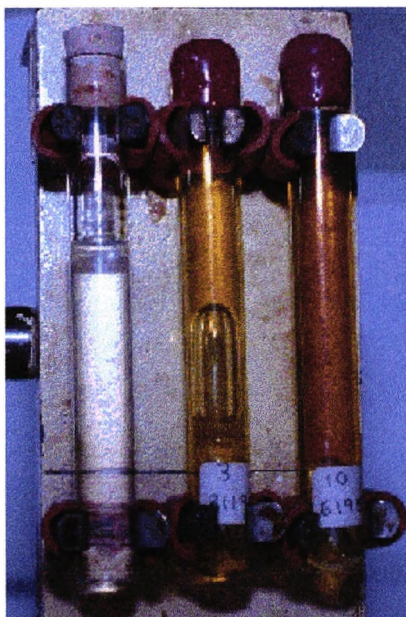
Figure 4.2. Comparison of viscosity using PRA standard bubble viscometers. Water is in the tube on the left, a one poise oil in the middle, and a five poise oil on the right. The bubble has reached the top of the water, which is clearly much thinner than the one poise oil, where the bubble is about half-way up the tube. The bubble for the five poise oil has yet to start to rise, and is just visible behind the tube label.
