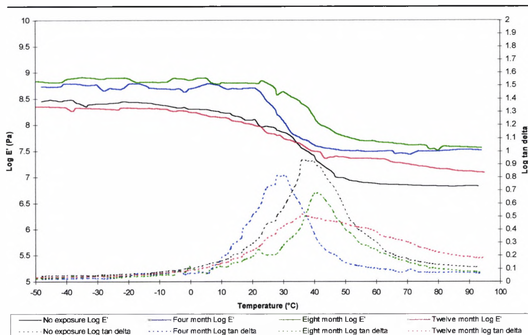
Figure 9.3.1.5.a. The effect of up to twelve months natural weathering on System 7
