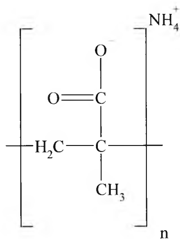
Ammonium methacrylate
