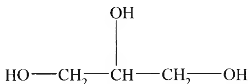
glycerol
