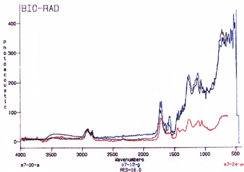
Figure 9.4.2.4. The effect of natural exposure on the infra-red spectra of System 7. The black, blue and red spectra are of the coating unexposed, and after 12, and 24 months respectively. Peaks due to the organic portion have been suppressed by the relatively high pigment content.
