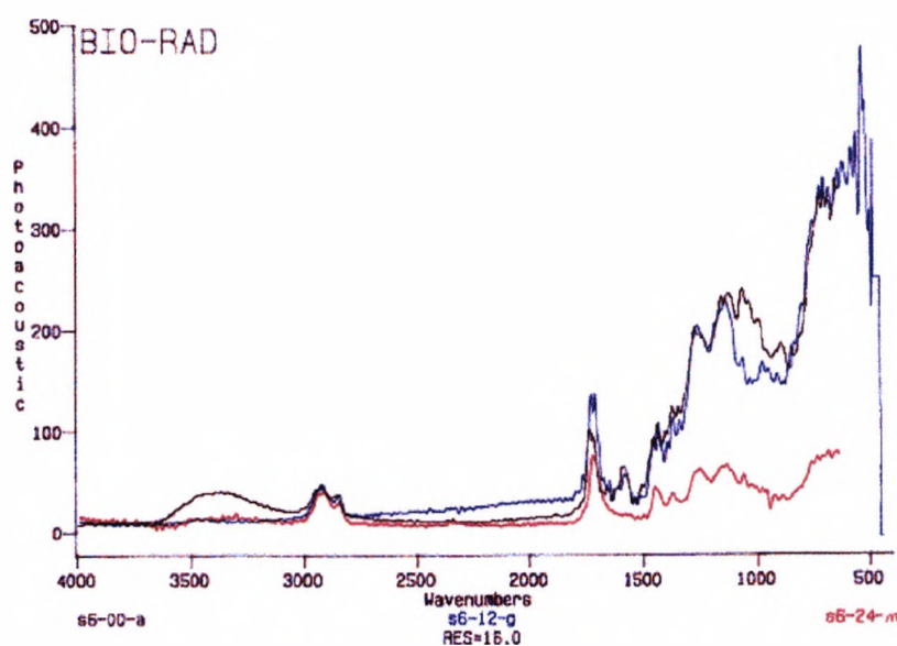
Figure 9.4.4. The effect of natural exposure on the infra-red spectra of System 6. The black, blue and red spectra are of the coating unexposed, and after 12, and 24 months respectively.
