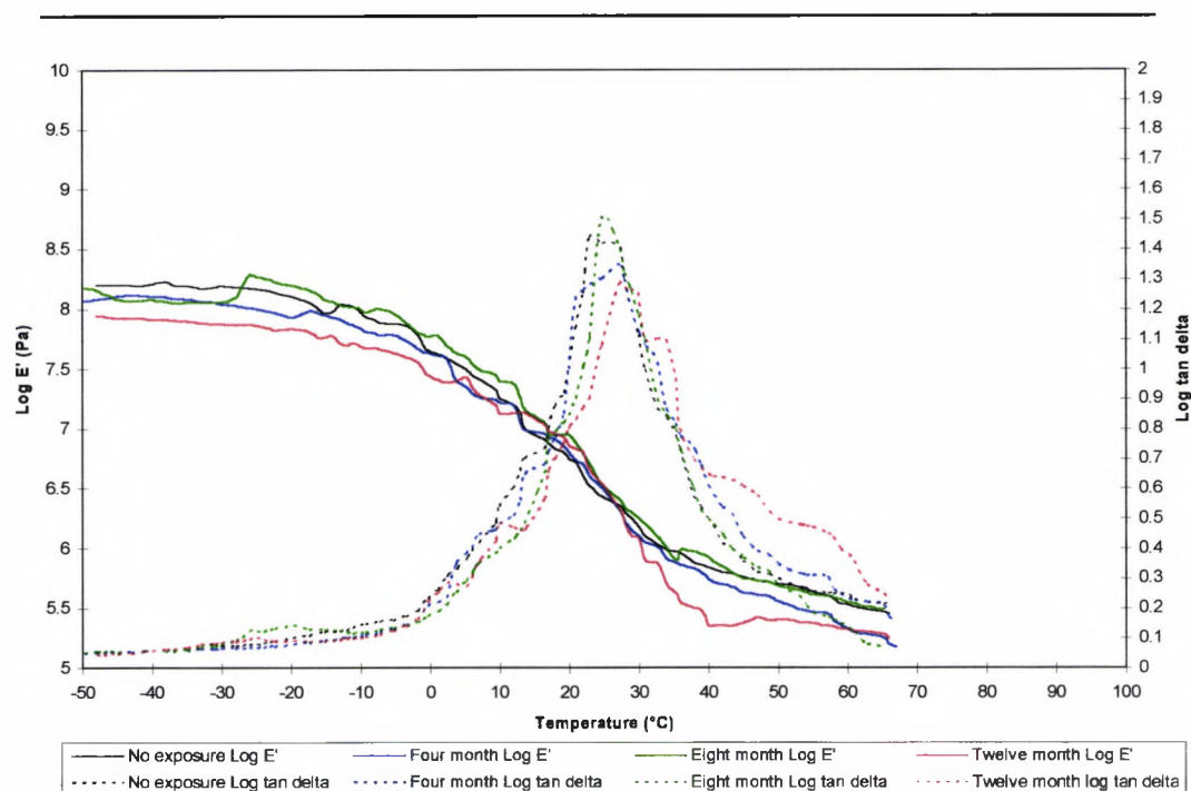
Figure 9.3.2.2.a. The effect of up to twelve months natural weathering on System 4
