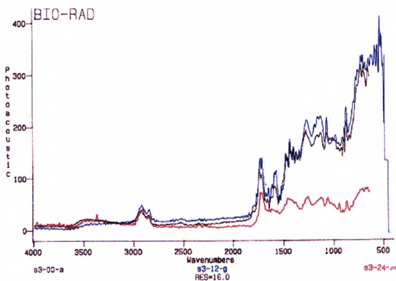
Figure 9.4.2.3. The effect of natural exposure on the infra-red spectra of System 3. The black, blue and red spectra are of the coating unexposed, and after 12, and 24 months respectively. Peaks due to the organic portion have been suppressed by the relatively high pigment content.
