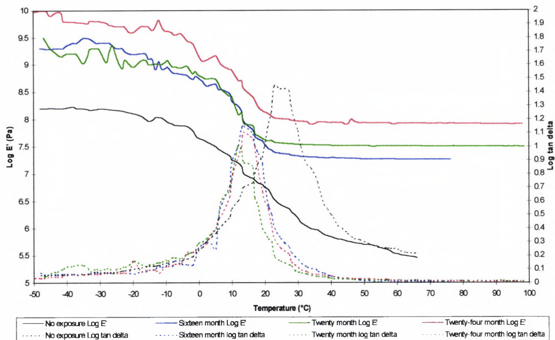
Figure 9.3.2.2.b. The effect of up to twenty-four months natural weathering on System 4
