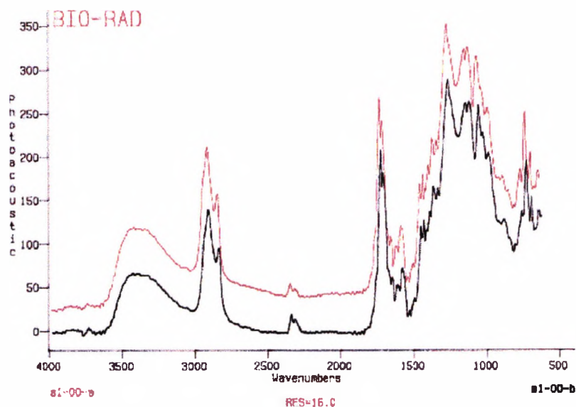
Figure 9.4.1.1. Unexposed System 1. The two spectra are taken from different samples, within a few minutes of each other.
