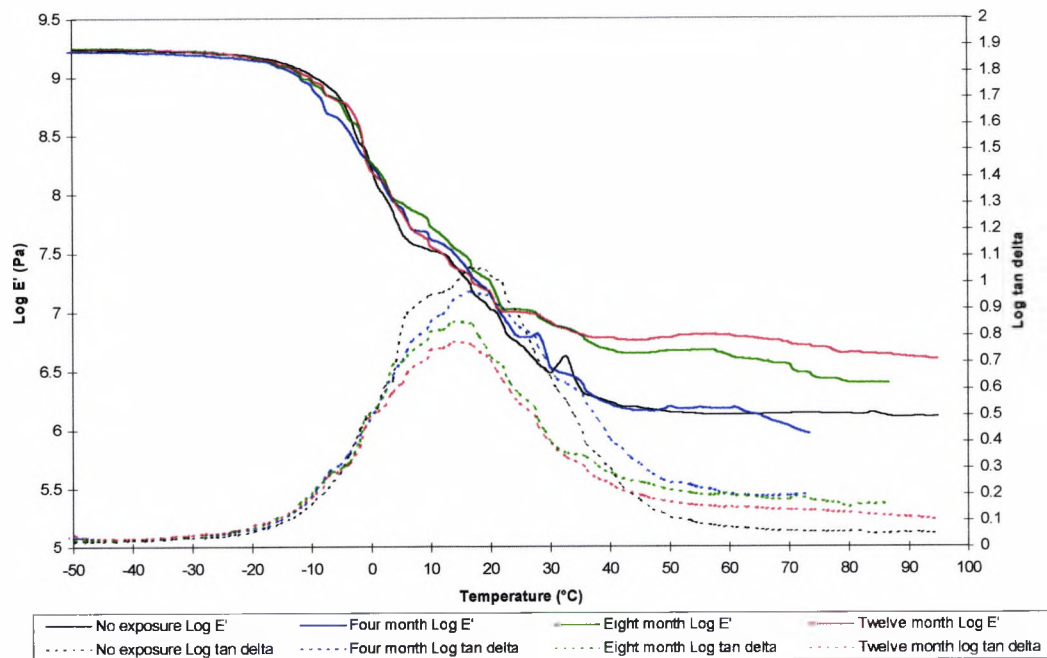
Figure 9.3.1.3.a. The effect of up to twelve months natural weathering on System 2
