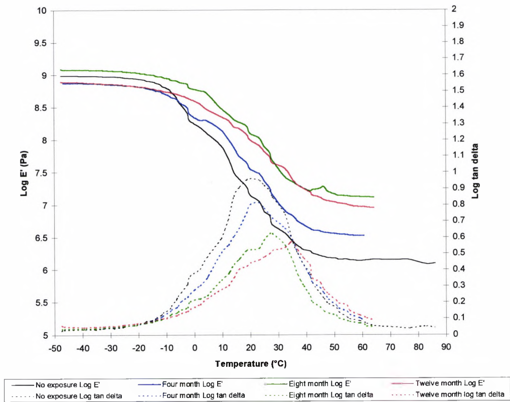
Figure 9.3.1.2.a. The effect of up to twelve months natural weathering on System 1
