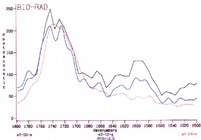
Figure 9.4.2.2.b. An expanded view of the mid range infra-red spectra of System 2. The black, blue and red spectra are of the coating unexposed, and after 12, and 24 months respectively.
