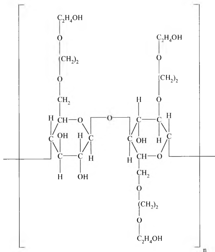
idealised Fischer diagram of hydroxyethyl cellulose
