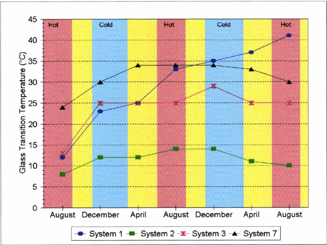
Figure 9.3.1.1. Variation of T_g of alkyds with month of measurement.
