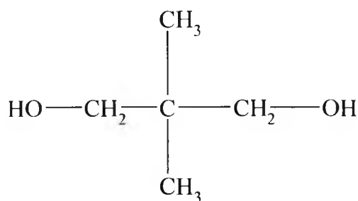
neopentyl glycol
