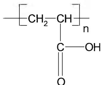
Polyacrylic acid
