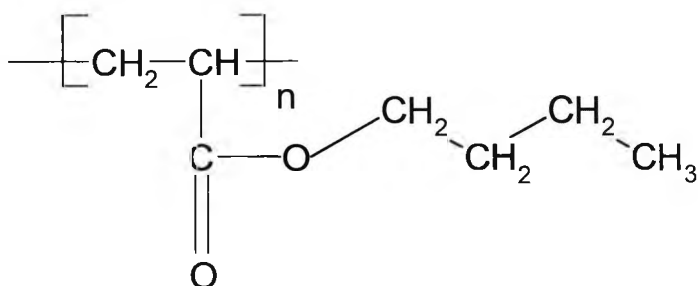
Poly-n-butyl acrylate
