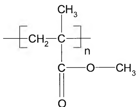
Poly-methyl methacrylate
