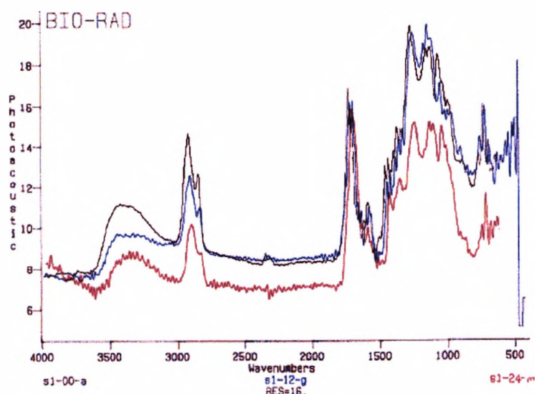
Figure 9.4.2.1. The effect of natural exposure on the infra-red spectra of System 1. The black, blue and red spectra are of the coating unexposed, and after 12, and 24 months respectively.
