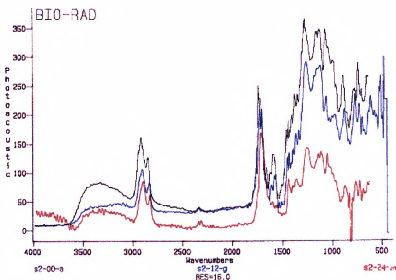
Figure 9.4.2.2.a. The effect of natural exposure on the infra-red spectra of System 2. The black, blue and red spectra are of the coating unexposed, and after 12, and 24 months respectively.
