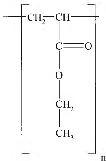
Ethyl acrylate
