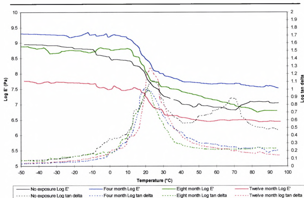
Figure 9.3.2.3.a. The effect of up to twelve months natural weathering on System 5
