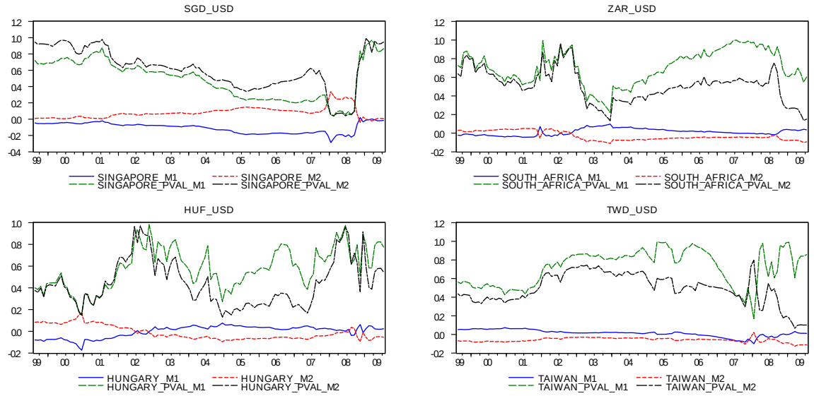
Figure 1.2. Emerging Markets panel: Coefficients and p-values for the MA model at the 1-month horizon.
