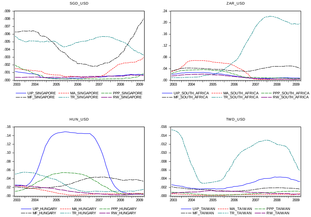
Figure 1.6. Rolling Regression Results for the Emerging Markets panel: RMSPEs at the 1-year horizon.
