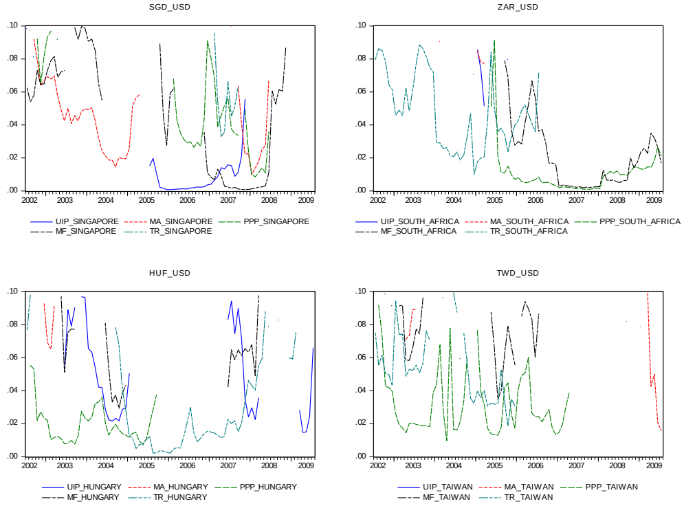
Figure 1.11. Emerging Markets panel: P-values for the Combined model at the 1-month horizon.
