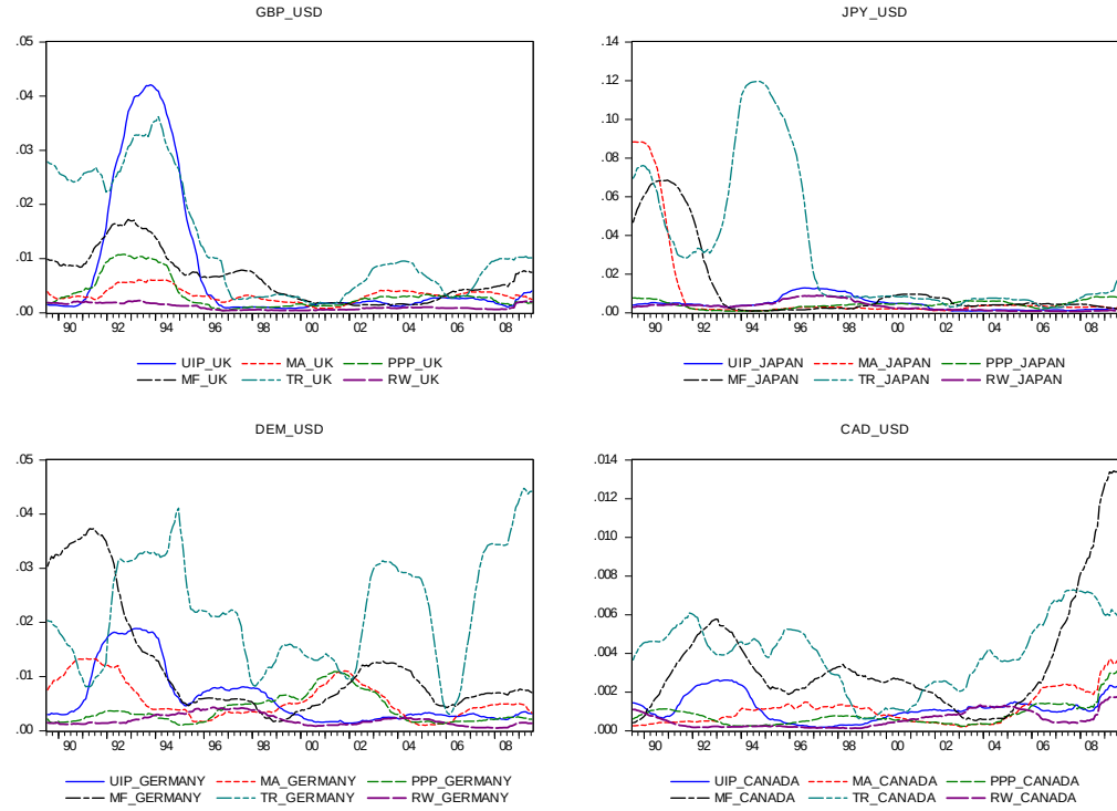
Figure 1.5. Rolling Regression Results for the Developed Markets panel: RMSPEs at the 1-year horizon.
