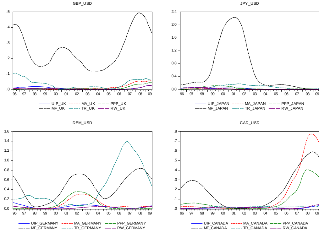
Figure 1.7. Rolling Regression Results for the Developed Markets panel: RMSPEs at the 5-year horizon.
