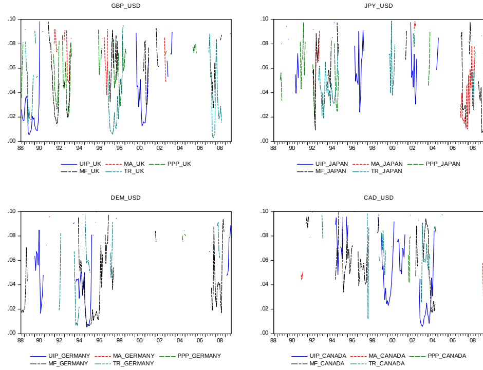
Figure 1.10. Developed Markets panel: P-values for the Combined model at the 1-month horizon.
