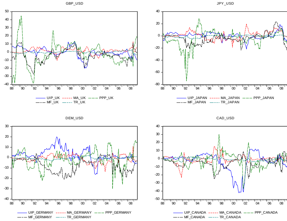
Figure 1.9. Developed Markets panel: Coefficients for the Combined model at the 1-month horizon.
