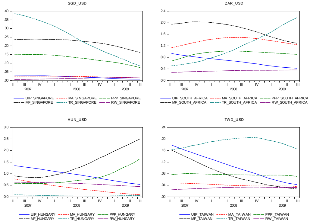
Figure 1.8. Rolling Regression Results for the Emerging Markets panel: RMSPEs at the 5-year horizon.
