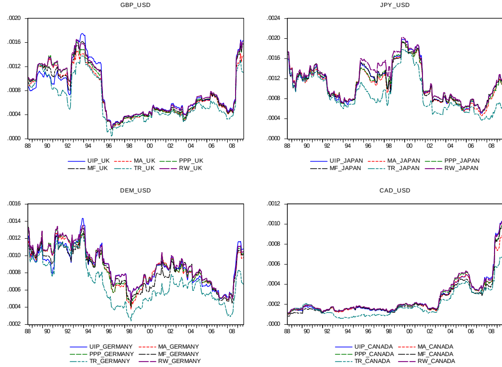
Figure 1.3. Rolling Regression Results for the Developed Markets panel: RMSPEs at the 1-month horizon.
