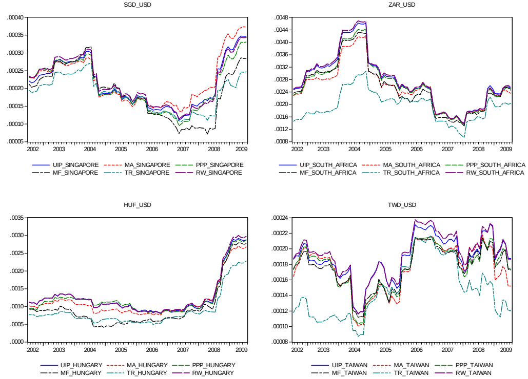
Figure 1.4. Rolling Regression Results for the Emerging Markets panel: RMSPEs at the 1-month horizon.
