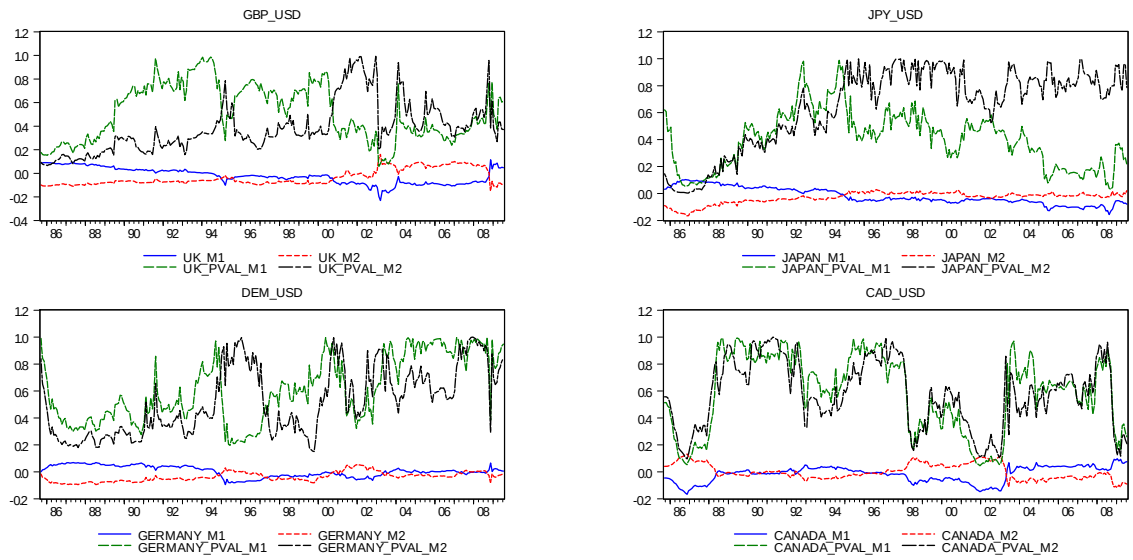
Figure 1.1. Developed Markets panel: Coefficients and p-values for the MA model at the 1-month horizon.
