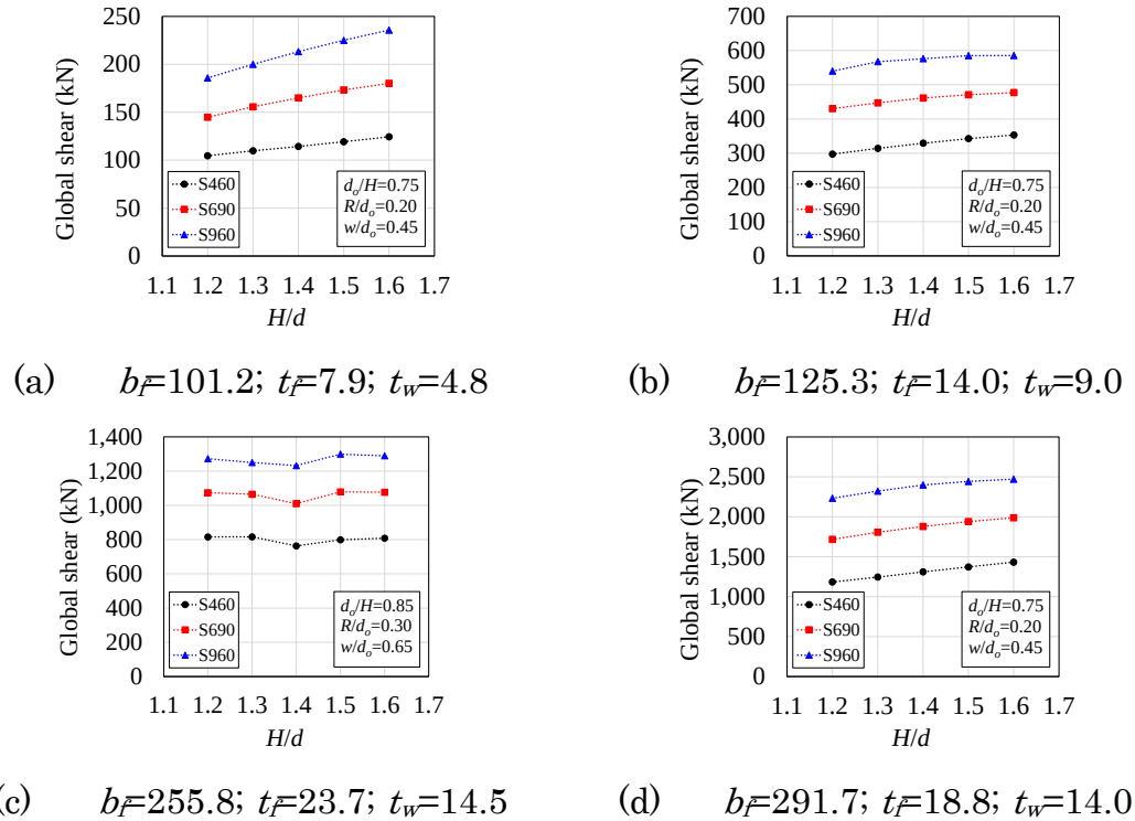
Fig. 13: Influence of H/d ratio on capacity (dimensions in mm)
