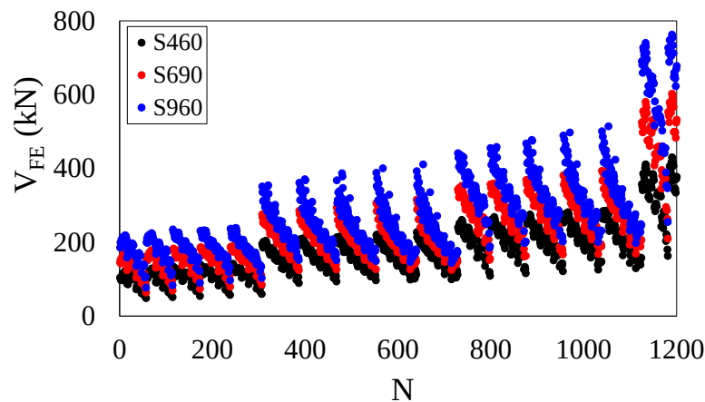
Fig. 12: Capacity of the web-post made of high-strength steels
