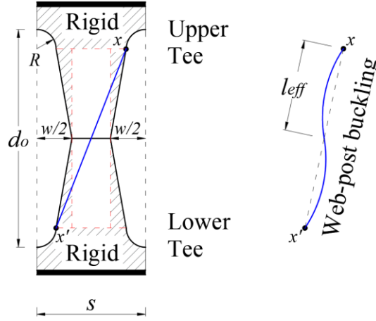
Fig. 2: Compressed truss model [16]
