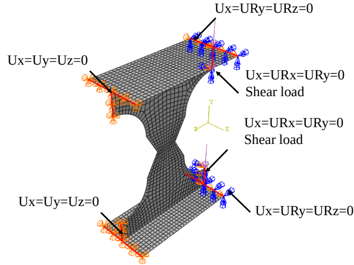
Fig. 5: Boundary conditions
