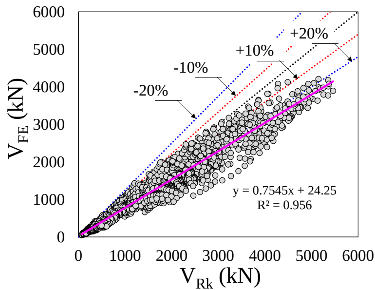
Fig. 17: FEM vs. Design equation for common strength steels
