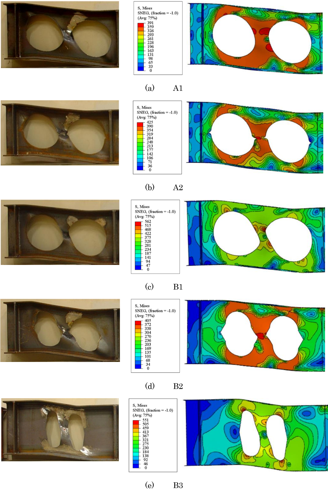
118 Fig. 3: Comparison between tests and finite element models by load- 119 displacement relationships
