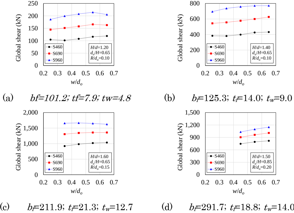
Fig. 16: Influence of w/d_o ratio on capacity (dimensions in mm)
