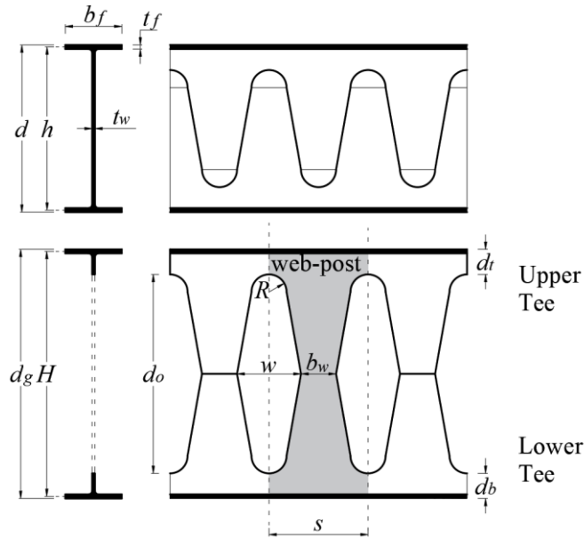
Fig. 1: Steel beams with elliptically-based web openings [18]
