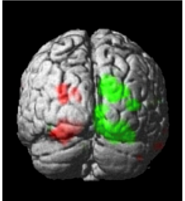
Event-related
