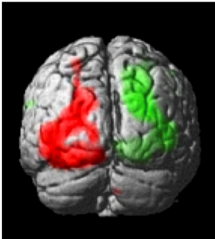
Block-related
