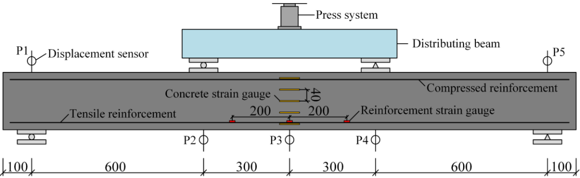
Fig. 4. Test setup of beam specimens.
