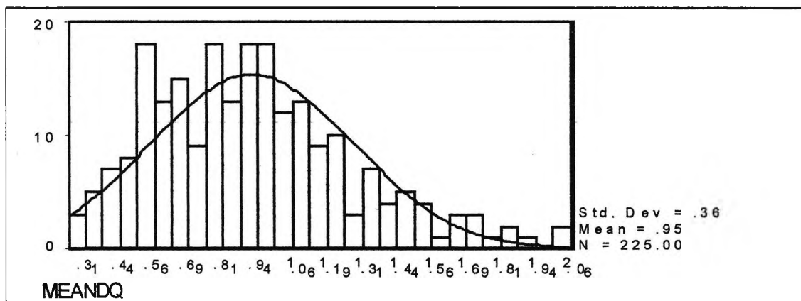
Figure 1: Distribution of total scores, expressed as mean item scores (potential range 0 - 4.0) in controls for the D90, with superimposed normal distribution curve
