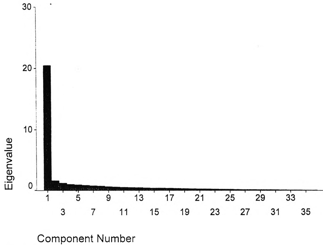
Scree Plot of D36 catalogue
