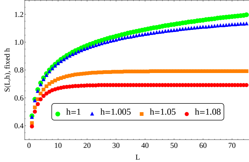
Figure 5.5: Behavior of the entanglement entropy for fixed h as a function of the block length.
