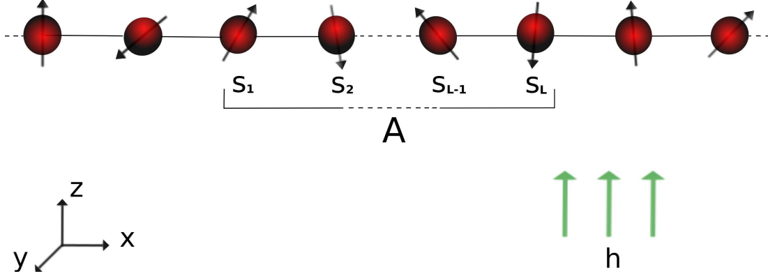
Figure 5.3: Representation of the bipartition in the two regions A , and its complement. The external magnetic field is aligned along the z -axis, while the black links between spins represent the bond interaction.
