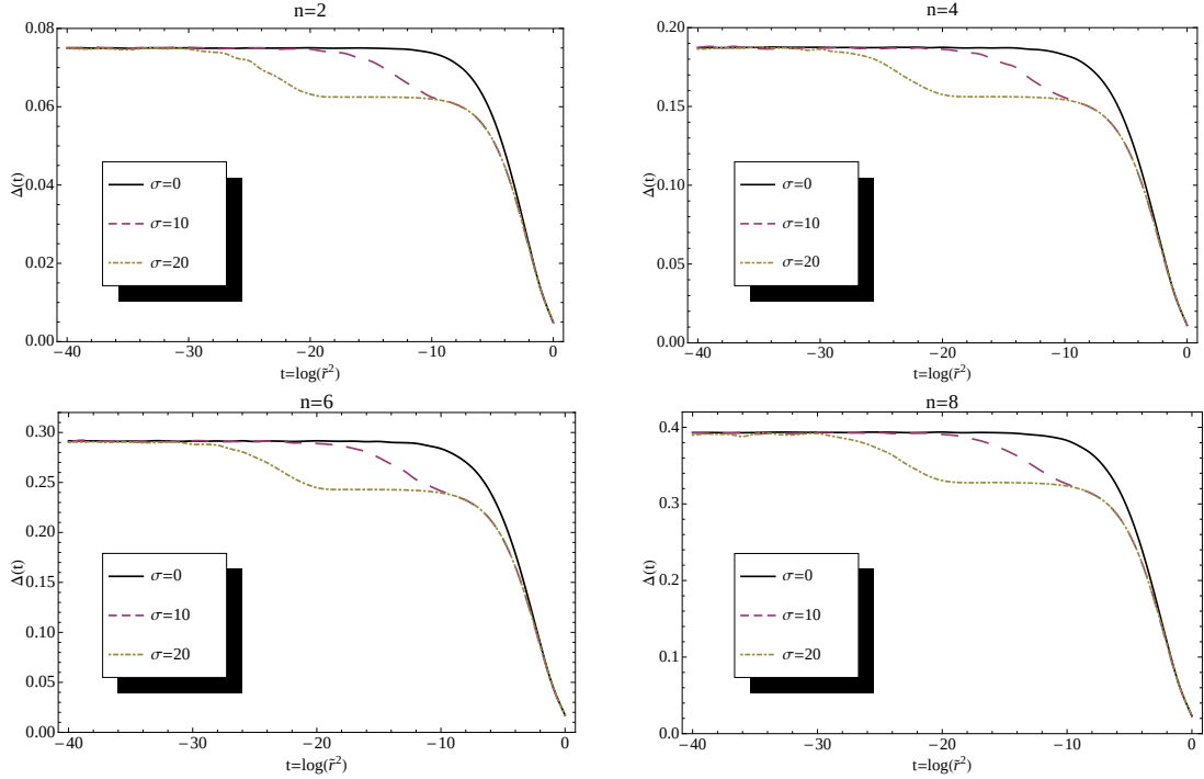
Figure 3.1: The function \Delta(t) := \Delta_{\mathcal{T}}(t) with t = 2\log(\tilde{r}) and \tilde{r} = mr . In these figures we show the behaviour of \Delta_{\mathcal{T}}(t) along the renormalization group flow, from the infrared to the ultraviolet fixed point, for different values of the resonance parameter \sigma . Our results are consistent with (2.67) and c = 1 for the first plateau and (2.67) with c = 6/5 for the second plateau.
