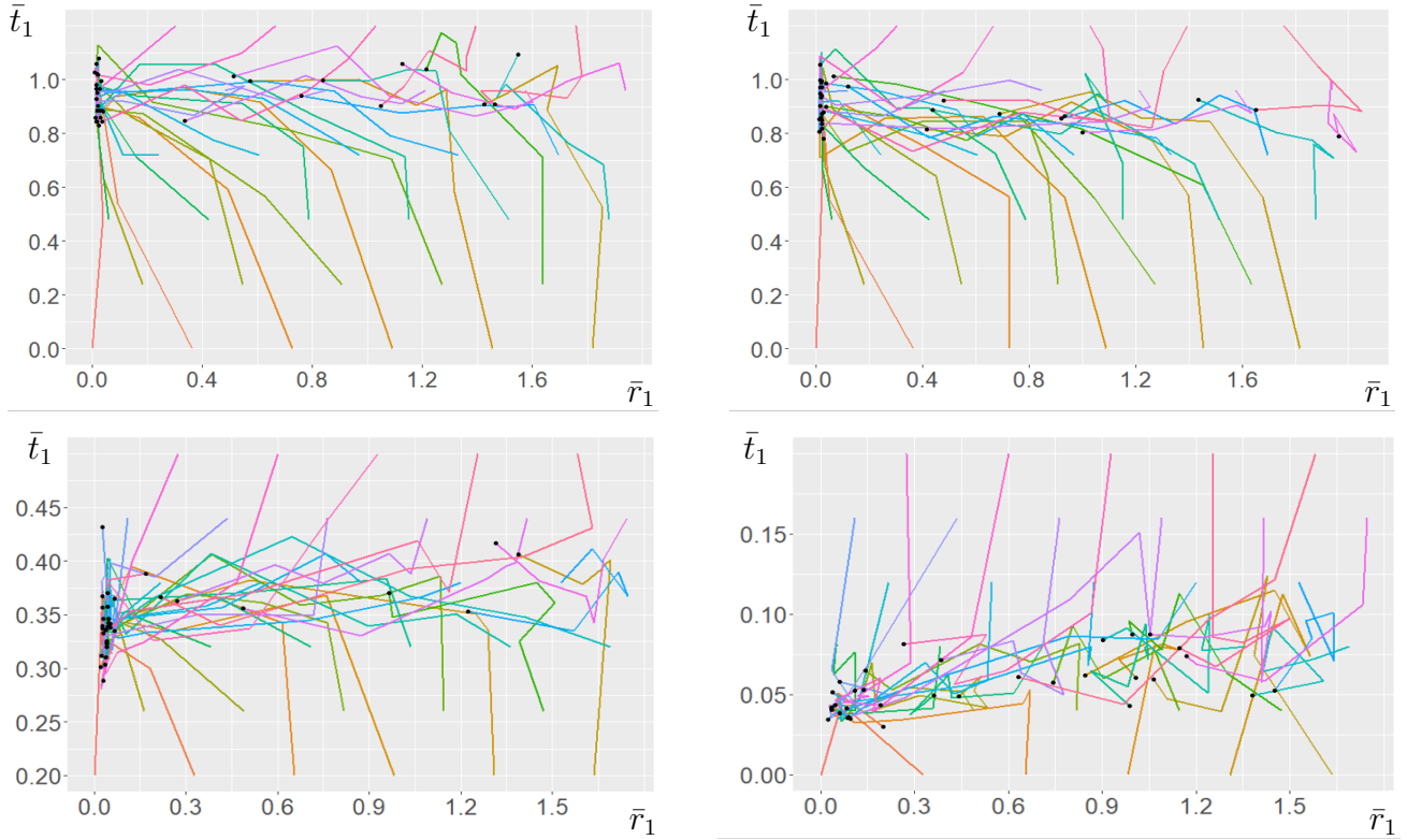
Figure 4.6: Parameters a = 0, f = 5/6, k = 5, t_c = 0.25, q = 0.4, N = 100, n = 10, v = 1 with plots in increasing order of the parameter \lambda with (a) [Top left] \lambda = 0.0001 ; (b) [Top right] \lambda = 0.0015 ; (c) [Bottom left] \lambda = 0.2 and (d) [Bottom right] \lambda = 2 . Together the plots (mostly) confirm that increasing \lambda causes a decrease in the associated level of toxicity (for fixed conspicuousness) and that the relationship between t_1^* and r_1^* switches from decreasing (in 4.6a and 4.6b) to increasing (in 4.6c and 4.6d) as the predicted level of defence t_1^* drops below c(r_1^*) as \lambda increases. The accumulation of black markers suggests strong selection for crypsis, likely driven by directional preference of mutant fitness in that direction. We also remark that trajectories in (a) convey a mostly flat equilibrium at t \approx 1/f - 1/k and that in (d) trajectories are traced out within the non-aversive - and unstable in the sense of (4.1.15) - region \bar{t}_1 \leq t_c = 0.25 .
