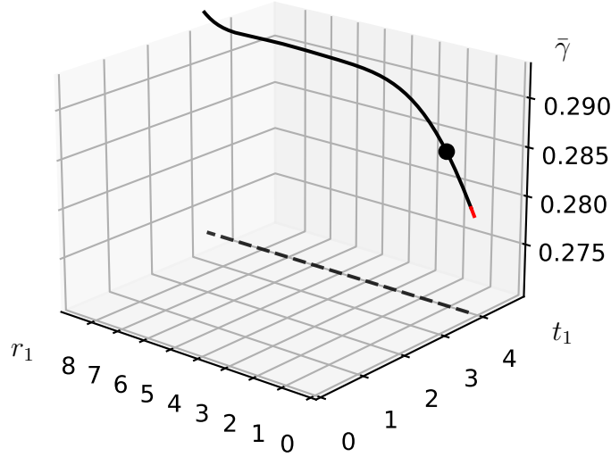
Figure 6.3: Solid black curve shows the continuum of eco-evolutionarily stable solutions that are defined in the vicinity of the initial example (r_1, t_1, \bar{\gamma}) = (1, 3.8522..., 2/7) , which is shown as a solid black marker. The red section of the curve shows that the continuum is unstable (mimic invaded by the less conspicuous type) for smaller values of the conspicuousness and becomes stable for increasing values (black section of the curve). The figure is to be viewed in tandem with Table 6.1 in which the exact values at each coordinate of the curve provide an indication of how stable each is and with respect to which potential invader.
