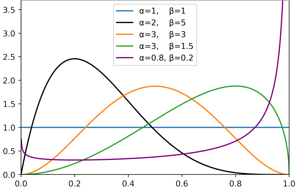
Figure 6.1: Plots of beta probability density functions with shape parameters as specified in the legend. By construction in our context the x -axis represents the proportion of mimics \gamma over the population. The black curve with parameters \alpha = 2, \beta = 5 is used in section 6.6 to generate a working example of a Batesian mimicry complex that is eco-evolutionarily stable.
