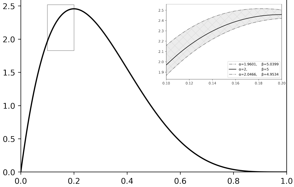
Figure 6.2: Solid black curve shows plot of probability density for the proportion of mimics ( \gamma ) in the population of prey, which is beta distributed with mean \bar{\gamma} = 2/7 and \delta = 7 . The interior of the grey rectangle is shown in greater detail in the close-up figure on the top right, in which the shaded region represents a perturbation of the density function about the mean value \bar{\gamma} = 2/7 within the interval (1.965/7, 2.045/7) keeping \delta = 7 fixed.
