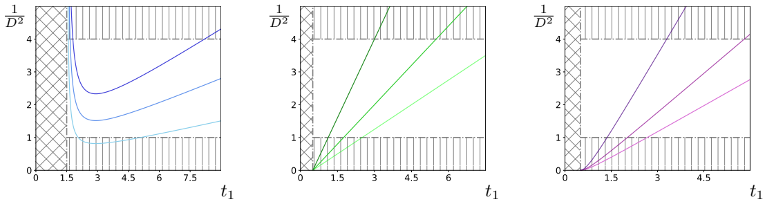
Figure 3.3: Plots show variation in \alpha of the RHS of (3.2.9) for the regimes b < 1 (blue), b = 1 (green) and b > 1 (magenta), such that in each plot the darker shades correspond to higher values of \alpha . Only sections of curves contained inside the unshaded region correspond to real ESSs and there are two grey-shaded regions that are empty of solutions: (i) the diagonally-checked vertical strips, on which the RHS of (3.2.10) is negative; (ii) the vertically-striped horizontal sections, on which the LHS of (3.2.10), i.e. 1/D^2(r_1) assumes values outside of the admissible range (1, 4] . (a) Values f = 0.5 , k = 2 , t_c = 0.5 and \alpha = 0.035, 0.065, 0.1 have been used; curves with \alpha < 0.042 have minima inside the bottom grey region, curves with 0.042 \leq \alpha \leq 0.171 have minima inside the unshaded region and curves with \alpha > 0.171 are entirely contained in the top grey-shaded region - see also (3.3.4) and (3.3.5). (b) Values b = 1 , f = 1 , k = 2 , t_c = 0.5 and \alpha = 0.25, 0.4, 0.8 are used and curves with \alpha > 4 (not shown) would be entirely outside the unshaded region. (c) Values b = 1.5 , f = 1.5 , k = 2 , t_c = 0.5 and \alpha = 0.4, 0.6, 1.2 have been used and all values of \alpha yield solutions.
