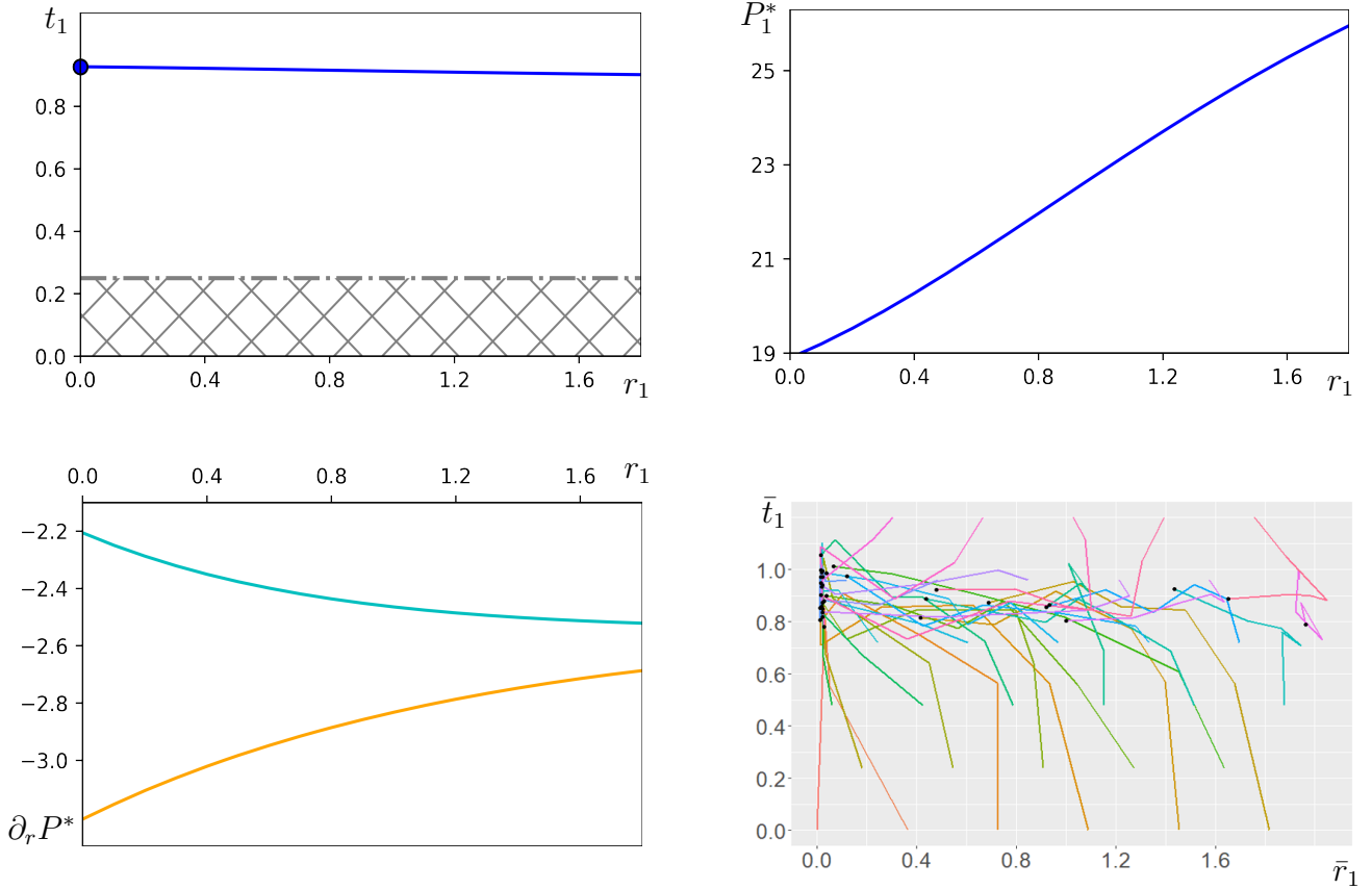
Figure 4.5: Parameter values \lambda = 0.0015, a = 0, f = 5/6, k = 5, t_c = 0.25, q = 0.4, N = 100, n = 10, v = 1 (a) [Top left] Unique cryptic ESS represented as a solid marker at (0, 0.927) co-exists alongside a continuum of conspicuous ESSs shown in blue and defined implicitly through setting a = 0 into (4.1.2). Strategies (r_1^*, t_1^*) on the curve (4.1.2) are such that t_1^* > c(r_1^*) so that the level t_1^* is predicted to decrease (slowly) with respect to r_1^* . (b) [Top right] Absolute resident fitness defined implicitly through (4.1.27) and plotted as a function of the conspicuousness. (c) [Bottom left] Invasion fitness gradient associated with less (cyan) and more conspicuous (orange) mutant types at equilibrium given through (4.1.15) and (4.1.16). (d) [Bottom right] Average population traits plotted as trajectories with averaging frequency g = 2,000 . Black markers show strong converge to crypsis, which is mostly supported from Figures 4.5(b) and 4.5(c).
