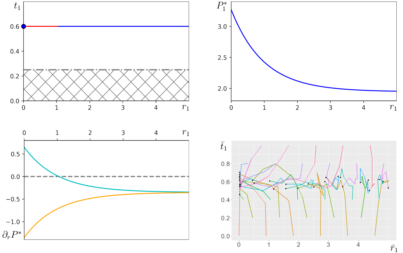
Figure 4.2: Parameter values \lambda = 0, a = 0, f_0 = q_0 = k_0 = 1, f = 1, k = 2.5, t_c = 0.25, q = 0.1, N = 100, n = 10 and v = 1 (a) [Top left] Strategies within the grey-shaded region \{(r_1, t_1) : r_1 > 0, t_1 \leq 0.25\} fail (4.1.15). Unique cryptic ESS at (r_1^*, t_1^*) = (0, 0.6) shown with blue marker, succeeded by strategies on (4.1.7) that fail (4.1.15) for r_1^* < 1.05 but are stable beyond that value (blue section). (b) [Top right] Resident fitness evaluated along (4.1.7) as per (4.1.22). (c) [Bottom left] Invasion fitness gradient along r - see (4.1.19) as well as (4.1.15) and (4.1.16) - for incrementally less (cyan curve) and incrementally more conspicuous mutants (orange curve). (d) [Bottom right] Average population traits plotted as trajectories with averaging frequency g = 2,000 . Black markers represent the average traits of a single population after 10,000 iterations.
