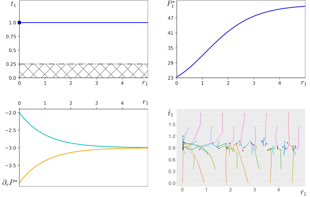
Figure 4.3: Parameter values \lambda = 0, a = 0, f_0 = q_0 = k_0 = 1, f = 5/6, k = 5, t_c = 0.25, q = 0.4, N = 100, n = 10 and v = 1 (a) [Top left] Grey-scale region \{(r_1, t_1) : r_1 > 0, t_1 \leq 0.25\} contains strategies that fail (4.1.15). Solid blue marker at (0, 1) is the unique cryptic ESS followed by a horizontal blue line of conspicuous ESSs evaluated at (4.1.7). (b) [Top right] Plot of resident fitness along (4.1.7) as per (4.1.22). (c) [Bottom left]: Invasion fitness gradient along r evaluated at equilibrium for incrementally less (cyan) and incrementally more (orange) conspicuous mutants as in (4.1.15) and (4.1.16) (d) [Bottom right]: Average population traits plotted as trajectories with averaging frequency g = 2,000 . Black marks represent the average traits of a population after 10,000 iterations.
