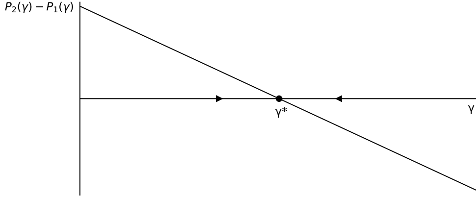
Figure 5.1: The figure illustrates condition (5.1.15). It is clear that values of \gamma < \gamma^* result in the first type having smaller payoff than the second type playing (r_2, t_2) , which leads to the fractional increase in the size of the latter ( \gamma ) until it reaches the critical value \gamma^* , at which both types grow at the same rate. If, on the other hand \gamma > \gamma^* , the converse is true so that \gamma decreases until it re-settles at \gamma^* , indicating that \gamma^* is a parameter value associated with stable co-existence.
