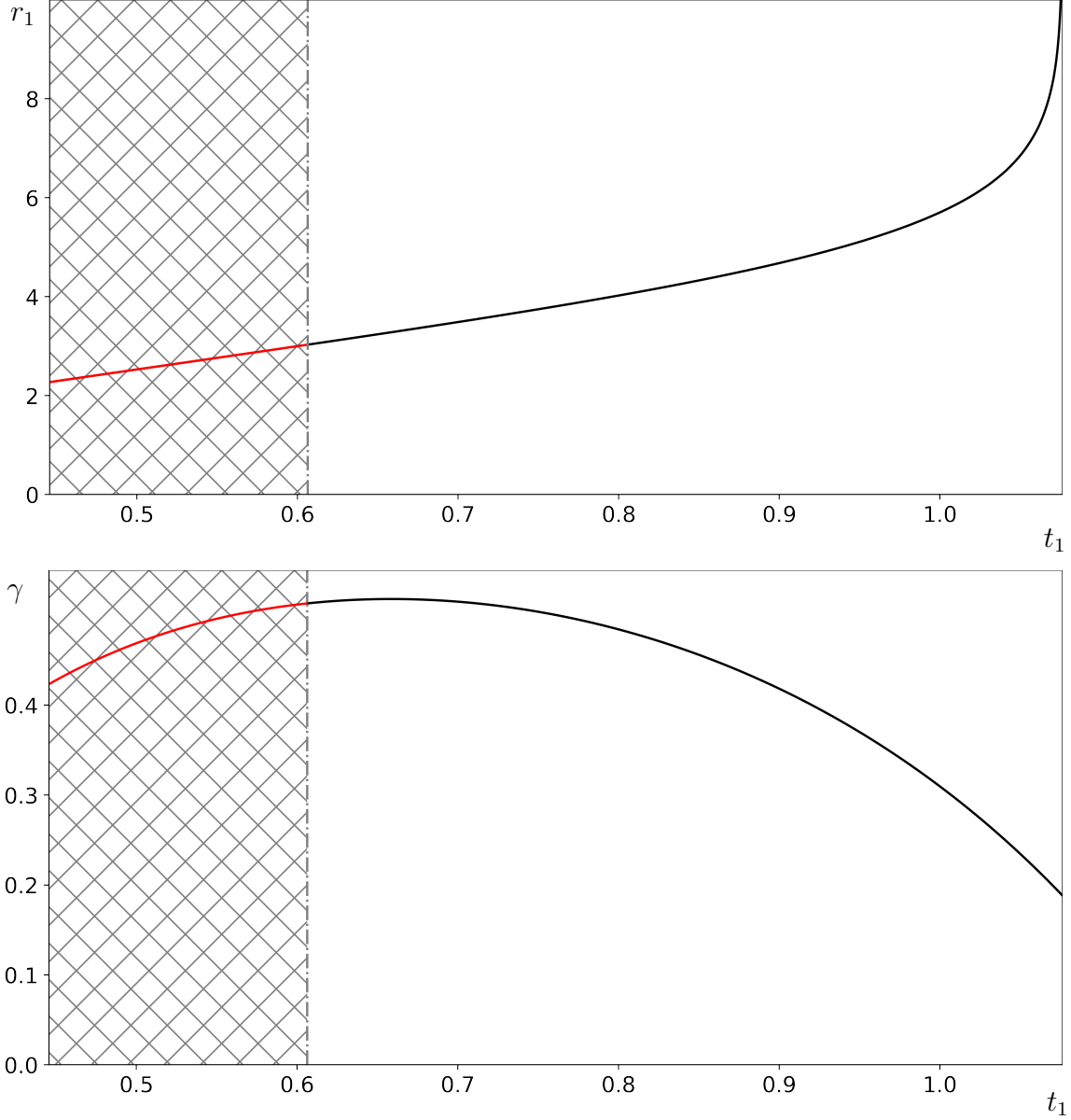
Figure 5.2: The shaded regions span the interval 0.4456 < t_1 < 0.612 in condition (5.4.35) for the mimic fails - the curves mentioned in (a) and (b) are drawn in red over these regions. The region t_1 < 0.4456 is not shown because on this I'_2 < I_\varepsilon , which is also a violation. (a) [Top] Solid curve shows conspicuousness versus model defence as provided implicitly through (5.4.29); the red section is unstable in the sense of failing (5.4.35) while the black section beyond t_1 \approx 0.612 admits a continuum that is eco-evolutionarily stable when viewed in tandem with the continuum in (b). (b) [Bottom] Solid curve shows the mimetic load vs. model defence as provided explicitly through (5.4.31); as mentioned earlier only the black section on t_1 > 0.612 admits an equilibrium that is eco-evolutionarily stable. Plots (a) and (b) can be viewed in tandem and thus perceived as a single curve (t_1, r(t_1), \gamma(t_1)) defined through (5.4.29) and (5.4.31) within the subregion (0.612, 1.0765) \times (3.0577, +\infty) \times (0, 188, 0.5179] of the extended strategy space.
