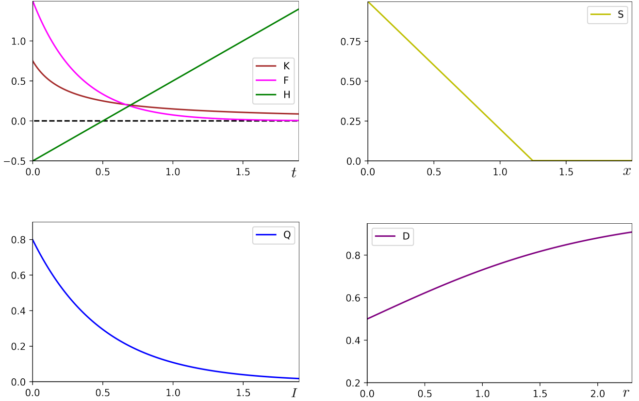
Figure 4.1: The example functions of (4.1.1) as used in the genetic algorithm model with specific parameter values chosen for purposes of demonstration only. (a) [Top Left] The functional forms for the probability of escaping a mounted attack ( K ), the fecundity ( F ) and the aversiveness of an experience ( H ) plotted as functions of prey toxicity. Parameter values given as k_0 = 0.75 and k = 4 ; f_0 = 1.5 and f = 3 and t_c = 0.5 respectively. (b) [Top Right] The functional form for the (uni-variate) similarity function S plotted with respect to the generic variable x and parameter v = 0.8 . (c) [Bottom Left] The form for the probability of attack Q with q_0 = 0.8 and q = 2 plotted as a function of the perceived aversiveness; (d) [Bottom Right] The form for the rate of detection plotted as a function of prey conspicuousness D with d_0 = 0.5 .
