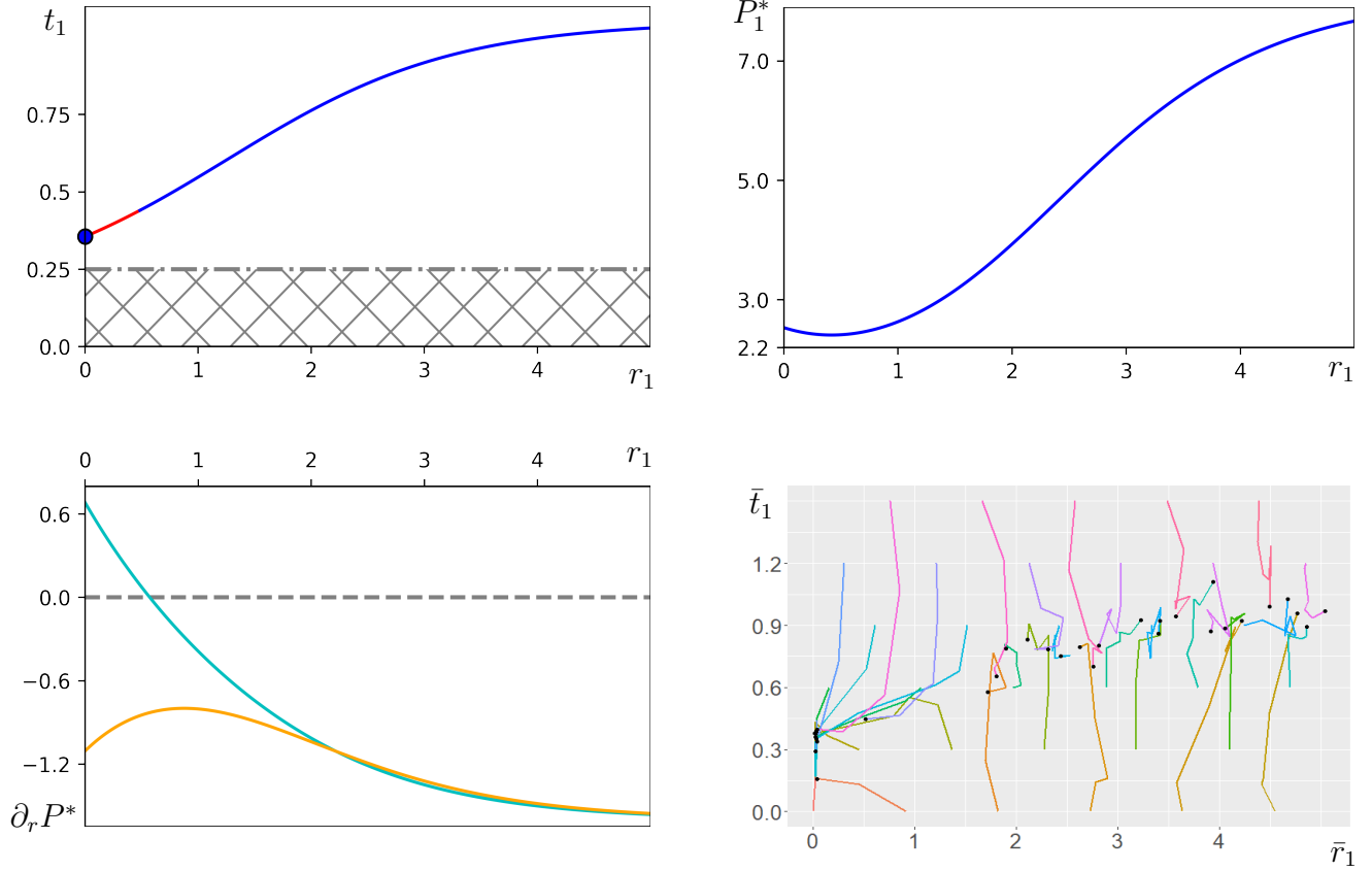
Figure 4.4: Parameter values \lambda = 0, a = 0.5, f_0 = k_0 = q_0 = 1, f = 2.8, k = 5, t_c = 0.25, q = 0.4, N = 100, n = 10, v = 1 (a) [Top left] Strategies inside grey-scaled region \{r_1 > 0, t_1 \leq 0.25\} violate (4.1.15). Blue marker at (0, 0.356) represents the unique cryptic solution, which co-exists alongside a continuum of conspicuous unstable (red) and stable ESSs (blue) on the curve of (4.1.8). (b) [Top right] Resident fitness as a function of conspicuousness along (4.1.8) conspicuousness. (c) [Bottom left] Cyan and orange curves represent the invasion fitness gradient given through (4.1.15) and (4.1.16) and evaluated along (4.1.8) (d) [Bottom right] Average population traits plotted as trajectories with averaging frequency g = 2,000 . Black markers represent traits averaged over the population after 10,000 iterations and mostly converge to t_1^*(r_1^*) in (4.1.8) in Figure 4.4(a).
