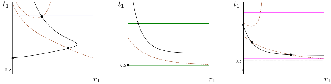
Figure 3.5: All three figures contain plots of local ESSs in strategy space as subsections of the t -equilibrium curve (3.3.2) shown as black solid lines and partitioned by black markers (filled X marks indicate cryptic solutions). The dashed-dotted lines mark the natural cut-off at t_c = 0.5 , while the brown dashed lines represent the zero level sets of the LHS of (3.3.6) and (3.3.7). In (a) we have set b = 0.5, a = 0.4, f = 0.5, k = 2, \alpha = 0.0445 and v = 0.04 . The solid curve has an r_{max} -type vertex at t_1 = T_{SIGN}^+ = 1.5 + \sqrt{2} and unique cryptic ESS at the aversive level t_1 \approx 1.601 . In (b) we have set b = 1, a = 0.3, f = 1, k = 2, \alpha = 0.3 and v = 0.4 . The section of the t -equilibrium curve that lies under the upper green solid line and above the brown dashed line consists of a continuum on which the ESS level of defence decreases with increasing level of the conspicuousness; t_1 = 1/2 is the unique cryptic ESS, although this may be non-generic. In (c) we have set b = 1.5, a = 0.2, f = 1.5, k = 2, \alpha = 1.6 and v = 0.05 . The section of the solid black curve in between the lower and upper brown dotted lines consists of a decreasing continuum of local ESSs, the section under the lower brown curve does not contain ESSs, while the last section that is once more in between the middle and top brown lines consists of a second decreasing continuum of ESSs. The intersection of the equilibrium curve with r_1 = 0 is an aversive cryptic ESS, while t_1 = 1/6 admits a non-aversive cryptic solution.
