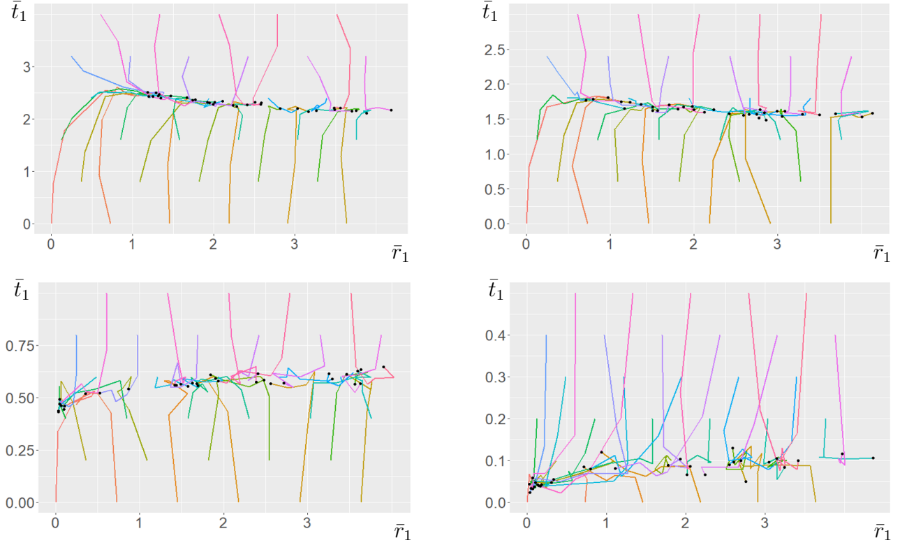
Figure 4.7: Parameter values a = 0.5, f_0 = q_0 = k_0 = 1, f = 5/6, k = 5, t_c = 0.25, q = 0.4, N = 100, n = 10, v = 1 . Plots are positioned in increasing order of \lambda such that (a) [Top left] \lambda = 0.0001 ; (b) [Top right] \lambda = 0.0015 ; (c) [Bottom left] \lambda = 0.2 and (d) [Bottom right] \lambda = 2 . The plots validate more clearly than in Figure 4.6 that increasing \lambda is associated with a decrease in the associated level of toxicity and that the relationship between toxicity and conspicuousness switches from negative (in 4.7a and 4.7b) to positive (in 4.7c and 4.7d). In Figures 4.7(a) and 4.7(b) there is strong selection for solutions with strong signalling component, likely on account of the absolute resident fitness being highest in that direction. In Figures 4.7(c) and 4.7(d) it is clear that the resident fitness is not sufficient to counterbalance the impact of a strong invasion fitness gradient (from the left and along r ). Large spaces between black markers (such as at \bar{r}_1 \approx 1 in Figure 4.7c) are likely due to a balancing effect of these opposite pulls.
