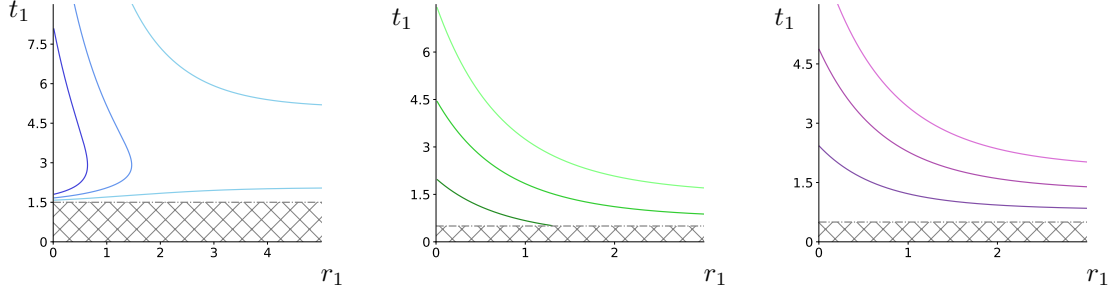
Figure 3.4: Plots show curves of (3.3.2) that result from the root-finding process illustrated in Figure 3.3, such that like-coloured curves correspond to outcomes with equal parameter values. For instance, the bottom curve in Figure 3.3(a), with the lightest shade of blue corresponds to the right-most equilibrium curve of Figure 3.4(a) with the same colour-shading. The diagonally-checked vertical strips of Figure 3 are seen here as horizontal grey-shaded strips. In Figure 3.4(a) the equilibria are disjoint for small values of \alpha and join together at a local r_{max} , which shifts toward lower conspicuousness until undefined at r_1 < 0 . In Figures 3.4(b) & (c) The level of toxicity t_1^* satisfying (??) shrinks with increasing levels of r_1^* and \alpha .
