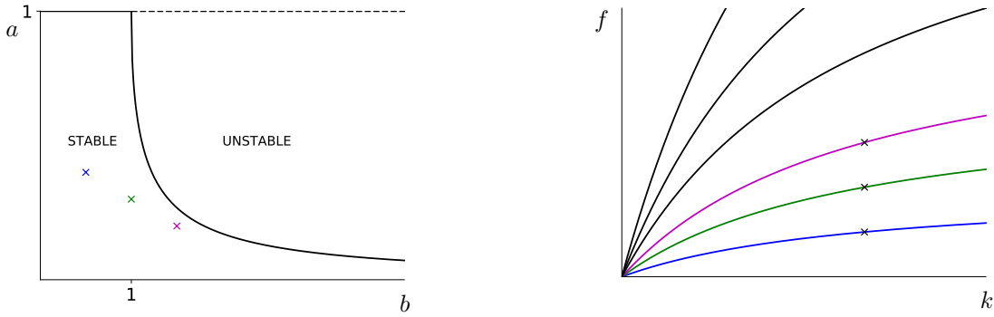
Figure 3.1: On the left figure 3.1(a) are shown the sizes a of mutant groups, against which the residents can withstand invasion (along the t -direction) for given choice of b . A t -stable strategy with f, k and t_c giving b \geq 1 have a maximum associated mutant group size of a^-(b) as described in (3.2.14) - which decreases down to zero as b increases - whereas t -stable strategies with b < 1 can withstand invasion against mutant groups of all sizes. The three x marks with colours blue, green and magenta have coordinates (b, a) given by (0.5, 0.4) , (1, 0.3) and (1.5, 0.2) respectively. Figure 3.1(b) on the right shows the b -level curves of the map (f, k) \mapsto f(\frac{1+kt_c}{k}) , with t_c = 0.5 . Blue, green and magenta correspond to b = 0.5 , b = 1 and b = 1.5 (as do the x marks in (a)) and the x marks in this figure are positioned at coordinates (f, k) = (0.5, 2) , (f, k) = (1, 2) and (f, k) = (1.5, 2) .
