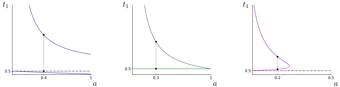
Figure 3.2: Plots showing T_{STAB}^+ (darker colour shades - top branches) and T_{STAB}^- (lighter colour shades - bottom branches) versus a are shown in accordance with (3.2.15), where t_c = 0.5 (dashed horizontal lines) has been used. The specific values of b used in Figures 3.2 (a), (b) and (c) have been generated using the values of f and k that are indicated by the x marks in Figure 3.1(b). The x marks in Figure 3.1(a) indicate the values of a at which the dotted vertical line segments are drawn (their lengths indicating the width of the stable bands in Figure 3). Notably the monotonicities of the curves are in agreement with conditions (3.2.16) and (3.2.18). In particular, Figure 3.2(a) contains curves T_{STAB}^\pm(a) = \frac{1}{a} + 0.5 \pm \frac{1}{a}\sqrt{a^2 + 1} , line drawn at a = 0.4 . Figure 3.2(b) shows T_{STAB}^\pm(a) = \frac{1}{2a} \pm \sqrt{a^2 - 2a + 1}/2a , with T_{STAB}^- = t_c , dotted line drawn at a = 0.3 . Figure 3.2(c) shows \frac{1}{3a} - \frac{1}{6} \pm \frac{1}{3a}\sqrt{a^2 - 4a + 1} with the dotted line drawn at a = 0.2 .
