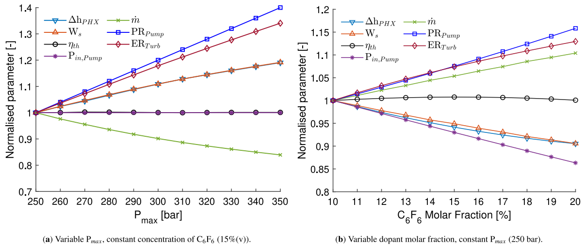
Fig. 7. Relative variation of various cycle parameters as a function of maximum pressure and dopant concentration. A precompression cycle operated with \text{CO}_2/\text{C}_6\text{F}_6 is considered.
