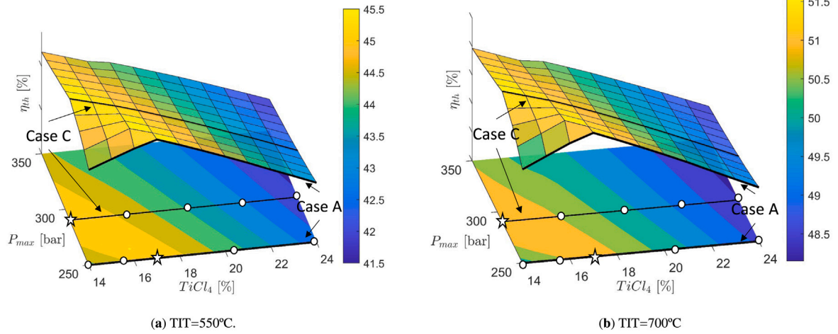
Fig. B.18. Thermal efficiency of a simple recuperated cycle operated with CO_2/TiCl_4 blends as a function of maximum cycle pressure and dopant molar fraction. Two turbines inlet temperatures are considered. The operating conditions employed in turbine design as identified by markers, the different Cases by black solid lines.
