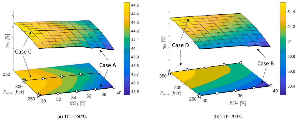
Fig. B.20. Thermal efficiency of a recompression cycle operated with s\text{CO}_2/\text{SO}_2 blends as a function of maximum cycle pressure and dopant molar fraction. Two turbines inlet temperatures are considered. The operating conditions employed in turbine design as identified by markers, the different Cases by black solid lines.
