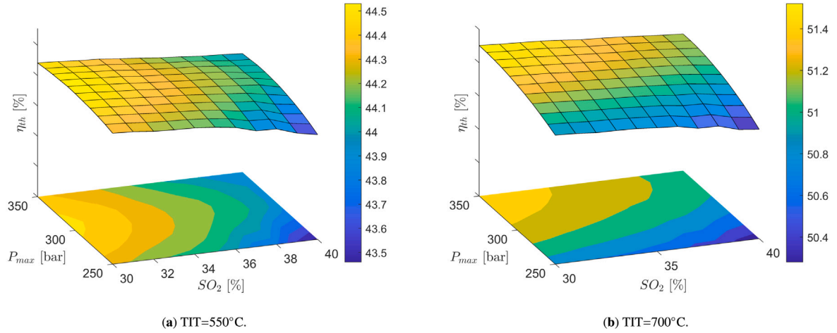
Fig. 5. Thermal efficiency of a recompression cycle operated with CO 2 /SO 2 blends as a function of maximum cycle pressure and dopant molar fraction. Two turbines inlet temperatures are considered.
