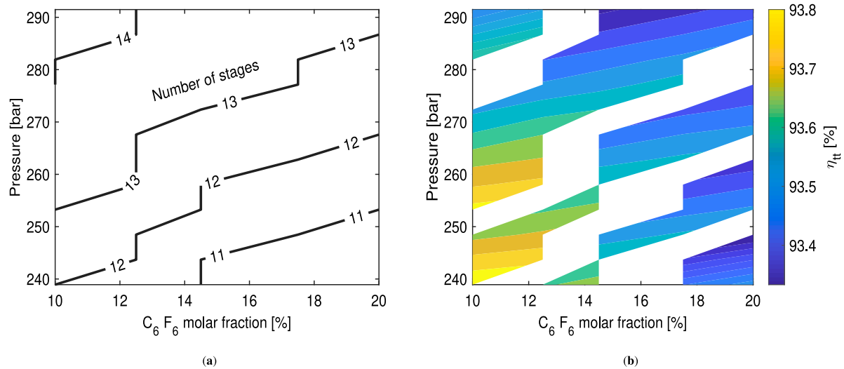
Fig. 14. Contours of the optimal (a) number of stages contours, (b) and total-to-total efficiency [%] for \text{CO}_2/\text{C}_6\text{F}_6 flow paths at a turbine inlet temperature of 550 °C at different turbine inlet pressures and dopant concentrations. Results are generated assuming a 100 MW e power plant.
