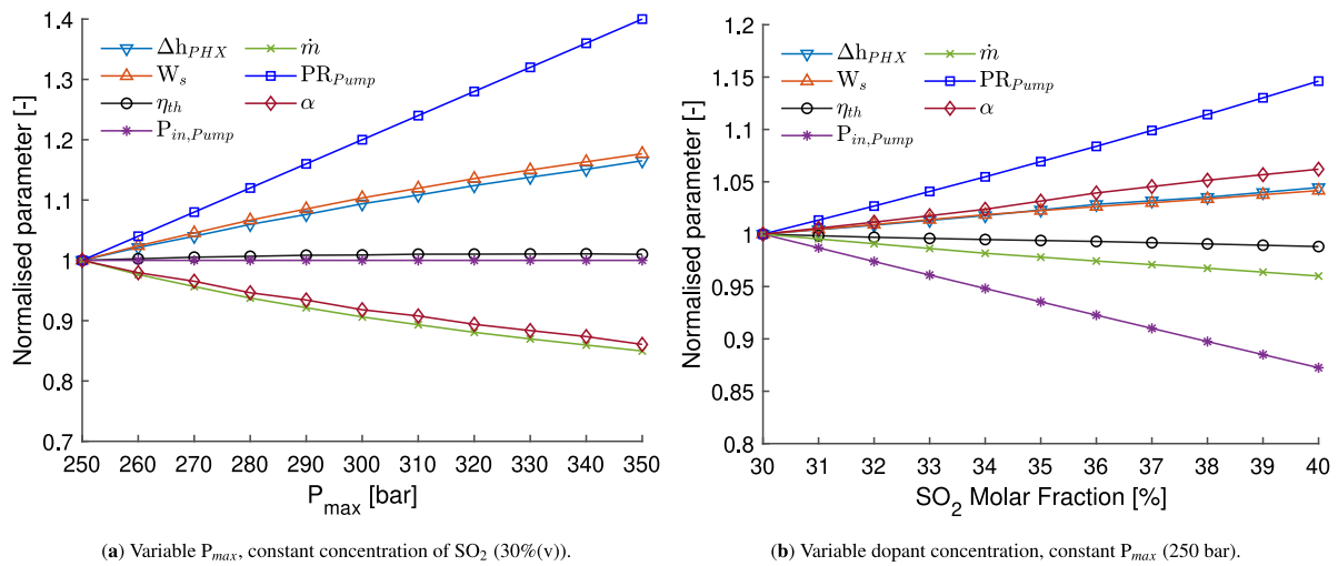
Fig. 8. Relative variation of various cycle parameters as a function of maximum pressure and dopant concentration. A recompression cycle running on \text{CO}_2/\text{SO}_2 is considered. Turbine Expansion ratio is not plotted since this is equivalent to pump Pressure Ratio.
