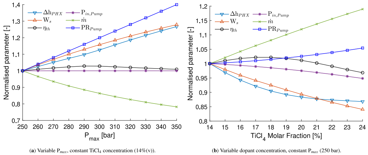
Fig. 6. Relative variation of various cycle parameters as a function of maximum pressure and dopant concentration. A simple recuperated cycle operating on \text{CO}_2/\text{TiCl}_4 blends is considered. Turbine Expansion ratio is not plotted since it is equivalent to pump Pressure Ratio.
