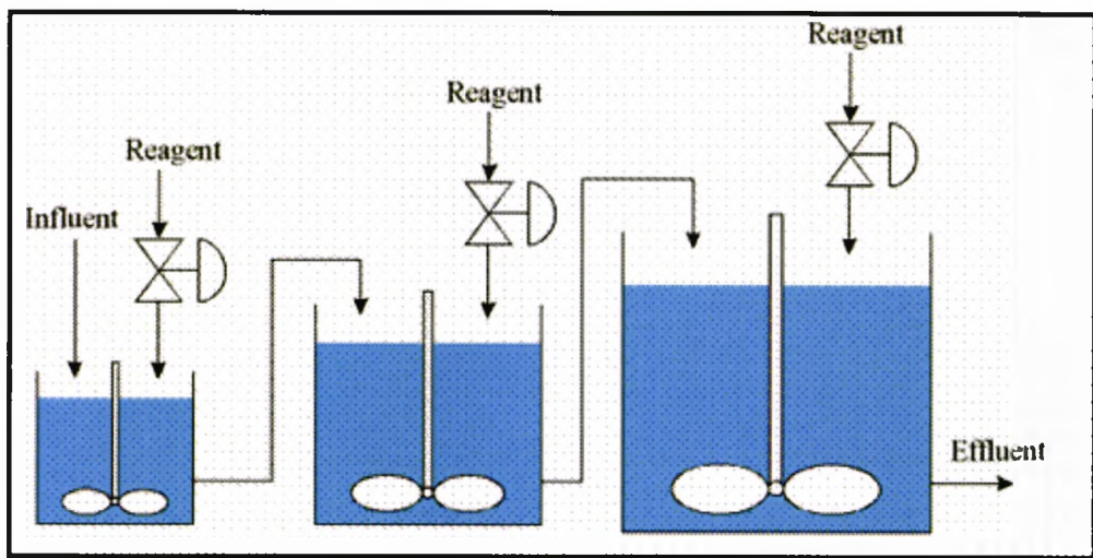
Fig. 2.2: Successive treatment pH control – precision is achieved in three stages from “coarse” to “fine” regulation to prevent the system response overshooting (Omega Engineering).
