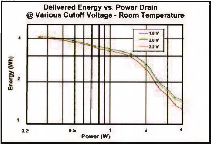
Fig. 6.9: Energy utilization of \text{LiMnO}_2 DL123 cell at various constant power loads and different cut-off voltages (Duracell).
