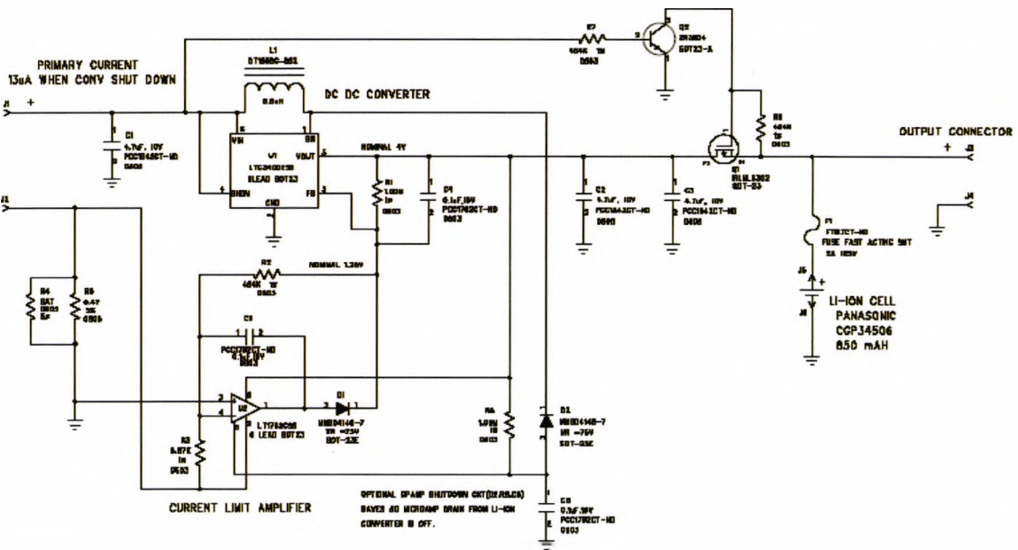
Fig. 6.17: Hybrid circuit diagram, showing all electronic components and their connections to create a very efficient voltage booster/Li-ion charger (shown expanded in Appendix 10).
