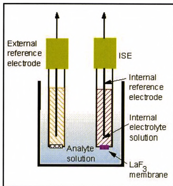
Fig. 3.1: Ion selective electrode, based on measurement of the potential difference between two reference electrodes separated by an ion-selective membrane (Omega Engineering).
