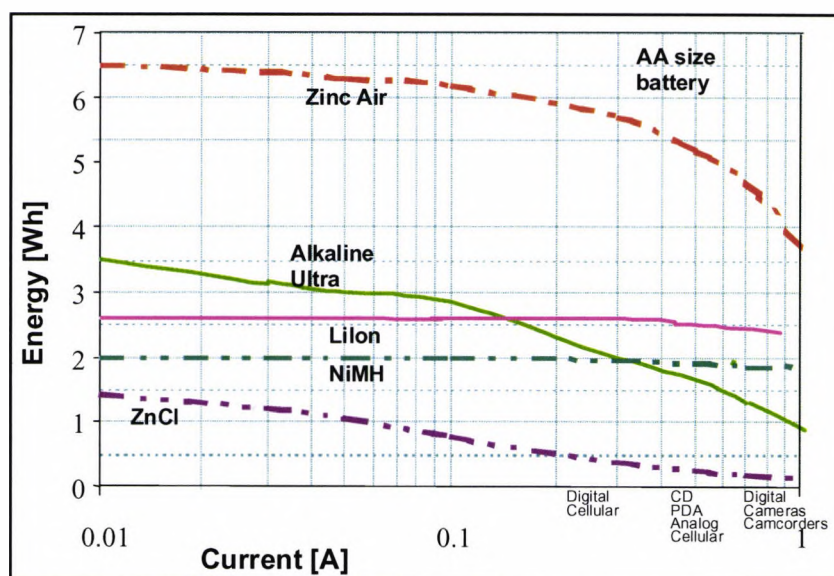
Fig. 6.2: Deliverable energy versus current drain: at high rate of discharge, primary batteries lose efficiency and rechargeable batteries provide better energy utilization (Duracell).
