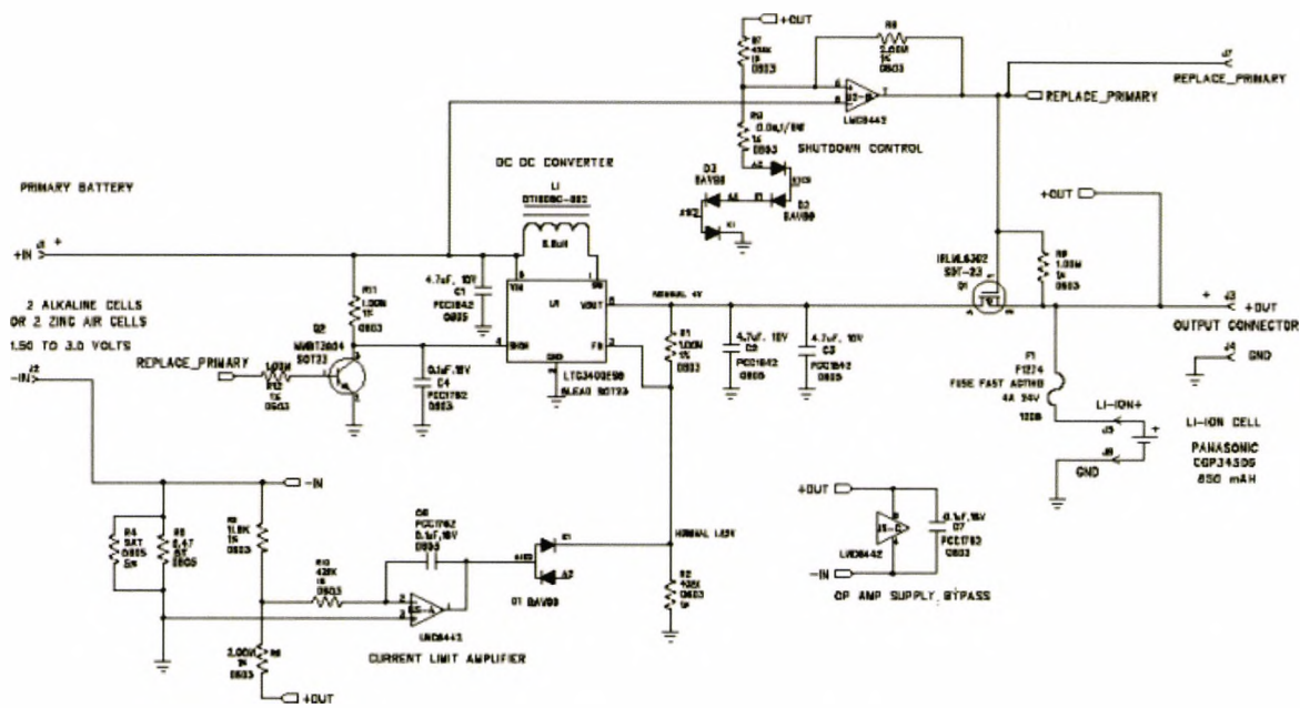
Figure 6.20: Hybrid circuit diagram (Version 2).
