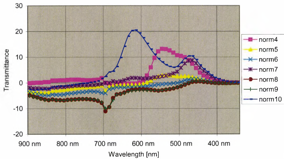
Fig.8.8: Indicator Normalized Spectra.
