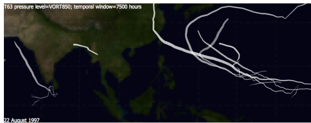
Figure 3: 'Sticky tracks' in the West Pacific where multiple storms follow similar paths within a relatively short temporal window, zoomed to the West Pacific region.
