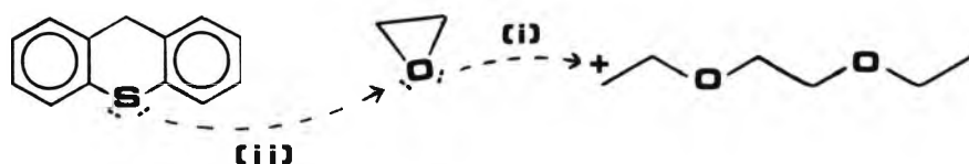
Scheme 4.4 The nucleophilic character of sulphur in the cationic polymerisation of an epoxide
