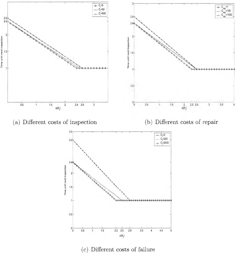
Figure 6.11: Optimal inspection scheduling functions m_1 for different inspection and maintenance costs, \xi = 3 .
