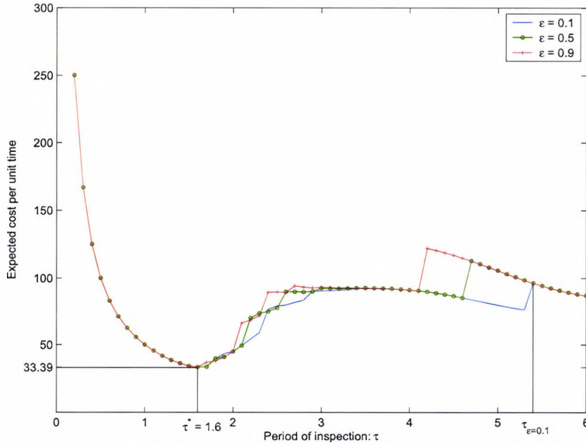
Figure 6.4: Effect of parameter \epsilon on the optimal solution C_{\tau}^{0*} with parameters (k, \xi^*, \tau^*) = (0.9, 9.5, 1.6) .
