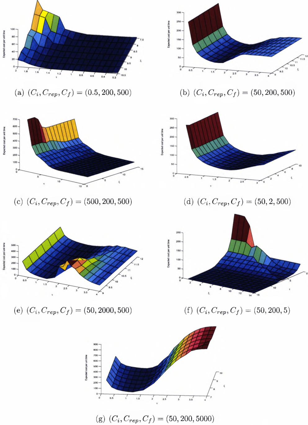
Figure 6.2: Expected cost per unit time for different cost values ( k = 0.9 , \epsilon = 0.5 ).
