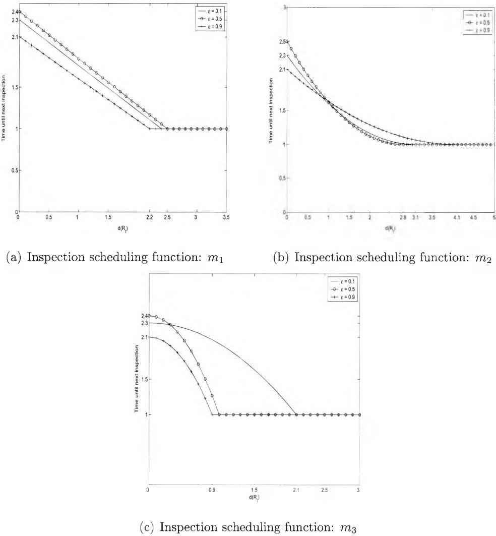
Figure 6.13: Optimal inspection scheduling functions for different values of parameter \epsilon , \xi = 3 .
