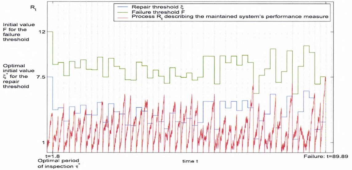
Figure 6.5: Simulation of the proposed model over a cycle, with (C_i, C_{rep}, C_f) = (50, 2, 500) and (k, \epsilon, \tau^*, \xi^*) = (0.9, 0.5, 1.8, 7.5) .
