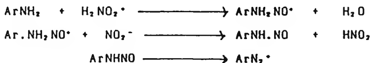
Scheme 3.3 nitrous acid diazotisation - mechanism 1
