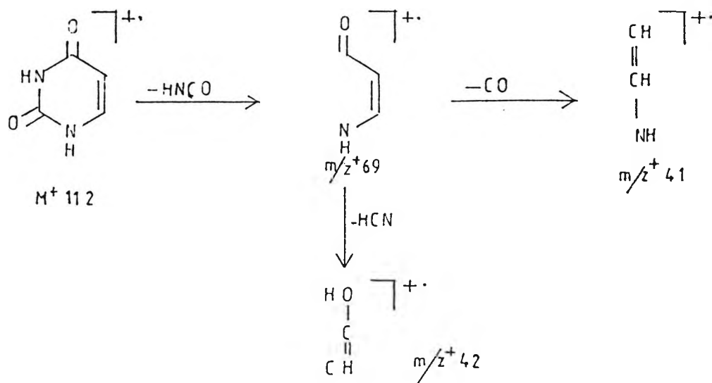
Scheme 4.4 Fragmentation of uracil
