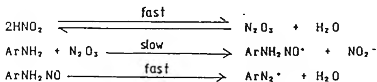
Scheme 3.4 Nitrous acid diazotisation - mechanism 2
