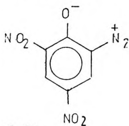
Scheme 3.1 Resonance forms of a diazo oxide
