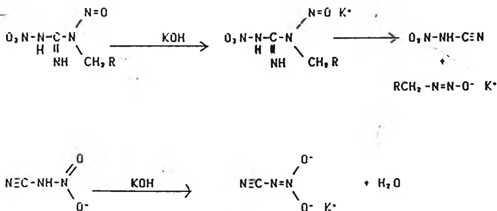
Scheme 3.16 Diazotization of N-nitrosoguanidines
