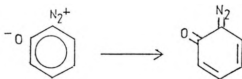
Scheme 3.1 Resonance forms of a diazo oxide
