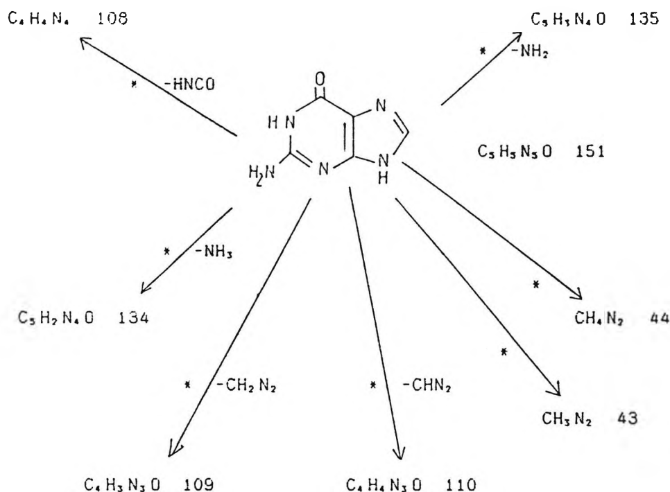
Scheme 4.7 Fragmentation of guanine
