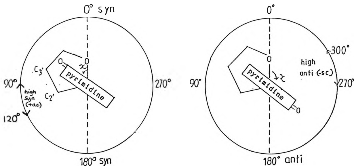
Scheme 1.6 "High syn" and "high anti" conformations
