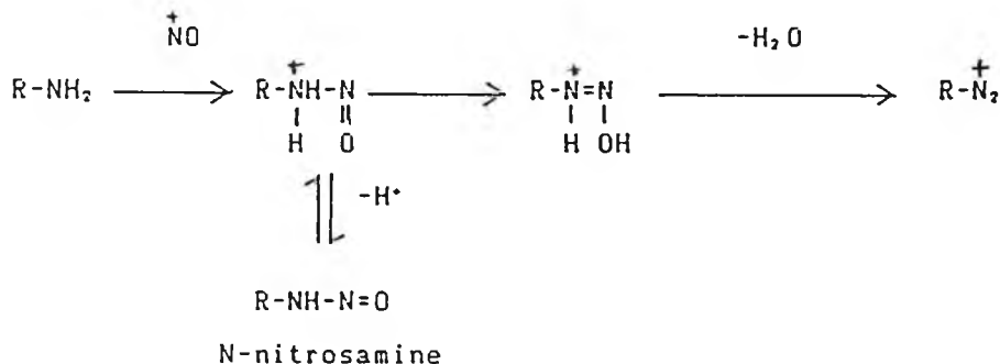
Scheme 3.5 Diazotization of an amine
