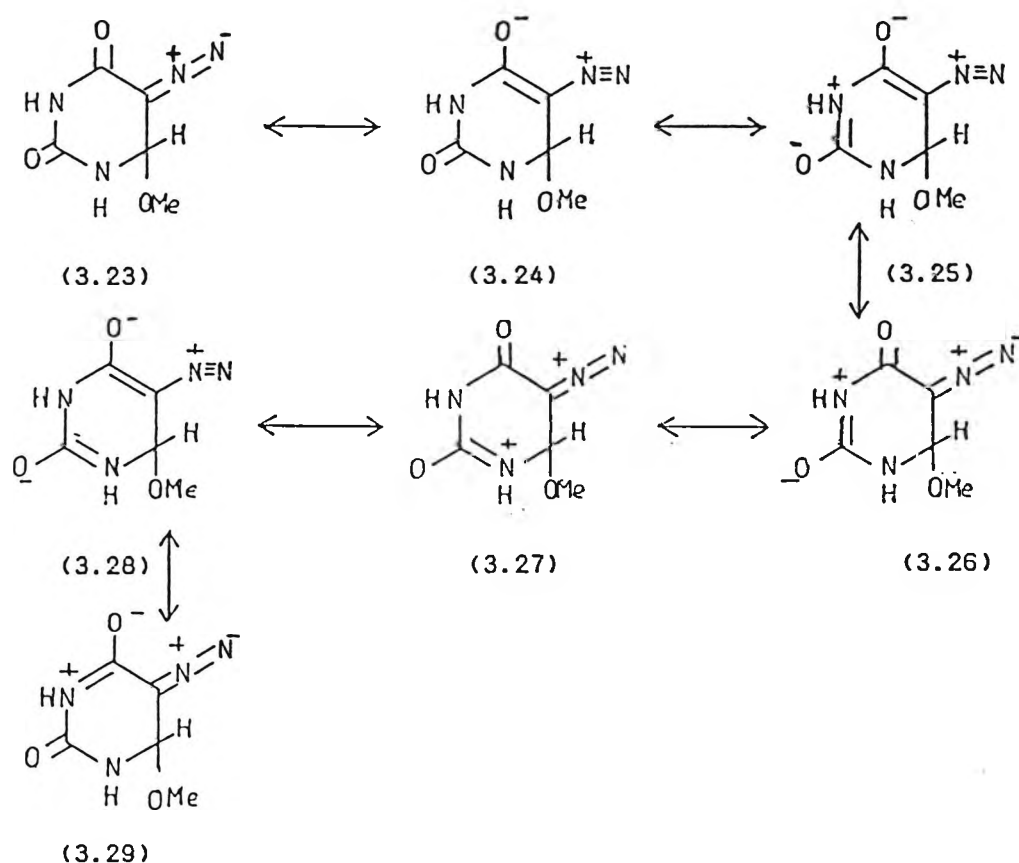
Scheme 3.25 Resonance forms of 5-diazo-6-methoxy-1,6-dihydrouracil
