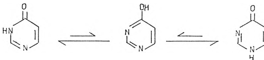
Scheme 4.1 Tautomeric forms of 4-pyrimidone
