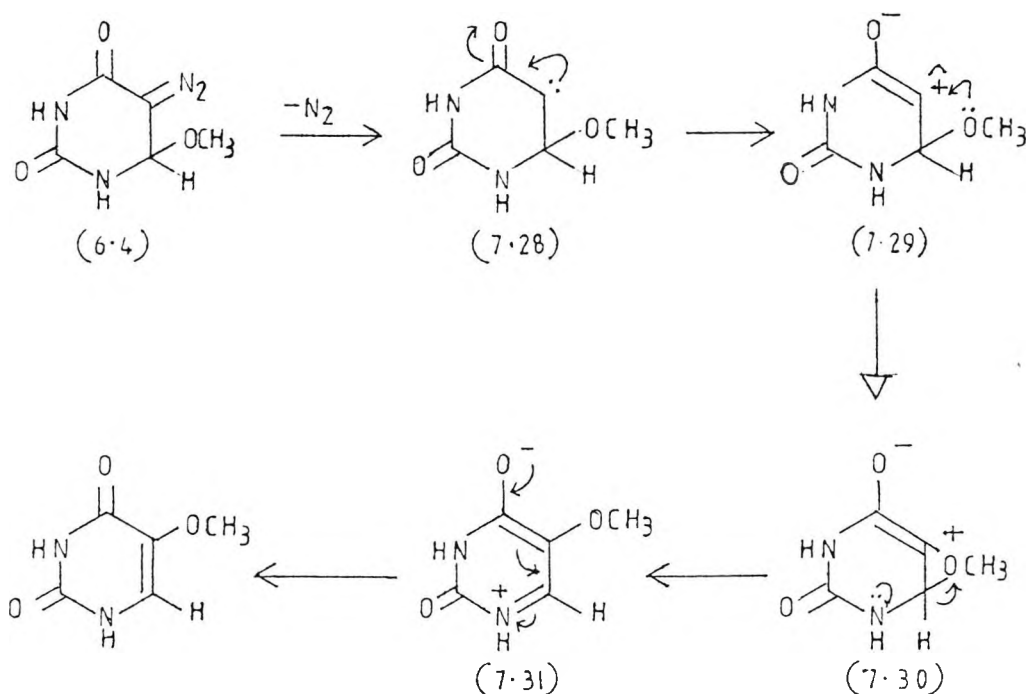
Scheme 7.29 Formation of 5-methoxyuracil
