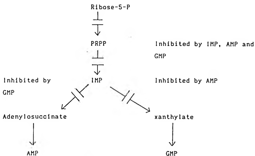
Scheme 2.3 Feedback control of AMP and GMP biosynthesis
