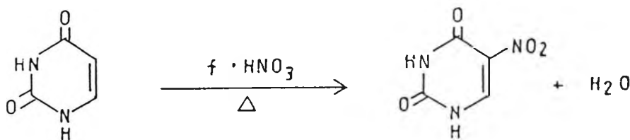
Scheme 6.25 Nitration of uracil
