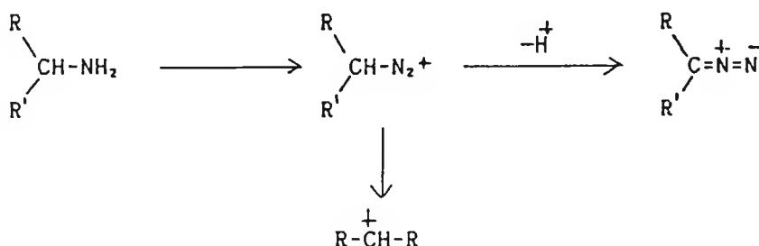
Scheme 3.6 Diazotisation of alkylamines
