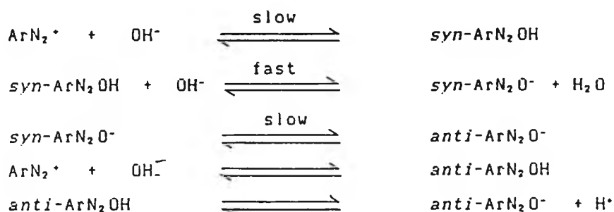
Scheme 3.21 Diazotate equilibria
