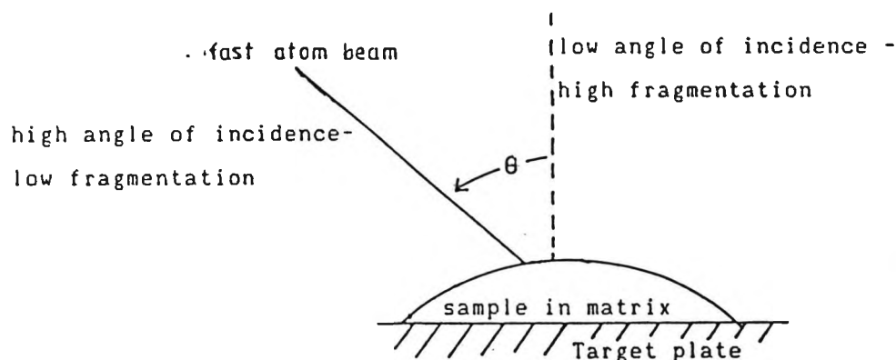
Diag. 4.8 Angle of incidence and fragmentation in FAB
