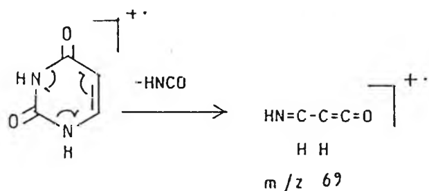
Scheme 6.4 Retro Diels-Alder fragmentation
