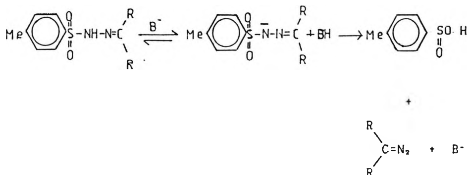
Scheme 3.11 Diazotization of Tosylhydrazones
