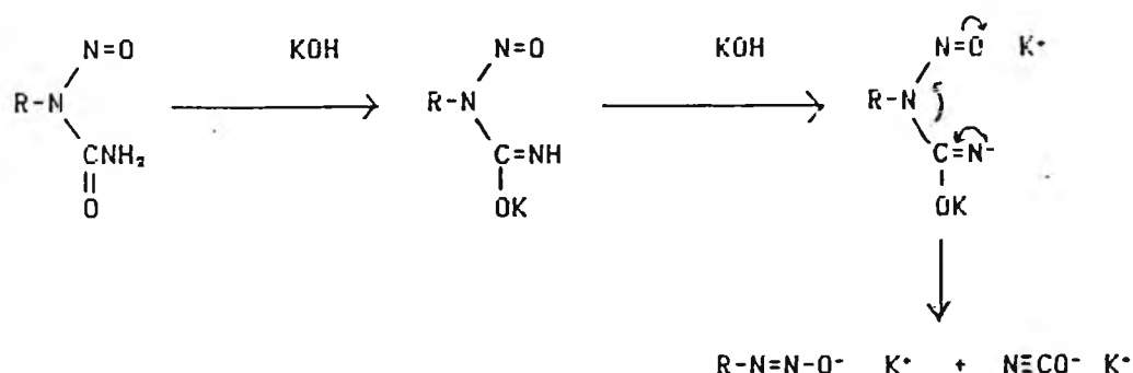
Scheme 3.14 Diazotization of N-nitrosoureas
