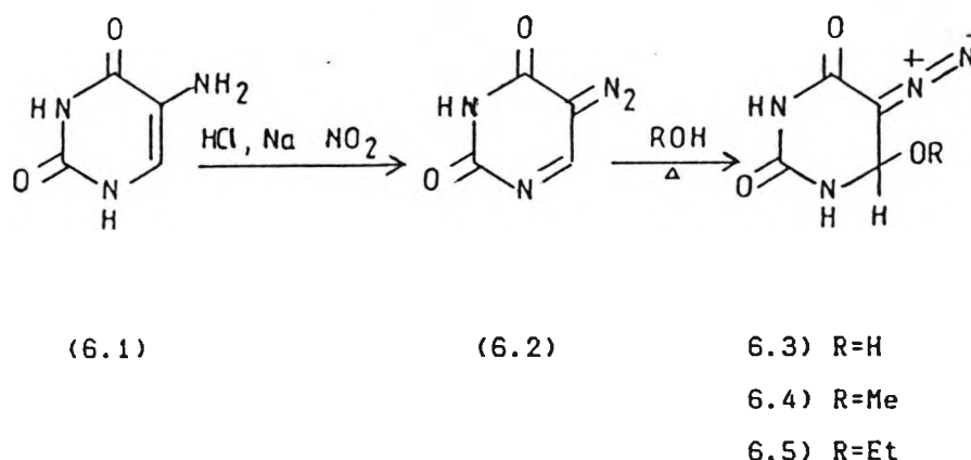
Scheme 6.1 Addition to 1,6-double bond of 5-diazouracil
