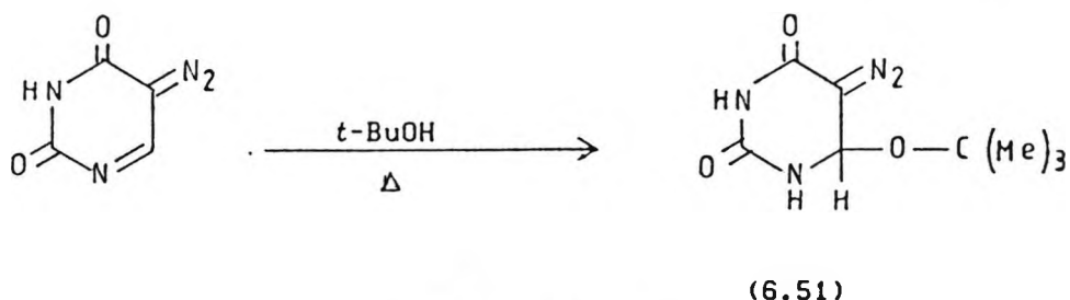
Scheme 6.22 Preparation of 5-Diazo-5- tert -butoxy-1,6-dihydrouracil
