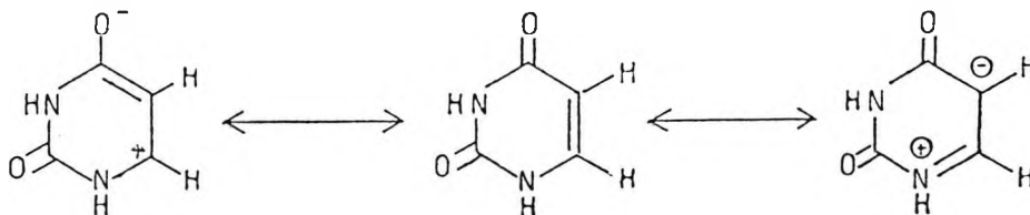
Scheme 6.26 C-5 activation and C-6 deactivation of uracil
