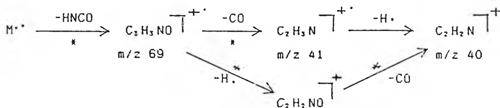
Scheme 6.3 EI-MS fragmentation of Uracil
