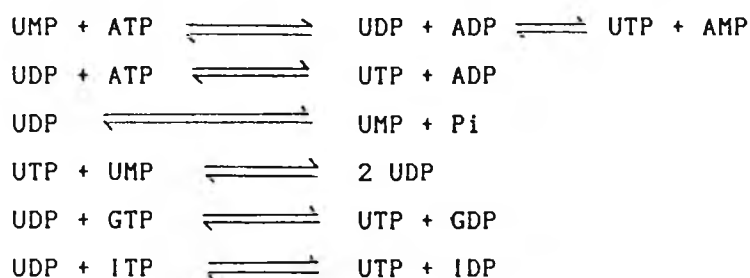
Scheme 2.5 Interconversion of nucleotides
