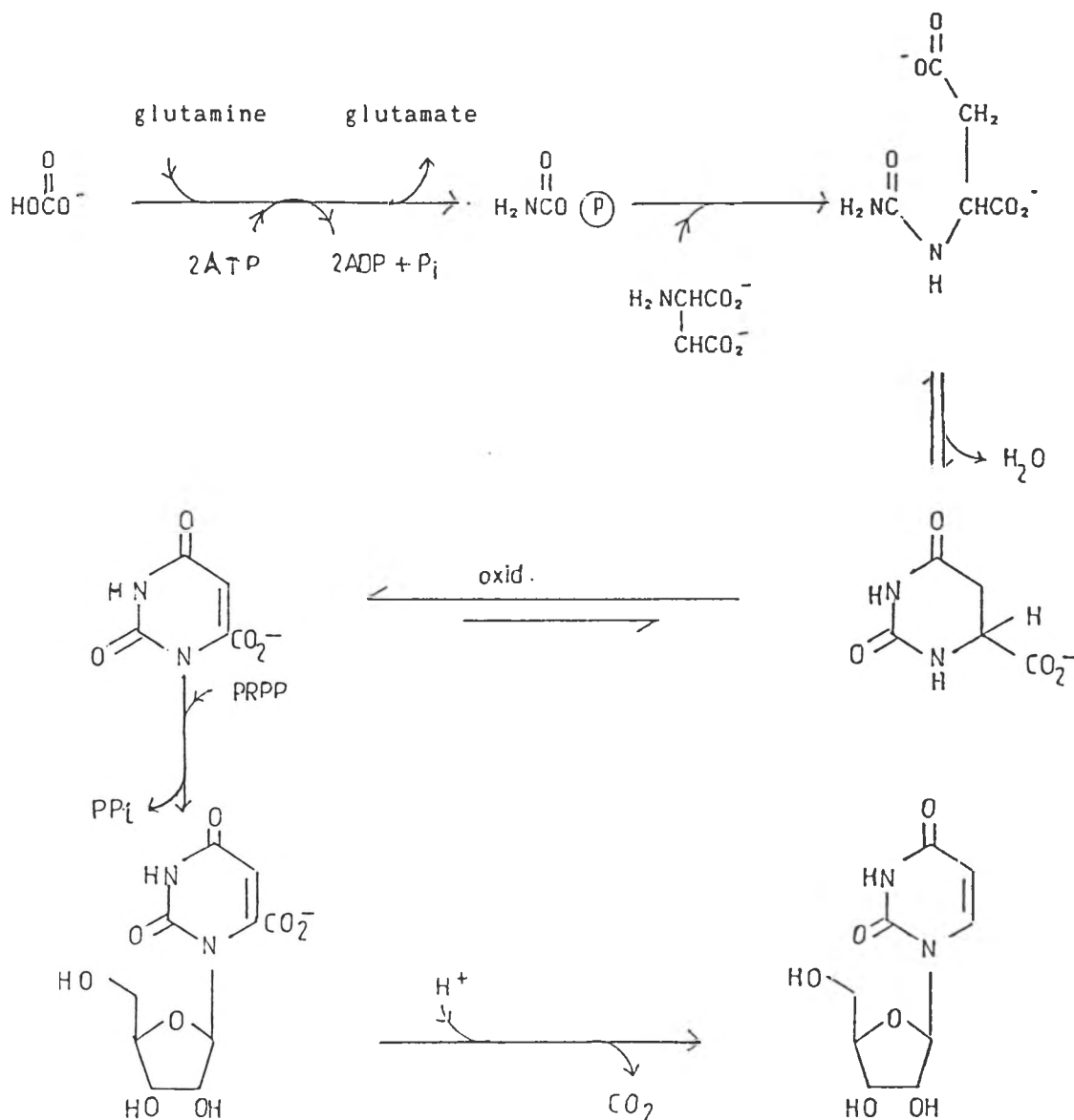
Scheme 2.4 Biosynthesis of uridine
