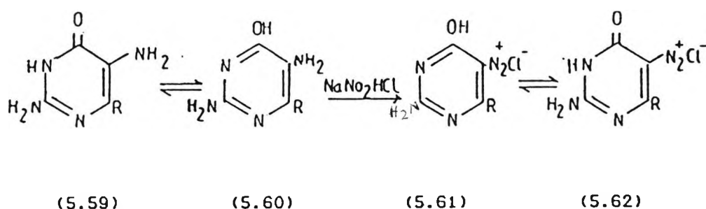
Scheme 5.22 Diazotization of 2,5-diaminopyrimidine
