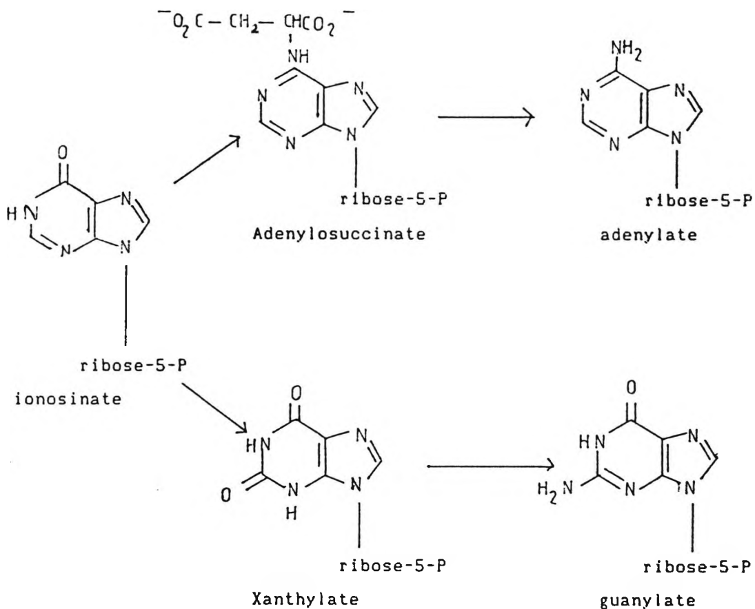
Scheme 2.2 Postsynthetic modification of Inosinate
