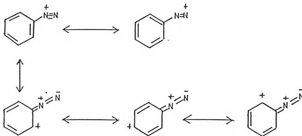
Scheme 3.20 Canonical forms for the benzenediazonium ion
