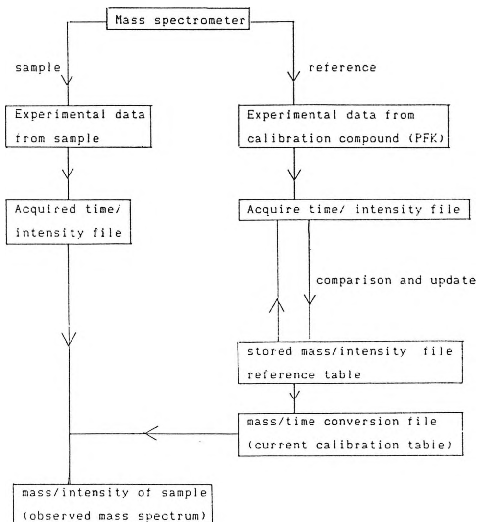
Scheme 4.3 Mass spectrometer operation.
