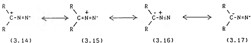
Scheme 3.23 Resonance forms for a diazoalkane
