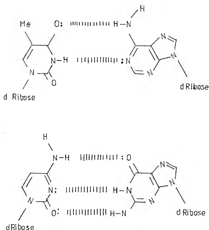
Scheme 2.6 Thymine-adenine and cytosine-guanine base-pairing
