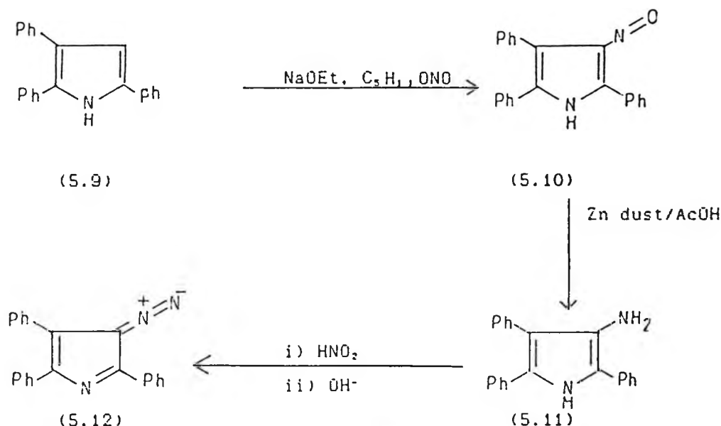
Scheme 5.2 Preparation of 3-diazo-2,4,5-triphenylpyrrole
