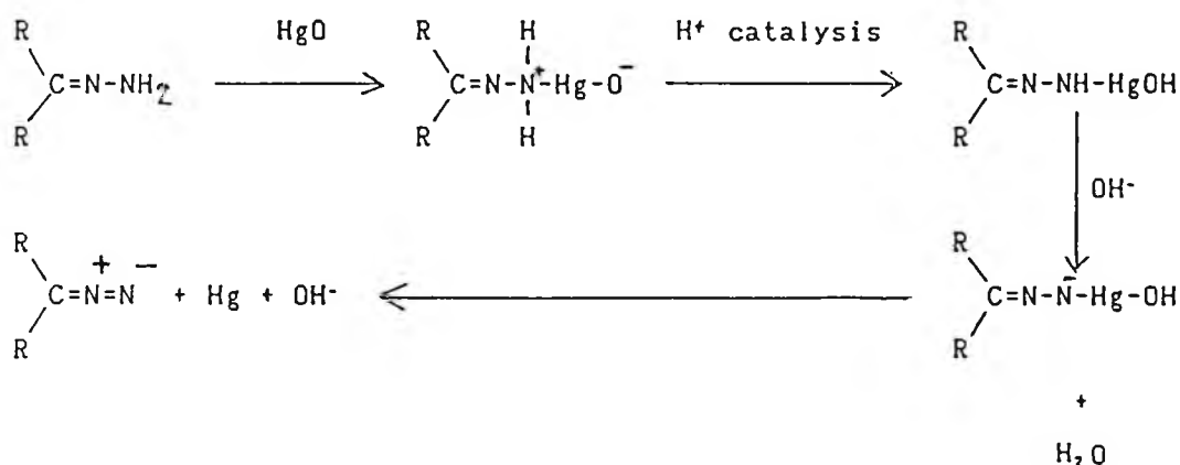
Scheme 3.10 Diazotization of hydrazones
