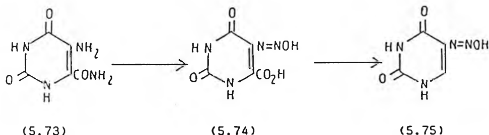
Scheme 5.25 Preparation of "5-diazouracil hydrate"
