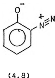
"Diazonium phenolate"
