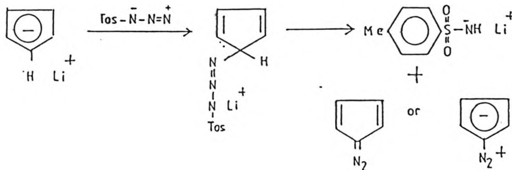
Scheme 3.17 diazo transfer to cyclopentadiene
