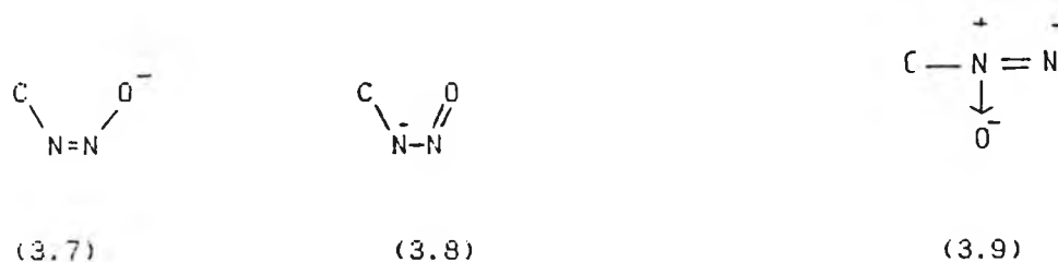
Scheme 3.22 Resonance forms for a diazotate
