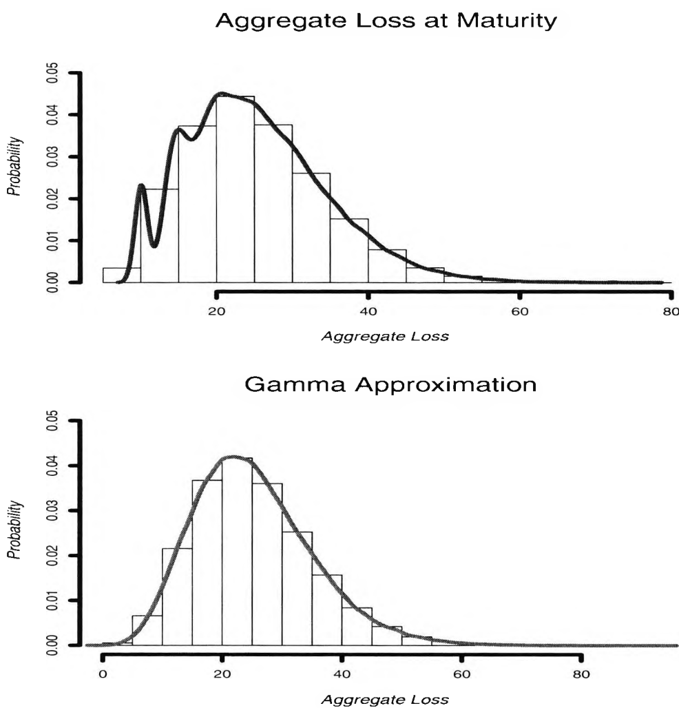
Figure 6.1: Distribution of the Aggregate Index Loss
