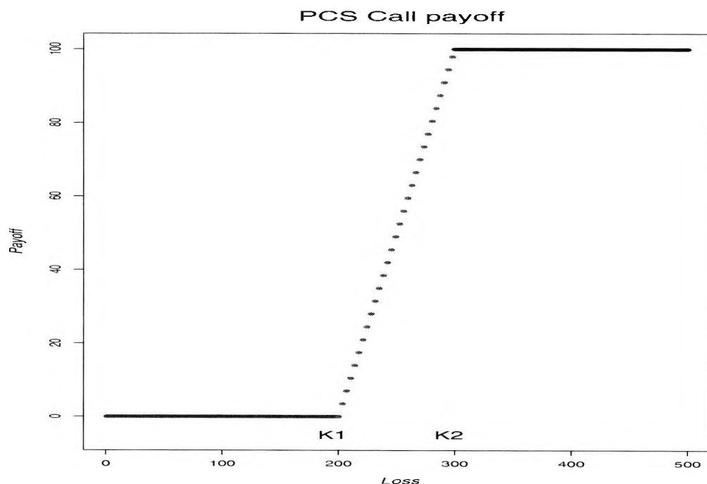
Figure 5.2: Illustration of a PCS call option
