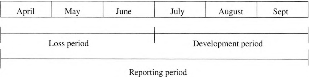
Figure 5.1: Illustration of a CAT contract
