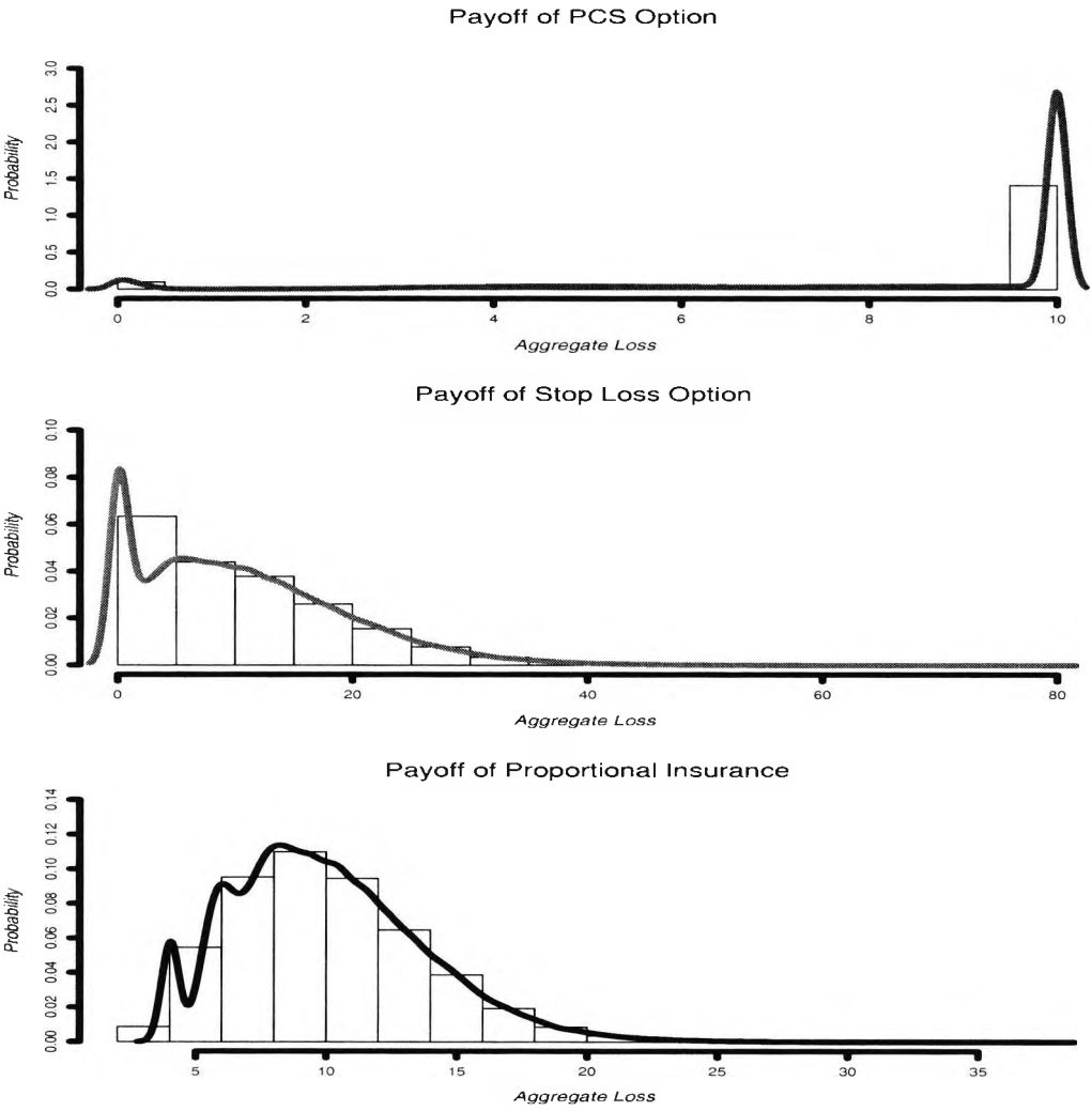
Figure 6.2: Distribution of the Payoff
