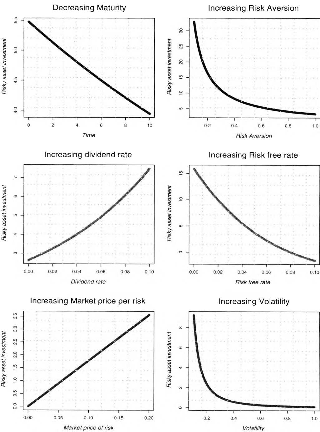
Figure 4.1: Optimal Asset allocation
