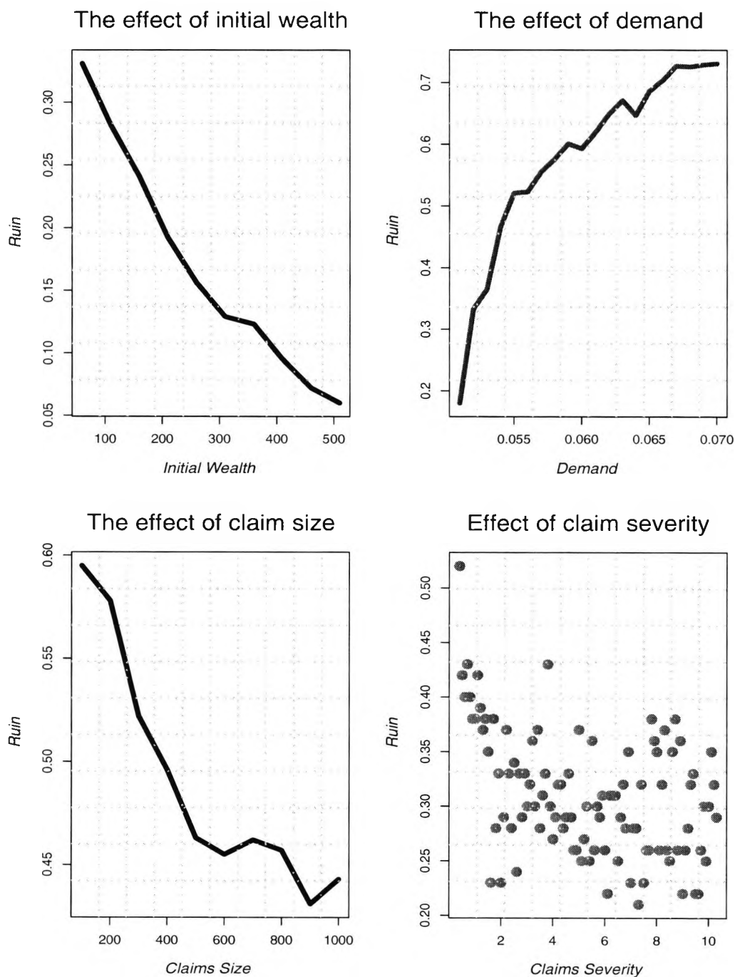
Figure 3.2: Sensitivity of the ruin probability
