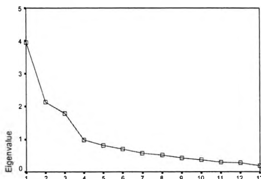
Scree Plot
