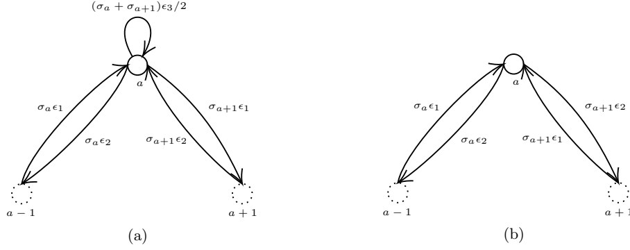
FIGURE E.0.2: The values of \tilde{\epsilon}_I associated to bifundamentals and adjoints subject to the loop and vertex constraints for generalized conifolds. We have (a) \varsigma_a = \varsigma_{a+1} and (b) \varsigma_a = -\varsigma_{a+1} , where \epsilon_{1,2,3} are parameters of the quiver Yangian.
