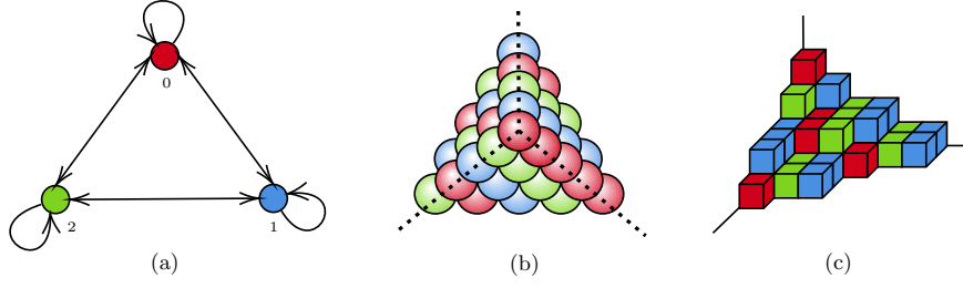
FIGURE 5.7.1: (a) The quiver for \mathbb{C} \times \mathbb{C}^2 / \mathbb{Z}_3 . (b) The corresponding crystal model with three colours. The dashed lines are the ridges of the crystal. (c) The equivalent crystal model visualized using coloured plane partitions.
