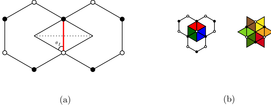
FIGURE 3.1.2: (a) The edge in red has length l . Its dashed dual edge is of length \sqrt{4-l^2} which equals the weight of the edge. The rhombus angle is labelled by \theta_I . The corresponding internal angle 2\theta_I of the rhombus gives the R-charge physically. (b) The left plot indicates \sum 2\theta_I = 2\pi which corresponds to each superpotential term while the right plot indicates \sum(\pi - 2\theta_I) = 2\pi which corresponds to (the fields connected to) each node in the quiver.
