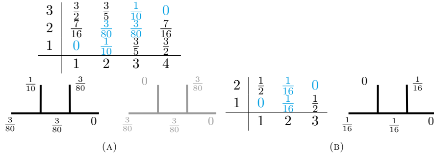
FIGURE C.2.2: Here we list the first possible examples of CBs that \Gamma_0(4) \cap \Gamma(2) corresponds to: (a) The first CB for (+, +, -, -) . For reference, the one in grey is the CB from (-, +, -, +) for this minimal model. (b) The first CB for (-, +, -, +) .
