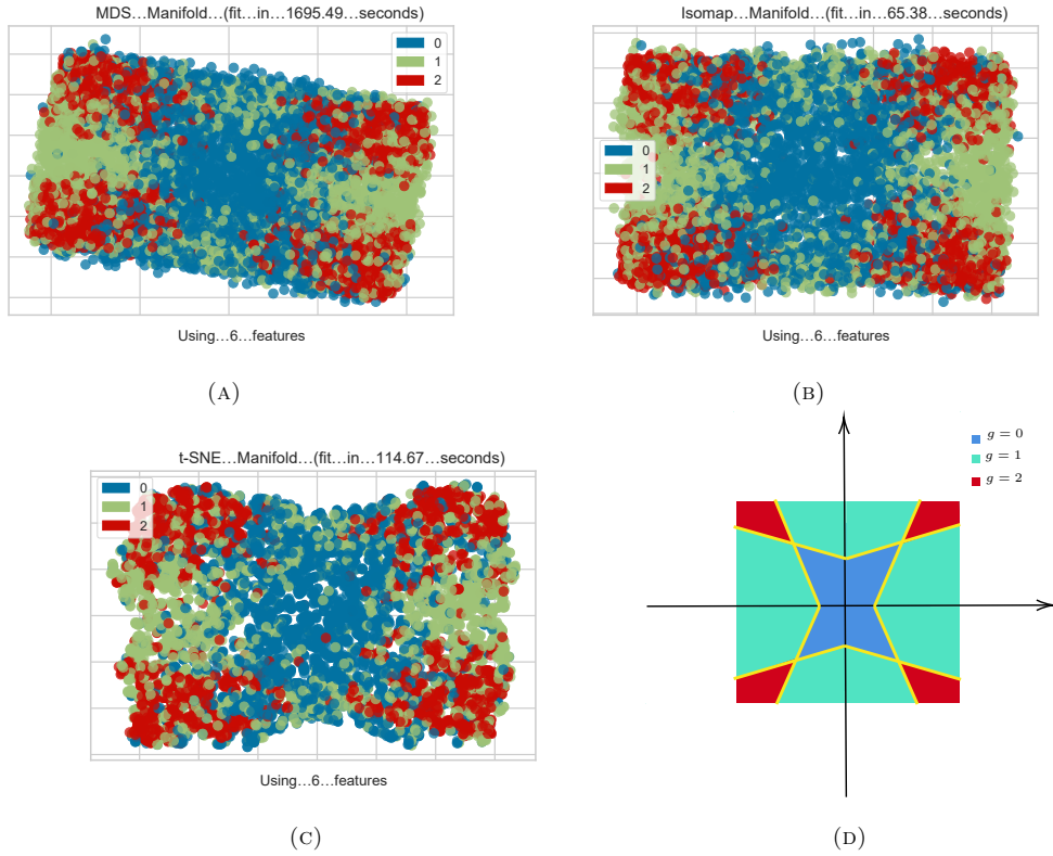
FIGURE 7.2.4: (a) The MDS embedding manifold projection of the dataset for L^{3,3,2} . (b) The Isomap embedding manifold projection. (c) The t-SNE embedding manifold projection. For instructions on these manifold projections, one is referred to [275]. (d) The sketch of an ideal separation of the data points.
