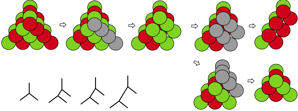
FIGURE 5.1.5: Peeling off the semi-infinite faces of the \mathbb{C} \times \mathbb{C}^2/\mathbb{Z}_2 crystal.
