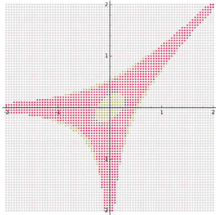
FIGURE 7.2.1: It is clear from this example that the lopsided amoeba contains the amoeba as a subset. Figure taken from [274, Figure 1].
