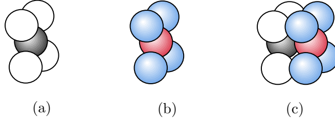
FIGURE 5.1.1: (a) The crystal for \tilde{C}_2 for the conifold \mathcal{C} . (b) The same copy with different colours. (c) The crystal which is a disjoint union of (a) and (b).
