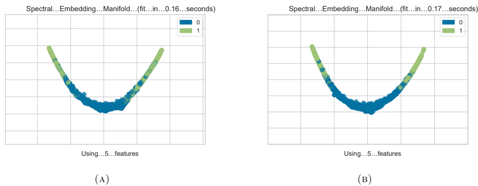
FIGURE 7.2.3: (a) The spectral embedding manifold projection of the dataset for F_0 . For the input vectors, c_{1,2,3,4} range from -5 to 5 while c_5 ranges from -20 to 20 . (b) To verify our explanation for (a), we generate a dataset whose two classes are separated by c_5'^2 = 4|c_1'c_3'| + 4|c_2'c_4'| + c_0 (with c_i' the same range as c_i ), where c_0 = 4 \times 2 \times 2.5^2 as 2.5 is the average of the possible values for c_{1,2,3,4} .
