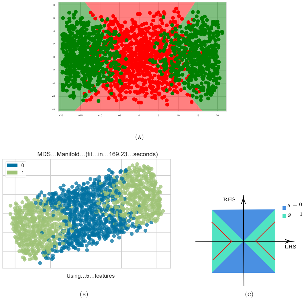
FIGURE 7.2.2: (a) The kernel PCA projection for an NN. (b) The MDS manifold projection which gives a better separation of the two classes of points. (c) Ideally, the blue and green regions would be separated by y = \pm x . In practice, due to the complication of square roots, the NN would get shifted. This shift, i.e., the actual separation of the blue and green points, is indicated by the red lines here.
