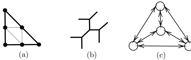
FIGURE F.1.2: (a) The toric diagram for \mathbb{C}^3/(\mathbb{Z}_2 \times \mathbb{Z}_2) . (b) Its dual web diagram. (c) The corresponding quiver (the Mercedes-Benz quiver).
