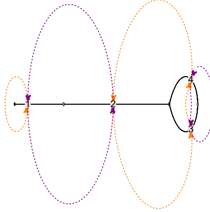
FIGURE 4.3.1: The dessin associated to \Gamma_0(3) with passport \{1^1 3^1, 2^2, 1^1 3^1\} . Here, the numbers are the labels of the edges, and the orange (purple) cycles indicate the permutations around black (white) vertices.
