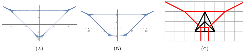
FIGURE 3.2.2: (a) The amoeba for the Newton polynomial P(z, w) = -w - z^{-1}w^{-1} - zw^{-1} - 2ew^{-1} + e^{10} . (b) The amoeba for the Newton polynomial P(z, w) = -w - z^{-1}w^{-1} - zw^{-1} - 2e^5w^{-1} + e^{10} . (c) The spine (in red) is the dual of the triangulated Newton polygon \Delta (in black).
