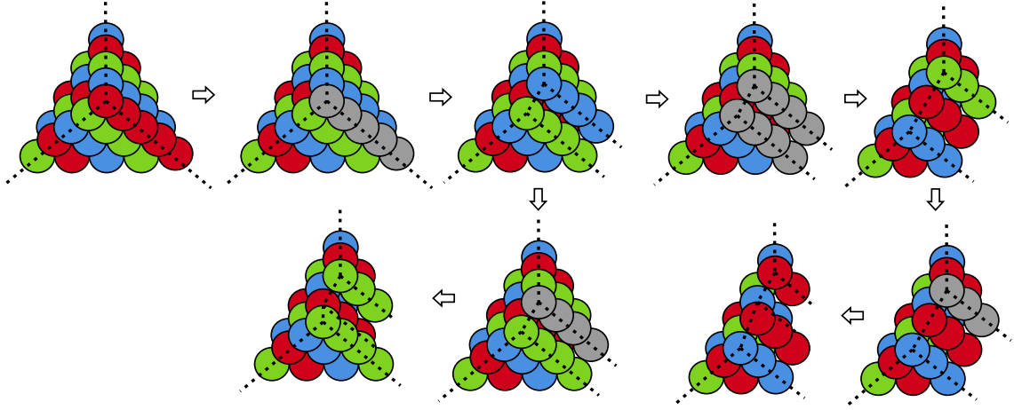
FIGURE 5.1.6: Peeling off the semi-infinite faces of the \mathbb{C} \times \mathbb{C}^2/\mathbb{Z}_3 crystal. The dashed brane webs is composed of the ridges.
