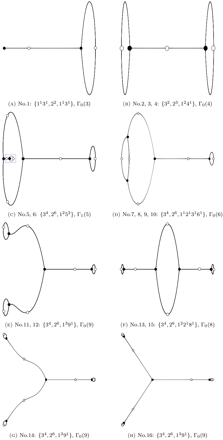
FIGURE 4.2.1: The dessins for reflexive polygons with maximally tempered coefficients, their passports and the corresponding congruence subgroups.
