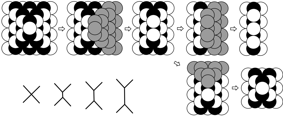
FIGURE 5.1.4: Peeling off the semi-infinite faces of the conifold crystal. This changes the length of the top row.
