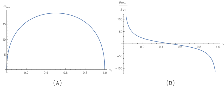
FIGURE 3.2.4: The plot of (a) m_{\text{iso}} and (b) \partial m_{\text{iso}}/\partial \nu_1 . Here \nu_2 = 1 - \nu_1 .
