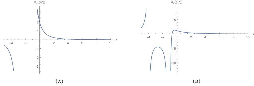
FIGURE 6.1.2: (a) The conifold w^2 + x^2 + y^2 + z^2 = 0 and \eta with charges (0, -1, -1, -1) , and a_0(\zeta(\epsilon)) = \frac{16}{(\epsilon+2)^3} . (b) The E_7 threefold w^2 + x^2 + y^3 + yz^3 = 0 and \eta with charges (-1, -1, 0, -1) , and a_0(\zeta(\epsilon)) = \frac{750(3\epsilon+2)}{(\epsilon+4)(17\epsilon+18)^2} .
