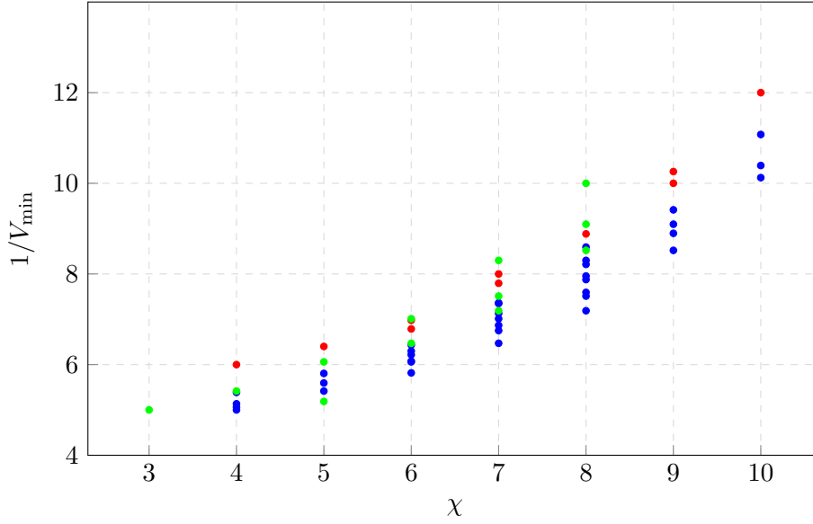
FIGURE 2.3.4: There are large gaps between red points and others. In other words, the red points are much closer to the lower bound of volumes.
