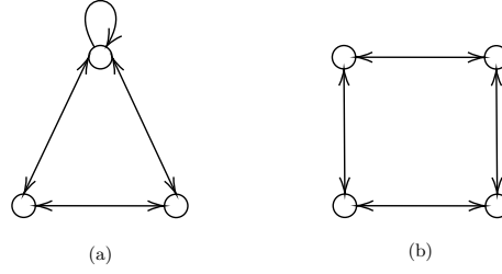
FIGURE 5.5.1: (a) The SPP quiver with (M, N) = (2, 1), (1, 2) . (b) The quiver for the \mathbb{Z}_2 orbifold of the conifold with (M, N) = (2, 2) in one of the toric phases.
