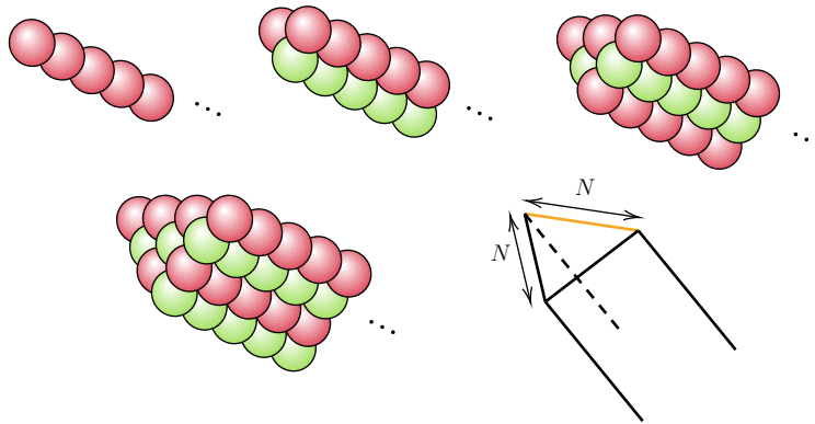
FIGURE 5.1.2: The crystal for chamber \tilde{C}_N for \mathbb{C} \times \mathbb{C}^2/\mathbb{Z}_2 . Here we show the cases for N = 1, 2, 3, 4 . We also give a sketch of general N with the orange line as the top row. The crystal is infinitely long.
