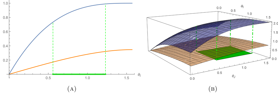
FIGURE 3.2.3: The a -function (blue) and isoradial Mahler measure (orange) plotted as functions of \theta_I . We can only visualize the (a) 1d and (b) 2d versions while physically there should be at least 3 \theta_I 's ( R_I 's) in our theory. Notice that we have shifted the a -function by (a) +1 and (b) +2 for better visualization and comparison. The green region is the conformal manifold on the \theta_I axis/ \theta_I - \theta_J plane.
