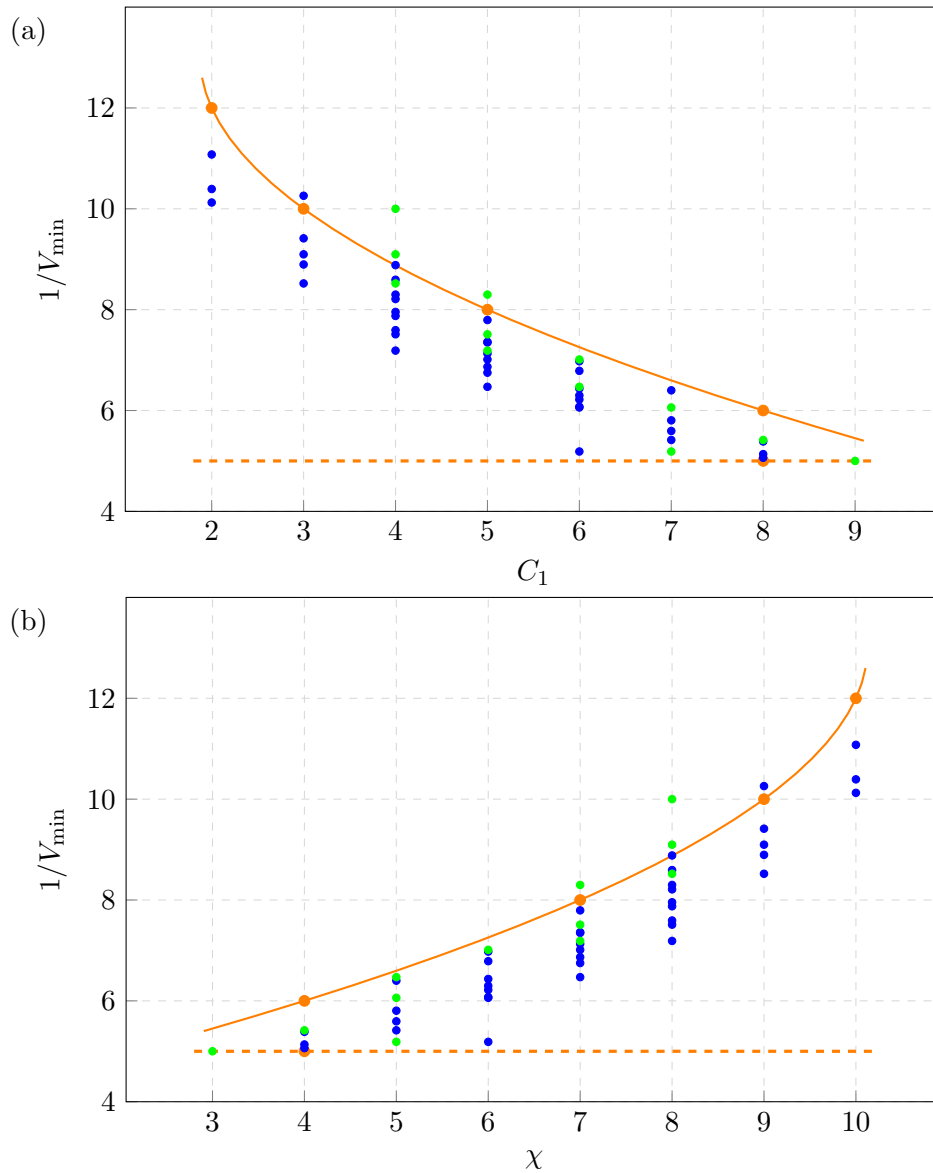
FIGURE 2.3.3: The green points correspond to \widetilde{X(\Delta)} built from first-grade points. The varieties (from zeroth-grade points) of triangles are in orange.
