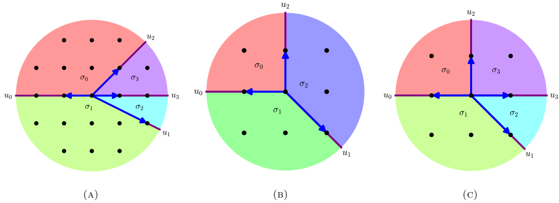
FIGURE 2.3.1: (a) The complete resolution \widetilde{X_0} is constructed from the zeroth-grade point. The Euler number \chi_0 is 4. (b) The toric variety X_1 is already smooth, viz, X_1 = \widetilde{X_1} . The Euler number \chi_1 is 3. (c) We make a further blow-up on X_1 by adding the ray u_3 = (1, 0) . The new variety \widetilde{X'_1} has Euler number \chi'_1 = 4 .
