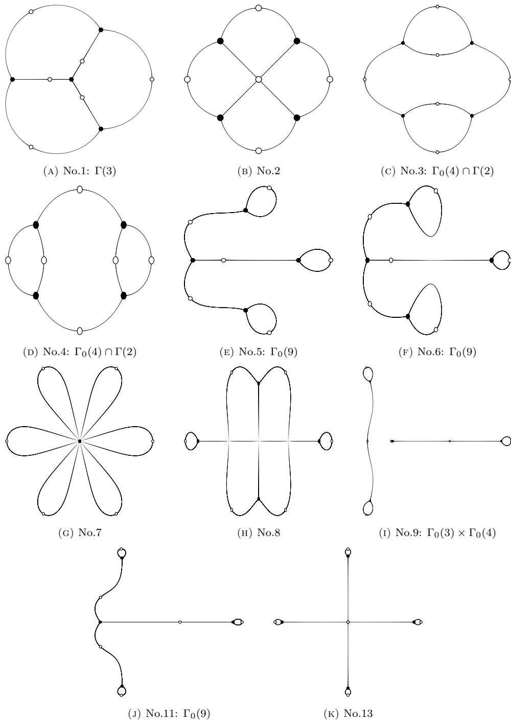
FIGURE D.1.1: The dessins (or just graphs from j/1728 ) for reflexive polygons with minimally tempered coefficients. As listed, some of them correspond to certain congruence subgroups (as coset graphs).
