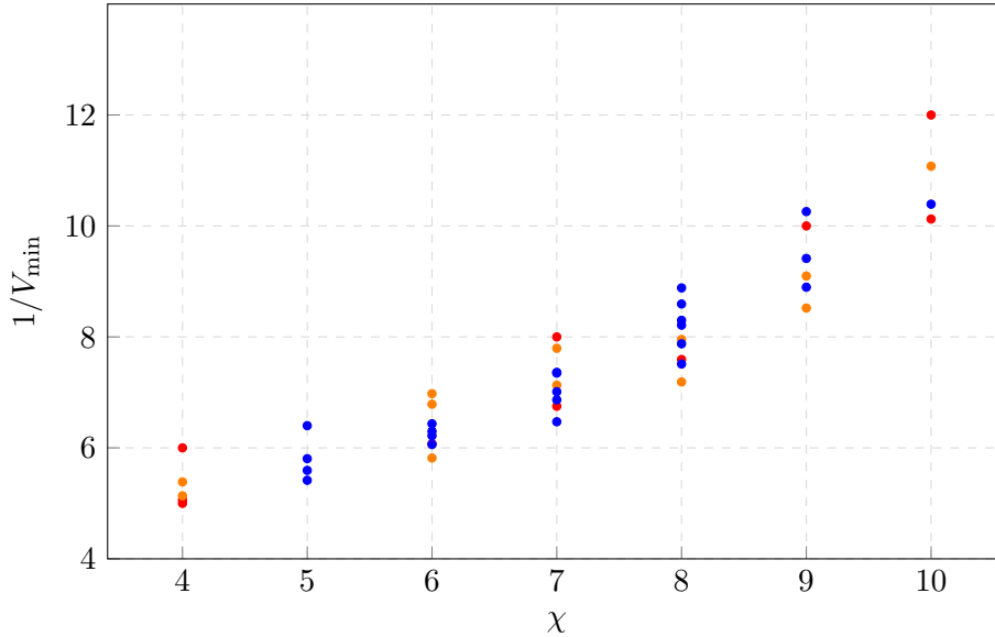
FIGURE A.1.1: The red points correspond to regular Sasaki-Einstein manifolds while the quasi-regular ones are in orange. We omit the first-grade points in the plot.
