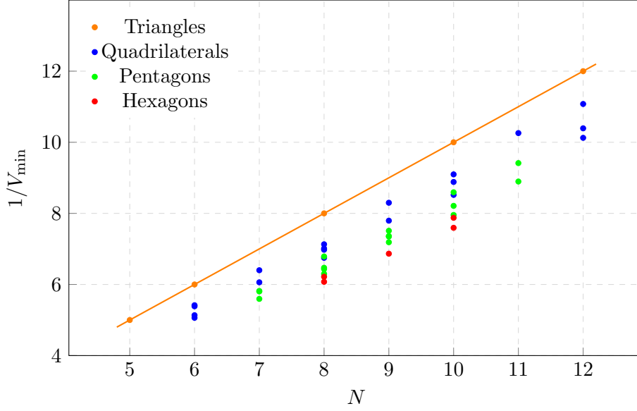
FIGURE 2.3.2: The reciprocals of minimized volumes against the number of lattice points N . This is bounded by the straight line 1/V_{\min} = N where the triangles live.
