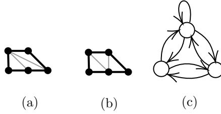
FIGURE F.1.1: The toric diagram with two different triangulations is shown in (a), (b). They give the same quiver as in (c). In the crystals, (a) has the initial atom corresponding to the node with an adjoint while (b) has the initial atom corresponding to one of the nodes without adjoints.
