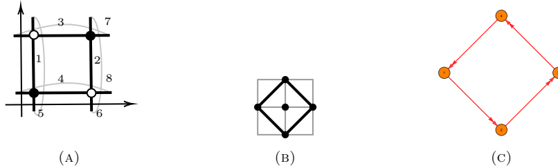
FIGURE 3.1.1: (a) The dimer model. (b) The toric diagram. (c) The quiver diagram.
