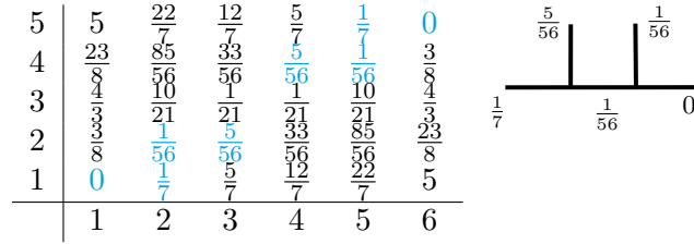
FIGURE C.2.4: The CB on the right has conformal dimensions coloured cyan in the Kac table.
