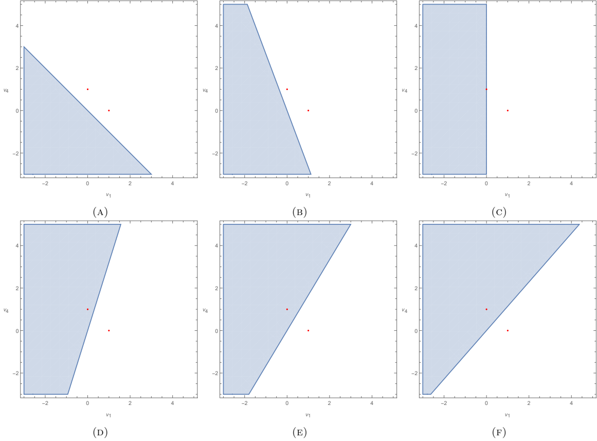
FIGURE 6.1.1: The region plot in v_i -space for w^2 + x^2 + y^2 + z^{n+1} = 0 at n = 1, \dots, 6 shown in (a)~(f) respectively. The red points correspond to the two test symmetries and the blue area is the region where F < 0 in each picture. A red point inside the blue region indicates that the ring is unstable.
