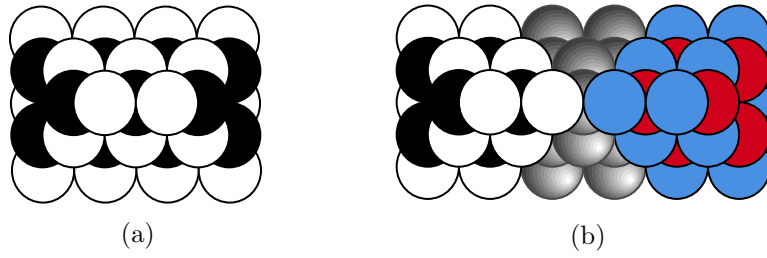
FIGURE 5.1.3: (a) The crystal for C_1 for the conifold \mathcal{C} . (b) “Merging” two such copies. Here, we still stay in the case \mathcal{C} , but with a different chamber. Each copy gives M(x)^2 \widetilde{M}_\Lambda(2)^{-1} where \widetilde{M}_\Lambda(2) := M(\prod q_i, x) M_\Lambda(\prod q_i, x; 2) . After merging the shaded pyramid (where the colours are ignored), we reach the chamber C_3 with partition function M^2 \widetilde{M}_\Lambda(4)^{-1} with the blue (red) colour identified with the white (black) colour.
