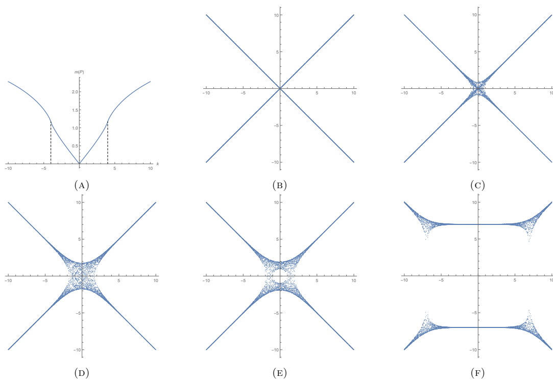
FIGURE B.0.1: The numerical m(P) along the Mahler flow in (a). The amoeba for P(z, w) when (b) k = 0 , (c) k = 3/4 , (d) k = k_{\text{iso}} = 4 , (e) k = 5 and (f) k = e^7 .
