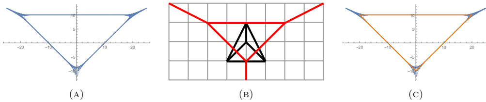
FIGURE 3.2.1: (a) The amoeba for the Newton polynomial P(z, w) = -w - z^{-1}w^{-1} - zw^{-1} - 2w^{-1} + k . As an example, we choose k = e^{10} . (b) The spine (in red) is the dual of the triangulated Newton polygon \Delta (in black). (c) The internal triangle in the spine is drawn explicitly in orange in the amoeba. In this example, we can see that the three vertices of the orange triangle are (20, 10) , (-20, 10) and (0, -10) respectively.
