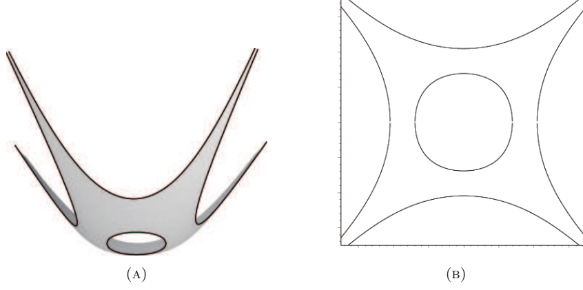
FIGURE 3.1.3: The Ronkin function (a) and the amoeba (b) of F_0 . Figures are taken from [139] (with slight modifications). The grey part in (a) gives the interior of amoeba in (b), which corresponds to the liquid phase. The hole in (a)/(b) is the gas phase. The unbounded white parts in (a) gives the unbounded complementary regions in (b). They correspond to solid phases.
