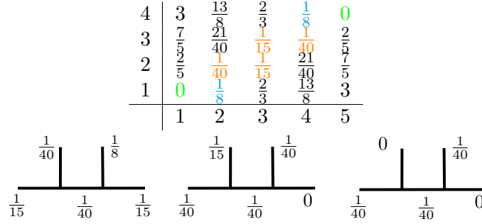
FIGURE C.2.3: The CBs from \Gamma(3) (cyan) and \Gamma_0(4) \cap \Gamma(2) (green) in the tetracritical Ising model. The ones in orange appear for both of the dessins. The three CBs, from left to right, come from \Gamma(3) , (+, +, -, -) and (-, +, -, +) in \Gamma_0(4) \cap \Gamma(2) respectively.
