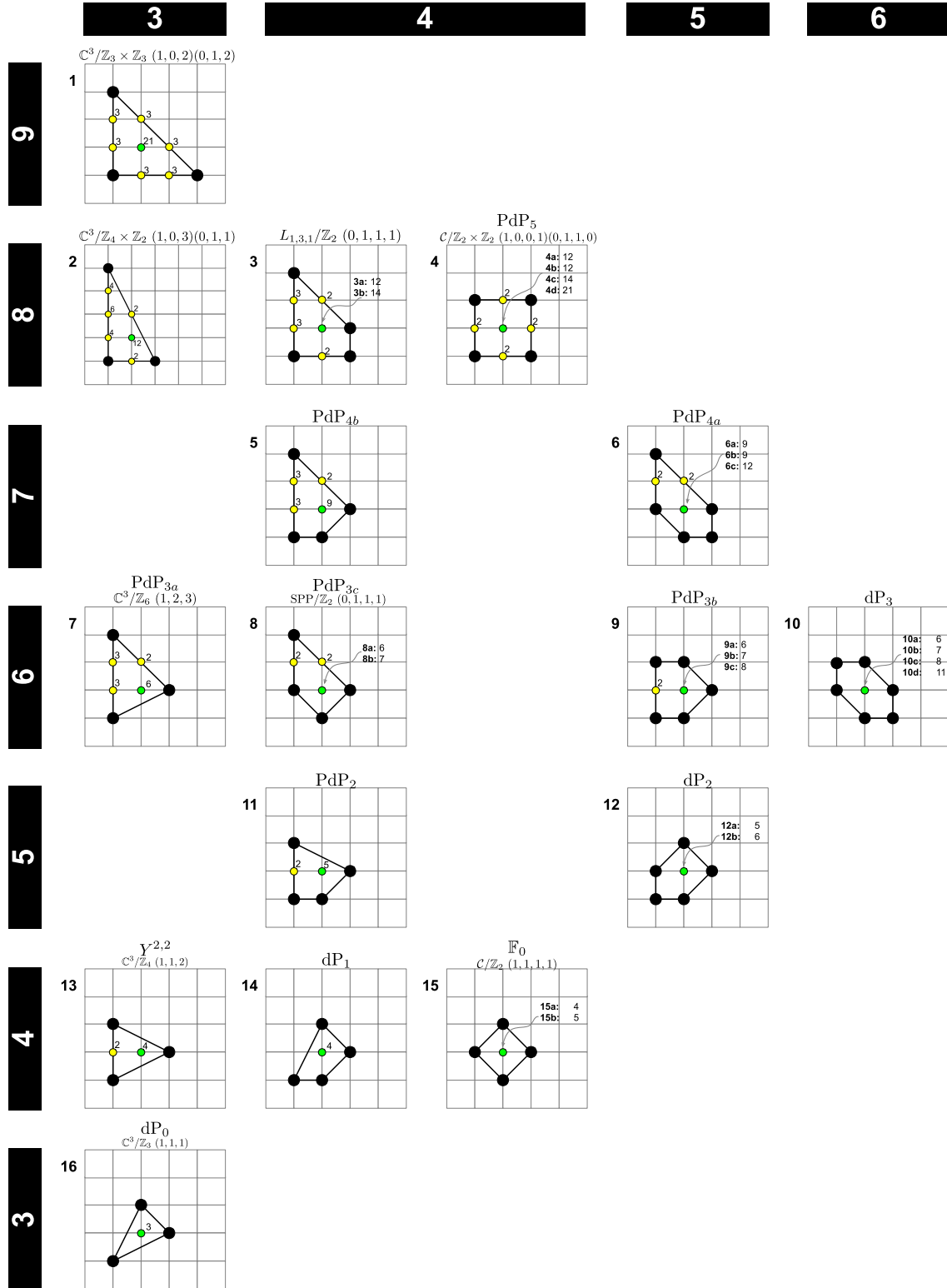
FIGURE 4.0.1: The 16 inequivalent reflexive polygons (up to \text{SL}(2, \mathbb{Z}) ). Figure taken from [105] (with slight modifications). The reflexive polygons are arranged such that the dual pairs are mirror symmetric with respect to the middle line (fourth row), and the four polygons in the middle line are therefore self-dual. In each row, the polygons have the same number of boundary points/(normalized) area. In each column, the polygons have the same number of vertices.
