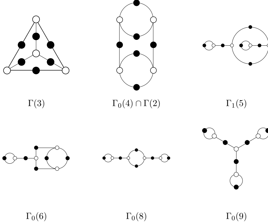
FIGURE C.1.1: The dessins d'enfants associated to the six Strebel points of the SU(2) , N_f = 4 theory.
