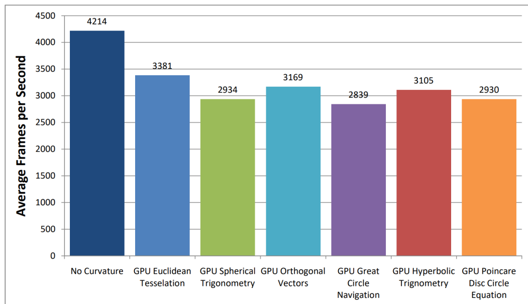
Figure 8.5: Average FPS values of GPU approaches (and non-curved baseline) from a test with progressively increasing number of shapes
