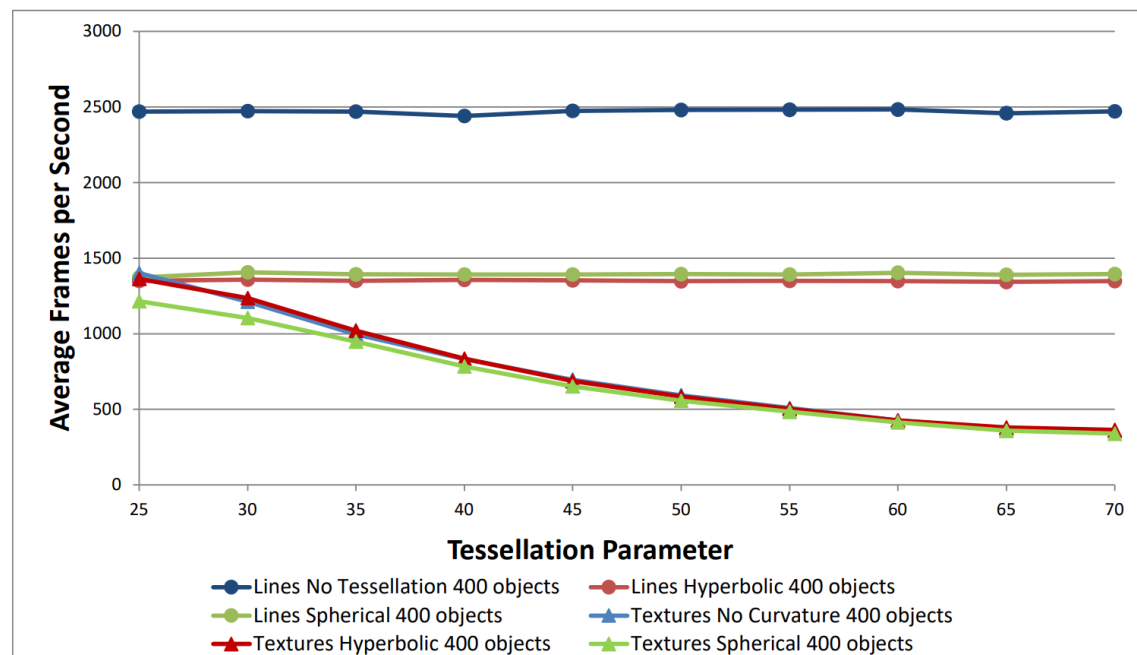
Figure 10.4: Performance test with 400 quadrilateral objects rendered with increasing tessellation parameter.
