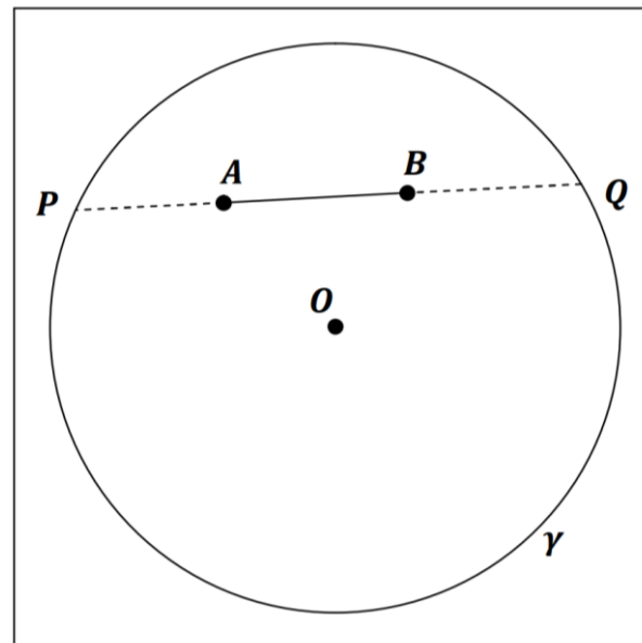
Figure 2.3: Hyperbolic plane in the Beltrami-Klein model. Disk \gamma with an origin O ; P, Q , ideal points; \overline{PQ} , hyperbolic line; A, B \in \overline{PQ} .
