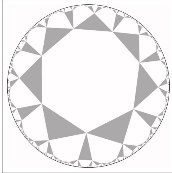
Figure 2.4: Quasiregular \mathbf{r}\{7, 3\} tiling of the hyperbolic plane in the Beltrami-Klein model. Heptagons and triangles are alternated to tile the plane. Rendered using KaleidoTile software (Weeks, KaleidoTile, 2020).
