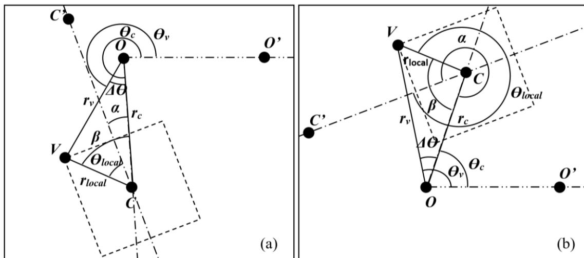
Figure 4.3: Finding the coordinates of an object's vertex V(\mathbf{r}_p, \theta_p) from a triangle \triangle OCV .
