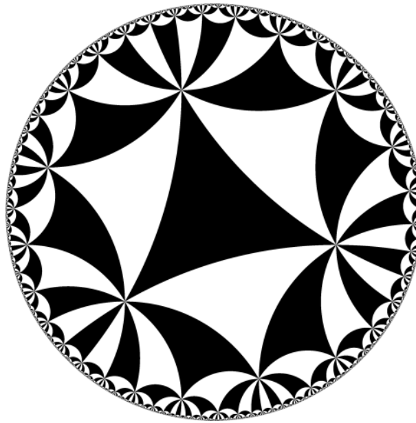
Figure 1.3: Poincaré disc with hyperbolic equilateral triangle tiling. Straight lines in this projection are represented as arcs of circles perpendicular to the disc's boundary. Triangles tiling the plane are identical on the hyperbolic plane, but appear exponentially smaller towards the boundary of the projection disc.
