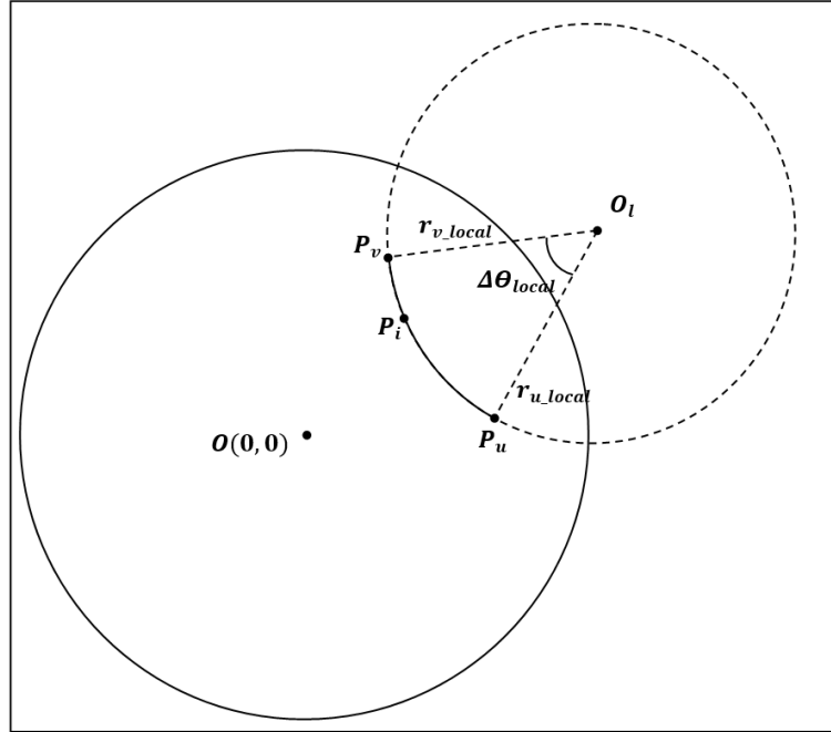
Figure 6.3: Using the Poincaré disc projection to find points between P_v(x_v, y_v) and P_u(x_u, y_u) lying on a geodesic. O(0, 0) , origin of the Cartesian Poincaré coordinate system; O_l(x_l, y_l) , origin of the local polar coordinate system; P_v(r_{v\_local}, \theta_{v\_local}) and P_u(r_{u\_local}, \theta_{u\_local}) . \Delta\theta_{local} = \theta_{v\_local} - \theta_{u\_local}
