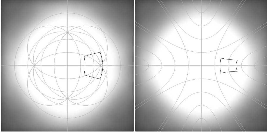
Figure 4.6: A regular quadrilateral with the centre at position (200 px, 0 rad) and rotation of 0 rad . Rendered with spherical trigonometry (left) and hyperbolic trigonometry (right). The white circle has the radius of 500 px .
