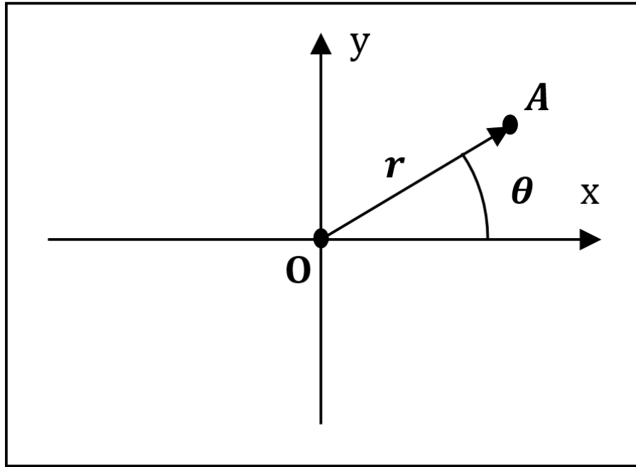
Figure 3.8: Position of a point A in polar coordinates. It has distance r and bearing \theta from the reference point O .
