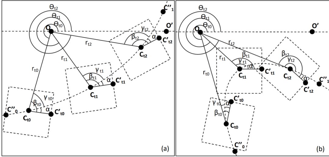
Figure 5.1: Movement of the object along a geodesic in Spherical (a) and Hyperbolic (b) space. Orientation with respect to the geodesic (angle \alpha ) is kept constant if the object is not rotating. O(0, 0) , reference point of the global coordinate system with; C_{tx}(r_{tx}, \theta_{tx}) , position of the object at time x ; \beta_{tx} , object's rotation angle at time x ; \gamma_{tx} , object's velocity vector direction at time x .
