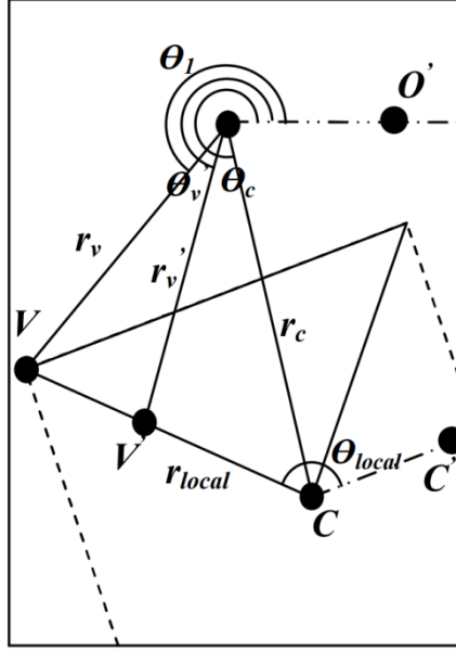
Figure 9.3: Finding an intermediate vertex V'(r'_v, \theta'_v) along the line \overline{VC} . O(0, 0) , reference point of the global coordinate system; OO' , reference direction of the global coordinate system; C(r_c, \theta_c) , object's position and reference point of local coordinate system; CC' , reference direction of local coordinate system; V(r_v, \theta_v) , object's vertex with local coordinates V(r_{local}, \theta_{local}) ; \overline{OV} = r_v ; \overline{OV'} = r'_v ; \overline{CV} = r_{local} ; \overline{OC} = r_c ; \angle VOO' = \theta_v ; \angle V'OO' = \theta'_v ; \angle COO' = \theta_c ; \angle VCC' = \theta_{local}
