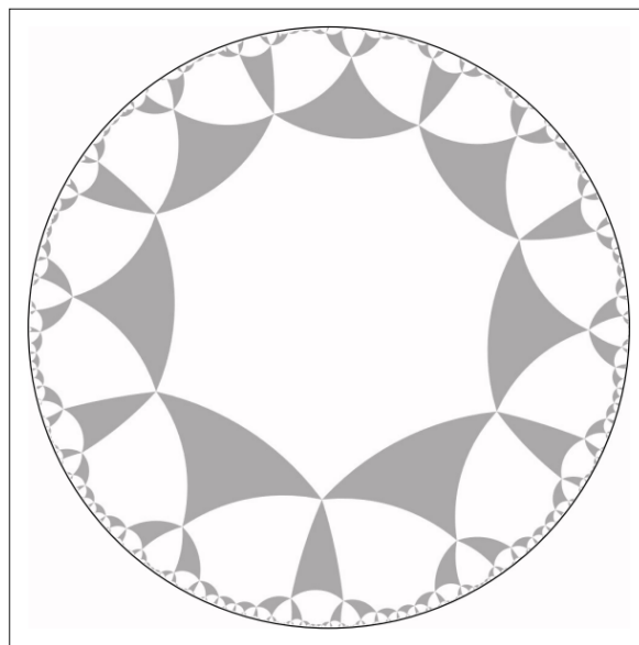
Figure 2.7: Quasiregular (3, 3, 7) tiling of the hyperbolic plane in the Poincaré Disc model. Heptagons and triangles are alternated to tile the plane. Rendered using KaleidoTile software (Weeks, KaleidoTile, 2020).
