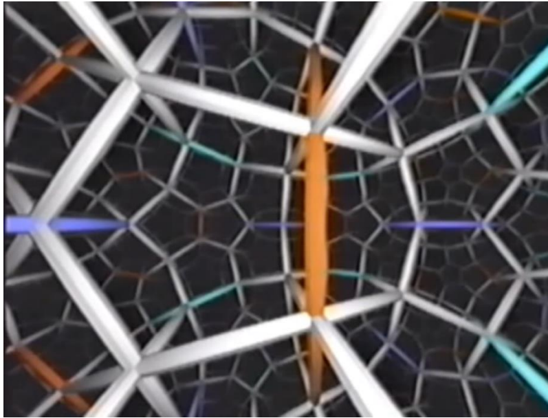
Figure 2.10: 3D hyperbolic space tiling with regular dodecahedra. Frame taken from a video “Not Knot” by the Geometry Center (Gunn, Epstein, & Maxwell, 1991).
