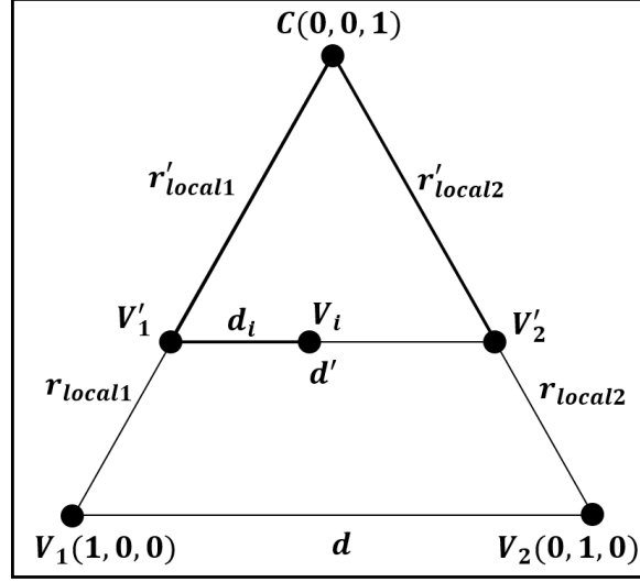
Figure 9.6: Tessellation of a triangle patch and barycentric coordinates of a triangle.
