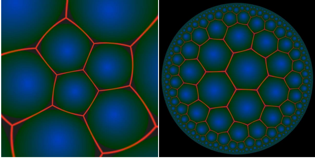
Figure 2.16: Stereographic projection of a sphere (left) and hyperbolic plane (right); from a video by David Madore (Madore, Visualizing the sphere and the hyperbolic plane: five projections of each , 2013).
