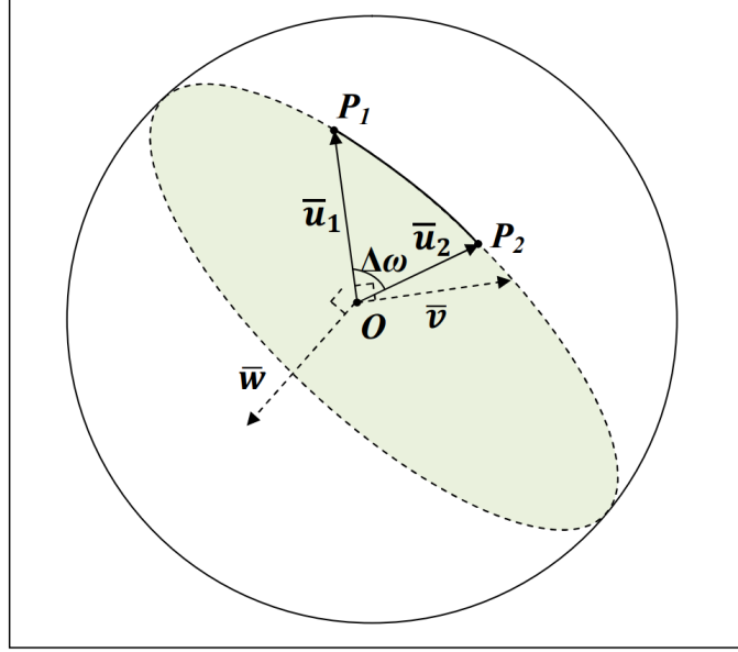
Figure 6.2: Finding the orthogonal vectors lying on the plane of a great circle given points P_1(x_1, y_1, z_1) and P_2(x_2, y_2, z_2) which passes through O(0, 0, 0) , origin of the Cartesian coordinate system; \bar{u}_1 = \overline{OP_1} ; \bar{u}_2 = \overline{OP_2} ; \bar{v}, \bar{u}_1, \bar{u}_2 \in \overline{OP_1P_2} ; \bar{w} \perp \overline{OP_1P_2} ; \bar{v} \perp \bar{u}_1 ; \Delta\omega = \angle P_1OP_2
