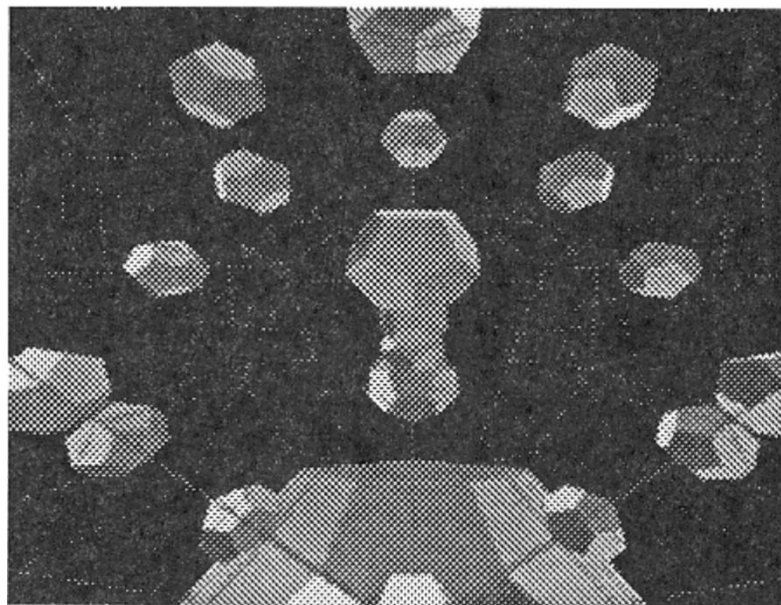
Figure 2.15: Dodecahedral tessellation of spherical 3-space. Rendering taken from an article by Hudson et al. (Hudson, Gunn, Francis, Sandin, & DeFanti, 1995).
