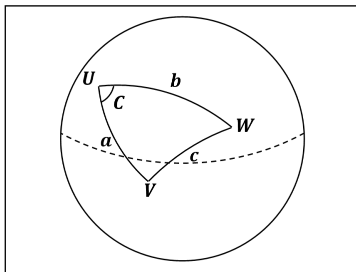
Figure 4.1: Spherical triangle with vertices U , V and W on the surface of a sphere; \overline{UV} = a ;
