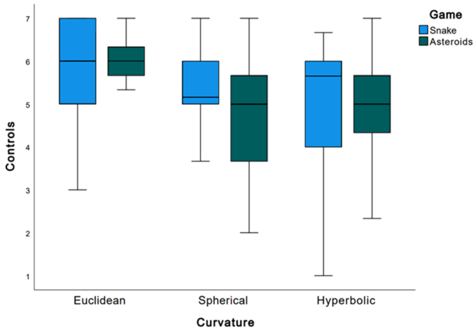
Figure 11.17: Box plot comparing data for the Controls dimension between Snake and Asteroids in Euclidean (left), spherical (centre) and hyperbolic (right) space.
