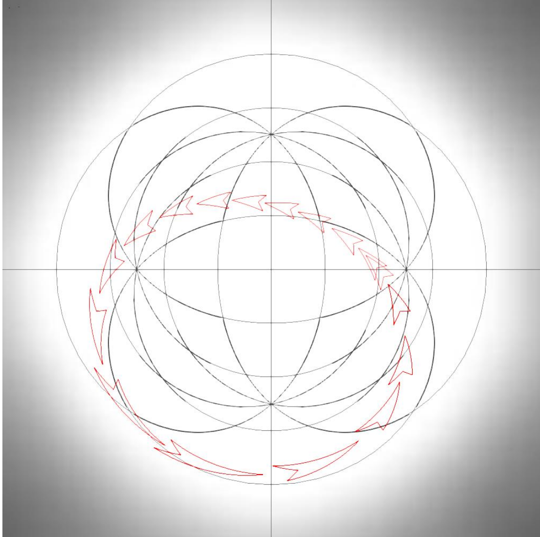
Figure 5.3: Object's movement in spherical space along the geodesic passing through the point (200 px, 0 rad) at \frac{\pi}{4} rad angle. The white circle has the radius of 500 px.
