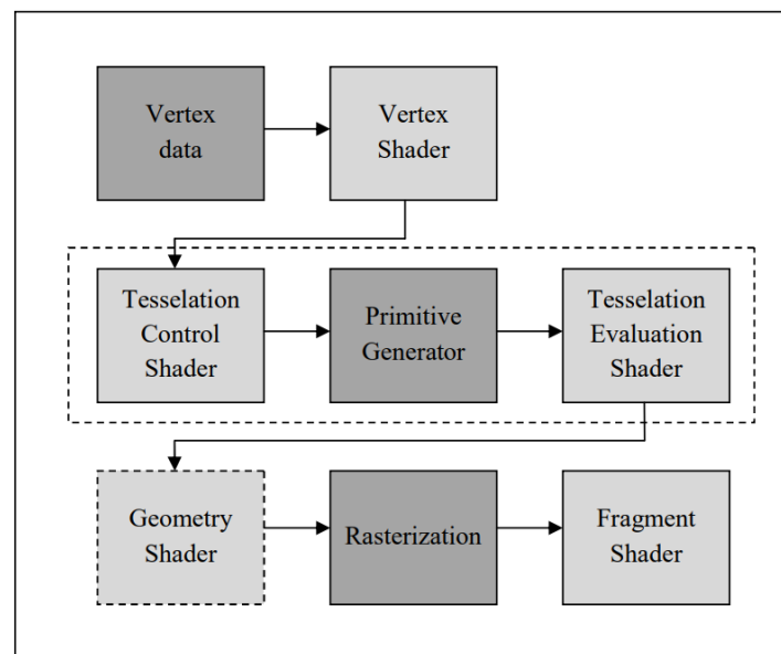
Figure 7.1: GLSL shader Pipeline. Allows for a direct control over 5 steps of the pipeline (shaded light grey). Vertex, Tessellation Control and Tessellation Evaluation shaders have been used for the project. Modifiable steps are shaded light grey, while non-modifiable are shaded dark grey. Optional steps in the pipeline are shaded light grey.
