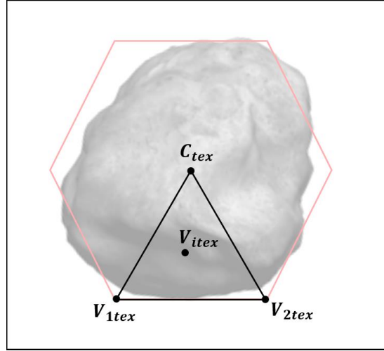
Figure 9.7: Triangle patch overlaid onto the texture file. V_{itex} , V_{1tex} , V_{2tex} , C_{tex} texture coordinates of points V_i , V_1 , V_2 , C respectively.
