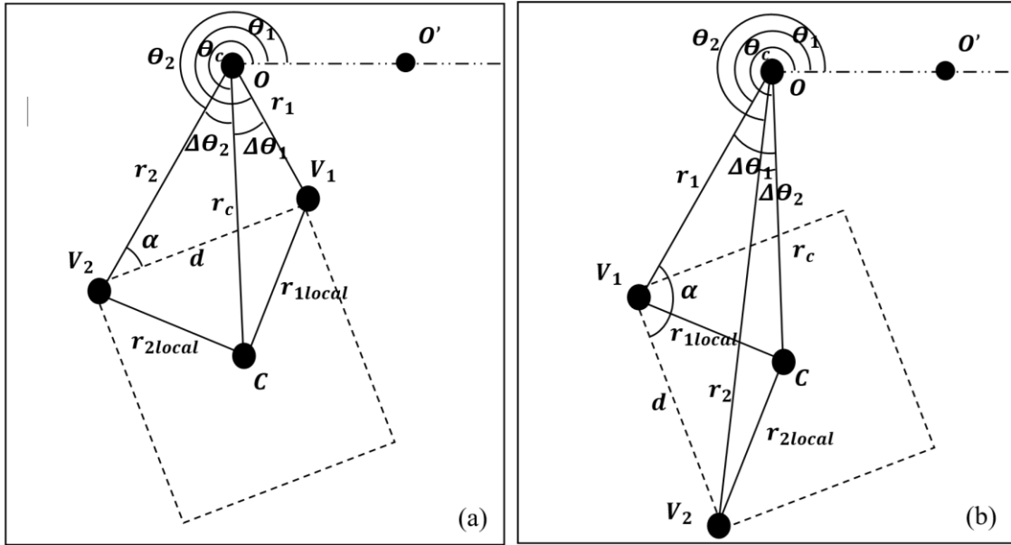
Figure 4.4: Finding preliminaries ( d , length of the edge \overline{V_1V_2} ; \Delta\theta , angle between \overline{OV_1} and \overline{OV_2} ) to calculate intermediate points on the edge \overline{V_1V_2} . Case (a): the angles \Delta\theta_1 and \Delta\theta_2 are diverging; case (b): the angles \Delta\theta_1 and \Delta\theta_2 are converging. O(0,0) , reference point of the global coordinate system; C(r_c, \theta_c) , position of the object; V_1(r_1, \theta_1) , V_2(r_2, \theta_2) , vertices of the object; \overline{OC} = r_c , \overline{OV_1} = r_1 , \overline{OV_2} = r_2 , \overline{CV_1} = r_{1local} , \overline{CV_2} = r_{2local} , \angle COO' = \theta_c , \angle V_1OO' = \theta_1 , \angle V_2OO' = \theta_2 , \angle V_1OC = \Delta\theta_1 , \angle V_2OC = \Delta\theta_2 , \angle OV_1V_2 = \alpha
