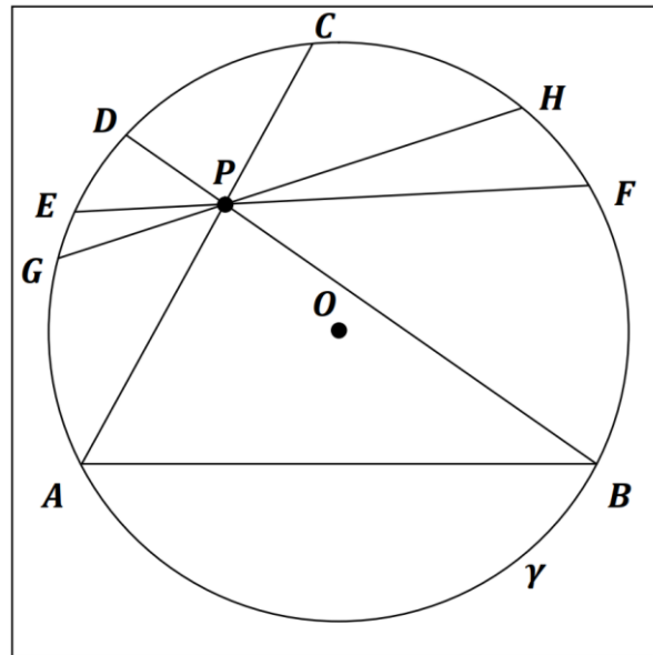
Figure 2.2: Hyperbolic plane in the Beltrami-Klein model. Disk \gamma with an origin O ; A, B, C, D, E, F, G, H , ideal points. Hyperbolic lines \overline{AC}, \overline{BD}, \overline{EF}, \overline{GH} through point P are parallel to \overline{AB}
