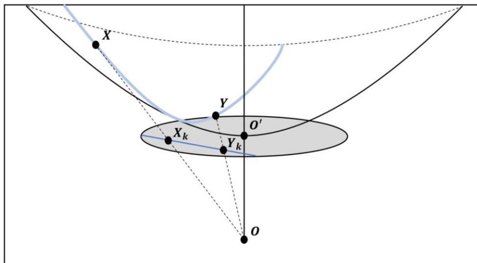
Figure 2.19: Gnomonic projection of a hyperboloid onto a unit Klein disc centred on the point O'(0, 1, 0) , which is also the lowest point of the hyperboloid. O(0, 0, 0) is the origin as well as the focal point of the gnomonic projection. Points X and Y lying on a line on the surface of the hyperboloid are projected to points X_k and Y_k on the Klein disc.
