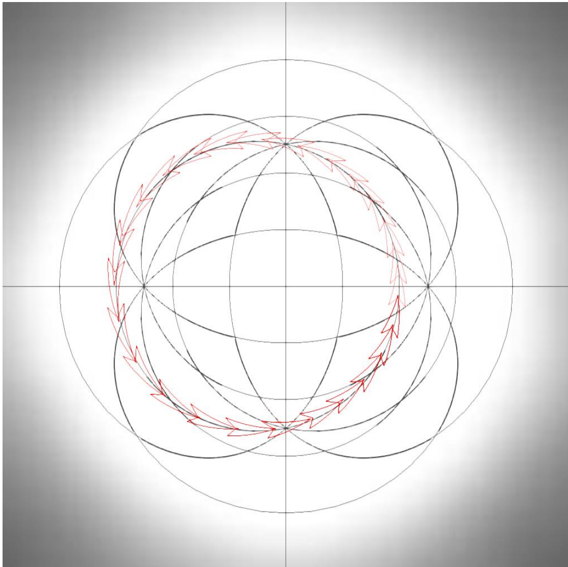
Figure 5.2: Object's movement in spherical space along the geodesic passing through the point (200 px, 0 rad) at \frac{\pi}{2} rad angle. The white circle has the radius of 500 px.
