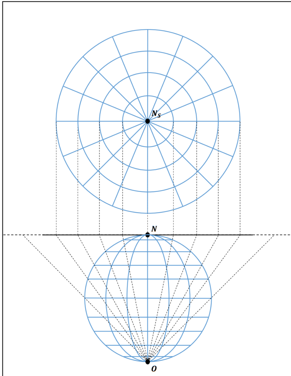
Figure 1.5: Stereographic projection of a globe onto a tangent plane. The globe is tangent to the plain at the North Pole, N , so it is chosen as the central point of the projection, N_s . The focal point of the projection, O , is located at the South Pole.
