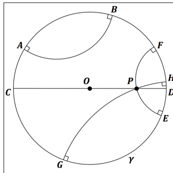
Figure 2.5: Hyperbolic plane in the Poincaré Disk model. Disk \gamma with an origin O ; A, B, C, D, E, F, G, H , ideal points; hyperbolic lines \overline{CD}, \overline{EF}, \overline{GH} through point P are parallel to \overline{AB} .
