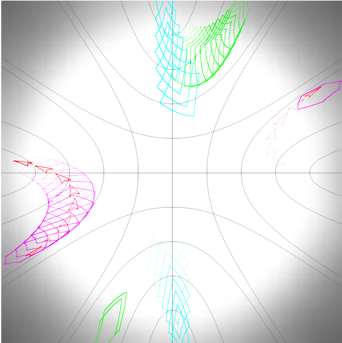
Figure 5.10: Time-lapse showing movement of multiple objects in hyperbolic space ( K = -1 ). A regular quadrilateral (cyan), a regular pentagon (green), a regular hexagon (magenta) and an arrow shape (red). The white circle has the radius of 500 px .
