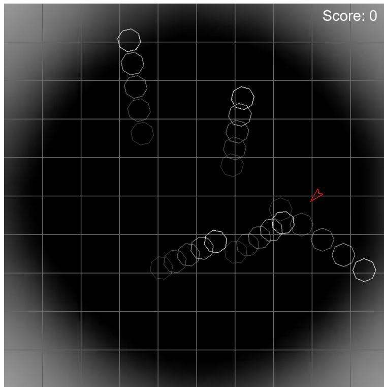
Figure 11.1: Time-lapse of the Asteroids game in Euclidean space rendered with the engine. 5 Asteroids move at different speed. The player's spaceship (red) remains stationary.
