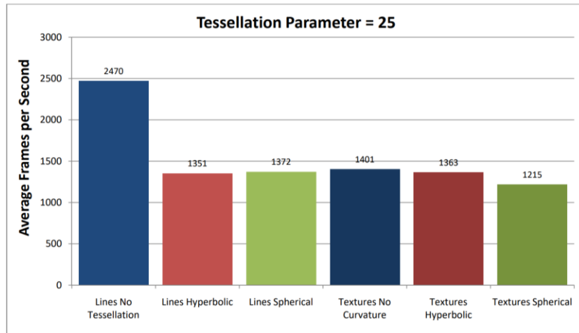
Figure 10.8: Average FPS values for the test with 400 shapes and tessellation parameter 25.
