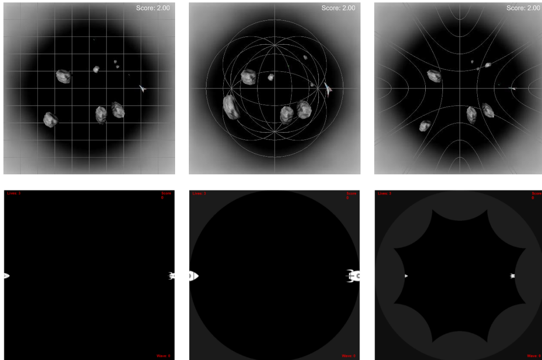
Figure 12.1: Comparison of adaptations of the Asteroids game rendered by this engine (top row) and Guimarães, et al. (bottom row) in Euclidean (left column), spherical (centre column) and hyperbolic (right column) space.
