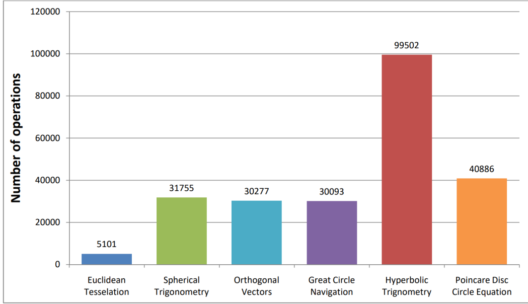
Figure 8.3: Theoretical number of operations for different approaches tessellating 1 shape with 4 vertices and a tessellation parameter of 150, based on CPU benchmarking of mathematical operations
