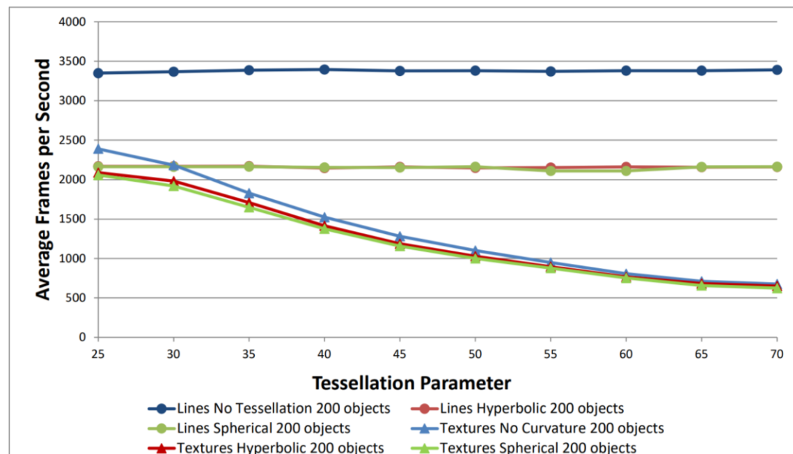
Figure 10.3: Performance test with 200 quadrilateral objects rendered with increasing tessellation parameter.
