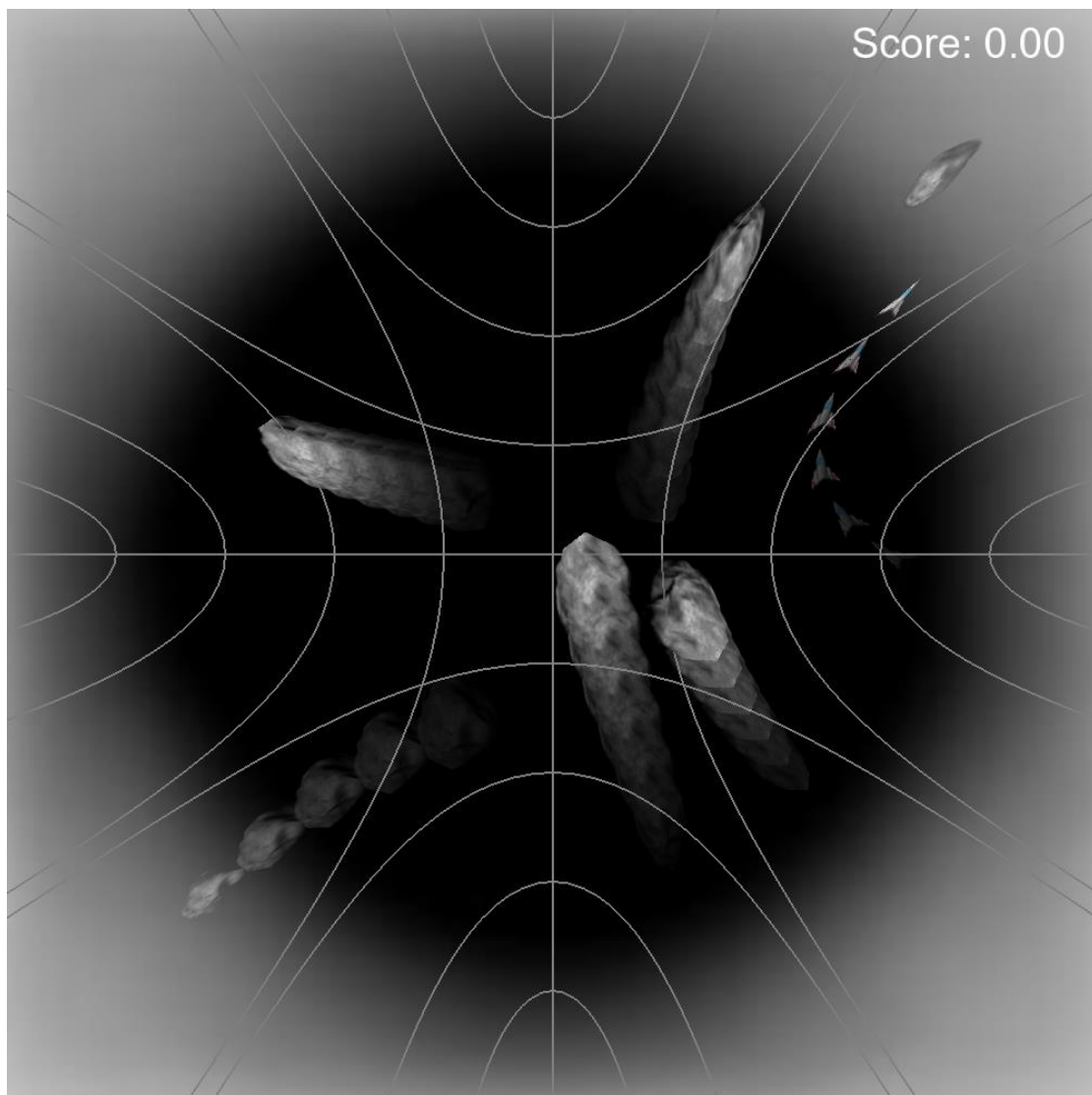
Figure 9.14: Time-lapse of multiple textured objects' (5 asteroids and a spaceship) movement through hyperbolic space within the Asteroids game simulation ( K = -1 ). This simulation is not the same playthrough as the one in Figure 9.10.
