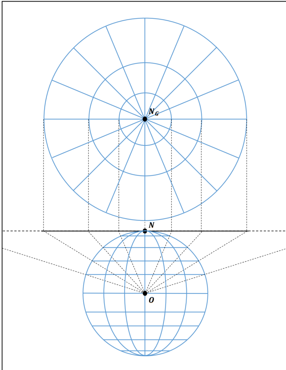
Figure 1.6: Gnomonic projection of a globe onto a tangent plane. The globe is tangent to the plane at the North Pole, N , so it is chosen as the central point of the projection, N_G . The focal point of the projection, O , is located at the centre of the globe.
