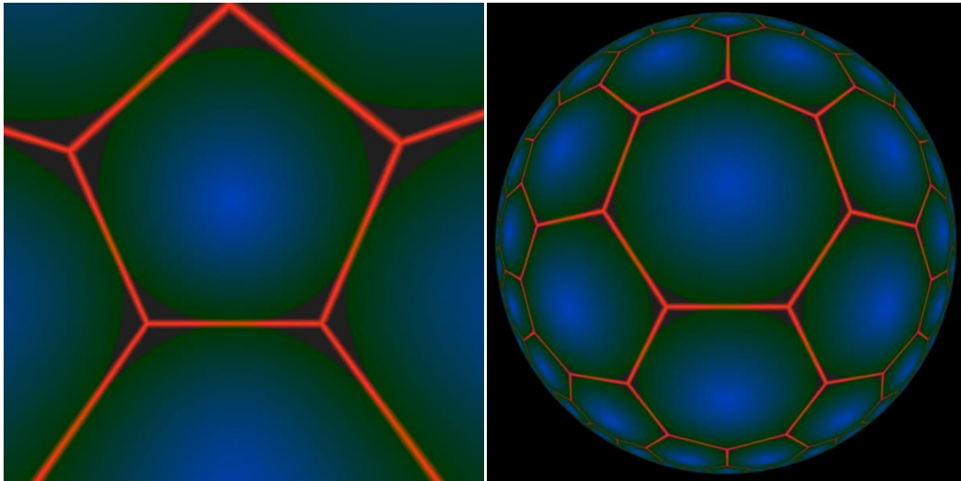
Figure 2.18: Gnomonic projection of a sphere (left) and hyperbolic plane (right); from a video by David Madore (Madore, Visualizing the sphere and the hyperbolic plane: five projections of each , 2013).
