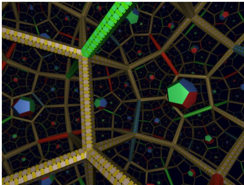
Figure 2.14: rendering of 3D hyperbolic space using jReality by Charles Gunn. It shows a tessellation of hyperbolic space by regular right-angled dodecahedra. Smaller dodecahedra are placed in the local centre of each larger dodecahedron (Gunn, 2010).
