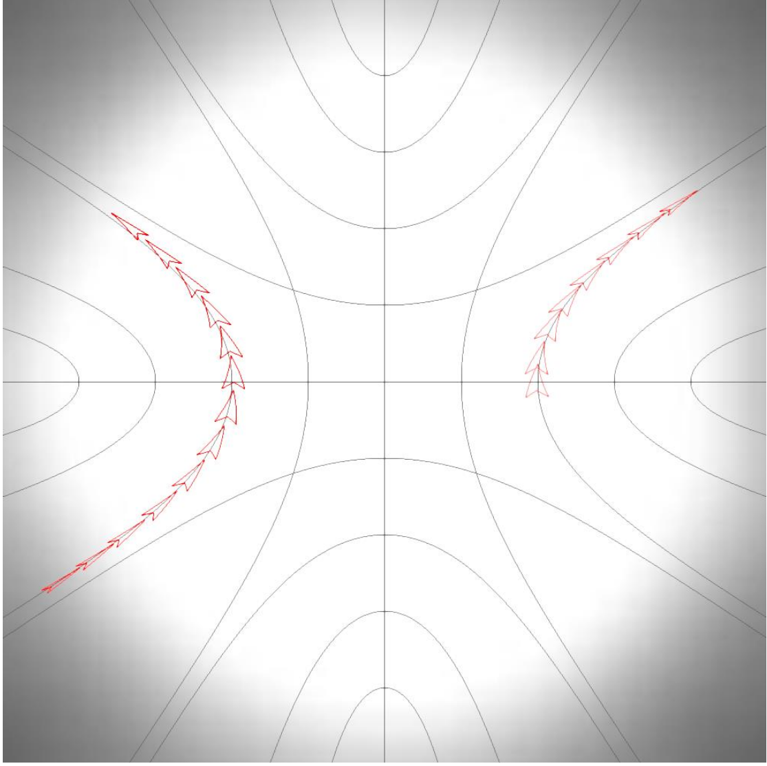
Figure 5.4: Object's movement in hyperbolic space along the geodesic passing through the point (200 \text{ px}, 0 \text{ rad}) at \frac{\pi}{2} \text{ rad} angle. The white circle has the radius of 500 \text{ px} .
