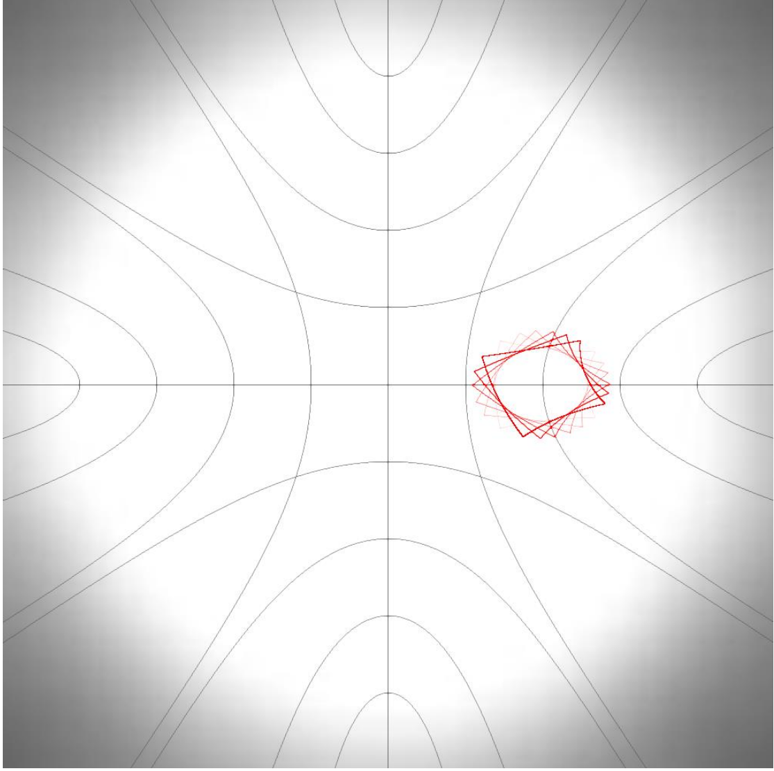
Figure 5.7: Time-lapse of the object's rotation around its centre point in hyperbolic space ( K = -1 ). The white circle has the radius of 500 px .
