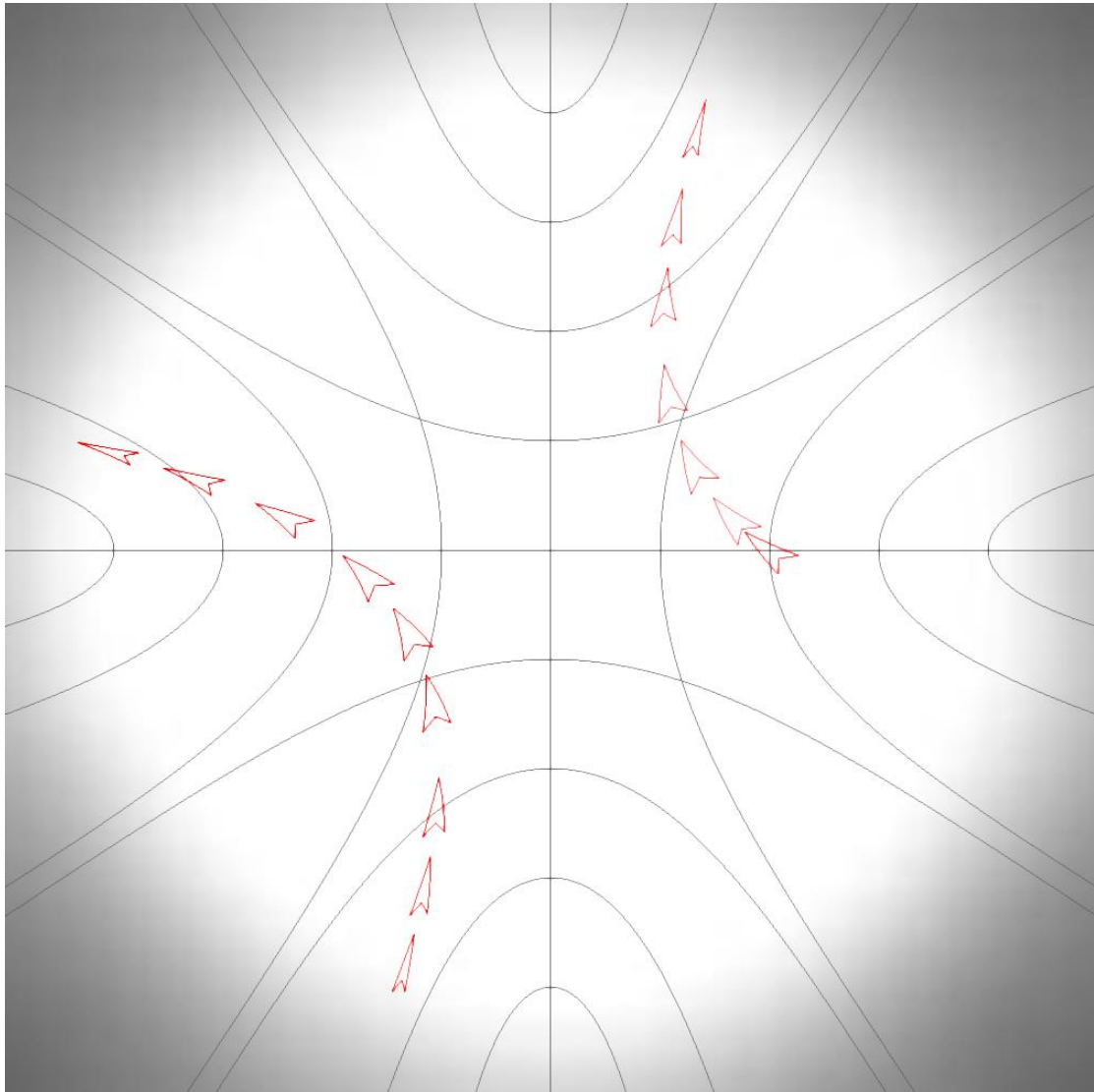
Figure 5.5: Object's movement in hyperbolic space along the geodesic passing through the point (200 px, 0 rad) at \frac{\pi}{4} rad angle. The white circle has the radius of 500 px.
