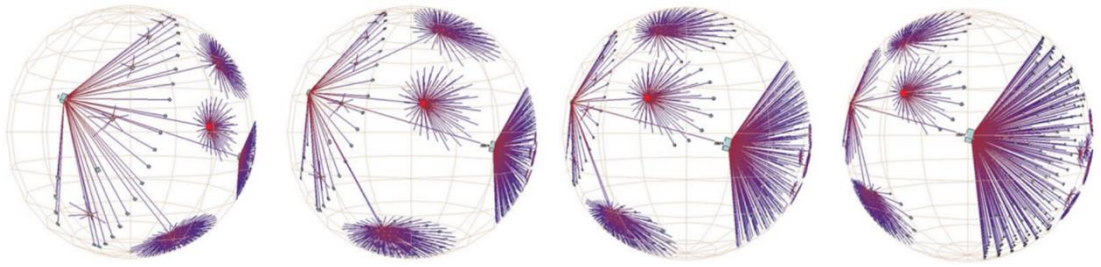
Figure 2.24: Hyperbolic motion over a 30,000-element Unix file system rendered with H3Viewer. Many nodes and edges project to subpixel areas and are not visible. Left to right, it shows translation of a node (cyan box in the figure) to the centre of the projection space (Munzner, 1998).
