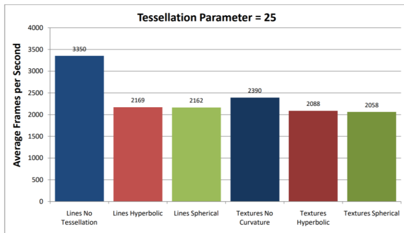
Figure 10.7: Average FPS values for the test with 200 shapes and tessellation parameter 25.
