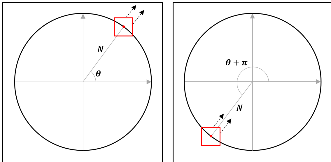
Figure 3.9: A quadrilateral object moves further than distance N away from the reference point and teleports to the antipodal point maintaining the orientation, velocity and rotation values.
