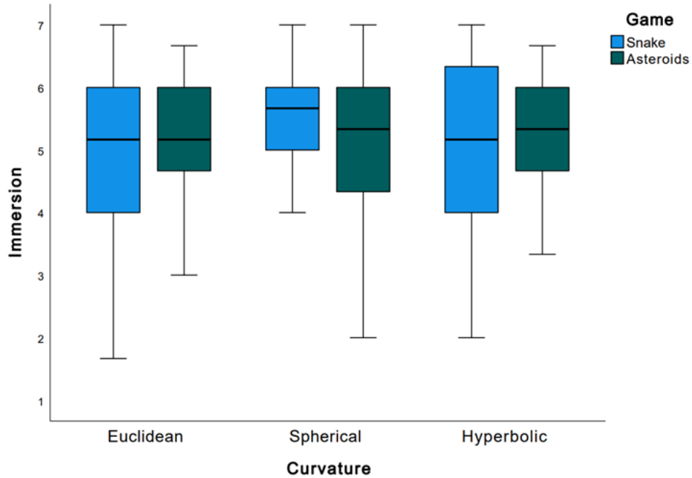
Figure 11.18: Box plot comparing data for the Immersion dimension between Snake and Asteroids in Euclidean (left), spherical (centre) and hyperbolic (right) space.
