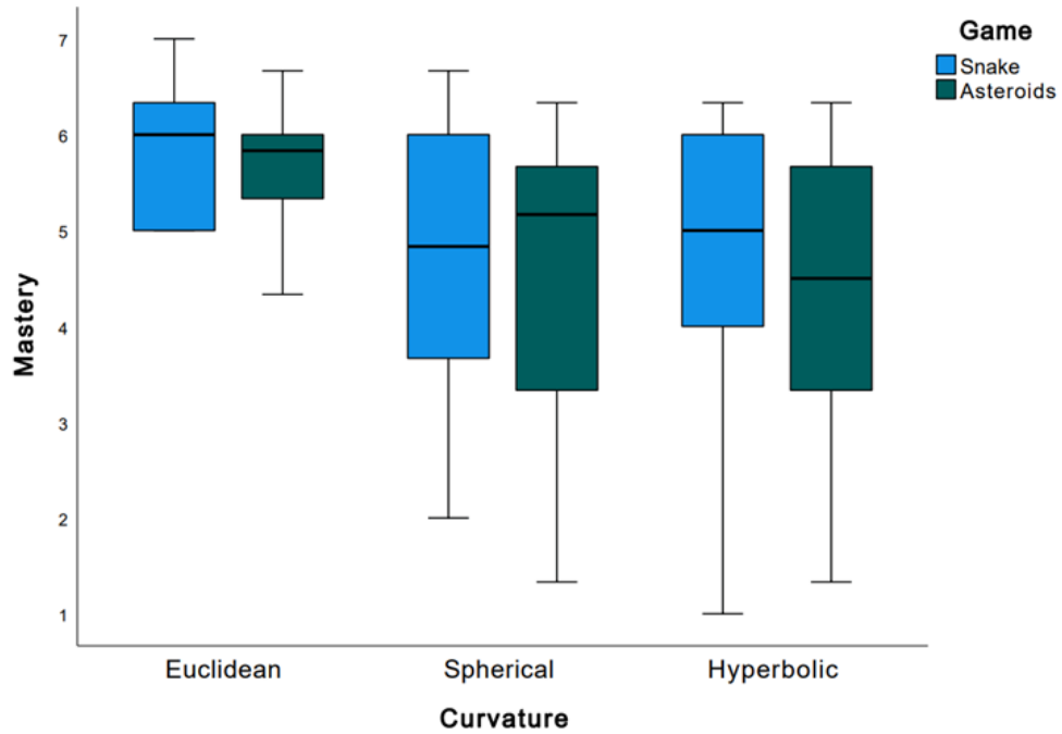
Figure 11.16: Box plot comparing data for the Mastery dimension between Snake and Asteroids in Euclidean (left), spherical (centre) and hyperbolic (right) space.
