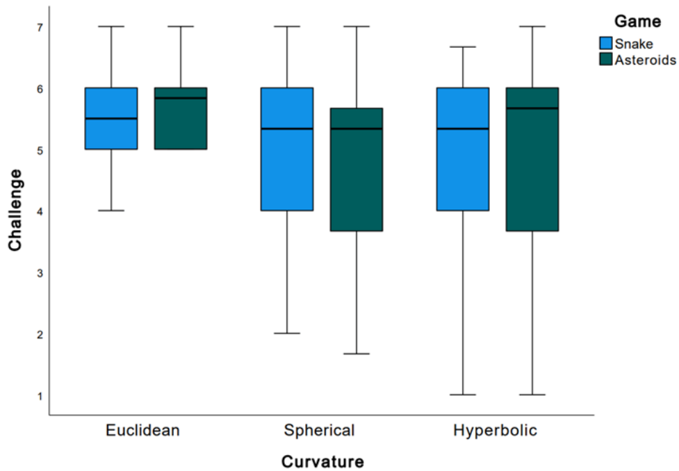
Figure 11.19: Box plot comparing data for the Challenge dimension between Snake and Asteroids in Euclidean (left), spherical (centre) and hyperbolic (right) space.
