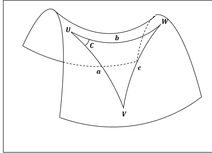
Figure 4.2: Hyperbolic triangle with vertices U , V and W on the surface of a hyperbolic plane;
