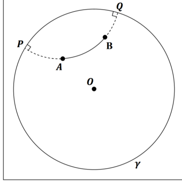
Figure 2.6: Hyperbolic plane in the Poincaré disk model. Disk \gamma with an origin O ; P, Q , ideal points; \overline{PQ} , hyperbolic line; A, B \subset \overline{PQ} .
