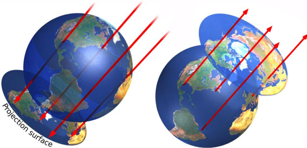
Figure 1.2: Orthographic projection of the sphere onto a tangent plane. Parallel rays are cast onto the surface (left) or from the surface (right) of a sphere; and the points are transferred onto the points of intersection of these rays with a tangent plane.
