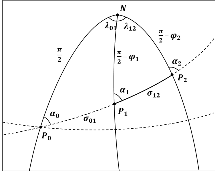
Figure 6.1: Great Circle Navigation. Finding waypoints along a great circle path between points P_1(\phi_1, \lambda_1) and P_2(\phi_2, \lambda_2) . N(\frac{\pi}{2}, 0) , North Pole of the latitude and longitude coordinate system; P_0(0, \lambda_0) , point of intersection of the great circle with equator geodesic; \alpha_0, \alpha_1, \alpha_2 , azimuths to the great circle path at points P_0, P_1, P_2 respectively; \sigma_{01} = \overline{P_0P_1} ; \sigma_{12} = \overline{P_1P_2} ; \lambda_{01} = \lambda_1 - \lambda_0 ; \lambda_{12} = \lambda_2 - \lambda_1
