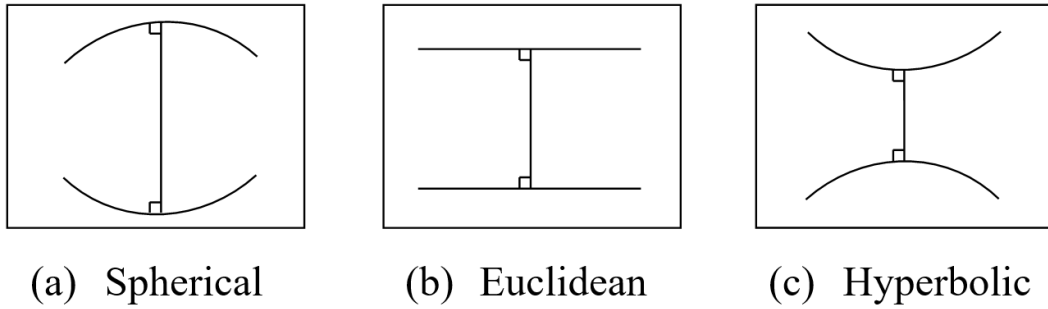
Figure 1.1: Comparison of parallel lines in the 2D spaces of different curvature
