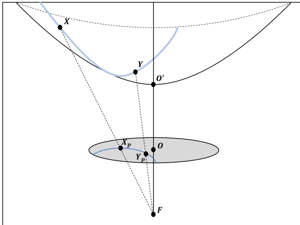
Figure 2.17: Stereographic projection of a hyperboloid onto a unit Poincaré disc centred on the origin O(0, 0, 0) . O'(0, 1, 0) is the lowest point of the hyperboloid. F(0, -1, 0) is the focal point of the stereographic projection. Points X and Y lying on a line on the surface of the hyperboloid are projected to points X_p and Y_p on the Poincaré disc.
