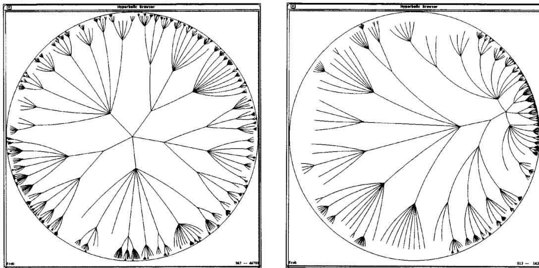
Figure 2.25: A large graph rendered with Hyperbolic Browser. The image on the right shows a transition, where the focus has moved to a node that was to the left and slightly below the origin in the left image (Lamping & Rao, 1996).
