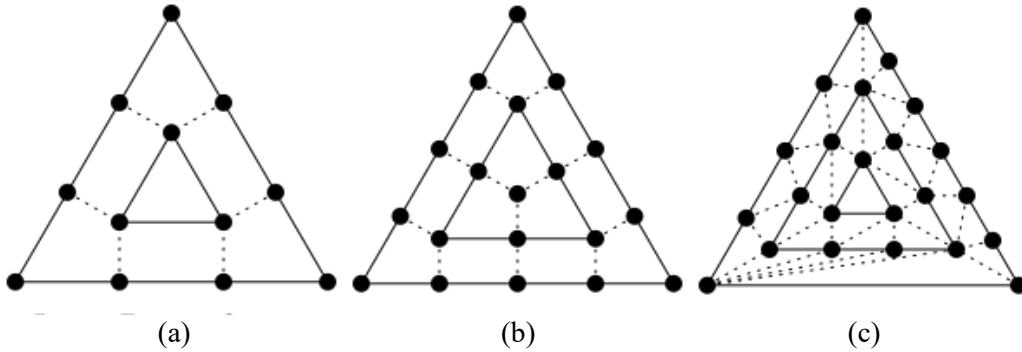
Figure 9.5: Tessellation of a triangle patch with different parameters of the inner and outer tessellation levels. (a) Inner tessellation levels 3, 3, 3 Outer tessellation level 3; (b) Inner tessellation levels 4, 4, 4 Outer tessellation level 4; (c) Inner tessellation levels 4, 1, 6 Outer tessellation level 5 (The Khronos Group, 2020).
