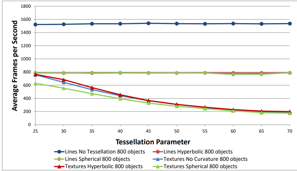
Figure 10.5: Performance test with 800 quadrilateral objects rendered with increasing tessellation parameter.
