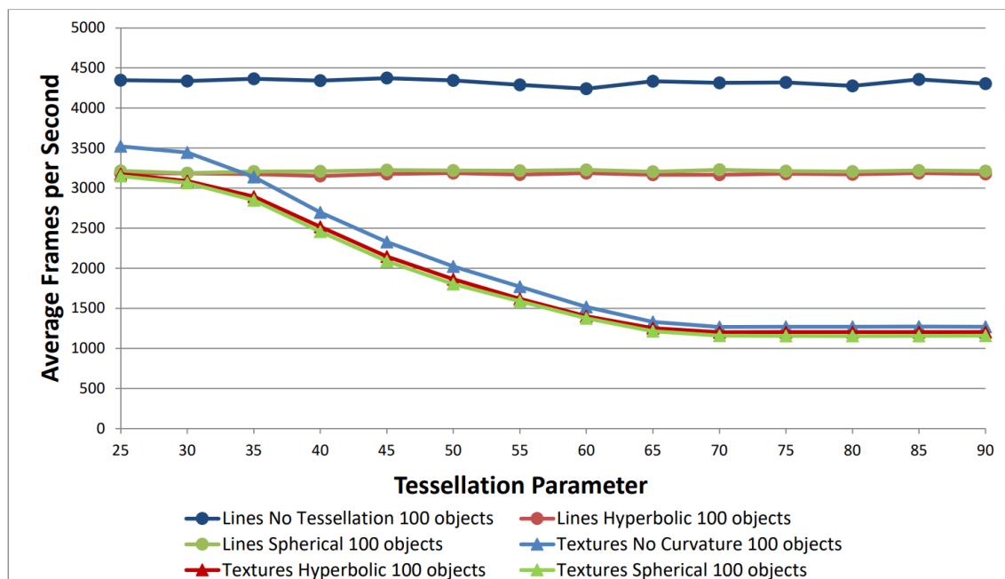
Figure 10.2: Performance test with 100 quadrilateral objects rendered with increasing tessellation parameter.
