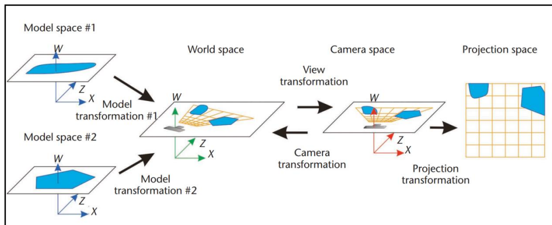
Figure 2.11: Four coordinate systems of standard rendering pipeline for 3D graphics, represented as a 3D hyperplane in 4D space and transformations connecting them represented as matrices (Weeks, 2002).
