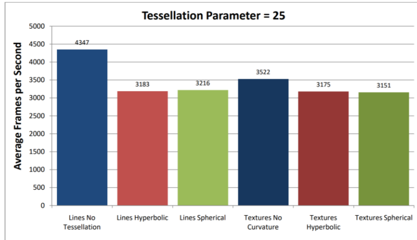
Figure 10.6: Average FPS values for the test with 100 shapes and tessellation parameter 25.
