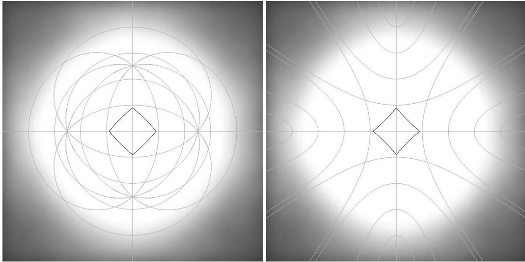
Figure 4.8: A regular quadrilateral with the centre at position (0 px, 0 rad) and rotation of \frac{\pi}{4} rad . Rendered with spherical trigonometry (left) and hyperbolic trigonometry (right). The white circle has the radius of 500 px .
