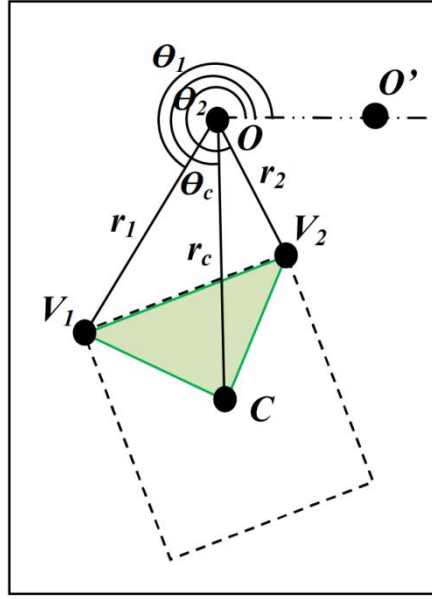
Figure 9.1: Texturing a shape by subdividing it into patches, one patch per edge. Patch V_1V_2C is highlighted. O(0, 0) , reference point of a polar coordinate system; V_1(r_1, \theta_1) , V_2(r_2, \theta_2) , vertices of the object; C(r_c, \theta_c) , object's position; \triangle , area of the shape rendered by the patch
