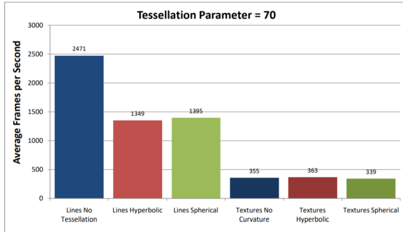
Figure 10.12: Average FPS values for the test with 400 shapes and tessellation parameter 70.
