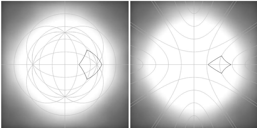
Figure 4.7: A regular quadrilateral with the centre at position (200 px, 0 rad) and rotation of \frac{\pi}{4} rad . Rendered with spherical trigonometry (left) and hyperbolic trigonometry (right). The white circle has the radius of 500 px .
