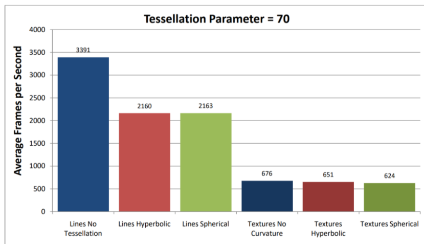
Figure 10.11: Average FPS values for the test with 200 shapes and tessellation parameter 70.
