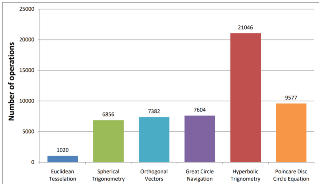
Figure 8.2: Theoretical number of operations for different approaches tessellating 1 shape with 4 vertices and a tessellation parameter of 30, based on CPU benchmarking of mathematical operations
