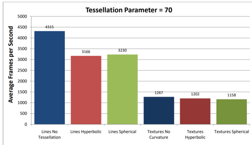
Figure 10.10: Average FPS values for the test with 100 shapes and tessellation parameter 70.
