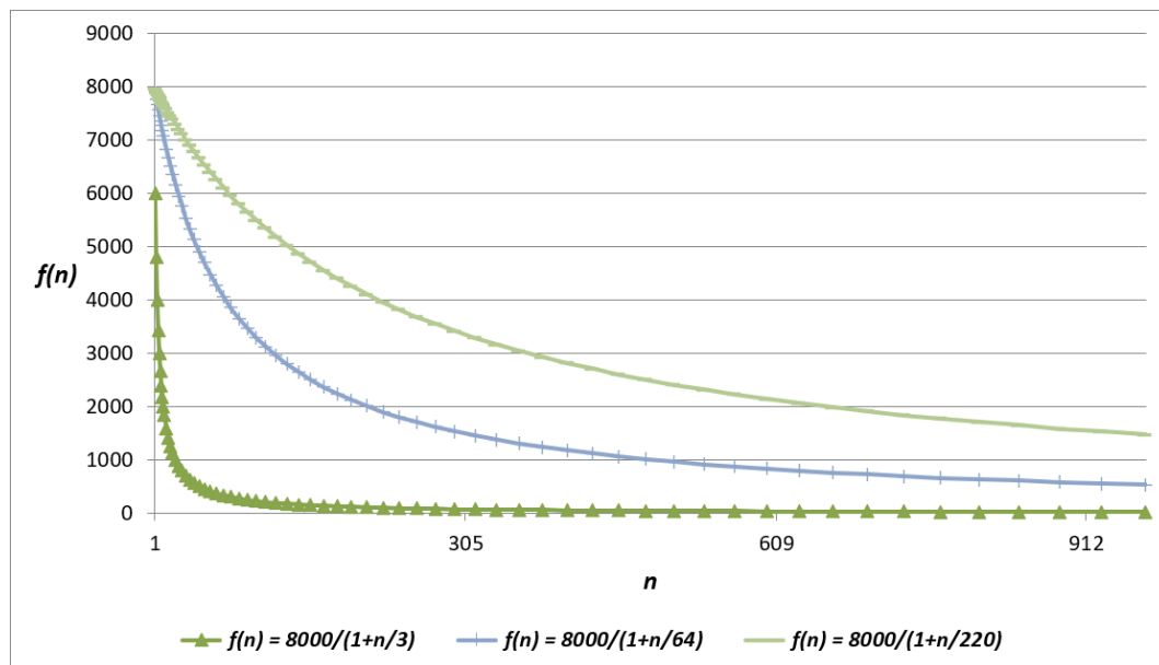
Figure 8.7: Number series of the general form f(n) = \frac{1}{n} scaled to approximately fit the shapes of graphs from Figure 8.6.
