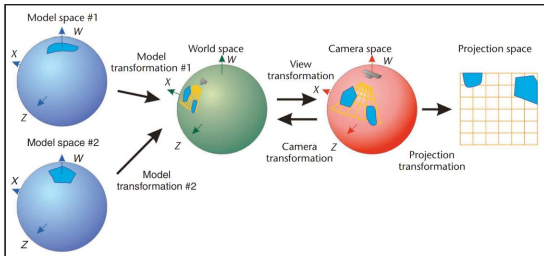
Figure 2.12: The rendering pipeline for a hypersphere (Weeks, 2002).
