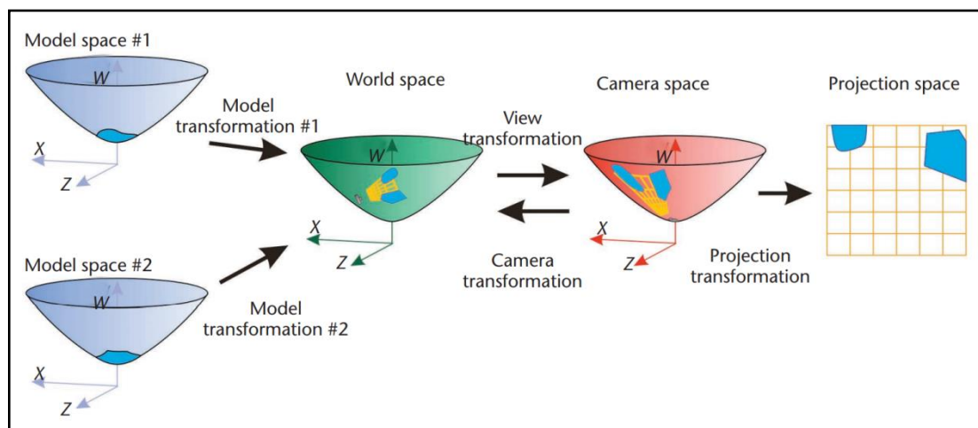
Figure 2.13: The rendering pipeline for a hyperbolic plane (Weeks, 2002).
