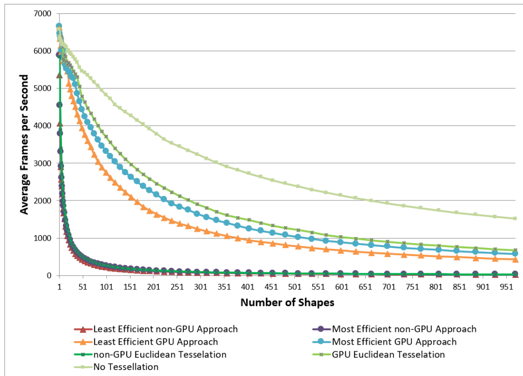
Figure 8.6: Line graph constructed from the data gathered in a test with a progressively increasing number of shapes from 1 to 1000. The graph only shows the best fitting lines for the most and the least efficient approaches for GPU and non-GPU rendering as well as three baseline tests: no tessellation, non-GPU Euclidean Tessellation and GPU Euclidean Tessellation.
