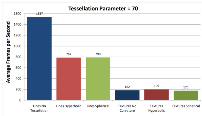
Figure 10.13: Average FPS values for the test with 800 shapes and tessellation parameter 70.
