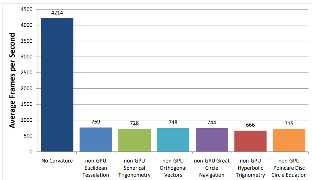
Figure 8.4: Average FPS values of non-GPU approaches (and non-curved baseline) from a test with progressively increasing number of shapes.
