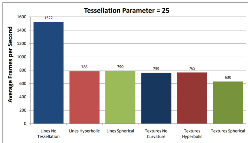
Figure 10.9: Average FPS values for the test with 800 shapes and tessellation parameter 25.
