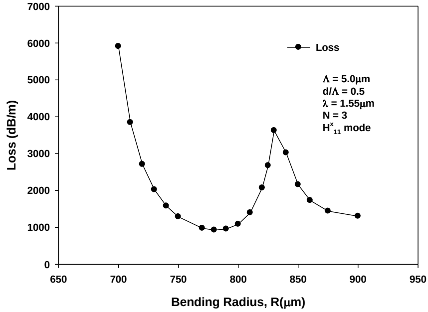
Fig. 4. 18: The variation of bending loss against bending radius, R , for values of R between 700\mu\text{m} to 900\mu\text{m} , when \Lambda = 5.0\mu\text{m} , d/\Lambda = 0.5 .
