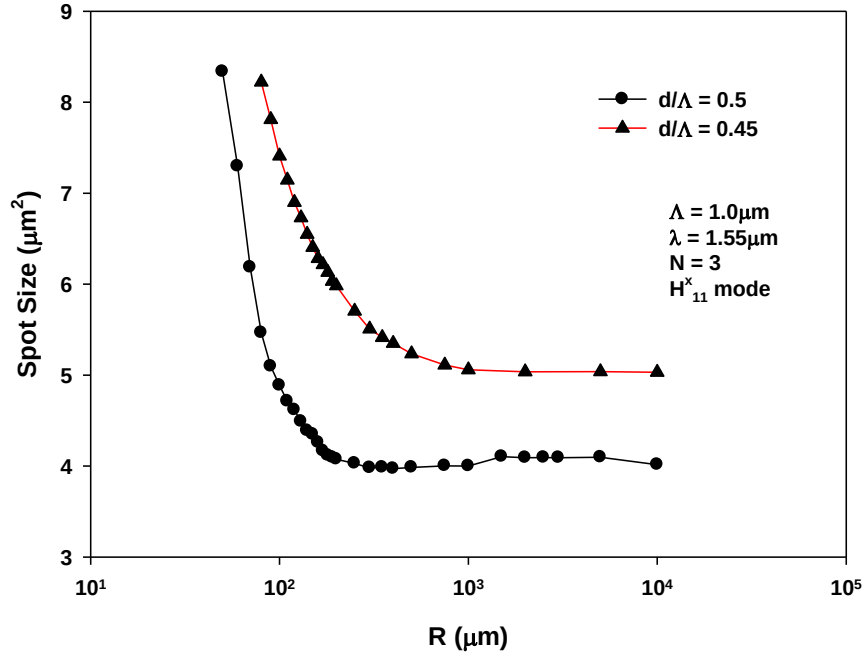
Fig. 4. 15: The variation of spot size with bending radius, R for \Lambda = 1.0 \mu\text{m} d/\Lambda = 0.5 and d/\Lambda = 0.45 .
