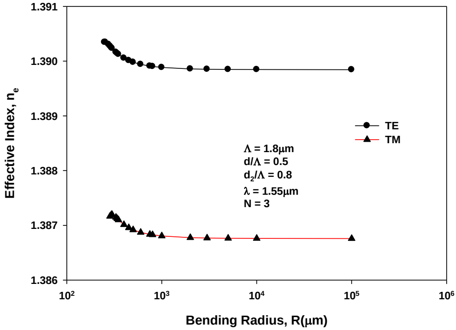
Fig. 5. 8: Variation of effective index with bending radius, R for \Lambda = 1.8\mu\text{m} , d/\Lambda = 0.5 , d_2/\Lambda = 0.8 for both quasi-TE and quasi-TM modes.
