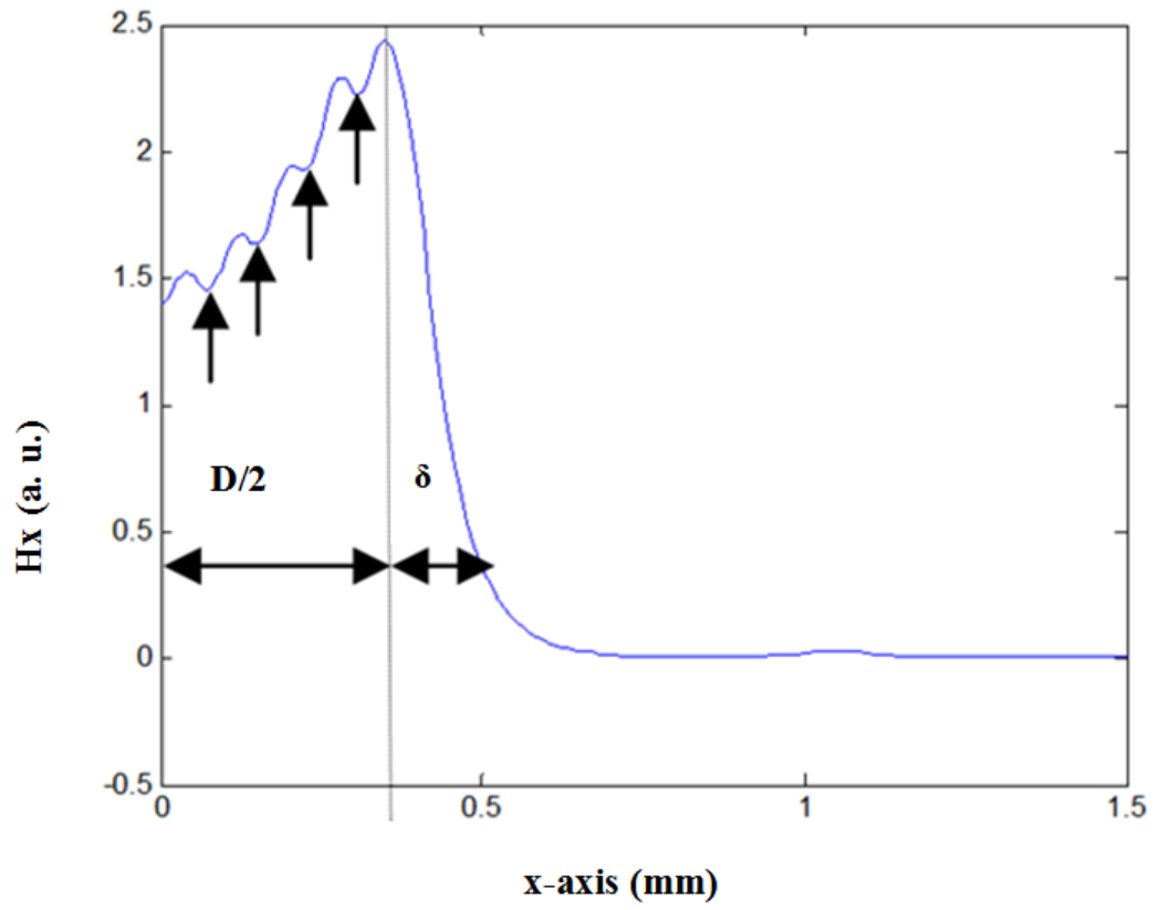
Fig. 7. 28: Variations of the H_x field of the H_{11}^x mode along the x-axis for \Lambda_0 = 0.7 mm.
