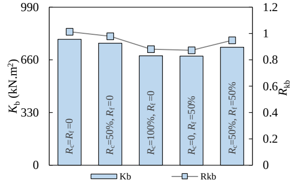
(b) K_b and R_{kb} of beams
