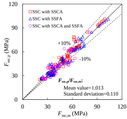
Fig. 14. Comparison between the predicted and measured compressive strength of the SSC.
