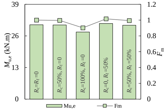
(b) M_{u,e} and F_m of beams
