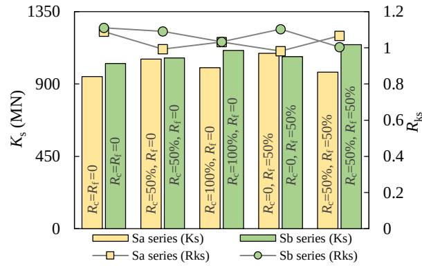
(a) K_s and R_{ks} of stub columns
