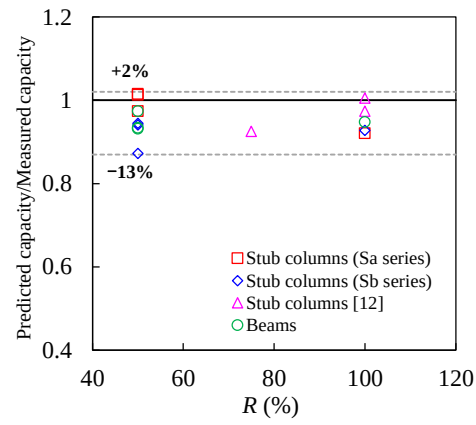
Fig. 17. The change in the ratio of predicted capacity to measured capacity of the SSC filled steel SHS specimens with respect to R .
