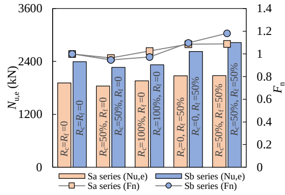
(a) N_{u,e} and F_n of stub columns
