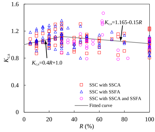
Fig. 13. Compressive strength index ( K_{c,s} ) of the SSC according to the experimental results.
