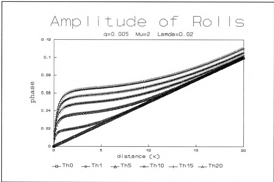
Fig. 4.59 : Numerical evolution for q=0.005 , \mu=2 and \lambda=0.02 showing the phase of x -rolls at successive times \tau
