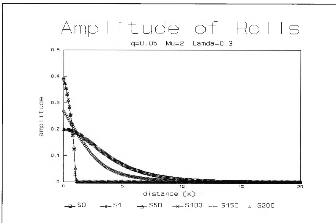
Fig. 4.18 : Numerical evolution for q=0.05 , \mu=2 and \lambda=0.3 showing the amplitude of y -rolls at successive times \tau
