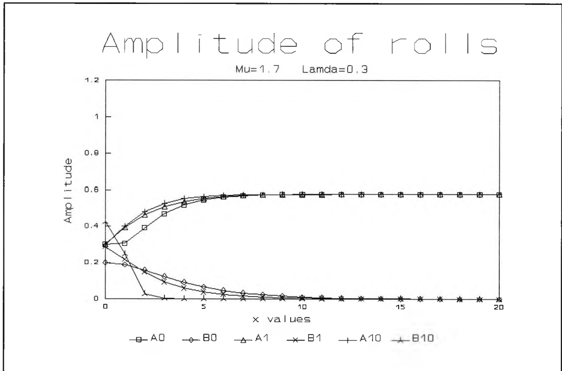
Fig. 2.10 : Numerical evolution for \mu=1.700 and \lambda=0.3 showing the amplitudes A and B of x -rolls and y -rolls at successive times \tau
