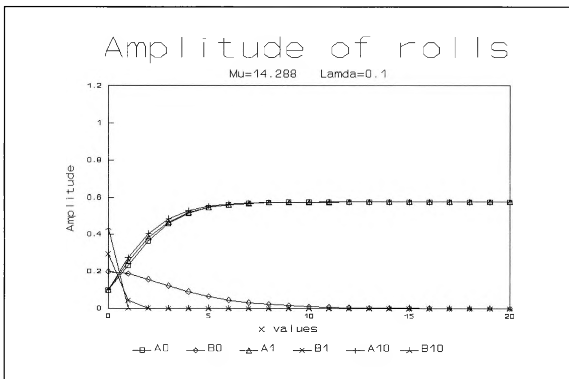
Fig. 2.17 : Numerical evolution for \mu=14.288 and \lambda=0.1 showing the amplitudes A and B of x -rolls and y -rolls at successive times \tau
