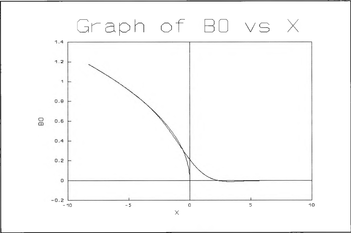
Fig. 3.1 : Graphs of \hat{B} and (-\hat{X}/6)^{1/2} versus \hat{X}
