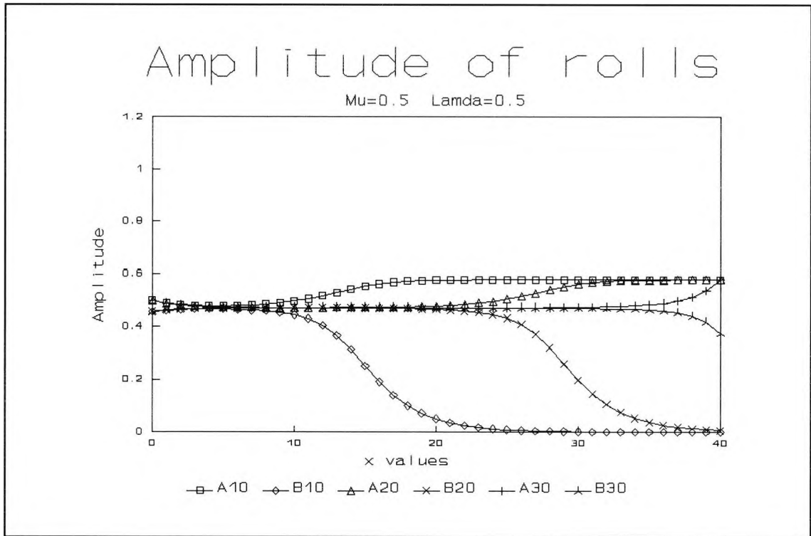
Fig. 2.20 : Numerical evolution for \mu=0.5 and \lambda=0.5 showing the amplitudes A and B of x -rolls and y -rolls at successive times \tau
