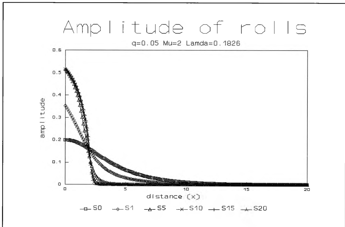
Fig. 4.12 : Numerical evolution for q=0.05 , \mu=2 and \lambda=0.1826 showing the amplitude of y -rolls at successive times \tau
