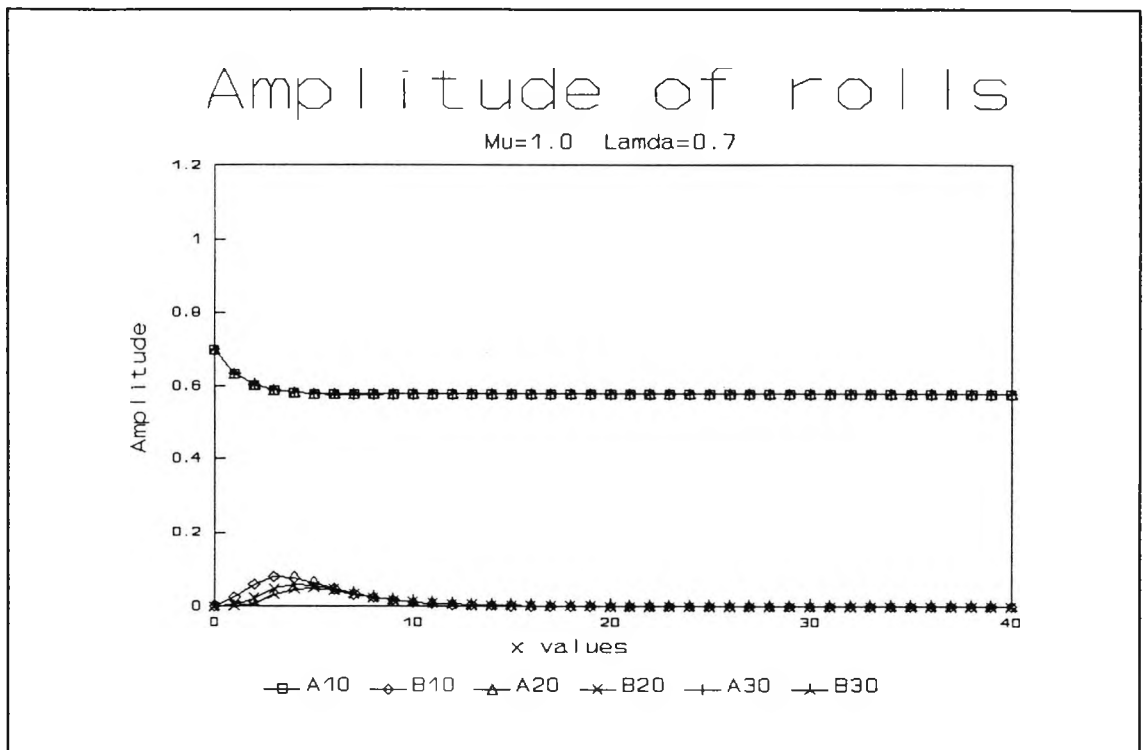
Fig. 2.24 : Numerical evolution for \mu=1.0 and \lambda=0.7 showing the amplitudes A and B of x -rolls and y -rolls at successive times \tau
