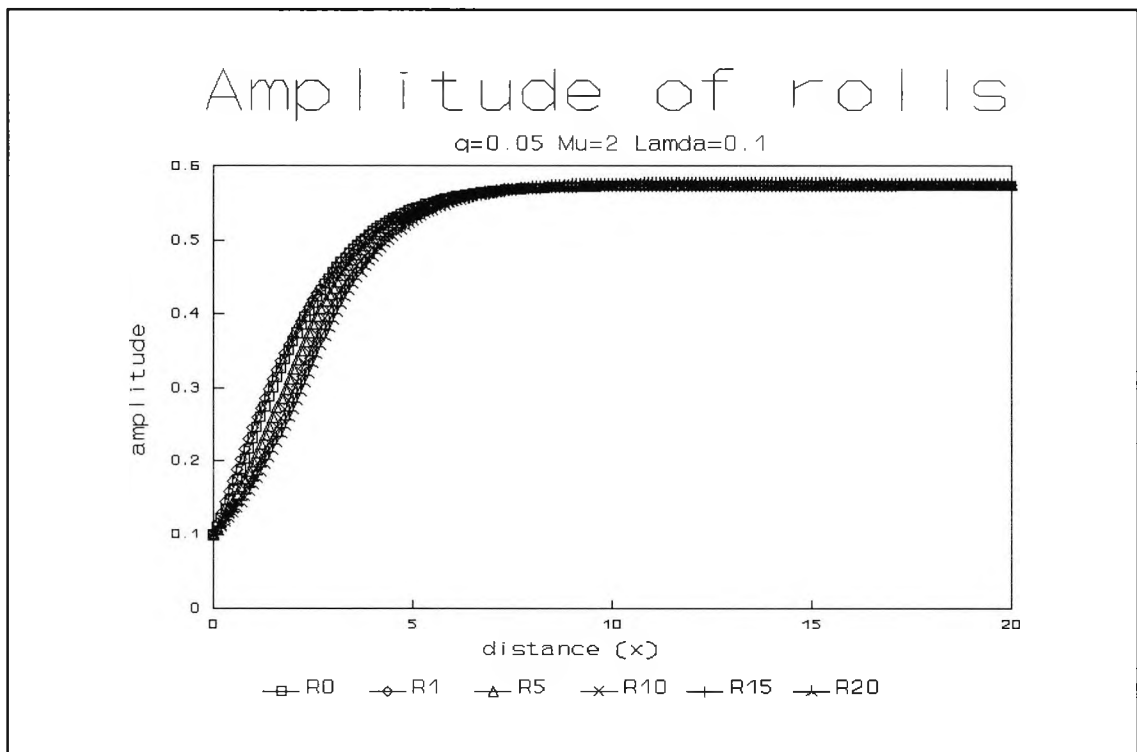
Fig. 4.7 : Numerical evolution for q=0.05 , \mu=2 and \lambda=0.1 showing the amplitude of x -rolls at successive times \tau
