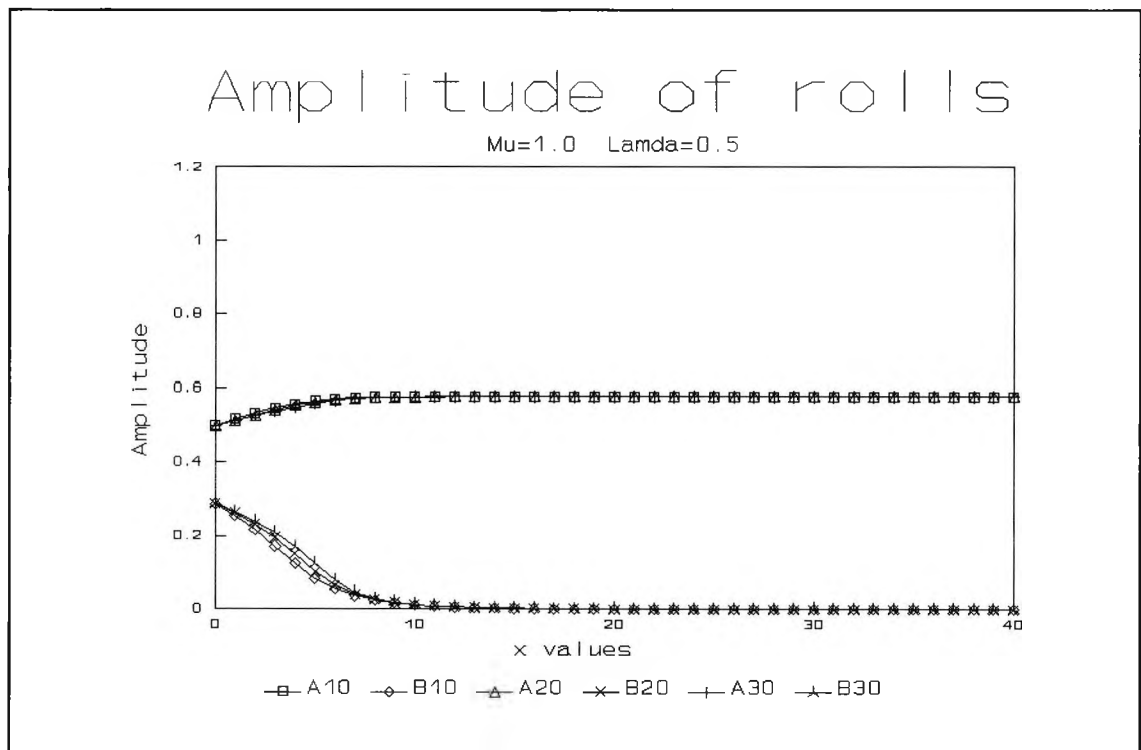
Fig. 2.23 : Numerical evolution for \mu=1.0 and \lambda=0.5 showing the amplitudes A and B of x -rolls and y -rolls at successive times \tau
