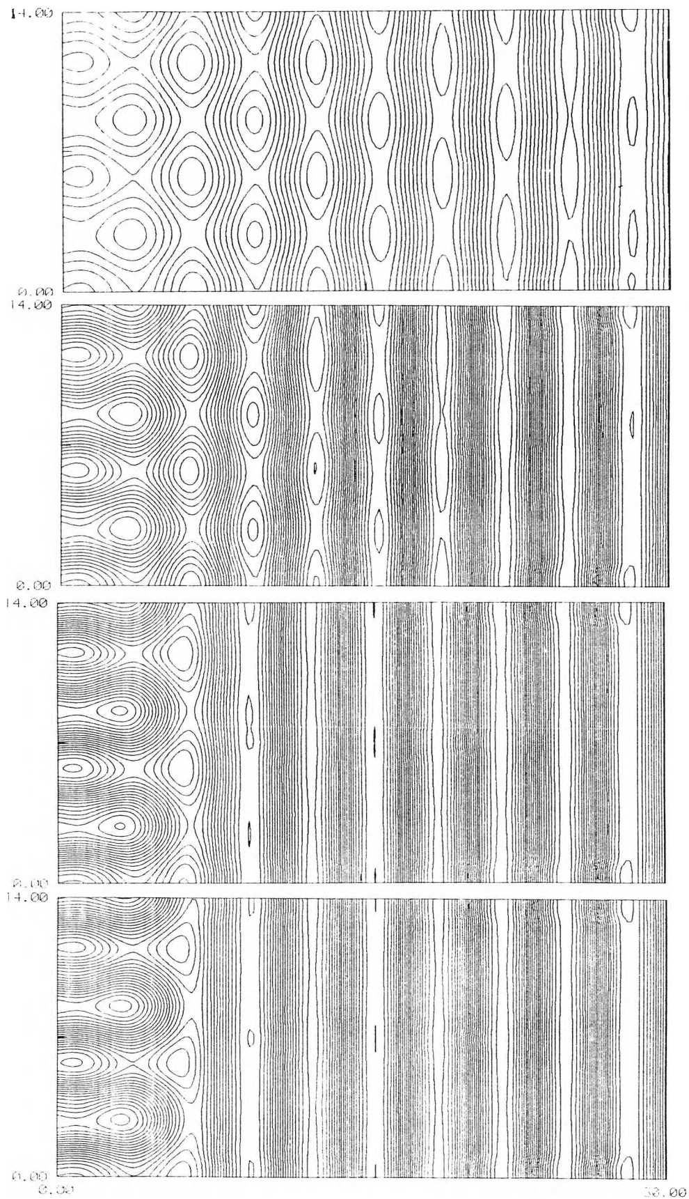
Fig. 5.4 : Contours of \psi at times \tau=0, 1, 5 and 20 for \delta^2=0.1, \mu=2.0, \lambda=0
