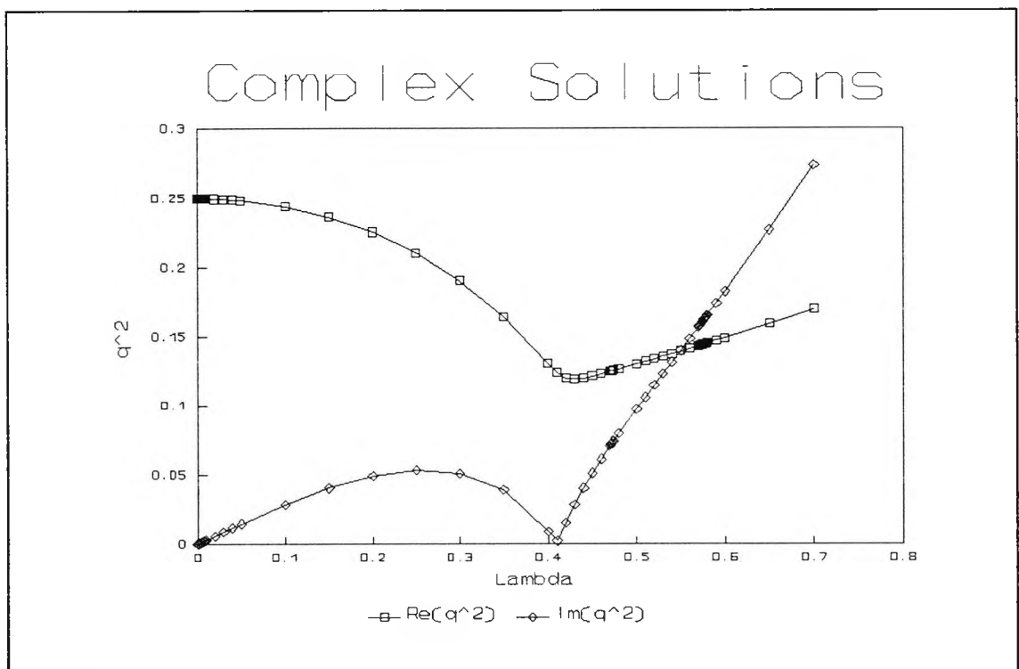
Fig. 4.2 : Complex conjugate roots of C(q^2, \lambda^2) = 0
