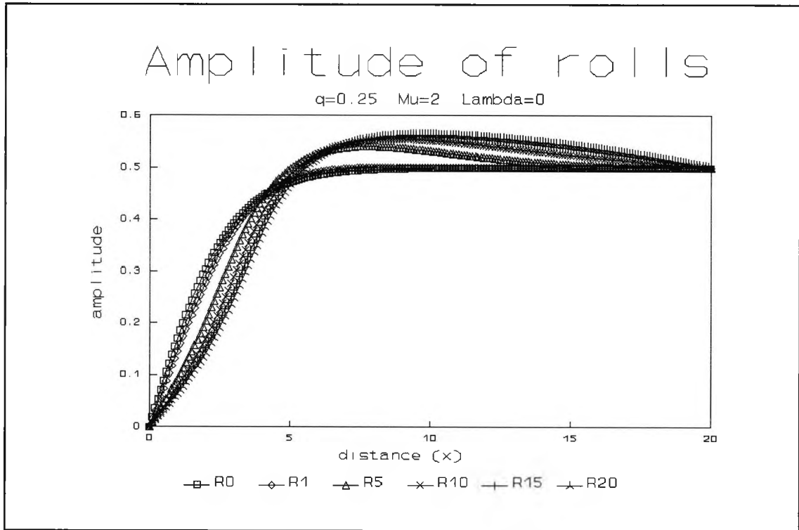
Fig. 4.43 : Numerical evolution for q=0.25 , \mu=2 and \lambda=0 showing the amplitude of x -rolls at successive times \tau
