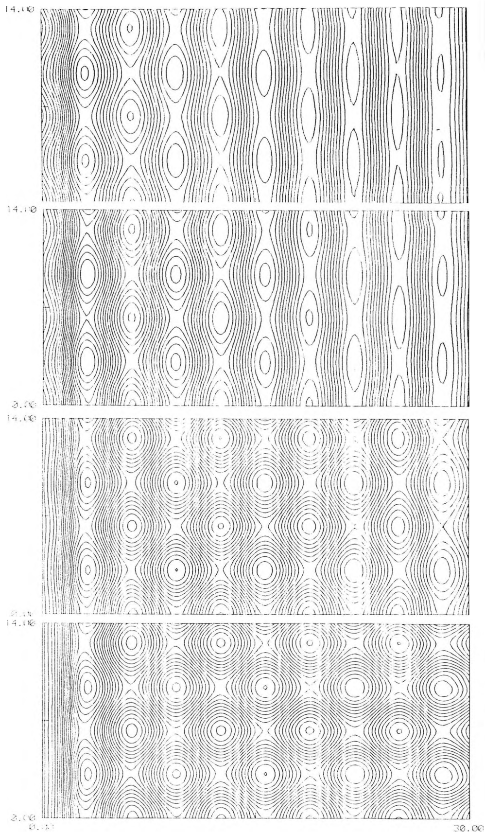
Fig. 2.33 : Contours of \psi at times \tau=0, 1, 5 and 20 for \mu=0.5, \lambda=1.0
