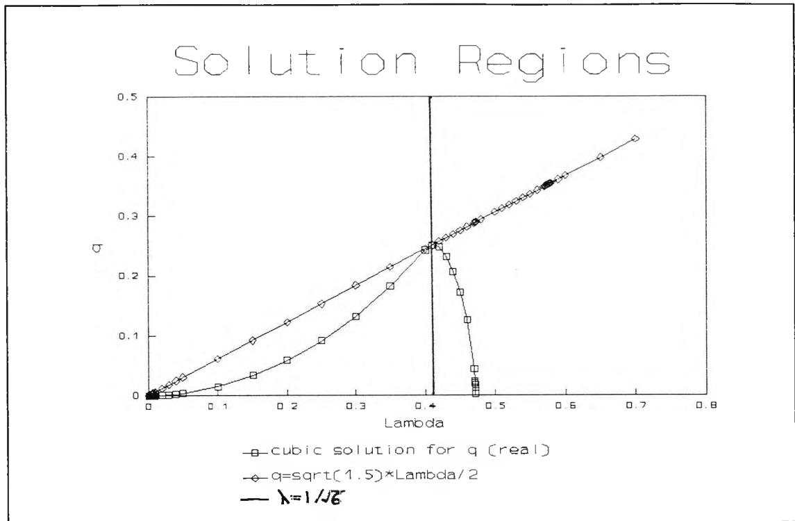
Fig. 4.1 : Real root of C(q^2, \lambda^2) = 0 and the lines q = \sqrt{3}\lambda/2\sqrt{2} and \lambda = 1/\sqrt{6} , defining the existence and stability of steady-state solutions
