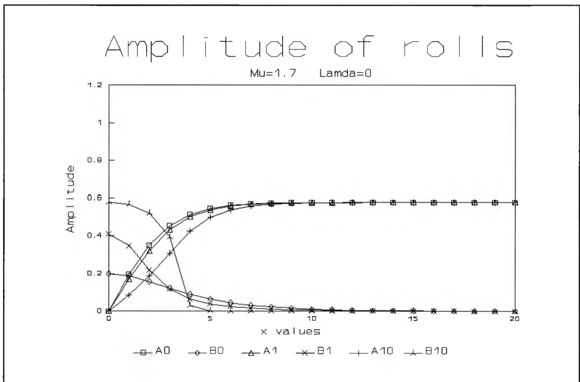
Fig. 2.9 : Numerical evolution for \mu=1.700 and \lambda=0 showing the amplitudes A and B of x -rolls and y -rolls at successive times \tau
