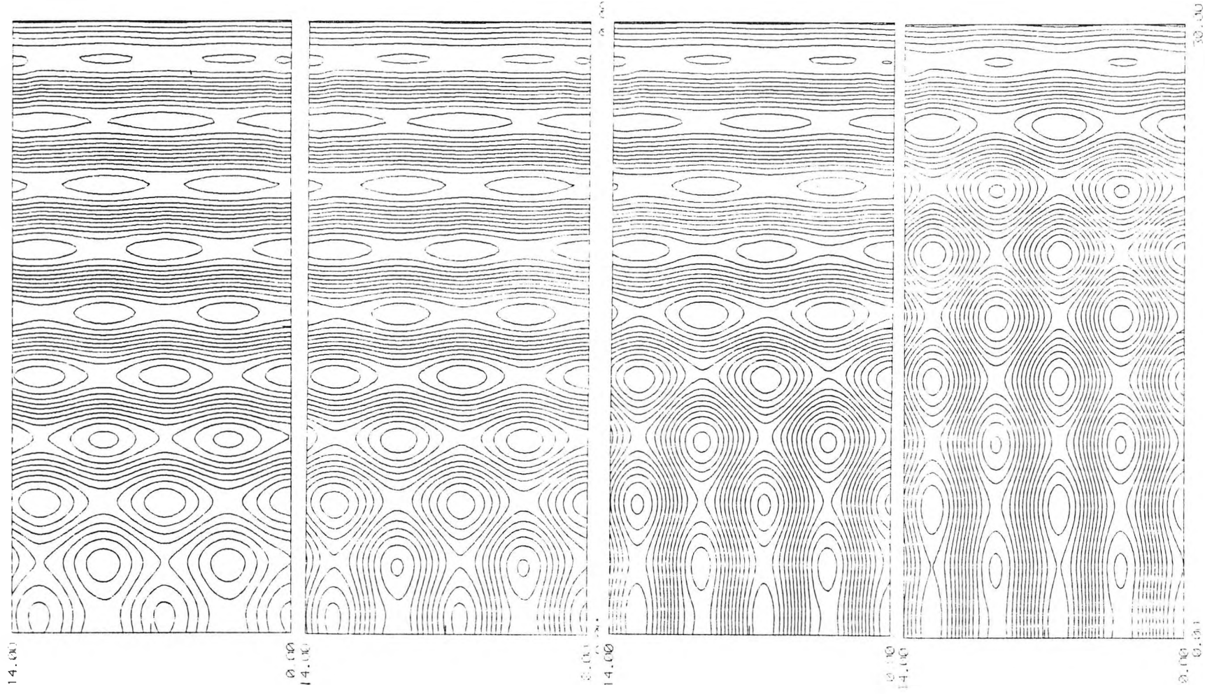
Fig. 2.35 : Contours of \psi at times \tau=0, 1, 5 and 20 for \mu=1.0, \lambda=0
