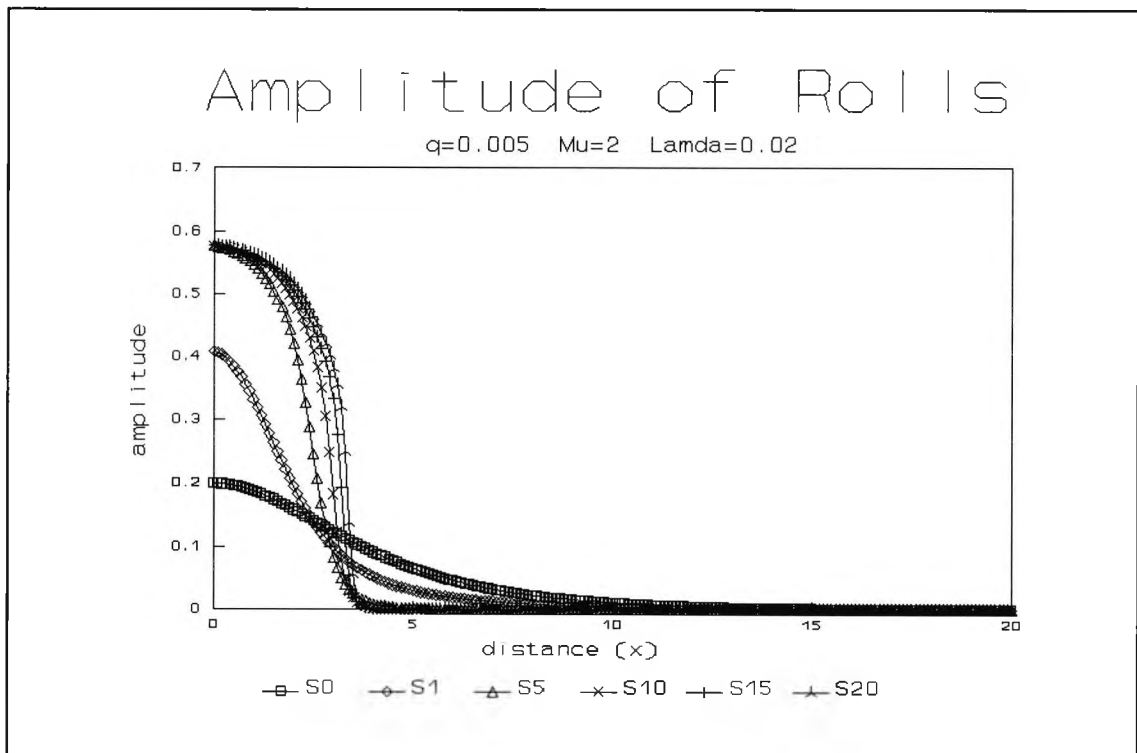
Fig. 4.60 : Numerical evolution for q=0.005 , \mu=2 and \lambda=0.02 showing the amplitude of y -rolls at successive times \tau
