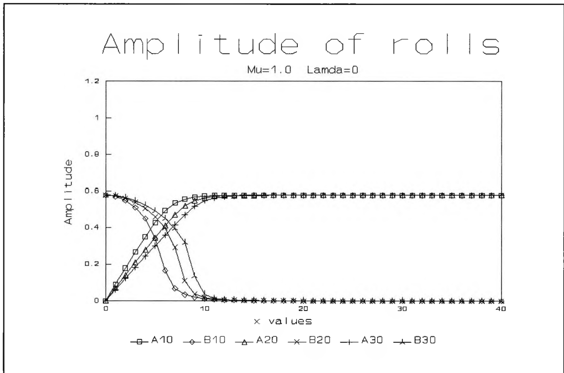
Fig. 2.22 : Numerical evolution for \mu=1.0 and \lambda=0 showing the amplitudes A and B of x -rolls and y -rolls at successive times \tau
