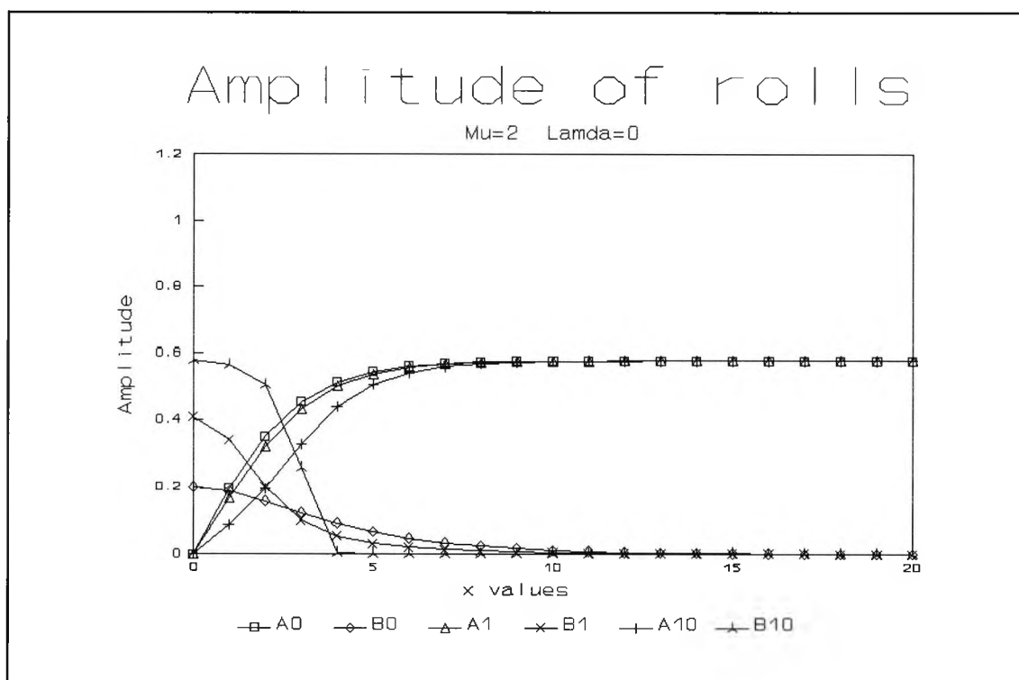
Fig. 2.12 : Numerical evolution for \mu=2.0 and \lambda=0 showing the amplitudes A and B of x -rolls and y -rolls at successive times \tau
