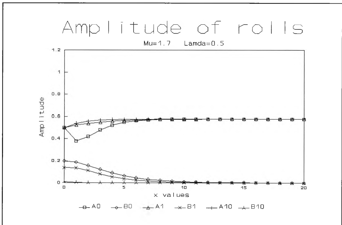
Fig. 2.11 : Numerical evolution for \mu=1.700 and \lambda=0.5 showing the amplitudes A and B of x -rolls and y -rolls at successive times \tau
