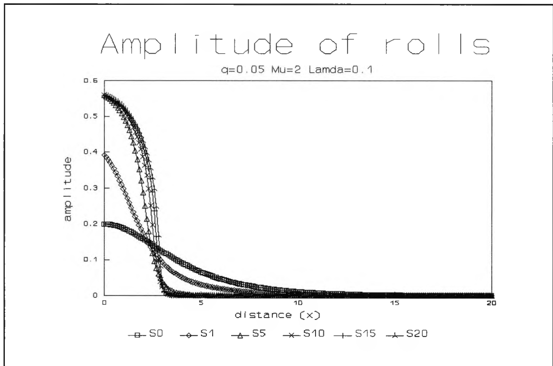
Fig. 4.9 : Numerical evolution for q=0.05 , \mu=2 and \lambda=0.1 showing the amplitude of y-rolls at successive times \tau
