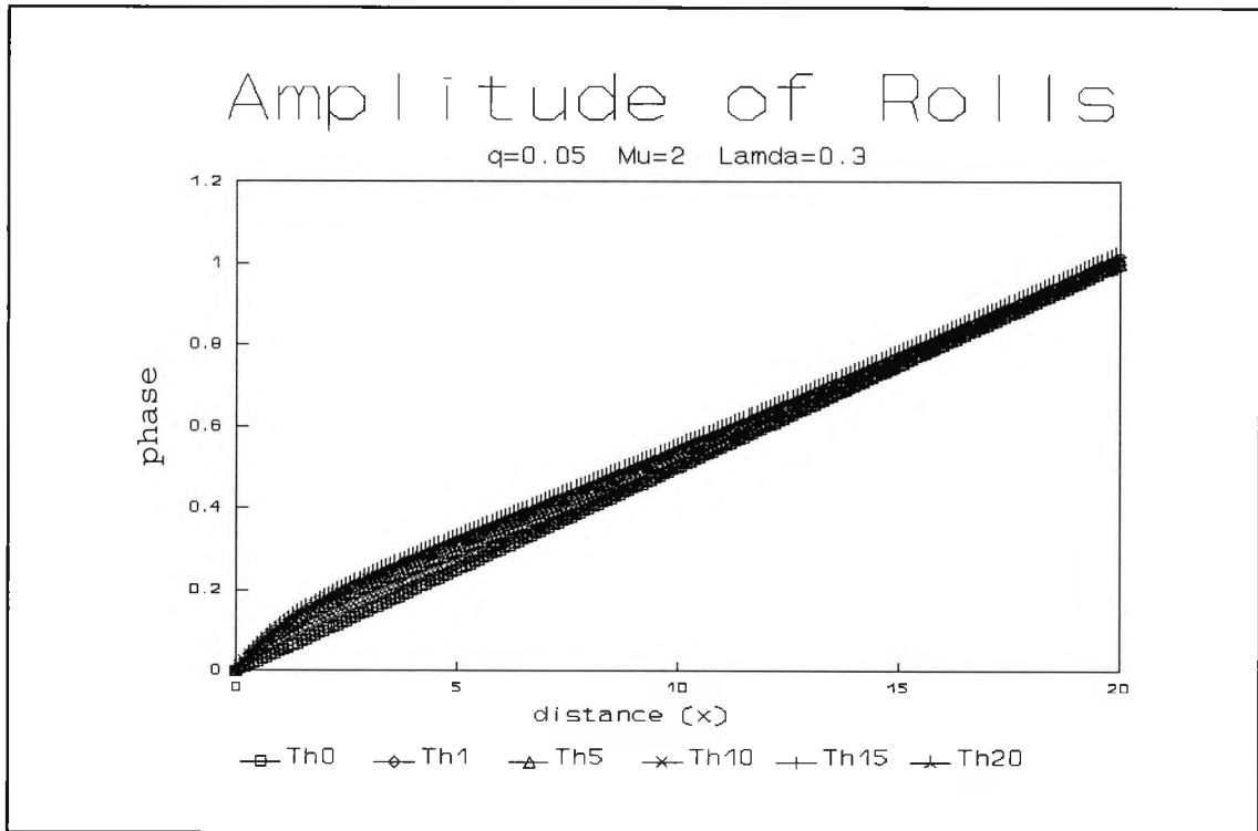
Fig. 4.14 : Numerical evolution for q=0.05 , \mu=2 and \lambda=0.3 showing the phase of x -rolls at successive times \tau
