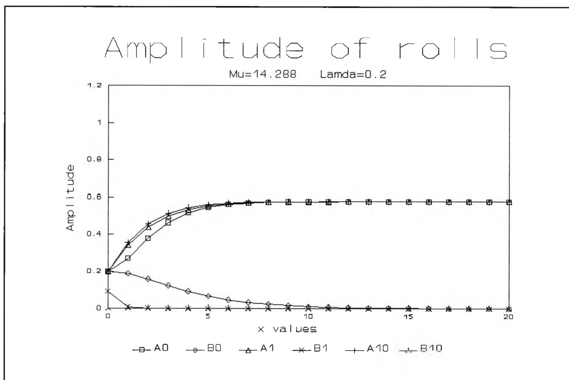
Fig. 2.18 : Numerical evolution for \mu=14.288 and \lambda=0.2 showing the amplitudes A and B of x -rolls and y -rolls at successive times \tau
