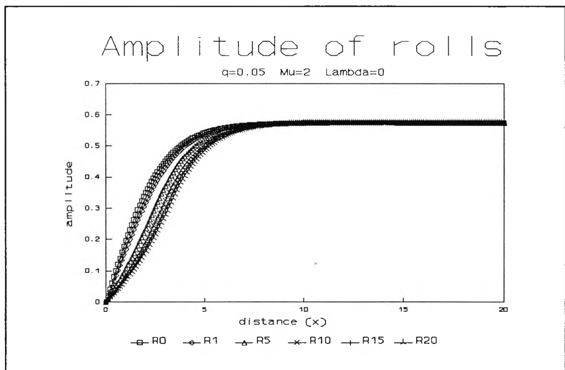
Fig. 4.4 : Numerical evolution for q=0.05 , \mu=2 and \lambda=0 showing the amplitude of x -rolls at successive times \tau
