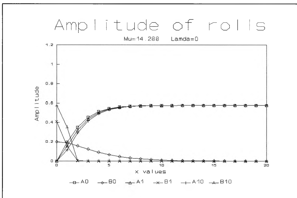
Fig. 2.16 : Numerical evolution for \mu=14.288 and \lambda=0 showing the amplitudes A and B of x -rolls and y -rolls at successive times \tau
