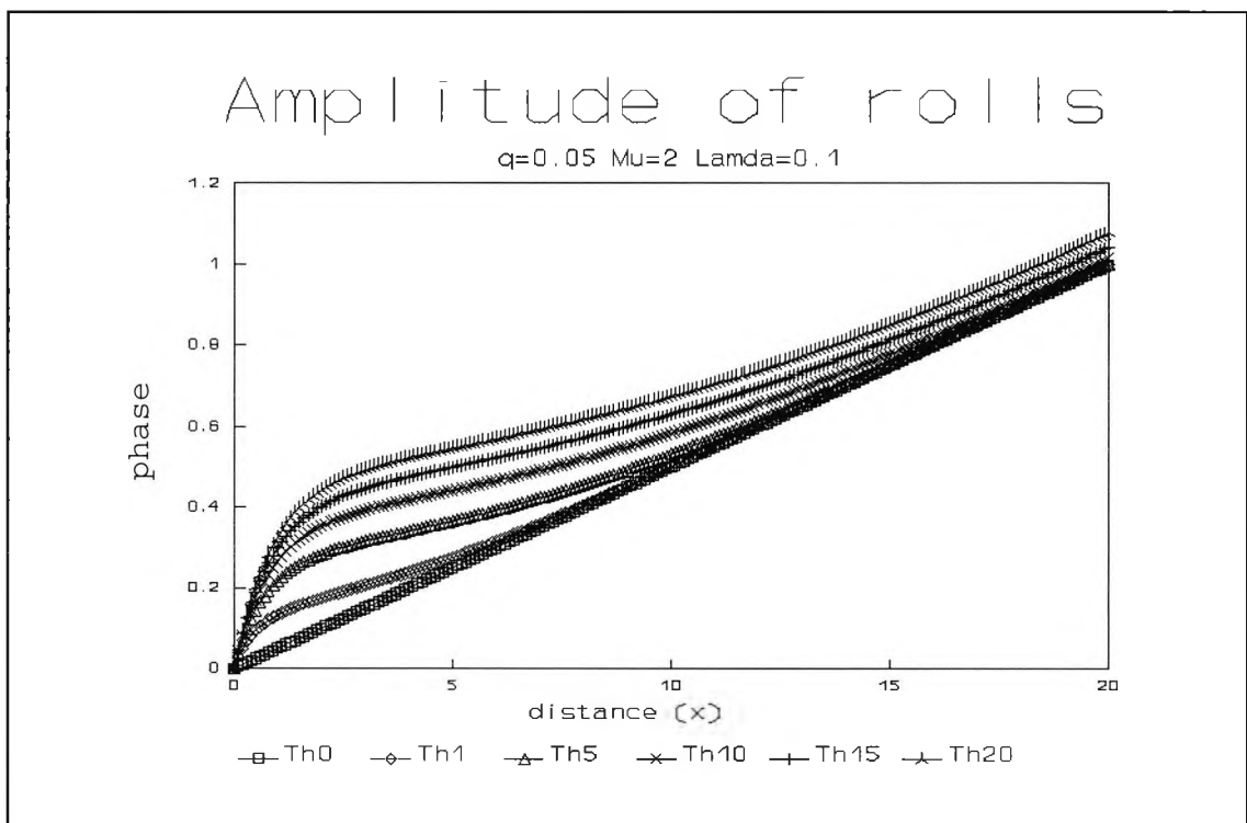
Fig. 4.8 : Numerical evolution for q=0.05 , \mu=2 and \lambda=0.1 showing the phase of x -rolls at successive times \tau
