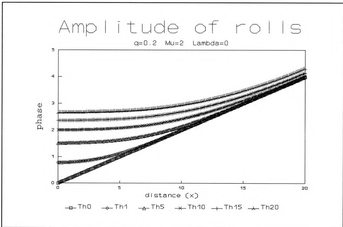
Fig. 4.26 : Numerical evolution for q=0.2 , \mu=2 and \lambda=0 showing the phase of x -rolls at successive times \tau
