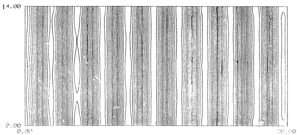
Fig. 4.61 : Contours of \psi at times \tau=0, 1 and 5 for q=0.2, \mu=2.0, \lambda=0.5
