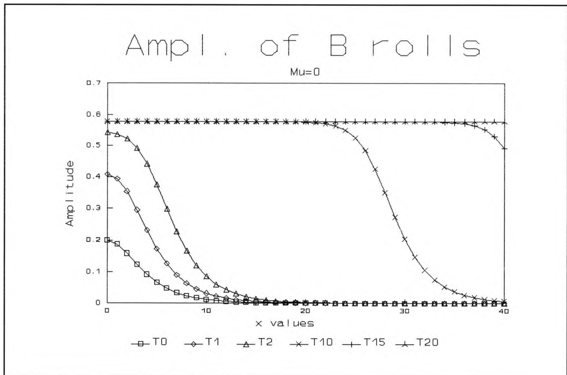
Fig. 2.26 : Analytical solution showing the amplitude B of y-rolls at successive times \tau
