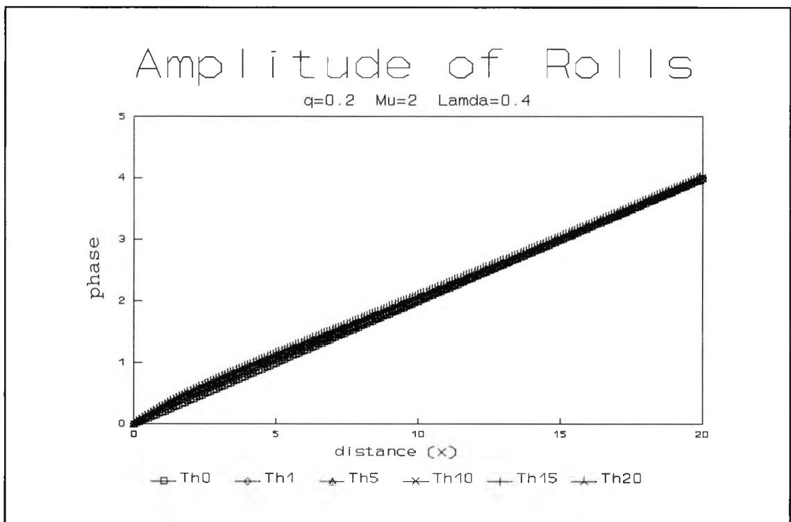
Fig. 4.38 : Numerical evolution for q=0.2 , \mu=2 and \lambda=0.4 showing the phase of x -rolls at successive times \tau
