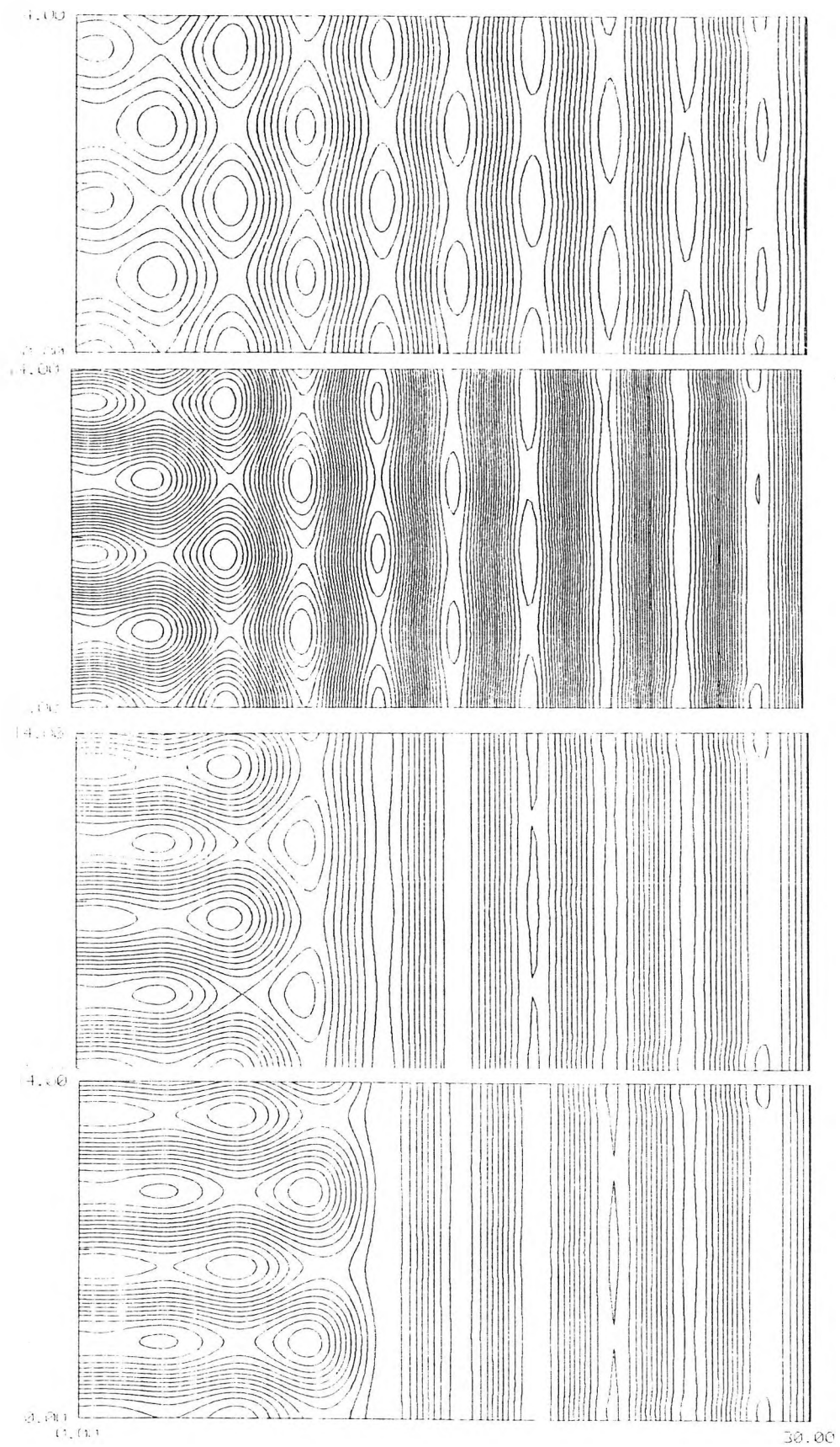
Fig. 2.27 : Contours of \psi at times \tau=0, 1, 5 and 20 for \mu=2.0, \lambda=0
