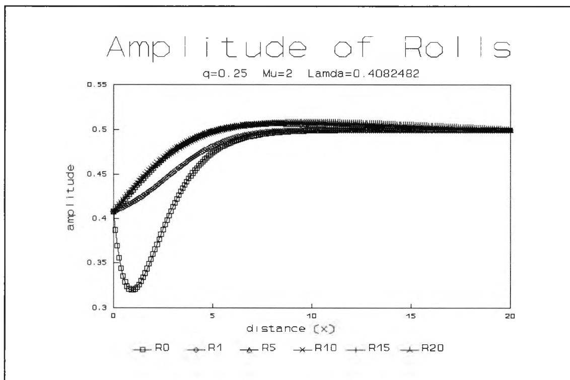
Fig. 4.49 : Numerical evolution for q=0.25 , \mu=2 and \lambda=0.4082 showing the amplitude of x -rolls at successive times \tau
