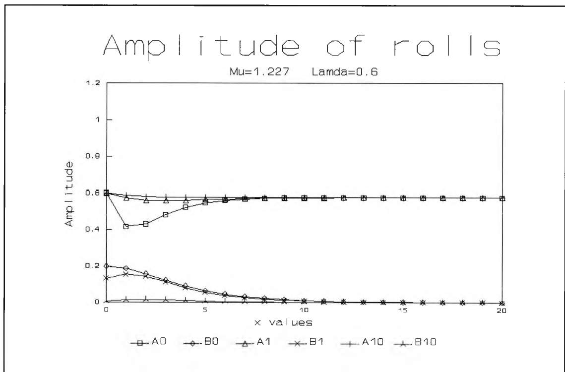
Fig. 2.5 : Numerical evolution for \mu=1.227 and \lambda=0.6 showing the amplitudes A and B of x -rolls and y -rolls at successive times \tau
