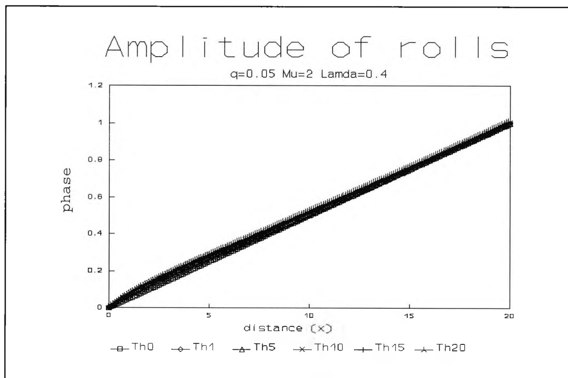
Fig. 4.20 : Numerical evolution for q=0.05 , \mu=2 and \lambda=0.4 showing the phase of x -rolls at successive times \tau
