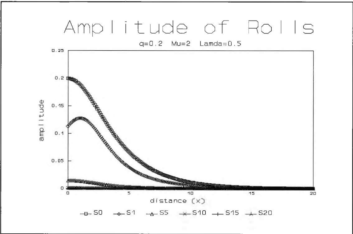
Fig. 4.42 : Numerical evolution for q=0.2 , \mu=2 and \lambda=0.5 showing the amplitude of y -rolls at successive times \tau
