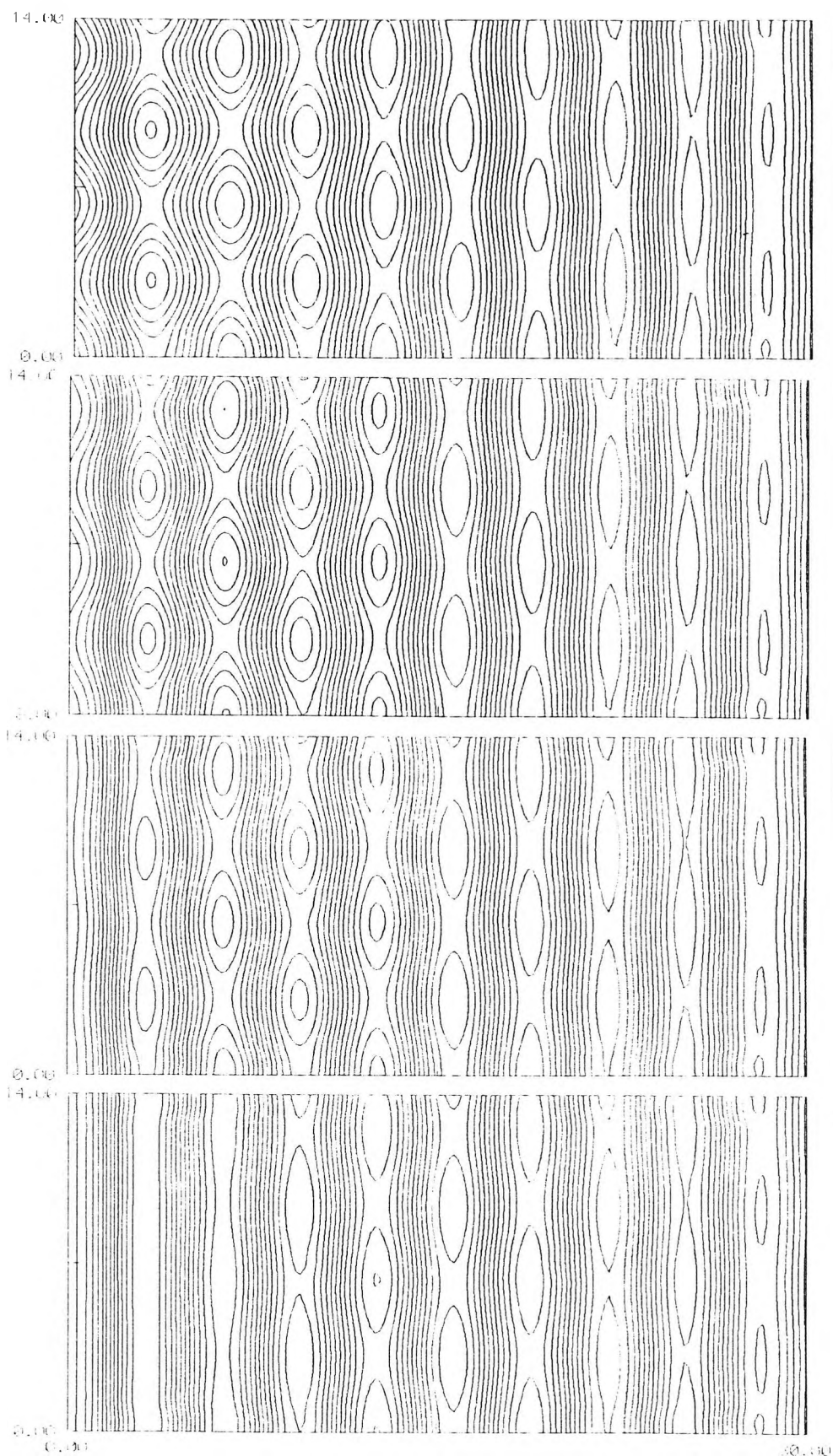
Fig. 2.37 : Contours of \psi at times \tau=0, 1, 5 and 20 for \mu=1.0, \lambda=0.7
