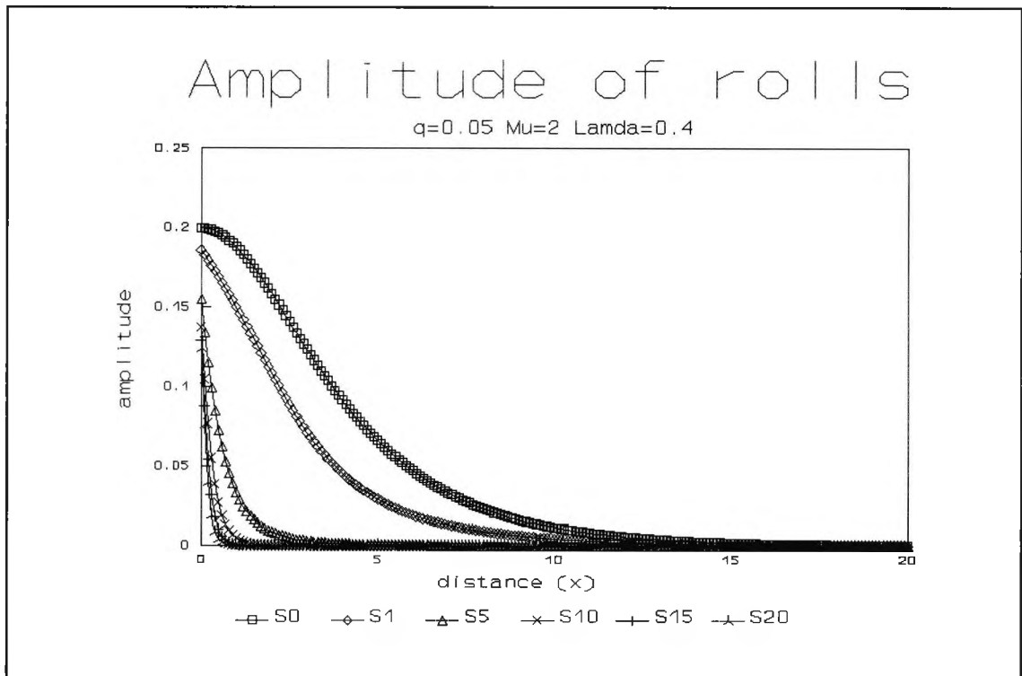
Fig. 4.21 : Numerical evolution for q=0.05 , \mu=2 and \lambda=0.4 showing the amplitude of y-rolls at successive times \tau
