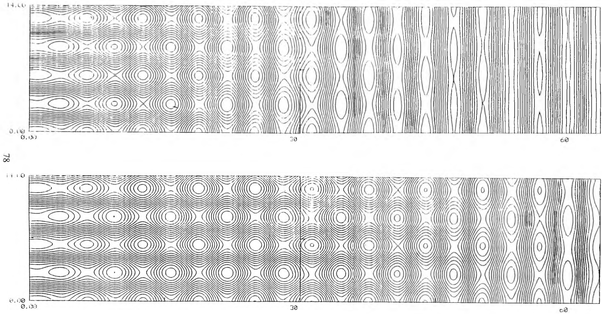
Fig. 2.34 : Contours of \psi at times \tau=5 and 10 for \mu=0.5 , \lambda=0 showing the solution structure
