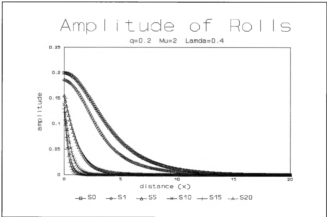
Fig. 4.39 : Numerical evolution for q=0.2 , \mu=2 and \lambda=0.4 showing the amplitude of y -rolls at successive times \tau
