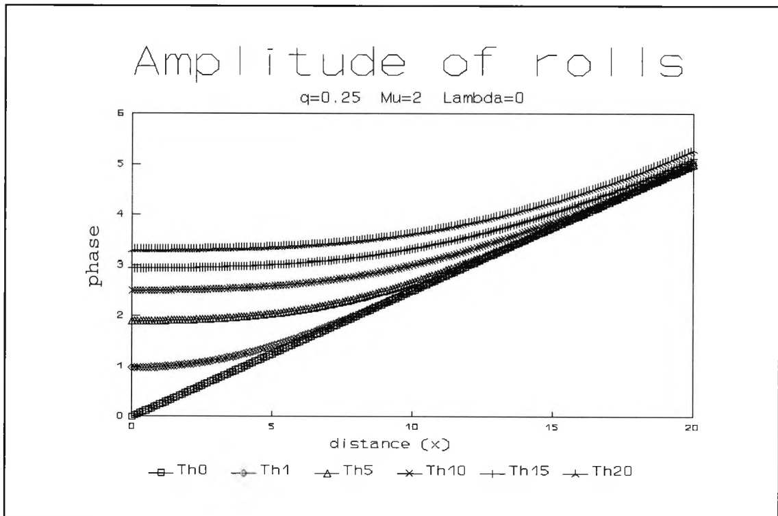
Fig. 4.44 : Numerical evolution for q=0.25 , \mu=2 and \lambda=0 showing the phase of x -rolls at successive times \tau
