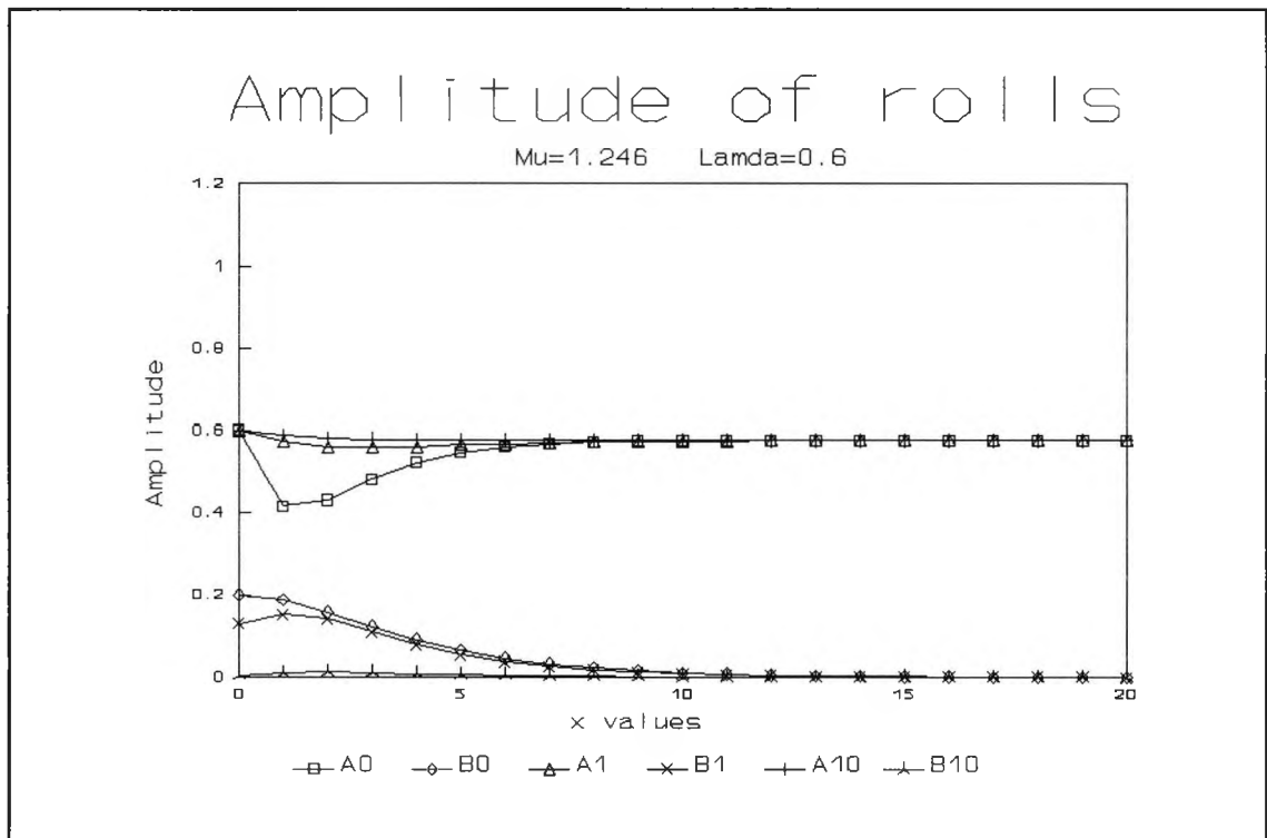
Fig. 2.8 : Numerical evolution for \mu=1.246 and \lambda=0.6 showing the amplitudes A and B of x -rolls and y -rolls at successive times \tau
