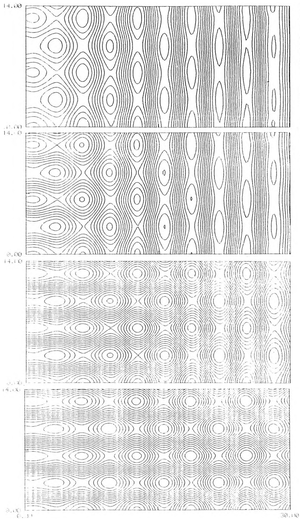
Fig. 2.31 : Contours of \psi at times \tau=0, 1, 5 and 20 for \mu=0.5, \lambda=0
