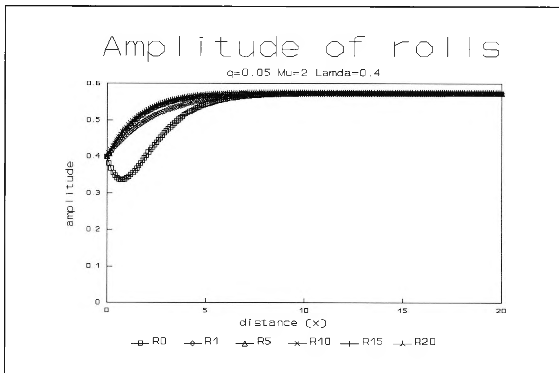
Fig. 4.19 : Numerical evolution for q=0.05 , \mu=2 and \lambda=0.4 showing the amplitude of x -rolls at successive times \tau
