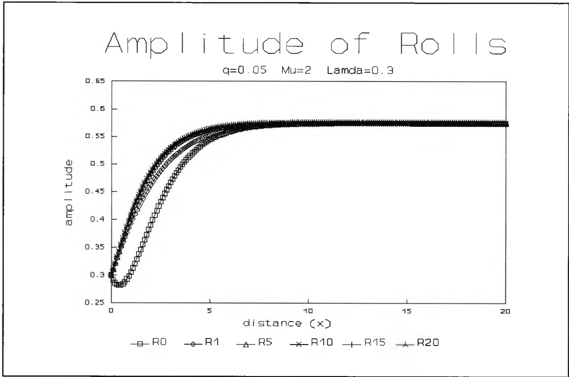
Fig. 4.13 : Numerical evolution for q=0.05 , \mu=2 and \lambda=0.3 showing the amplitude of x -rolls at successive times \tau
