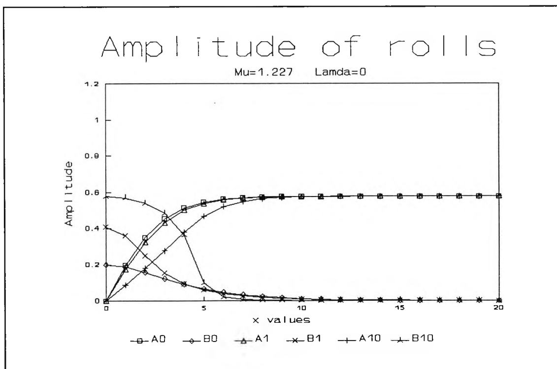
Fig. 2.3 : Numerical evolution for \mu = 1.227 and \lambda = 0 showing the amplitudes A and B of x -rolls and y -rolls at successive times \tau = 0, 1, 10 indicated by A_0, B_0, A_1, B_1, A_{10}, B_{10} respectively
