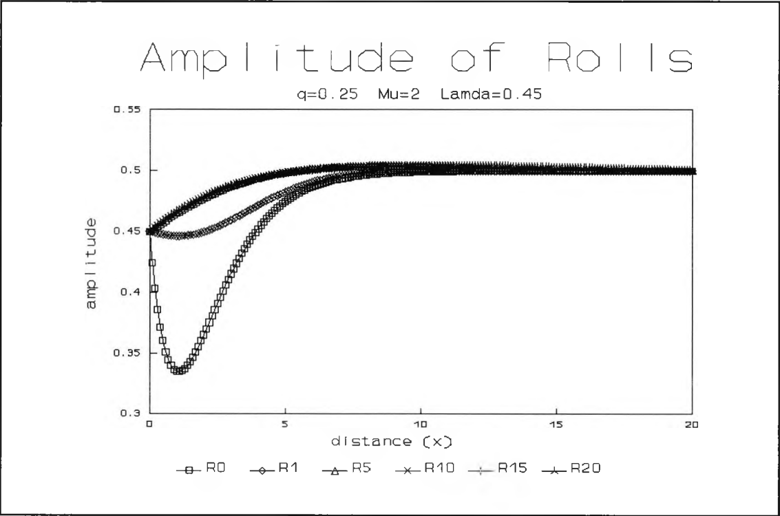
Fig. 4.52 : Numerical evolution for q=0.25 , \mu=2 and \lambda=0.45 showing the amplitude of x -rolls at successive times \tau
