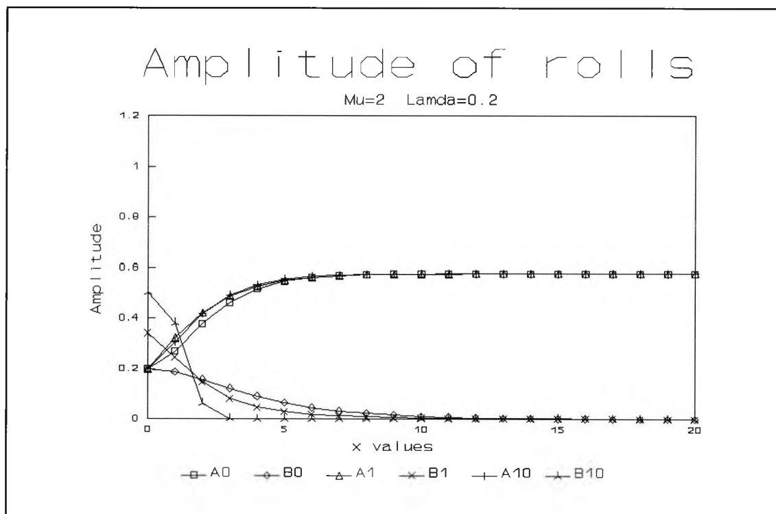
Fig. 2.13 : Numerical evolution for \mu=2.0 and \lambda=0.2 showing the amplitudes A and B of x -rolls and y -rolls at successive times \tau
