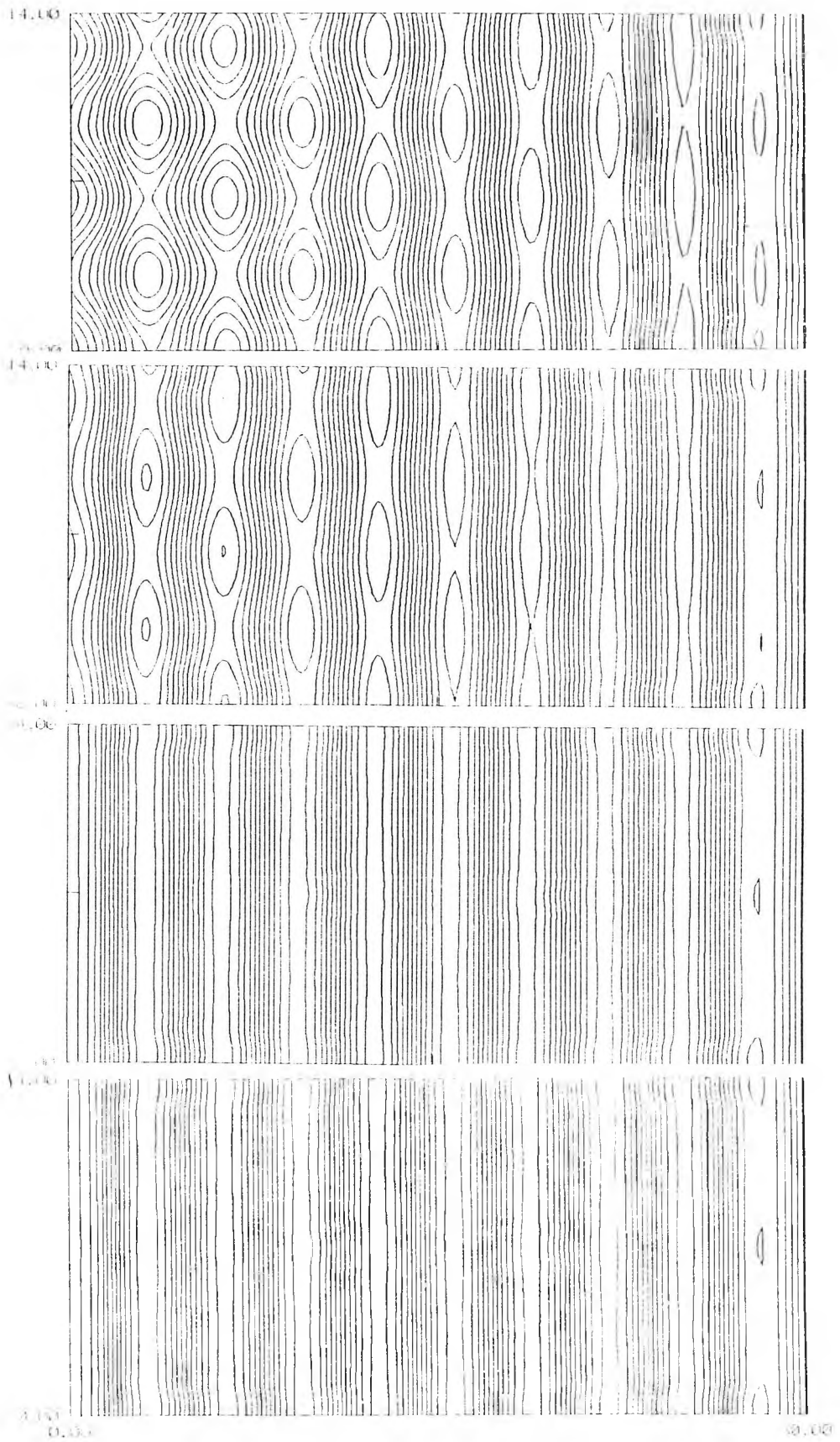
Fig. 2.30 : Contours of \psi at times \tau=0, 1, 5 and 20 for \mu=2.0, \lambda=0.6
