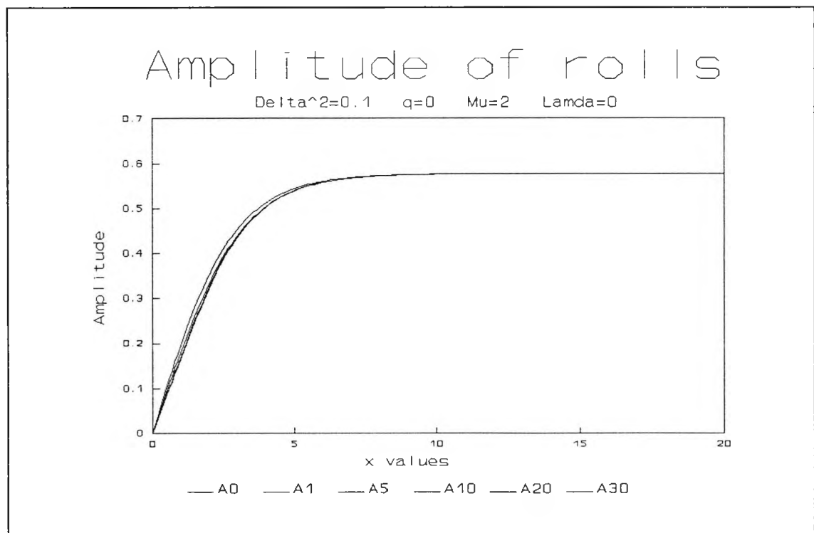
Fig. 5.2 : Amplitude of x -rolls when \delta^2=0.1 , q=0 , \mu=2 and \lambda=0 at successive times \tau=0, 1, 5, 10, 20, 30 indicated by A_0, A_1, A_5, A_{10}, A_{20}, A_{30} respectively
