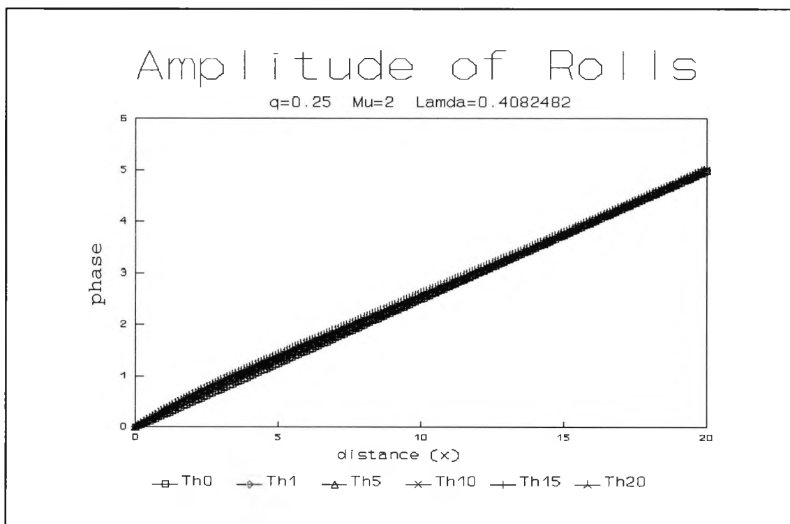
Fig. 4.50 : Numerical evolution for q=0.25 , \mu=2 and \lambda=0.4082 showing the phase of x -rolls at successive times \tau
