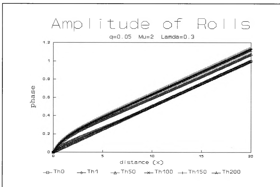
Fig. 4.17 : Numerical evolution for q=0.05 , \mu=2 and \lambda=0.3 showing the phase of x -rolls at successive times \tau
