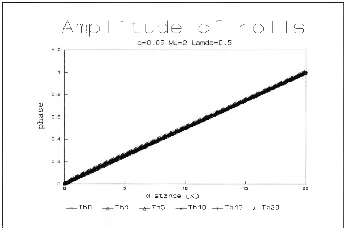
Fig. 4.23 : Numerical evolution for q=0.05 , \mu=2 and \lambda=0.5 showing the phase of x -rolls at successive times \tau
