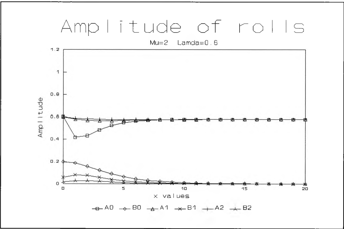
Fig. 2.15 : Numerical evolution for \mu=2.0 and \lambda=0.6 showing the amplitudes A and B of x -rolls and y -rolls at successive times \tau
