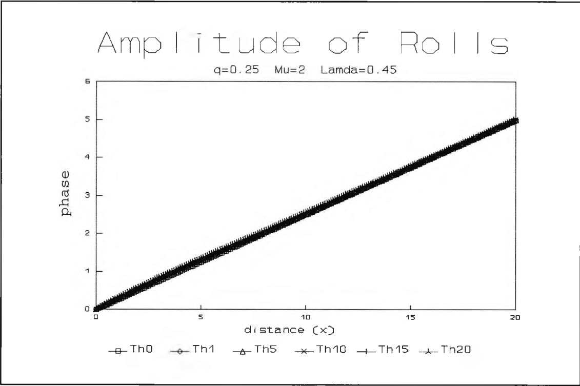
Fig. 4.53 : Numerical evolution for q=0.25 , \mu=2 and \lambda=0.45 showing the phase of x -rolls at successive times \tau
