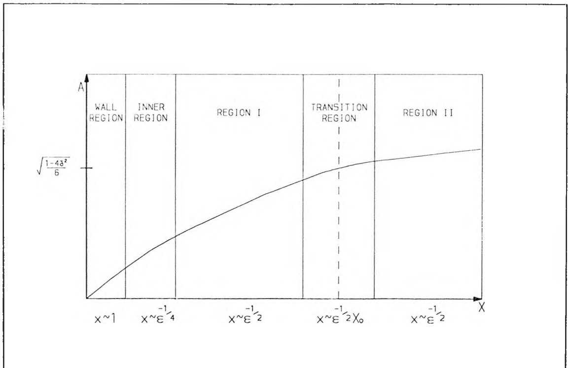
Fig. 6.1 : Schematic diagram showing the main flow regions
