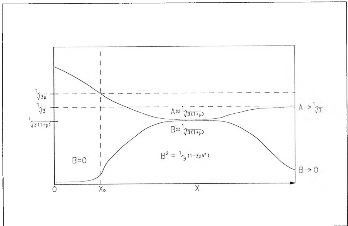
Fig. 2.25 : Schematic diagram showing the main flow regions for \mu < 1 and \lambda > 1/\sqrt{3\mu}
