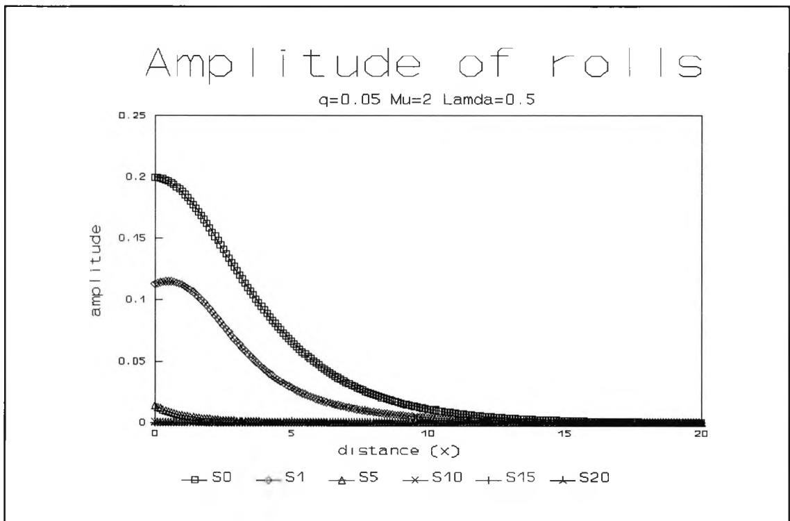
Fig. 4.24 : Numerical evolution for q=0.05 , \mu=2 and \lambda=0.5 showing the amplitude of y -rolls at successive times \tau
