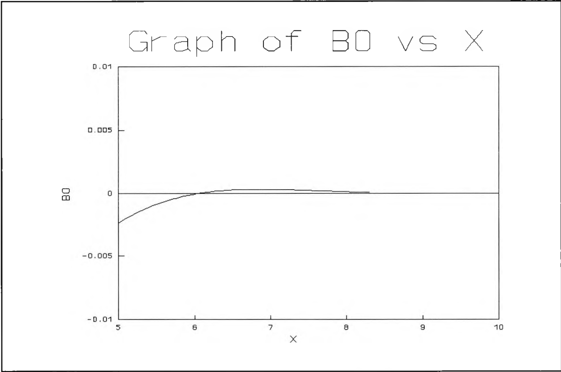
Fig. 3.2 : Detailed graph of \hat{B} vs \hat{X}
