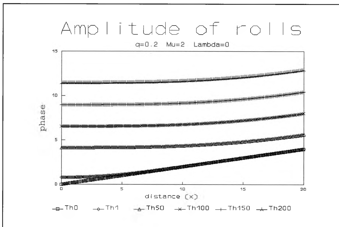
Fig. 4.29 : Numerical evolution for q=0.2 , \mu=2 and \lambda=0 showing the phase of x -rolls at successive times \tau
