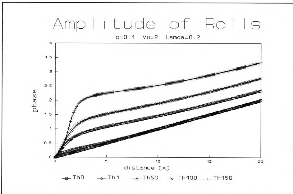
Fig. 4.56 : Numerical evolution for q=0.1 , \mu=2 and \lambda=0.2 showing the phase of x -rolls at successive times \tau
