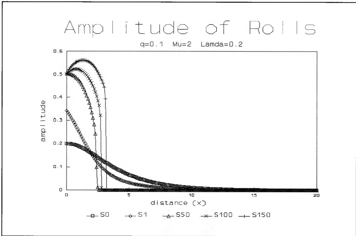
Fig. 4.57 : Numerical evolution for q=0.1 , \mu=2 and \lambda=0.2 showing the amplitude of y-rolls at successive times \tau
