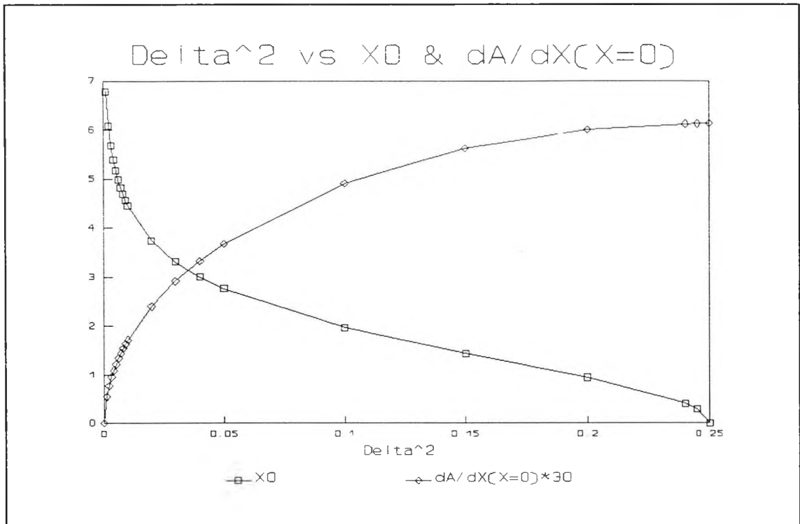
Fig. 5.1 : Graphs of X_0 and \partial A/\partial X (X=0) versus \delta^2 for \lambda=0
