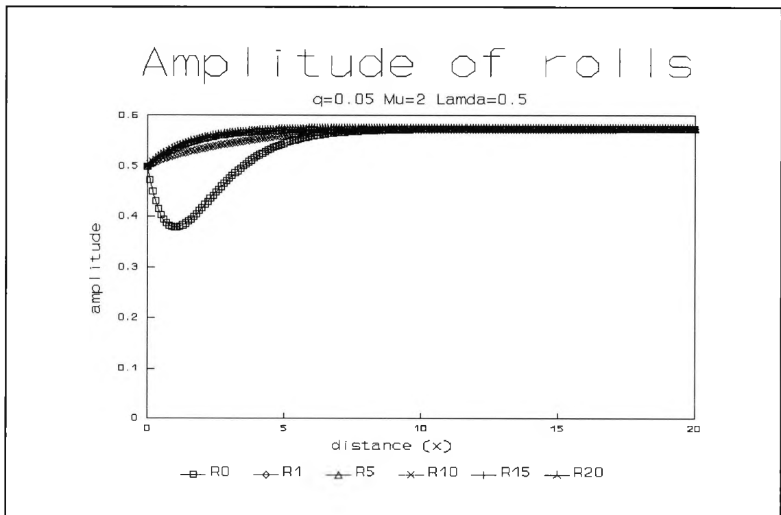
Fig. 4.22 : Numerical evolution for q=0.05 , \mu=2 and \lambda=0.5 showing the amplitude of x-rolls at successive times \tau
