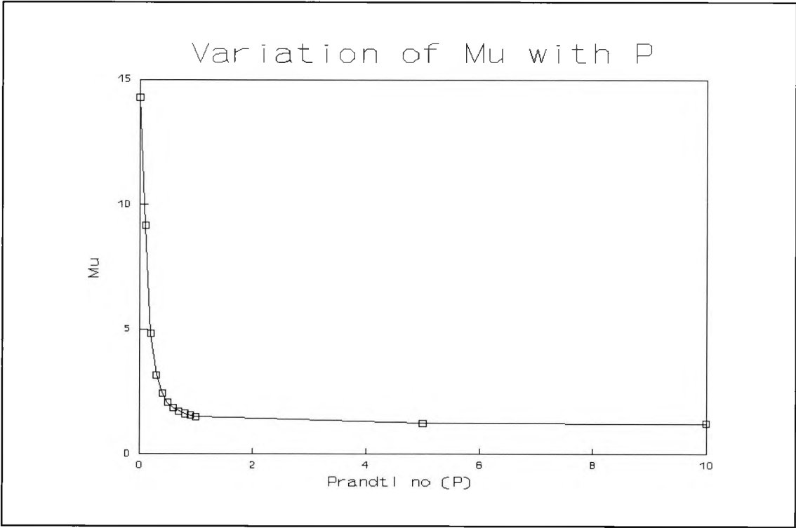
Fig. 2.1 : Variation of \mu with the Prandtl number P
