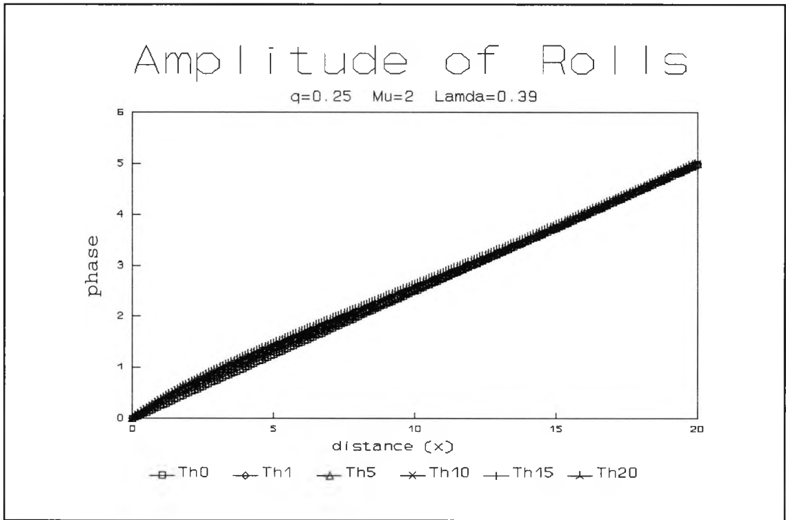
Fig. 4.47 : Numerical evolution for q=0.25 , \mu=2 and \lambda=0.39 showing the phase of x -rolls at successive times \tau
