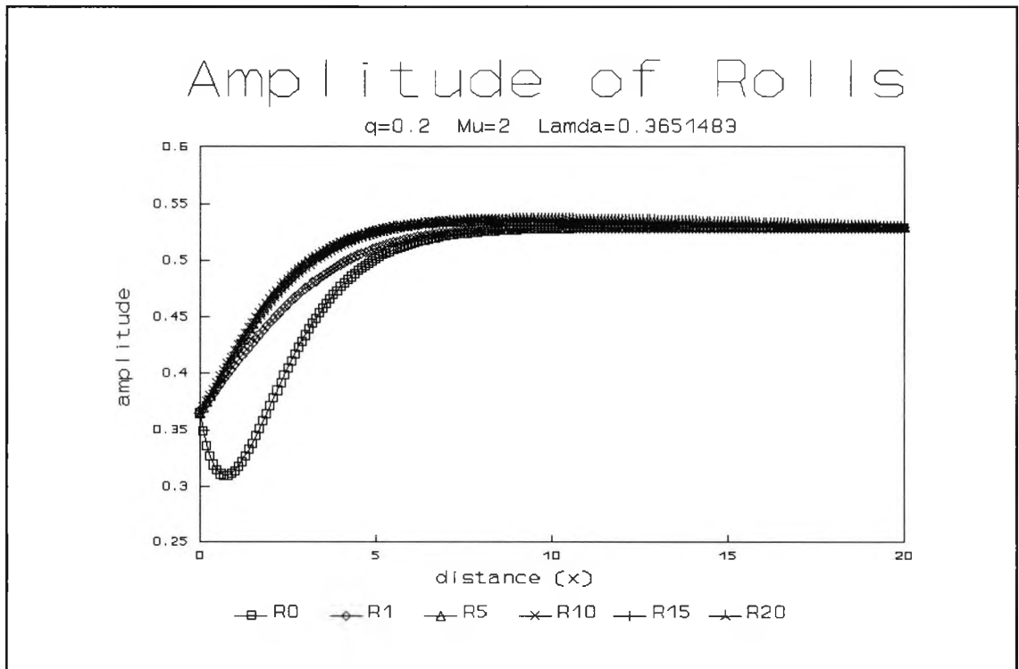
Fig. 4.34 : Numerical evolution for q=0.2 , \mu=2 and \lambda=0.3651 showing the amplitude of x -rolls at successive times \tau
