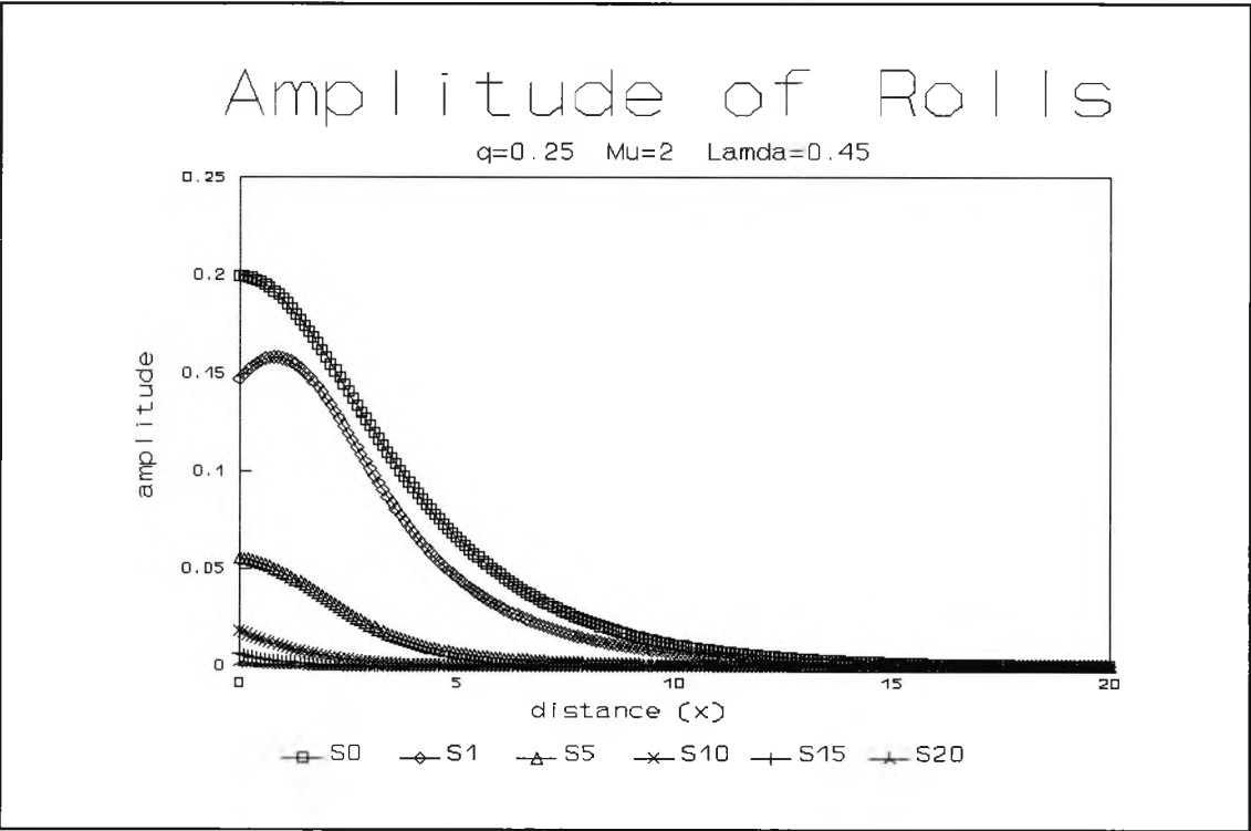
Fig. 4.54 : Numerical evolution for q=0.25 , \mu=2 and \lambda=0.45 showing the amplitude of y -rolls at successive times \tau
