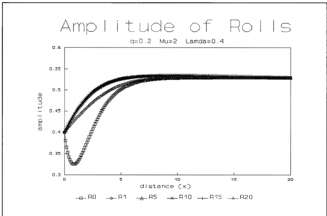
Fig. 4.37 : Numerical evolution for q=0.2 , \mu=2 and \lambda=0.4 showing the amplitude of x -rolls at successive times \tau
