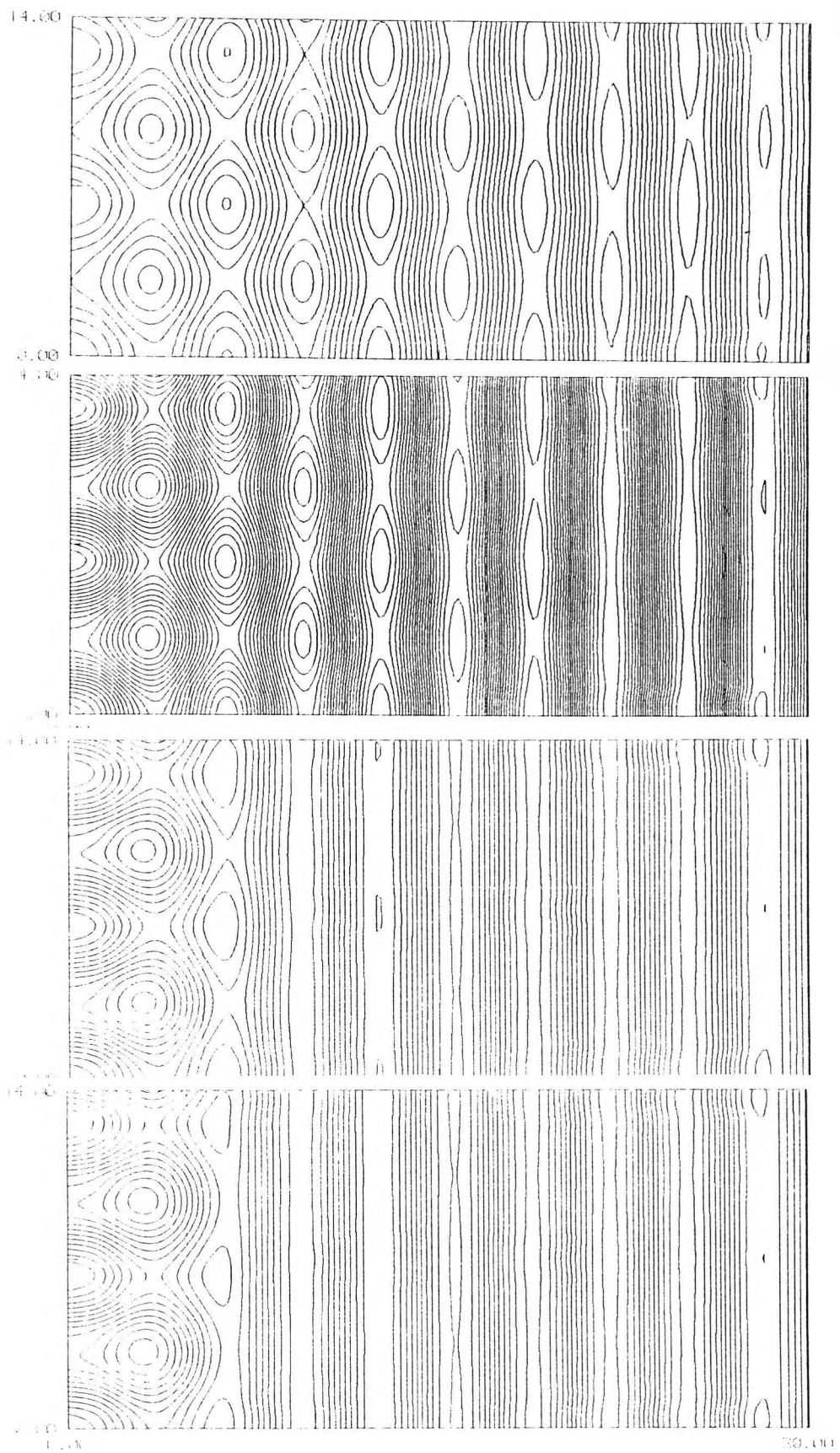
Fig. 2.28 : Contours of \psi at times \tau=0, 1, 5 and 20 for \mu=2.0, \lambda=0.2
