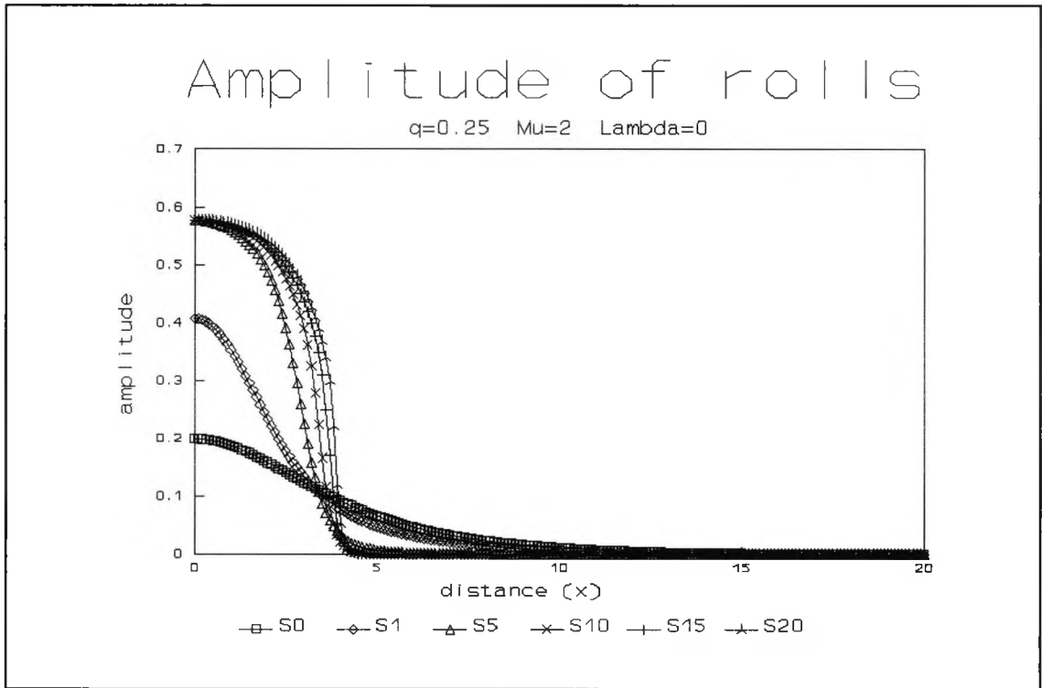
Fig. 4.45 : Numerical evolution for q=0.25 , \mu=2 and \lambda=0 showing the amplitude of y -rolls at successive times \tau
