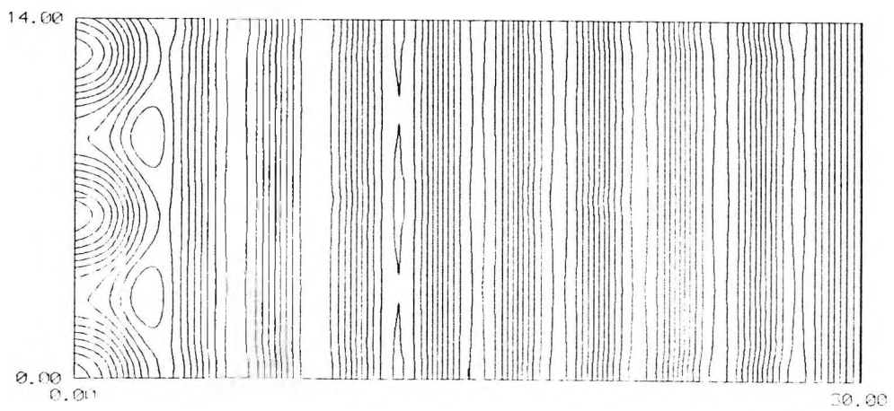
Fig. 4.63 : Contours of \psi at times \tau=0, 1 and 50 for q=0.05, \mu=2.0, \lambda=0.3
