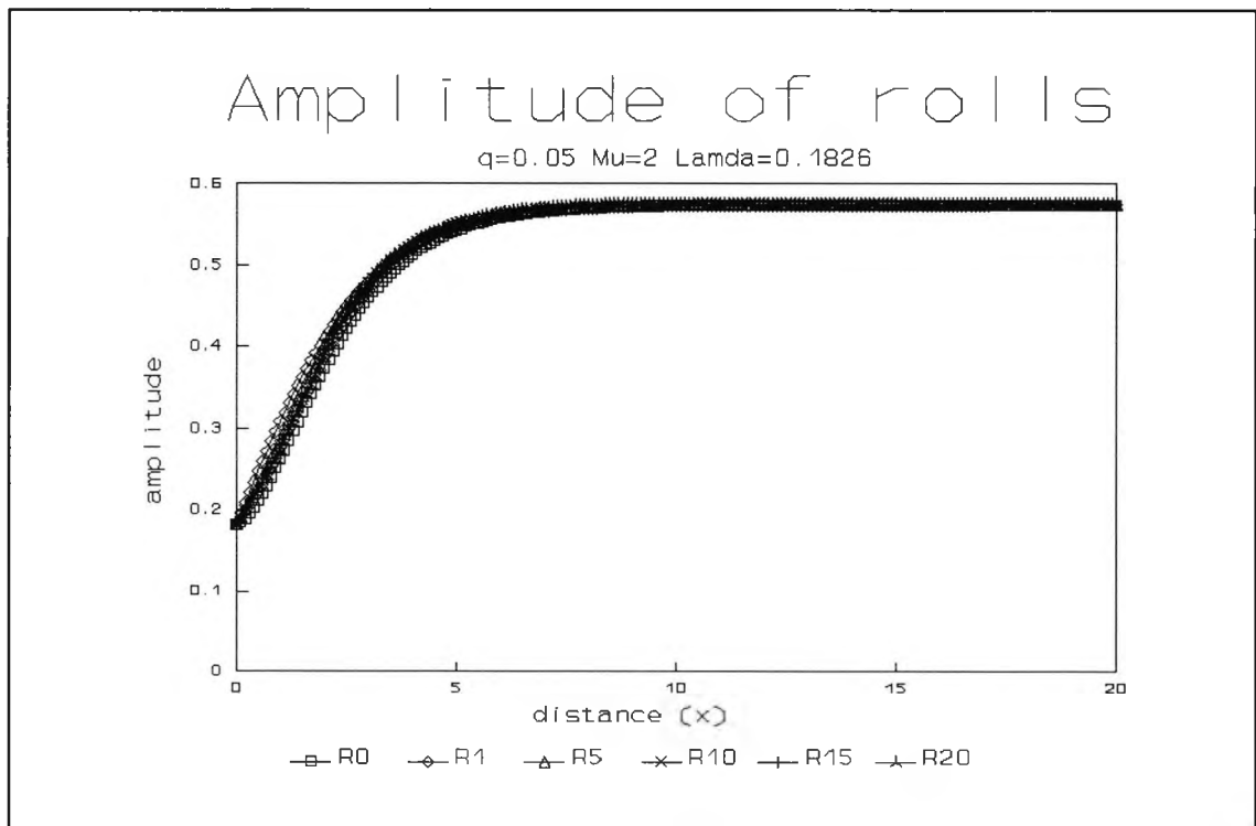
Fig. 4.10 : Numerical evolution for q=0.05 , \mu=2 and \lambda=0.1826 showing the amplitude of x-rolls at successive times \tau
