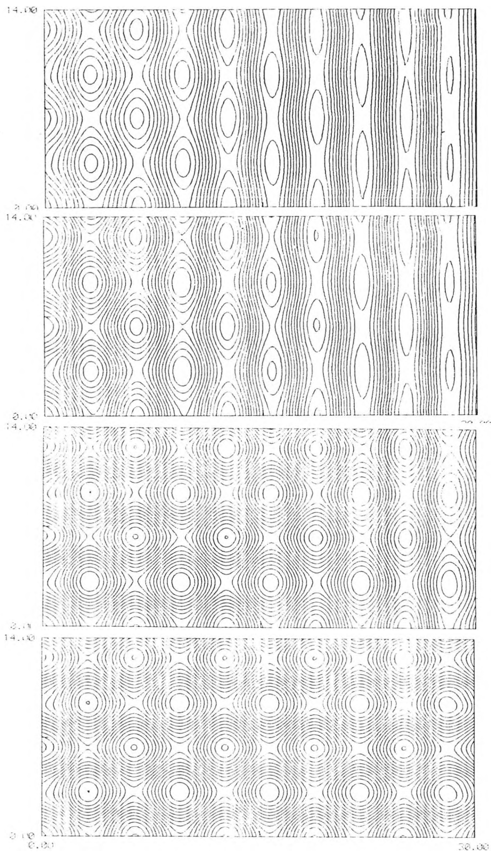
Fig. 2.32 : Contours of \psi at times \tau=0, 1, 5 and 20 for \mu=0.5, \lambda=0.5
