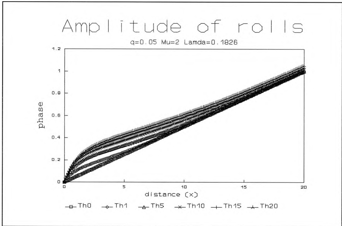
Fig. 4.11 : Numerical evolution for q=0.05 , \mu=2 and \lambda=0.1826 showing the phase of x -rolls at successive times \tau
