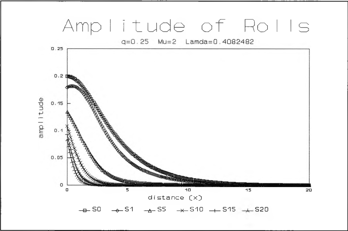
Fig. 4.51 : Numerical evolution for q=0.25 , \mu=2 and \lambda=0.4082 showing the amplitude of y -rolls at successive times \tau
