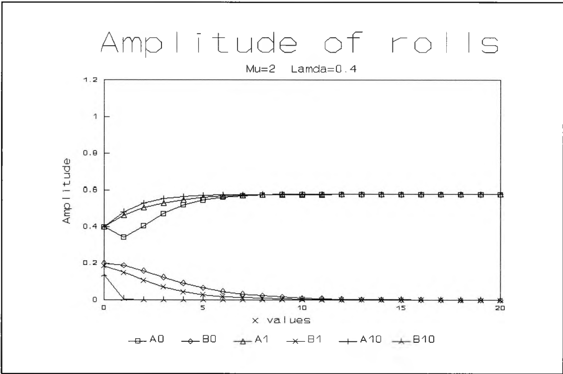
Fig. 2.14 : Numerical evolution for \mu=2.0 and \lambda=0.4 showing the amplitudes A and B of x -rolls and y -rolls at successive times \tau
