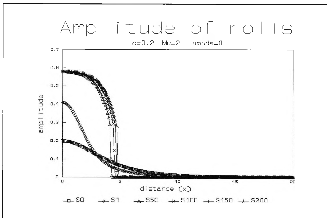
Fig. 4.30 : Numerical evolution for q=0.2 , \mu=2 and \lambda=0 showing the amplitude of y -rolls at successive times \tau
