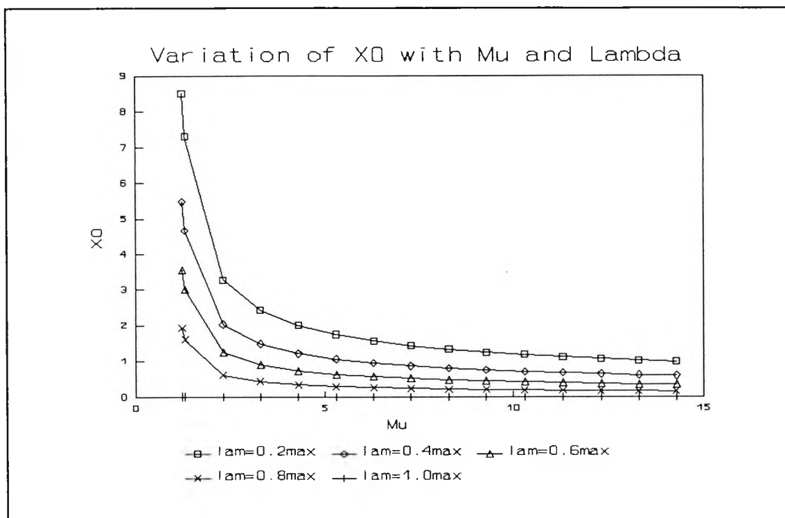
Fig. 2.2 : Variation of X_0 with \mu and \lambda
