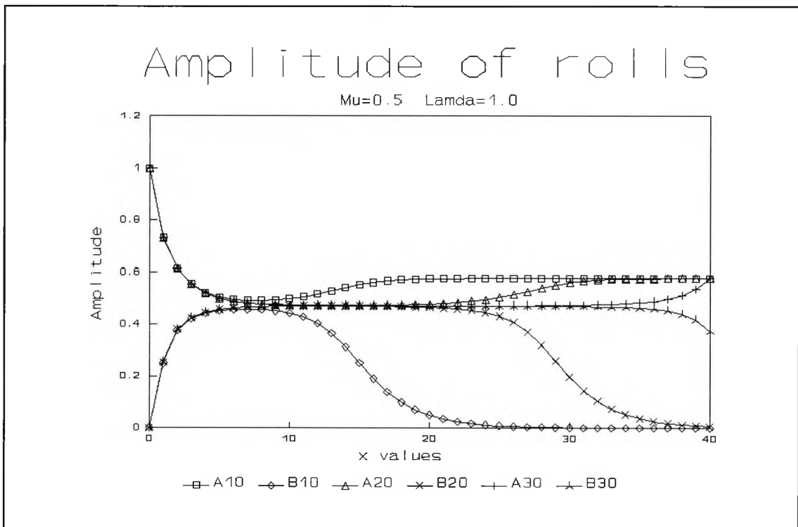
Fig. 2.21 : Numerical evolution for \mu=0.5 and \lambda=1.0 showing the amplitudes A and B of x -rolls and y -rolls at successive times \tau
