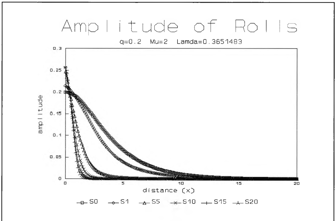
Fig. 4.36 : Numerical evolution for q=0.2 , \mu=2 and \lambda=0.3651 showing the amplitude of y -rolls at successive times \tau
