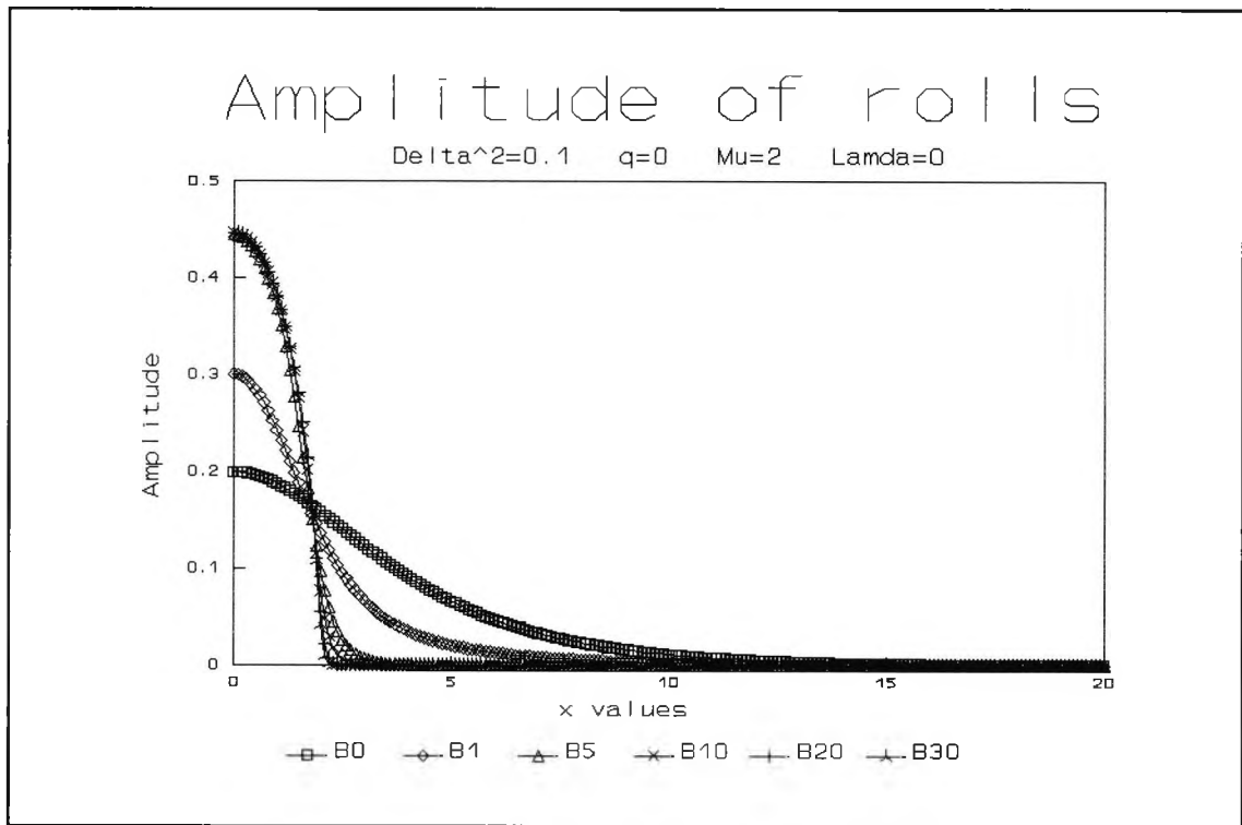
Fig. 5.3 : Amplitude of y-rolls with time when \delta^2=0.1 , q=0 , \mu=2 and \lambda=0
