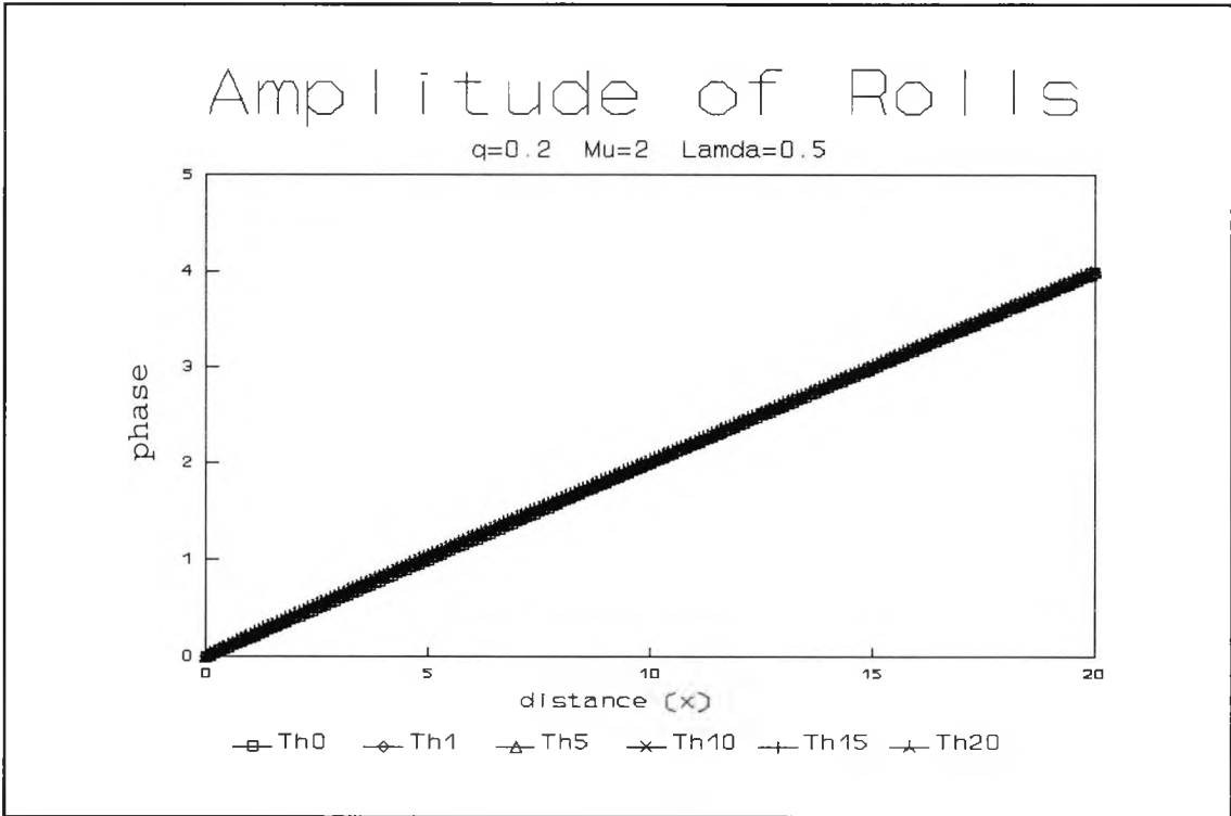
Fig. 4.41 : Numerical evolution for q=0.2 , \mu=2 and \lambda=0.5 showing the phase of x -rolls at successive times \tau
