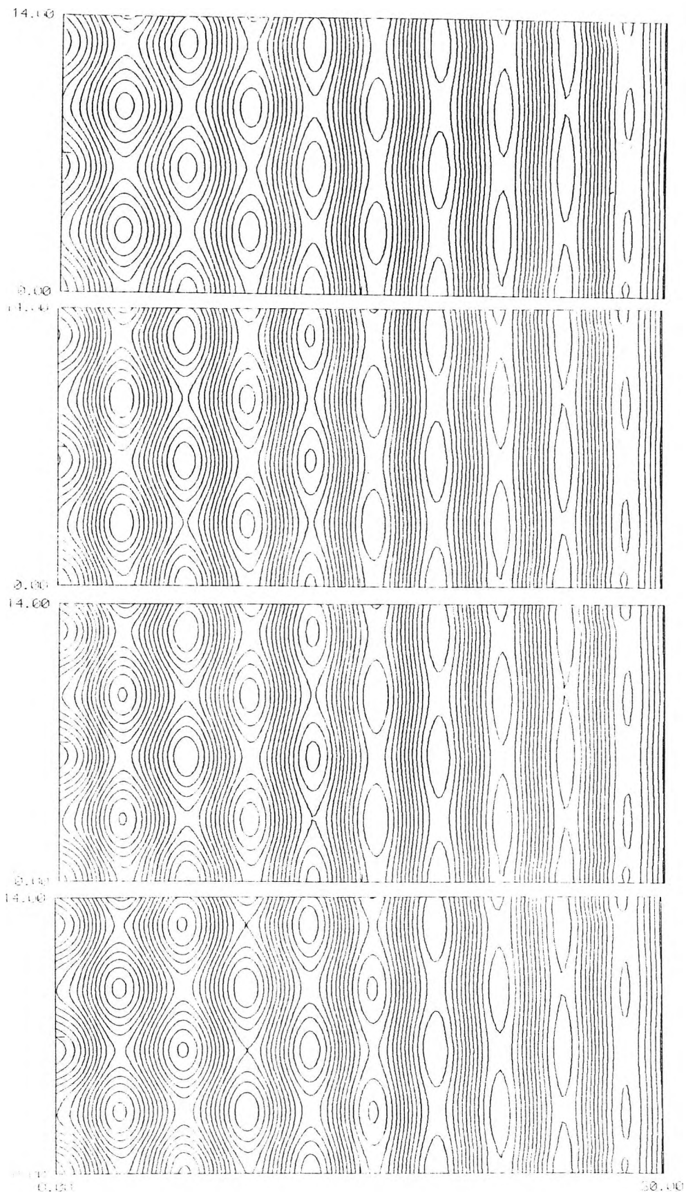
Fig. 2.36 : Contours of \psi at times \tau=0, 1, 5 and 20 for \mu=1.0, \lambda=0.5
