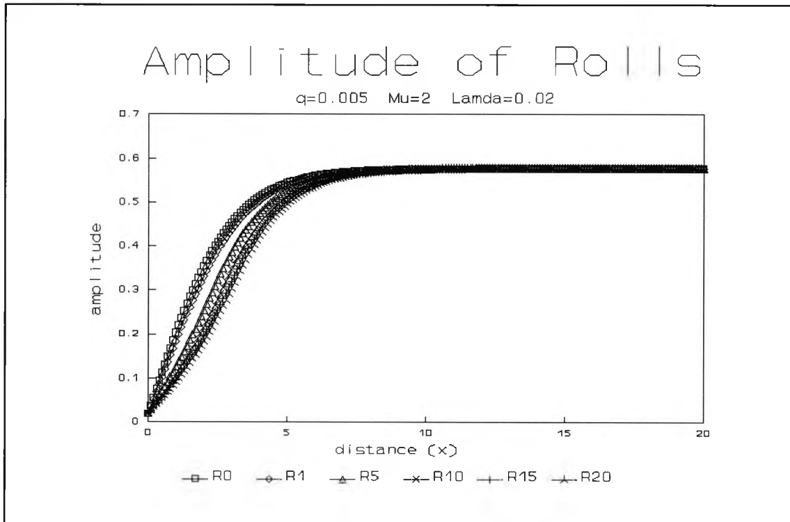
Fig. 4.58 : Numerical evolution for q=0.005 , \mu=2 and \lambda=0.02 showing the amplitude of x-rolls at successive times \tau
