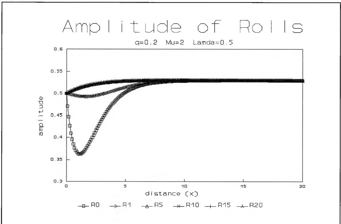
Fig. 4.40 : Numerical evolution for q=0.2 , \mu=2 and \lambda=0.5 showing the amplitude of x -rolls at successive times \tau
