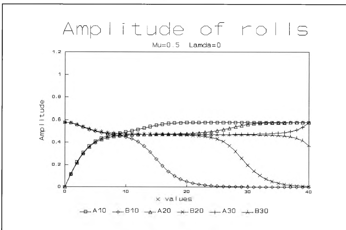
Fig. 2.19 : Numerical evolution for \mu=0.5 and \lambda=0 showing the amplitudes A and B of x -rolls and y -rolls at successive times \tau
