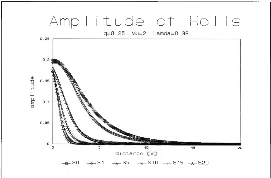
Fig. 4.48 : Numerical evolution for q=0.25 , \mu=2 and \lambda=0.39 showing the amplitude of y -rolls at successive times \tau
