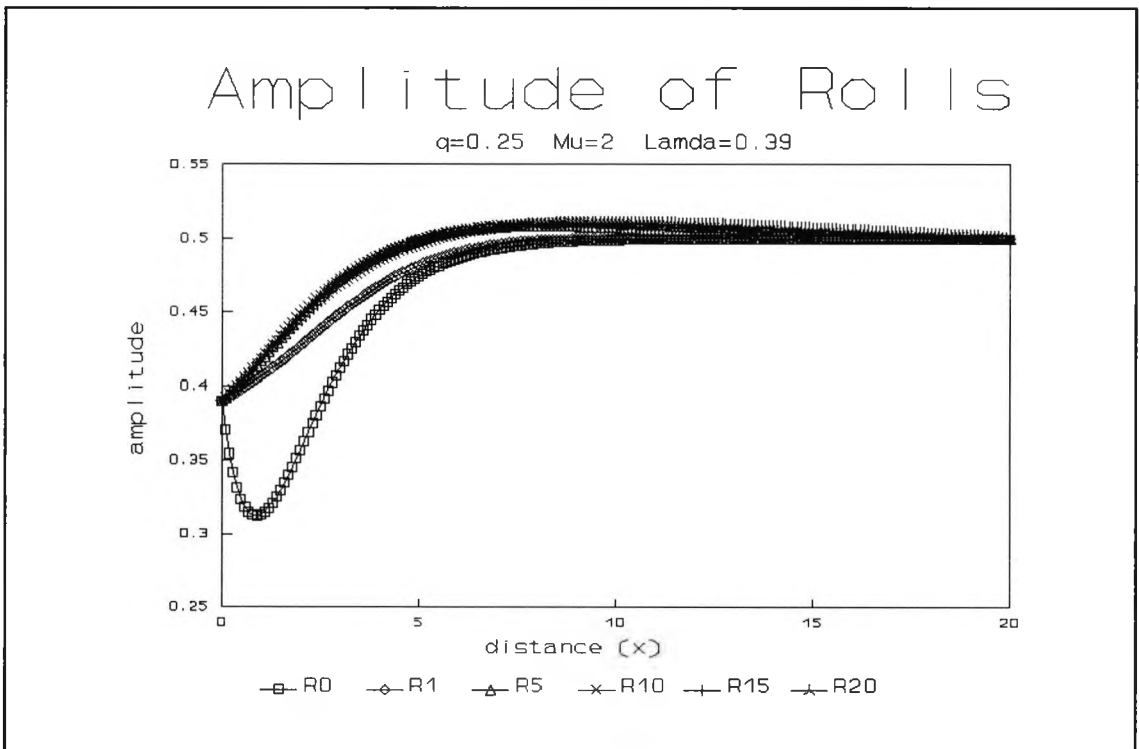
Fig. 4.46 : Numerical evolution for q=0.25 , \mu=2 and \lambda=0.39 showing the amplitude of x -rolls at successive times \tau
