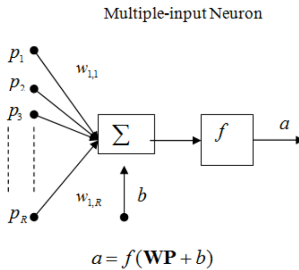
Figure 2.5 Multiple-input Neuron
