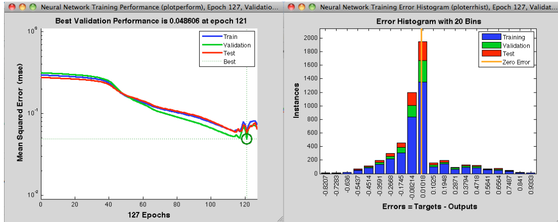
Figure 4.9 Training performance and error histogram: the classification of five classes
