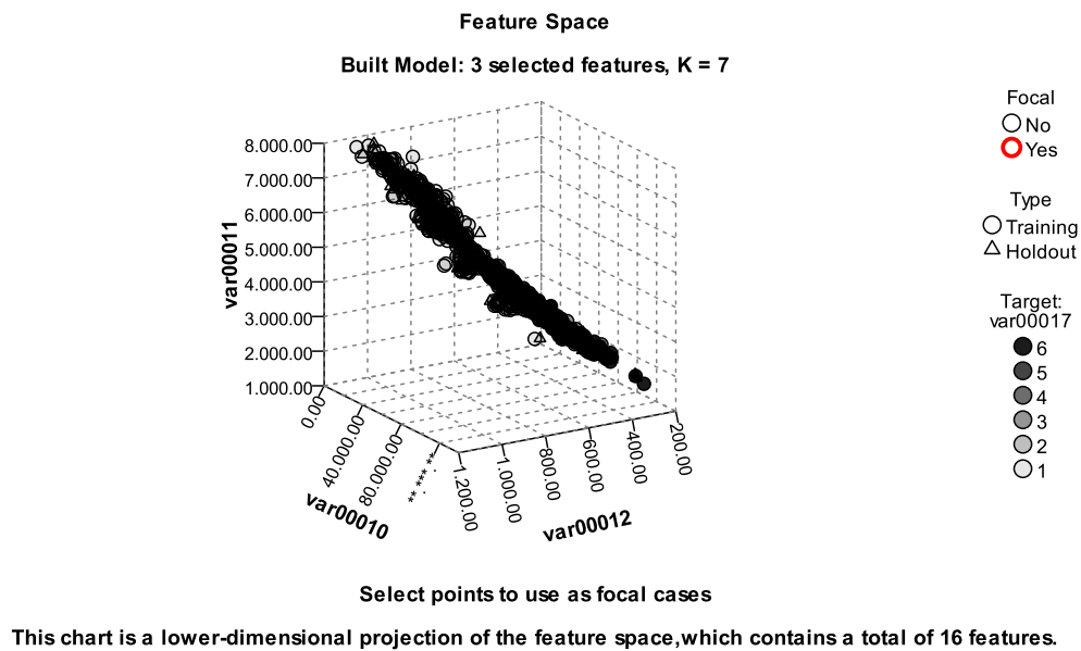
Figure 4.18 KNN feature space – classification of six classes
