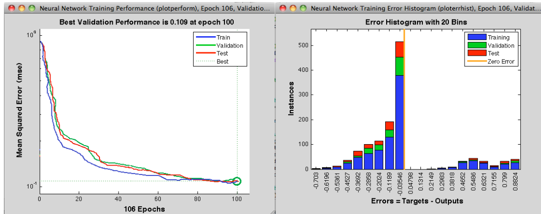
Figure 4.4 Training performance and error histogram: the binary classification of the class four
