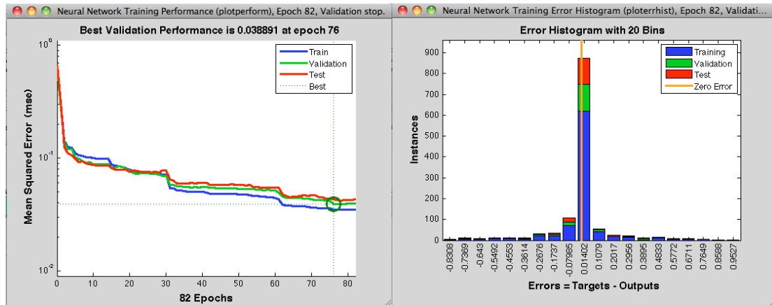
Figure 4.3 Training performance and error histogram: the binary classification of the class three
