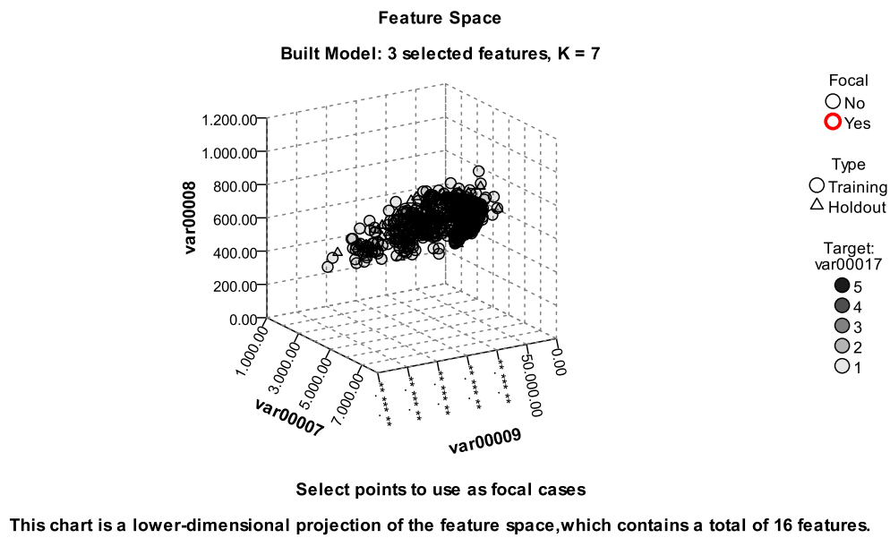
Figure 4.17 KNN feature space – classification of five classes
