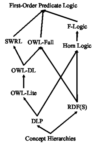
Figure 2: Some ontology languages. Arrows indicate inclusions between the languages. Concept hierarchies are simple is-a hierarchies corresponding to certain fragments of propositional logic. The standard OWL [2; 23] already comes in different versions. DLP [14; 29] refers to a weak but practically interesting datalog fragment of OWL. F-Logic [20; 1] provides an alternative ontology paradigm.
