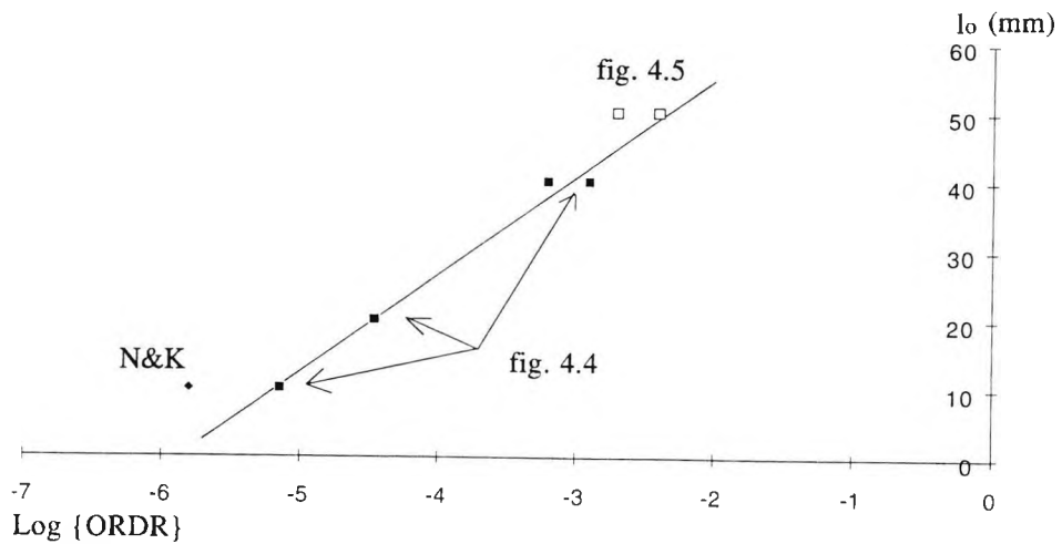
Figure 4.9: Relationship between orifice length and [\text{ORDR}]_{\text{crit}}
