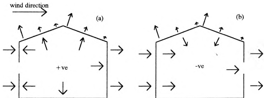
Figure 1.1: Influence of a windward and leeward opening on internal pressure
