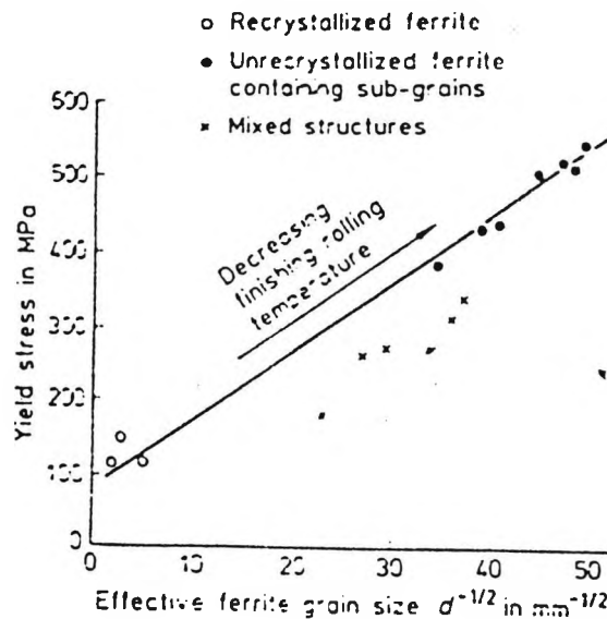
Figure 2.3: The effect of the 'effective' ferrite grain size on the yield stress of controlled rolled steel [21] .
