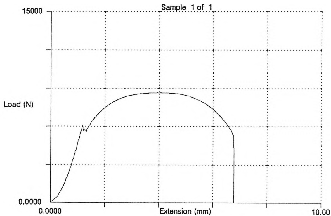
Figure 4.10: Stress-strain curve for sample oil quenched and tempered at 600°C.
