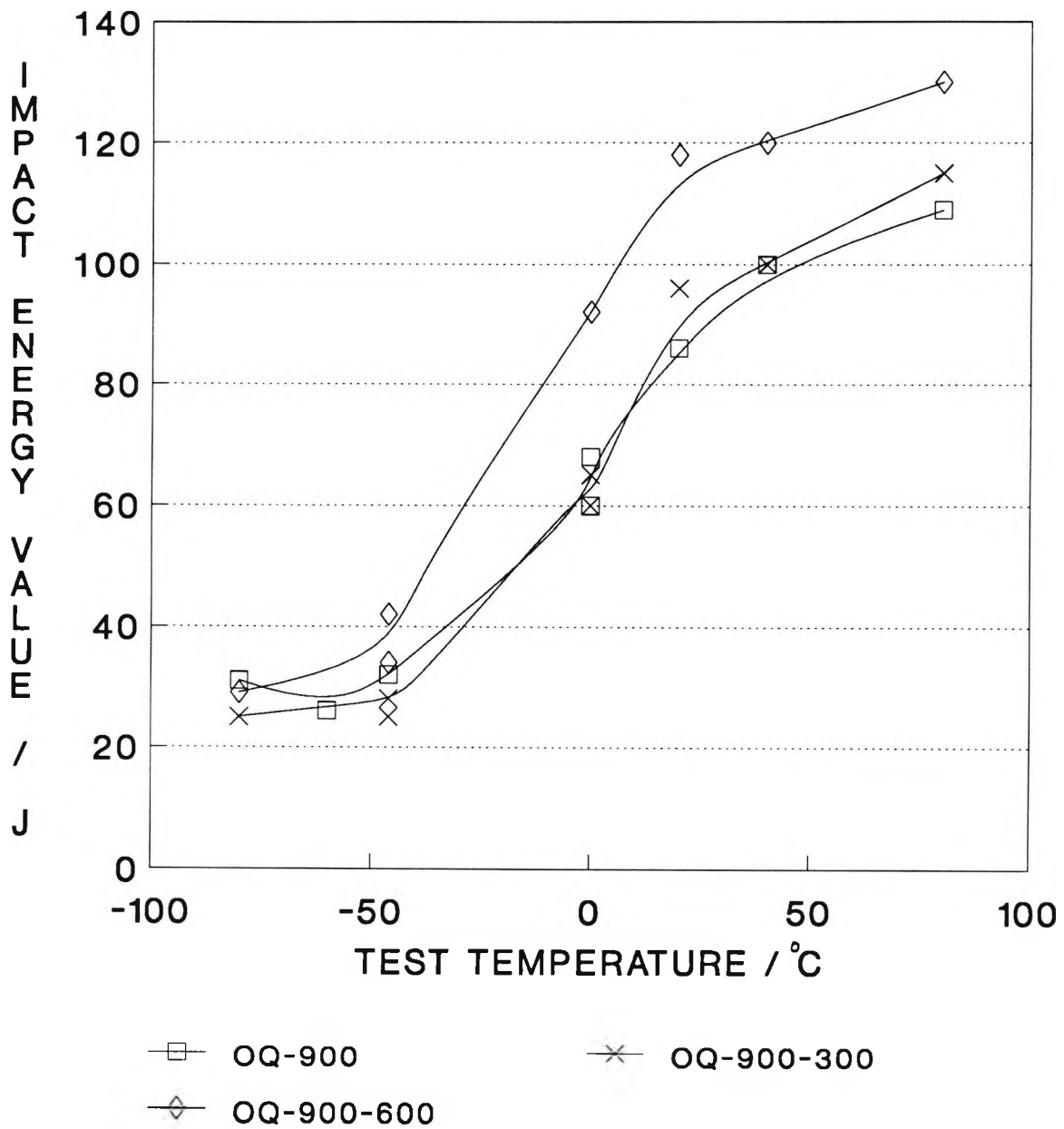
Fig 5.5 IMPACT TRANSITION CURVES FOR OIL QUENCHED SAMPLES FROM 900 °C.
