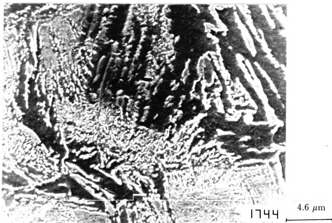
Figure 5.17: Microstructure of steel flanges ice-water quenched from 900°C after holding for 1 hour. (SEM)
