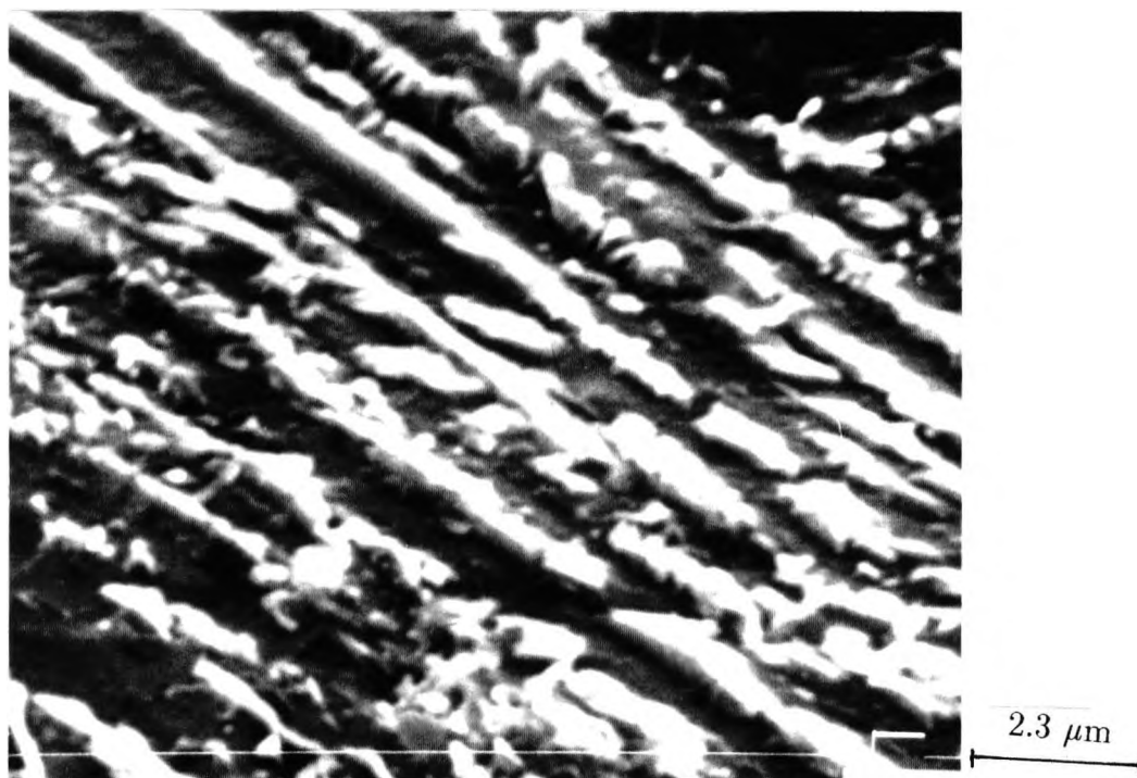
Figure 4.17: Microstructure of steel flanges ice-water quenched from 950°C. (SEM)
