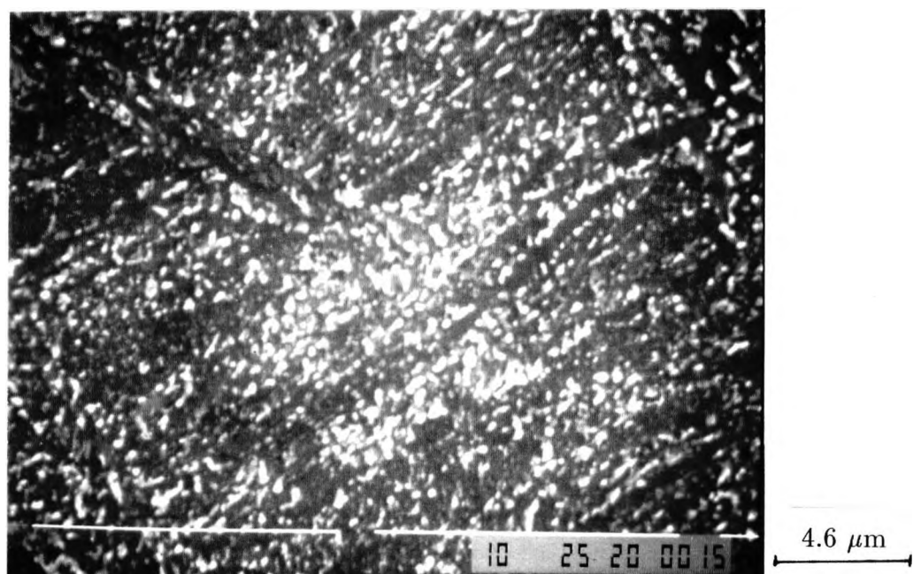
Figure 5.21: Microstructure of steel flanges ice-water quenched from 1250°C and tempered at 600°C. (SEM)
