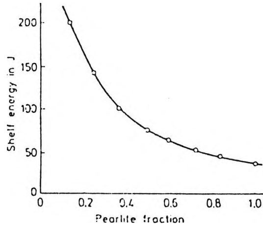
Figure 2.18: The effect of the pearlite volume fraction on the shelf energy in normalized ferrite- pearlite microstructures [58] .
