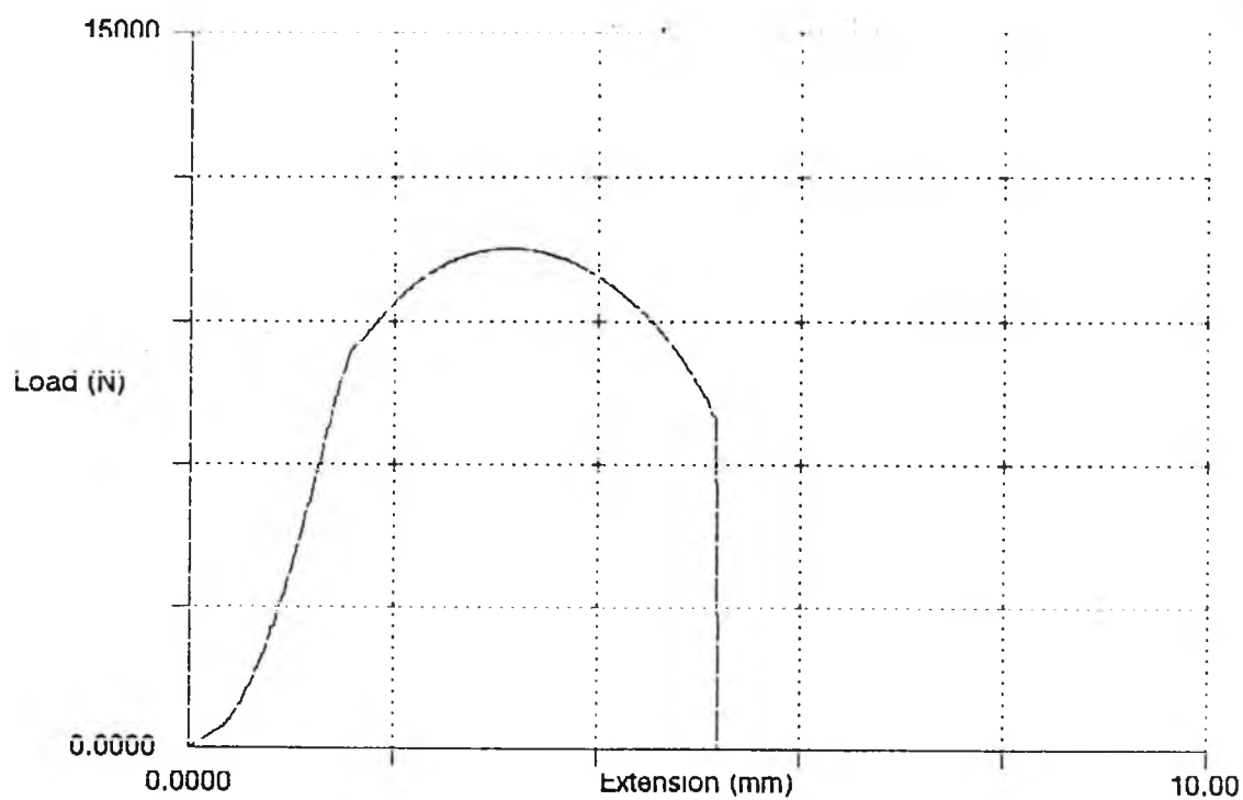
Figure 4.6: Stress-strain curve for sample ice-water quenched and tempered at 600°C.
