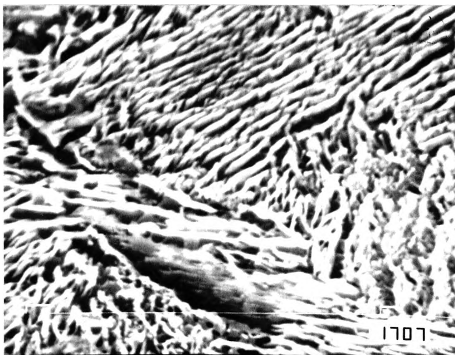
Enlarged view of carbide in second phase region
