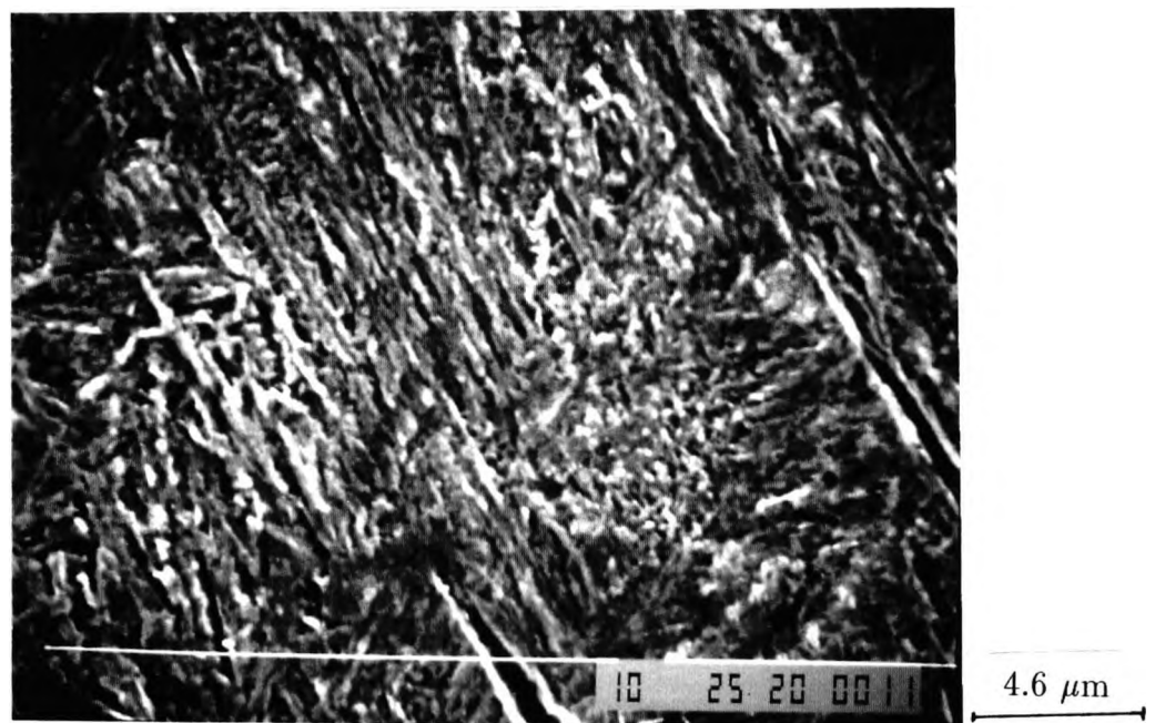
Figure 5.20: Microstructure of steel flanges ice-water quenched from 1250°C and tempered at 300°C. (SEM)
