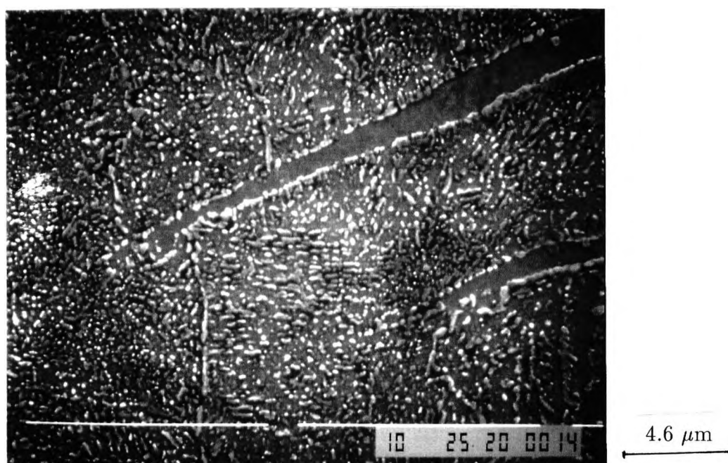
Figure 5.26: Microstructure of steel flanges oil-quenched from 1250°C and tempered at 600°C.
