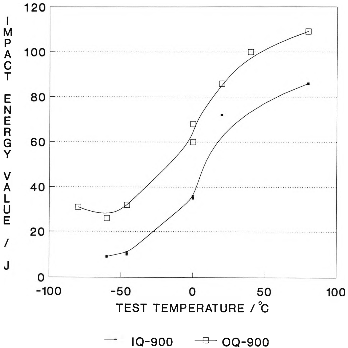
Fig 5.34 IMPACT TRANSITION CURVES FOR SAMPLES ICE-WATER AND OIL QUENCHED FROM 900 °C
