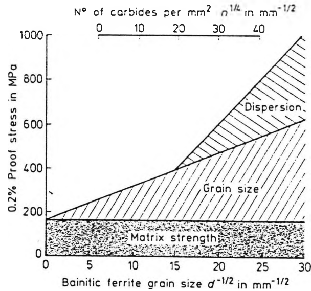
Figure 2.22: The contributions of the bainitic ferrite grain size and the carbide dispersion strengthening to the 0.2% proof stress of low carbon bainitic microstructures containing 0.05-0.15 wt.% C [25] .
