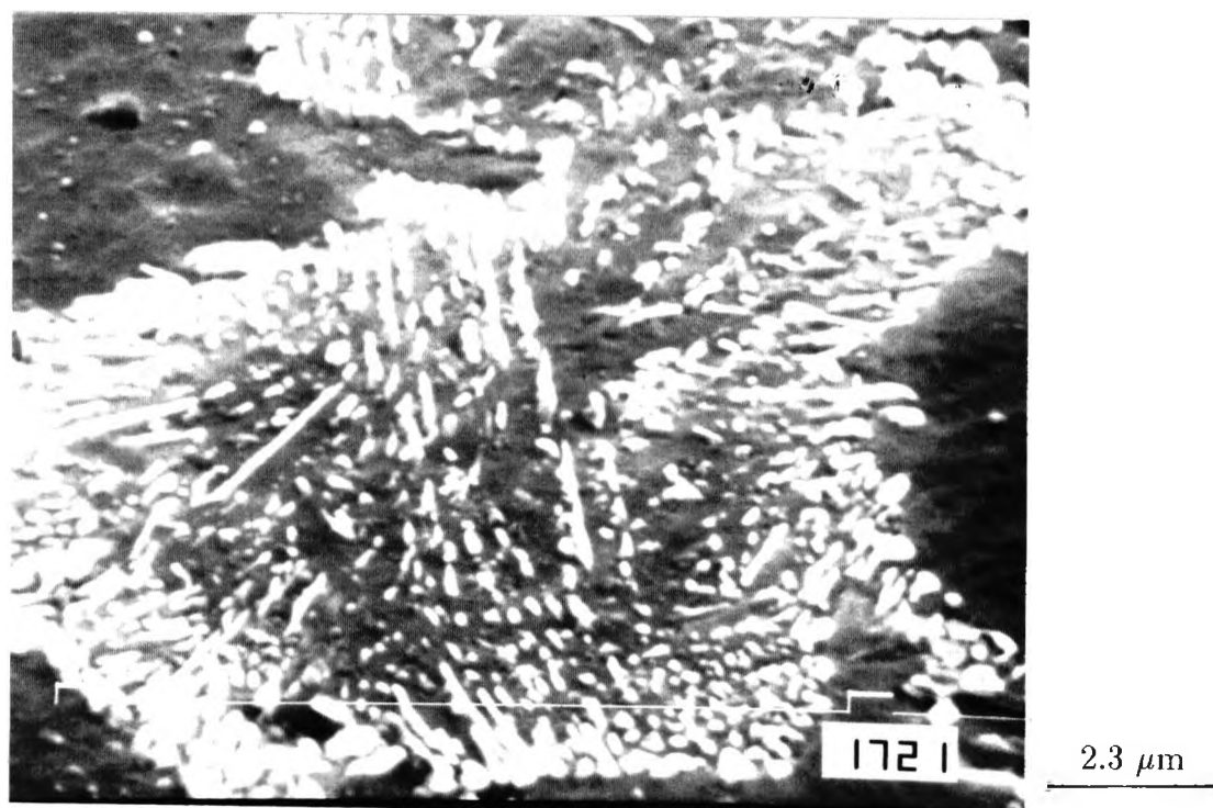
Figure 4.14: Partial spheroidisation of carbides when tempered at 600°C for 1 hour. Steel was oil quenched from 950°C. (SEM)
