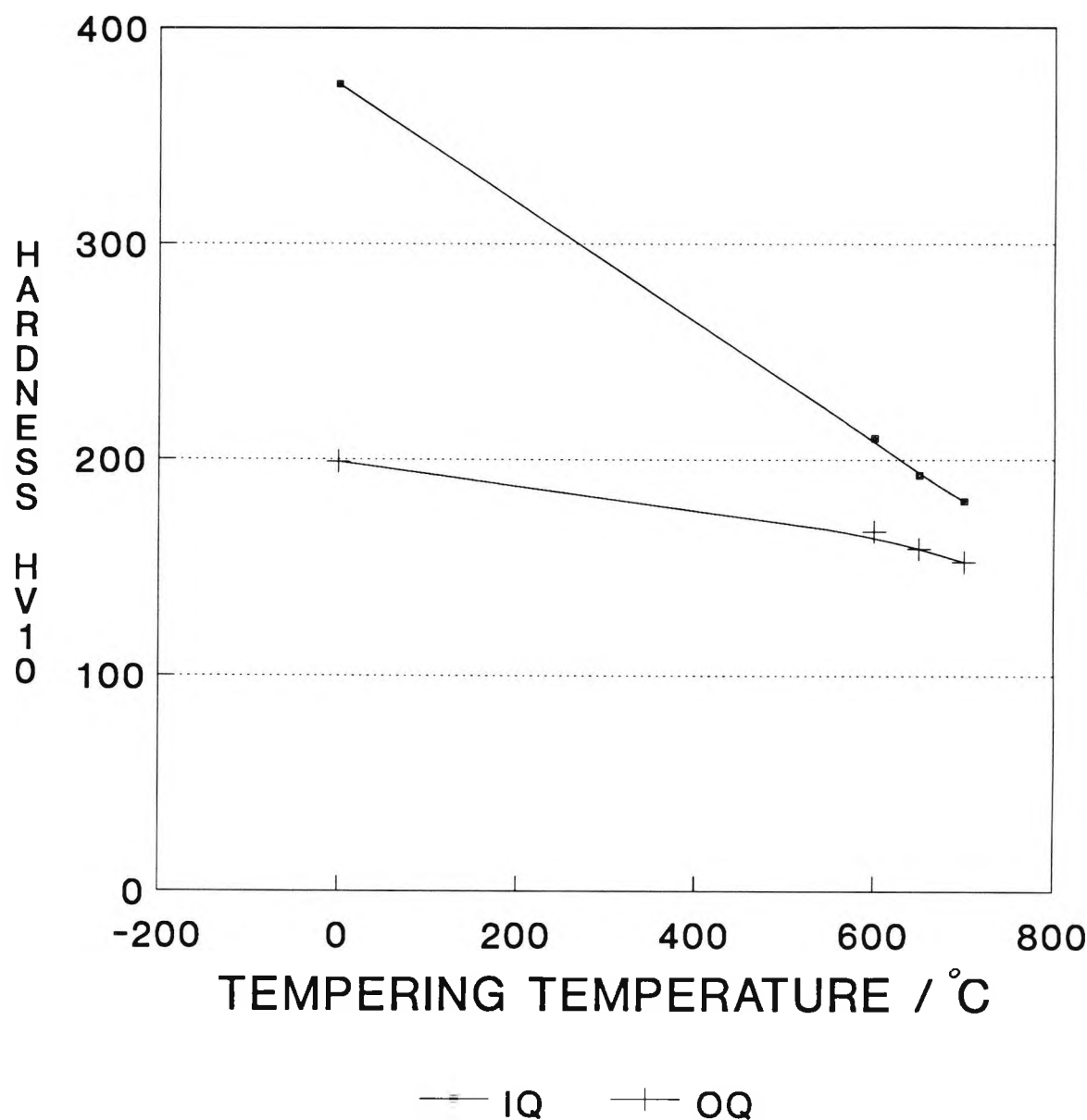
Fig 4.8 Effect of tempering on hardness of samples ice-water or oil quenched from 950 °C (0 = AQ)
