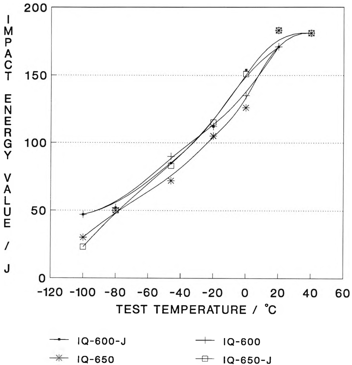
Figure 4.21: Impact transition curves for samples ice-water quenched from 950°C as compared with previous work [8] . Previous work by Kolahi-aval is denoted by letter J.
