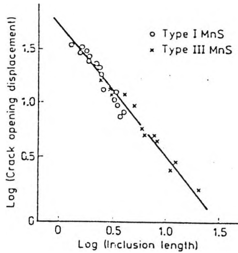
Figure 2.13: The relationship between the inclusion length and the fracture toughness measured by the crack opening displacement [47] .
