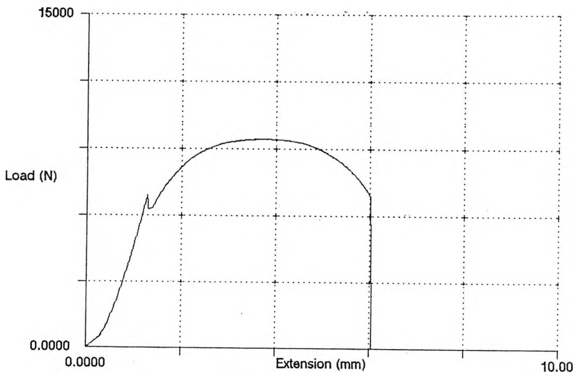
Figure 5.7: Stress/strain curve for the flange oil quenched and tempered at 300°C.
