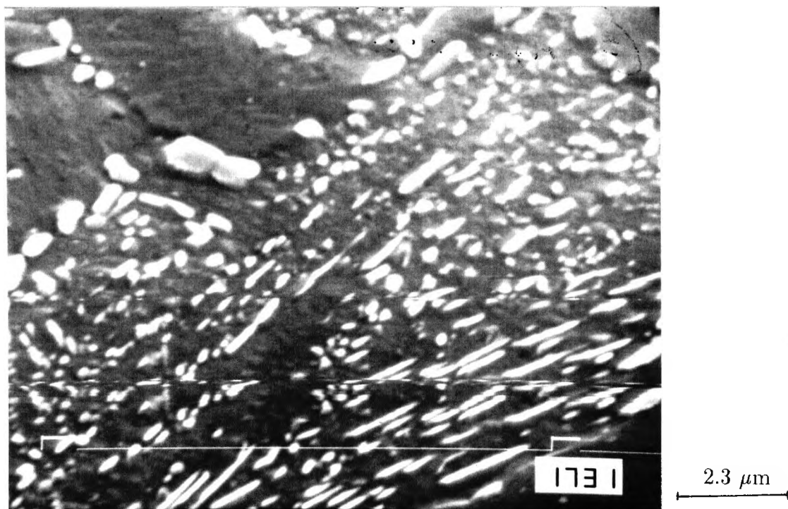
Figure 4.15: Partial spheroidization when tempered at 650°C for 1 hour. Steel was oil quenched from 950°C after holding for 1 hour. (SEM)
