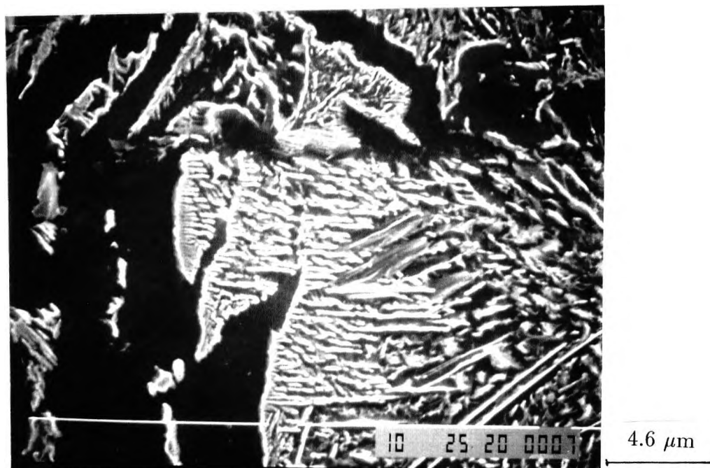
Figure 5.25: Microstructure of steel flanges oil quenched from 1250°C and tempered at 300°C.
