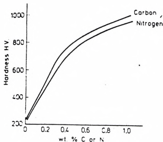
Figure 2.26: The effect of carbon or nitrogen on the hardness of quenched fully martensitic microstructures [78] .
