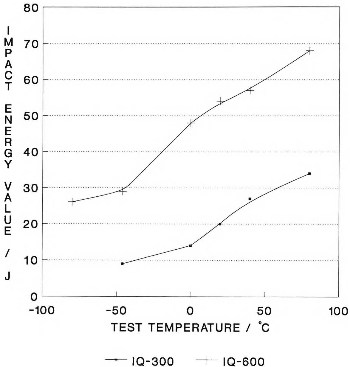
Fig 5.22 IMPACT TRANSITION CURVES FOR SAMPLES ICE-WATER QUENCHED FROM 1250 °C AND TEMPERED.
