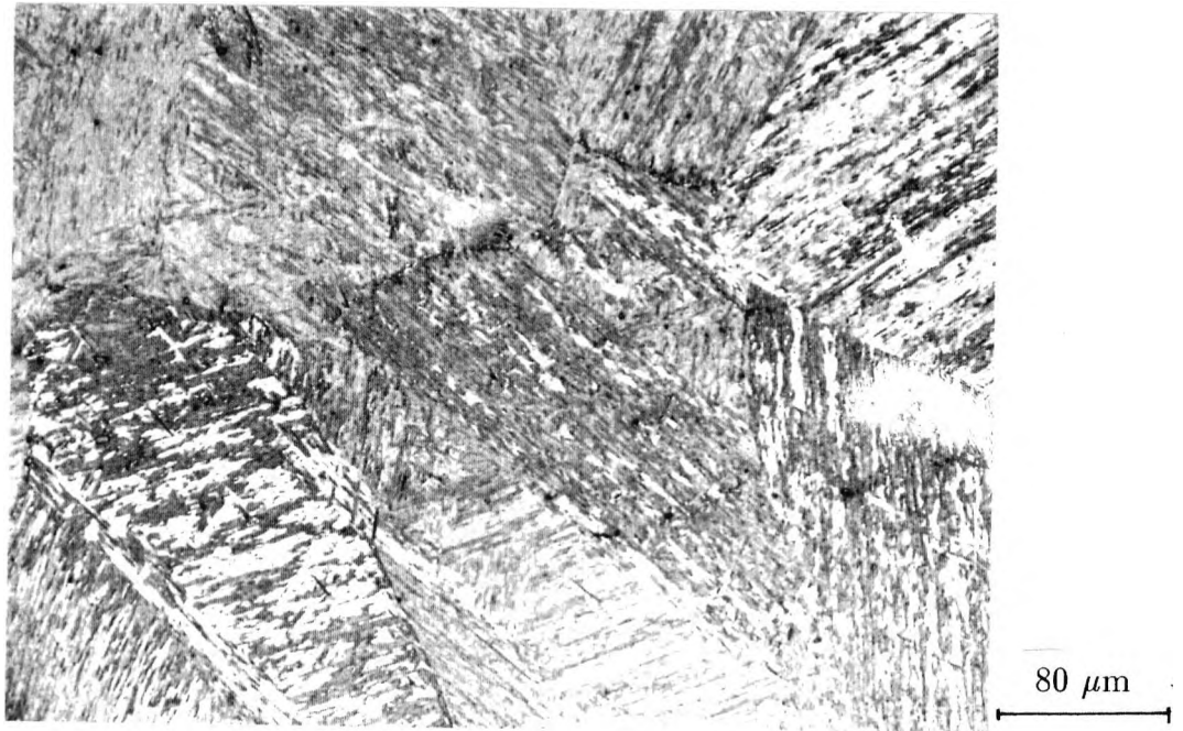
Figure 5.3: Microstructure of steel flanges ice-water quenched from 1250°C after holding for 1 hour. (optical)
