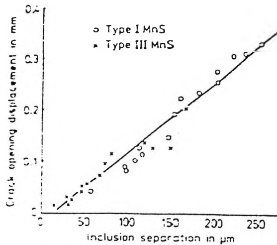
Figure 2.14: The relationship between the separation between inclusions and the fracture toughness measured by the crack opening displacement [48] .
