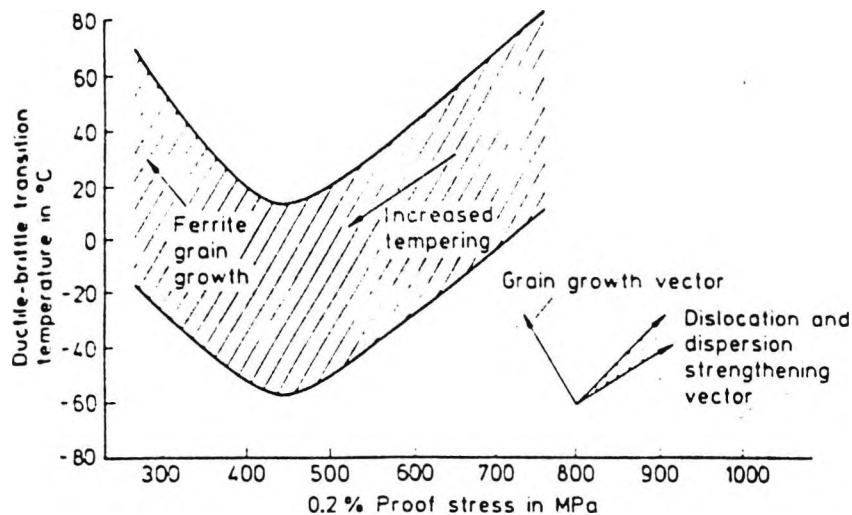
Figure 2.31: The effect of tempering on the relationship between the 0.2% proof stress and the ductile-brittle transition temperature for low carbon bainitic microstructures, showing the effect of different strengthening mechanisms [34] .
