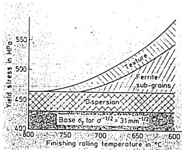
Figure 2.4: The effect of controlled rolling finishing temperature on the contributions of various strengthening mechanisms to the yield stress of ferrite [22] .
