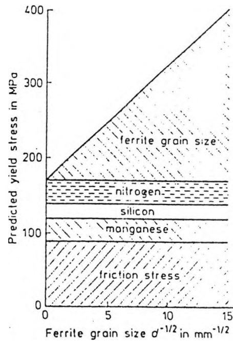
Figure 2.5: The effect of ferrite grain size on the yield stress of normalized steel containing 0.20 wt.%C, 1.0 wt.% Mn, 0.20 wt.%si, 0.010wt.%N [23] .
