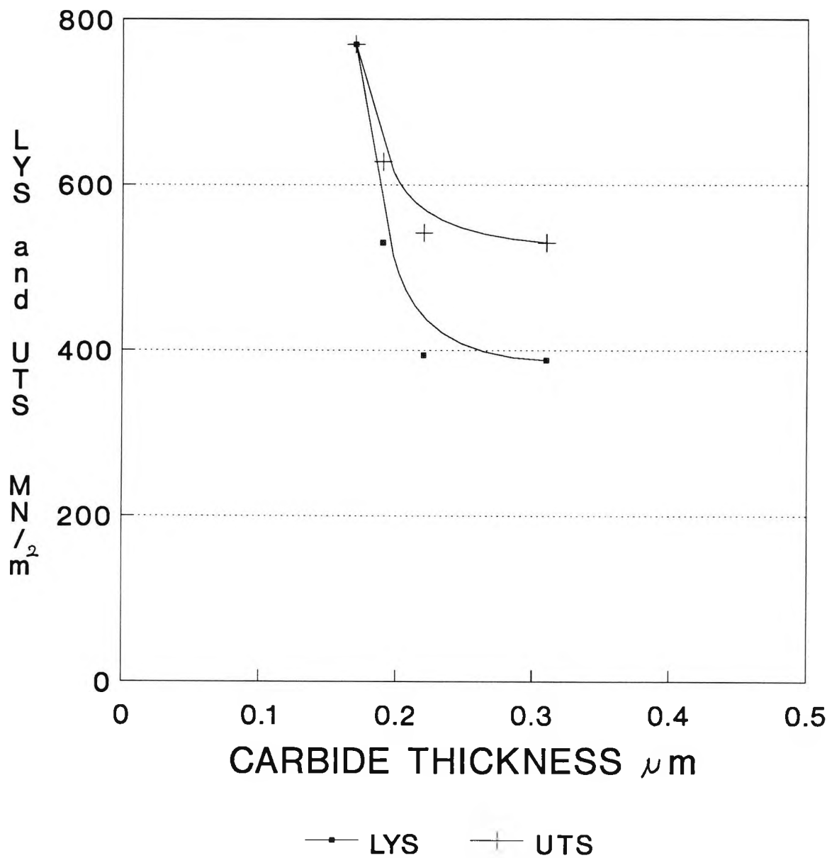
FIG 4.29 Variation of LYS and UTS with carbide thickness for ice-water quenched samples on tempering
