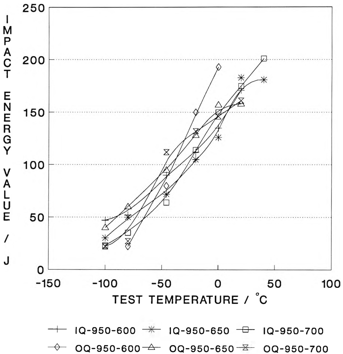
Fig 4.4 Impact transition curves for samples ice-water or oil quenched from 950 °C and tempered.
