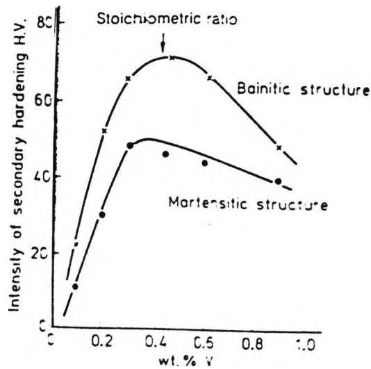
Figure 2.28: The effect of vanadium on the intensity of the secondary hardening in tempered 0.1 wt.% C steels comprising prior bainitic or martensitic microstructures, showing the maximum effect at the stoichiometric ratio [90] .
