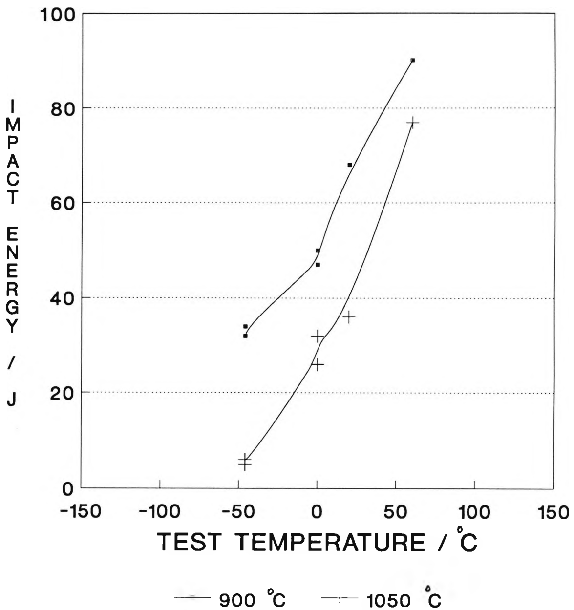
FIG 6.2 IMPACT TRANSITION CURVES FOR Al CONTAINING STEEL
