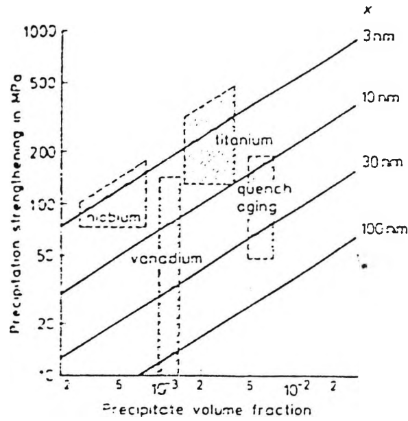
Figure 2.6: Dispersion strengthening as predicted by a modified Ashby-Orowan model compared with the observed strengthening by quench aging and by microalloy carbonitrides [25] .
