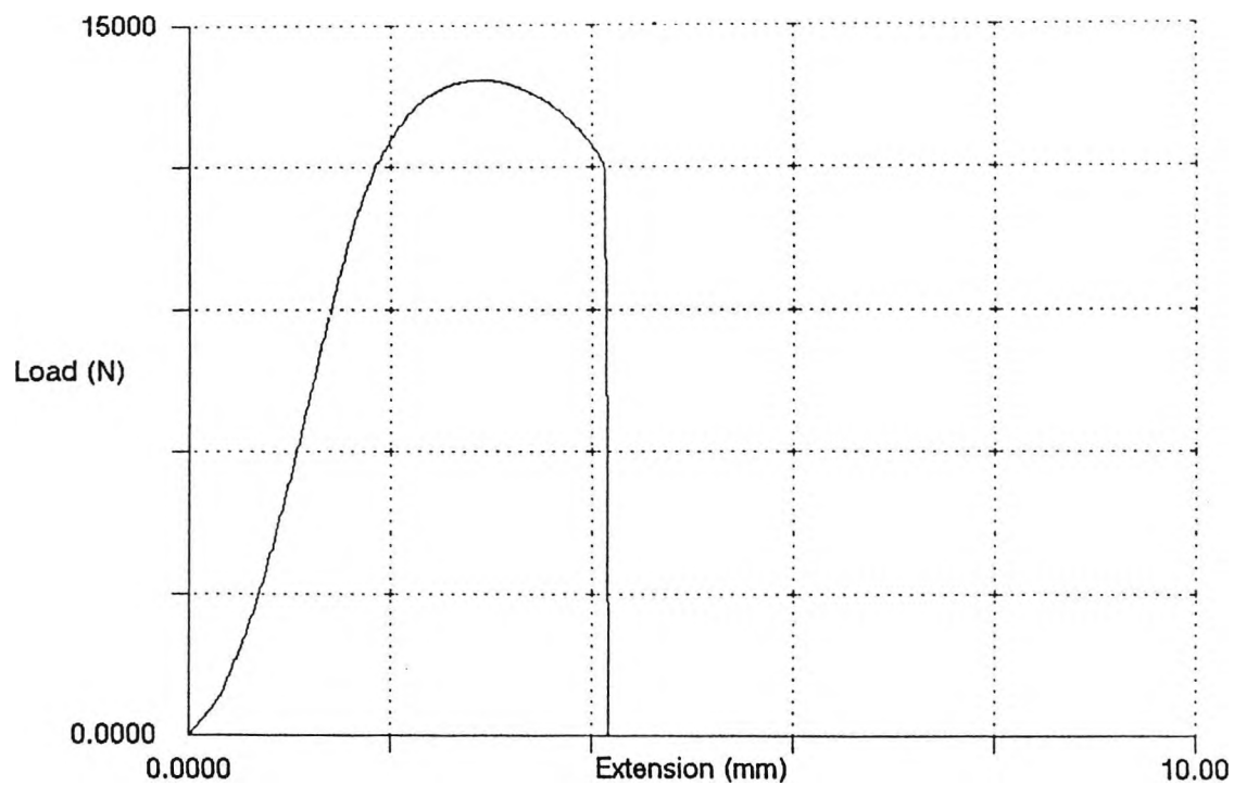
Figure 4.5: Stress-strain curve for sample ice-water quenched from 950°C.
