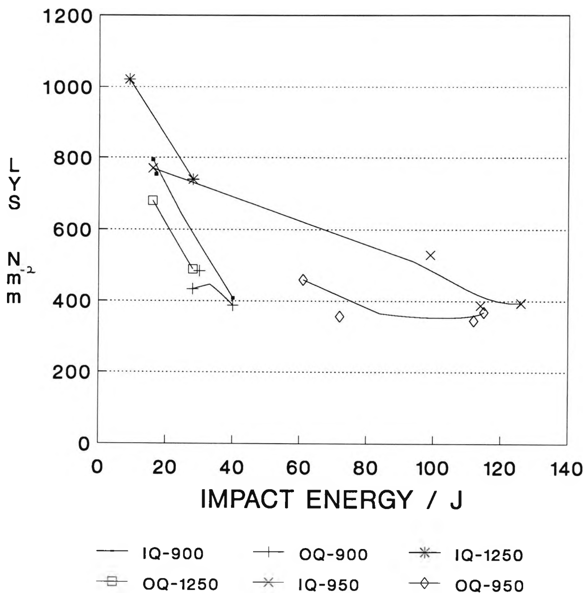
FIG 5.46 Variation of impact energy at -46°C with changes in strength on tempering
