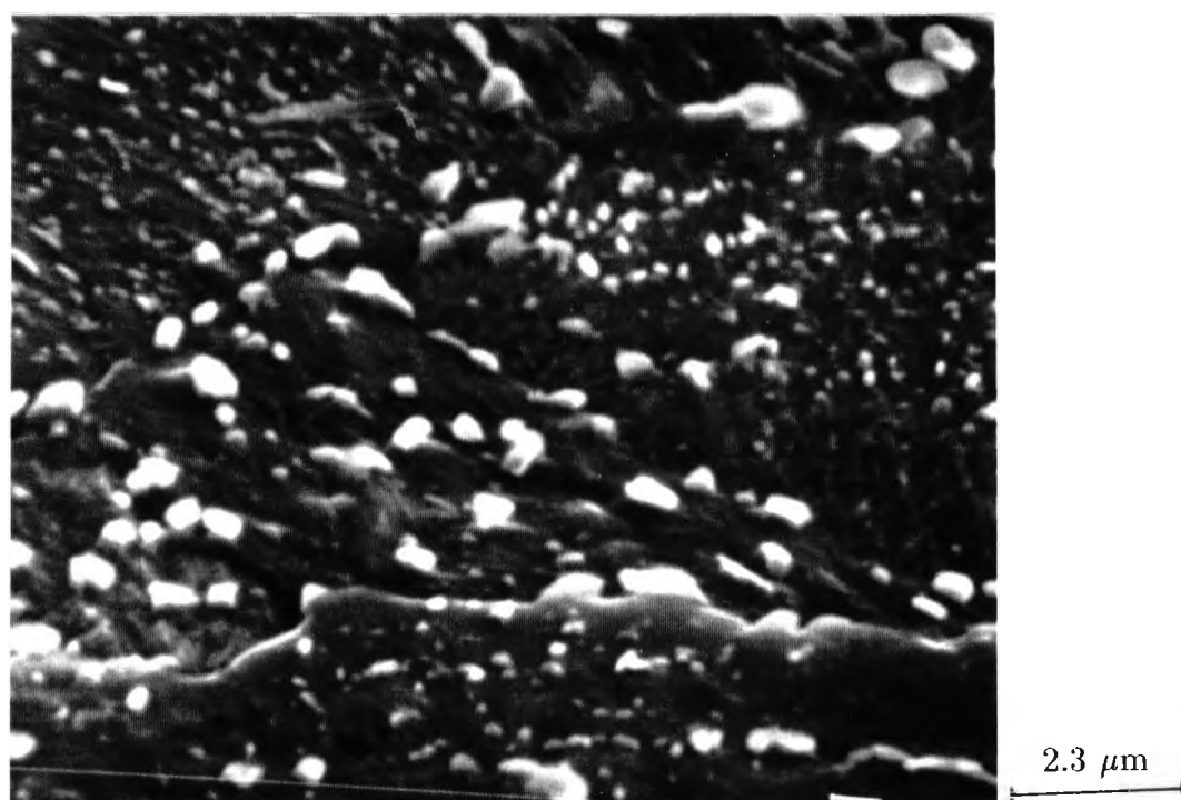
Figure 4.20: microstructure of steel flanges ice-water quenched from 950° C after holding for 1 hour and tempered at 700° C for 1 hour. (SEM)
