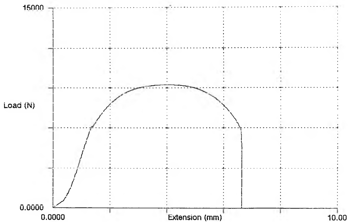
Figure 4.9: Stress-strain curve for sample oil quenched from 950°C.
