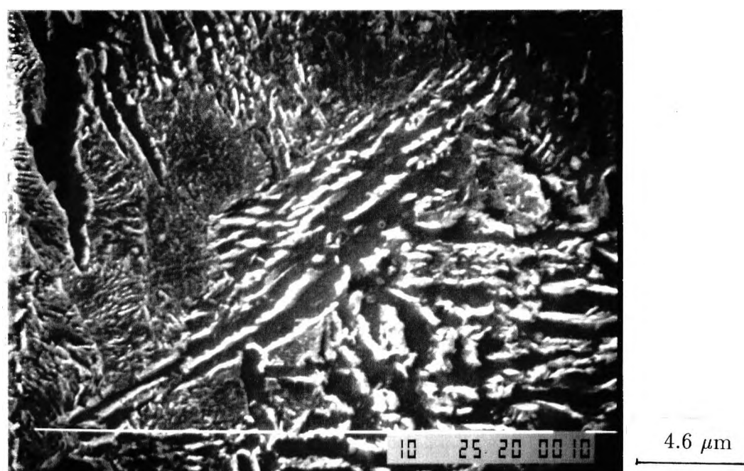
Figure 5.18: Microstructure of steel flanges ice-water quenched from 900°C and tempered at 300°C for 1 hour. (SEM)
