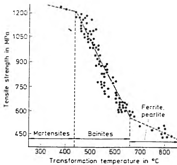
Figure 2.21: The relationship between the transformation temperature and the tensile strength in low carbon bainitic microstructures containing 0.05-0.15 wt.% C [62] .
