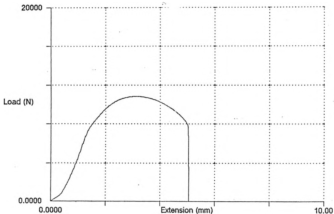
Figure 5.28: Stress/strain curve of the flange oil quenched from 1250°C and tempered at 300°C.
