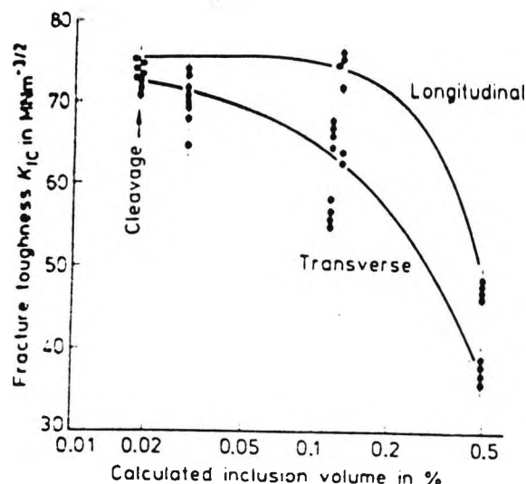
Figure 2.34: The effect of the non-metallic inclusion content on the fracture toughness parameter ( K_{1C} ) for a quenched and tempered high strength steel, showing the anisotropy of toughness [96] .
