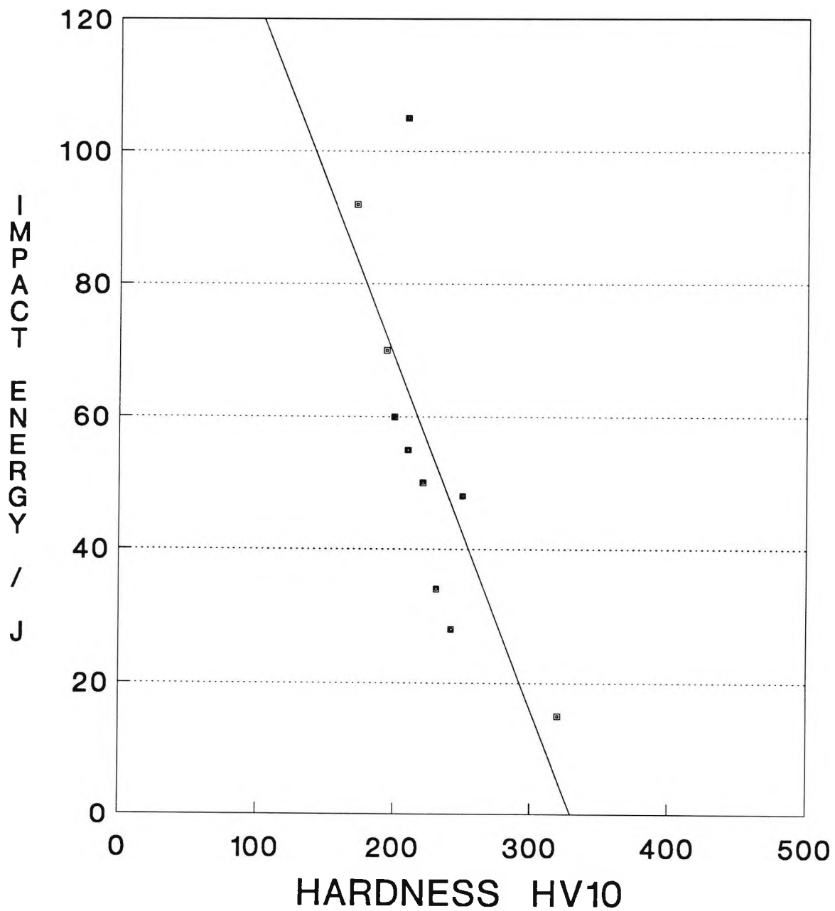
FIG 5.33 VARIATION OF IMPACT ENERGY WITH HARDNESS
