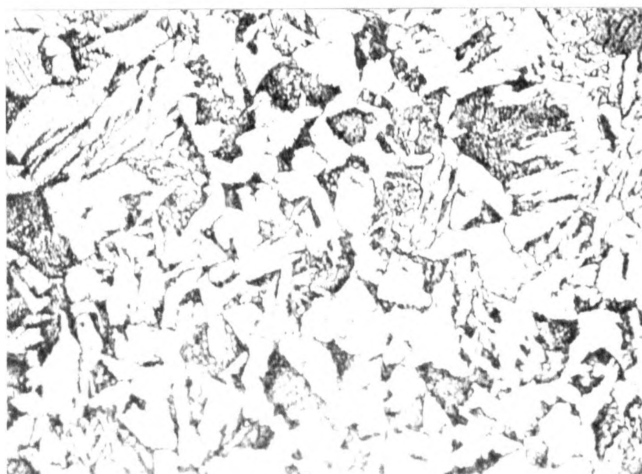
Fig 4.11 Microstructure of steel flanges oil quenched from 950 °C. (optical)
