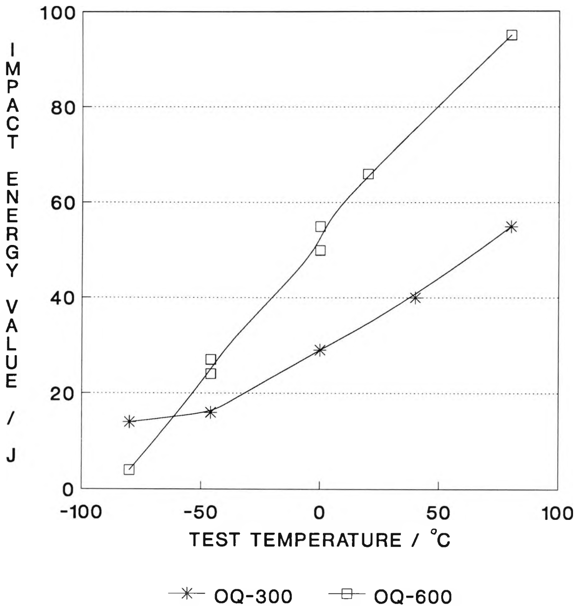
Fig 5.27 IMPACT TRANSITION CURVES FOR SAMPLES OIL QUENCHED FROM 1250 °C AND TEMPERED.
