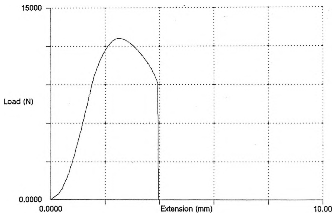
Figure 5.14: Stress/strain curve for the flanges ice-water quenched from 900°C after holding for 1 hour.
