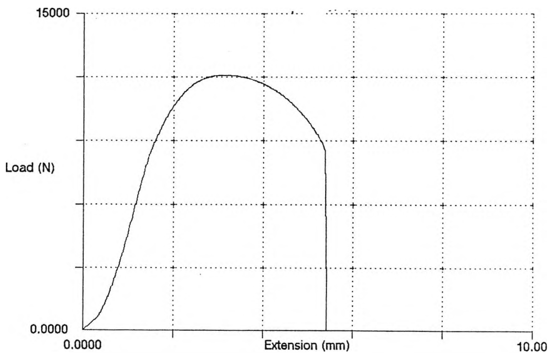
Figure 5.15: Stress/strain curve for the flange ice-water quenched and tempered at 300°C.
