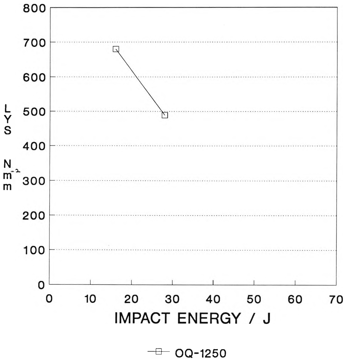
Figure 5.45: Variation of impact energy at -46^{\circ}\text{C} with changes in strength on tempering for flanges oil quenched from 1250^{\circ}\text{C} .
