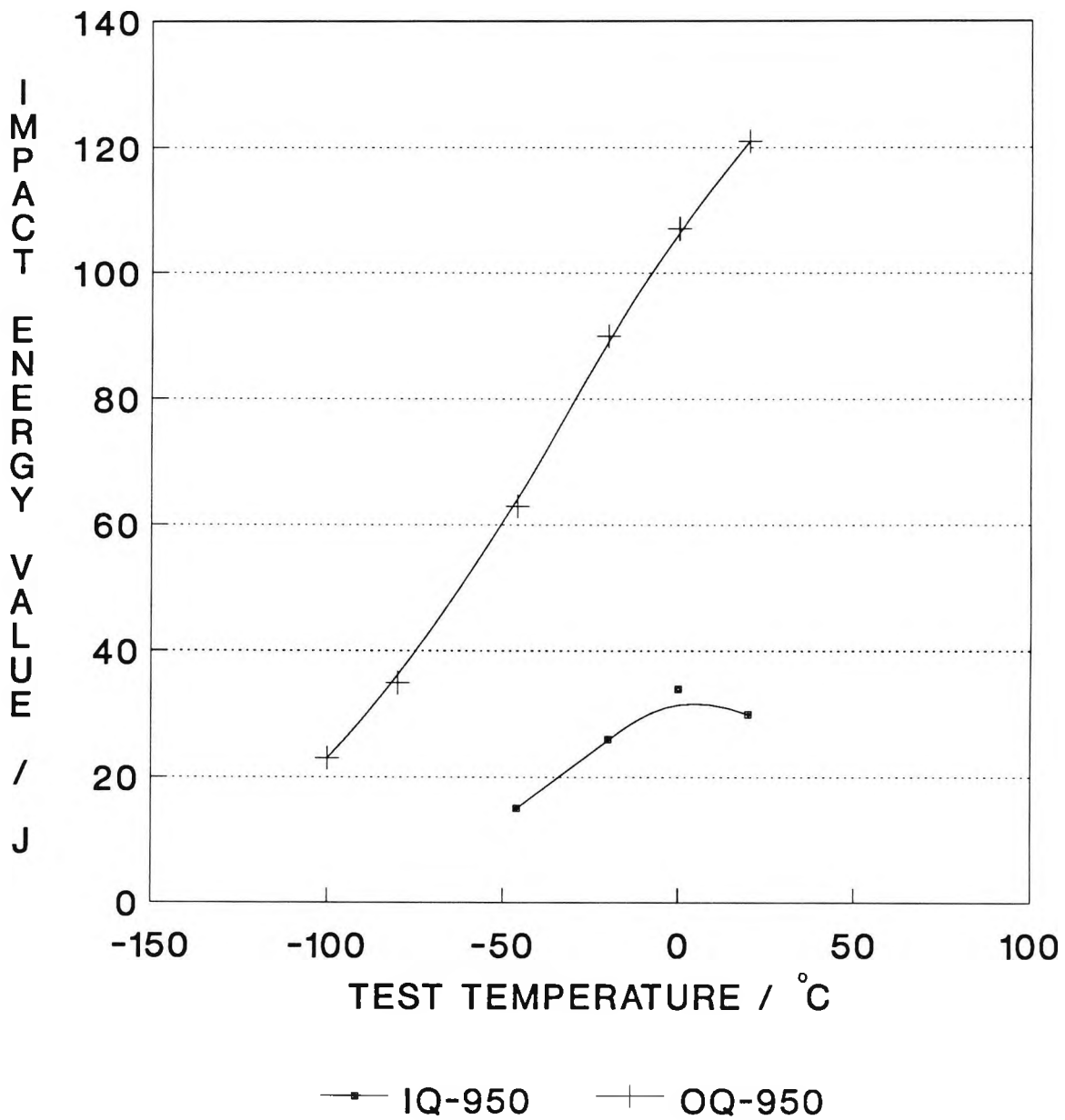
Fig 4.3 Impact transition curves for samples ice-water or oil quenched from 950 °C.
