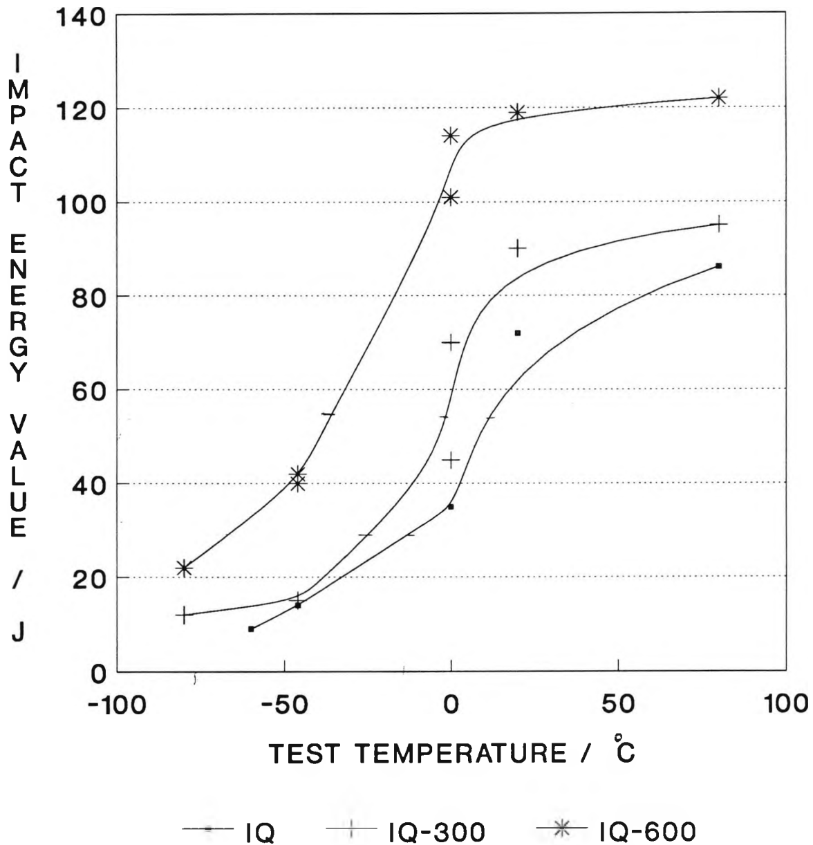
Fig 5.13 Impact transition curves for samples ice-water quenched from 900 °C
