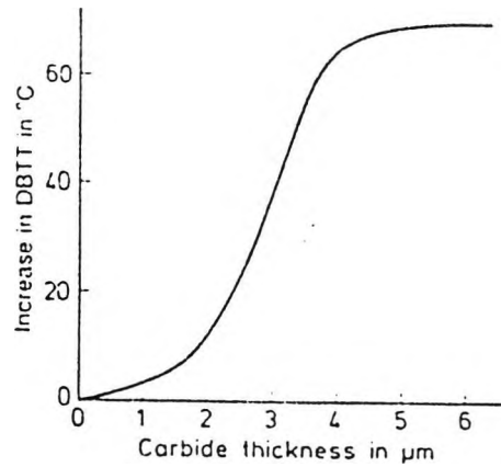
Figure 2.9: The effect of carbide thickness on the ductile-brittle transition temperature (DBTT) [33] .
