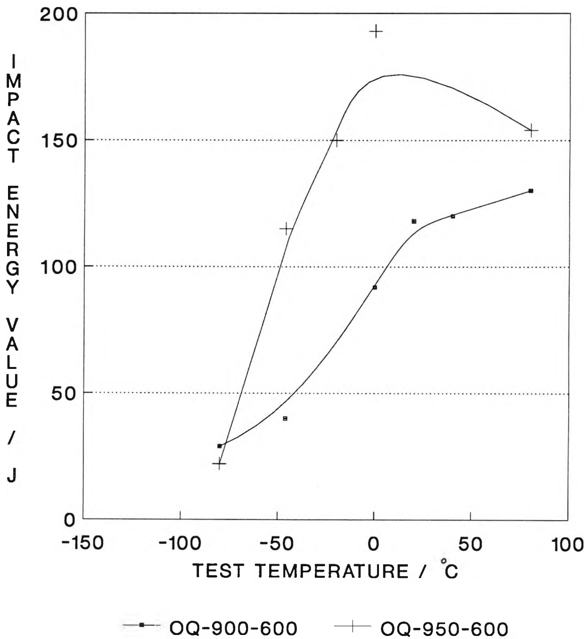
Figure 5.38: Impact transition curves for oil quenched flanges from 950 or 900°C and tempered at 600°C.
