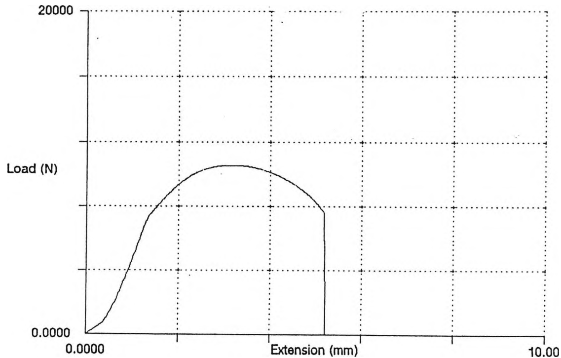
Figure 5.29: Stress/strain curve of the flange oil quenched from 1250°C and tempered at 600°C.
