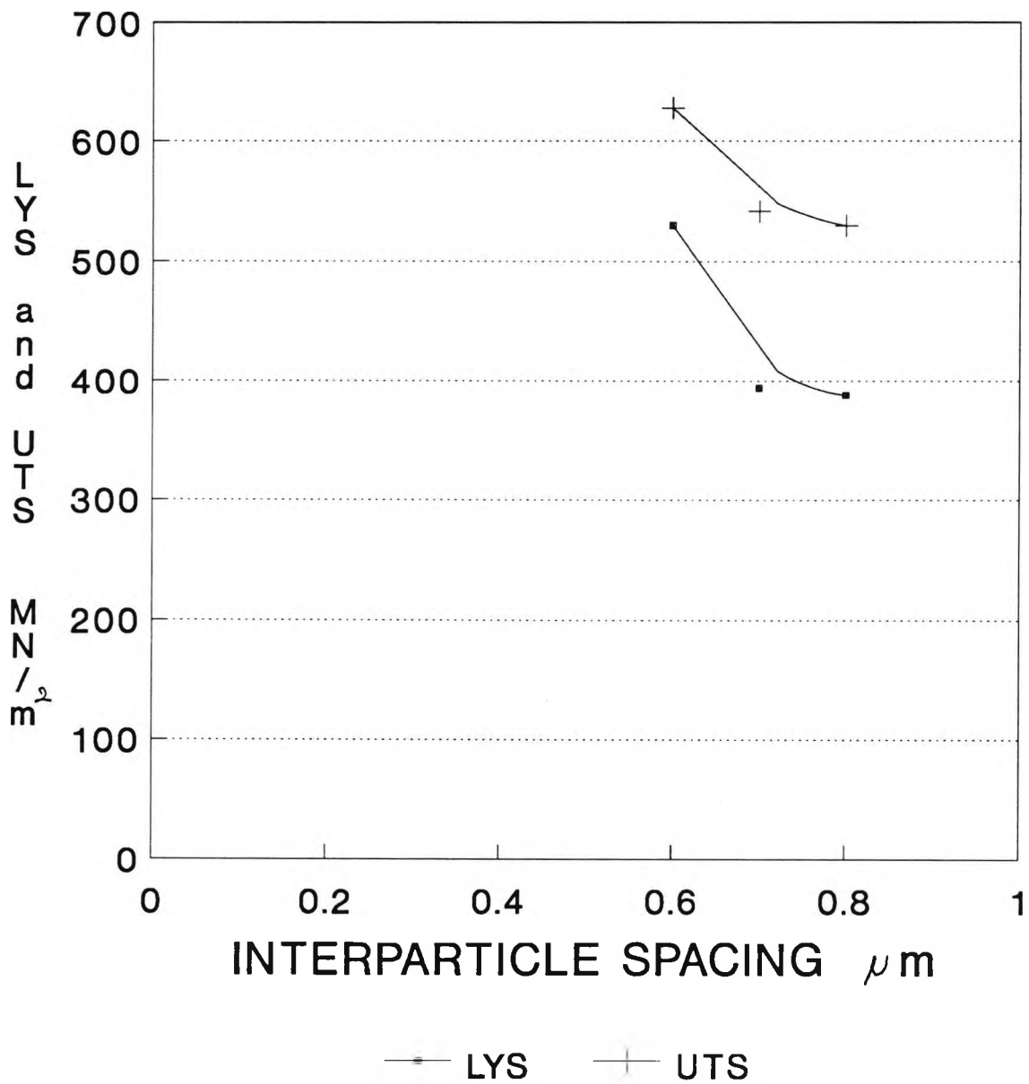
FIG 4.30 Variation of LYS and UTS with interparticle spacing for ice-water quenched samples during tempering
