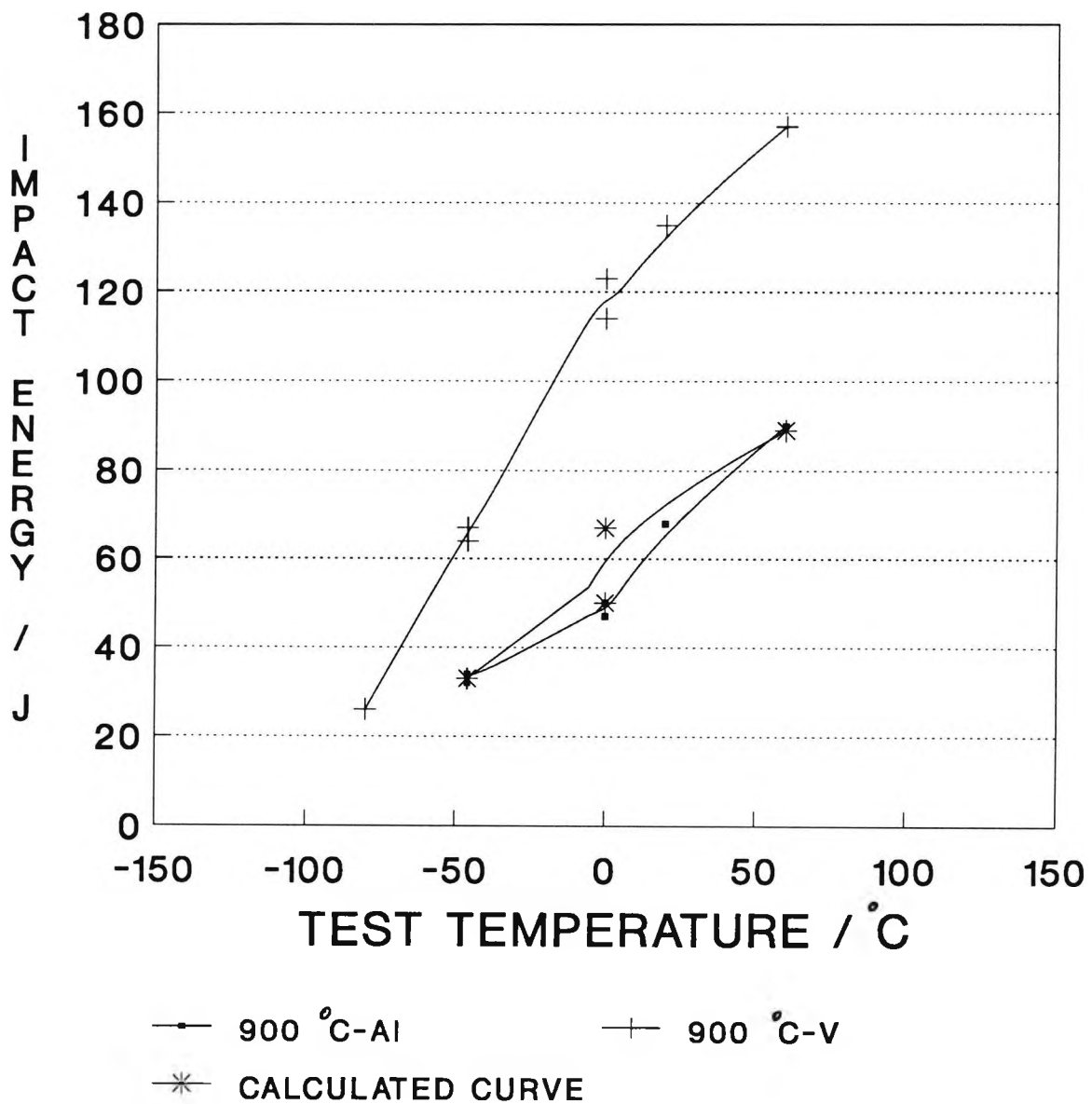
FIG 6.11 CALCULATED IMPACT TRANSITION CURVE ON THE BASIS OF CHANGES IN THE DUCTILE SHELF ENERGY
