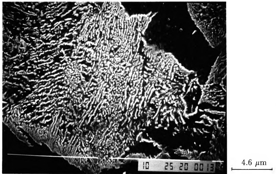
Figure 5.11: Microstructure of oil quenched flanges when tempered at 300°C. (SEM)
