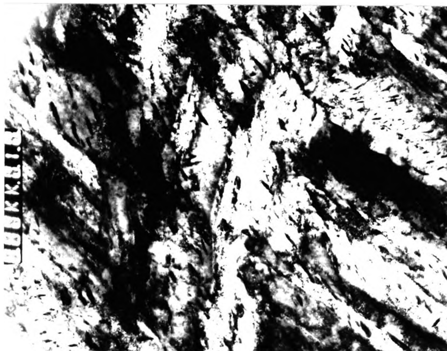
Figure 5.42: TEM microstructure of steel flange ice-water quenched from 1250°C and tempered at 300°C. (MAG 12000X)
