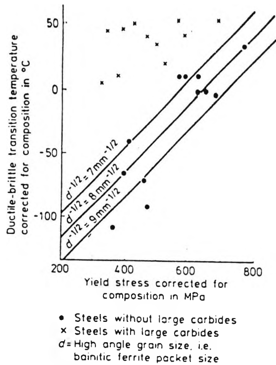
Figure 2.25: The relationship between the yield stress and the ductile-brittle transition temperature for bainitic microstructures containing 0.05-0.15 wt.% C [35] .
