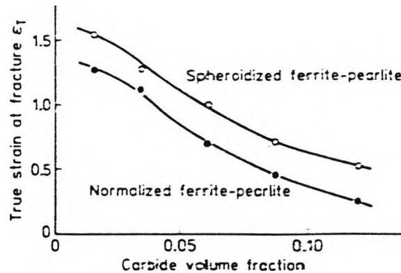
Figure 2.20: The effect of the volume fraction of carbides on the true strain at fracture for normalised and spheroidized ferrite-pearlite microstructures. The normalized microstructure contained lamellar pearlite [58] .
