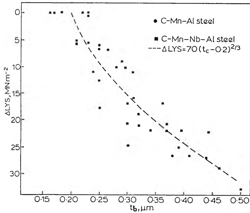
Figure 2.7: Influence of GBC thickness on fall in LYS [32]
