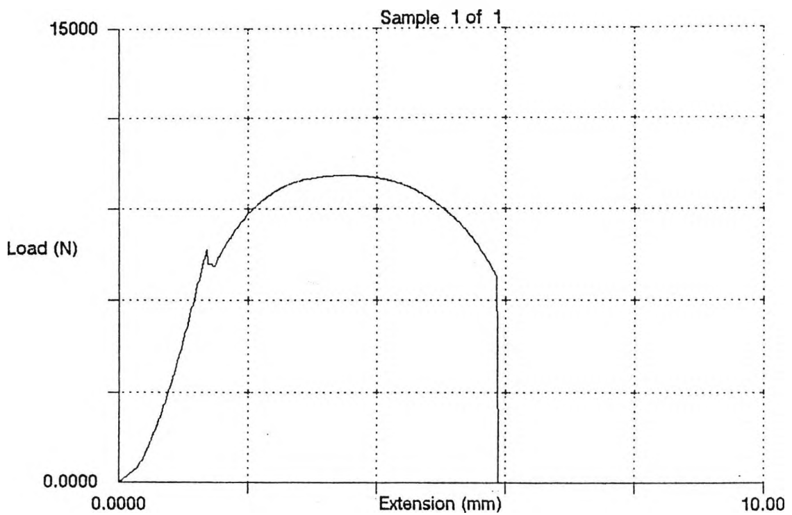
Figure 5.6: Stress/strain curve for the flanges oil quenched from 900°C.
