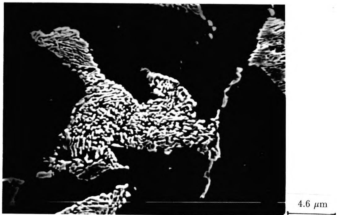
Figure 5.12: Microstructure of oil quenched flanges when tempered at 600°C. (SEM)
