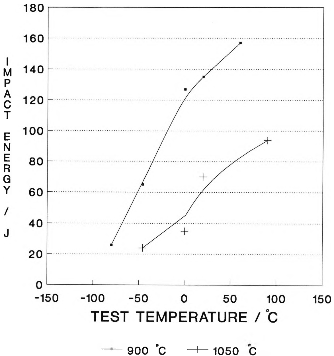
FIG 6.1 IMPACT TRANSITION CURVES FOR V CONTAINING STEEL
