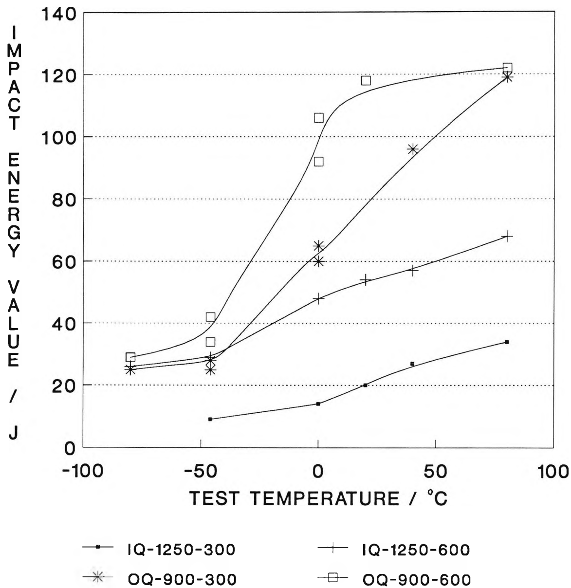
Fig 5.30 Impact transition curves for samples ice-water quenched from 1250 or 900 °C and tempered.
