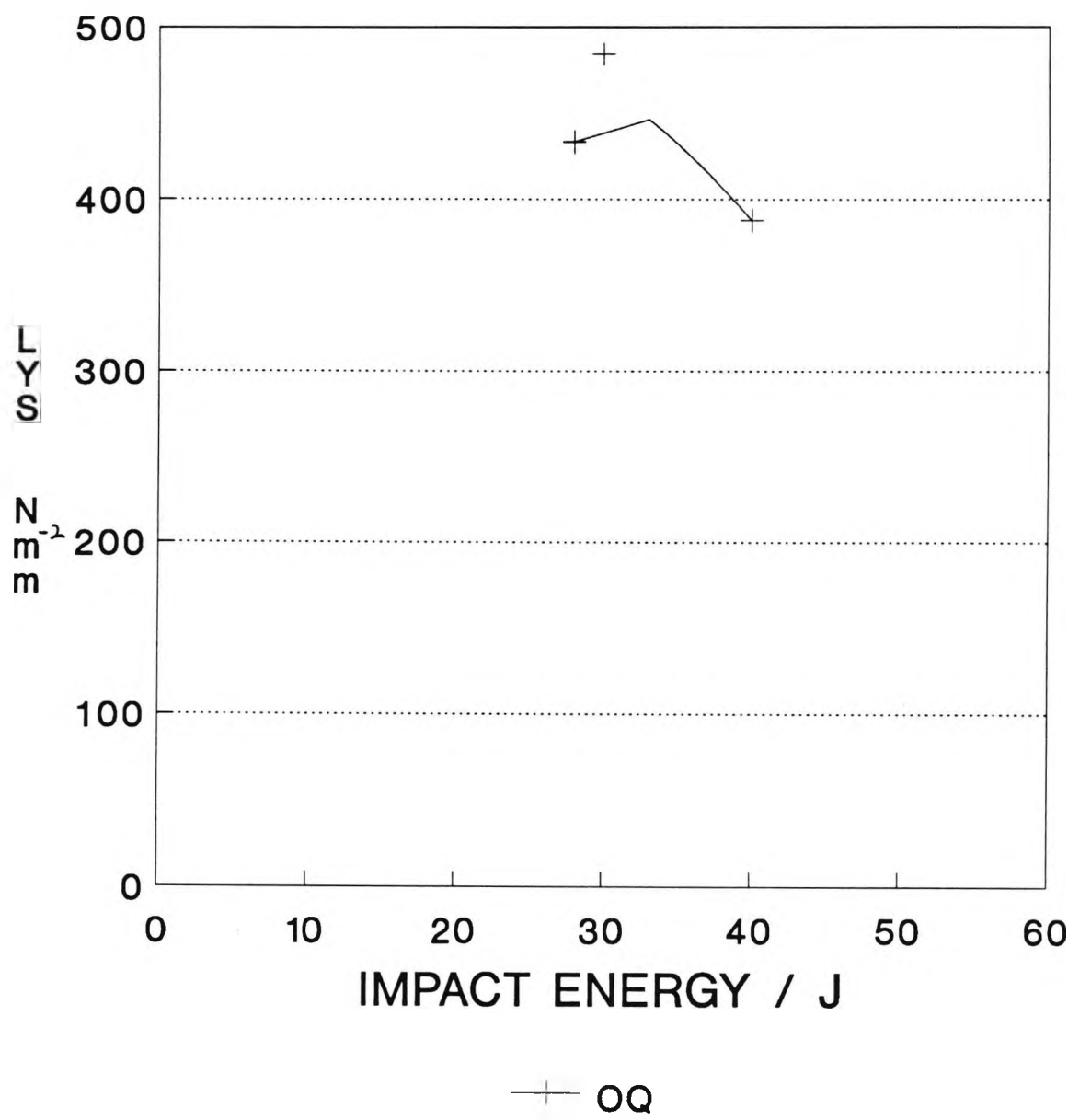
FIG 5.37 Variation of impact energy at -46°C with changes in strength on tempering for oil quenched steels
