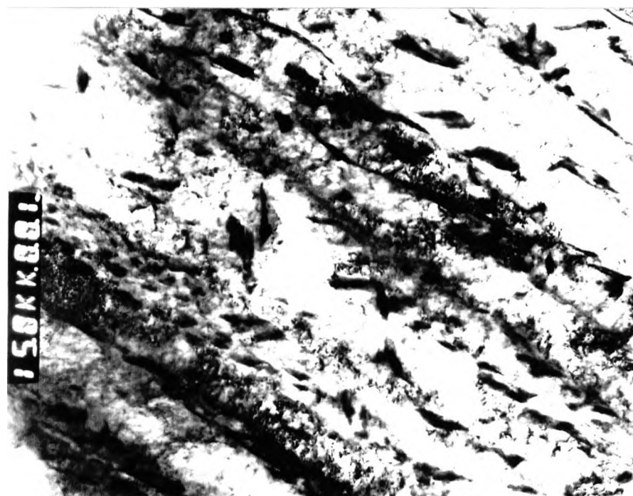
Figure 5.43: TEM microstructure of steel flange ice-water quenched from 1250°C and tempered at 300°C. (MAG 21000)
