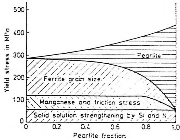
Figure 2.15: The effect of the pearlite fraction on the yield stress of normalized carbon-manganese steels, showing the effect of the various strengthening mechanisms [50] .
