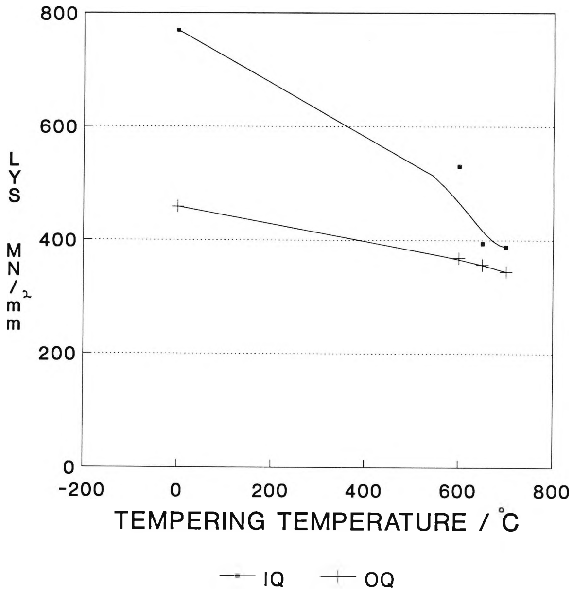
Fig 4.7 Effect of tempering on LYS of samples ice-water or oil quenched from 950^{\circ}\text{C}
