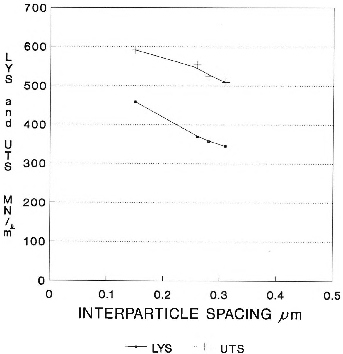
FIG 4.27 Variation of LYS and UTS with interparticle spacing for oil quenched samples
