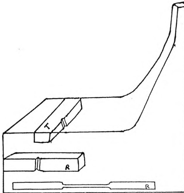
Figure 3.3: Position of charpy and tensile samples cut out of flanges
