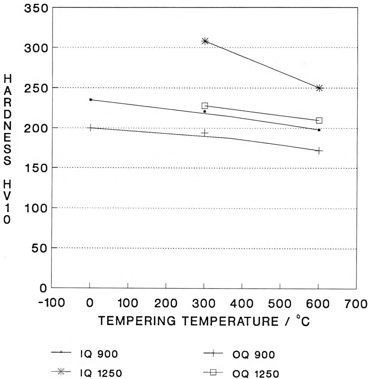
Fig 5.9 Effect of tempering on hardness for samples ice-water or oil quenched from 900 and 1250 °C. (0 = As quenched)
