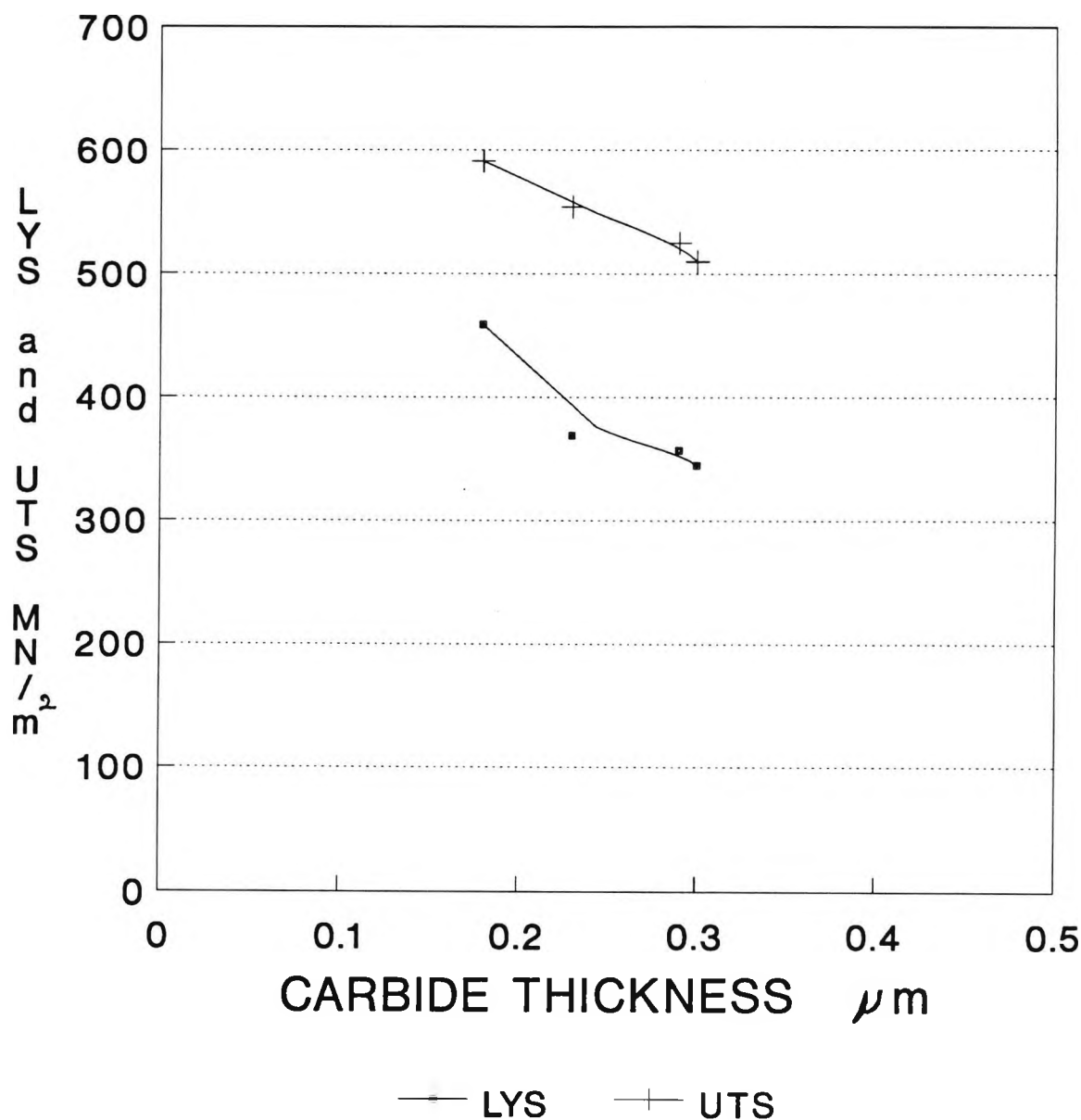
FIG 4.26 Variation of LYS and UTS with carbide thickness for oil quenched samples
