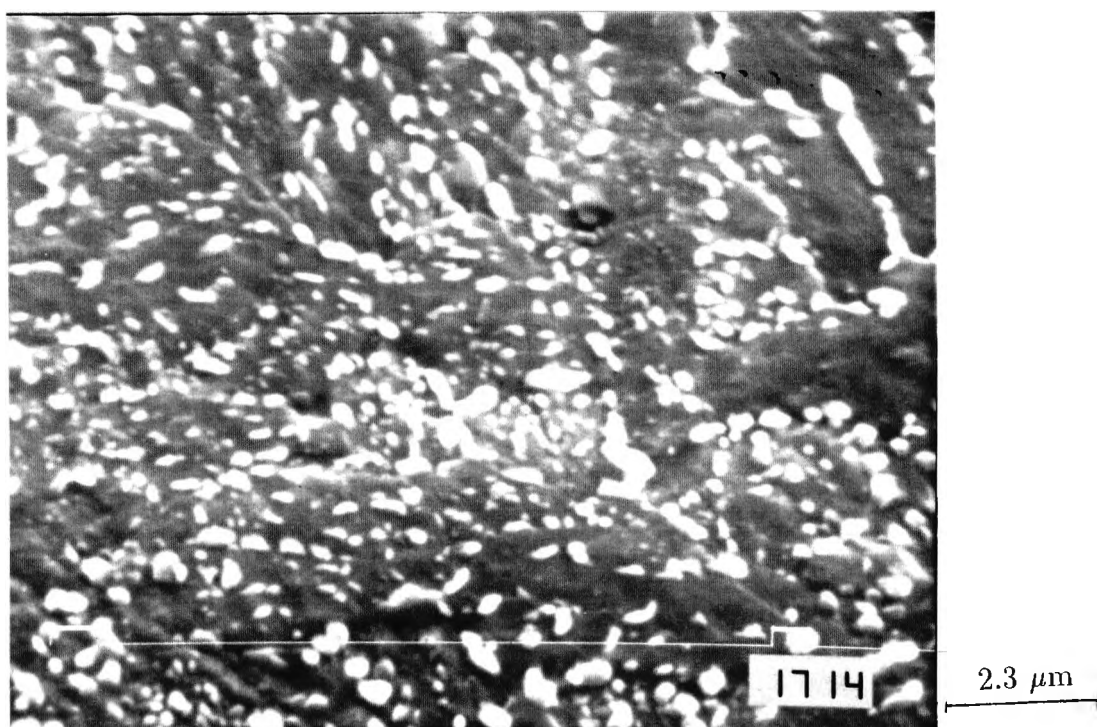
Figure 4.16: Almost complete spheroidization when tempered at 700°C for 1 hour. Steel was oil quenched from 950°C for 1 hour. (SEM)
