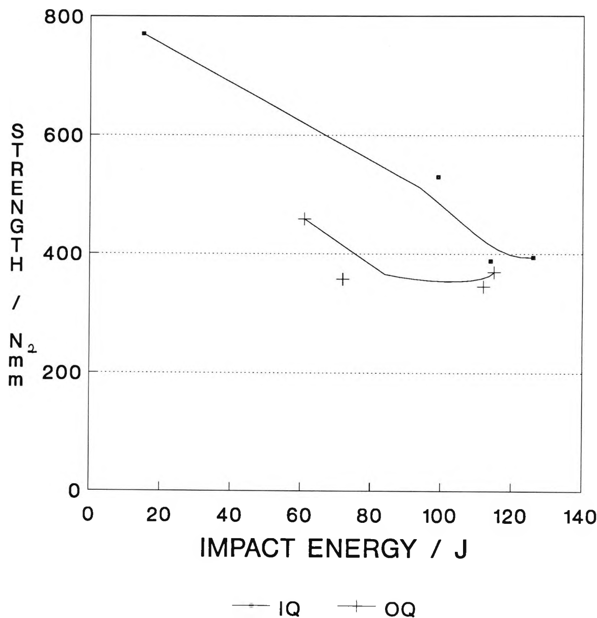
FIG 4.32 Variation of impact energy at -46^{\circ}\text{C} with changes in strength on tempering
