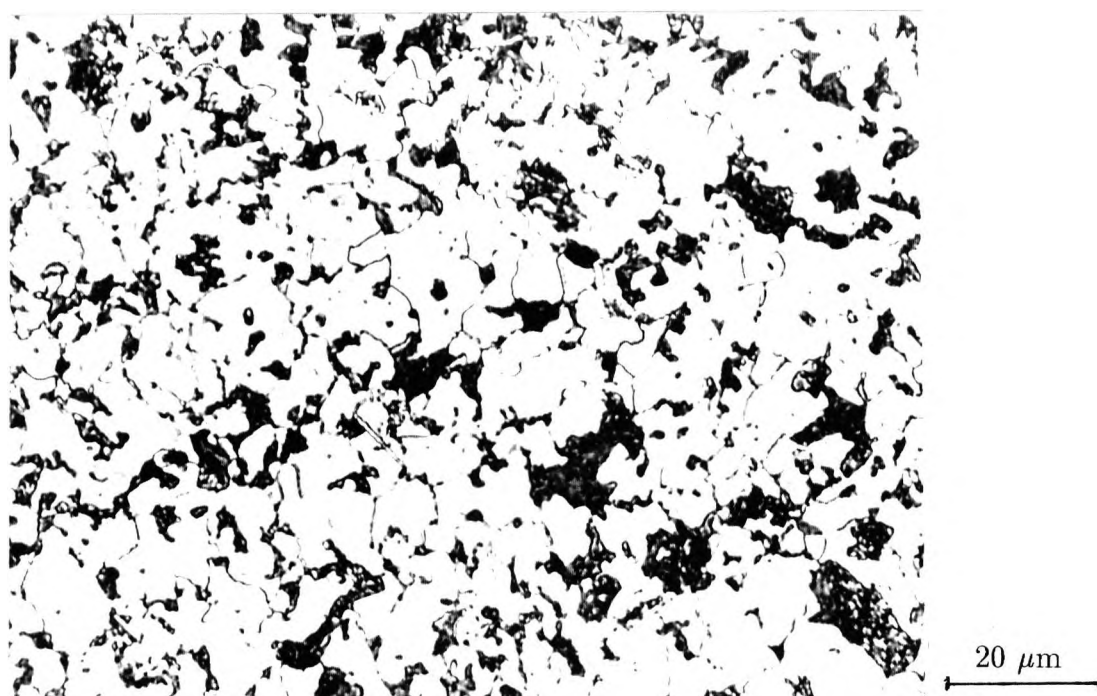
Figure 6.3: Microstructure of V containing steel obtained when normalised from 900^{\circ}\text{C} after holding for 1 hour.
