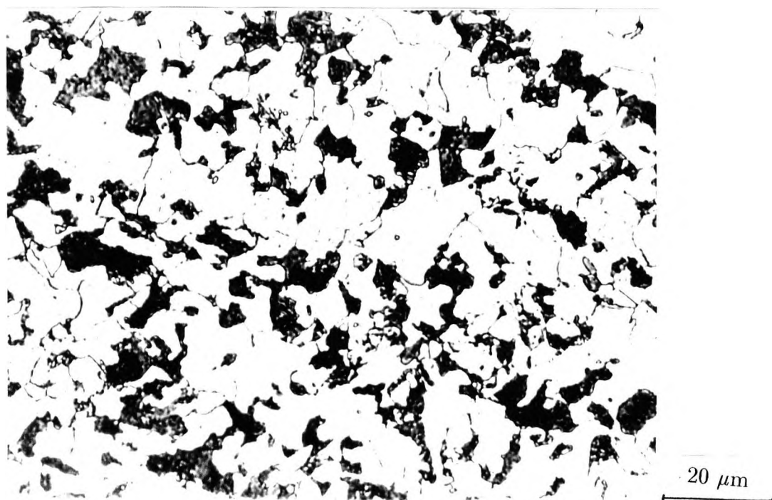
Figure 6.4: Microstructure of Al containing steel obtained when normalised from 900^{\circ}\text{C} after holding for 1 hour.
