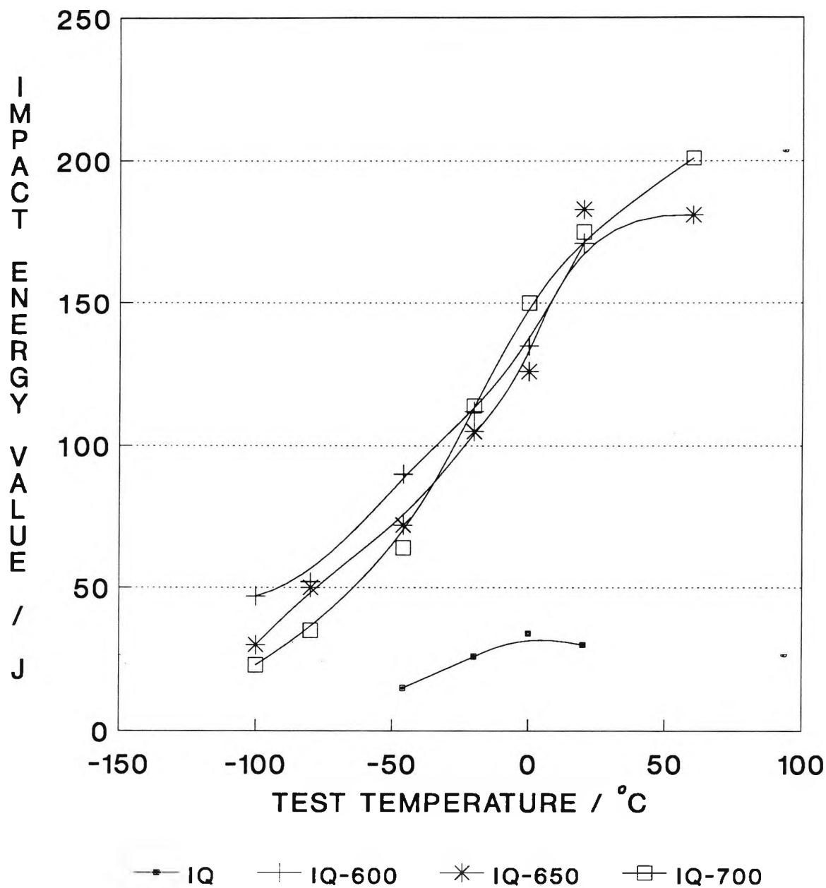
Fig 4.1 Impact transition curves for samples ice-water quenched from 950 °C
