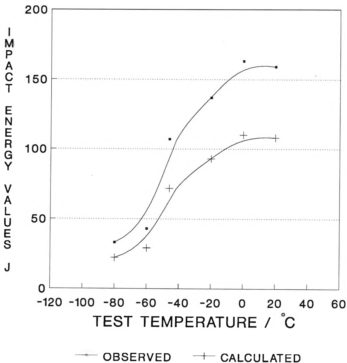
Figure 4.28: Upper curves is the average impact energy for the tempered flanges after oil quenching. The lower curve represents the calculated from the upper curve assuming a lower shelf energy.
