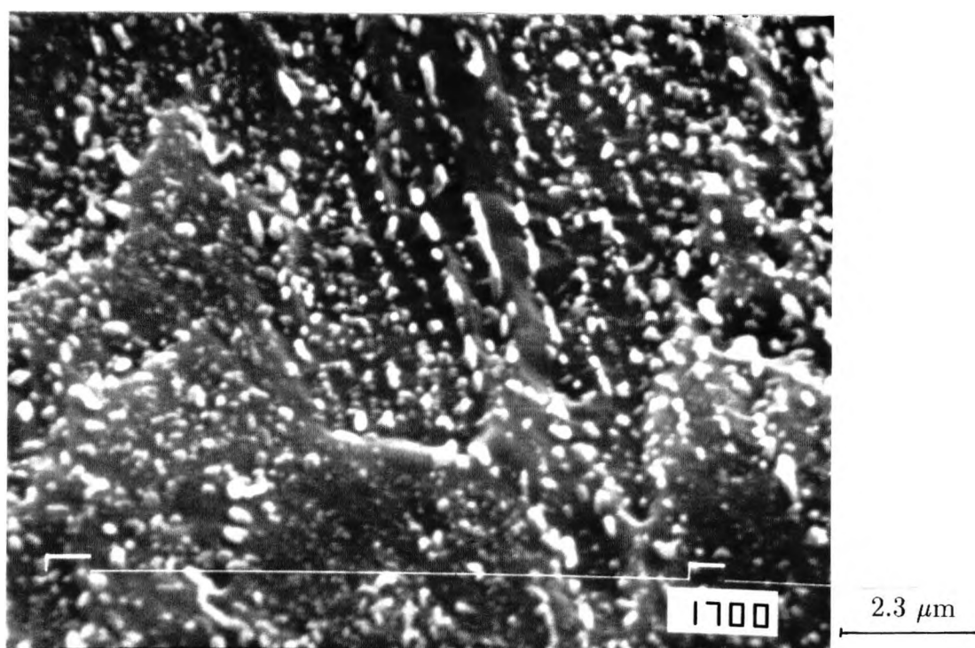
Figure 4.18: Microstructure of steel flanges ice-water quenched from 950°C after holding for 1 hour and tempered at 600°C for 1 hour. (SEM)
