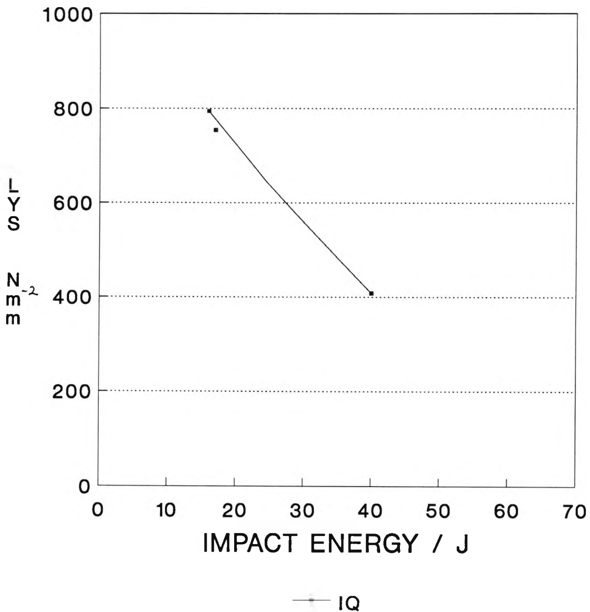
FIG 5.40 Variation of impact energy at -46^{\circ}\text{C} with changes in strength on tempering for ice-water quenched steels.
