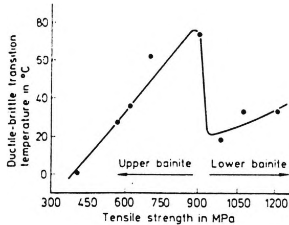
Figure 2.23: The relationship between the ductile-brittle transition temperature and the tensile strength for low carbon bainitic microstructures containing 0.05-0.15 wt.% C [65] .
