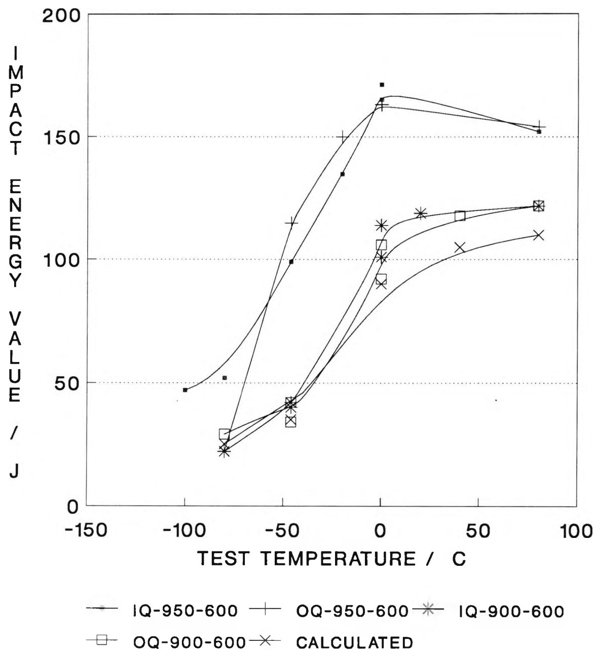
Figure 5.36: Comparing impact transition curves for flanges ice-water or oil quenched from 950 or 900°C and tempered at 600°C with calculated curve.
