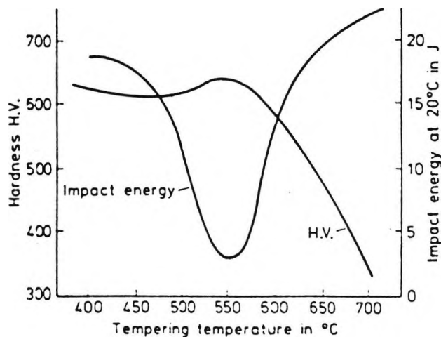
Figure 2.32: Embrittlement caused by secondary hardening during the tempering of a 0.4 wt.% C, 5 wt.% Cr-Mo-V steel [93] .
