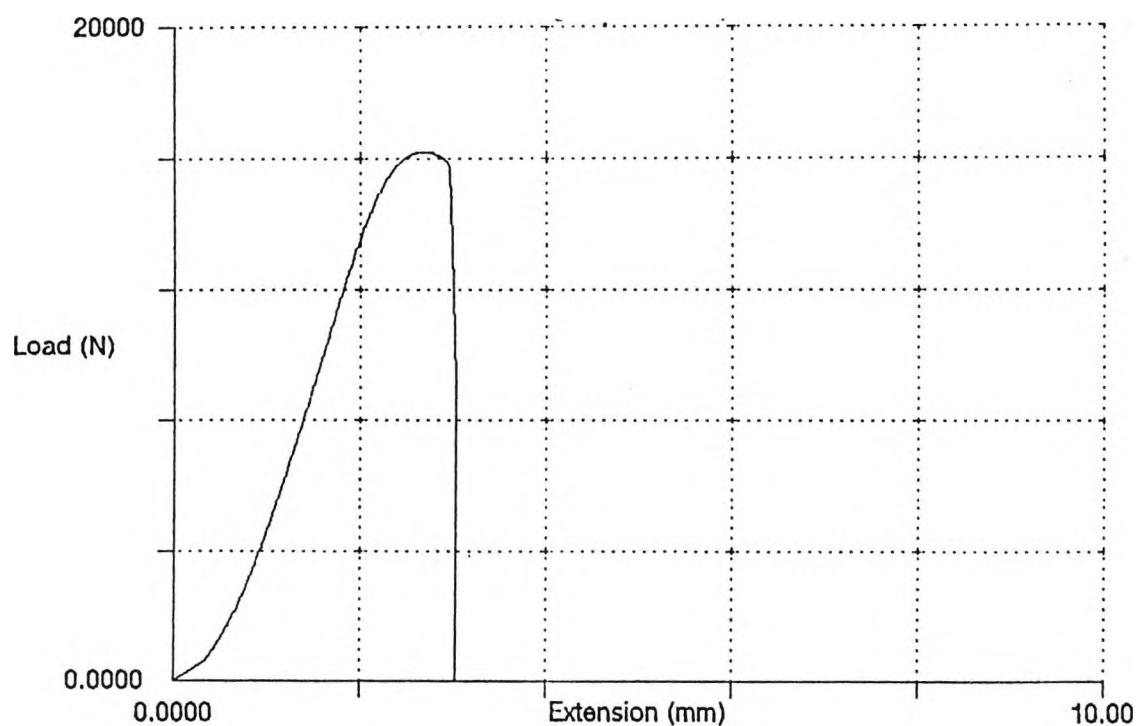
Figure 5.23: Stress/strain curve for the flange ice-water quenched from 1250°C and tempered at 300°C.
