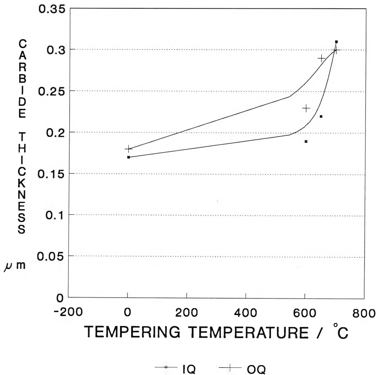
FIG 4.23 Variation of carbide thickness with tempering temperature for both ice-water and oil quenched samples (0 = AQ).
