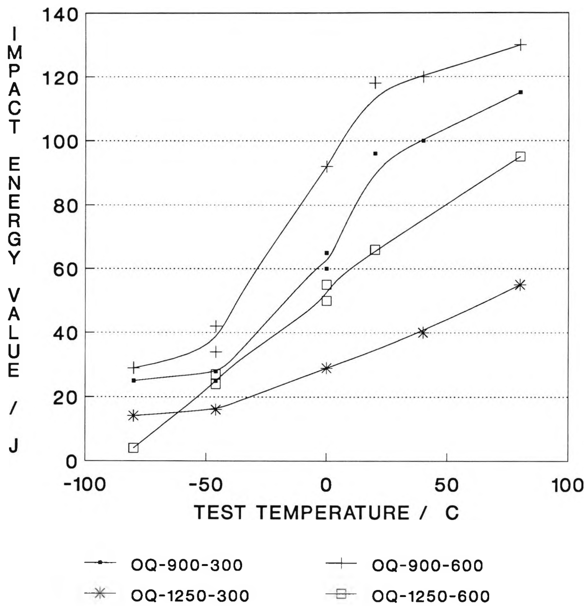
Fig 5.31 Impact transition curves for samples oil quenched from 1250 or 900 °C and tempered.
