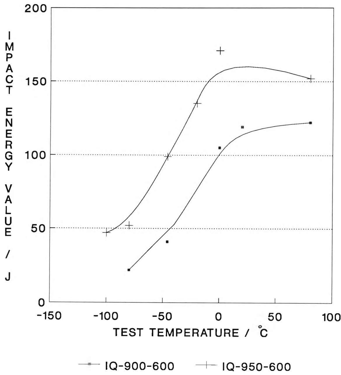
Figure 5.41: Impact transition curves for flanges ice-water quenched from 900 or 950°C and tempered at 600°C.
