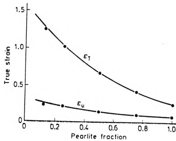
Figure 2.19: The effect of the pearlite fraction on the uniform true strain ( \epsilon_u ) and the true strain at fracture ( \epsilon_T ) in normalized ferrite-pearlite microstructures [58] .
