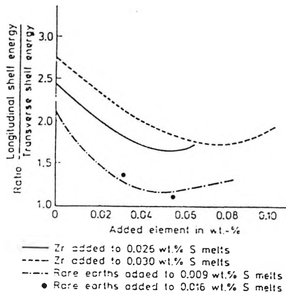
Figure 2.12: The elimination of the anisotropy of shell energy by inclusion shape control additions [46] .
