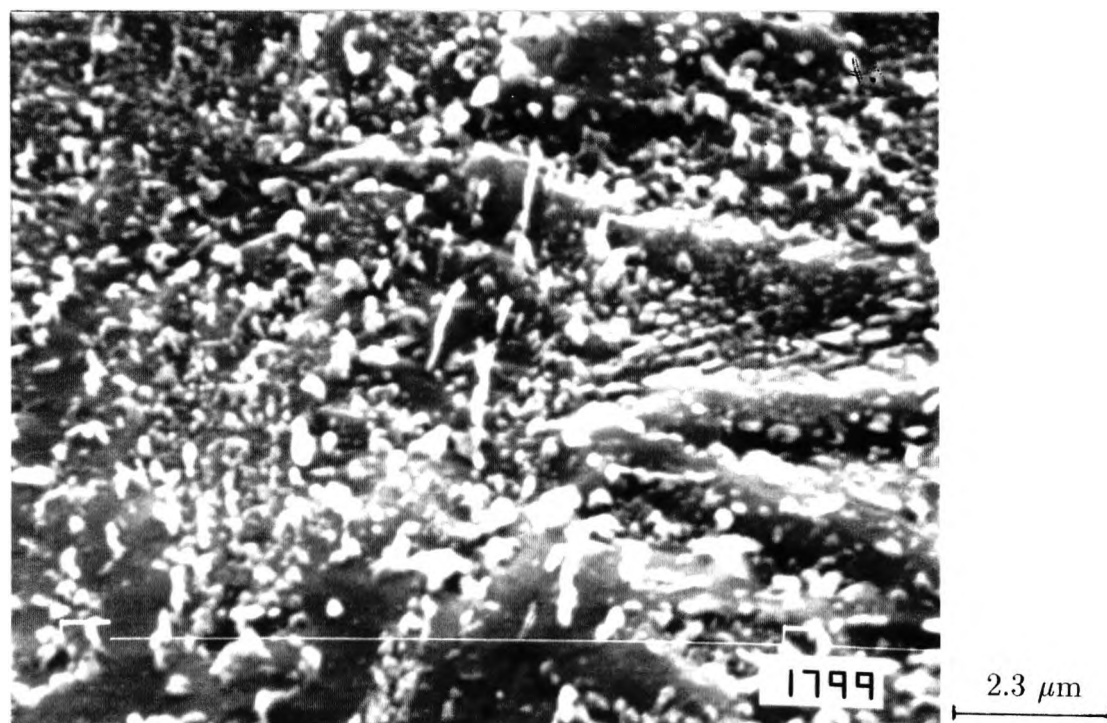
Figure 4.19: Microstructure of steel flanges ice-water quenched from 950°C after holding for 1 hour and tempered at 650°C for 1 hour. (SEM)
