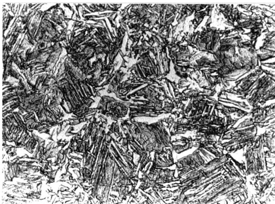
Fig 4.12 Microstructure of steel flanges ice-water quenched from 950 °C.
