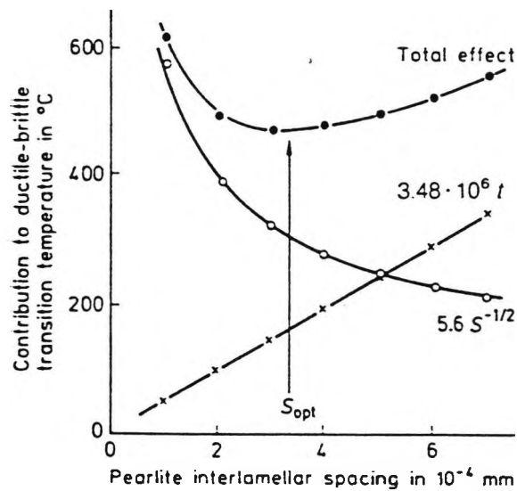
Figure 2.16: The contributions of the pearlite interlamellar spacing ( S ) and the carbide lamella thickness ( t ) to the ductile-brittle transition temperature, showing the occurrence of an optimum value of the inter lamellar spacing [58] .
