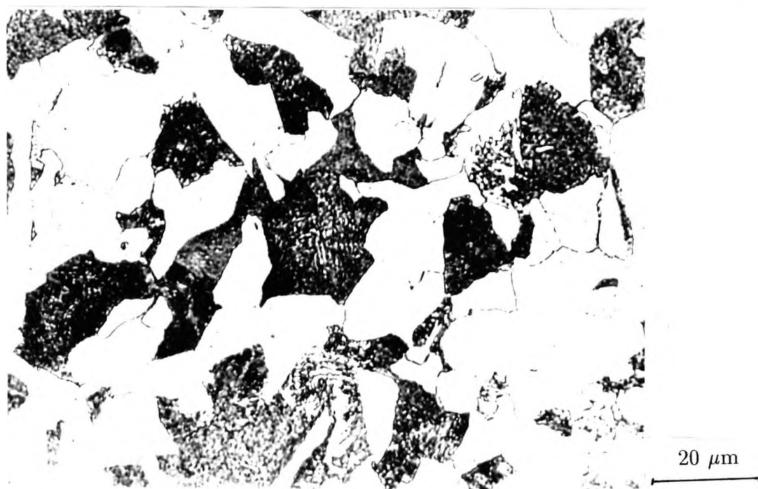
Figure 6.6: Microstructure of Al containing steel obtained when normalised from 1050°C after holding for 1 hour.
