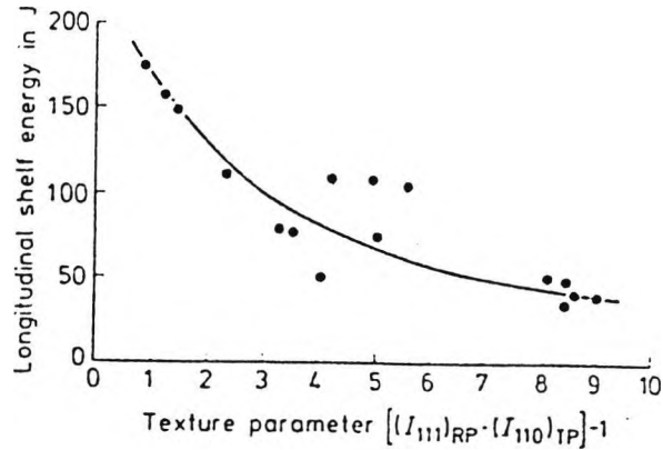
Figure 2.10: The relationship between the longitudinal shelf energy and the texture parameter [30] .
