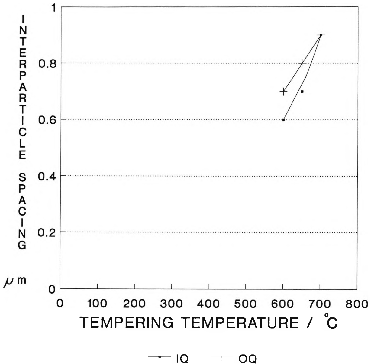
FIG 4.24 Variation of interparticle spacing with tempering temperature for both ice-water and oil quenching
