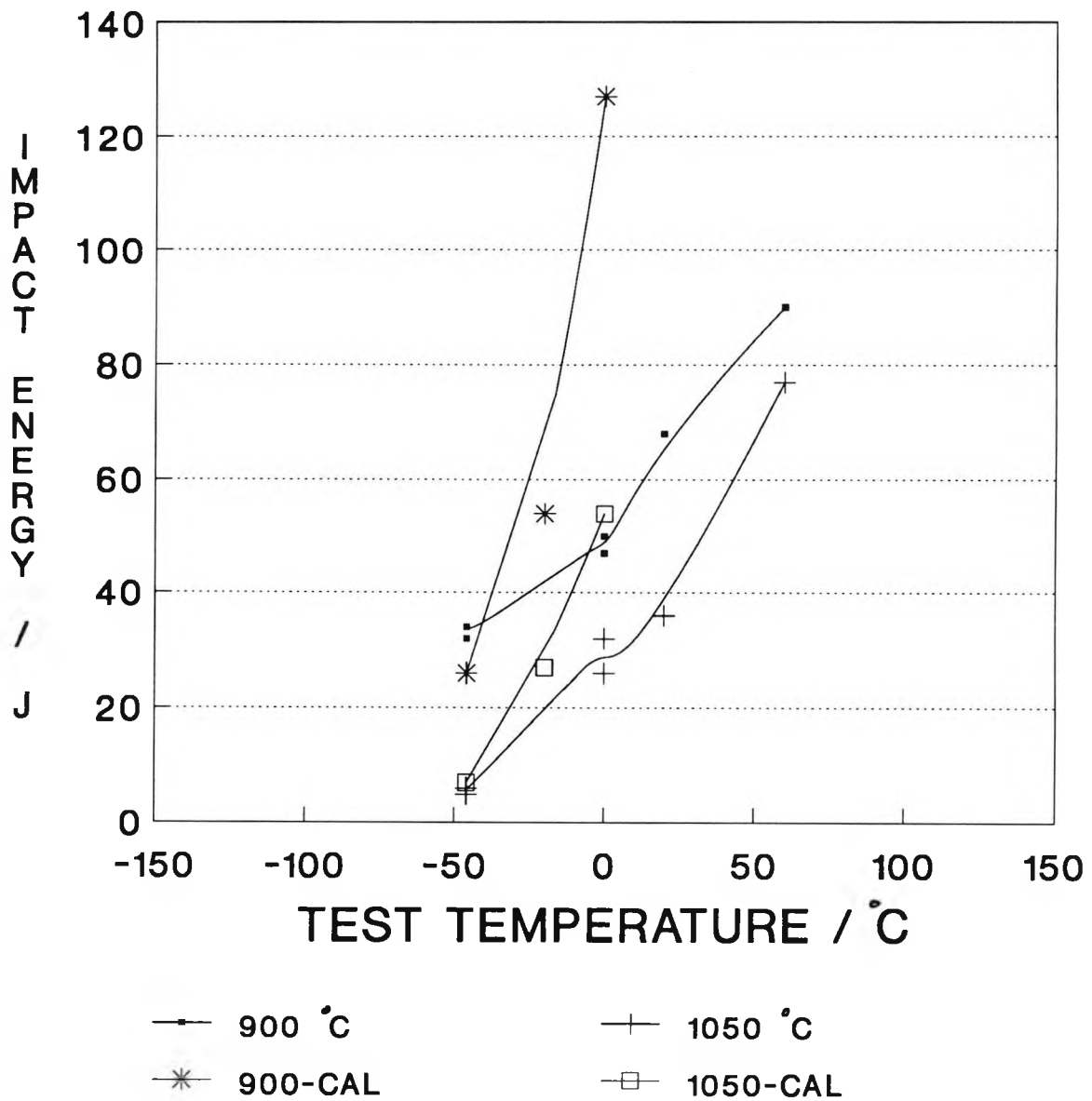
FIG 6.10 OBSERVED AND CALCULATED IMPACT TRANSITION CURVES FOR AL CONTAINING STEEL (CAL = CALCULATED)
