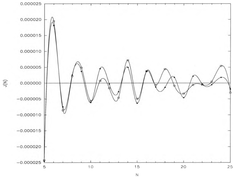
Figure 3.59: Comparison of the exchange coupling obtained using 8256 (squares) and 32896 (circles) k_{\parallel} points in the k_{\parallel} summation for the reduced BZ.
