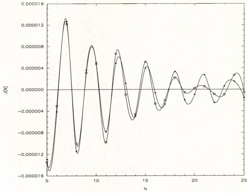
Figure 2.20: Comparison of the exchange coupling obtained using 8256 (squares) and 32896 (circles) k_{||} points in the k_{||} summation for the reduced BZ.
