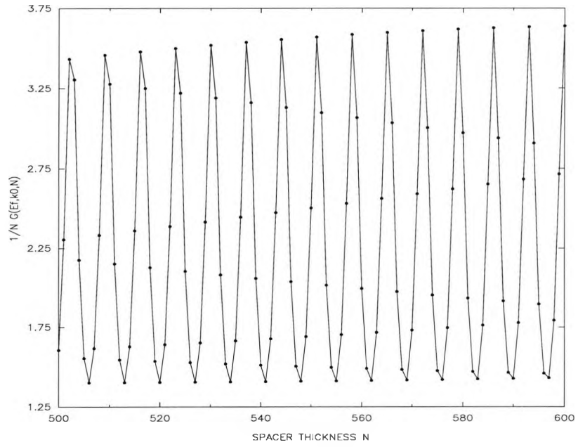
Figure 3.25: Dependence of the spectral density on N for the up and down spin bands of the AF configuration of the trilayer. It is evaluated at k_x = k_y = 0 and E = E_f .
