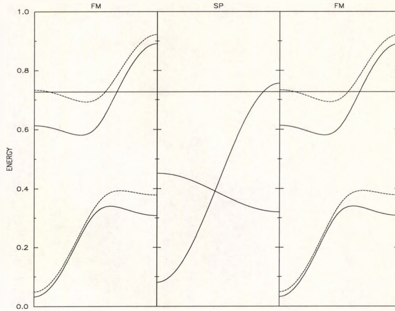
Figure 3.11: Bands in the ferromagnetic layers \text{FM}^\uparrow (solid line) and \text{FM}^\downarrow (dashed line) and the spacer layer SP. The straight solid line is the Fermi energy level.
