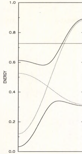
Figure 3.5: Comparison of the energy bands of the unhybridized semi-infinite crystal (Dotted lines) and the hybridized adlayers (Solid lines). The straight solid line is the Fermi energy level.
