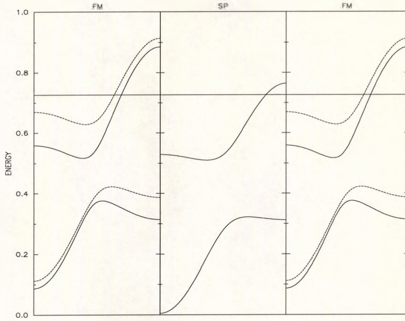
Figure 3.43: Bands in the ferromagnetic layers \text{FM}^\uparrow (solid line) and \text{FM}^\downarrow (dashed line) and the spacer layer SP. The straight solid line is the Fermi energy level.
