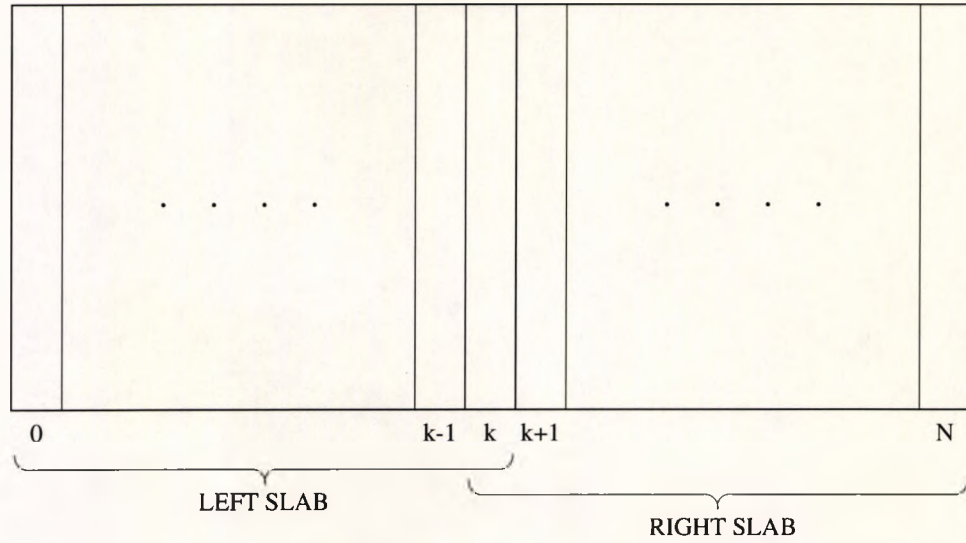
Figure 2.14: Diagram showing two finite slabs that meet at the k th atomic plane. The left slab contains k atomic planes and the right slab contains N-k atomic planes.
