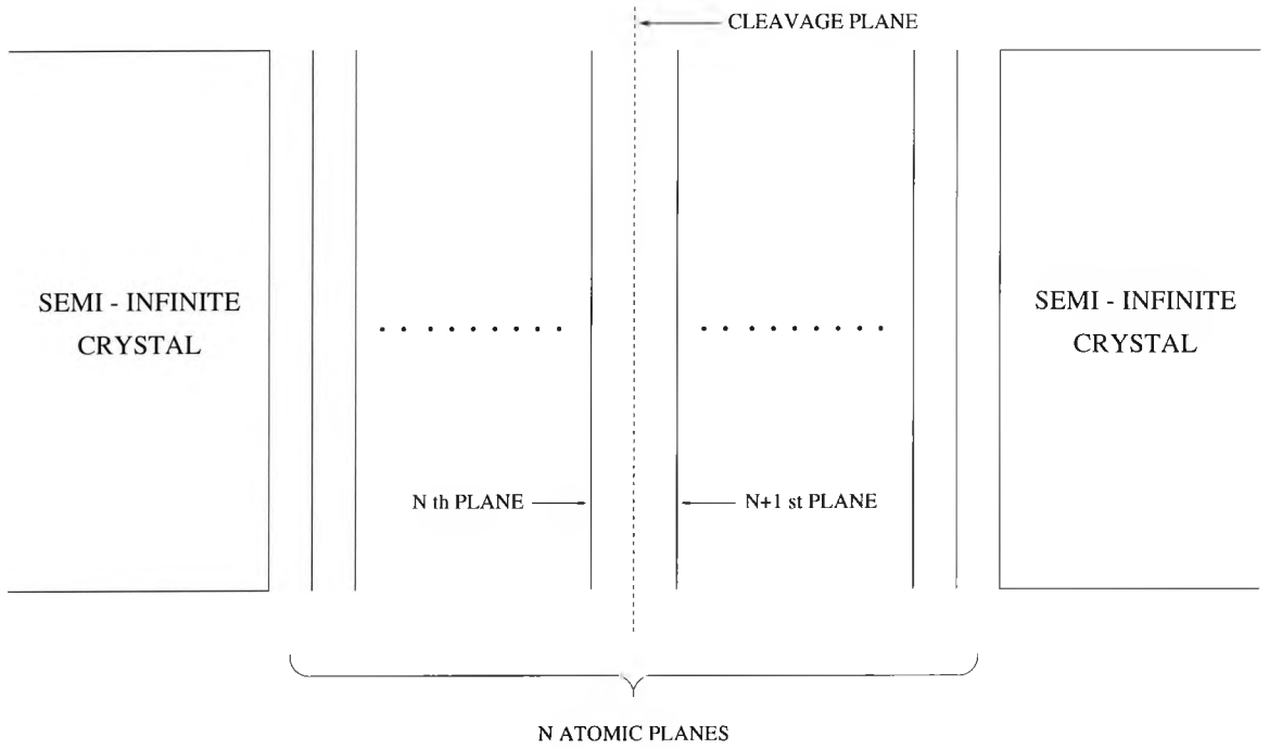
Figure 3.9: Diagram of a trilayer consisting of N atomic planes in the spacer layer sandwiched between two semi-infinite crystals.
