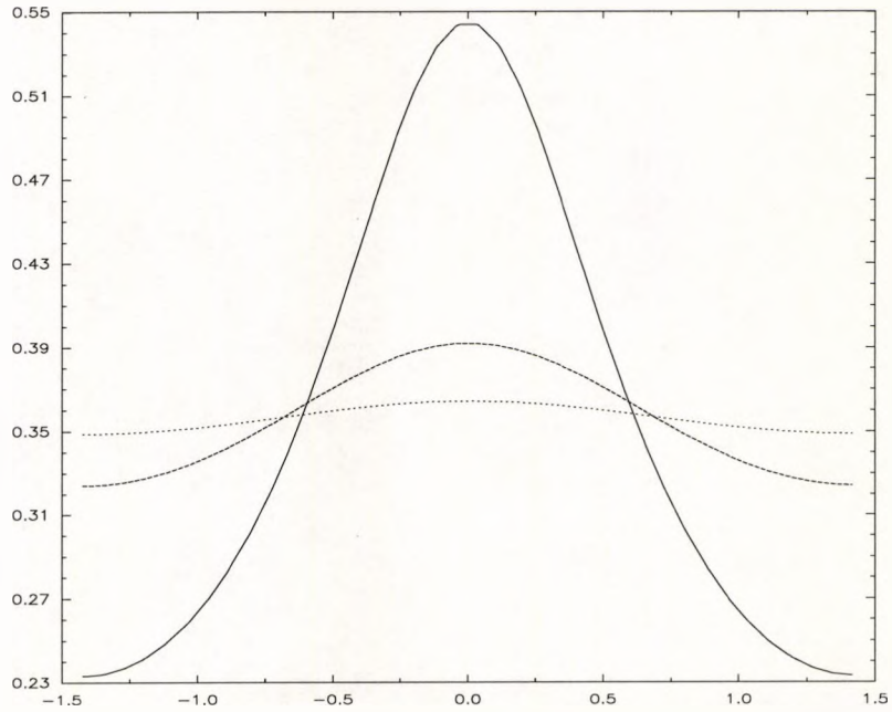
Figure 2.25: Shifted spectral densities of the up spin band (solid line) and down spin band (dotted line) of the ferromagnetic configuration and the up and down spin bands (dashed line) of the antiferromagnetic configuration.
