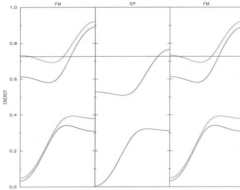
Figure 3.27: Bands in the ferromagnetic layers \text{FM}^I (solid line) and \text{FM}^{II} (dashed line) and the spacer layer SP. The straight solid line is the Fermi energy level.
