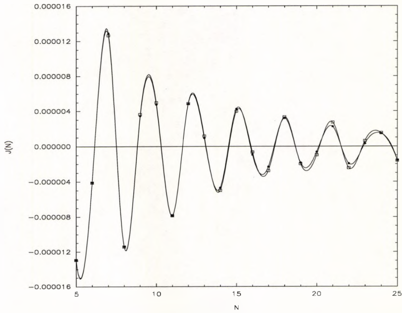
Figure 2.21: Comparison of the exchange coupling obtained using 32896 (squares) and 131328 (circles) k_{||} points in the k_{||} summation for the reduced BZ.
