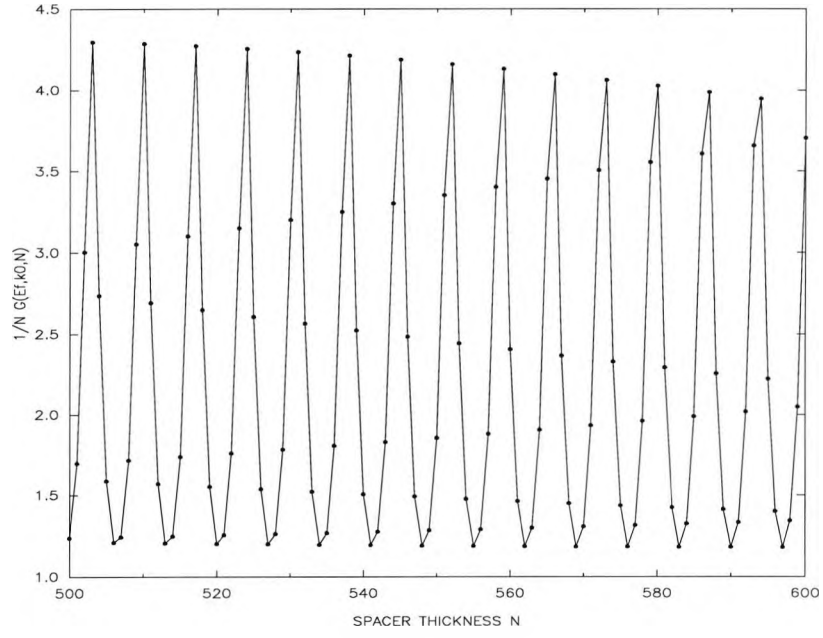
Figure 3.24: Dependence of the spectral density on N for the down spin band of the FM configuration of the trilayer. It is evaluated at k_x = k_y = 0 and E = E_f .
