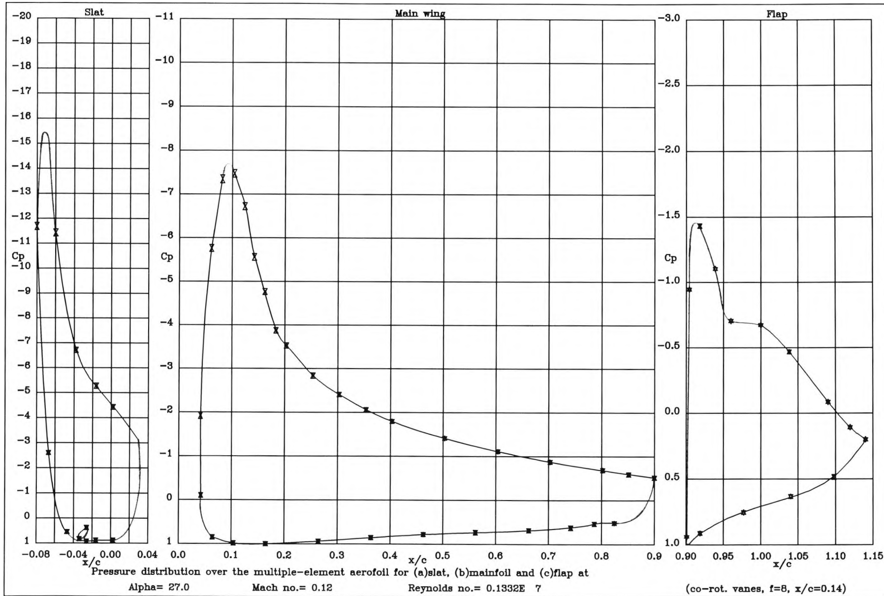
Figure 6.3 : Pressure distribution over the high lift system at 27^\circ when co-rot. vng's are at x/c = 0.14
