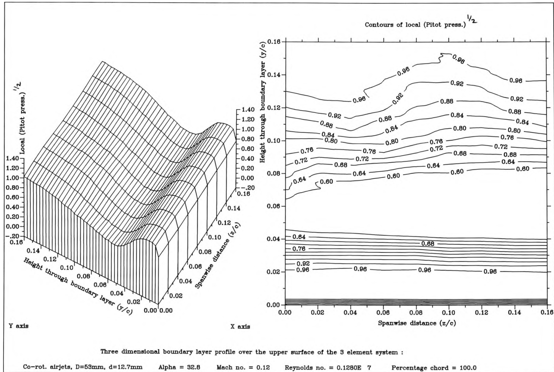
Figure 7.31 : Contour plot and surface plot of the shear layer structure above the flap at x/c = 1.0 for \alpha = 32.8^\circ when co-rot. airjets are at x/c = 0.14
