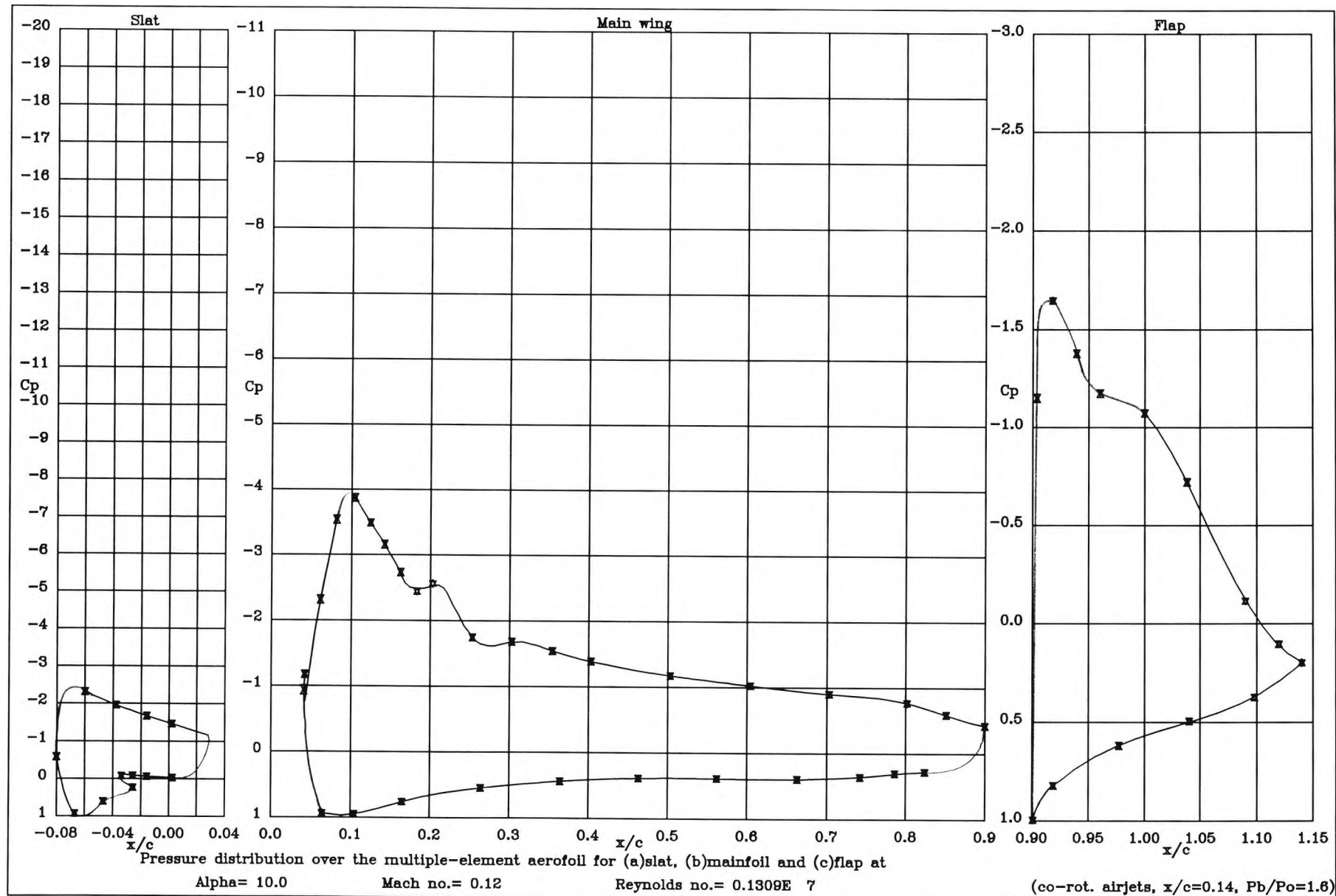
Figure 7.3 : Pressure distribution over the high lift system at 10^\circ when co-rot. airj's are at x/c=0.14
