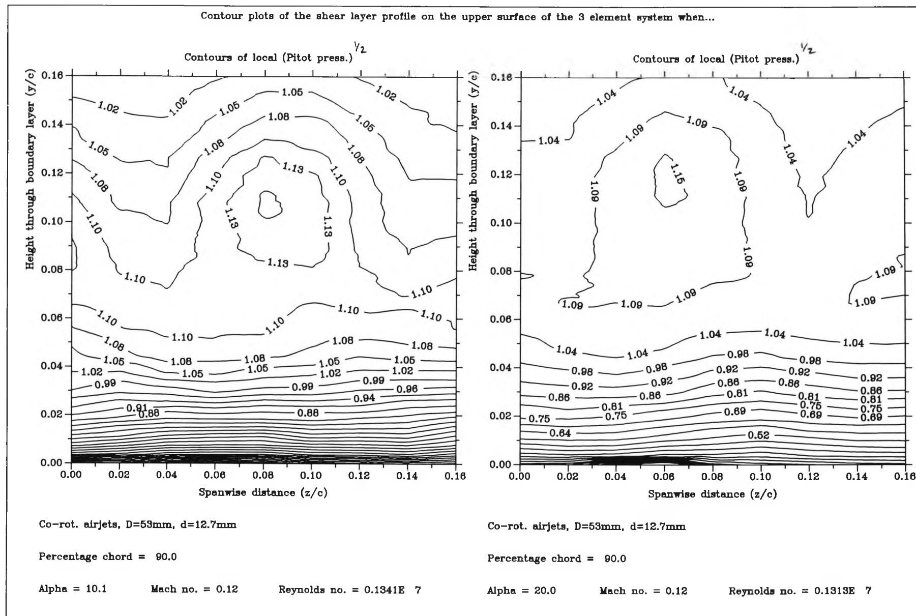
Figure 7.27 : Contour plots of the shear layer profile on the upper surface of the 3 element system when... \alpha = 10^\circ & 20^\circ when co-rot. airj's are at x/c = 0.14
