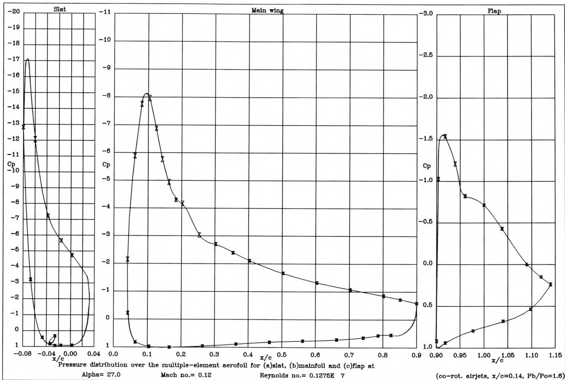
Figure 7.7 : Pressure distribution over the high lift system at 27^\circ when co-rot. airjets are
