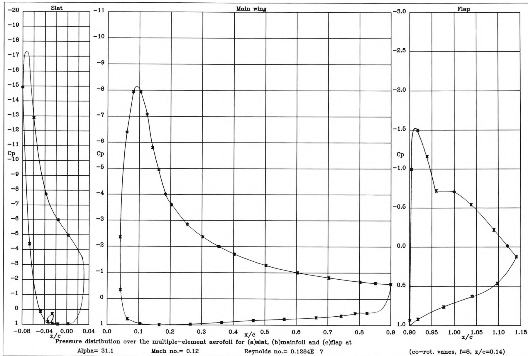
Figure 6.5 : Pressure distribution over the high lift system at 31.1^\circ when co-rot. vlg's are at x/c = 0.14
