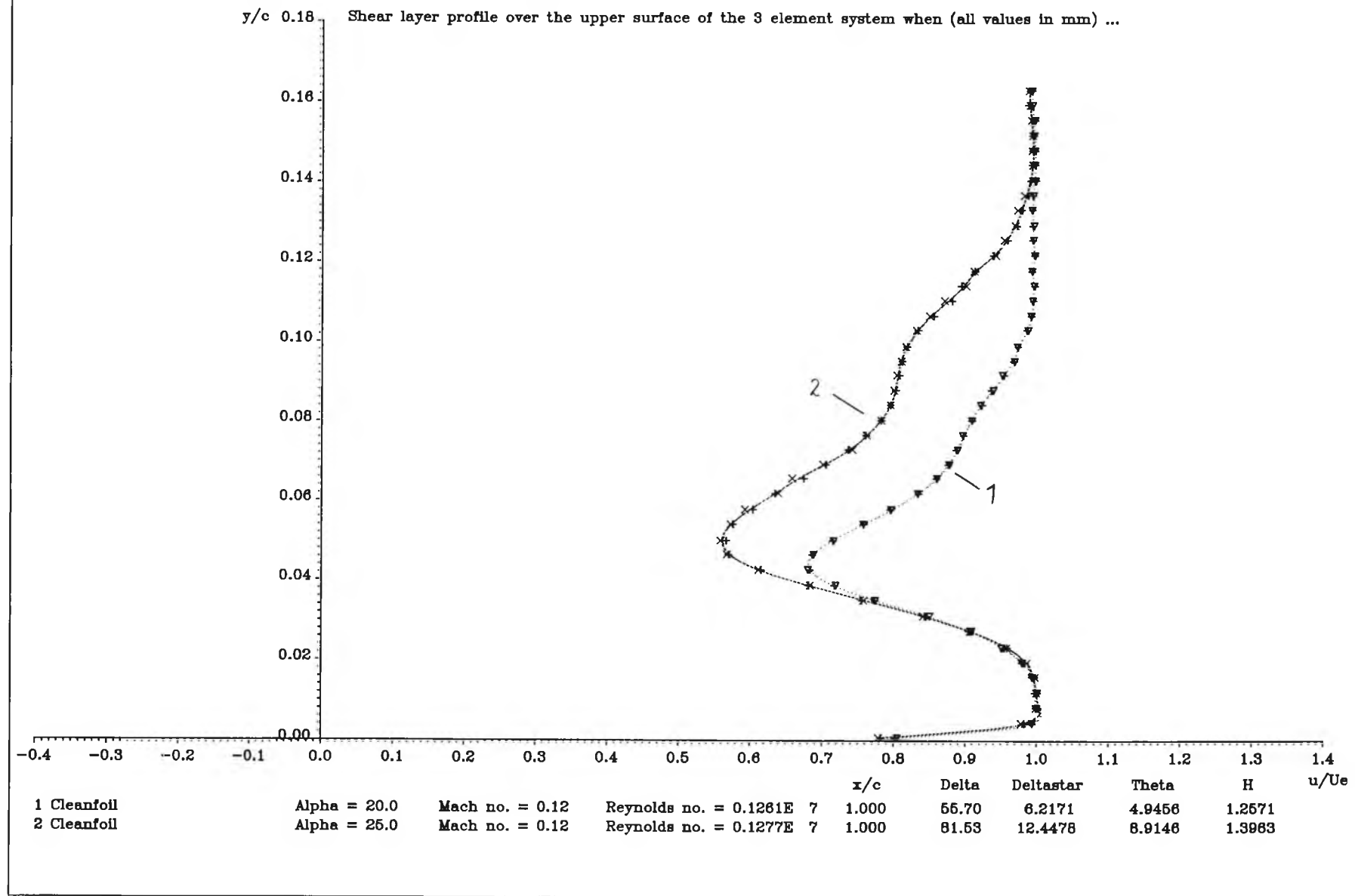
Figure 5.32 : Shear layer profiles over flap of the high lift system at 20° & 25°
