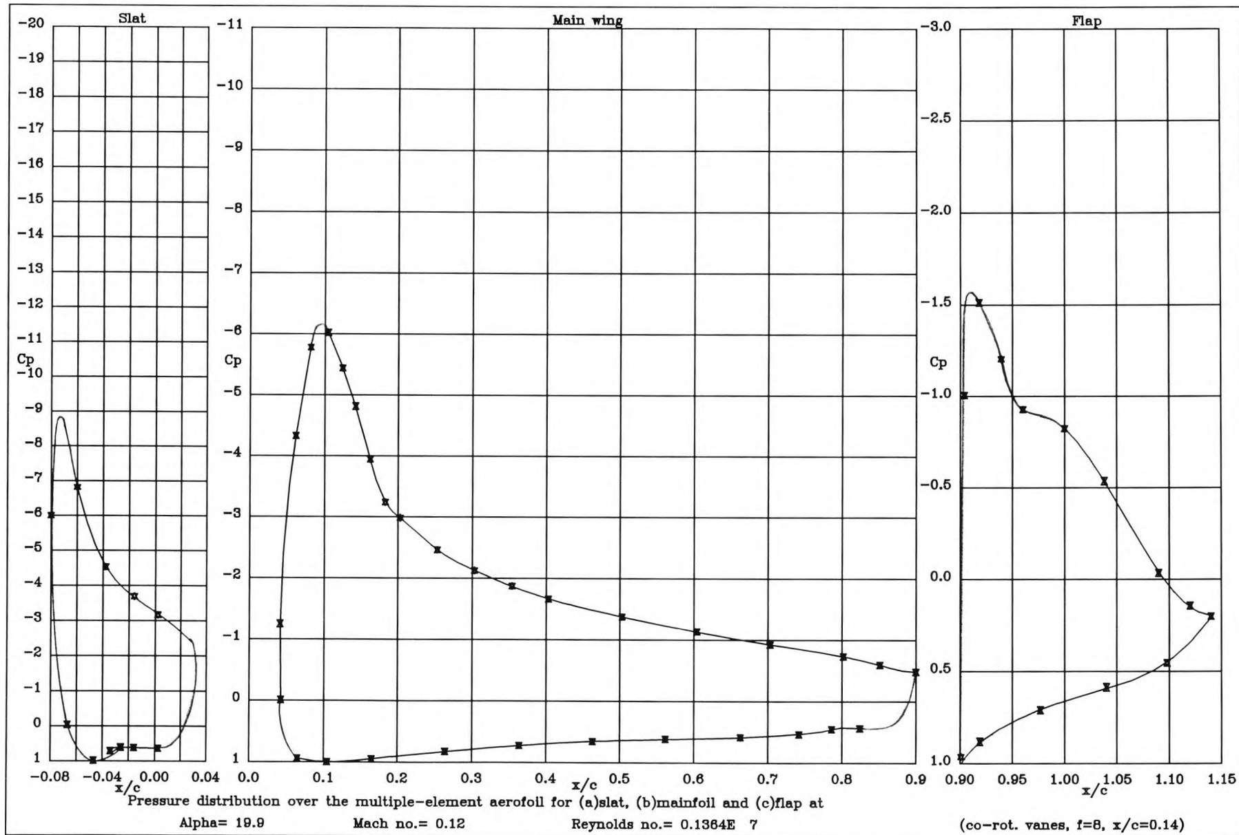
Figure 6.1 : Pressure distribution over the high lift system at 19.9^\circ when co-rot. vng's are at x/c=0.14
