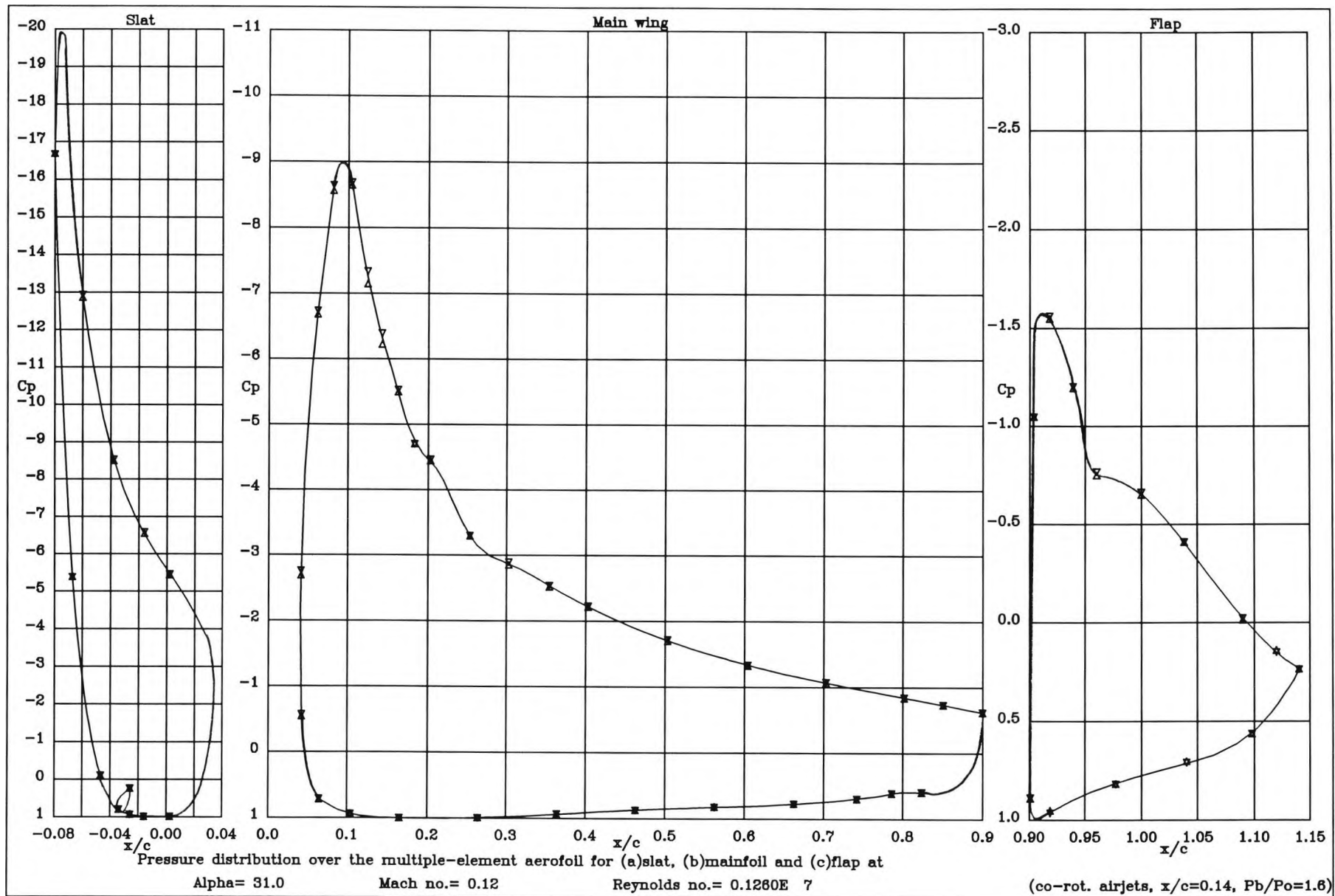
Figure 7.10 : Pressure distribution over the high lift system at 31° when co-rot. airjets are at x/c=0.14
