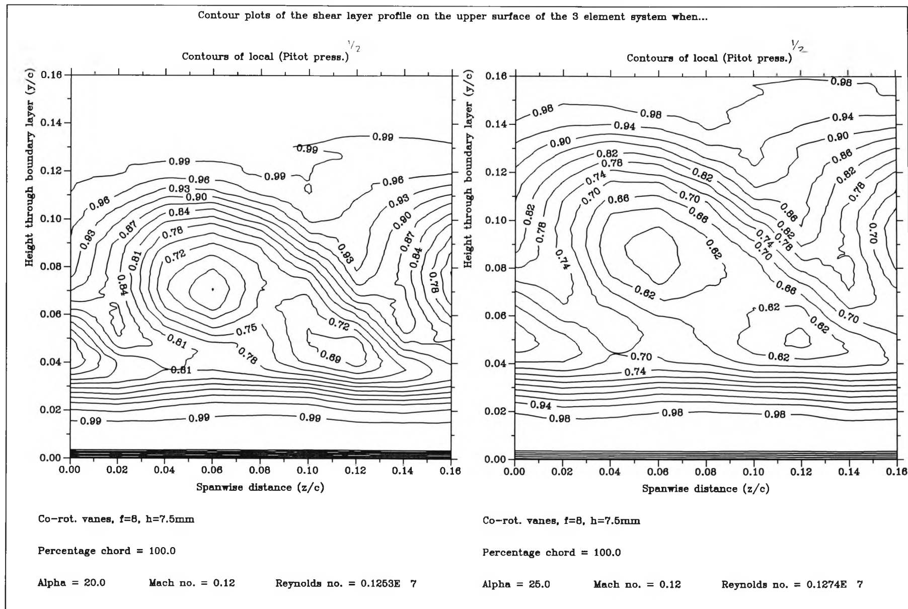
Figure 6.41 : Contour plots of the shear layer profile on the upper surface of the 3 element system when...
