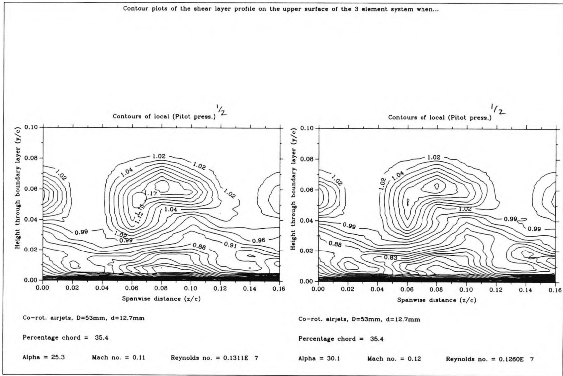
Figure 7.26 : Contour plots of the shear layer structure above the main wing at x/c = 0.354 for \alpha = 25^\circ & 30^\circ when co-rot. ajvg's are at x/c = 0.14
