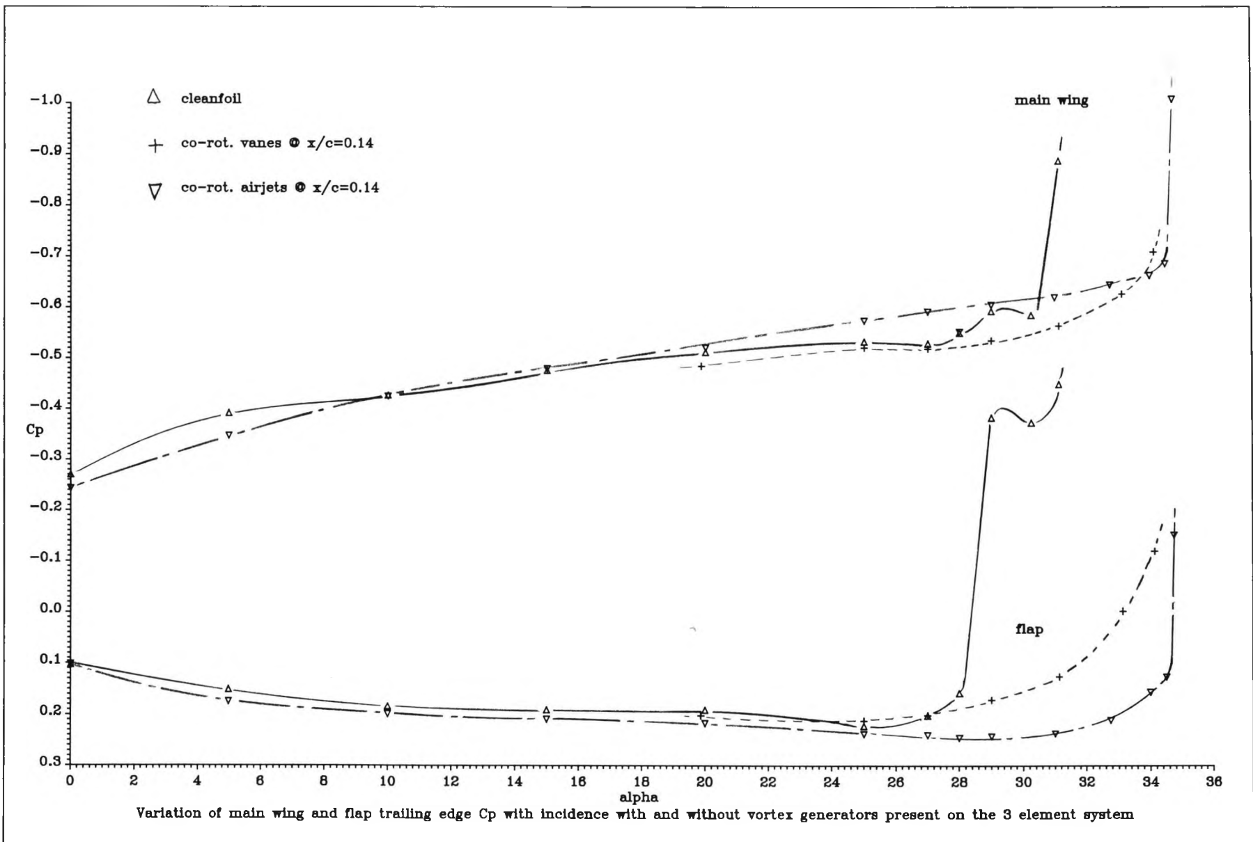
Figure 7.23 : Variation of main wing and flap trailing edge C_p 's with \alpha when co-rot. airjet vortex generators are at x/c=0.14
