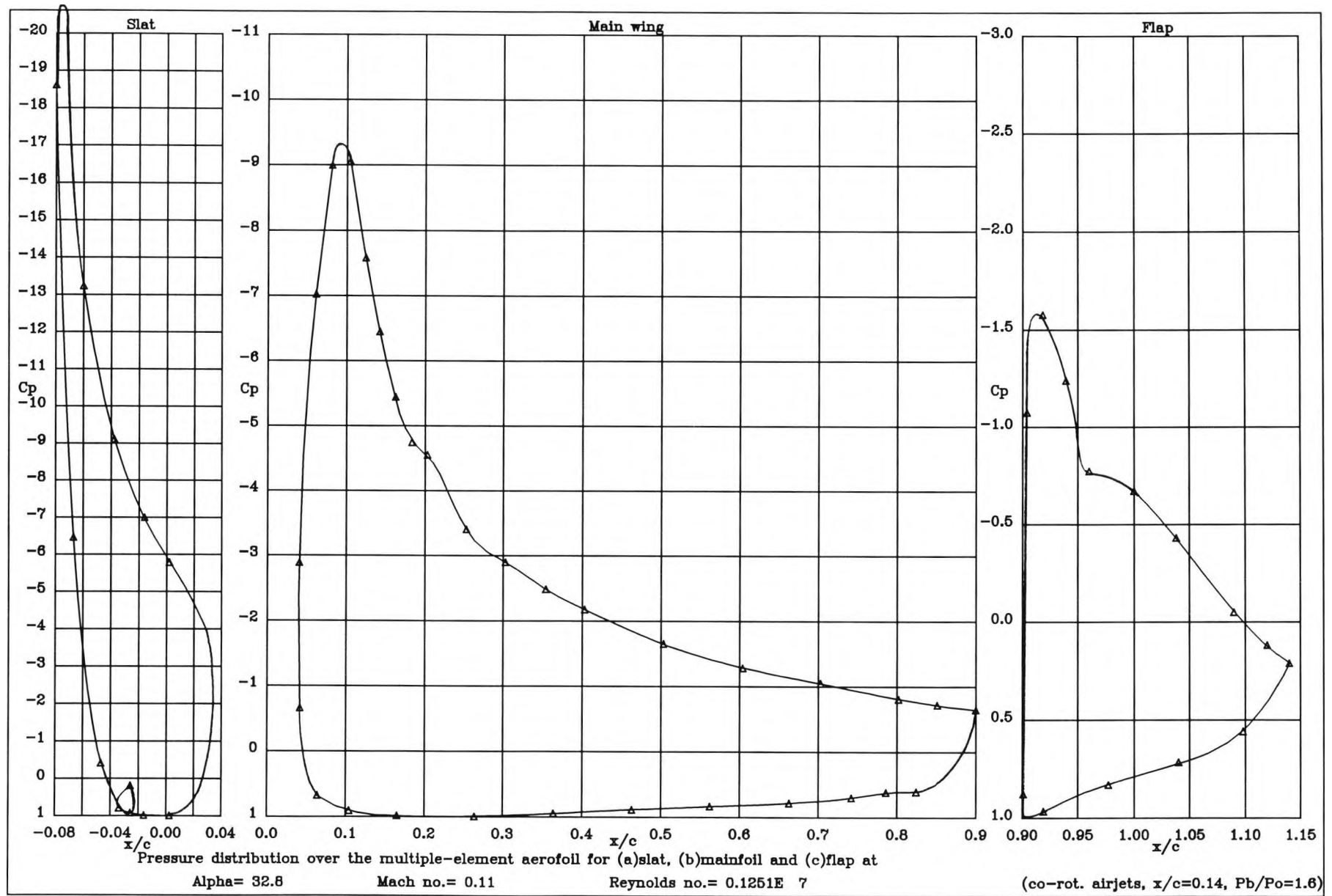
Figure 7.11 : Pressure distribution over the high lift system at 33^\circ when co-rot. airj's are at x/c = 0.14
