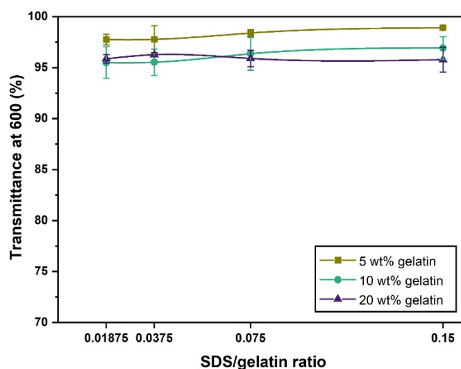
Figure 1. Transmittance (%) at 600 nm as a function of S/G ratio for 5, 10, and 20 wt.% hydrogels at their natural pH and 40 °C.
