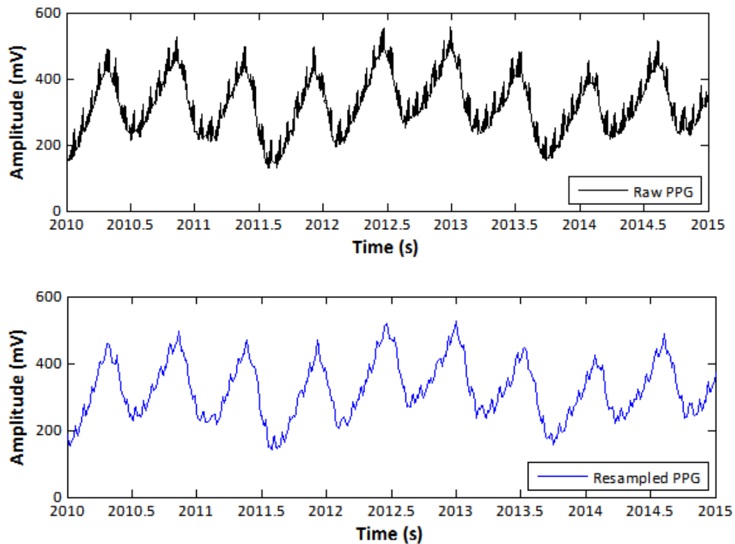
Figure 9.1: AC PPG signal re-sampling. The effect of the resample filter is to half the length of the signal vector and eliminate the high-frequency noise associated with F_s = 200 Hz (HF noise = F_s/2 ). The re-sampled signal (bottom plot) is notably smoother, the effect of anti-aliasing
