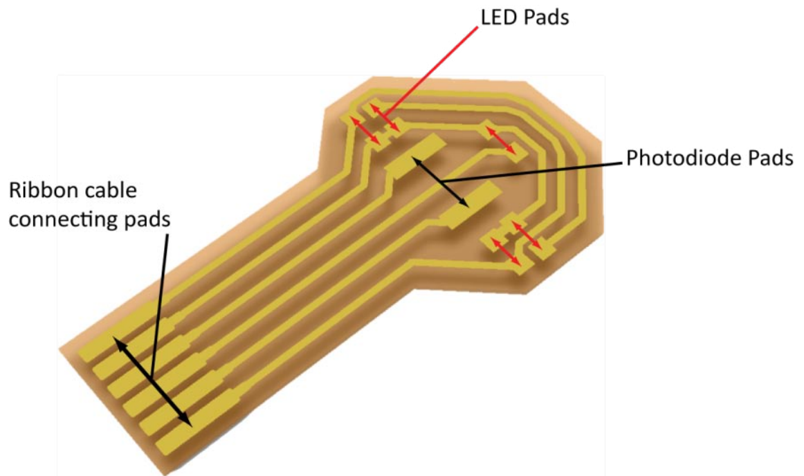
Figure 6.5: Three-dimensional concept of flexi-pcb layout for fontanelle sensor.
