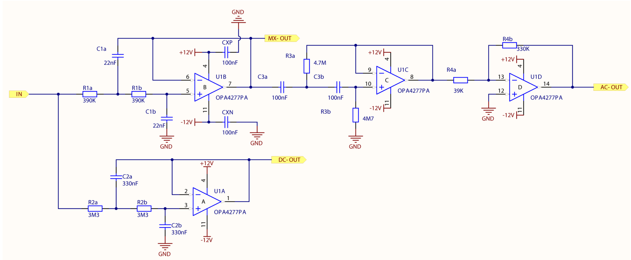
Filter Section
