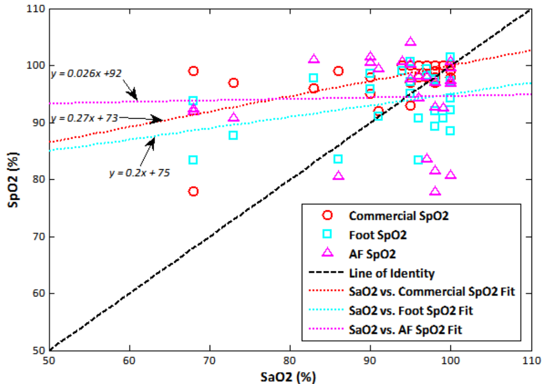
Figure 11.3: Linear regression scatter plot of blood gas analysis (x-axis) versus the various \text{SpO}_2 sensors (y-axis), n = 26 .
