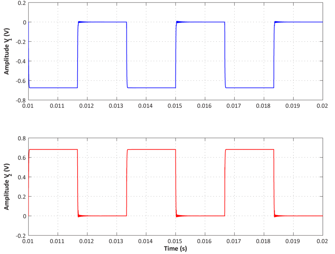
Figure 7.14: Simulated output of transimpedance amplifier stages, V_1 (top) and V_2 (bottom) C_d = 4 \text{ pF} , C_f = 10 \text{ pF} .
