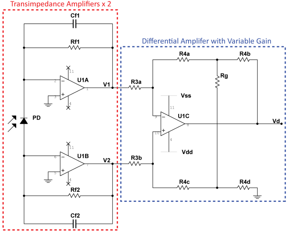
Figure 7.7: Preliminary dual transimpedance differential amplifier schematic.
