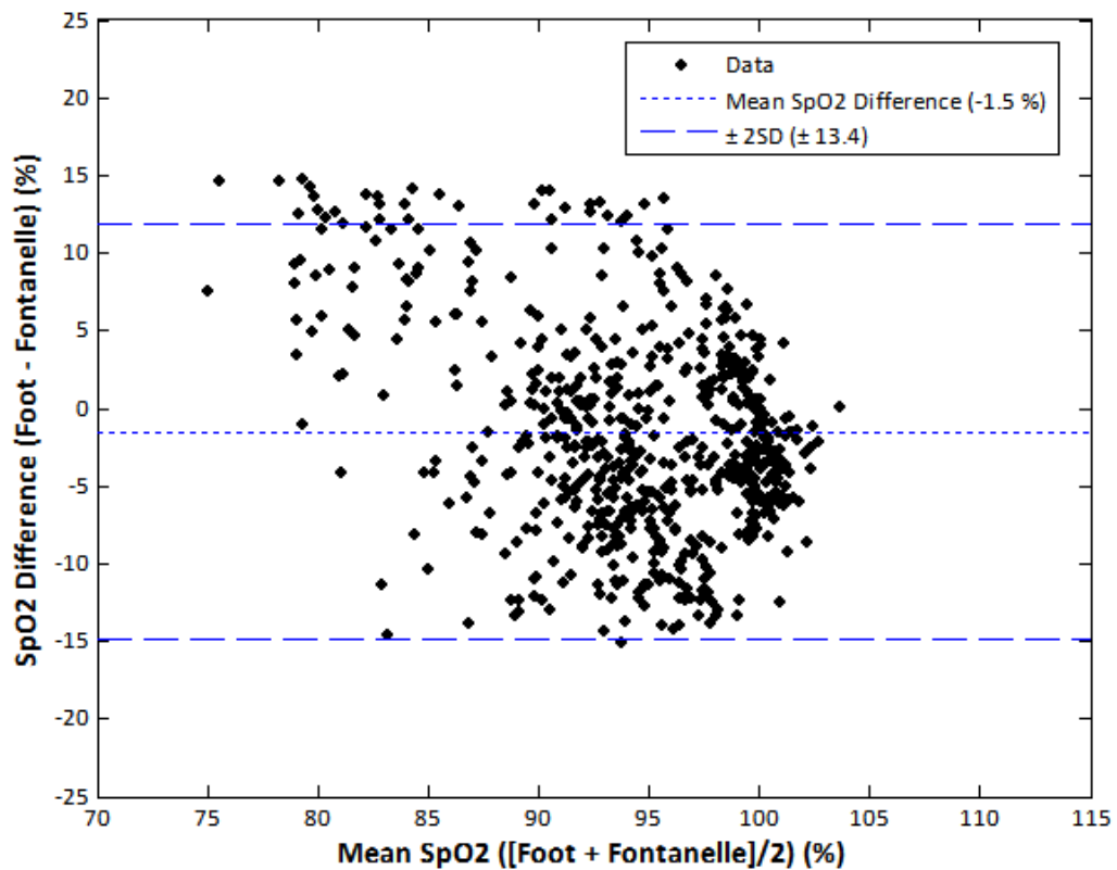
Figure 11.8: AF and foot \text{SpO}_2 /PPG sensor accuracy relative to each other.
